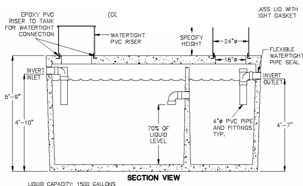
Figure 4-6 Diagram of typical precast concrete residential septic tank. (Adapted from Jensen Precast.)
