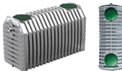
Figure 4-7 Views of the Premier Tech polyethylene septic tank. (Adapted from Premier Tech.)
