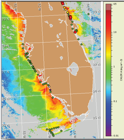
Fig. 4. A combination of satellite imagery (left), wind data, field samples, public health data, in situ currents, and an ecological model are used to determine HAB location and extent and to forecast the transport and likely impacts at the beach over several days. In this figure, green dots indicate field samples with low abundance and red dots indicate samples with high abundance of HAB cells.
