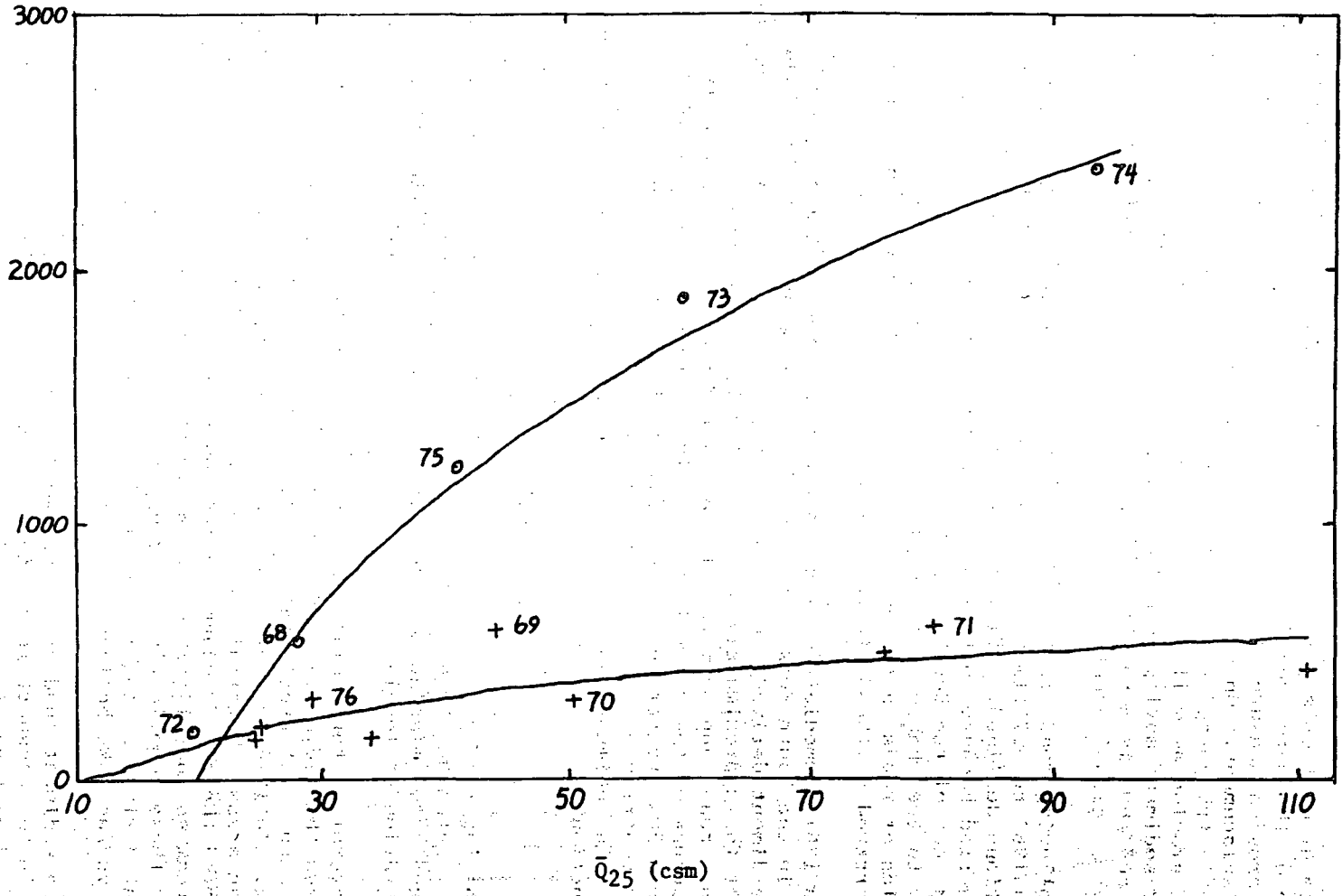
Figure 3. Sediment Discharge of South Fork of Caspar Creek as a function \bar{Q}_{25} (the mean discharge of the flow volume). (Rice, et. al., 1978)
