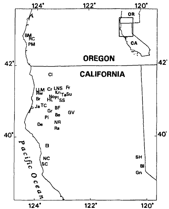
Figure 3. Location of study reaches. Abbreviations of channel names are defined in Table 1.
