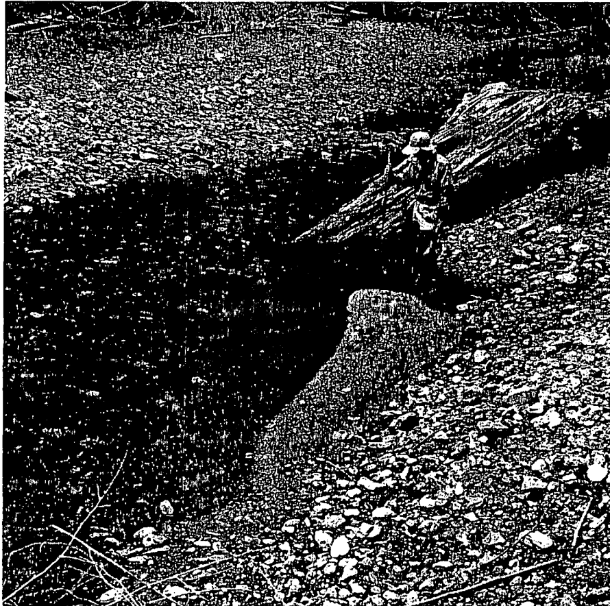
Figure 1. Deposit of fine bed material in a pool of Bridge Creek, northern California. Fine material occupies approximately 20% of the residual pool volume.
