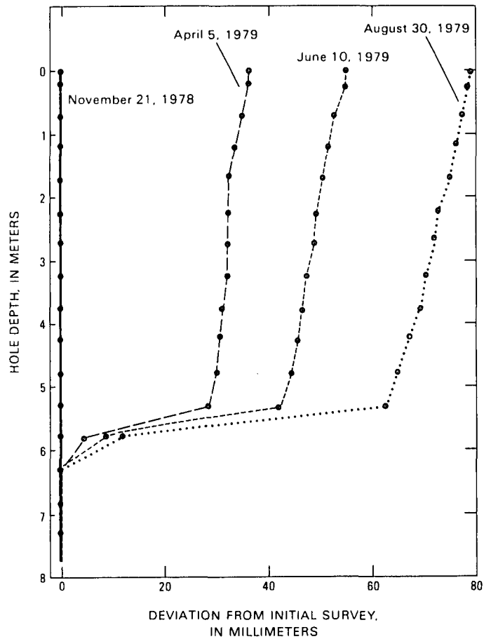
FIGURE 10.—Apparent deformation at inclinometer tube E, site 2. Deformation in tube after August 30, 1979, was too severe to allow penetration by inclinometer. Hole depth was 7.85 m. Data are from R. Ziemer, U.S. Forest Service, Arcata, Calif.
