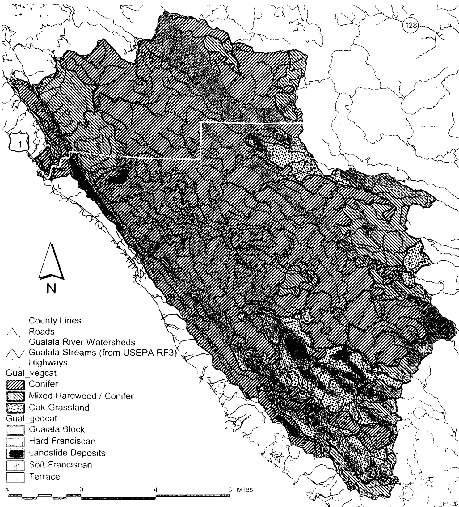
Plate 8. Geology-Vegetation Terrains of the Gualala River Watershed
