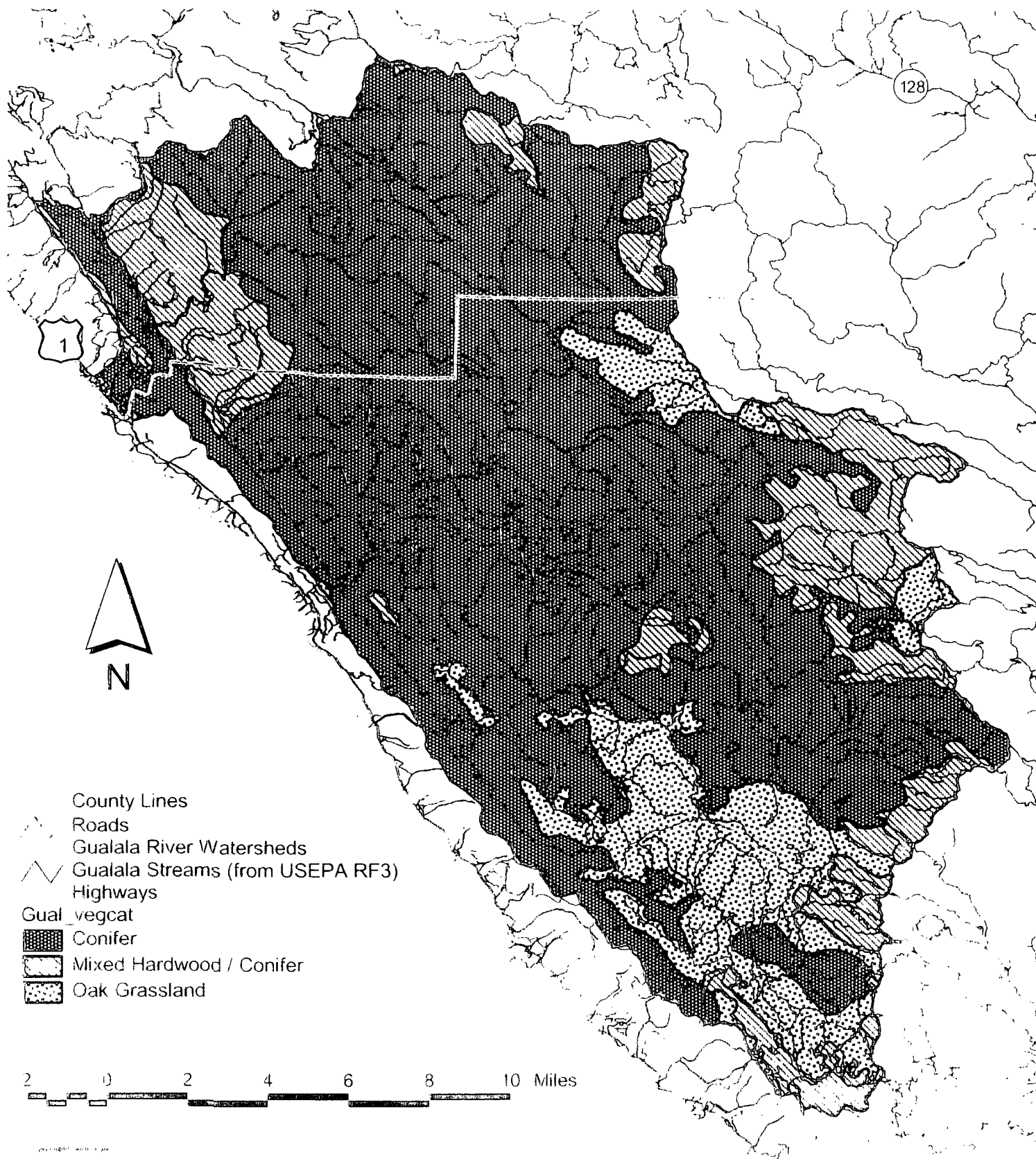
Plate 5. Vegetation of the Gualala River Watershed
