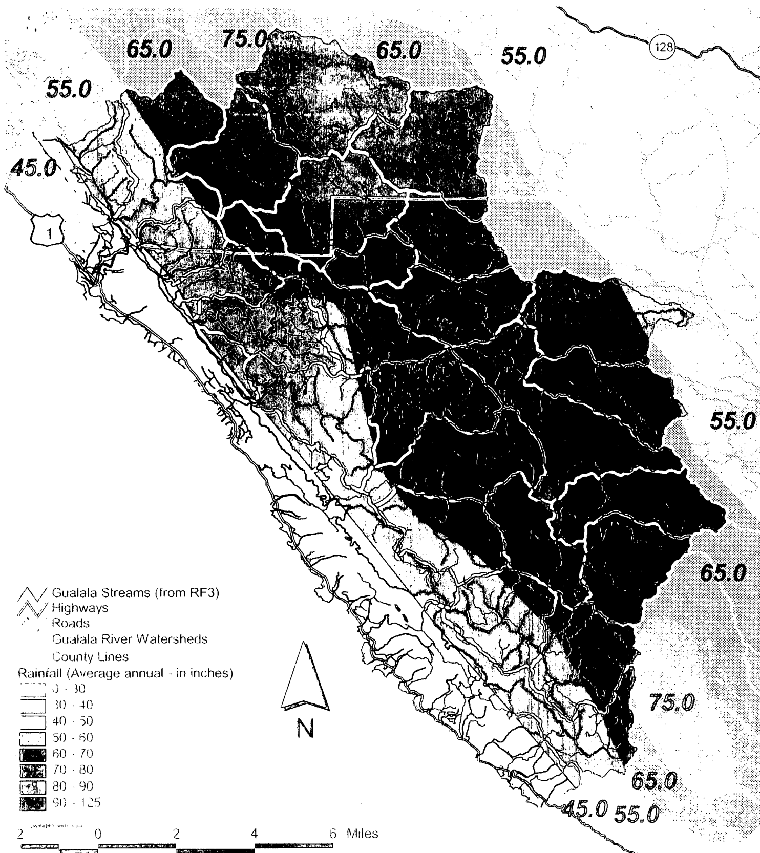
Plate 3. Precipitation in the Gualala River Watershed
