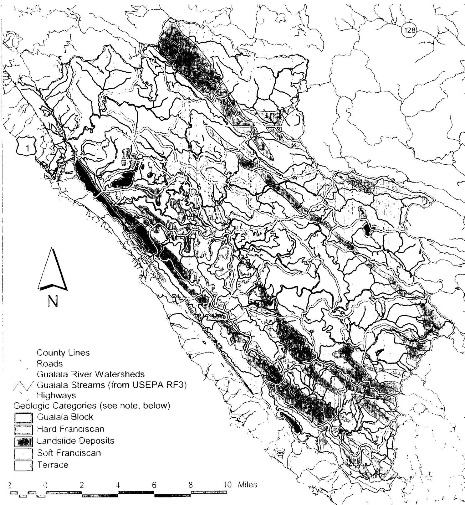
Plate 4. Geology of the Gualala River Watershed North Coast Regional Water Quality Control Board July 26, 2001
