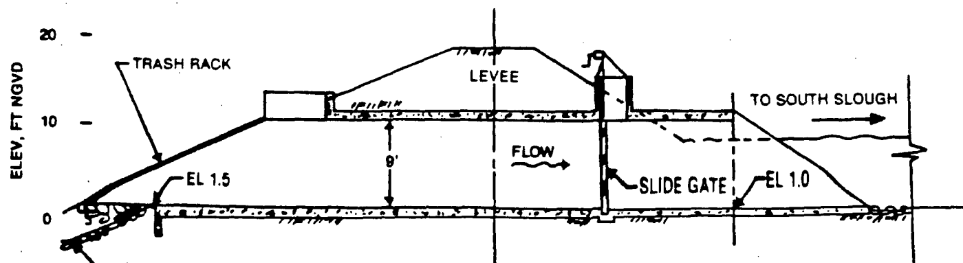
SECTION A-A SCALES: 1" = 20' HORIZ. 1" = 10' VERT.
