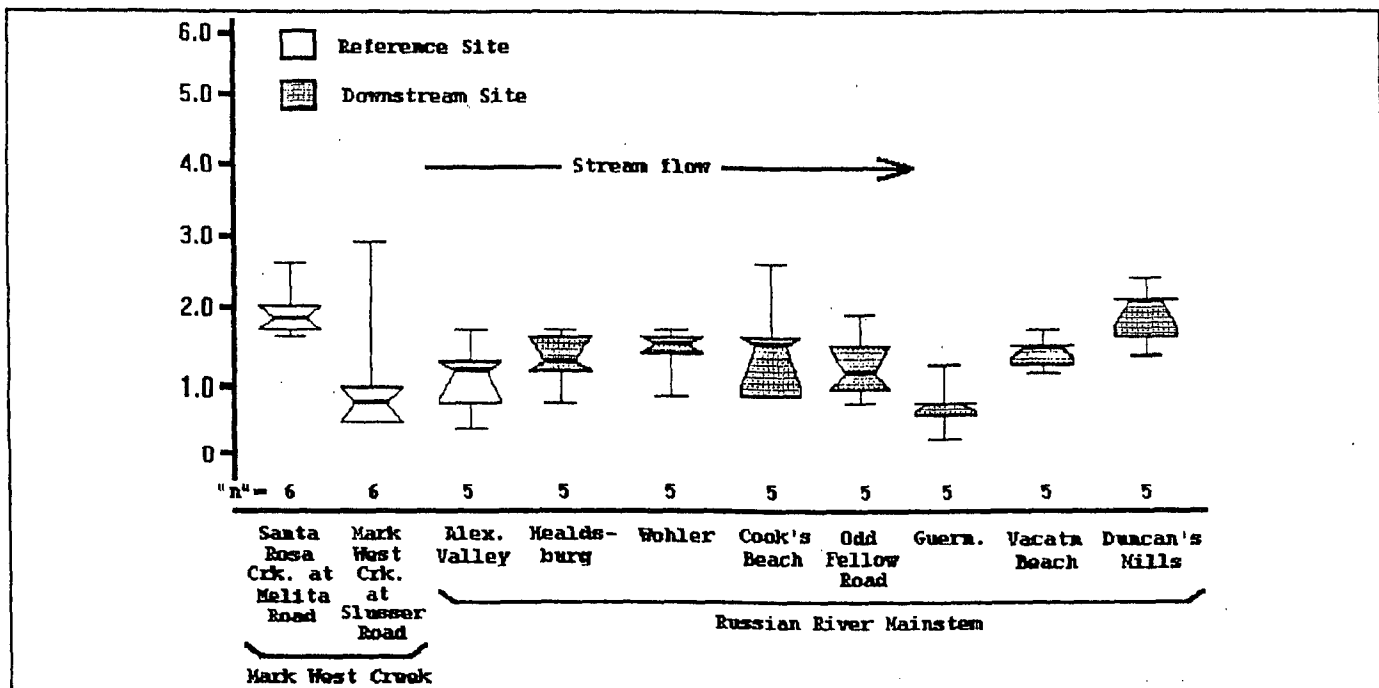
Figure 15. Sediment copper concentrations (mg/Kg) in the Russian River, 1985-86. Mark West Creek reference stations shown for comparison.
