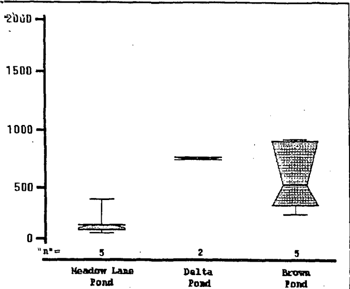
Figure 17. Total Kjeldahl nitrogen concentrations (mg N/Kg) in sediments of three wastewater ponds, 1985-86.
