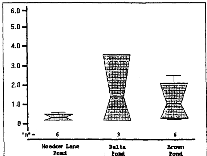
Figure 3. Sediment copper concentrations (mg/Kg) for the three wastewater ponds, 1985-86.
