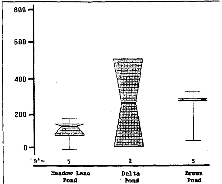
Figure 18. Total phosphate concentrations (mg P/Kg) in sediments of three wastewater ponds, 1985-86.
