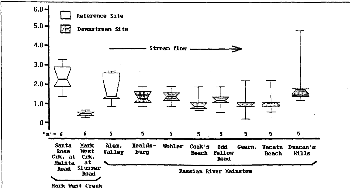
Figure 14. Sediment chromium concentrations (mg/Kg) in the Russian River, 1985-86. Mark West Creek reference stations shown for comparison.
