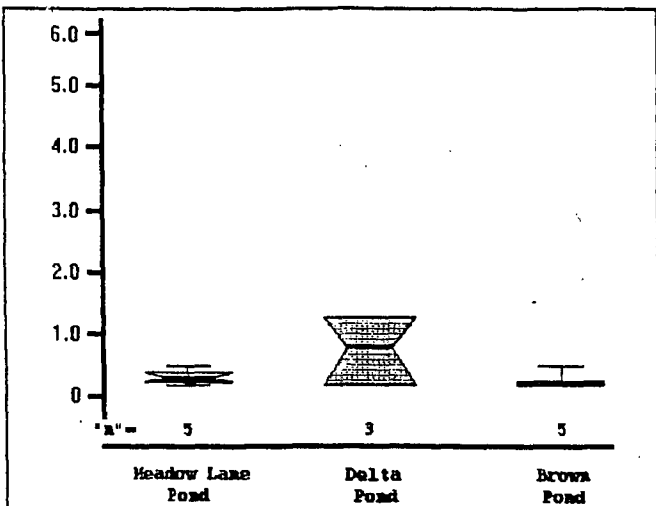
Figure 2. Sediment chromium concentrations (mg/Kg) for the three wastewater ponds, 1985-86.
