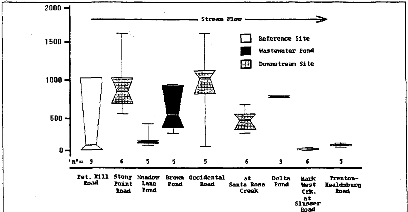
Figure 21. Total Kjeldahl nitrogen concentrations (mg N/Kg) in sediments in the Laguna/Mark West Creek system, 1985-86.
