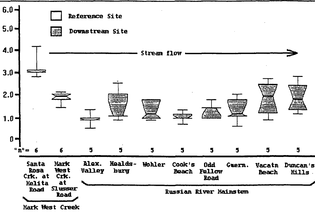
e 16. Sediment zinc concentrations (mg/Kg) in the Russian River, 1985-86. Mark West Creek reference stations shown for comparison.
