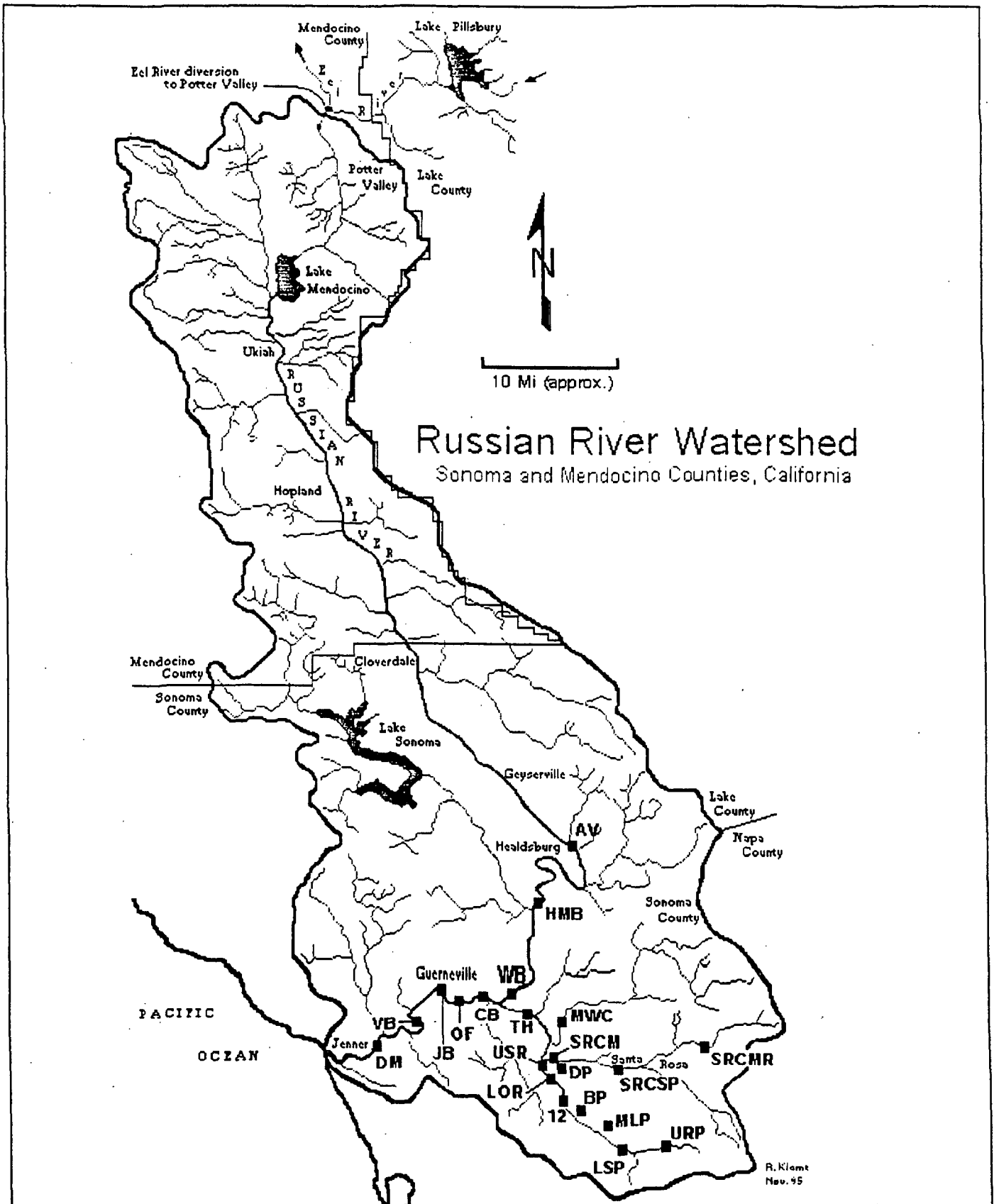
Figure 1. Sediment sampling sites in the Russian River and Mark West Creek systems, 1985-86 and 1995.
