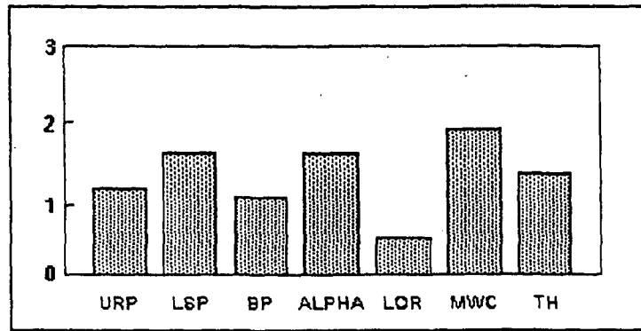
Figure 10A. Sediment concentrations (mg/Kg) for chromium (CR), zinc (Zn), copper (Cu), lead (Pb), and arsenic (As) in the Laguna de Santa Rosa, 1995. Please refer to Table 1 for station codes. Reference stations are: URP and MWC. Pond stations are: BP and ALPHA.
