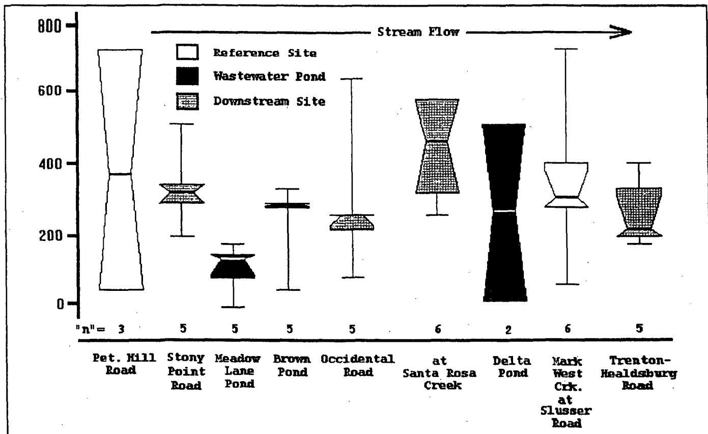
Figure 22. Total phosphate concentrations (mg P/Kg) in sediments in the Laguna/Mark West Creek system, 1985-86.
