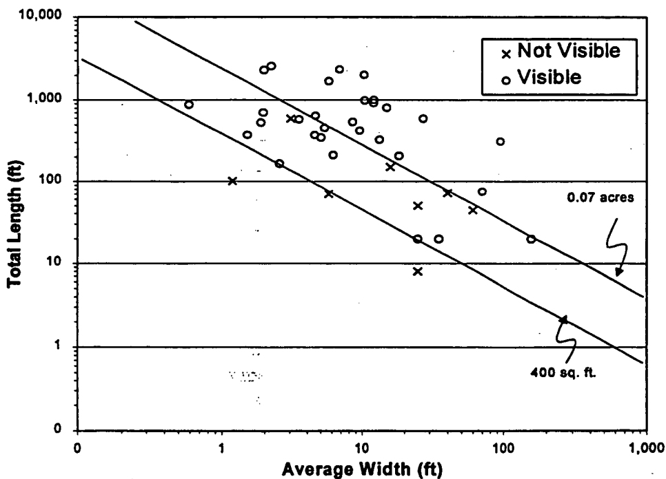
Figure 5. Visibility of road-related landslides (n=38) in 1:6,000 air-photos plotted by total length and width (both initial failure area and pre-channelized debris flow). All road-related landslides in Mapleton, Vida, and Tillamook within the area covered by the air photo surveys are included here.
