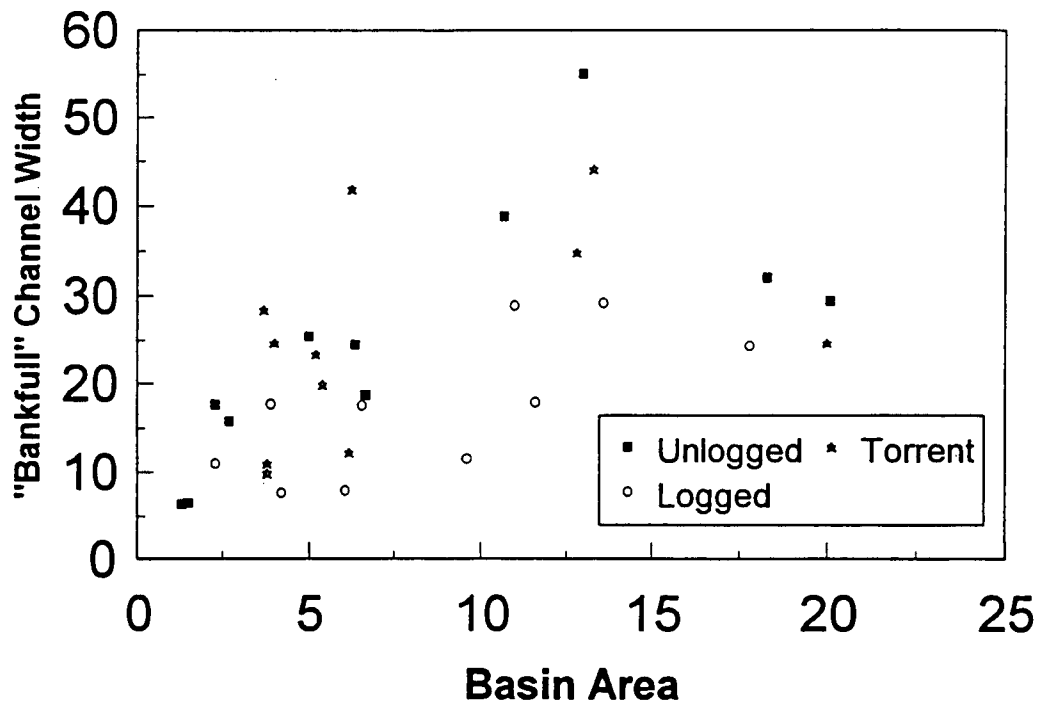
Figure 48. Bankfull channel width for several unlogged, logged and debris torrent impacted reaches in British Columbia (from Tripp and Poulin, 1992).
