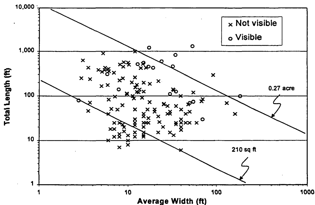
Figure 3. Visibility of non-road-associated landslides (n=143) in 1:6,000 air-photos plotted by total length and width (both initial failure area and debris flow). All non-road-related landslides in Mapleton, Vida, and Tillamook within the area covered by the air photo surveys in 30+ year-old forests are included here.
