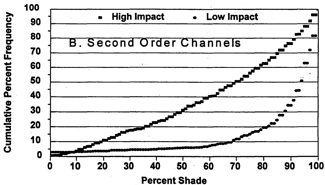
Figure 51. Cumulative frequency distribution for percent shade for first and second order streams that were highly impacted by debris torrents and dam-break floods associated with the storms of 1996 compared with streams that had little or no impacts.
