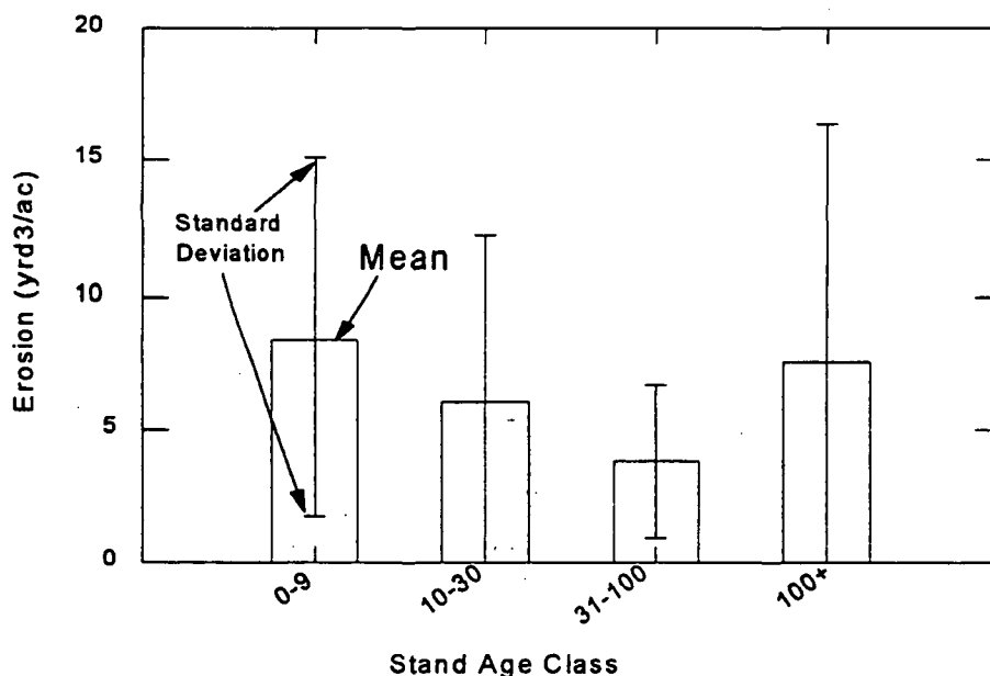
Figure 27. Bar graph showing distribution in erosion of the four multi-stand-age red zone study areas by age class.
