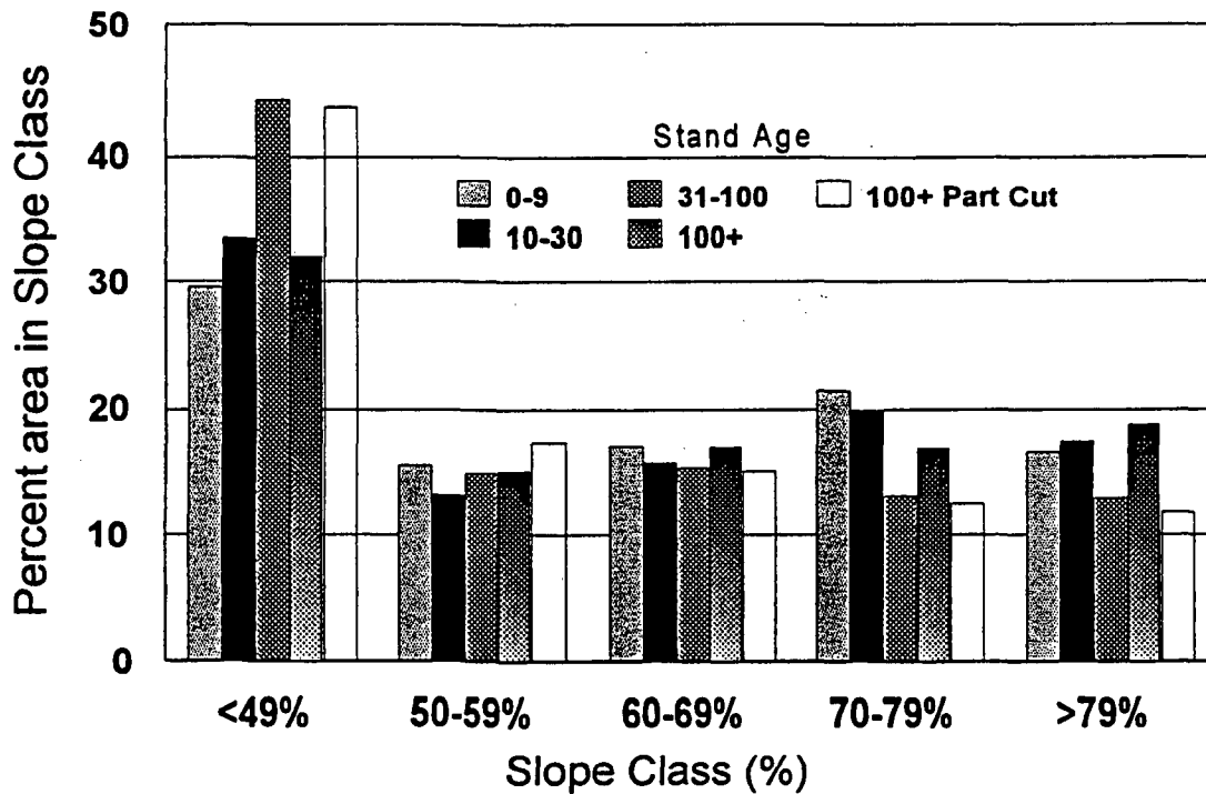
Figure 23. Slope steepness distribution by age class in the Elk Creek study area based on 6 meter DEM GIS coverage.
