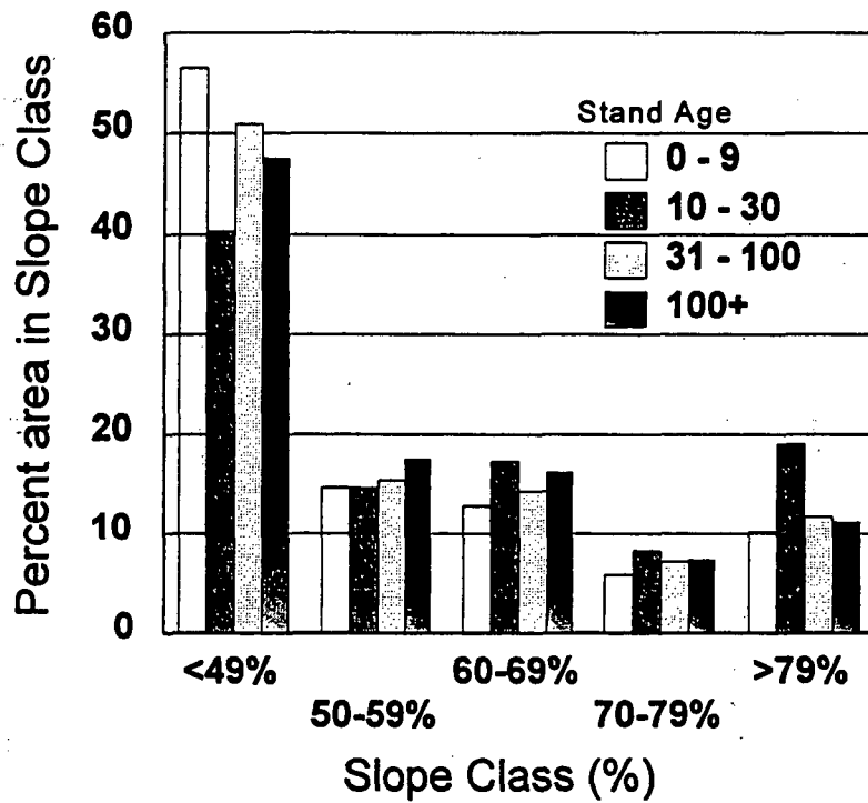
Figure 25. Slope steepness distribution by stand age class in the Mapleton study area based on 10 meter DEM GIS coverage.
