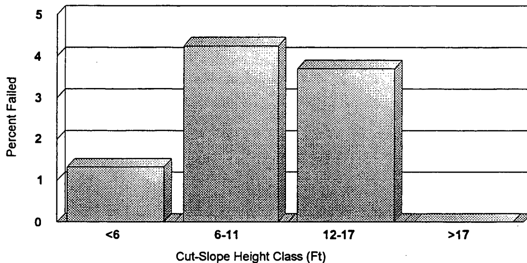
Figure 42. Fill failure rate by cutslope height for roads on steep slopes (over 50%) at locations without drainage discharge.
