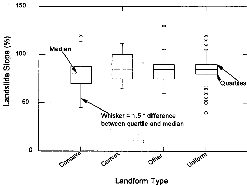
Figure 17. Graphic comparison of slope steepness distributions by landform for landslides in the three Tye red zone study areas. AOV tests were conducted on both of these sets of distributions. In both of these cases, there was no significant difference in slope steepness between any of the individual landforms.
