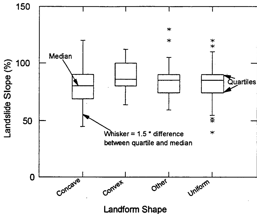
Figure 16. Graphical comparison of slope steepness distributions by landform type for up-slope landslides for all study areas. (A quartile includes 25 percent of the data.) There is a significant difference between the slope steepness of the concave and convex slopes, with an Analysis of Variance (AOV) p value equal to 0.008.
