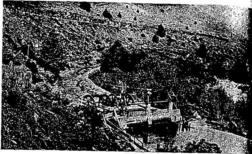
FIG. 42. A rotary fish screen which hinders the passage of small fish into a diversion.
