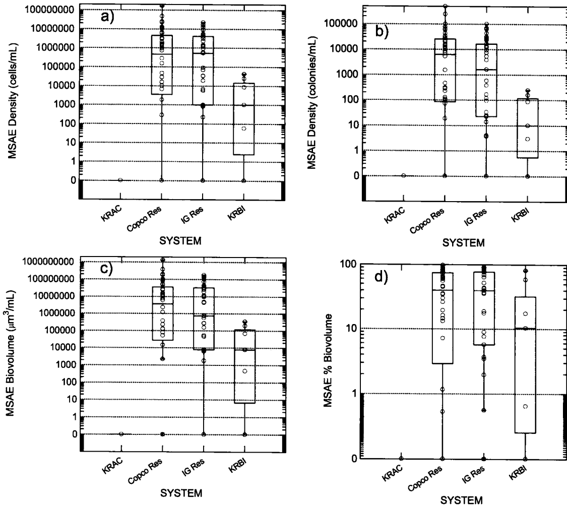
Figure 10. Karuk Tribe/SWRB MSAE cell density (a), colony density (b), biovolume (c), and % biovolume (d) in the Klamath River and Copco and Irongate Reservoirs, July-October 2005.
