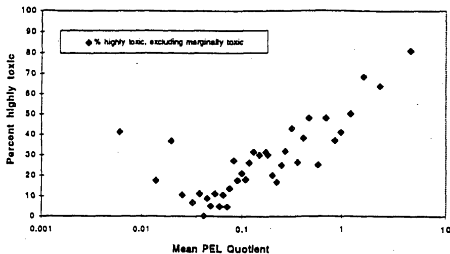
Fig. 2. The relationship between the incidence of toxicity in amphipod survival tests and mean probable effects level (PEL) quotients (plotted as the medians of 39 quotient intervals, each consisting of 25 samples).
