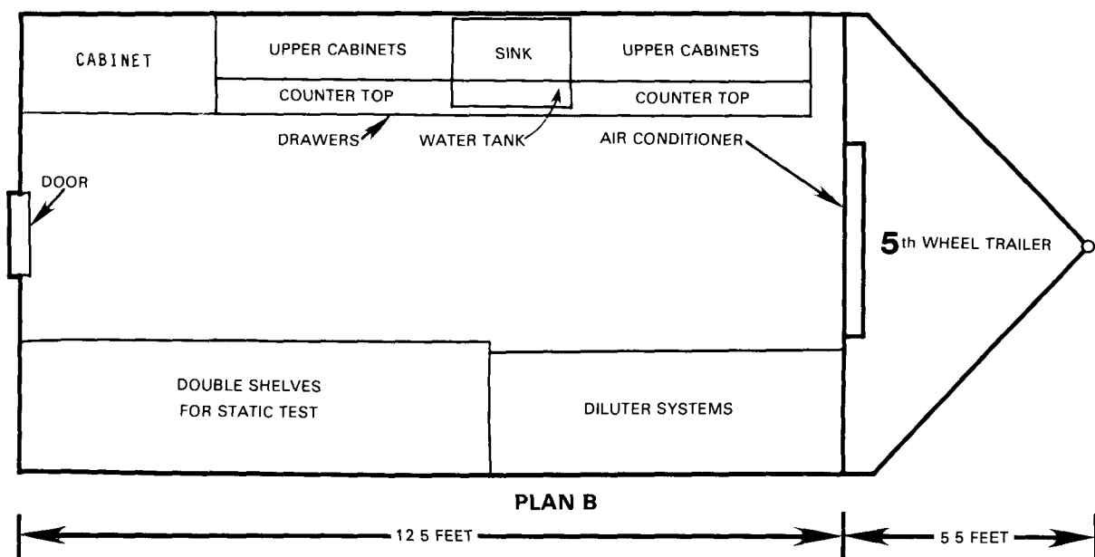
Figure 4. Mobile bioassay trailer, fifth-wheel trailer, internal view from above.
