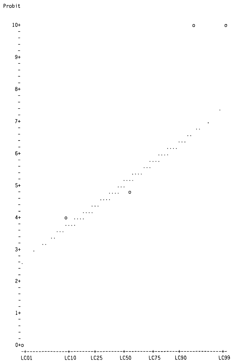
Figure 12. Plot of adjusted Probits and predicted regression line.
