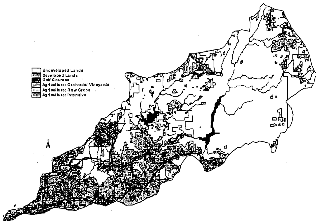
Figure 2. Watershed map of site SDR-1 showing the distribution of major land use categories in the watershed.
