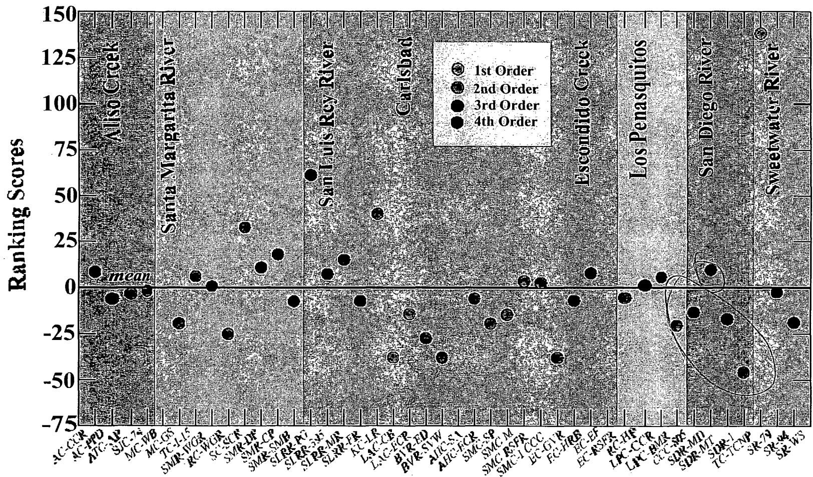
Figure 3d. BMI ranking scores for macroinvertebrate monitoring sites sampled in May 99 for the San Diego Regional Bioassessment Monitoring Project.
