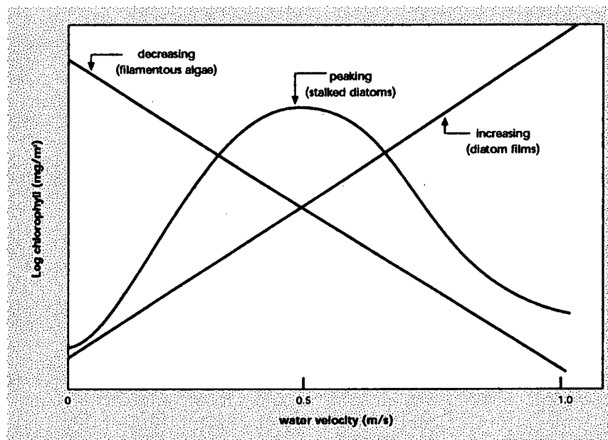
Figure 17: Three main community biomass responses to spatial variations in water velocity in streams.
