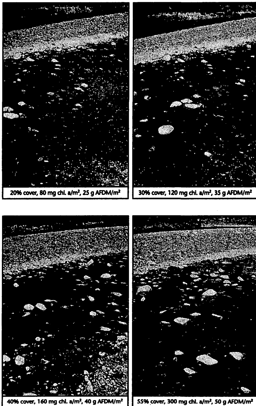
Figure 28: Gradient in percentage cover and biomass of filamentous algae, Waipara River, North Canterbury.
