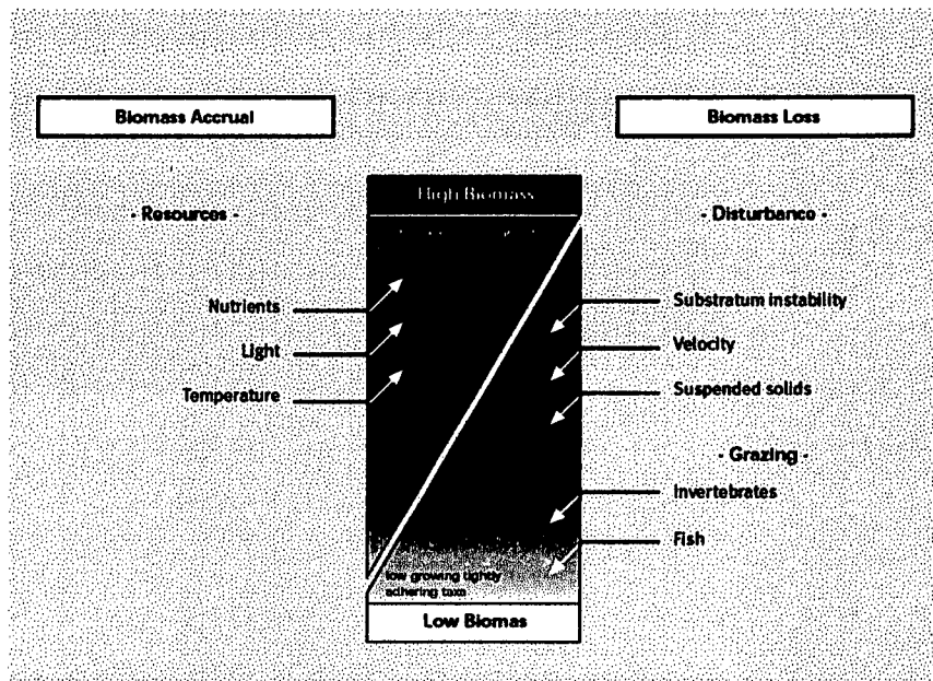
Figure 8: Summary of the counteracting processes of periphyton biomass accrual and biomass loss, and the principal local factors contributing to these processes, in a stream. Triangles in the central rectangle show relative balance of "biomass accrual" and "biomass loss". The growth form of the communities likely to dominate each end of the accrual – loss gradient is also shown (reproduced from Biggs, 1996a with permission from Academic Press).
