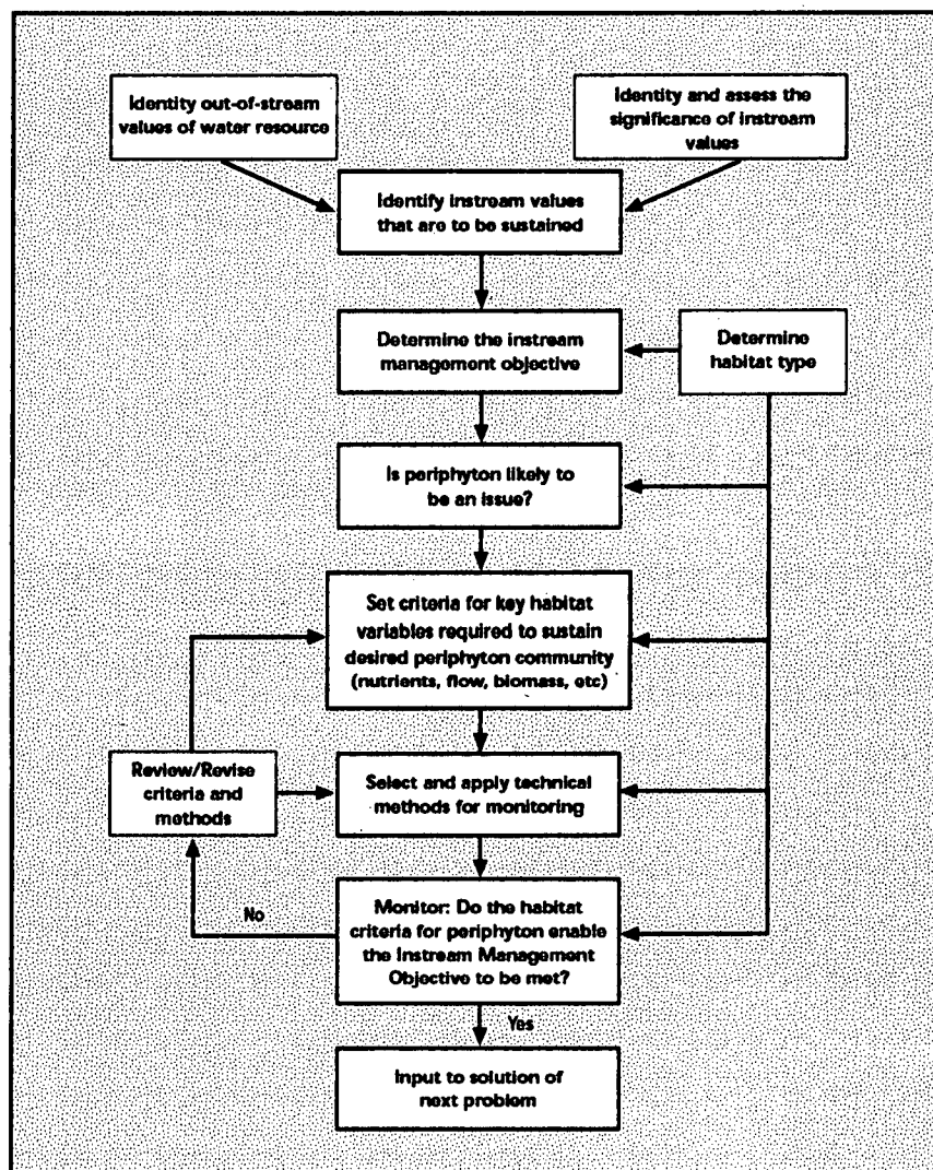
Figure 2: General procedures for planning, setting consent criteria and verifying appropriateness of consent criteria for managing instream values in relation to periphyton (based on Figure 9 of the Flow Guidelines for Instream Values (MfE, 1998)).
