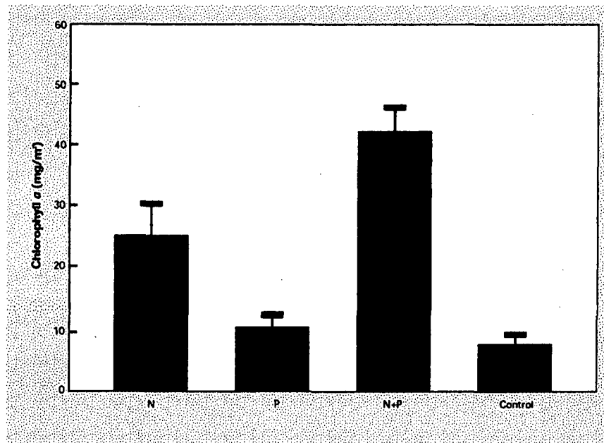
Figure 26: Example of the results of a nutrient diffusing substrate experiment in a hill country river (Kauru River, Otago). Vertical bars denote standard errors.
