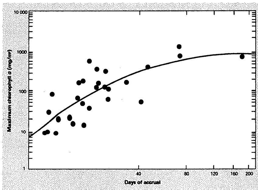
Figure 14: Maximum chlorophyll a concentrations as a function of mean days of accrual in 30 New Zealand rivers sampled every 2–4 weeks for at least 13 months (modified from Biggs, 2000 with permission from the Journal of the North American Benthological Society ).
