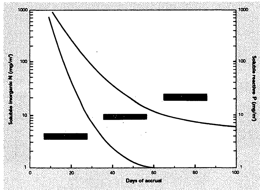
Figure 30: Nomograph of mean monthly soluble nutrient concentrations that are predicted to result in maximum benthic algal biomass indicative of oligotrophic, mesotrophic, and eutrophic conditions for varying days of accrual ( d_p ) in gravel/cobble-bed streams. The oligotrophic – mesotrophic boundary was set at 60 mg/m 2 chlorophyll a and the mesotrophic – eutrophic boundary was set at 200 mg/m 2 chlorophyll a (after Dodds et al. 1998). These boundaries approximate the maximum biomass criteria adopted for the protection of benthic biodiversity (oligo- to mesotrophic), aesthetics, and trout fishery values (meso- to eutrophic) (see Table 14 page 102). The lines delineating the trophic boundaries were calculated using the soluble inorganic N (SIN) equation on page 43. However, these lines also approximate boundaries for P-limited communities by reference to the right-hand scale, which has been set at 0.1 x the SIN scale, because the mean ratio of biomass from the SIN and soluble reactive P (SRP) models was 10.8. The left-hand (SIN) axis is used for nitrogen limited communities and the right-hand axis (SRP) is used for phosphorus limited communities.
