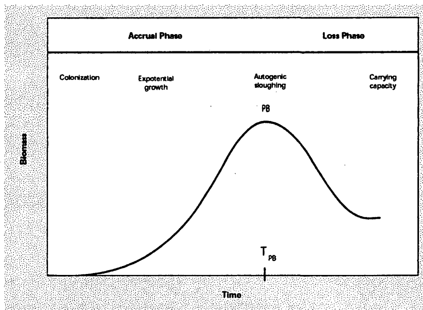
Figure 9: An idealised short-term periphyton accrual cycle after major flooding. PB (peak biomass) = maximum accrual cycle biomass; T_{PB} = time to PB from commencement of colonisation (reproduced from Biggs, 1996a with permission from Academic Press).
