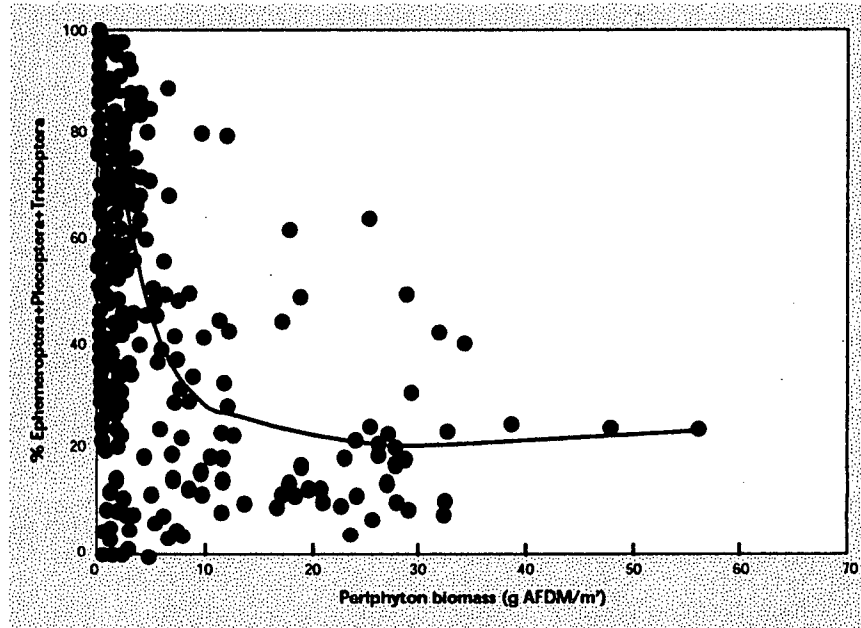
Figure 29: Relative abundance of "clean water" EPT invertebrates (Ephemeroptera (mayflies), Plecoptera (stoneflies), Trichoptera (caddisflies)) as a function of the ash-free dry mass of periphyton in the samples. The line of "best-fit" was determined using distance-weighted least squares regression. Most periphyton samples were dominated by diatoms ( Gomphonopsis , Cymbella , Synedra ) and filamentous cyanobacteria ( Phormidium ).
