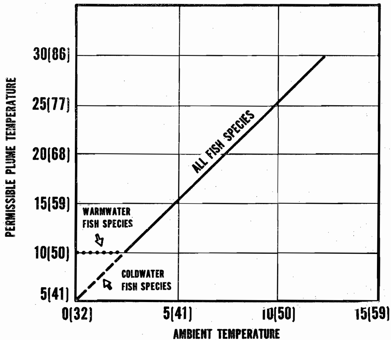
FIGURE 2. GRAPH TO ESTIMATE THE MAXIMUM WEEKLY AVERAGE TEMPERATURE OF PLOMES FOR VARIOUS AMBIENT TEMPERATURES, °C (°F)
