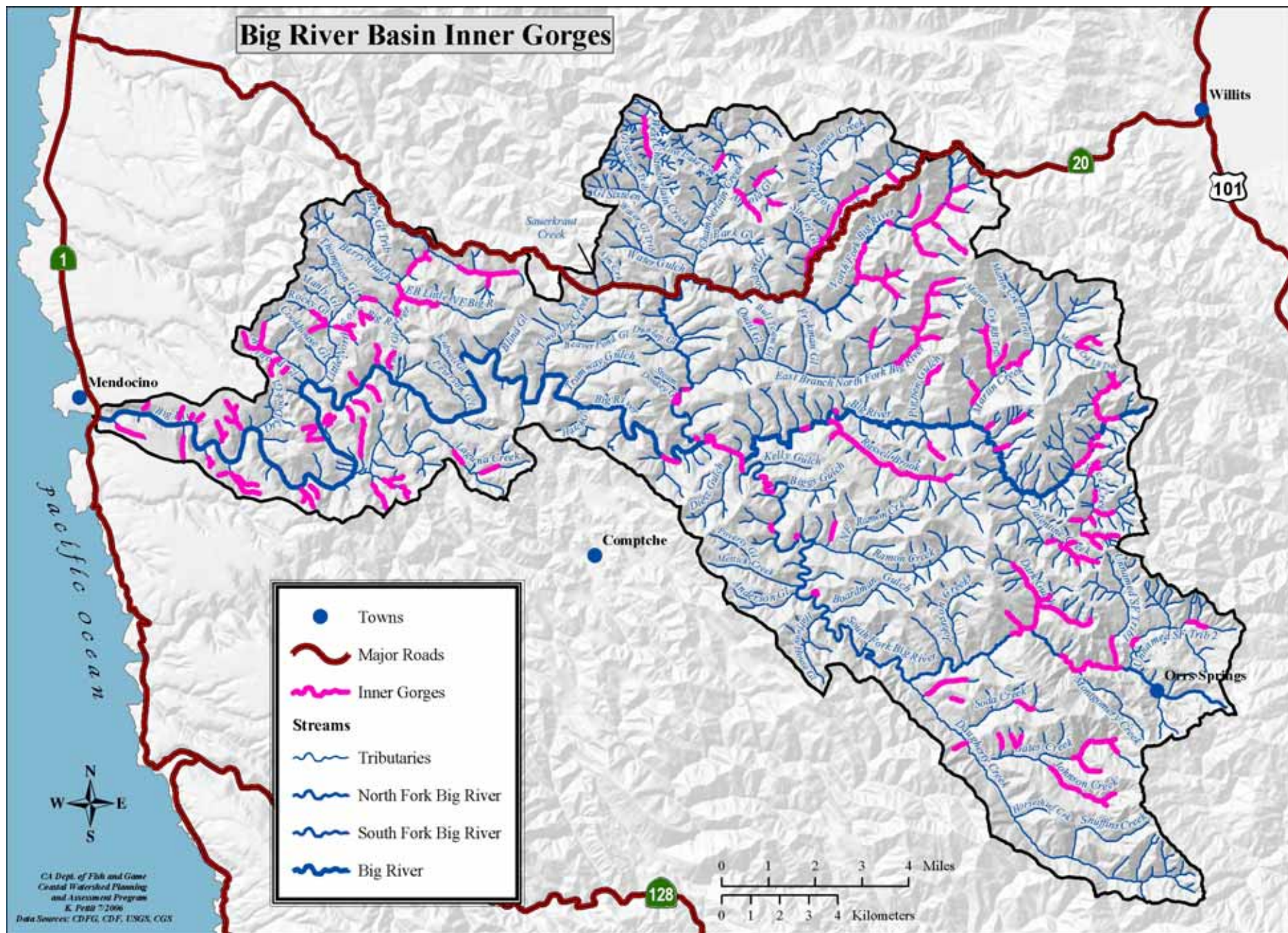
Figure 23. Inner gorges in the Big River Basin (CGS 2005).
