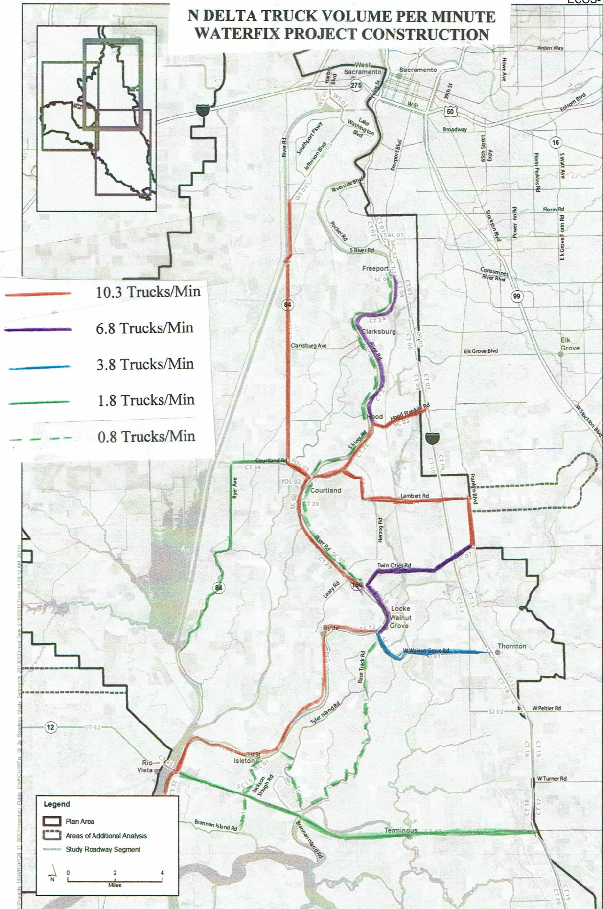
Figure 19-2a Roadway Segments
