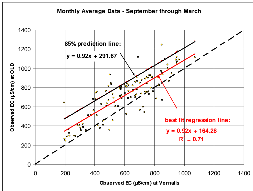
Figure 4.11. Monthly Average Salinity Data for September through March from 1993 through 2009 for Old River at Tracy (OLD) Plotted Against Corresponding Salinity Data at SJR near Vernalis, with Best Fit Regression and 85% Prediction Lines
