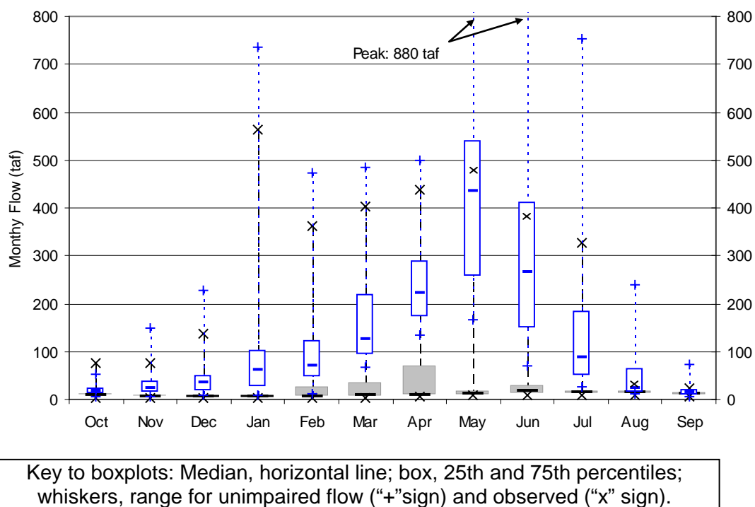
Figure 2.13. Monthly Unimpaired Flow (Open Bars) and Observed Flow (Filled Bars) in the SJR at Friant from 1984 to 2009
