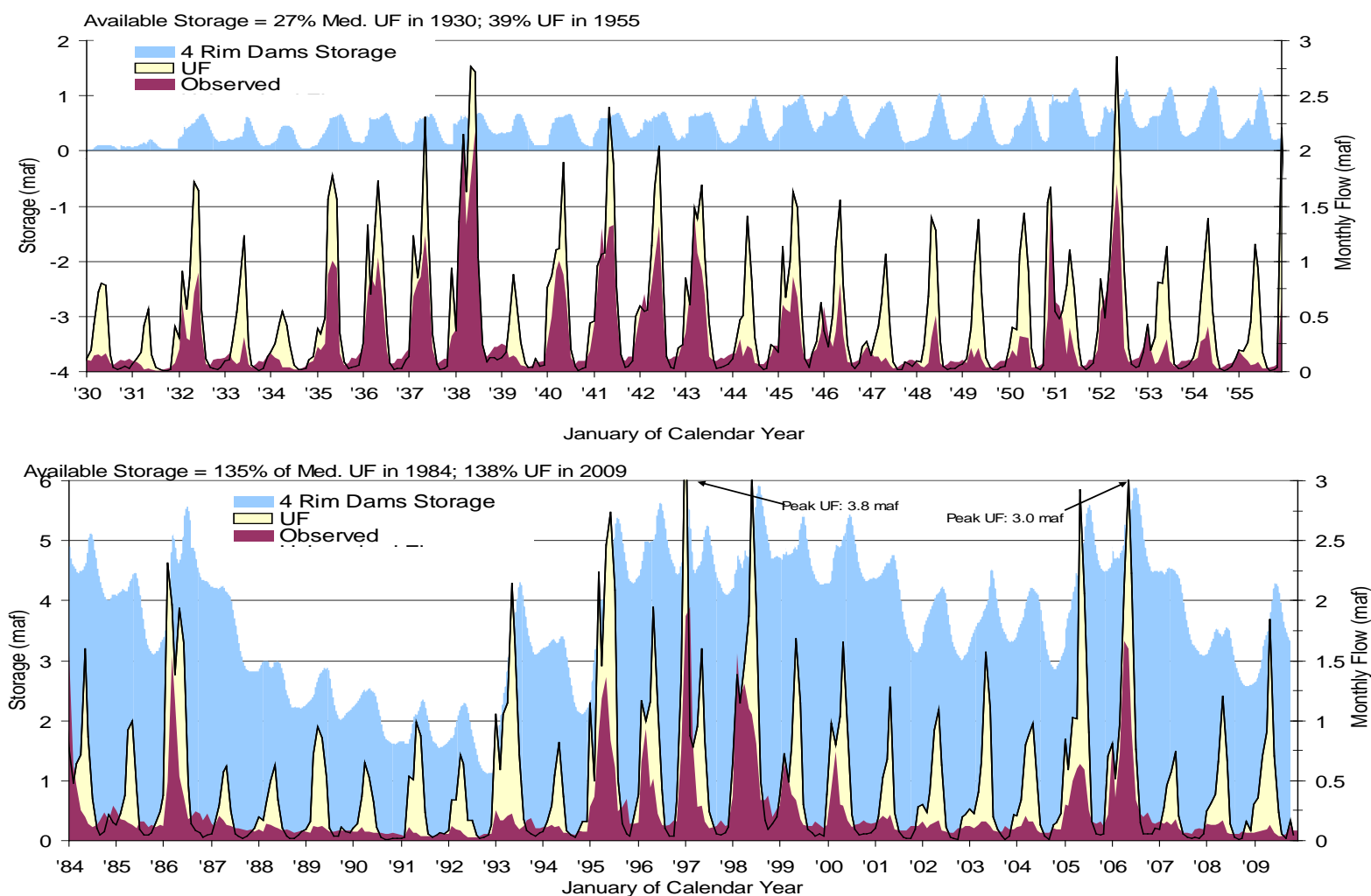
Figure 2.4. Monthly Unimpaired and Observed Flow in the San Joaquin River at Vernalis and Total Storage Behind New Melones, New Don Pedro, New Exchequer, and Friant Dams for Two Periods in Time (1930 to 1955 and 1984 to 2009)
