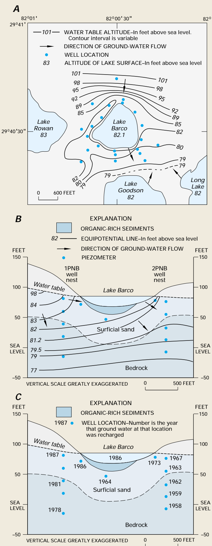
Figure L-2. Lake Barco, in northern Florida, is a flow-through lake with respect to ground water (A and B). The dates that ground water in different parts of the ground-water system was recharged indicate how long it takes water to move from the lake or water table to a given depth (C). (Modified from Katz, B.G., Lee, T.M., Plummer, L.N., and Busenberg, E., 1995, Chemical evolution of groundwater near a sinkhole lake, northern Florida, 1. Flow patterns, age of groundwater, and influence of lake water leakage: Water Resources Research , v. 31, no. 6, p. 1549–1564.)
