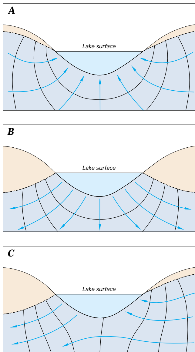
Figure 16. Lakes can receive ground-water inflow (A), lose water as seepage to ground water (B), or both
