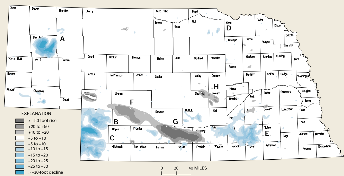
Figure N-2. The use of both ground water and surface water for irrigation in Nebraska has resulted in significant rises and declines of ground-water levels in different parts of the State. (Map provided by the University of Nebraska, Conservation and Survey Division.)
