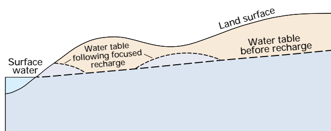
Figure 6. Ground-water recharge commonly is focused initially where the unsaturated zone is relatively thin at the edges of surface-water bodies and beneath depressions in the land surface.
