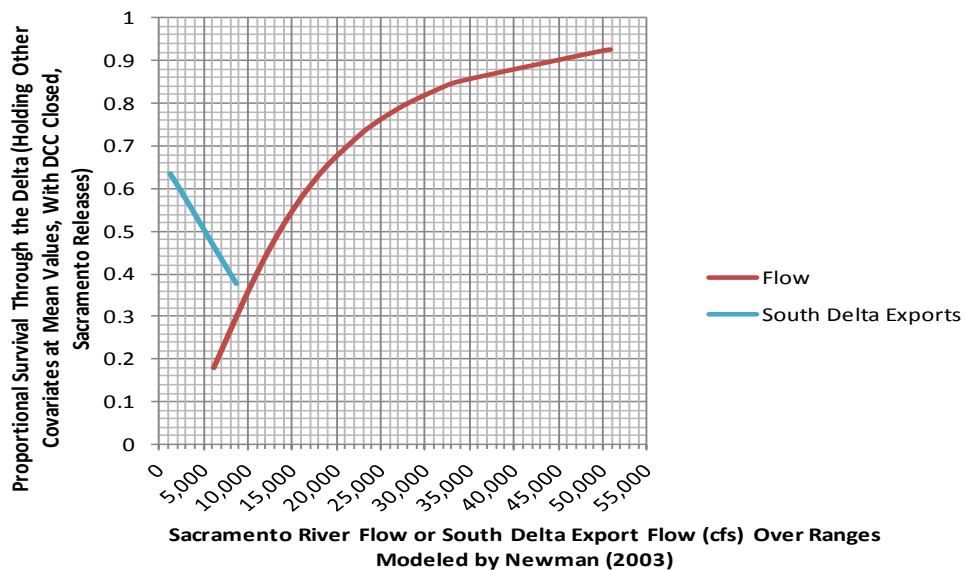
Figure 2. December 2012 BDCP Figure C.4-11: Effect varying Sacramento River flow and south Delta exports across the range of data modeled by Newman (2003), holding other covariates at mean values, assuming closed Delta Cross Channel gates, and fish releases from Sacramento.
