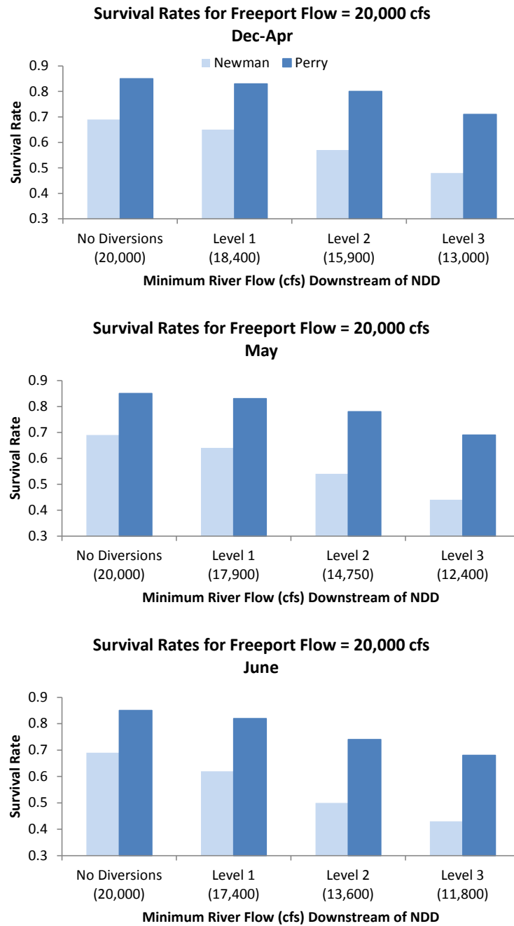
Figure 3. Perry (2010) and Newman (2003) survival rates for flows resulting after withdrawal at different north Delta bypass pumping levels.
