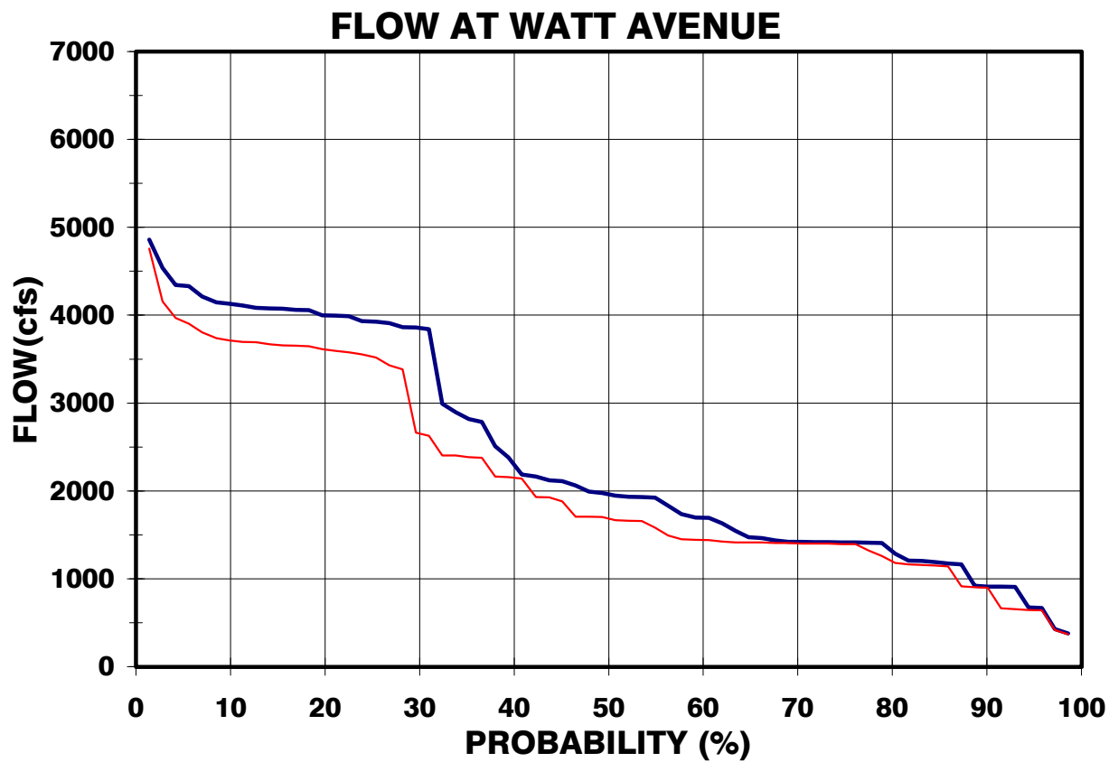
Figure 4.5-21. Probability that mean September flow in the Lower American River would exceed specified levels at Nimbus Dam and Watt Avenue.
