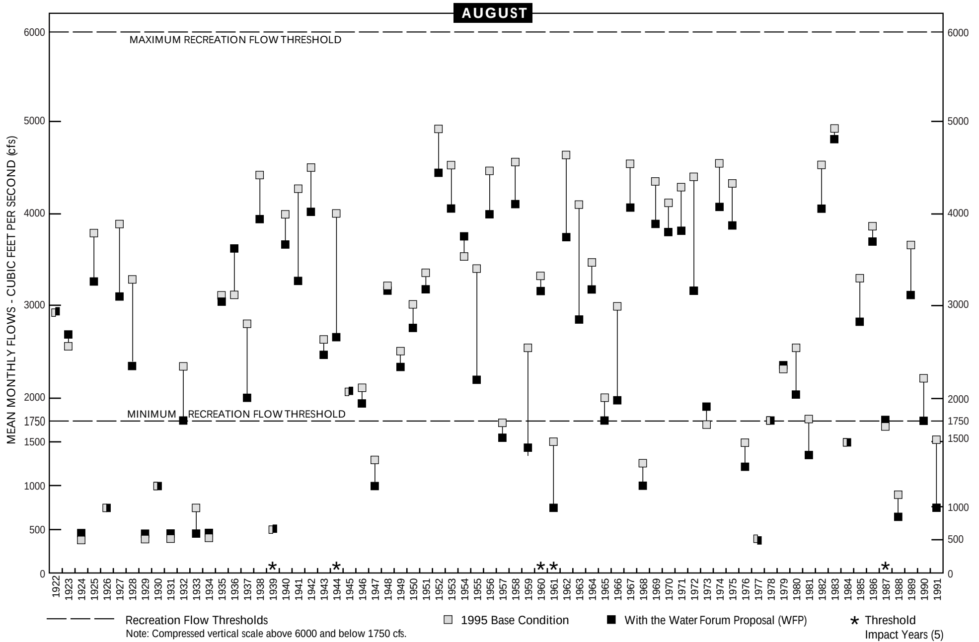
Lower American River Flows Compared to Recreation Thresholds in August
