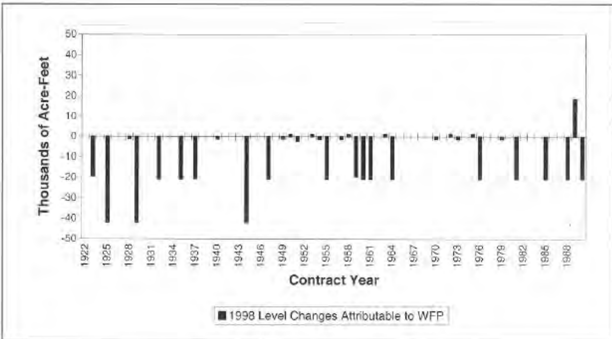
WFP Impact on Non-American River CVP Agricultural Deliveries North of Delta
