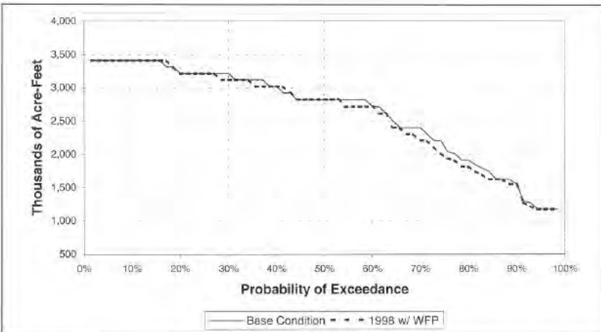
Total CVP Deliveries South of Delta
