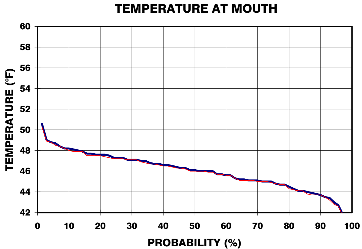
Figure 4.5-9. Probability that mean January temperature in the Lower American River would exceed specified levels at Nimbus Dam and at the Mouth.
