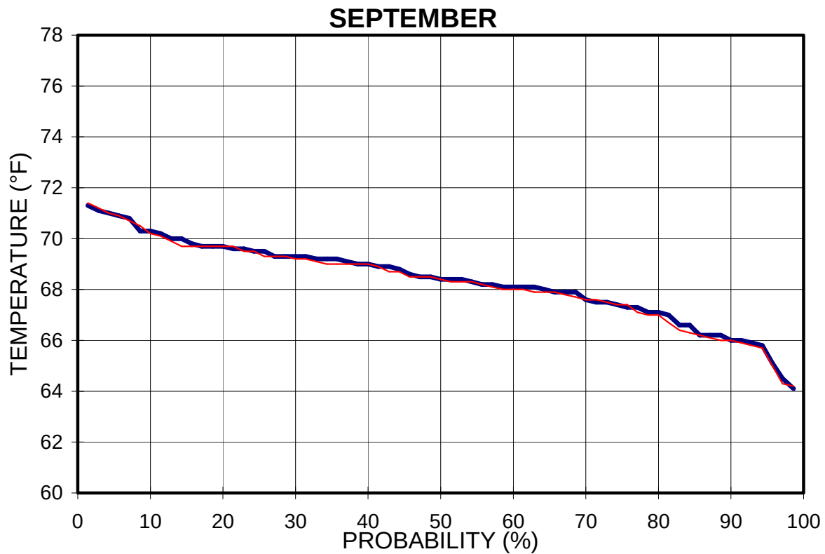
Figure 4.5-26. Probability that mean August and September temperatures in the Lower Sacramento River would exceed specified levels at Freeport.
