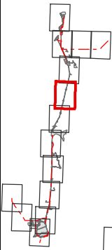
Figure M3-4: Sheet 6 of 15 Modified Pipeline/Tunnel Alignment (Alternative 4)
