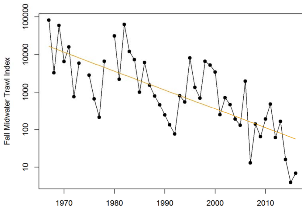
Figure 3.5-1. Inter-Year Trend in the FMWT Index for Longfin Smelt (1967 to 2016). The solid orange line is the least squares linear regression of the logarithm of the FMWT index against years. The slope of the regression differs significantly from zero ( R^2=0.51 ; P<0.001 , two-sided t-test).
