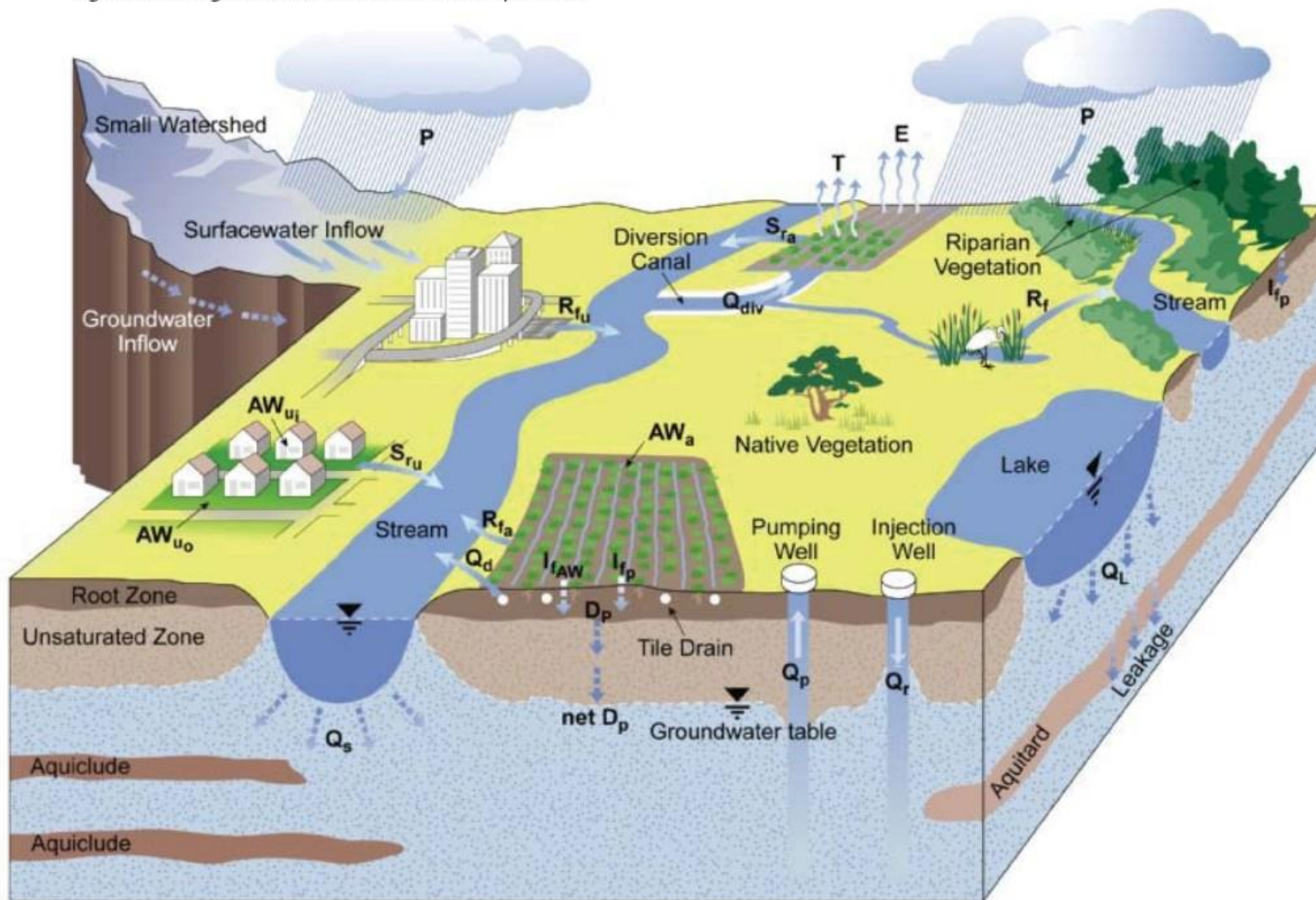
Figure 11. Integrated Water Flow Model components.
