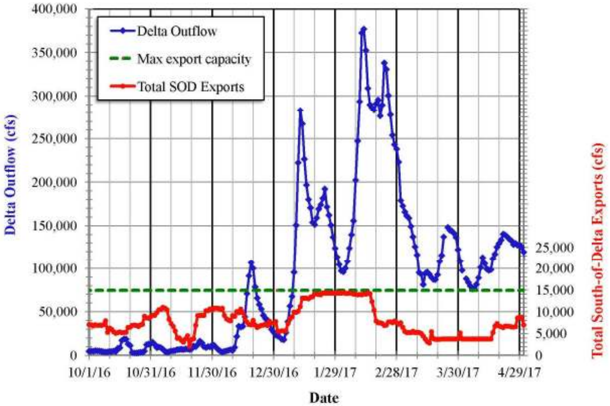
Figure 1: Daily-averaged total south-of-Delta SWP and CVP exports and estimated Delta outflow for the period October 1, 2016 through April 30, 2017
