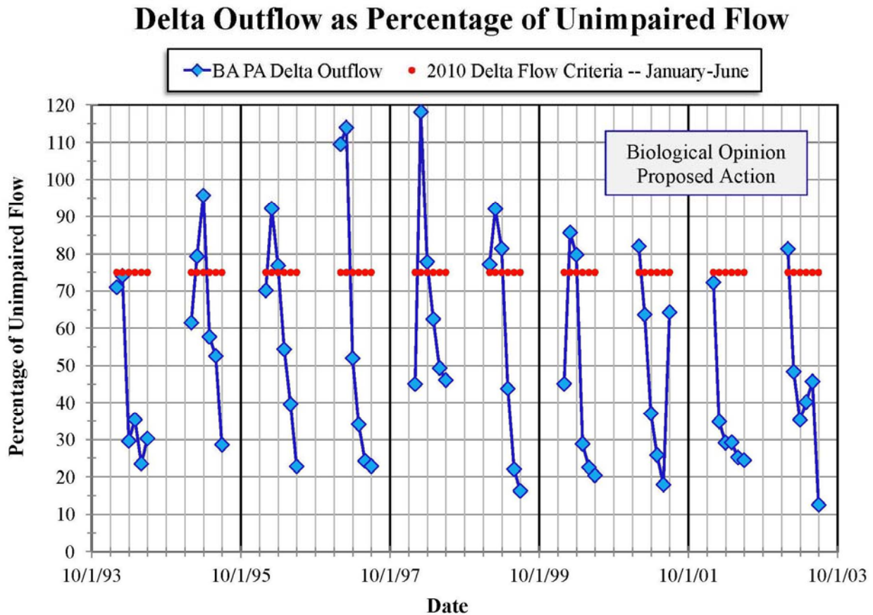
Figure 1: Simulated monthly-averaged Delta outflow as a percentage of unimpaired flow for the Biological Opinion Proposed Action for the period October 1993 through September 2003. Estimated historical unimpaired outflows are from DWR’s March 2006 draft report, “Estimates of Natural and Unimpaired Flows for the Central Valley of California: Water Years 1922-2014.” (CCC-SC-36).
