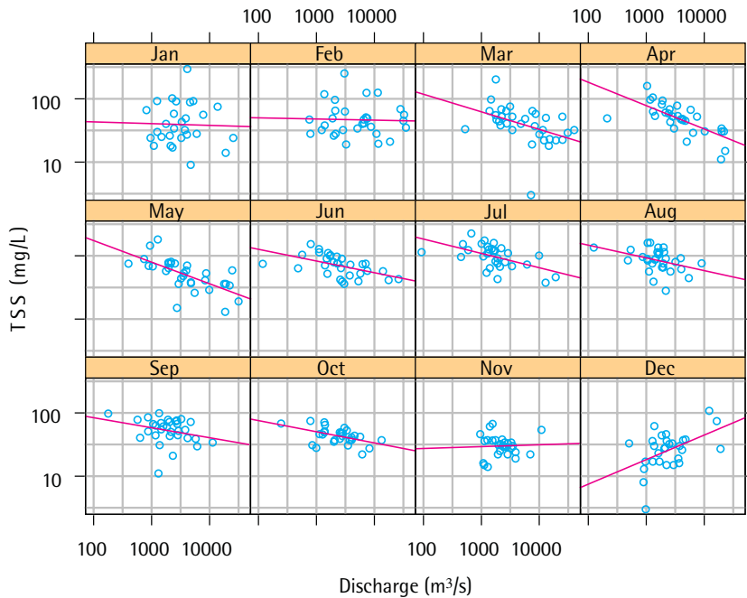
Figure 12. Total suspended solids versus discharge by month at Vernalis, 1969-2002. Straight lines , power relation between suspended matter and discharge.
