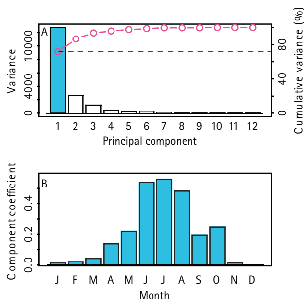
Figure 4. Principal component analysis of the chlorophyll a monthly time series. (A) Variance (bars) and cumulative variance (circles) corresponding to each principal component. Shading, statistically significant according to Rule N ( P < 0.05 ). (B) Coefficients for the first principal component.
