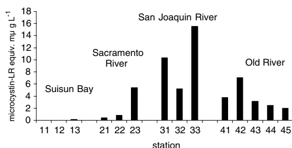
Figure 3. Surface microcystins equivalent concentration in the &gt;75 µm cell diameter size fraction.
