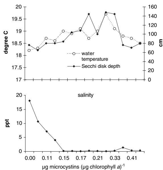
Figure 5. Variation of salinity, water temperature and Secchi disk depth with the microcystins to chlorophyll a ratio.
