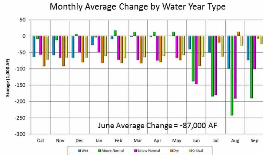
Figure 50. Oroville Reservoir Carryover Storage and Average Monthly Changes in Storage by Water Year Type MBK Alternative 4A and MBK NAA
