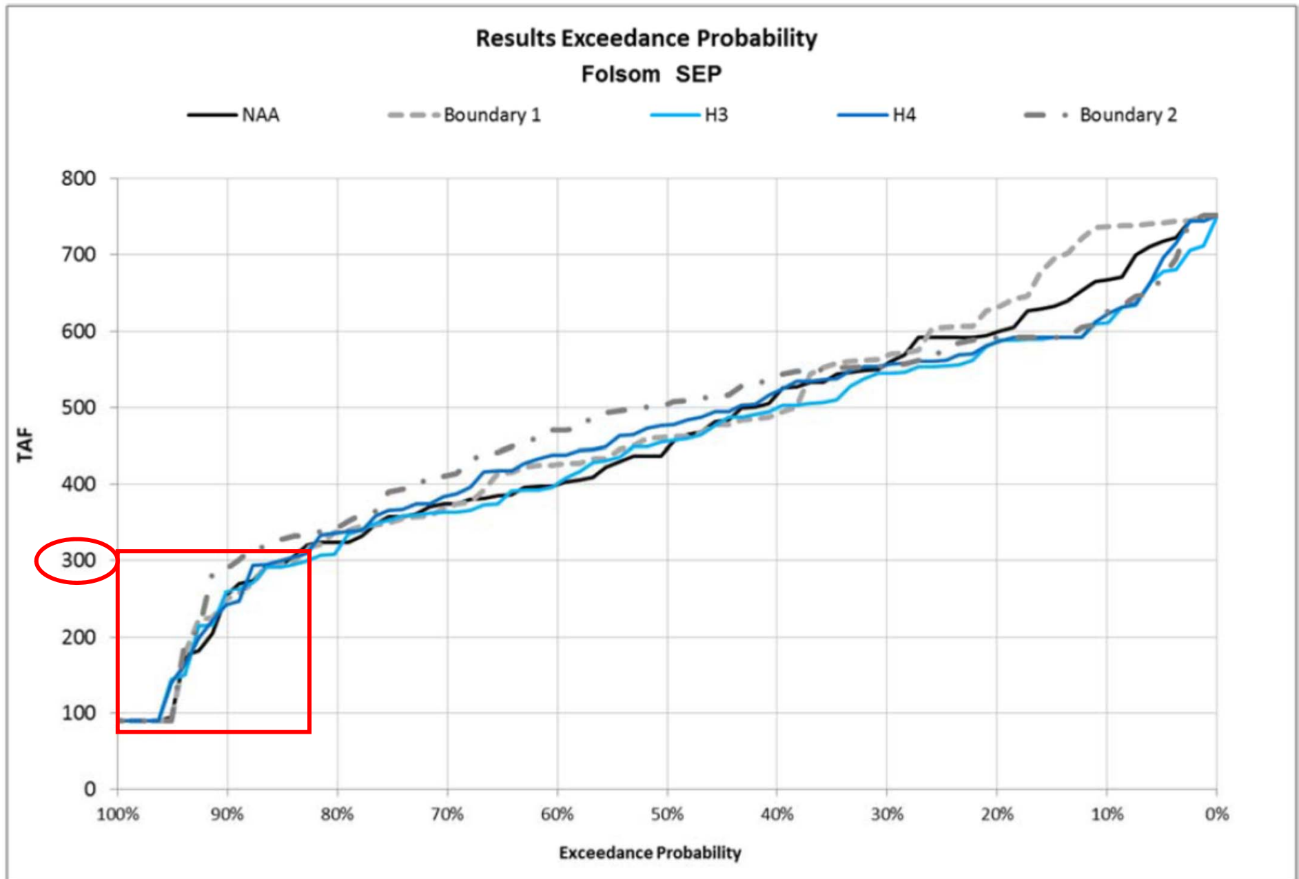
Figure 14. Simulated End of September Folsom Storage (From DWR-514)
