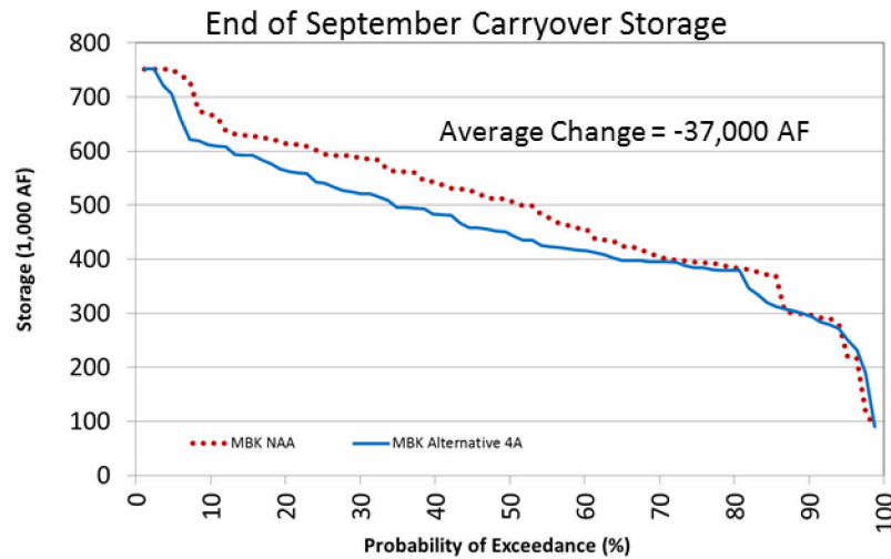
Figure 49. Folsom Reservoir Carryover Storage and Average Monthly Changes in Storage by Water Year Type MBK Alternative 4A and MBK NAA
