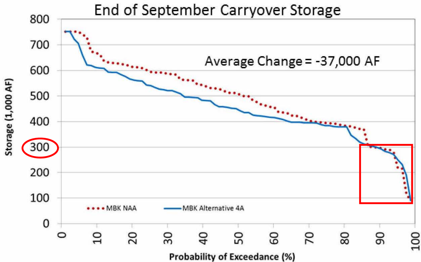
Figure 49. Folsom Reservoir Carryover Storage and Average Monthly Chan
