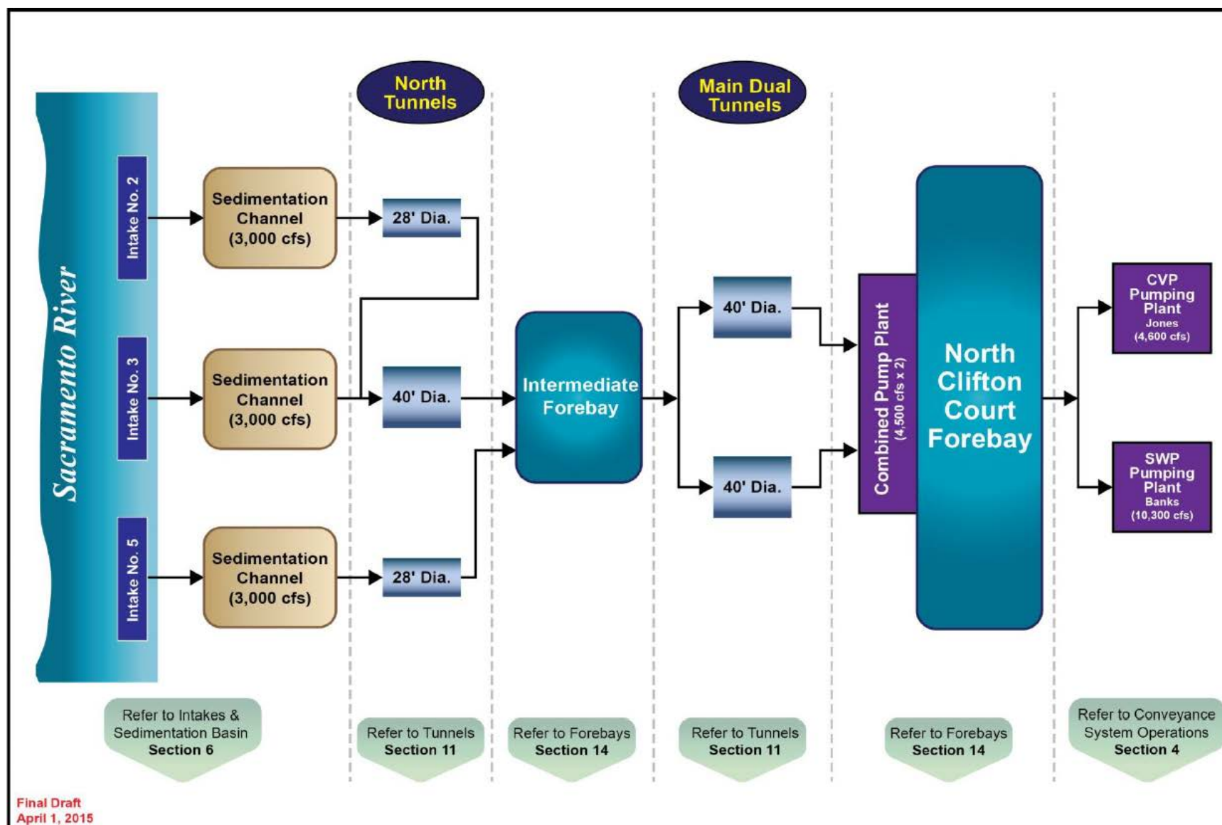
Figure 2 Conveyance Schematic
