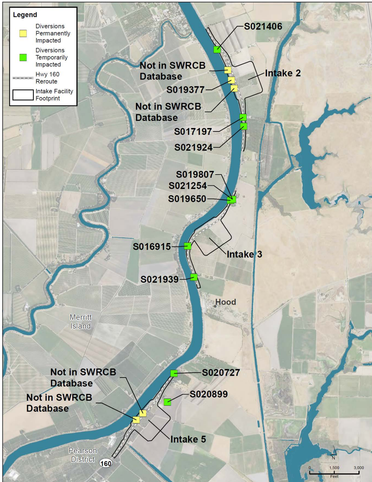
Figure 5 Existing Water Diversions at the Proposed Intake Sites
