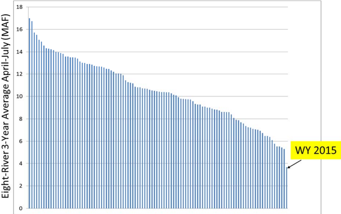
Figure 7- Eight River 3 Year Average April-July Runoff (1909-2015)
