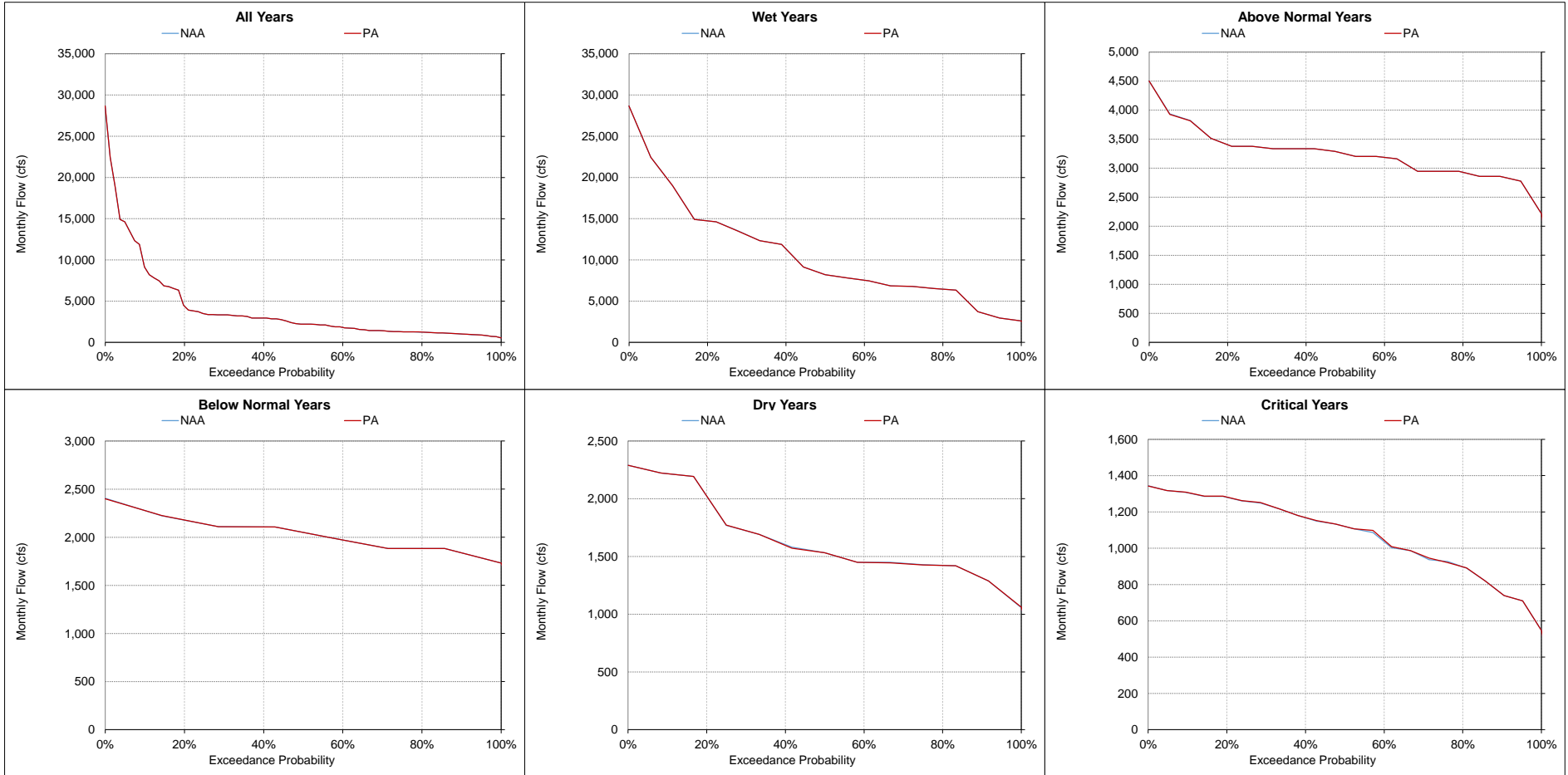
Figure 5.A.6-23-16. San Joaquin River at Vernalis, Monthly Flow
