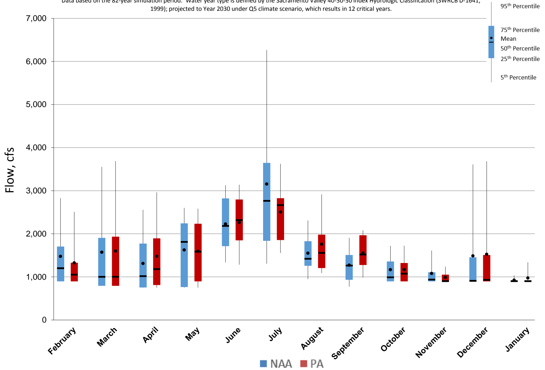
Figure 5.A.6-12-6. Monthly Flow Ranges For Feather River below Thermalito Diversion Dam, Critical Years
