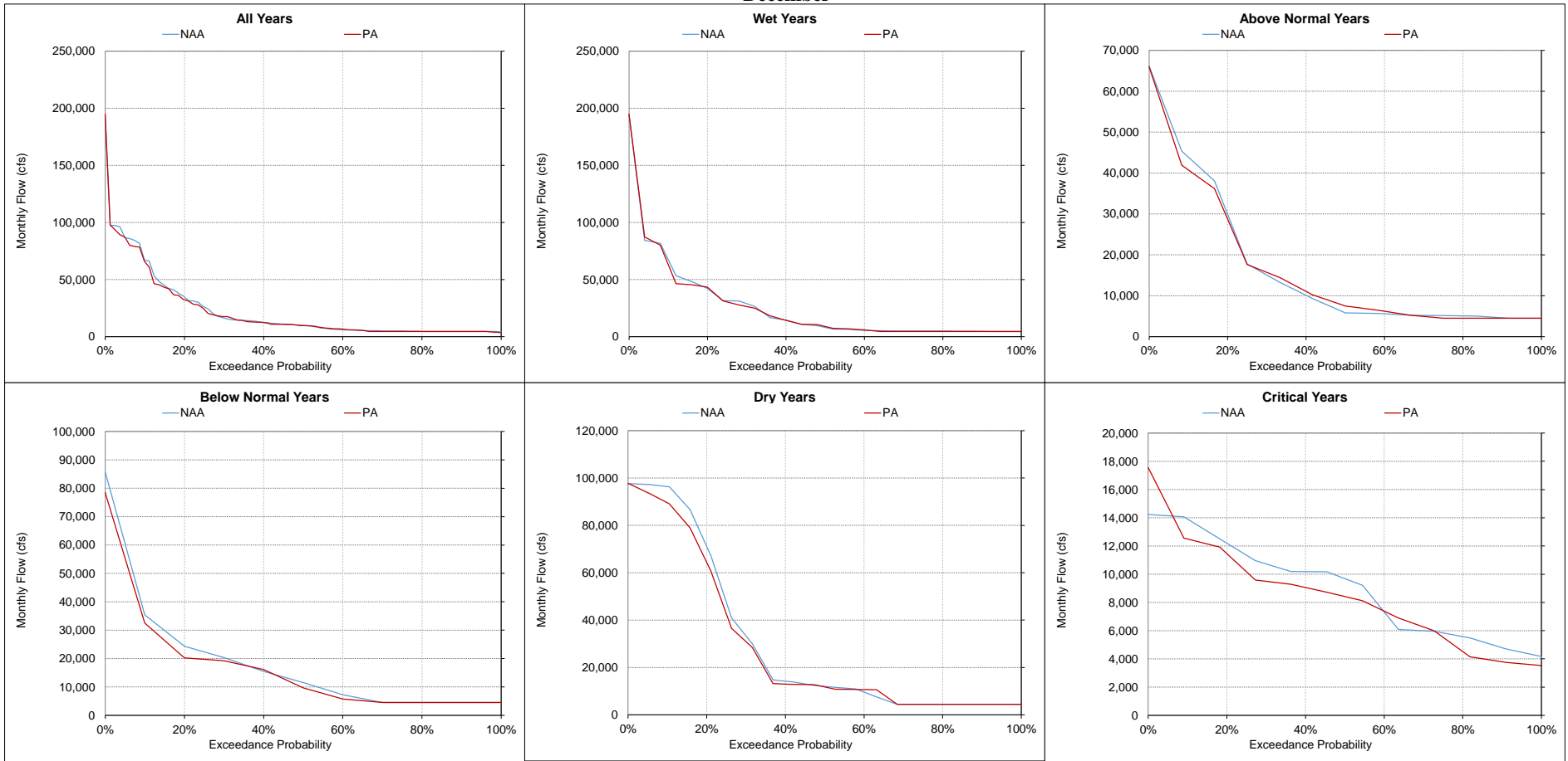
Figure 5.A.6-26-10. Delta Outflow, Monthly Flow December
