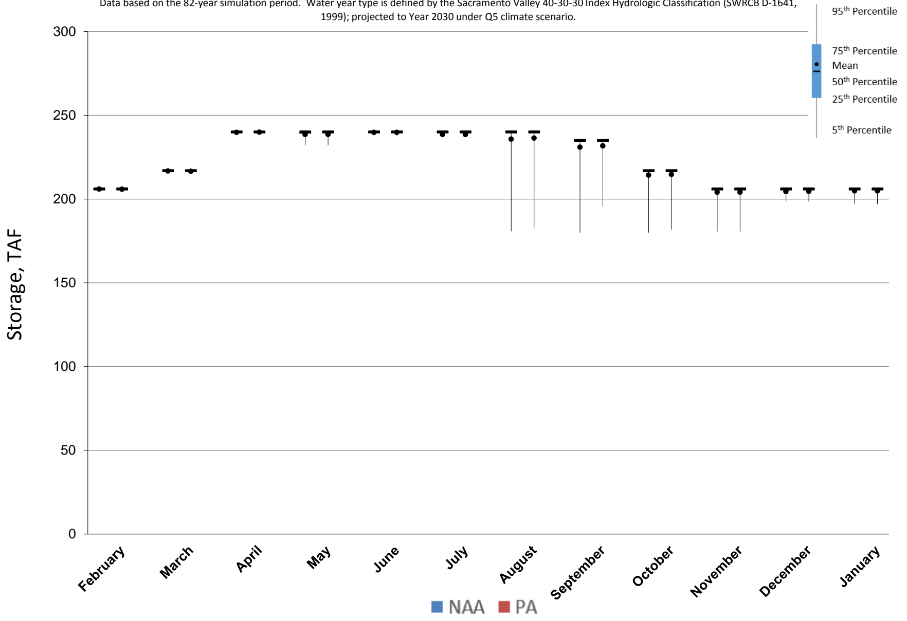
Figure 5.A.6-2-1. End of Month Storage Ranges For Whiskeytown Reservoir, All Years
