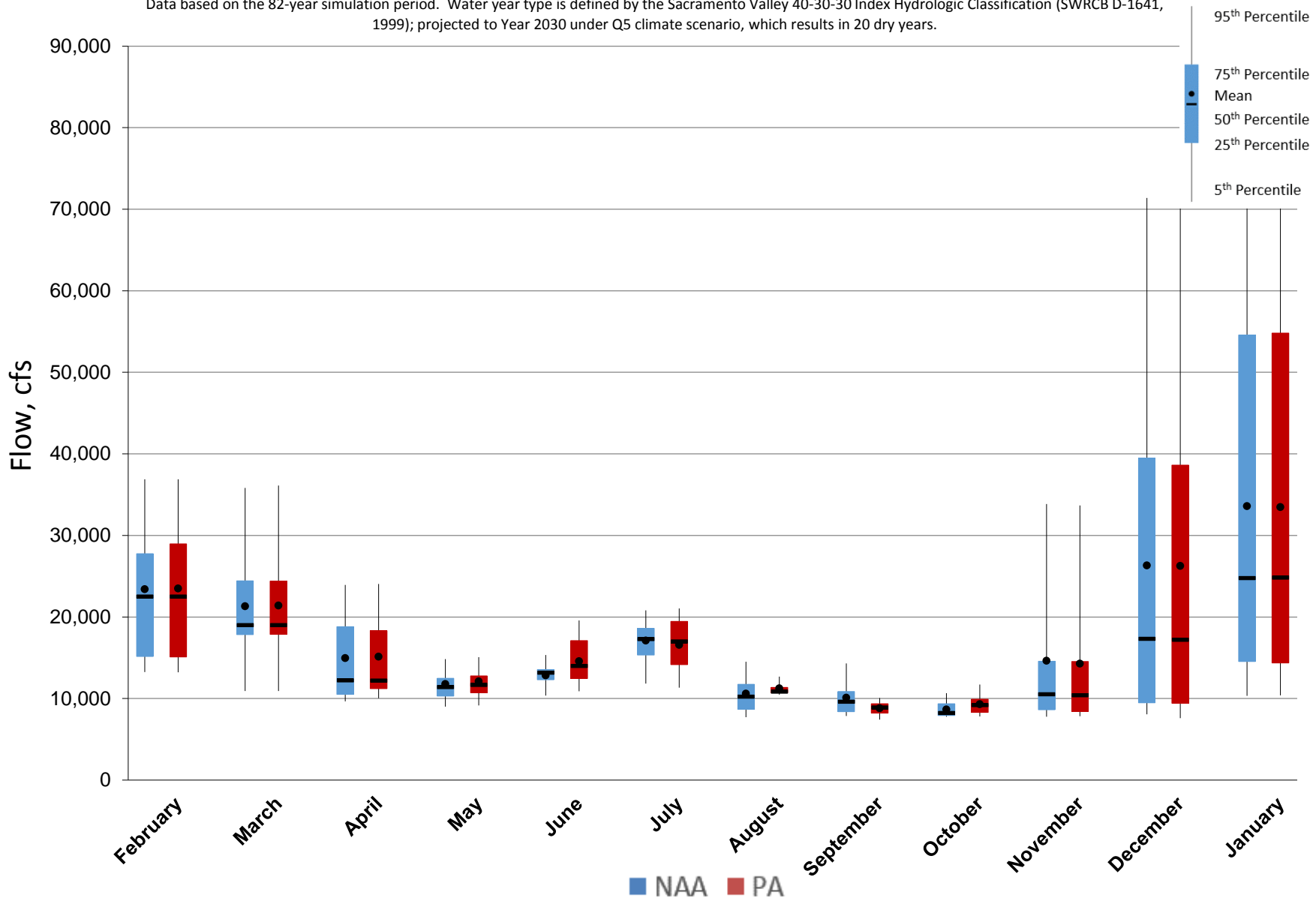
Figure 5.A.6-18-5. Monthly Flow Ranges For Sacramento River at Freeport, Dry Years
