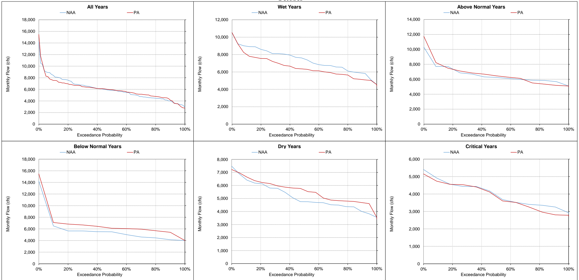
Figure 5.A.6-11-8. Sacramento River at Bend Bridge, Monthly Flow October
