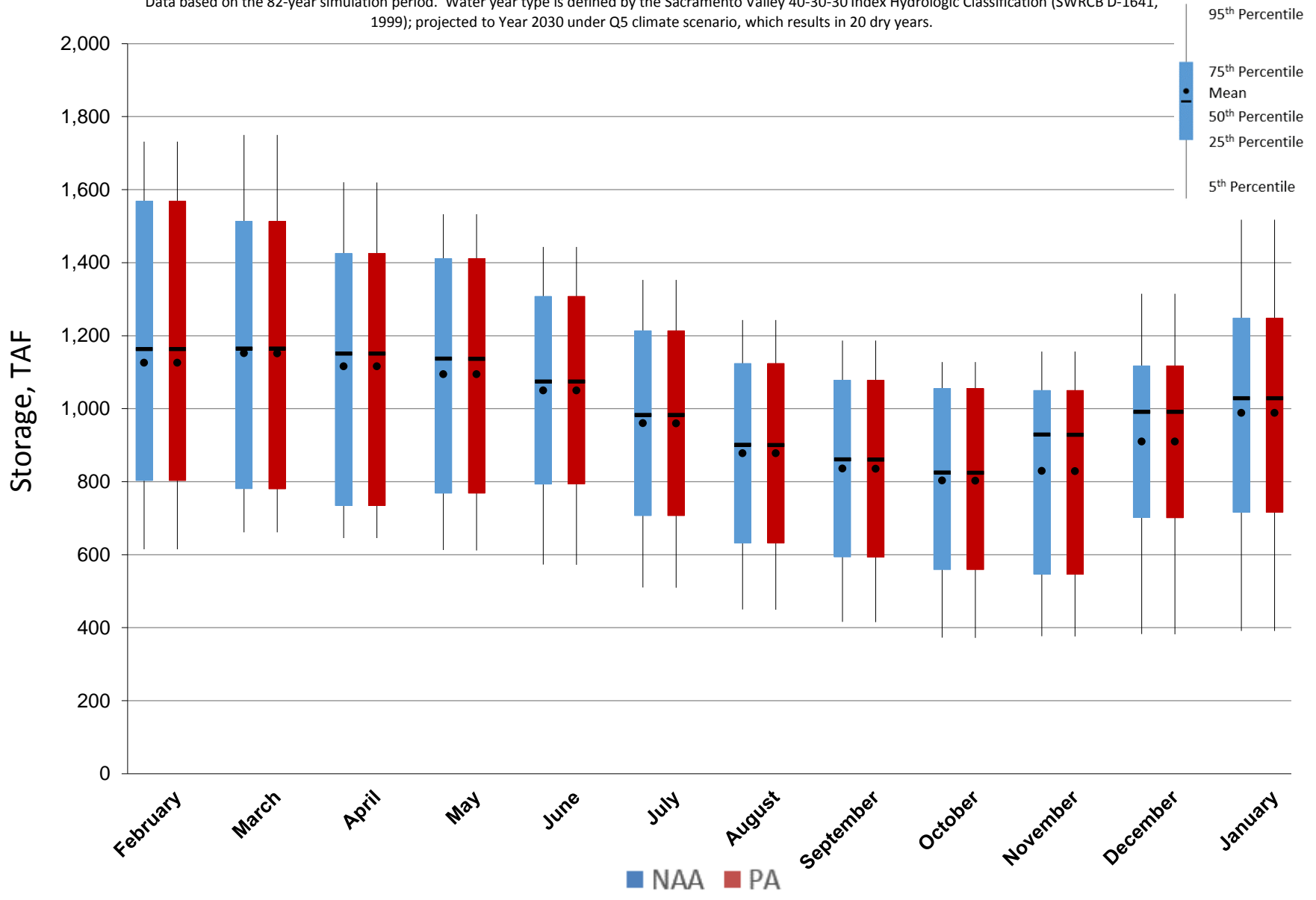
Figure 5.A.6-6-5. End of Month Storage Ranges For New Melones Lake, Dry Years
