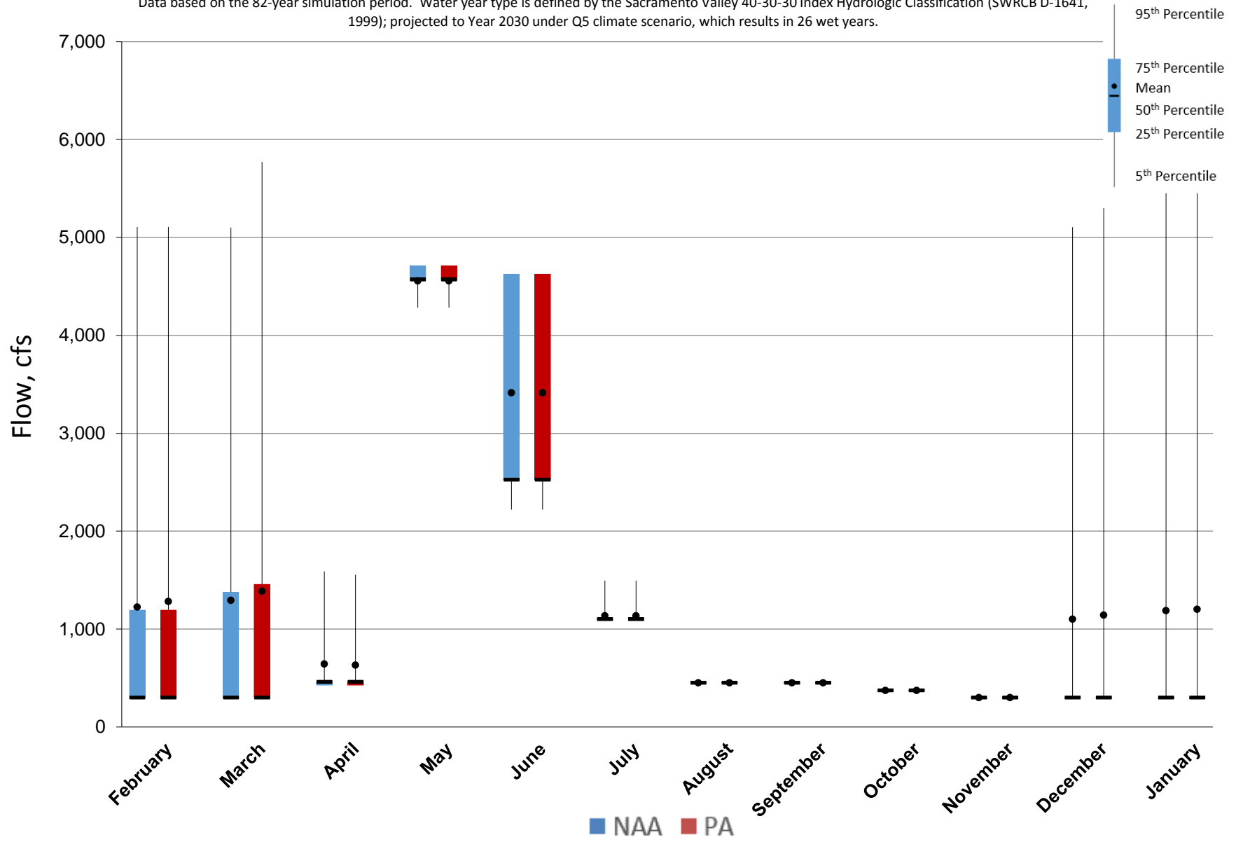
Figure 5.A.6-7-2. Monthly Flow Ranges For Trinity River below Lewiston Dam, Wet Years
