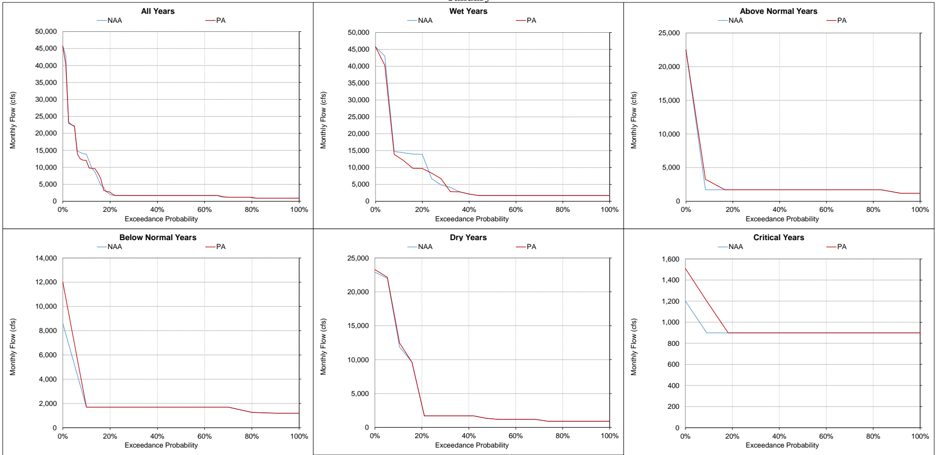
Figure 5.A.6-12-11. Feather River below Thermalito Diversion Dam, Monthly Flow January
