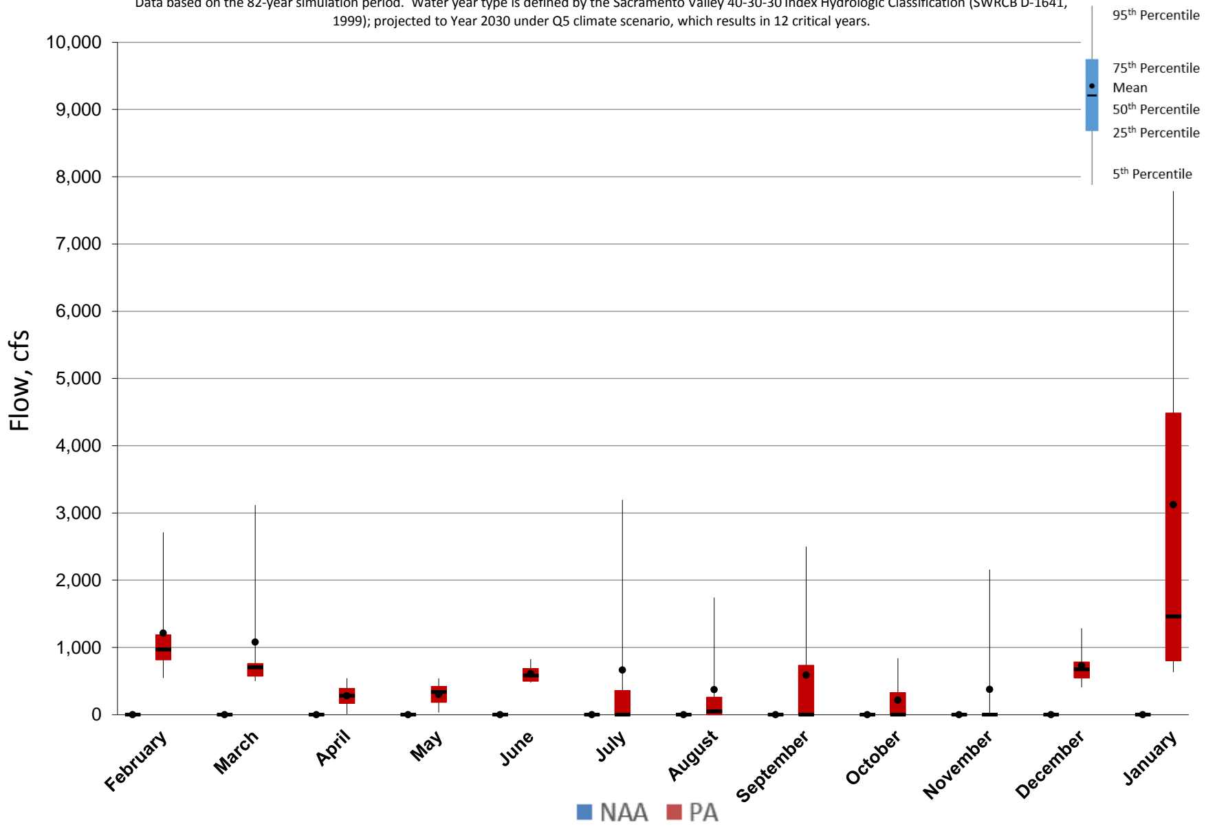
Figure 5.A.6-19-6. Monthly Flow Ranges For North Delta Diversions near Hood, Critical Years
