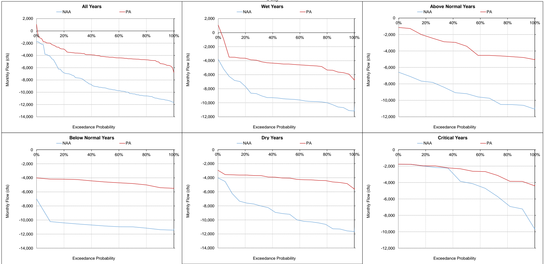
Figure 5.A.6-25-17. Old and Middle River, Monthly Flow July
