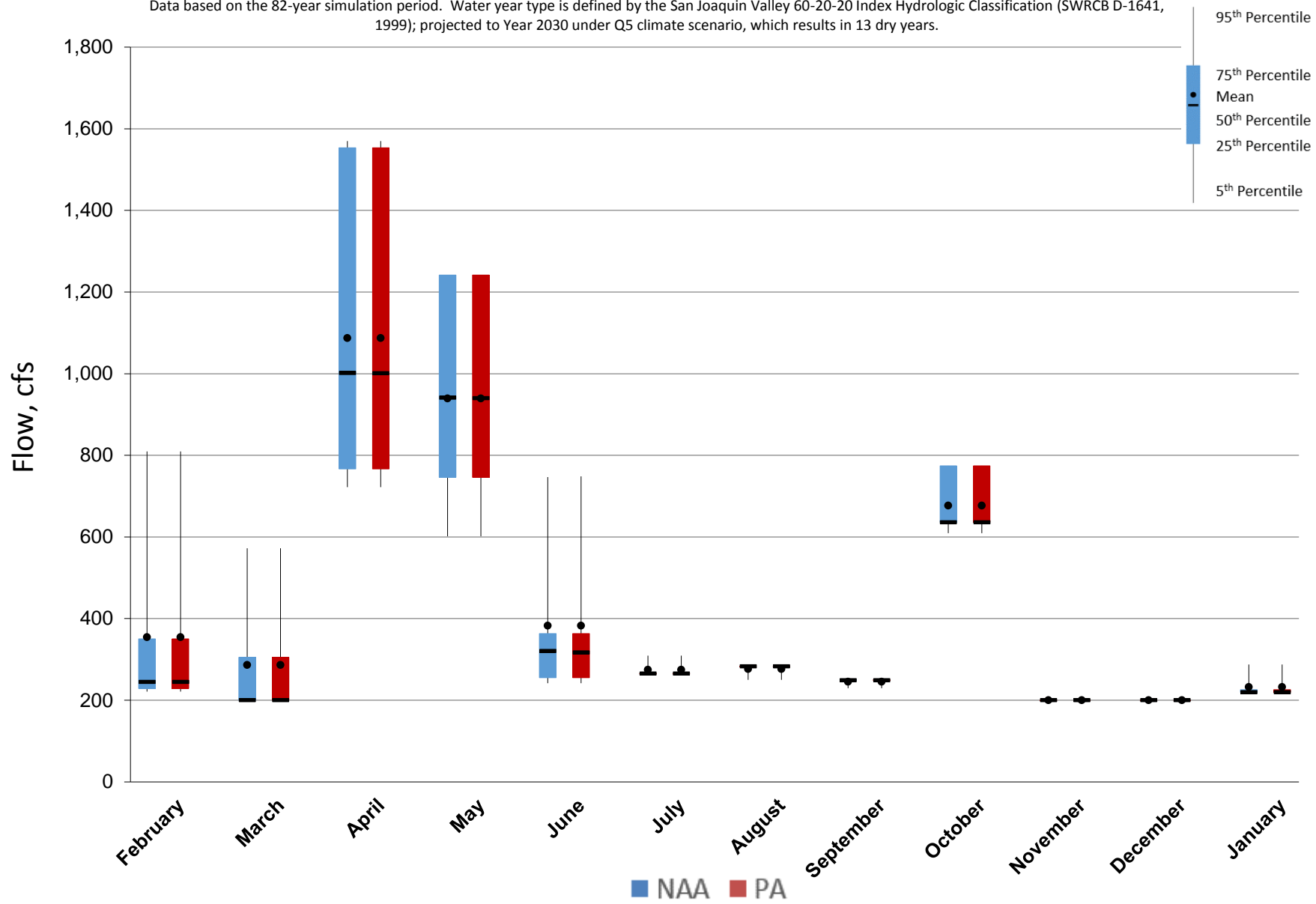
Figure 5.A.6-21-5. Monthly Flow Ranges for Stanislaus River at Ripon, Dry Years
