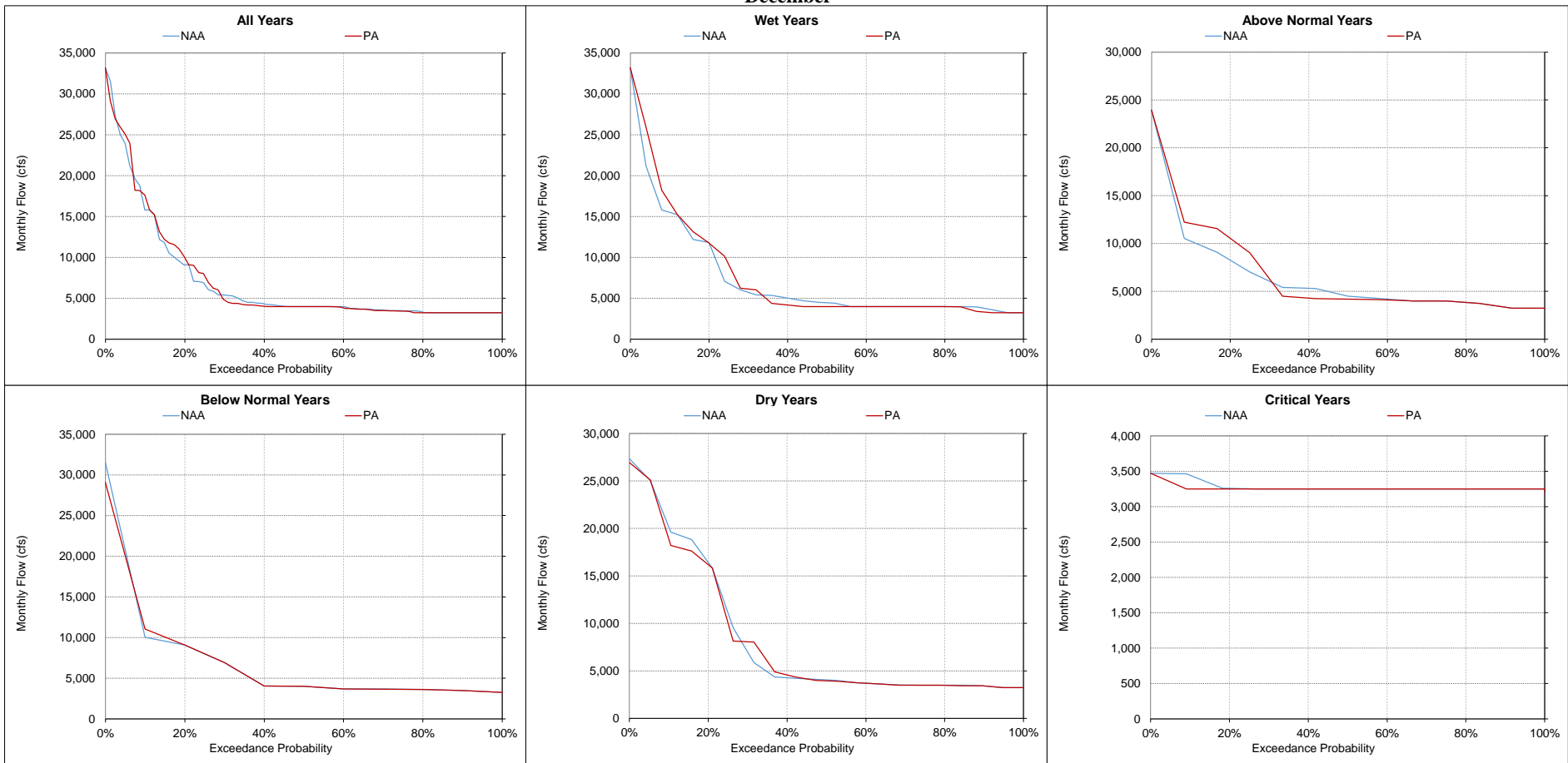
Figure 5.A.6-10-10. Sacramento River below Keswick Dam, Monthly Flow December
