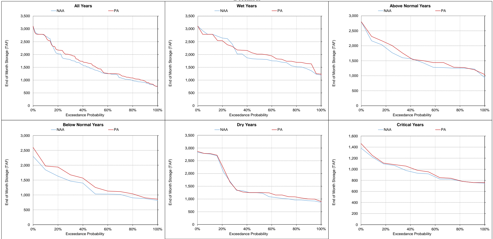
Figure 5.A.6-4-10. Lake Oroville, End of Month Storage December
