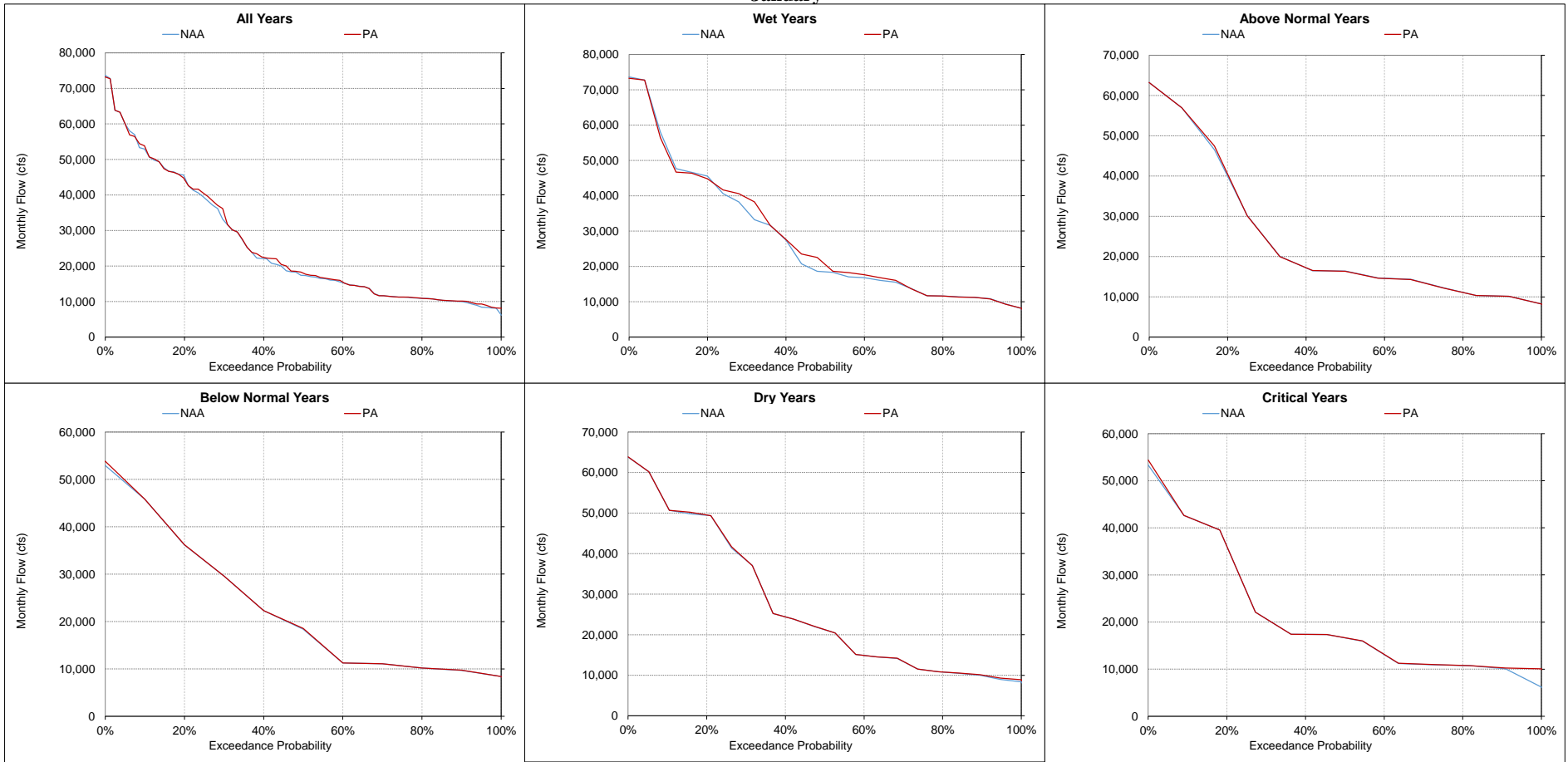
Figure 5.A.6-14-11. Sacramento River at Verona, Monthly Flow January
