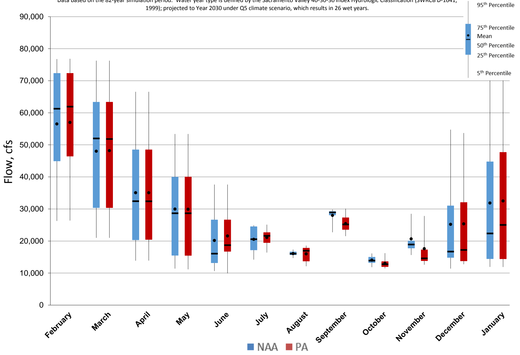
Figure 5.A.6-18-2. Monthly Flow Ranges For Sacramento River at Freeport, Wet Years
