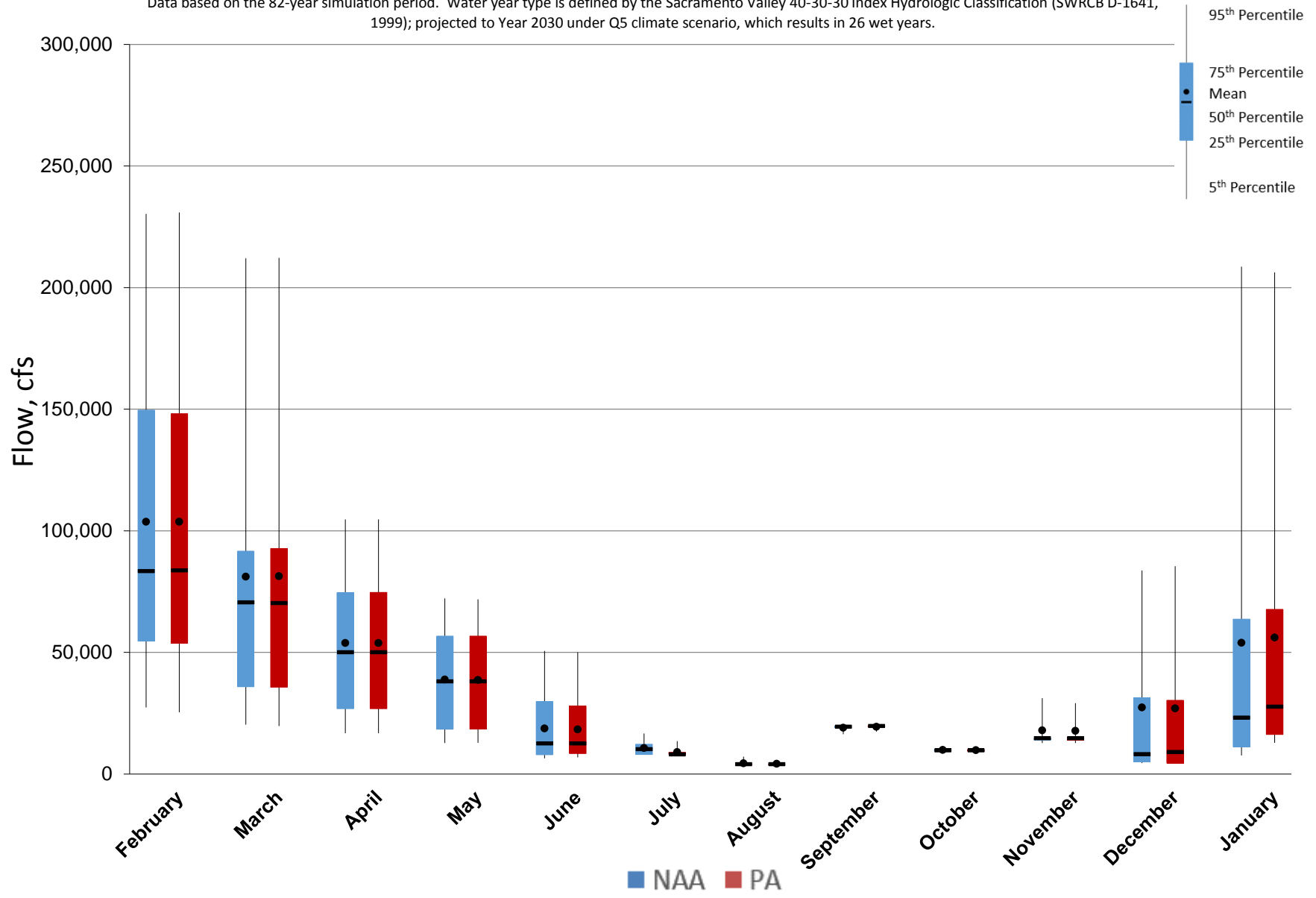
Figure 5.A.6-26-2. Monthly Flow Ranges For Delta Outflow, Wet Years
