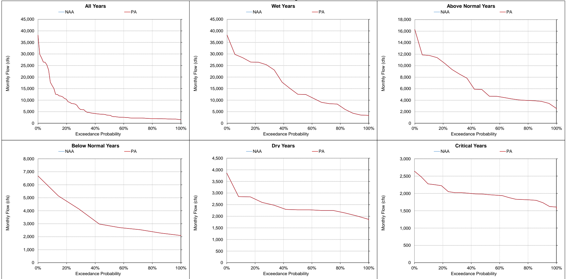
Figure 5.A.6-23-12. San Joaquin River at Vernalis, Monthly Flow February
