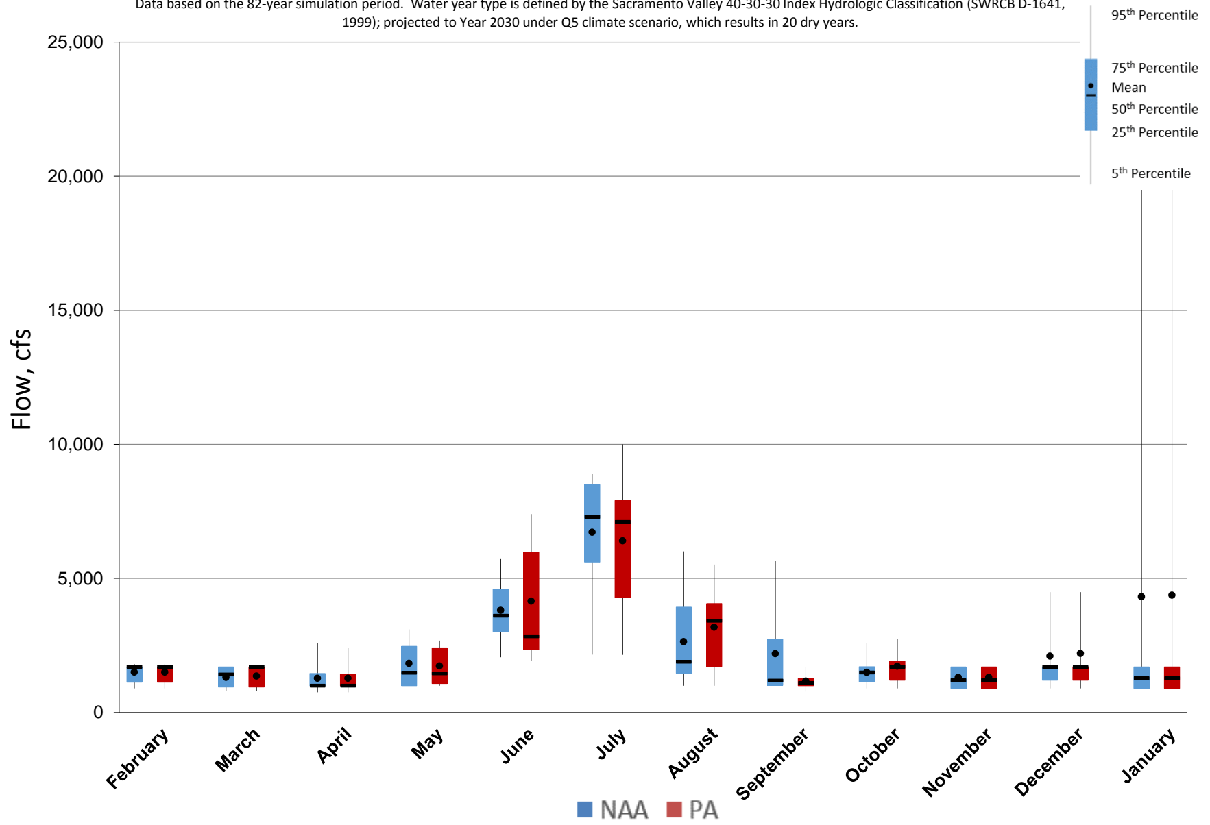
Figure 5.A.6-12-5. Monthly Flow Ranges For Feather River below Thermalito Diversion Dam, Dry Years
