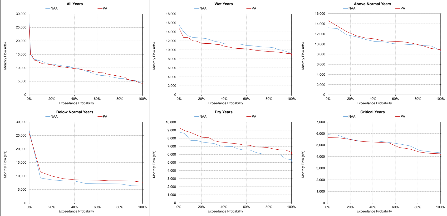
Figure 5.A.6-14-8. Sacramento River at Verona, Monthly Flow October
