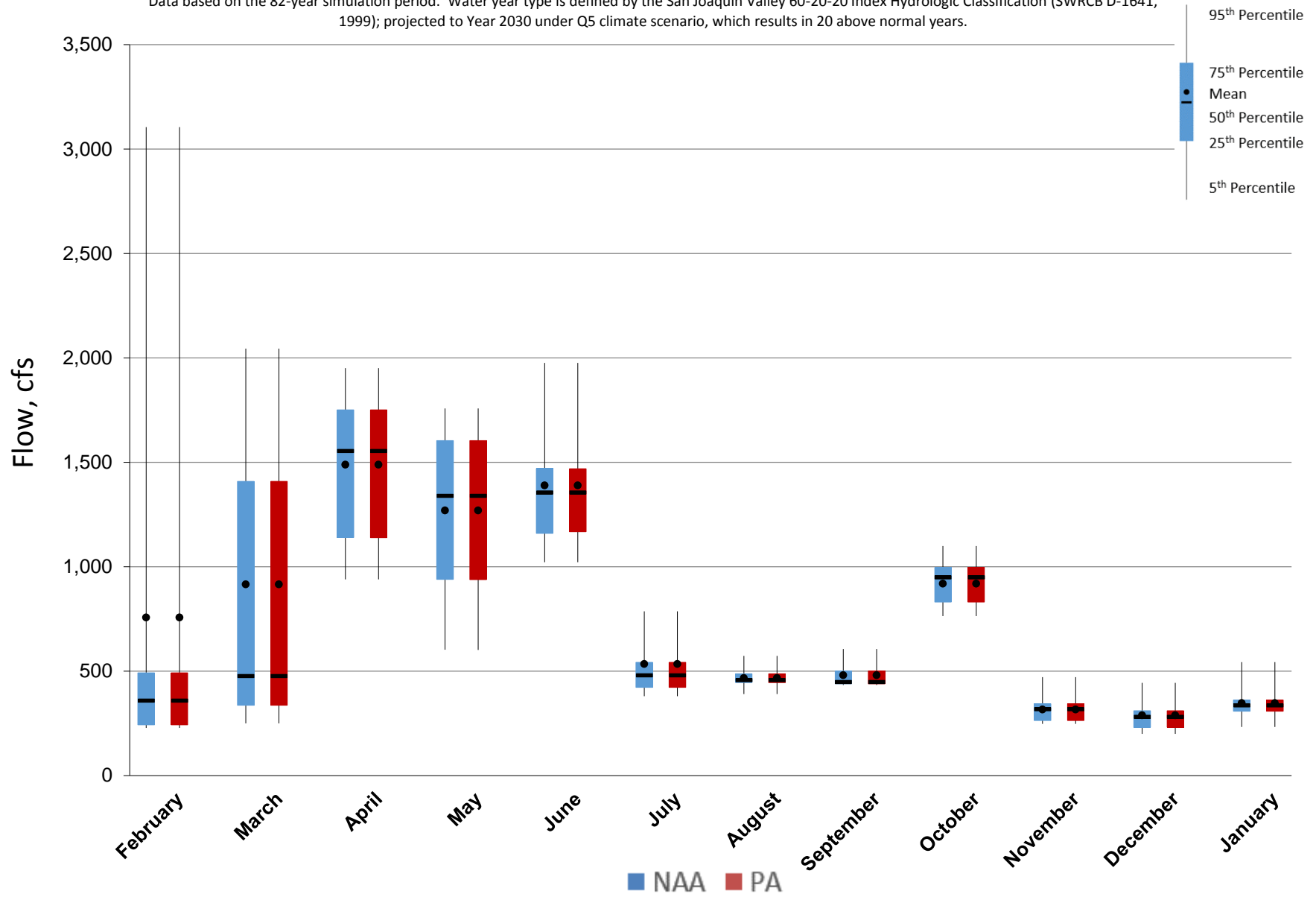
Figure 5.A.6-22-3. Monthly Flow Ranges for Stanislaus River at Mouth, Above Normal Years
