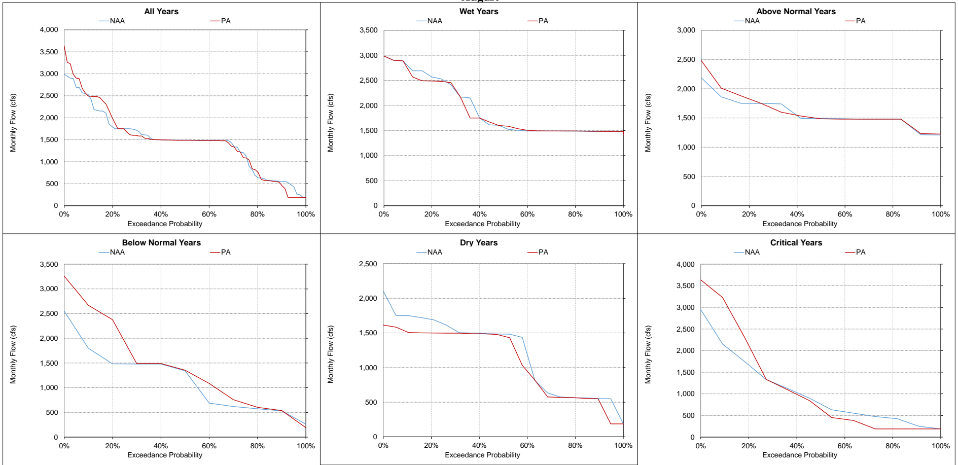
Figure 5.A.6-17-18. American River at Sacramento River Confluence, Monthly Flow August
