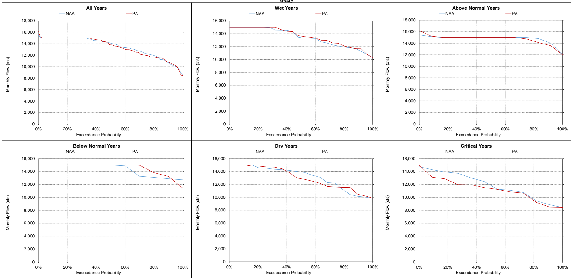
Figure 5.A.6-10-17. Sacramento River below Keswick Dam, Monthly Flow July
