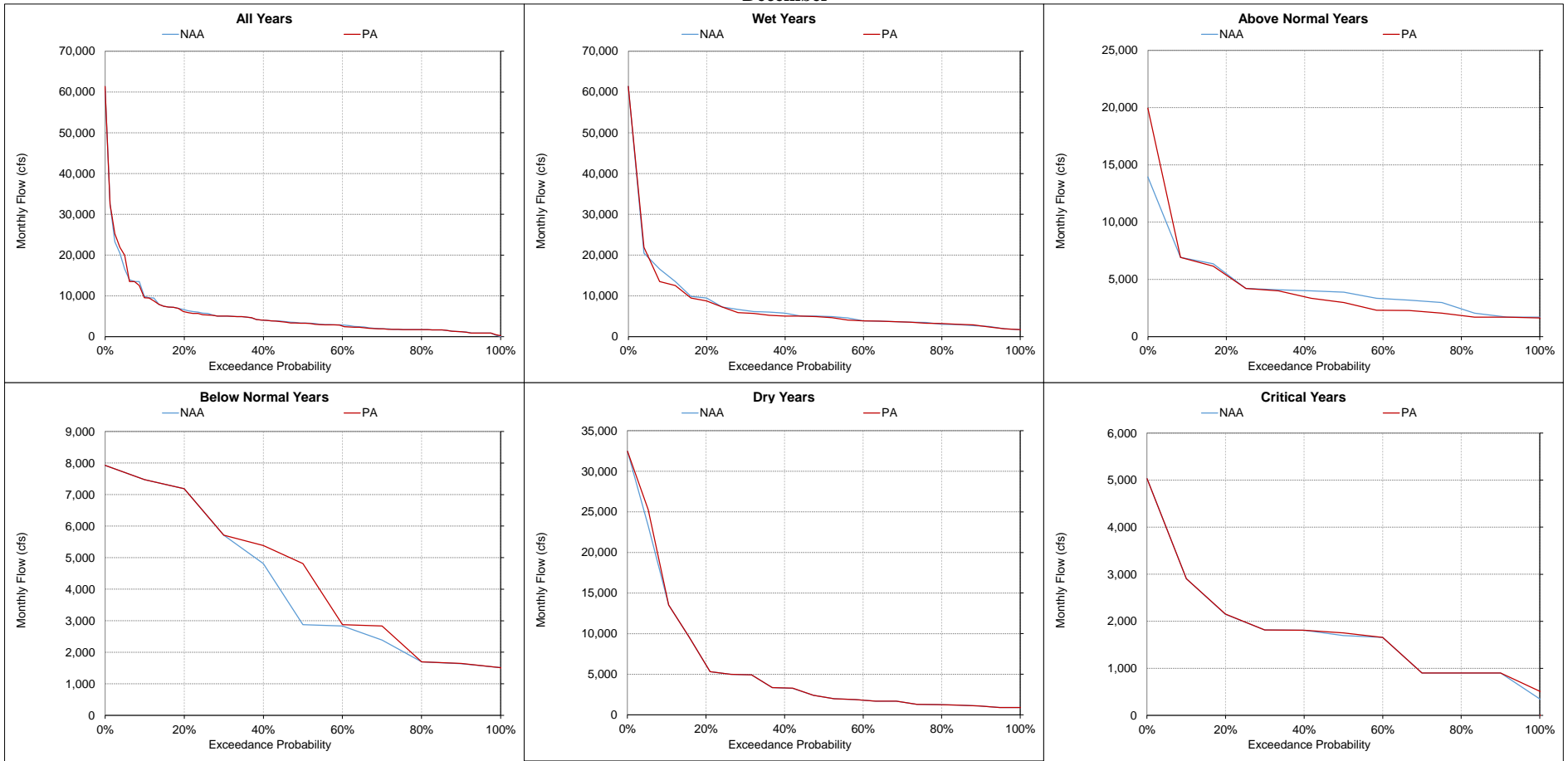
Figure 5.A.6-13-10. Feather River at Sacramento River Confluence, Monthly Flow December
