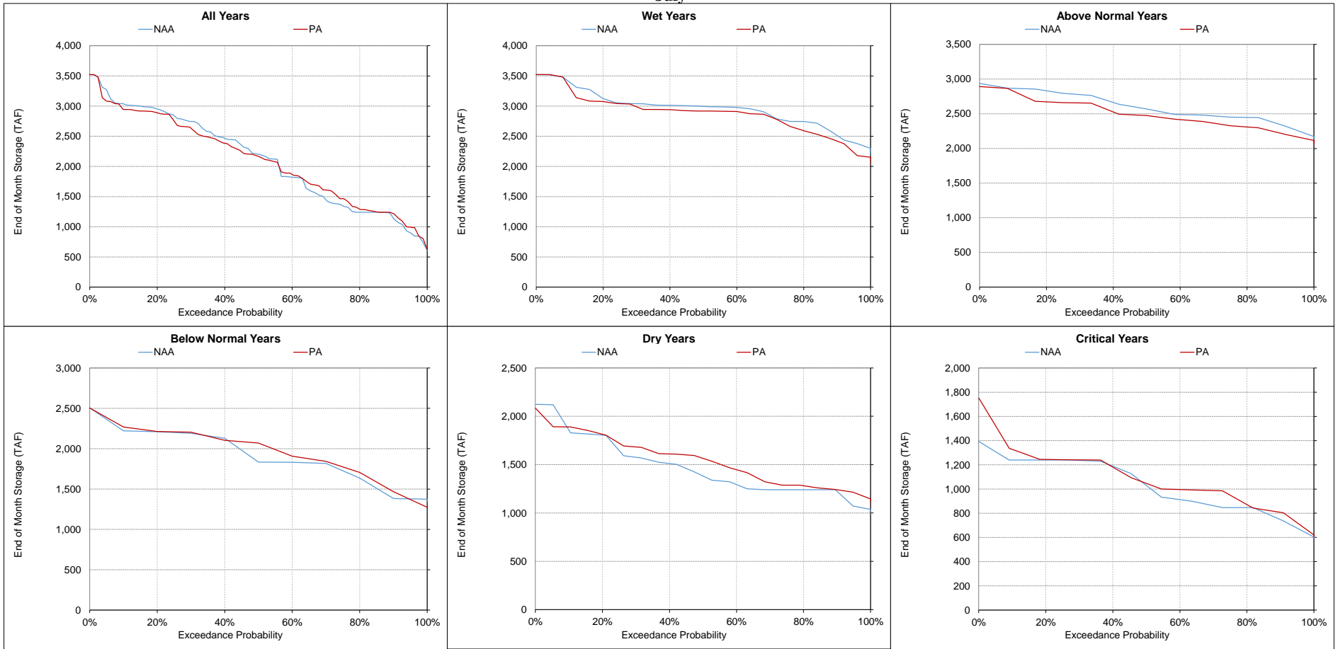
Figure 5.A.6-4-17. Lake Oroville, End of Month Storage July
