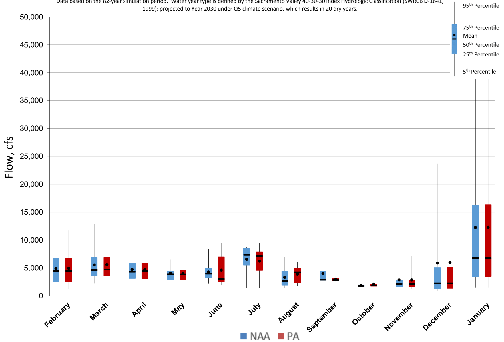
Figure 5.A.6-13-5. Monthly Flow Ranges For Feather River at Sacramento River Confluence, Dry Years
