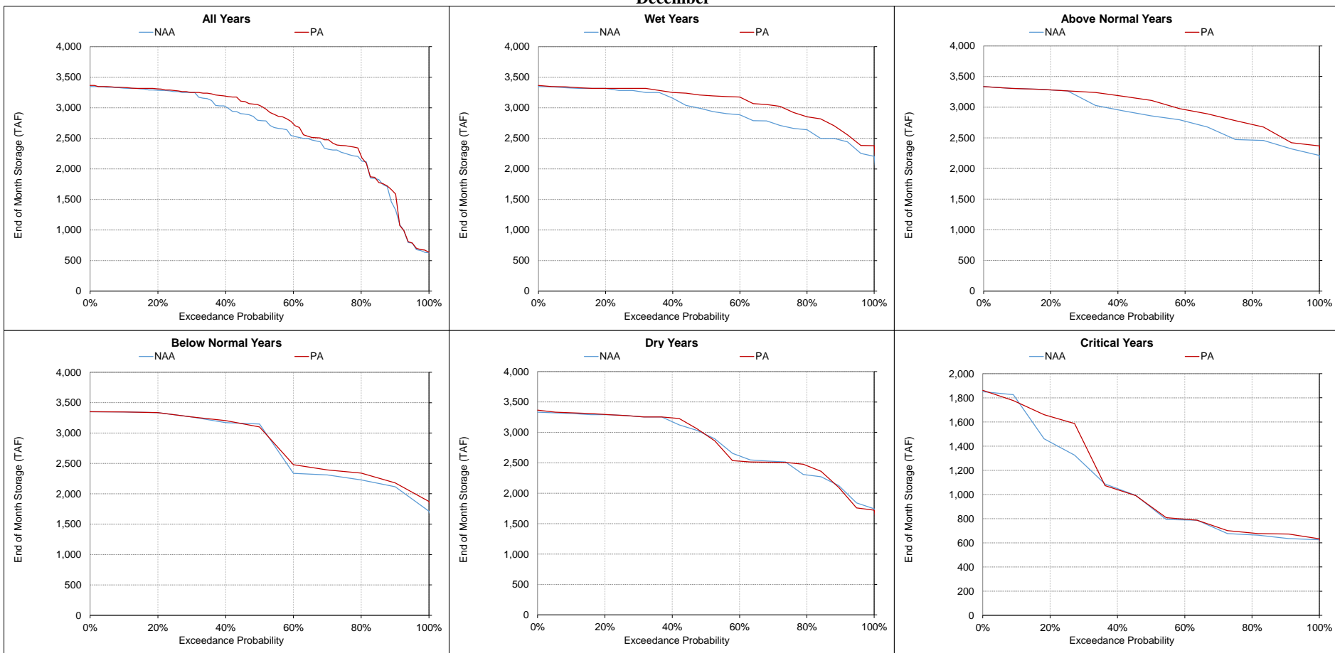
Figure 5.A.6-3-10. Shasta Lake, End of Month Storage December
