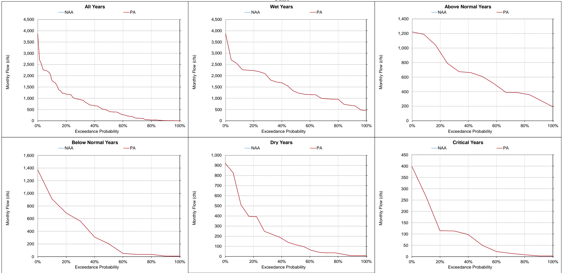
Figure 5.A.6-24-16. Mokelumne and Cosumnes River, Monthly Flow June
