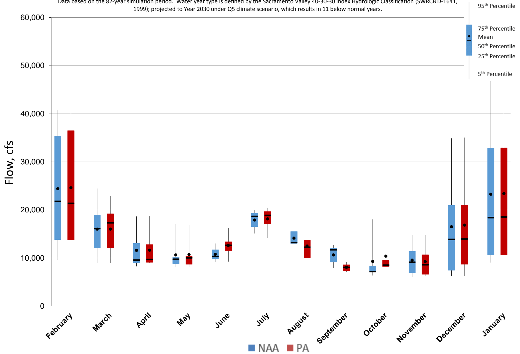
Figure 5.A.6-14-4. Monthly Flow Ranges For Sacramento River at Verona, Below Normal Years
