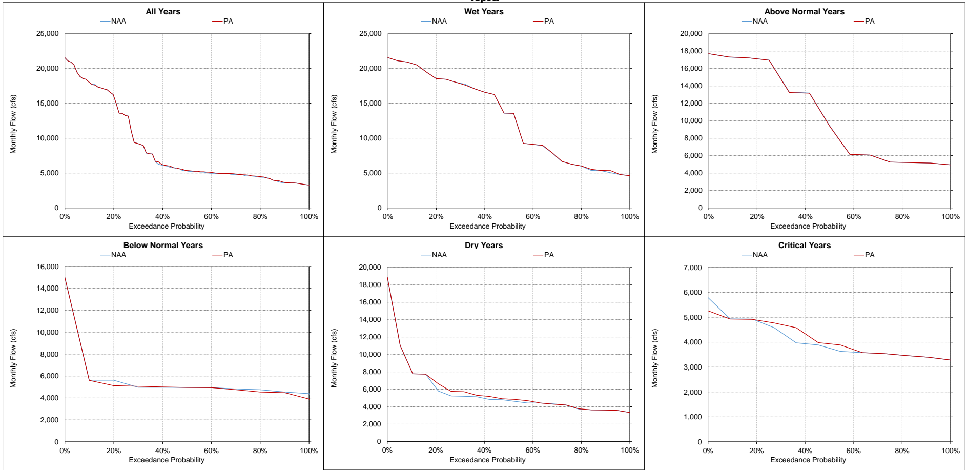
Figure 5.A.6-11-14. Sacramento River at Bend Bridge, Monthly Flow April
