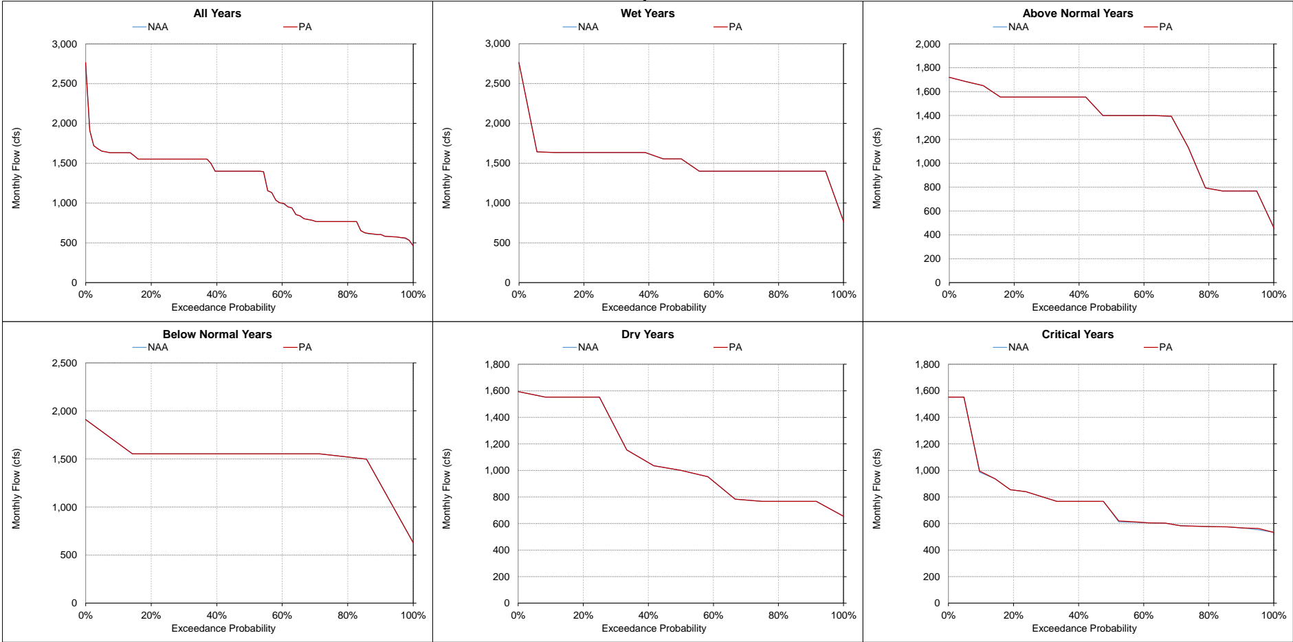
Figure 5.A.6-21-14. Stanislaus River at Ripon, Monthly Flow
