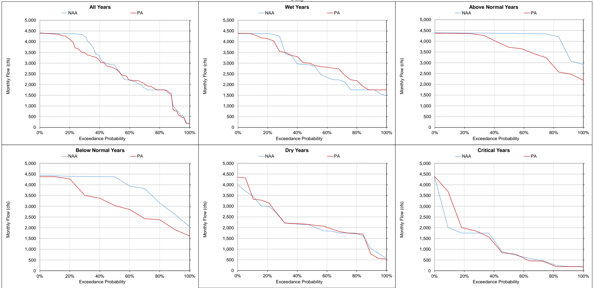
Figure 5.A.6-17-17. American River at Sacramento River Confluence, Monthly Flow July
