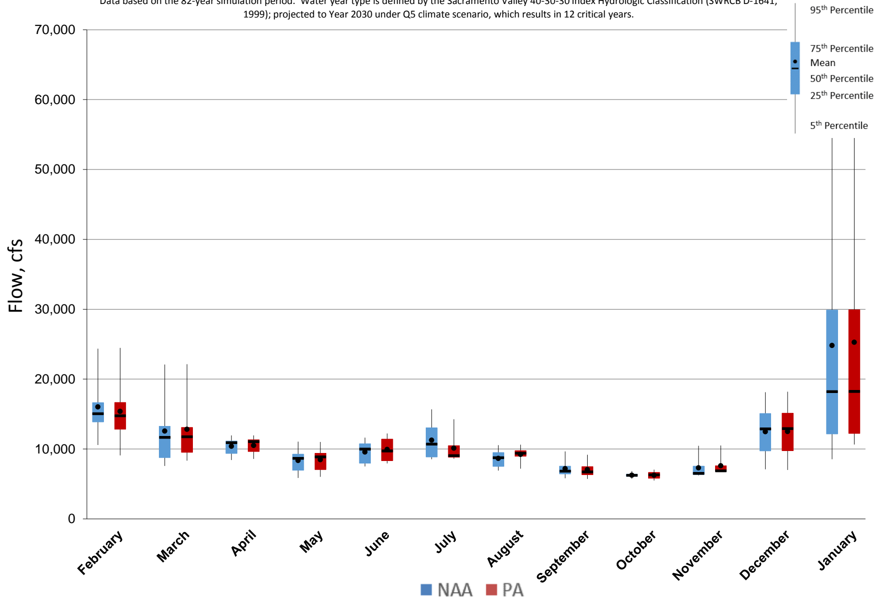
Figure 5.A.6-18-6. Monthly Flow Ranges For Sacramento River at Freeport, Critical Years
