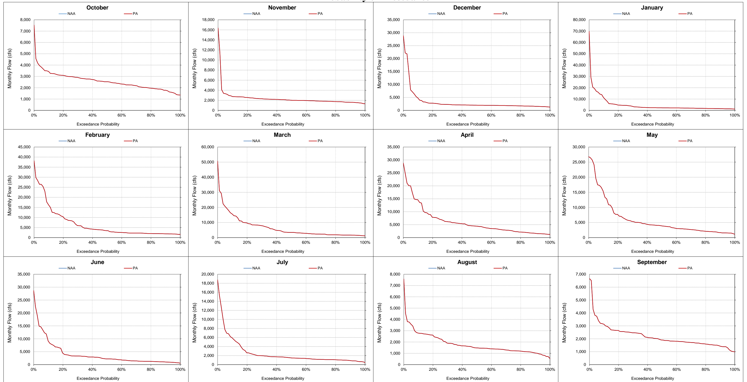
Figure 5.A.6-23-7. San Joaquin River at Vernalis, Monthly Flow Probability of Exceedance
