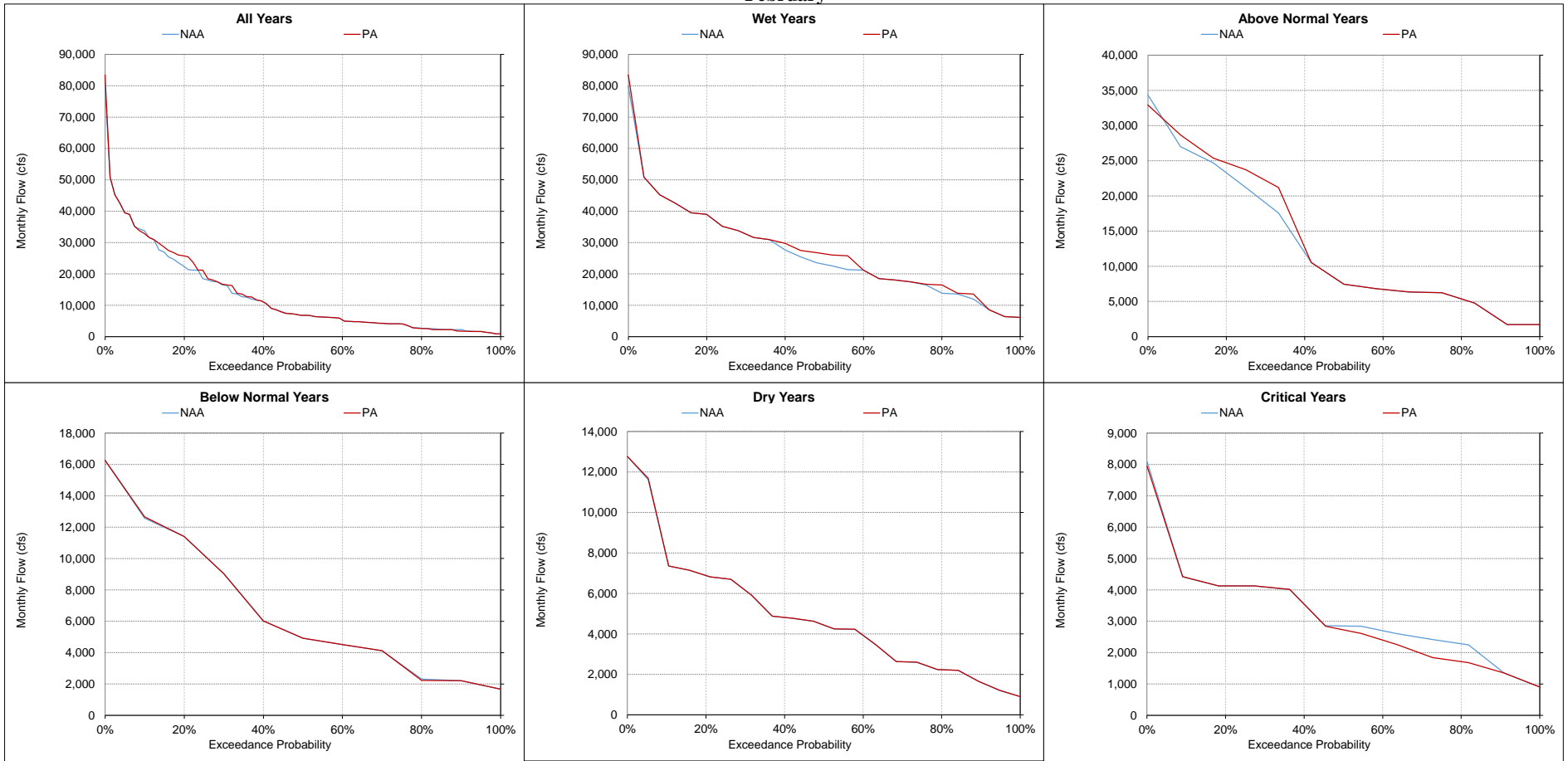
Figure 5.A.6-13-12. Feather River at Sacramento River Confluence, Monthly Flow February
