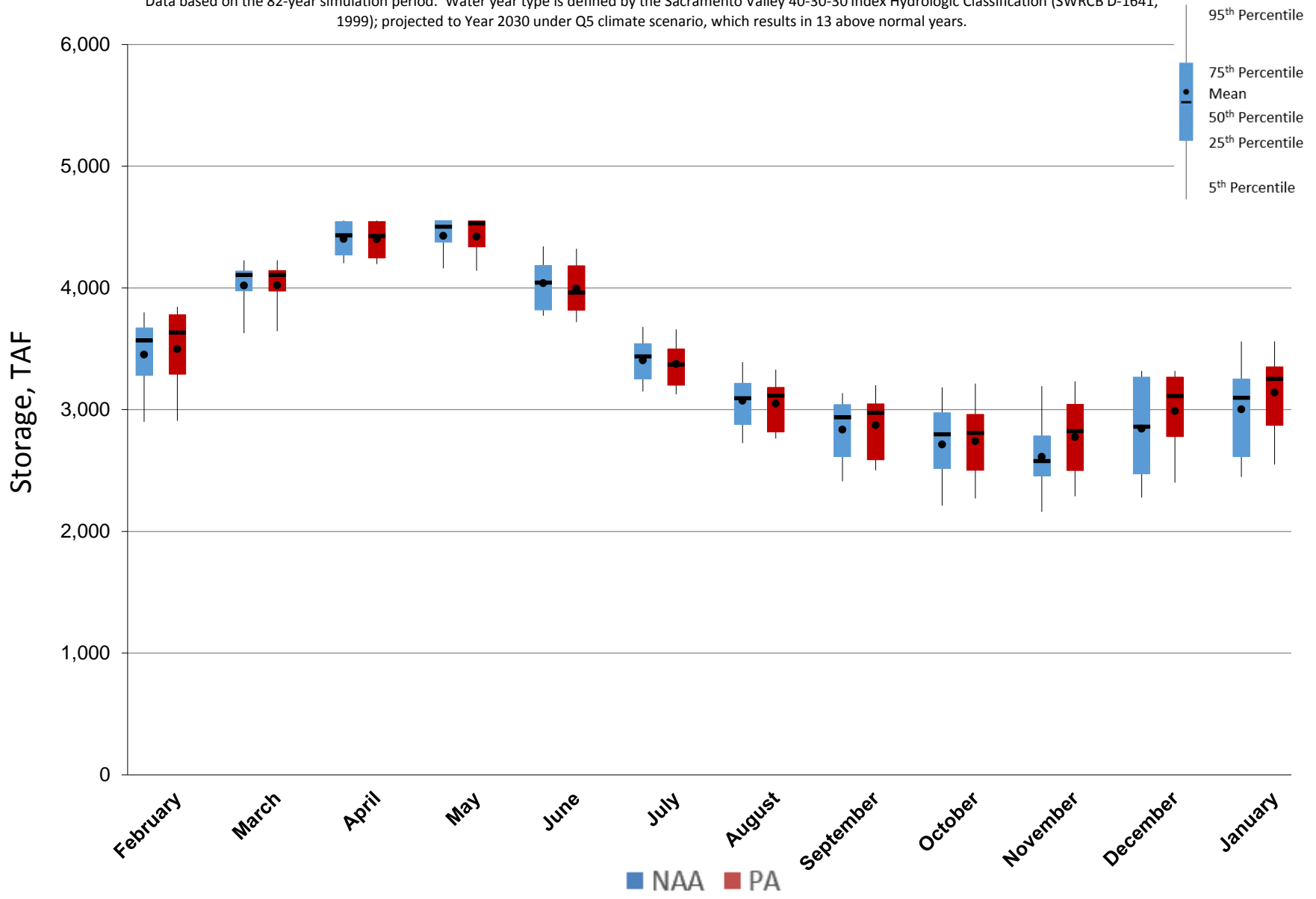
Figure 5.A.6-3-3. End of Month Storage Ranges For Shasta Lake, Above Normal Years
