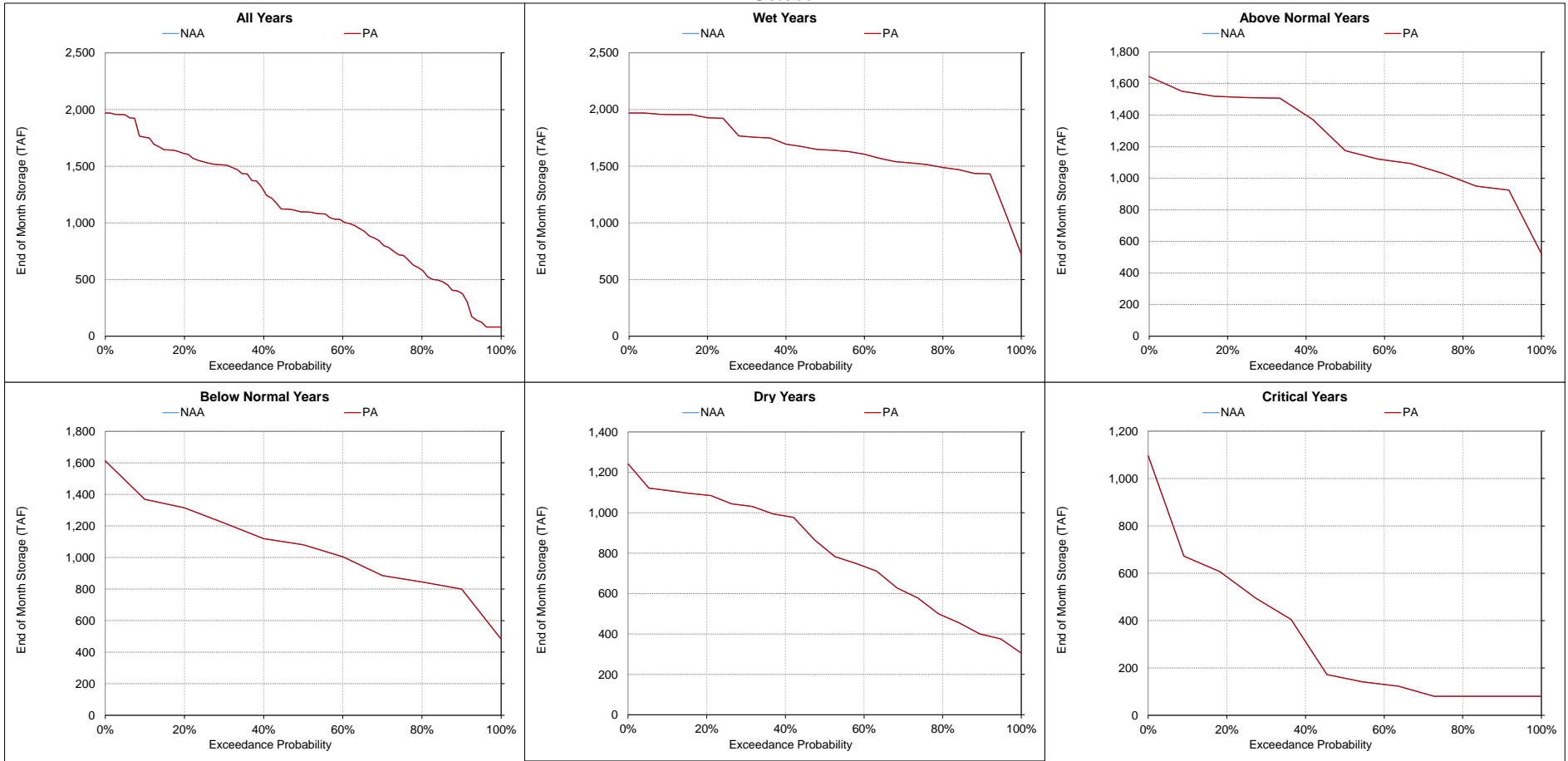
Figure 5.A.6-8. New Melones Lake, End of Month Storage October
