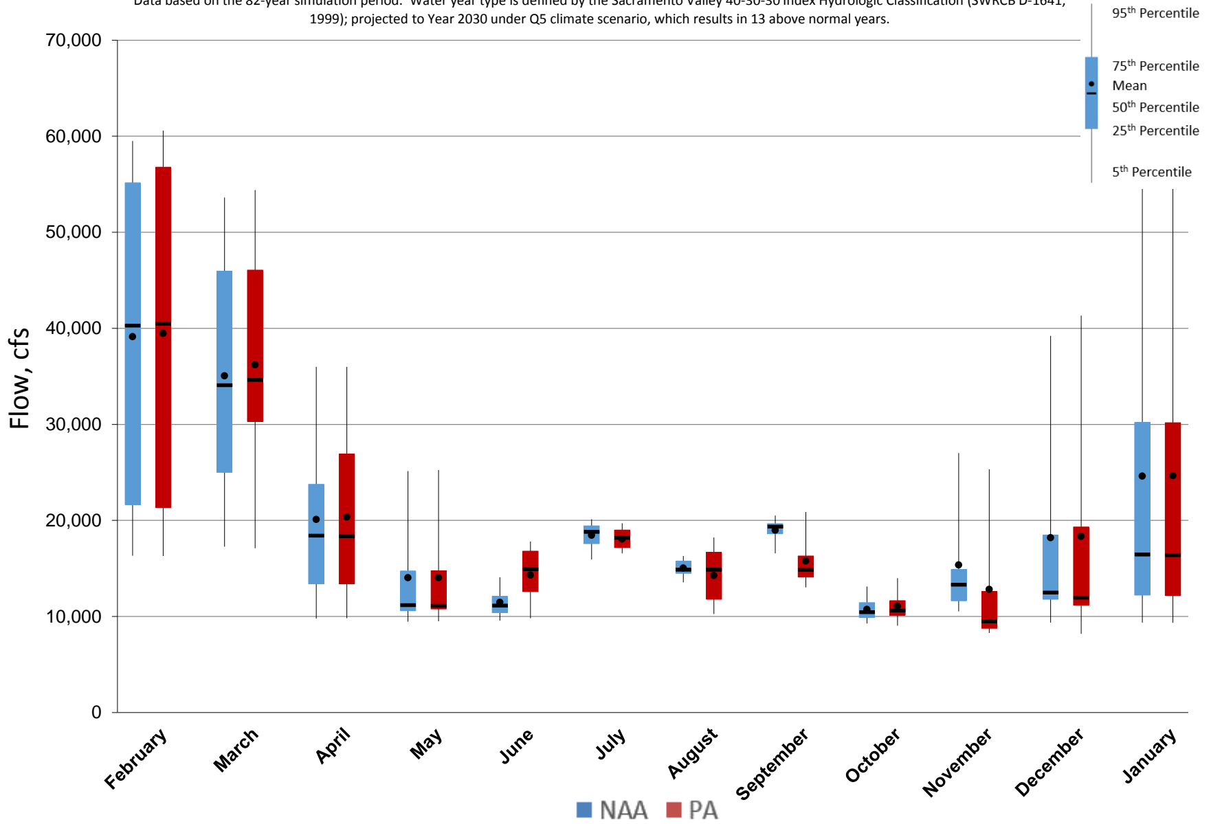
Figure 5.A.6-14-3. Monthly Flow Ranges For Sacramento River at Verona, Above Normal Years
