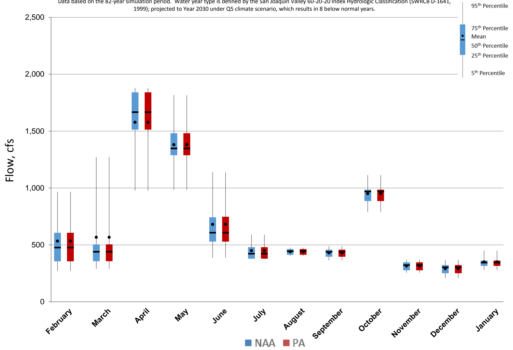
Figure 5.A.6-22-4. Monthly Flow Ranges for Stanislaus River at Mouth, Below Normal Years
