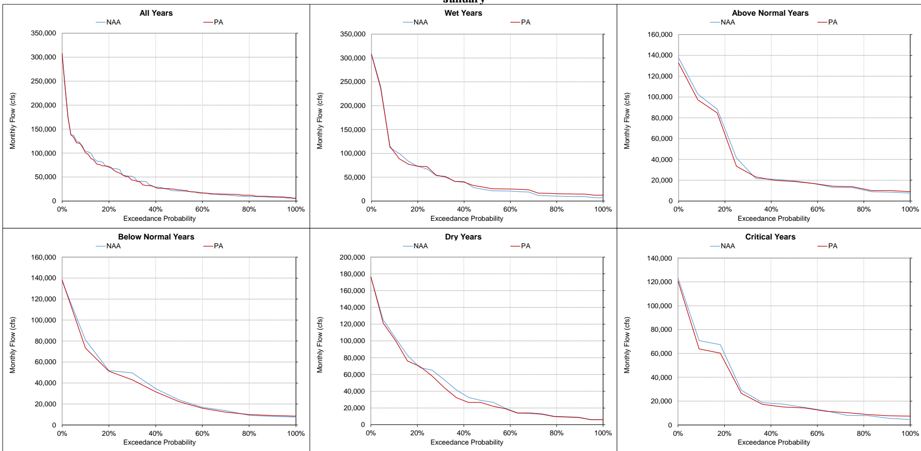
Figure 5.A.6-26-11. Delta Outflow, Monthly Flow January
