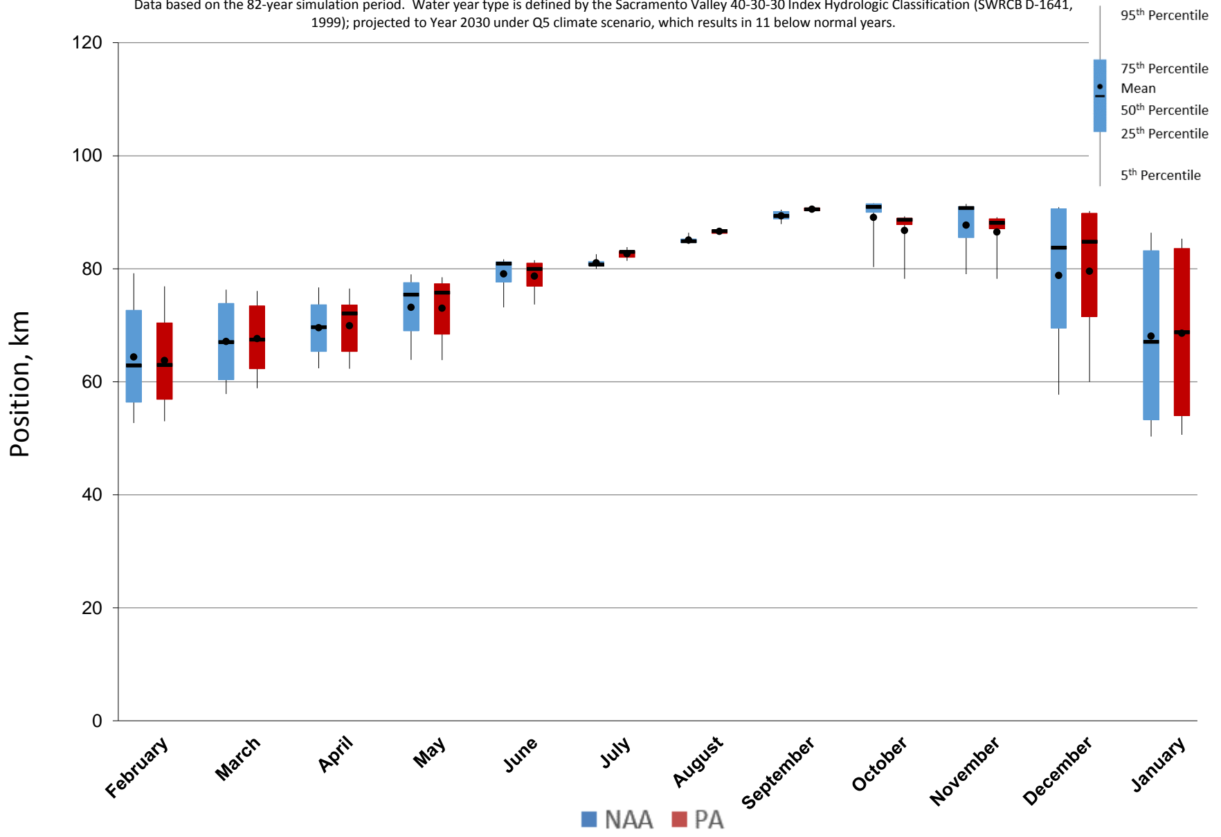
Figure 5.A.6-29-4. End of Month Position Ranges For X2, Below Normal Years
