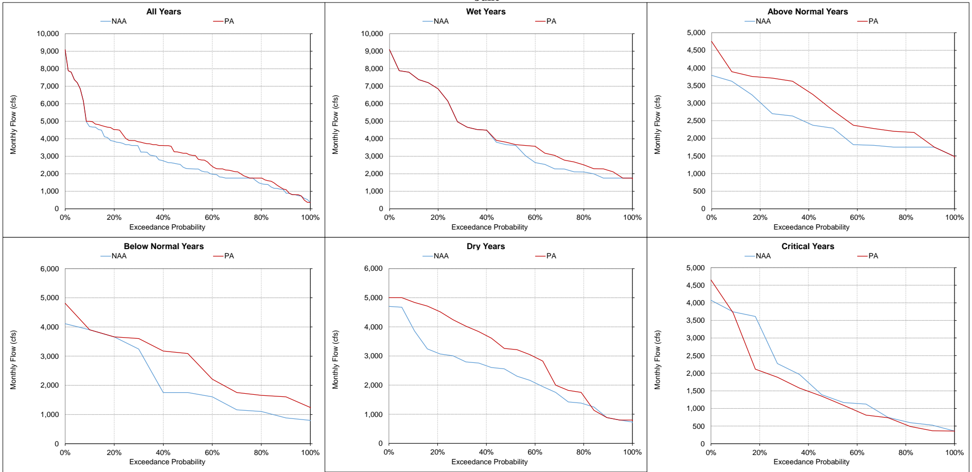
Figure 5.A.6-16-16. American River below Nimbus Dam, Monthly Flow June
