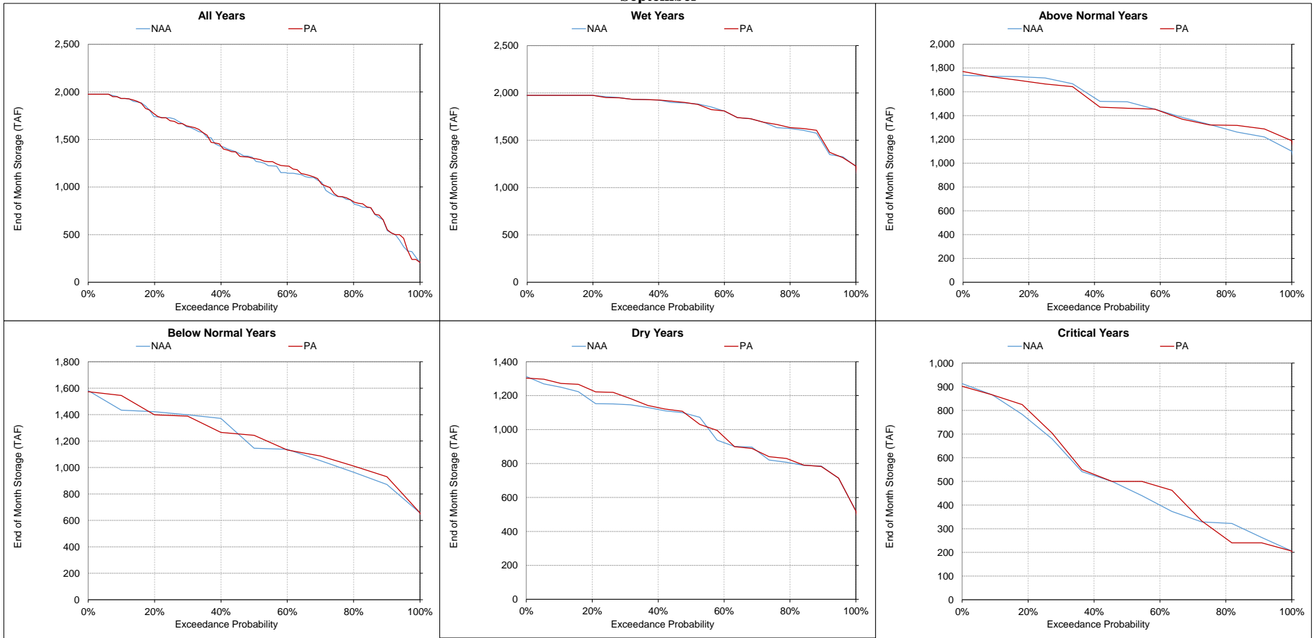
Figure 5.A.6-1-19. Trinity Lake, End of Month Storage September
