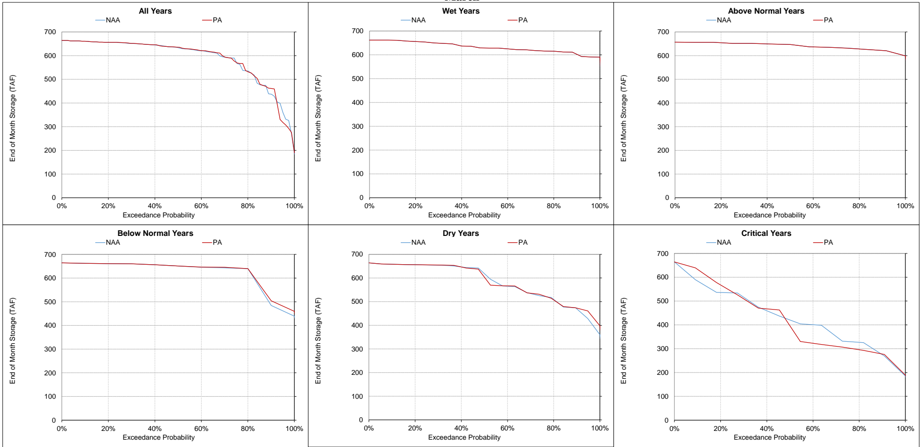
Figure 5.A.6-5-13. Folsom Lake, End of Month Storage March
