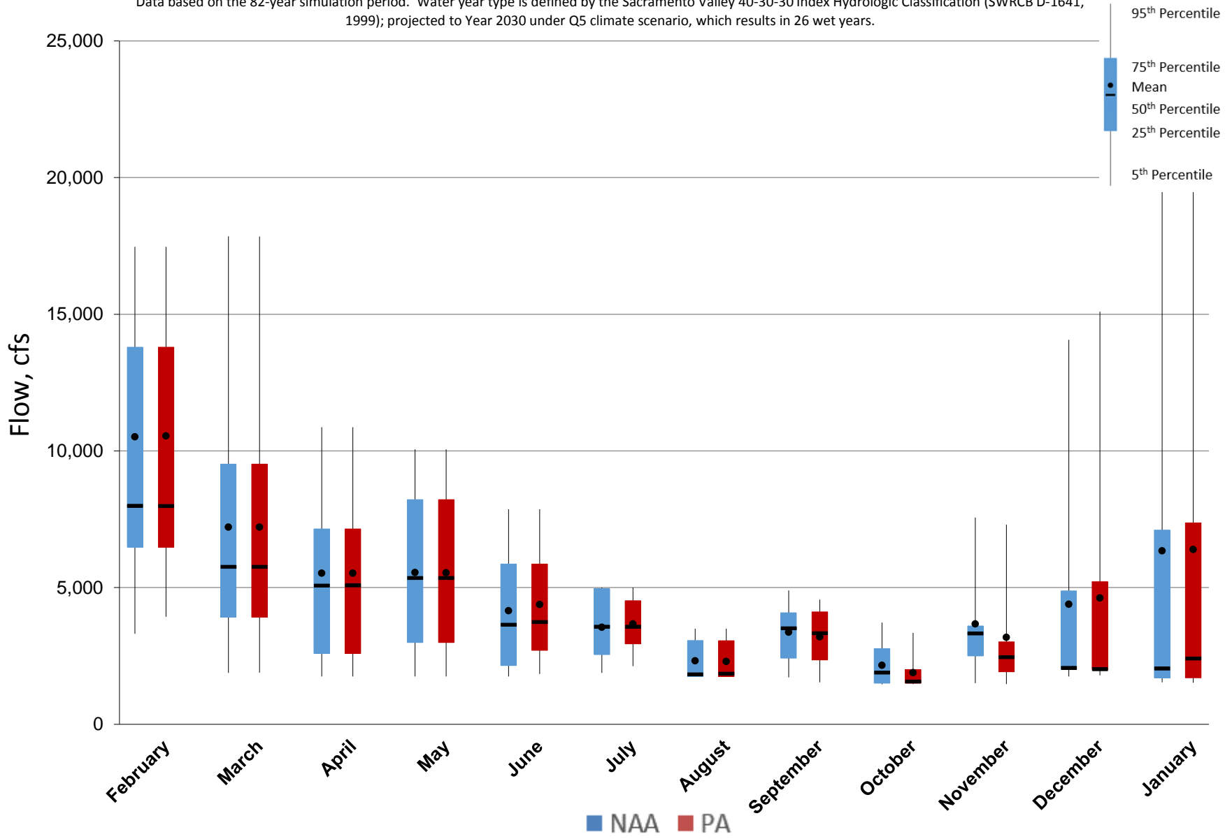
Figure 5.A.6-16-2. Monthly Flow Ranges For American River below Nimbus Dam, Wet Years
