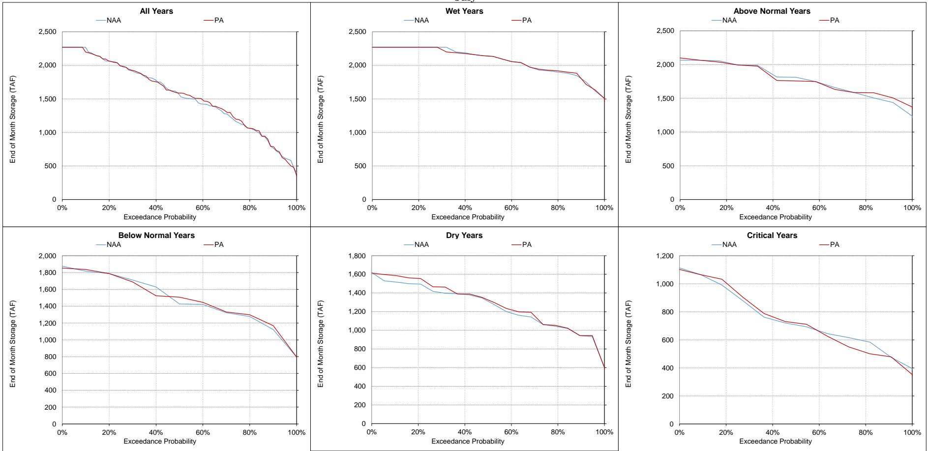
Figure 5.A.6-1-17. Trinity Lake, End of Month Storage July
