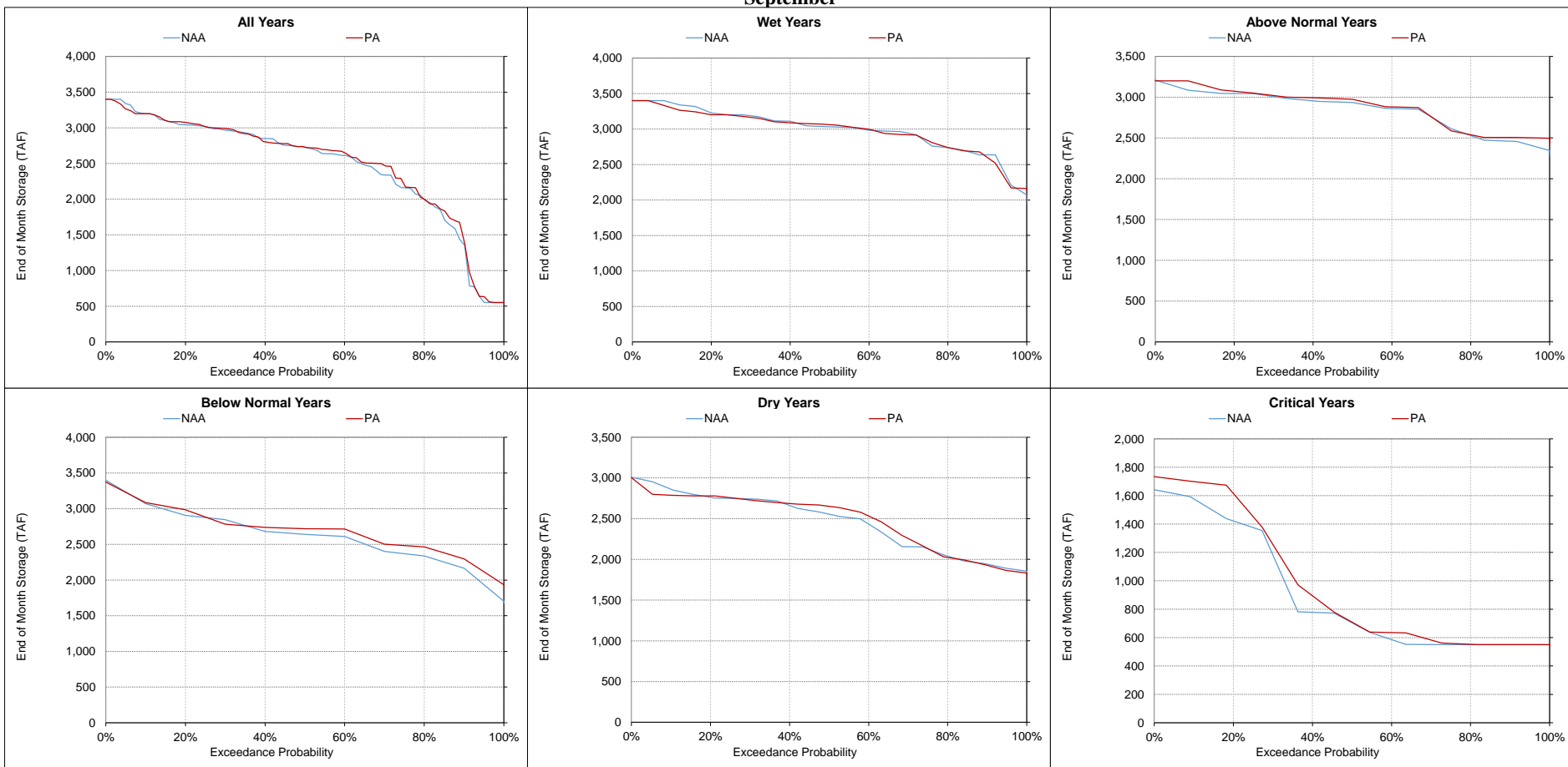
Figure 5.A.6-3-19. Shasta Lake, End of Month Storage September
