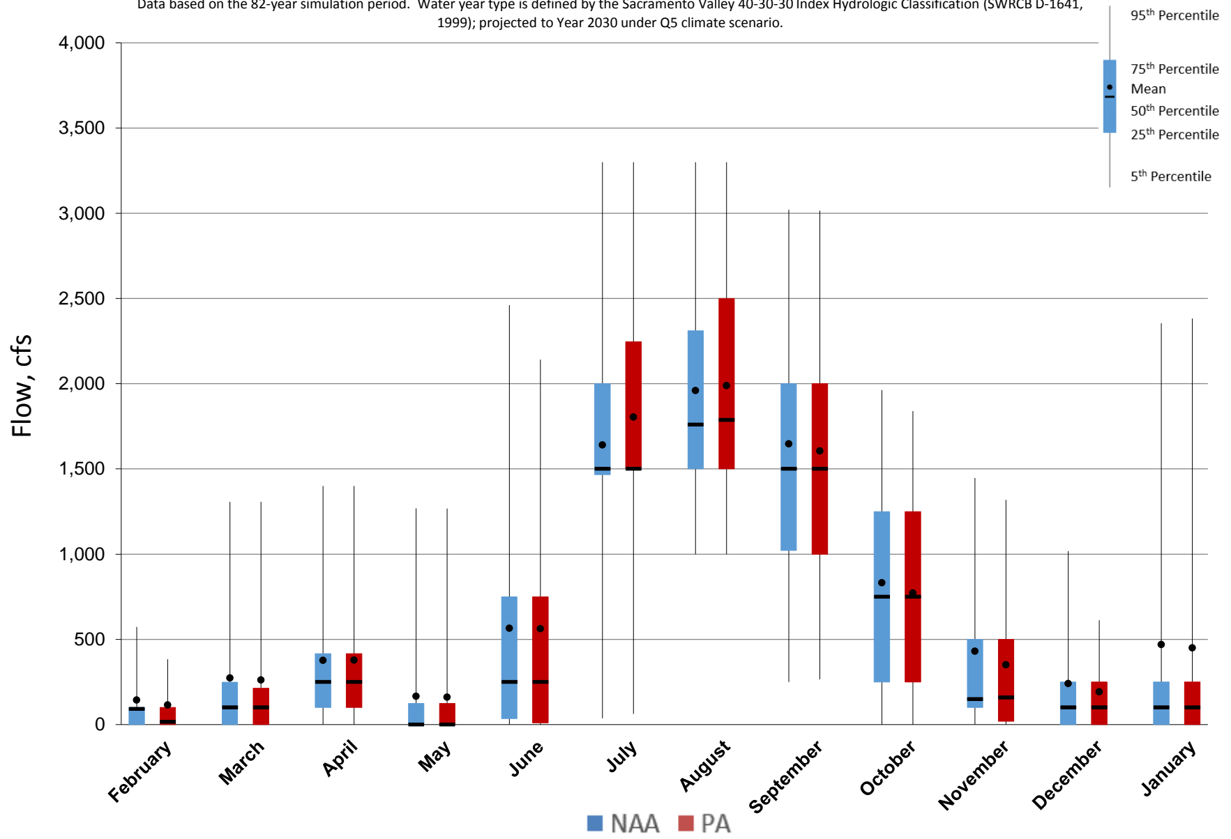
Figure 5.A.6-8-1. Monthly Flow Ranges For Clear Creek Tunnel Flow, All Years
