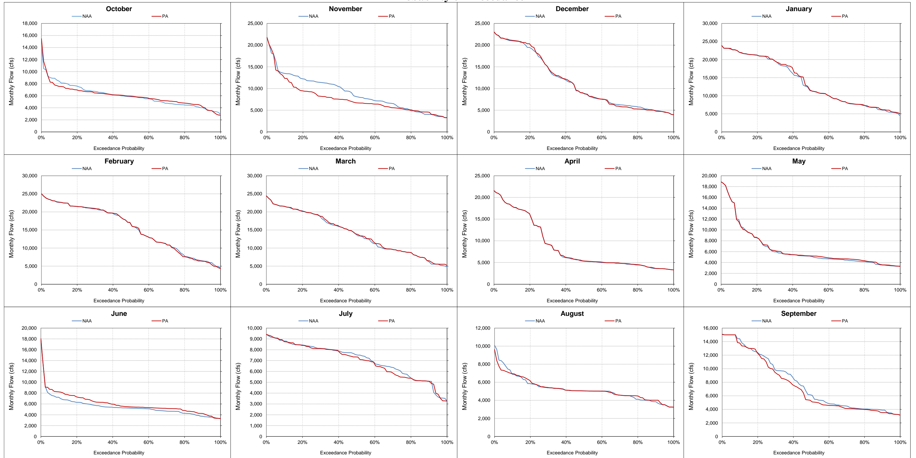
Figure 5.A.6-11-7. Sacramento River at Bend Bridge, Monthly Flow Probability of Exceedance
