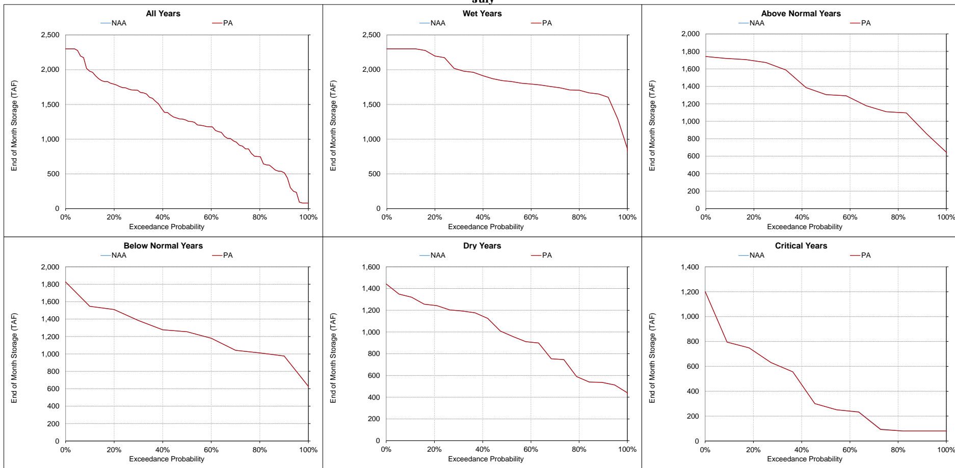
Figure 5.A.6-17. New Melones Lake, End of Month Storage July
