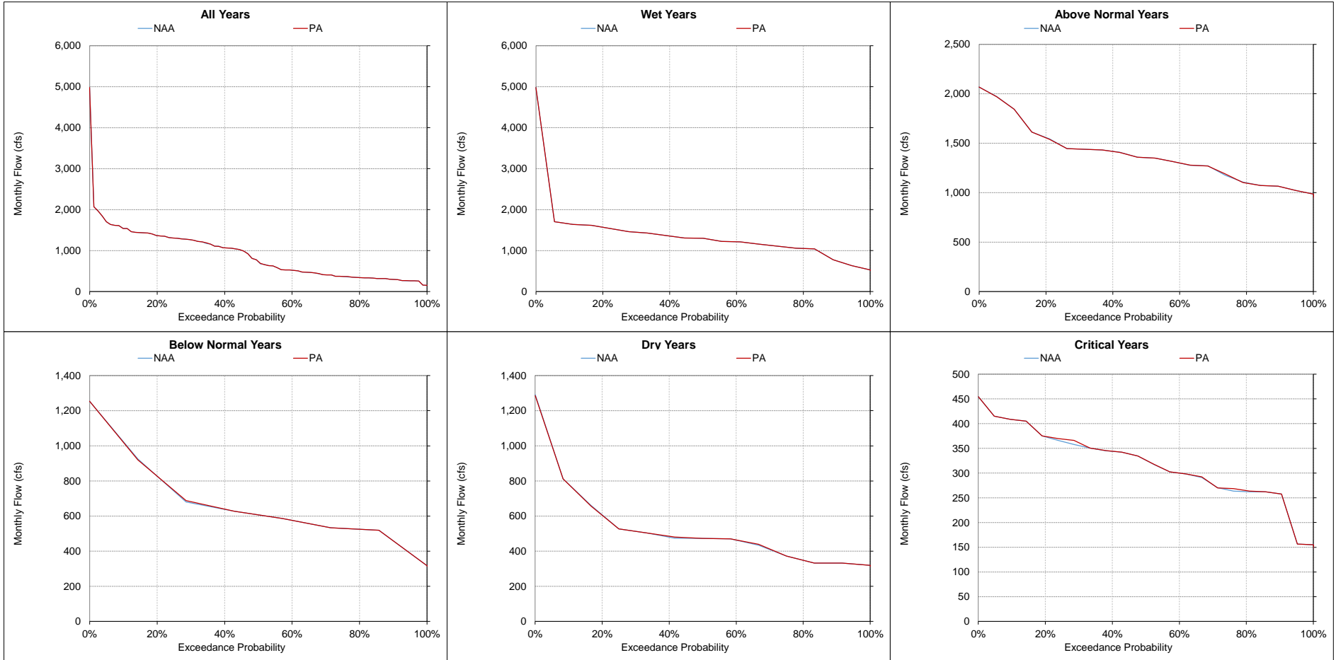
Figure 5.A.6-22-16. Stanislaus River at Mouth, Monthly Flow
