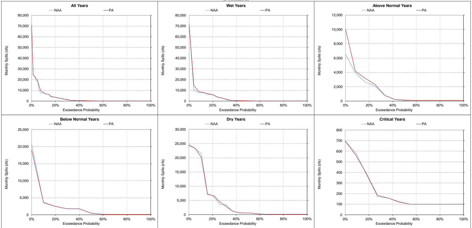
Figure 5.A.6-15-10. Fremont Weir, Monthly Spills December
