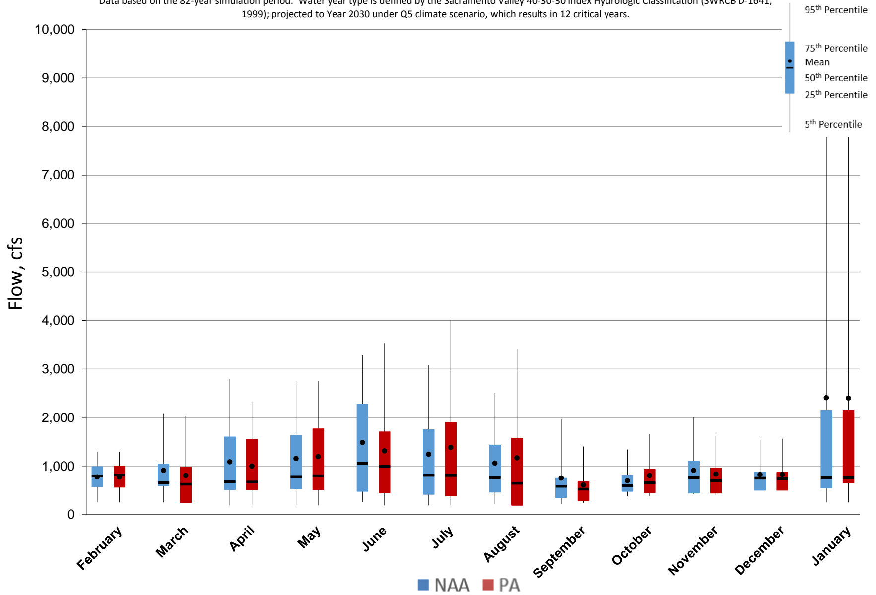
Figure 5.A.6-17-6. Monthly Flow Ranges For American River at Sacramento River Confluence, Critical Years
