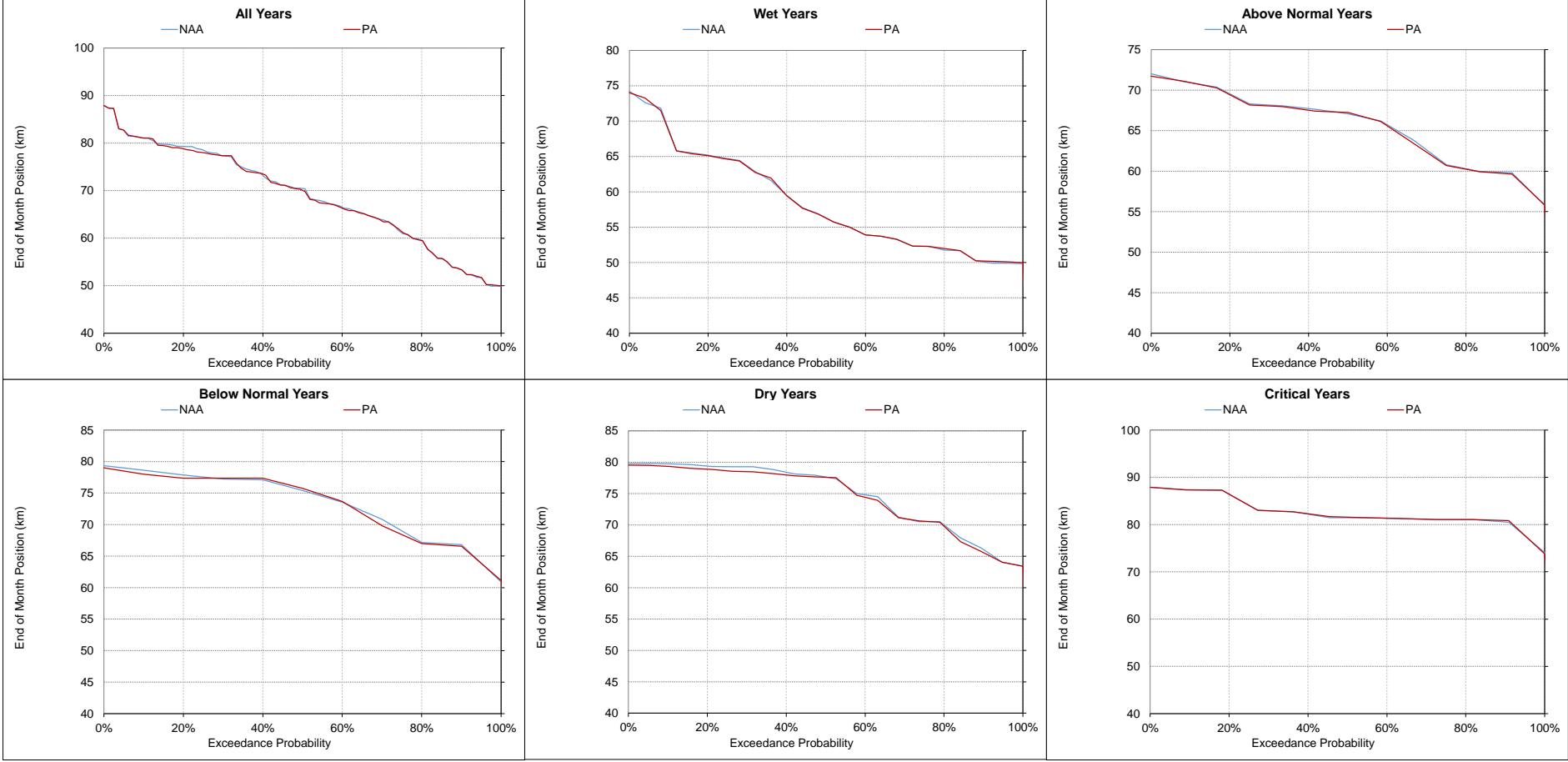
Figure 5.A.6-29-15. X2, End of Month Position May
