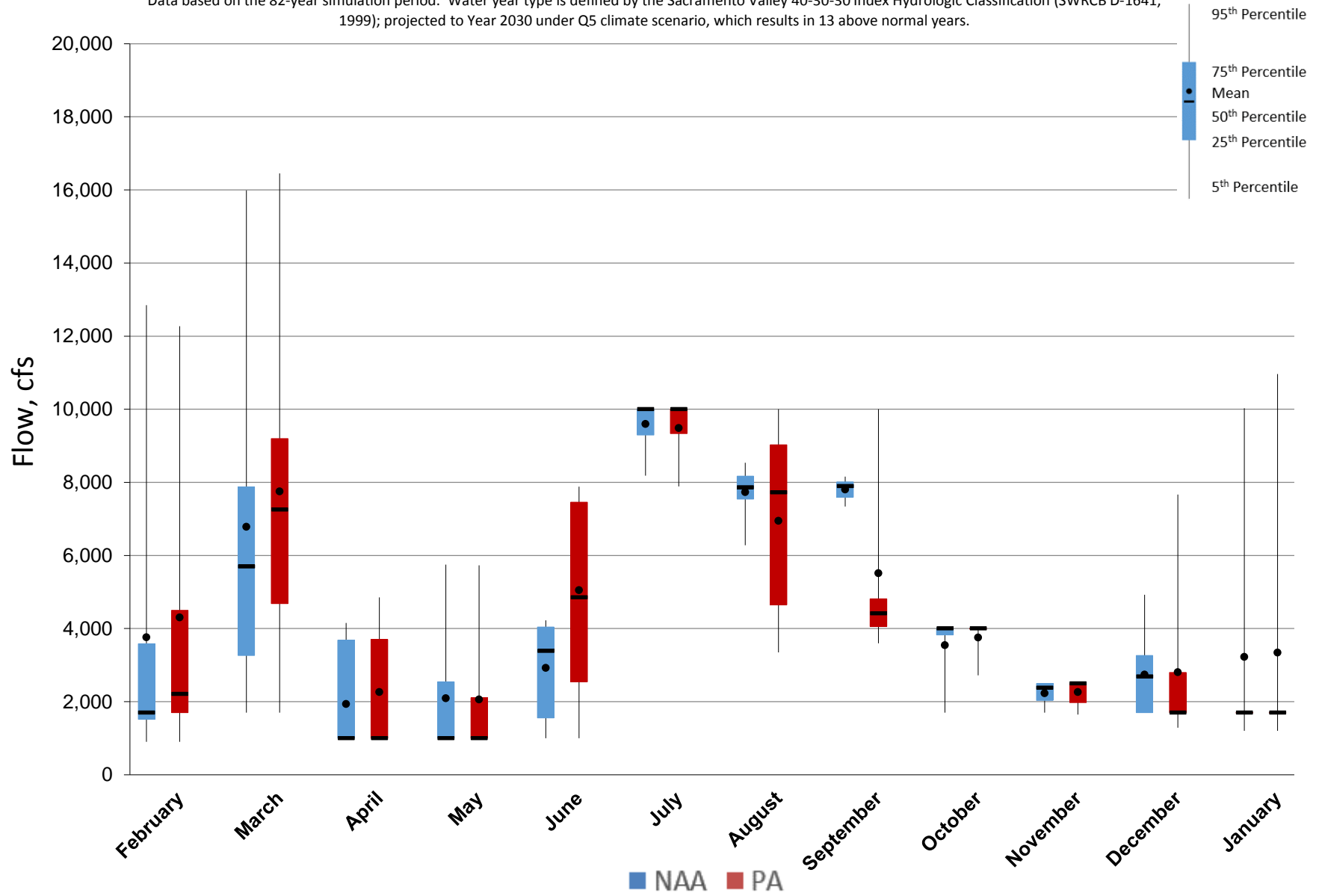
Figure 5.A.6-12-3. Monthly Flow Ranges For Feather River below Thermalito Diversion Dam, Above Normal Years
