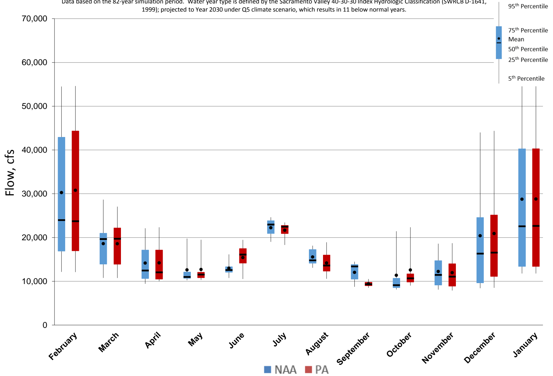
Figure 5.A.6-18-4. Monthly Flow Ranges For Sacramento River at Freeport, Below Normal Years
