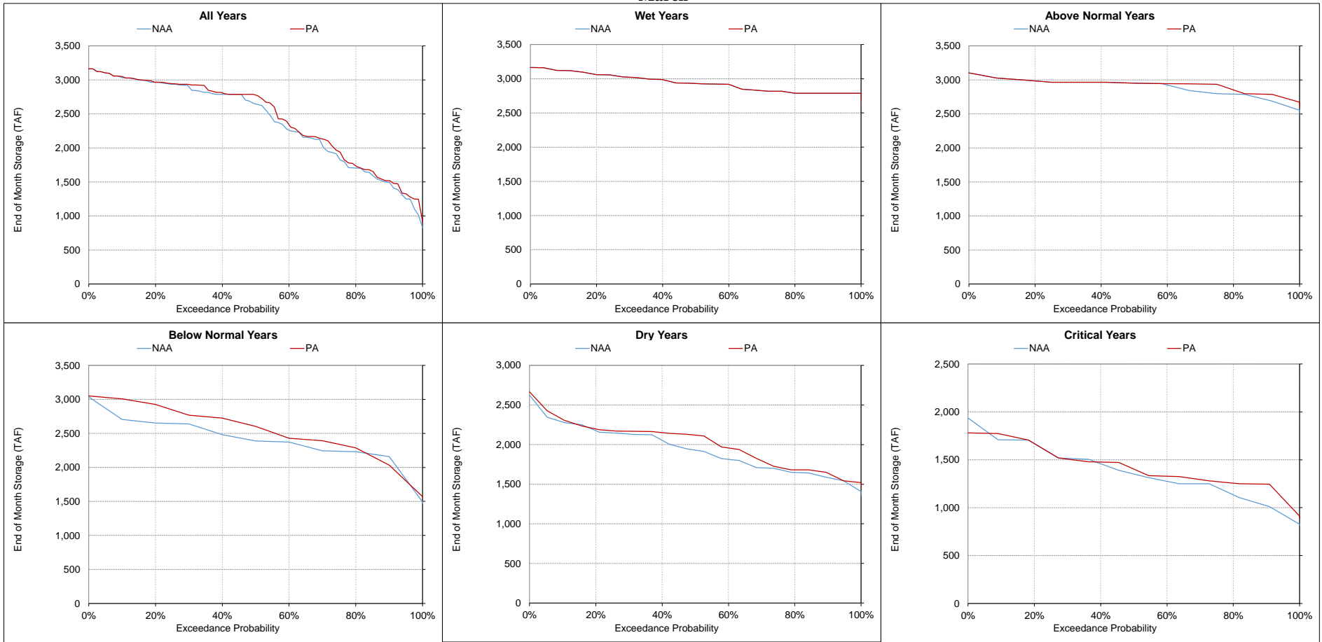
Figure 5.A.6-4-13. Lake Oroville, End of Month Storage March
