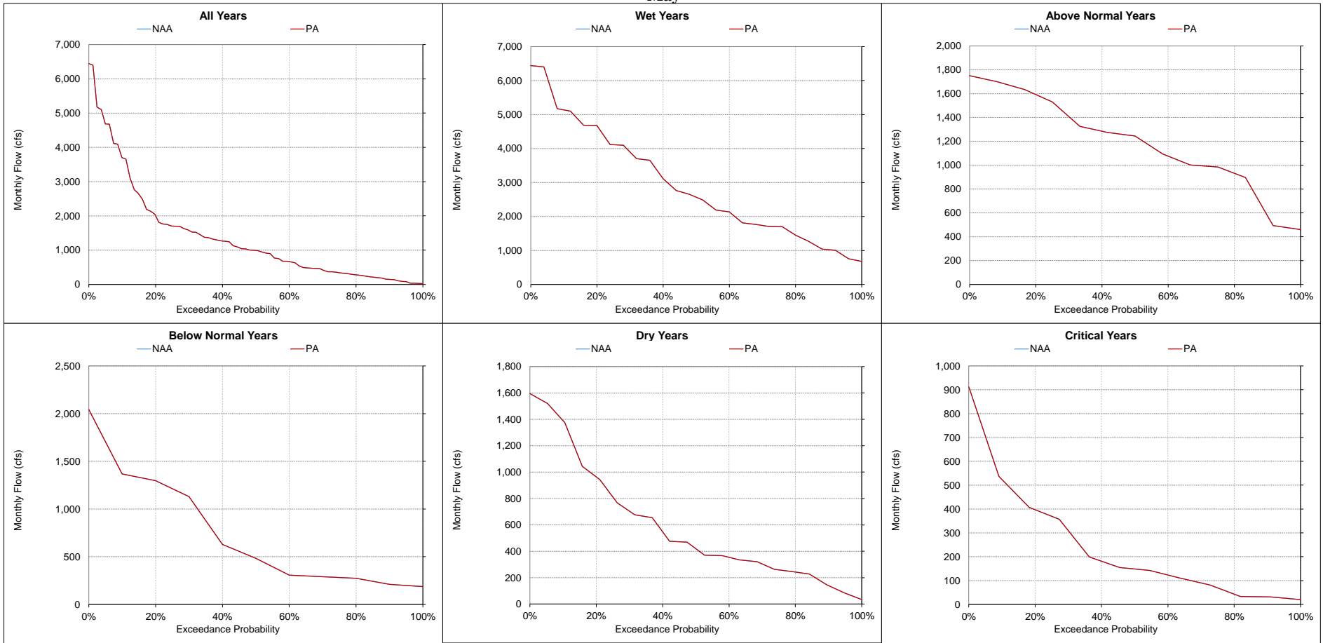
Figure 5.A.6-24-15. Mokelumne and Cosumnes River, Monthly Flow May
