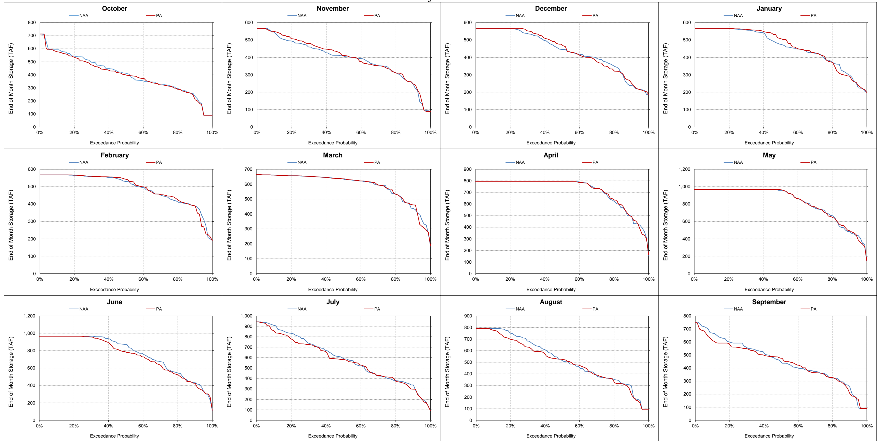
Figure 5.A.6-5-7. Folsom Lake, End of Month Storage Probability of Exceedance
