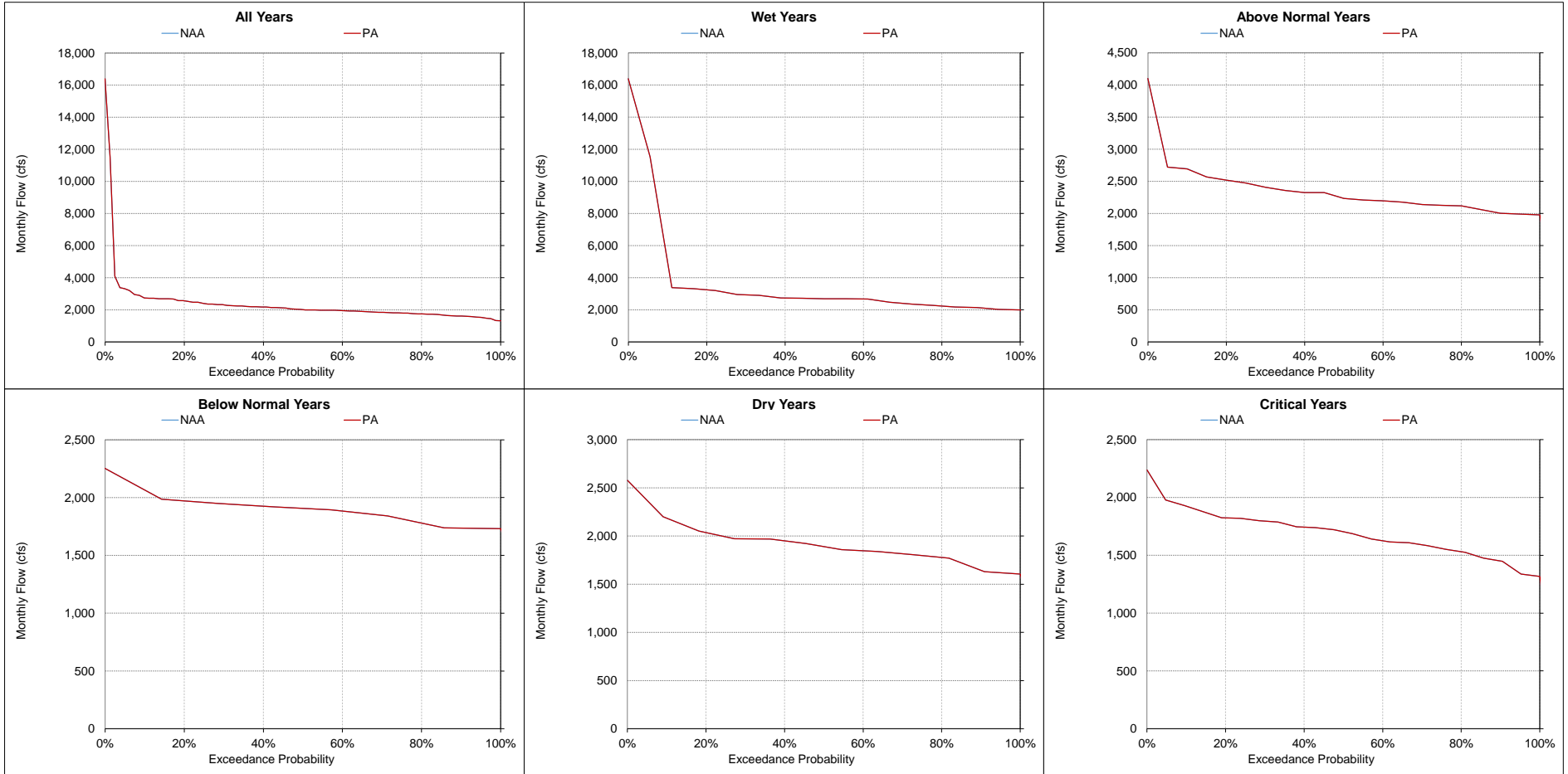
Figure 5.A.6-23-9. San Joaquin River at Vernalis, Monthly Flow November
