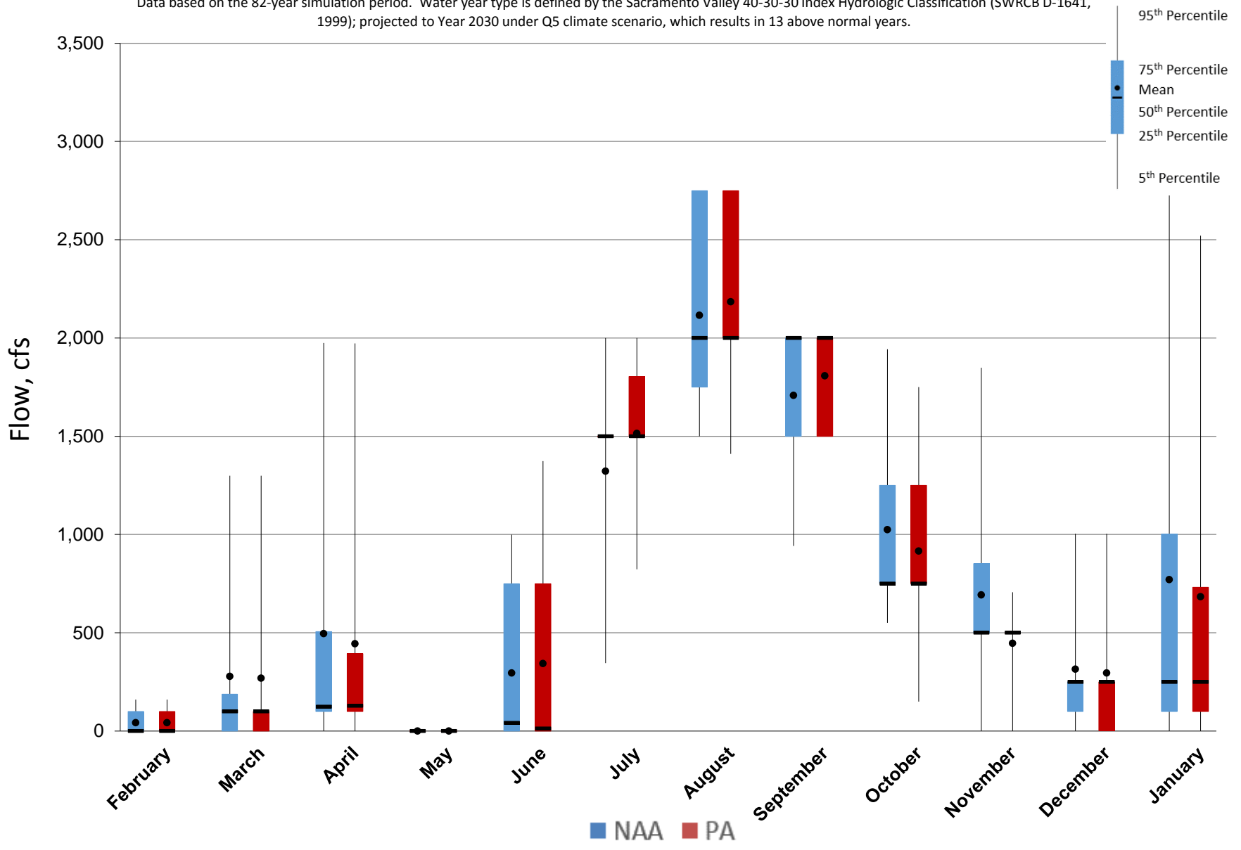
Figure 5.A.6-8-3. Monthly Flow Ranges For Clear Creek Tunnel Flow, Above Normal Years
