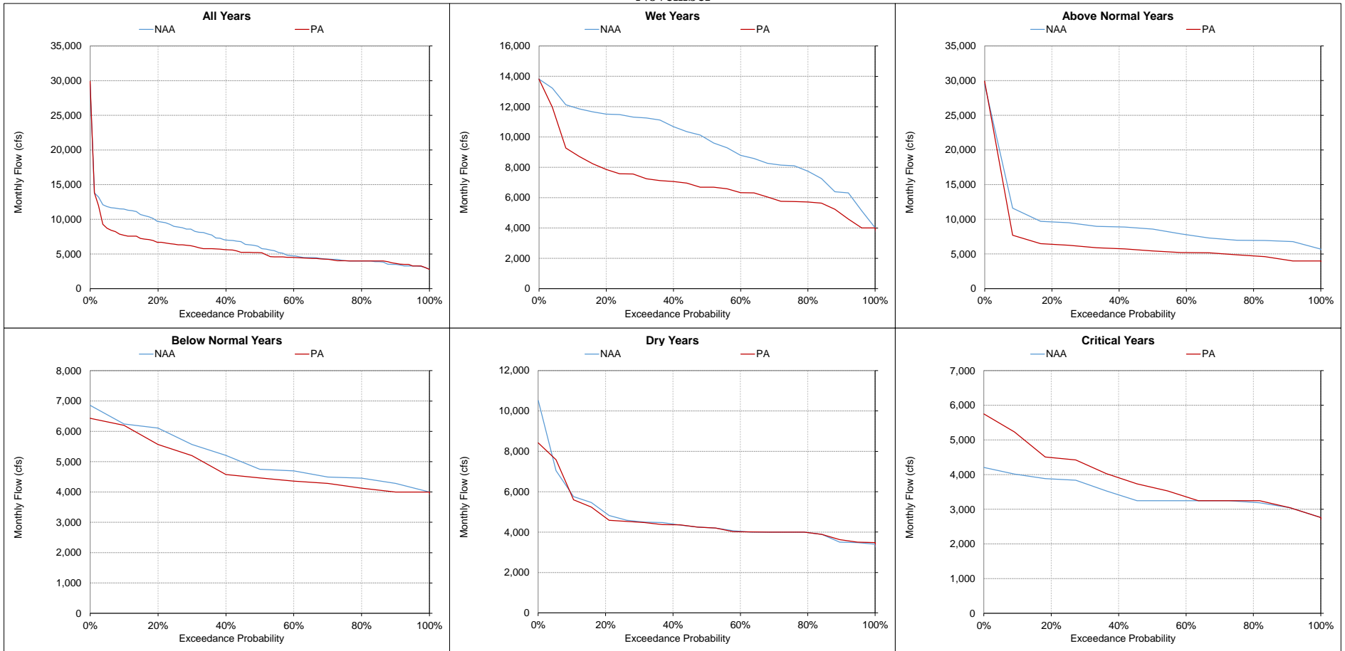
Figure 5.A.6-10-9. Sacramento River below Keswick Dam, Monthly Flow November
