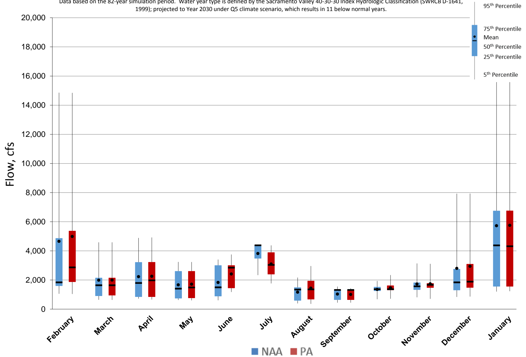
Figure 5.A.6-17-4. Monthly Flow Ranges For American River at Sacramento River Confluence, Below Normal Years
