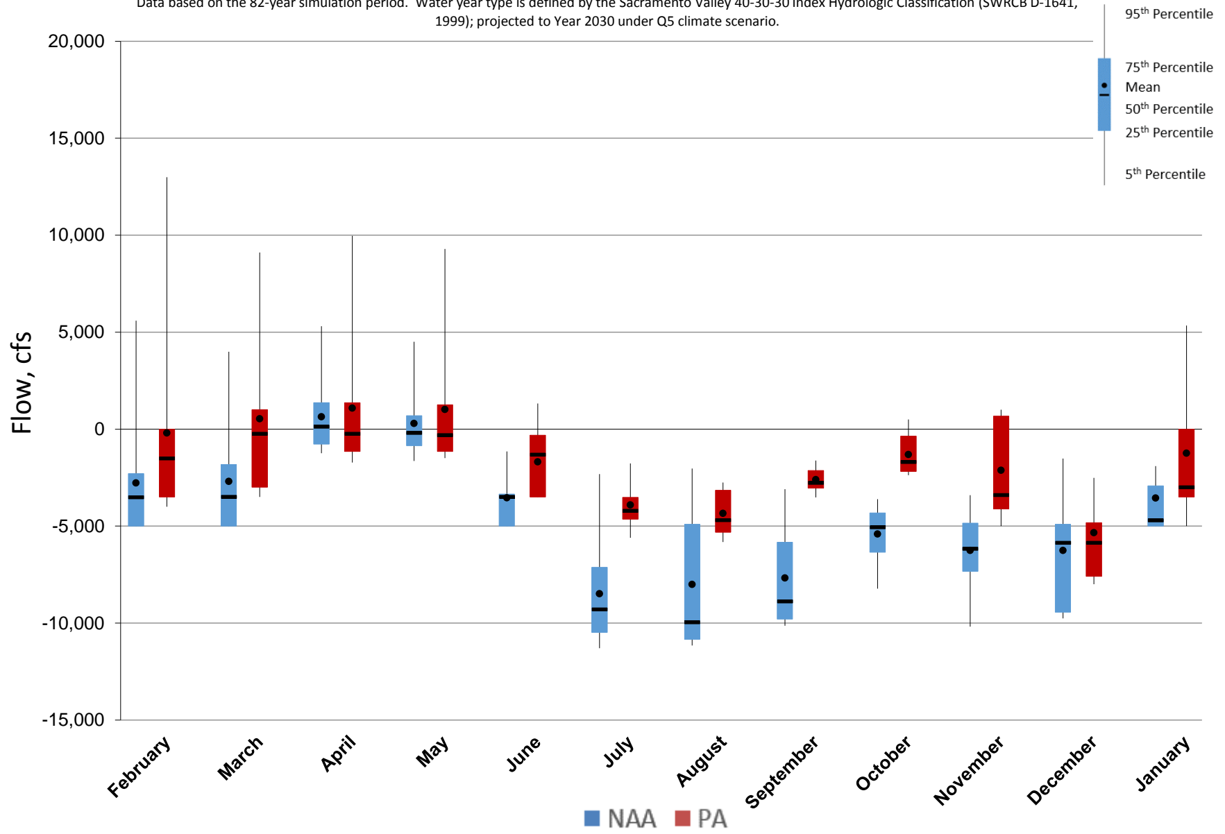
Figure 5.A.6-25-1. Monthly Flow Ranges For Old and Middle River, All Years
