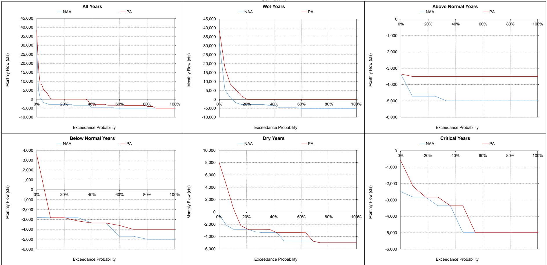
Figure 5.A.6-25-11. Old and Middle River, Monthly Flow January
