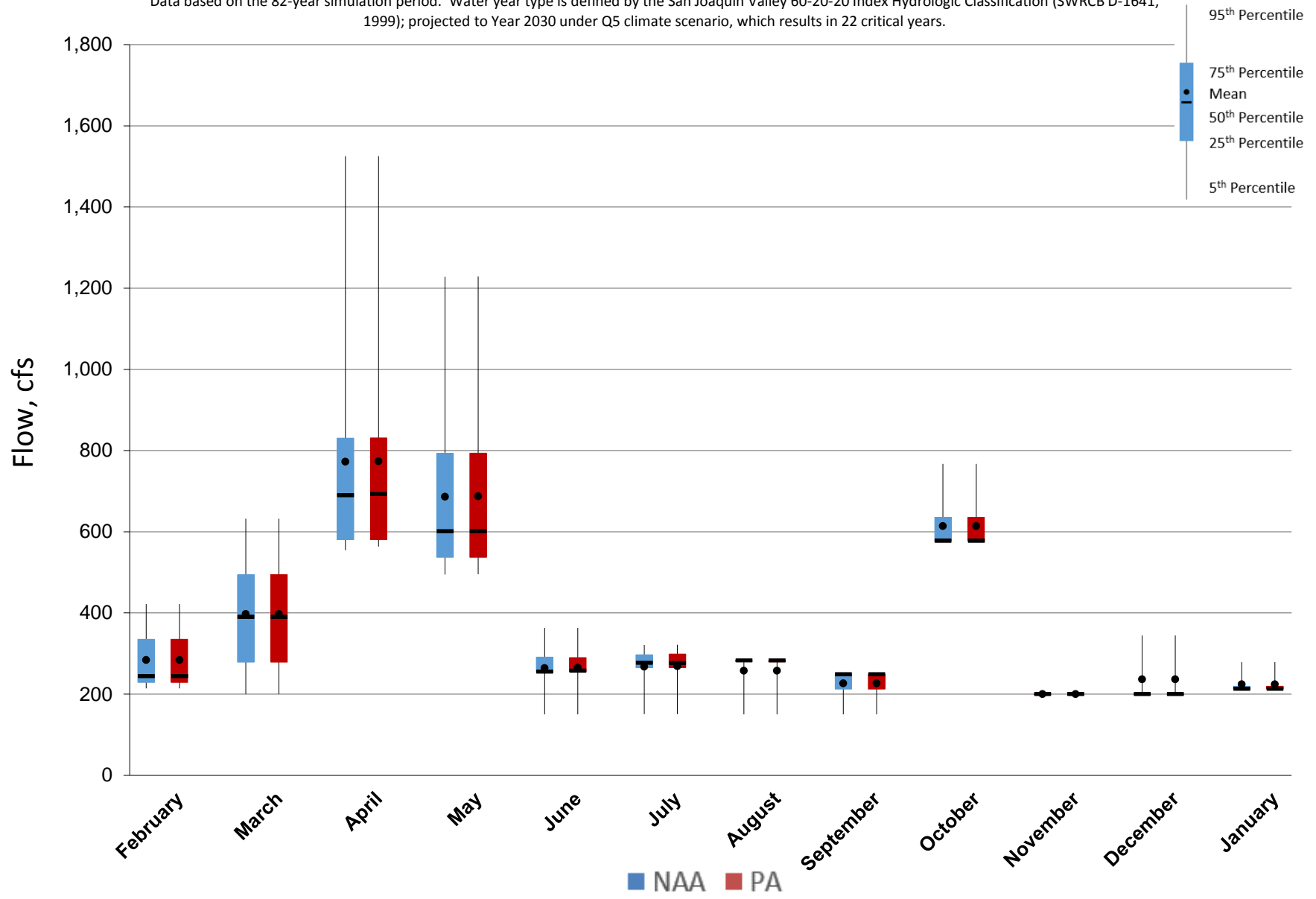
Figure 5.A.6-21-6. Monthly Flow Ranges for Stanislaus River at Ripon, Critical Years
