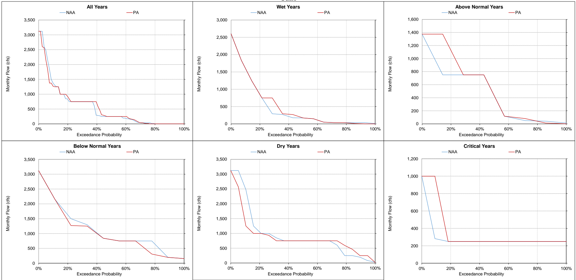
Figure 5.A.6-8-16. Clear Creek Tunnel Flow, Monthly Flow June
