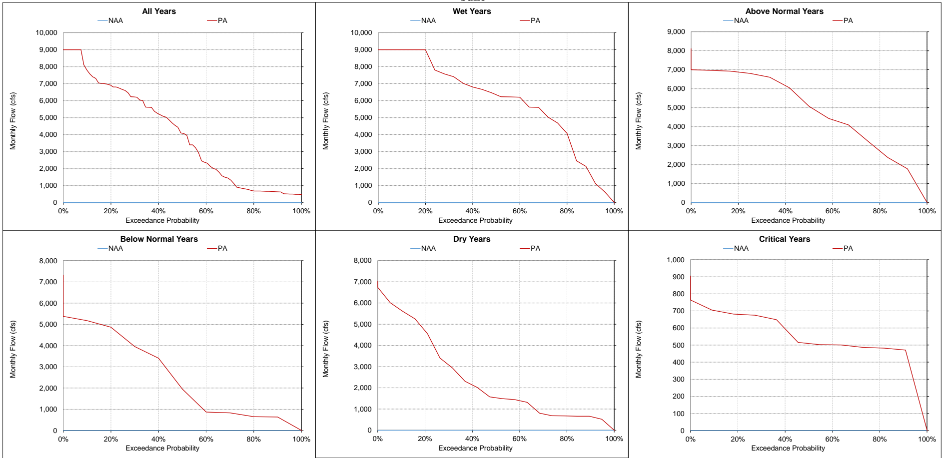
Figure 5.A.6-19-16. North Delta Diversions near Hood, Monthly Flow June
