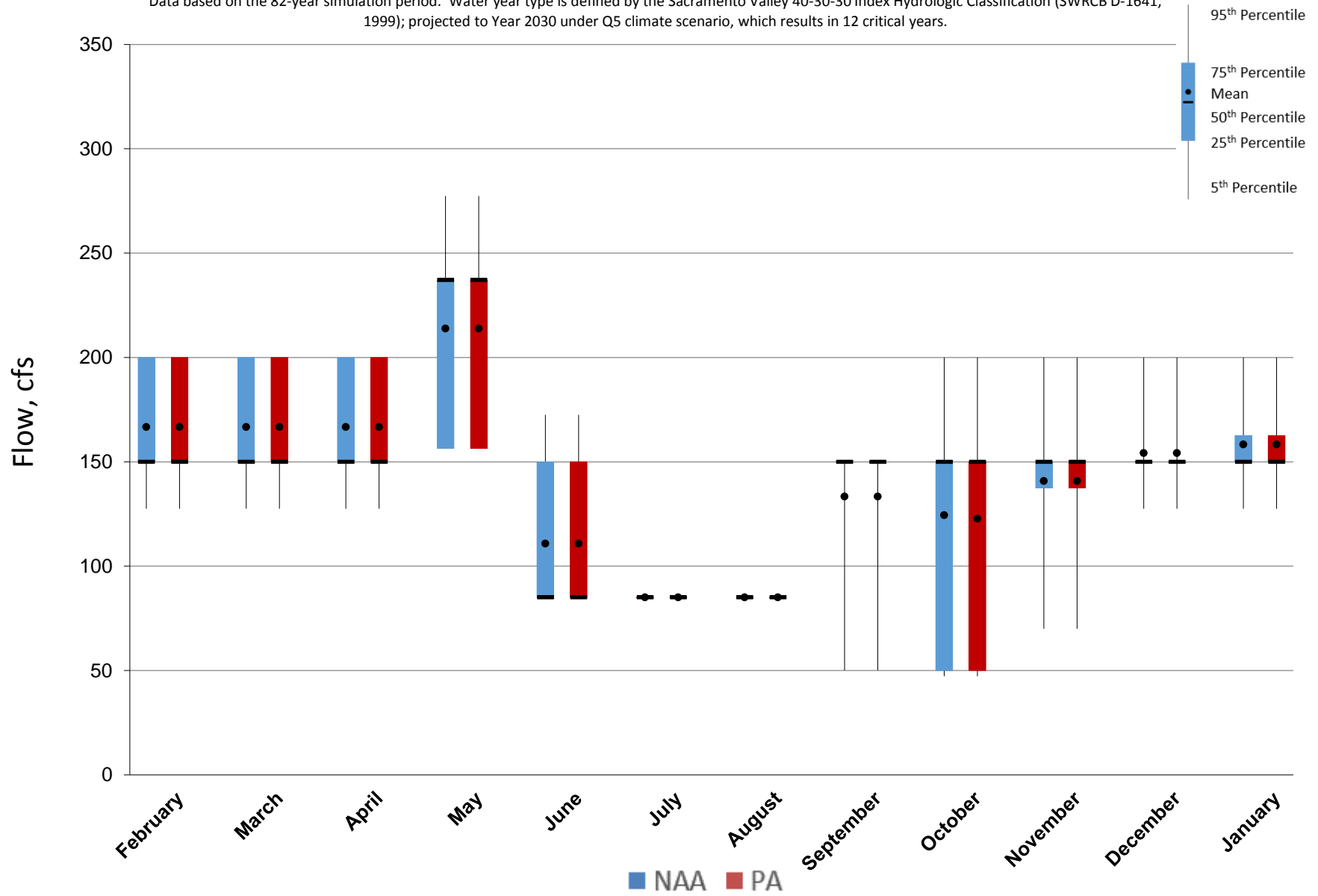
Figure 5.A.6-9-6. Monthly Flow Ranges For Clear Creek below Whiskeytown Dam, Critical Years
