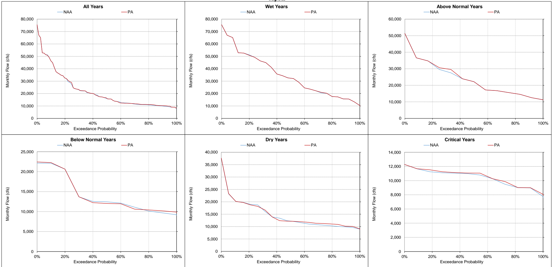
Figure 5.A.6-18-14. Sacramento River at Freeport, Monthly Flow April
