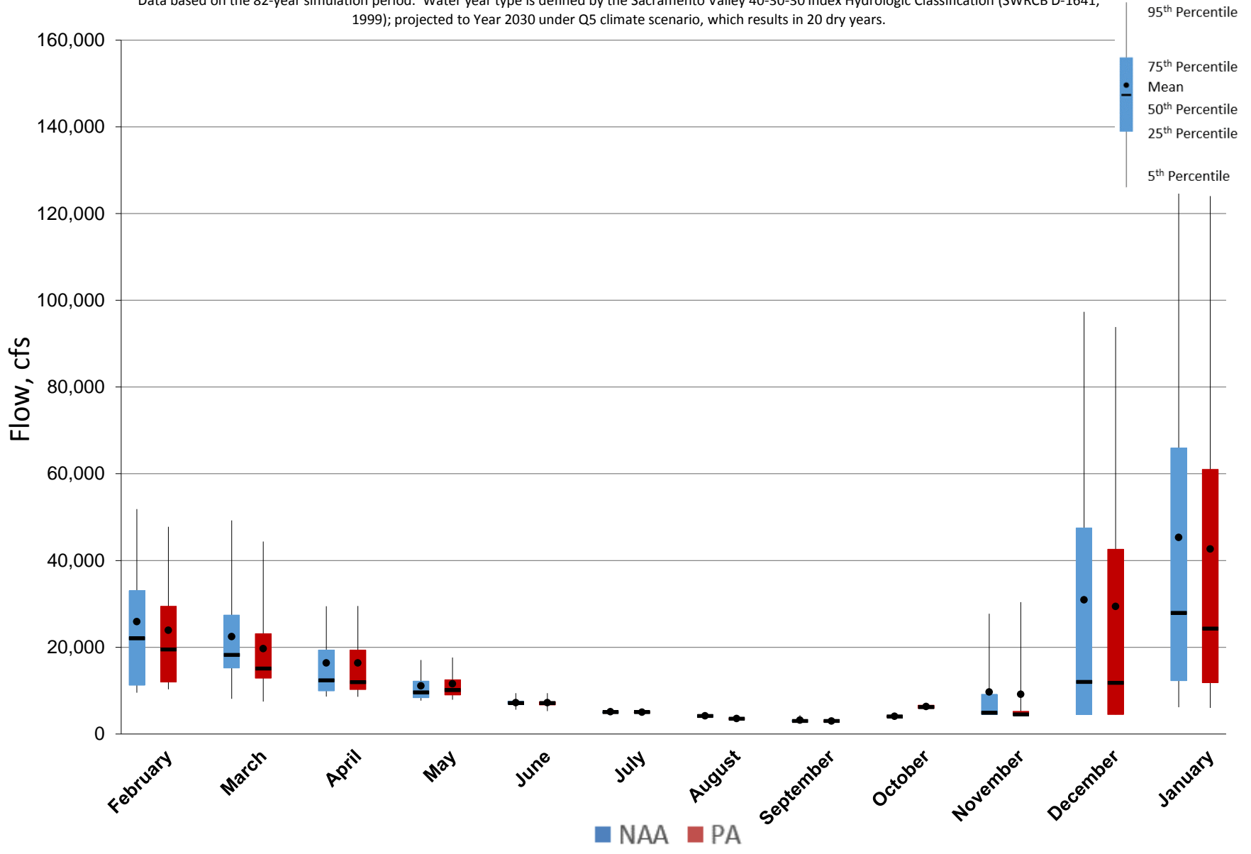
Figure 5.A.6-26-5. Monthly Flow Ranges For Delta Outflow, Dry Years
