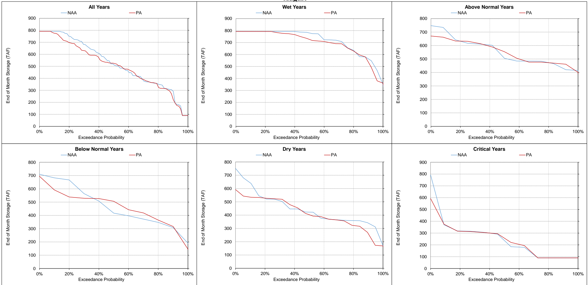
Figure 5.A.6-5-18. Folsom Lake, End of Month Storage August
