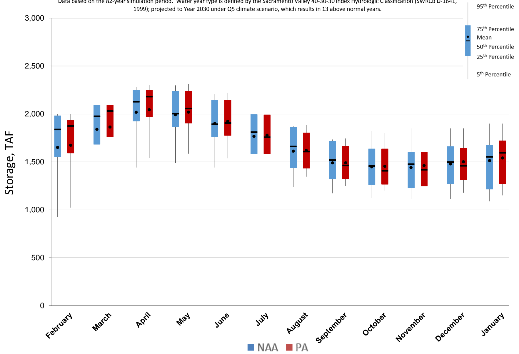
Figure 5.A.6-1-3. End of Month Storage Ranges For Trinity Lake, Above Normal Years
