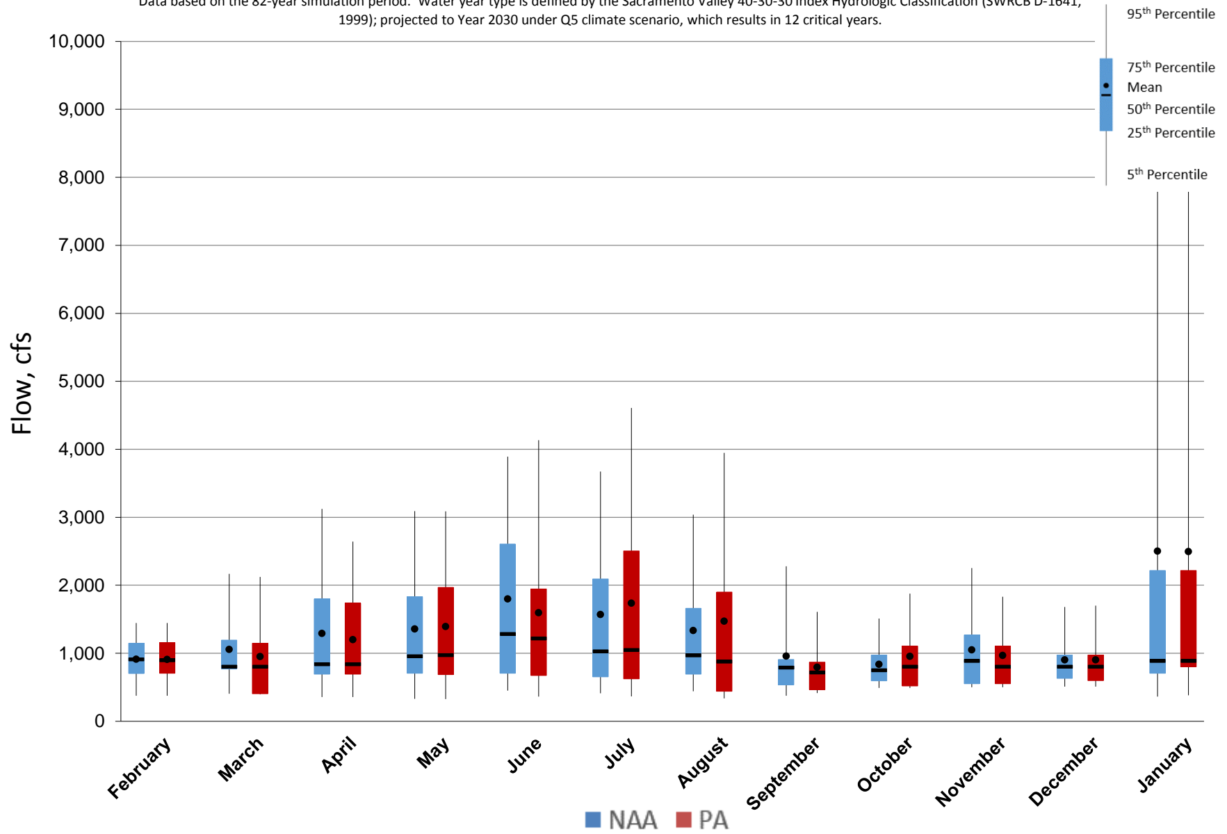
Figure 5.A.6-16-6. Monthly Flow Ranges For American River below Nimbus Dam, Critical Years
