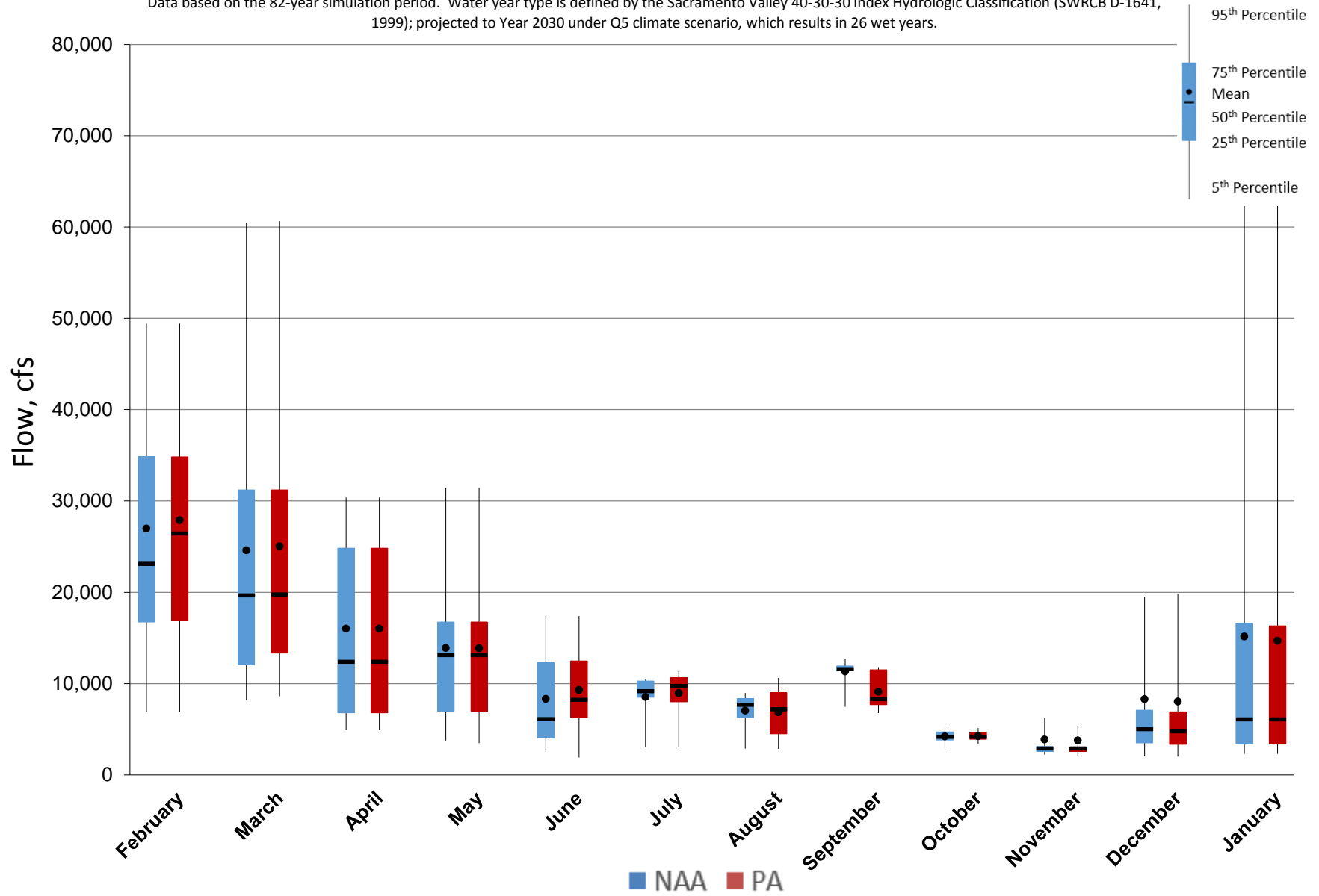
Figure 5.A.6-13-2. Monthly Flow Ranges For Feather River at Sacramento River Confluence, Wet Years
