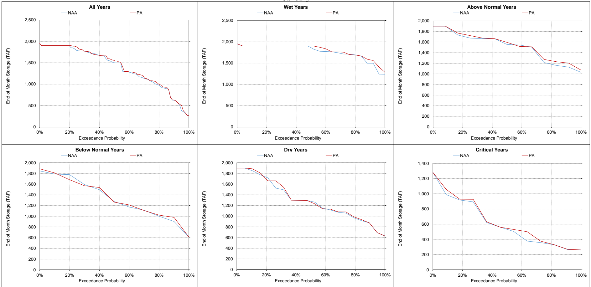
Figure 5.A.6-1-11. Trinity Lake, End of Month Storage January
