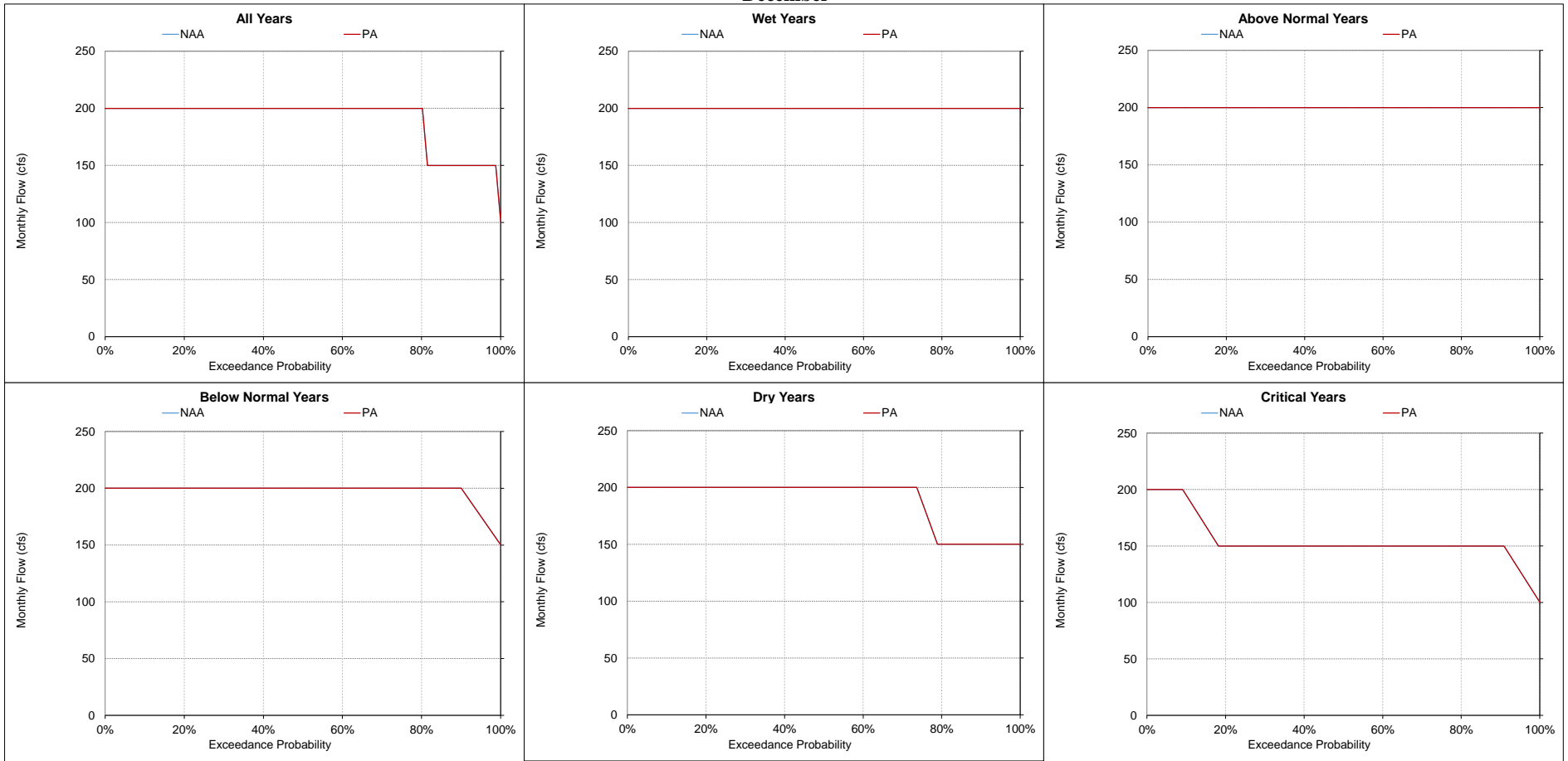
Figure 5.A.6-9-10. Clear Creek below Whiskeytown Dam, Monthly Flow December
