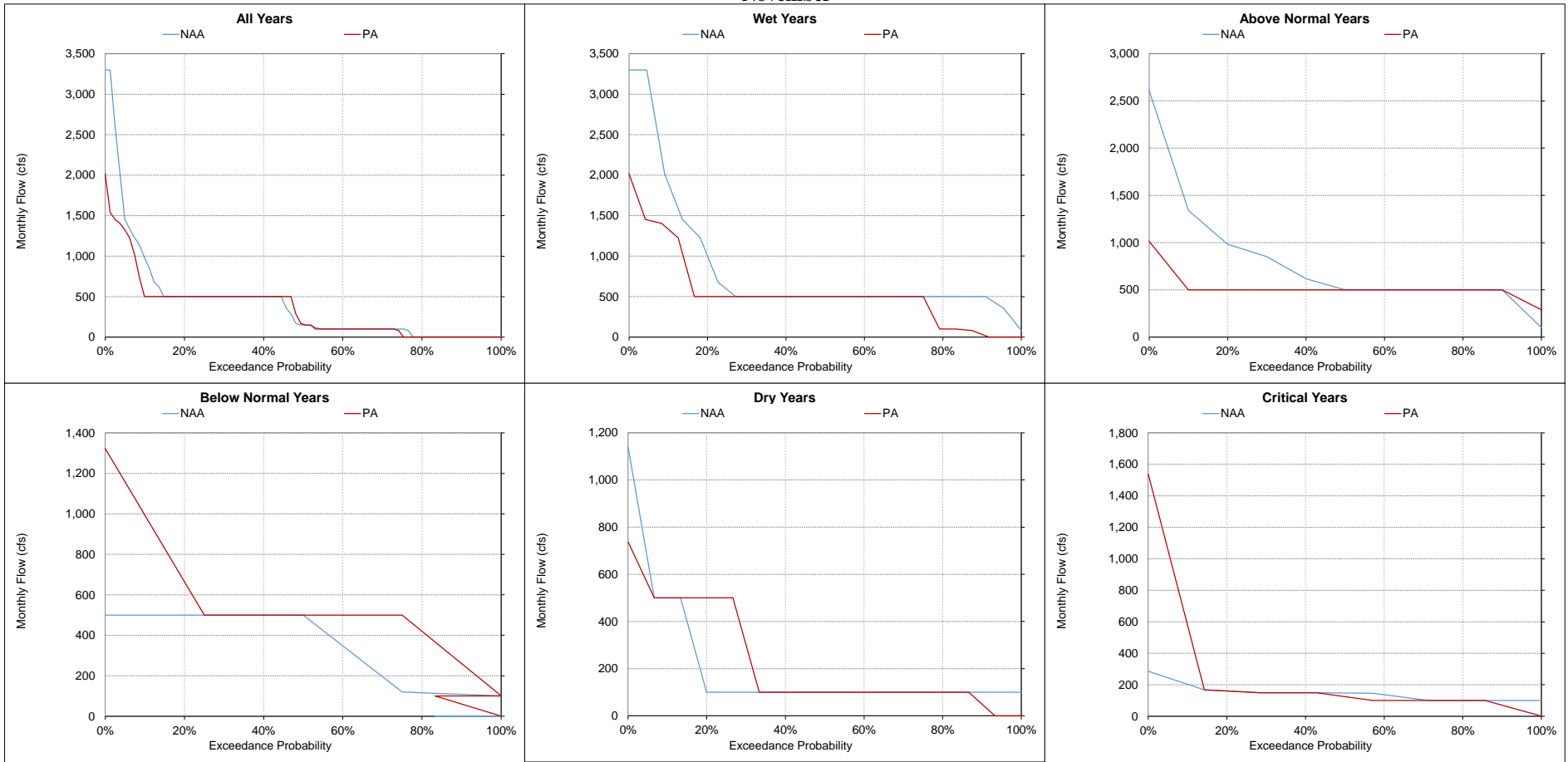
Figure 5.A.6-8-9. Clear Creek Tunnel Flow, Monthly Flow November
