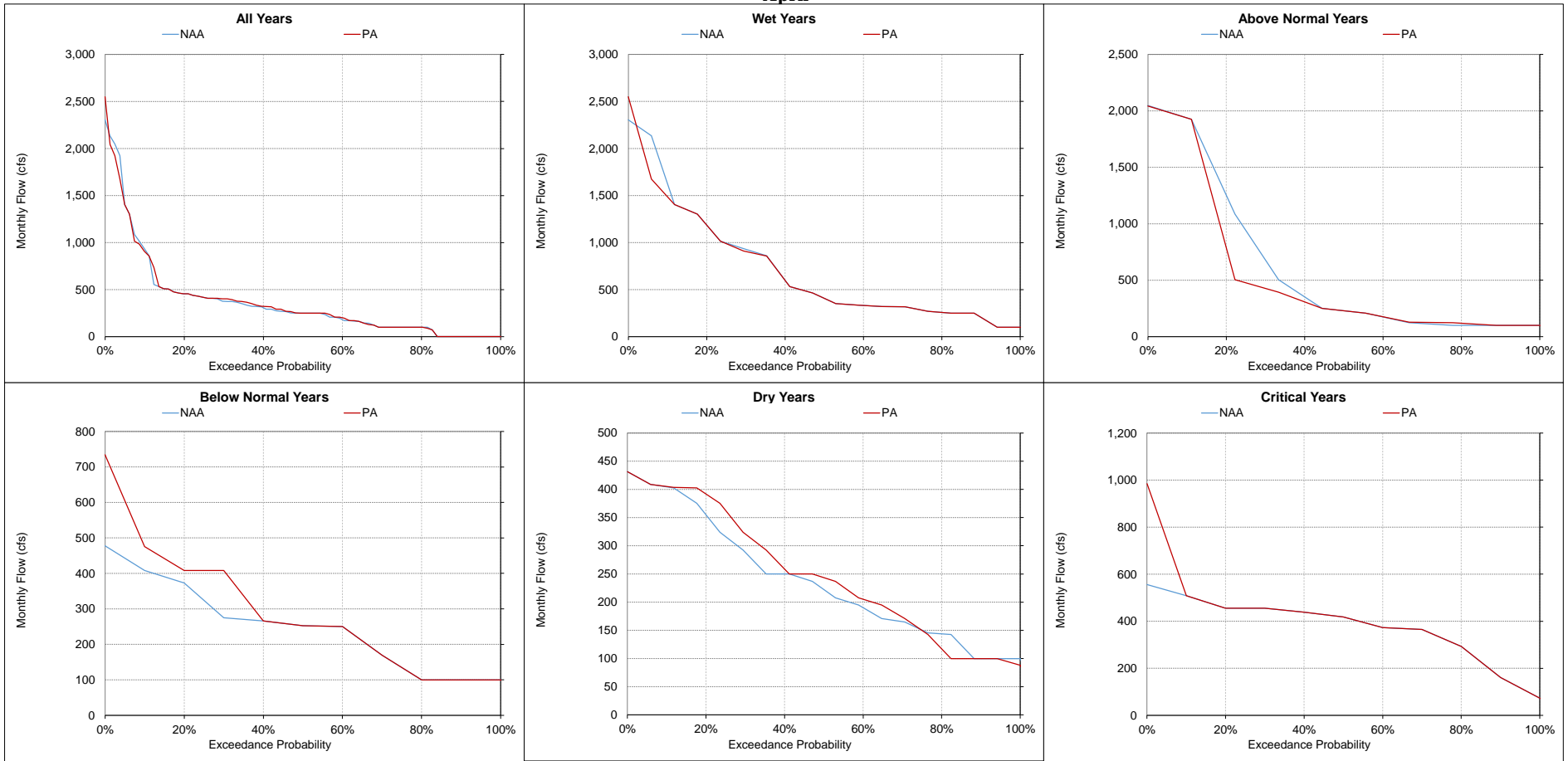
Figure 5.A.6-8-14. Clear Creek Tunnel Flow, Monthly Flow April
