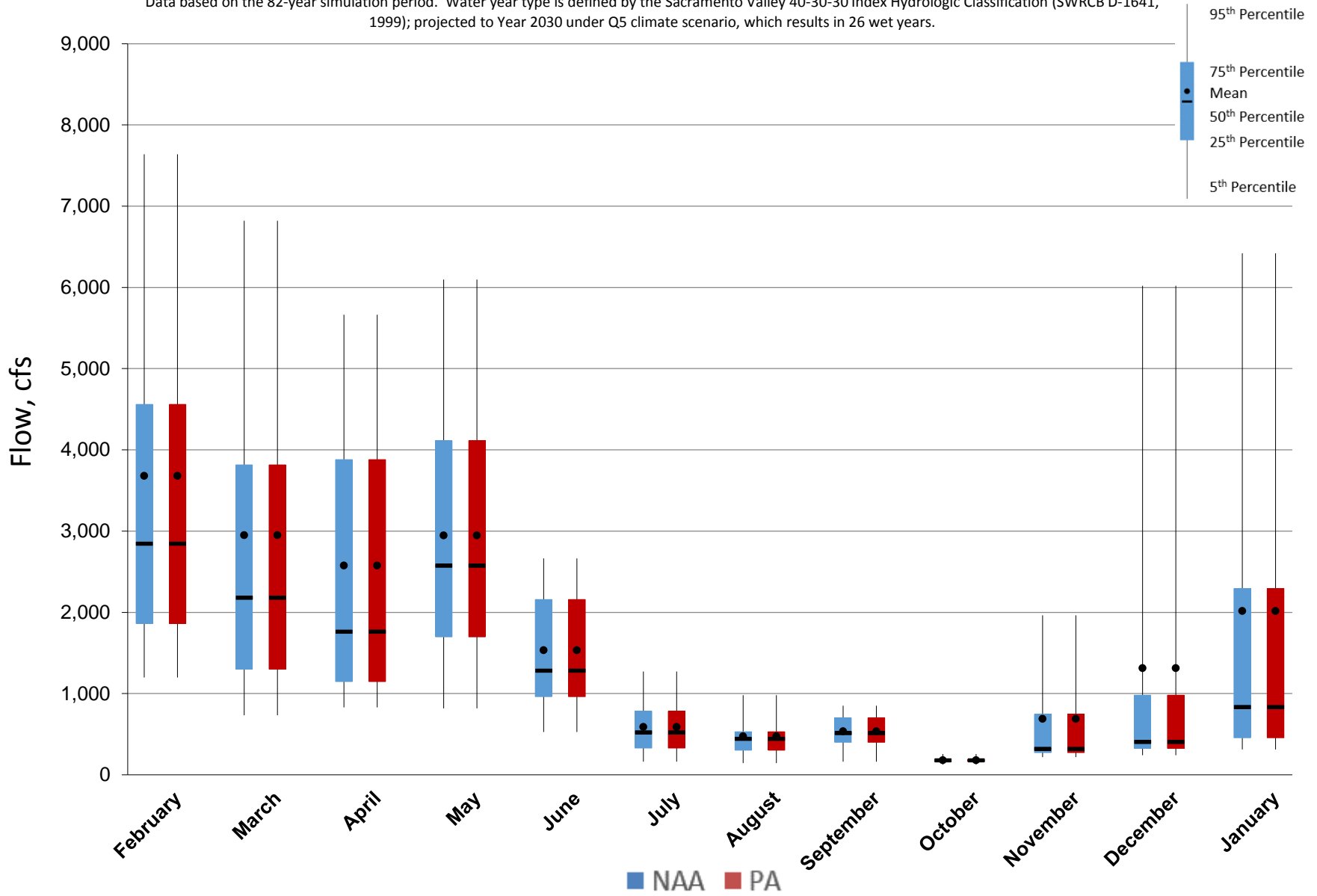
Figure 5.A.6-24-2. Monthly Flow Ranges For Mokelumne and Cosumnes River, Wet Years
