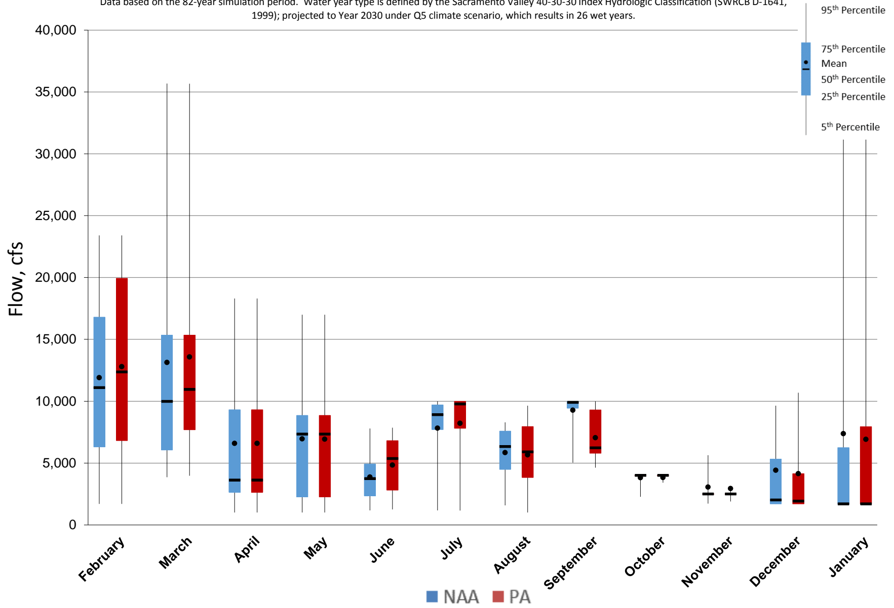
Figure 5.A.6-12-2. Monthly Flow Ranges For Feather River below Thermalito Diversion Dam, Wet Years
