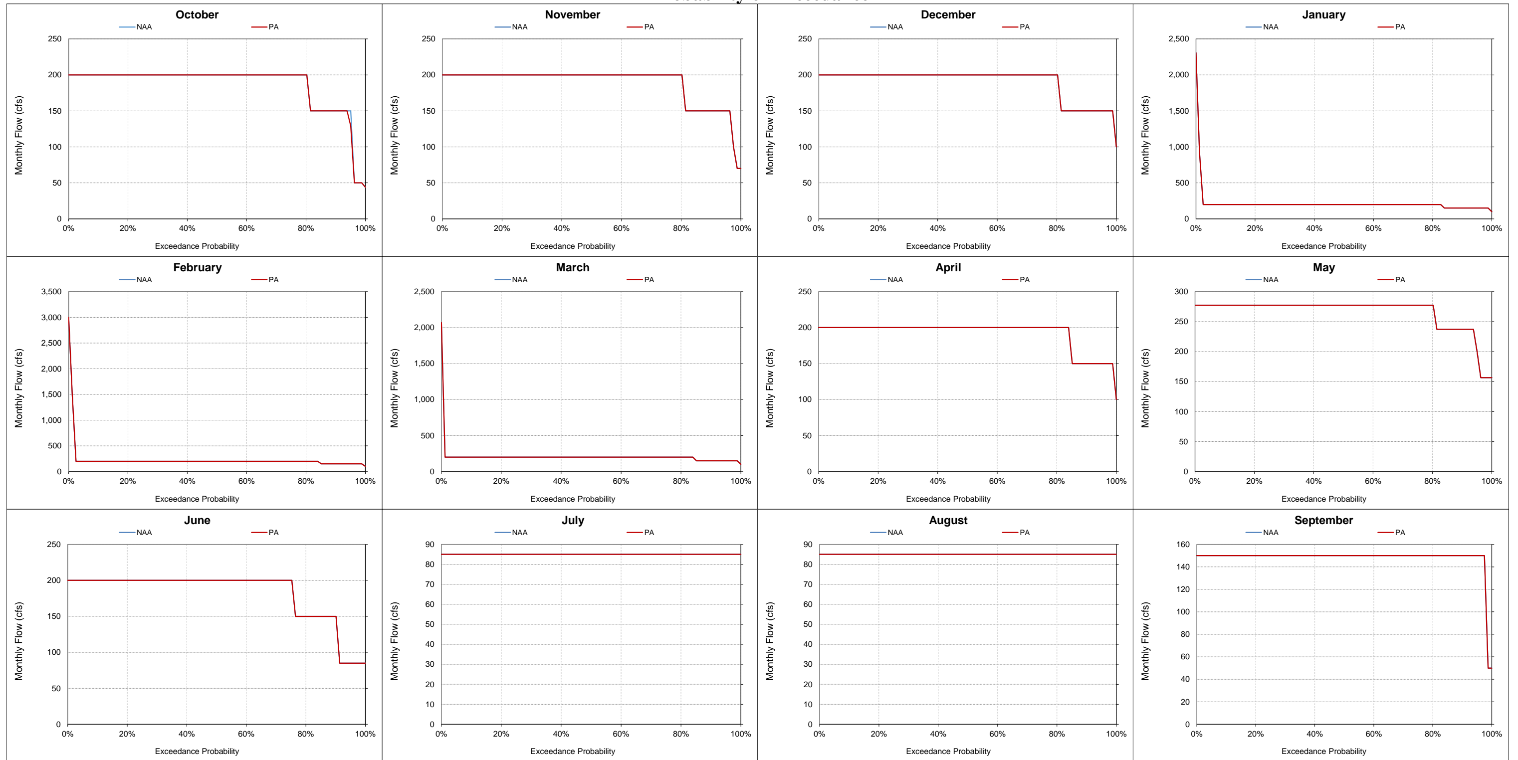
Figure 5.A.6-9-7. Clear Creek below Whiskeytown Dam, Monthly Flow Probability of Exceedance
