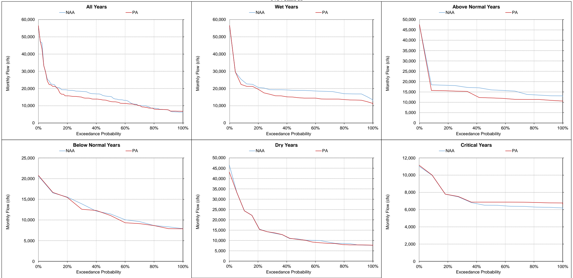
Figure 5.A.6-18-9. Sacramento River at Freeport, Monthly Flow November
