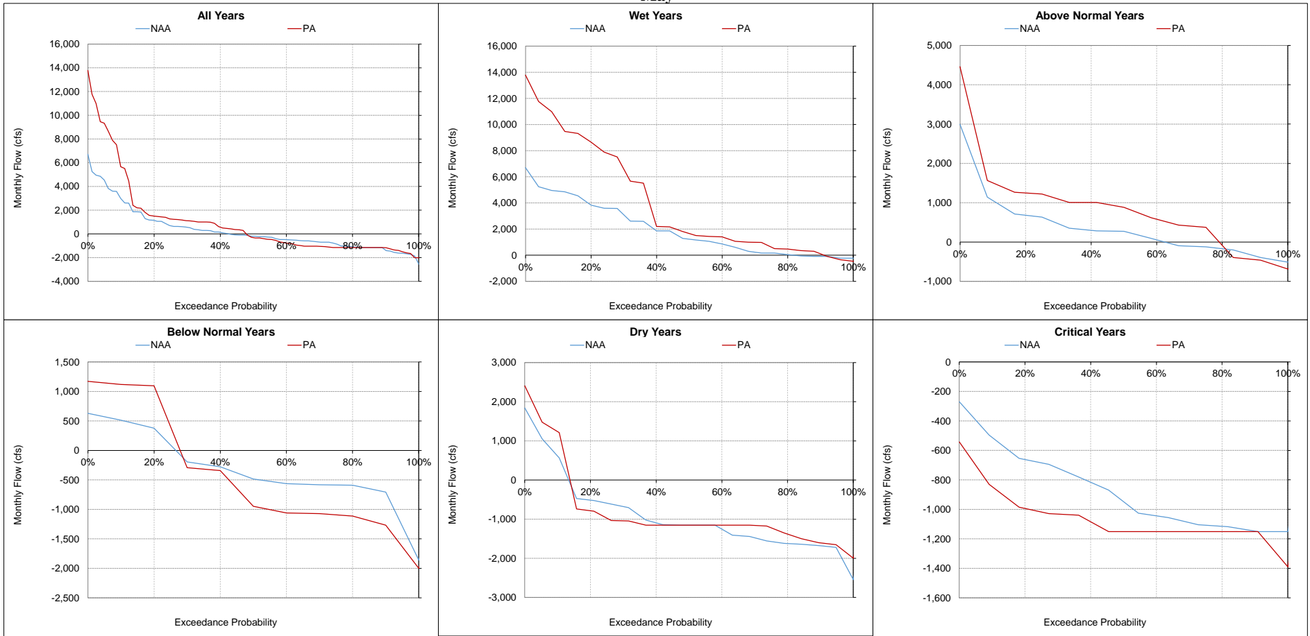
Figure 5.A.6-25-15. Old and Middle River, Monthly Flow May
