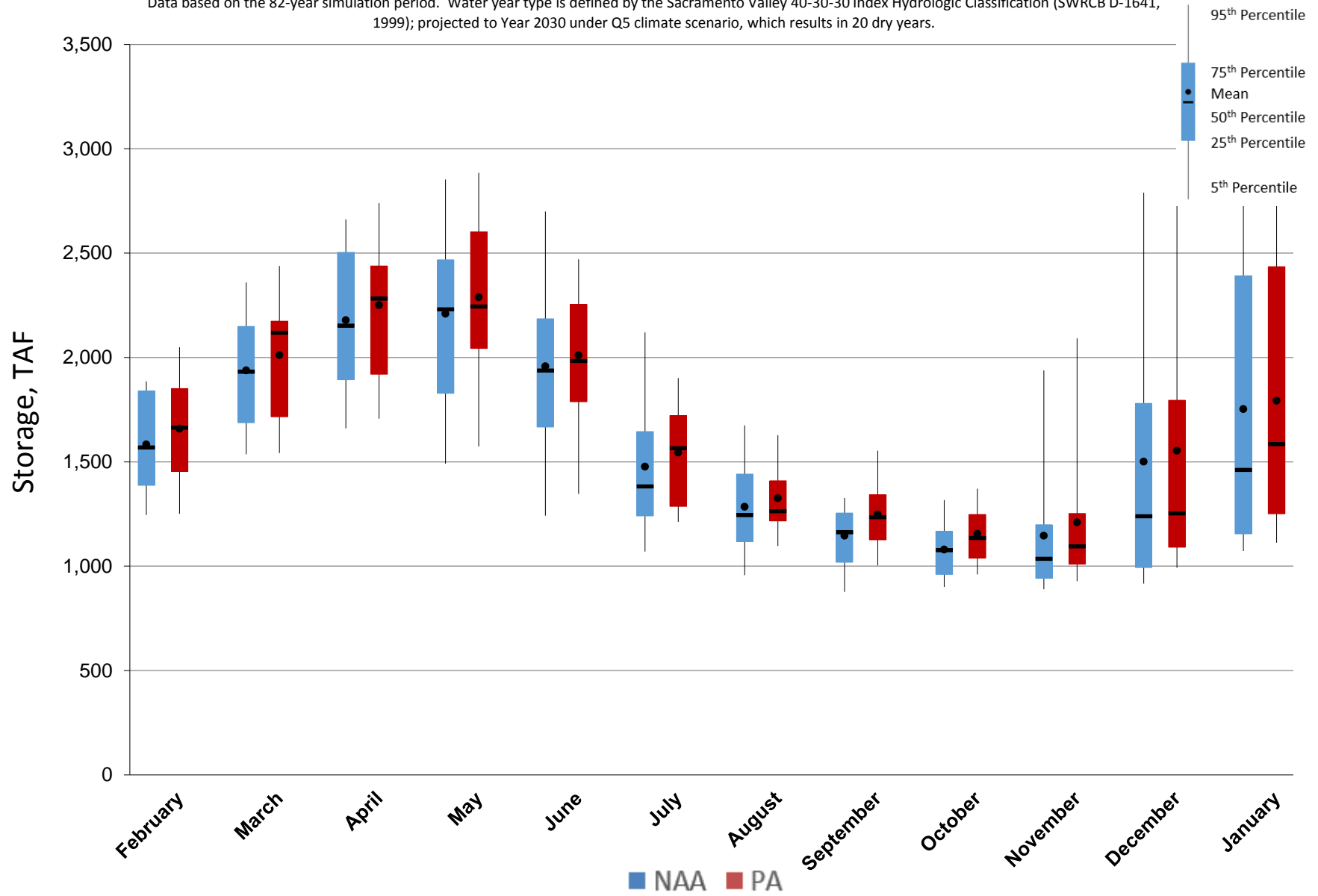
Figure 5.A.6-4-5. End of Month Storage Ranges For Lake Oroville, Dry Years
