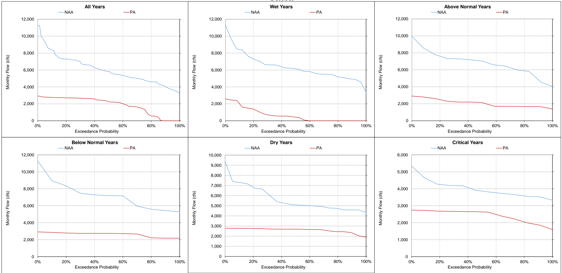
Figure 5.A.6-27-8. South Delta Exports, Monthly Flow October
