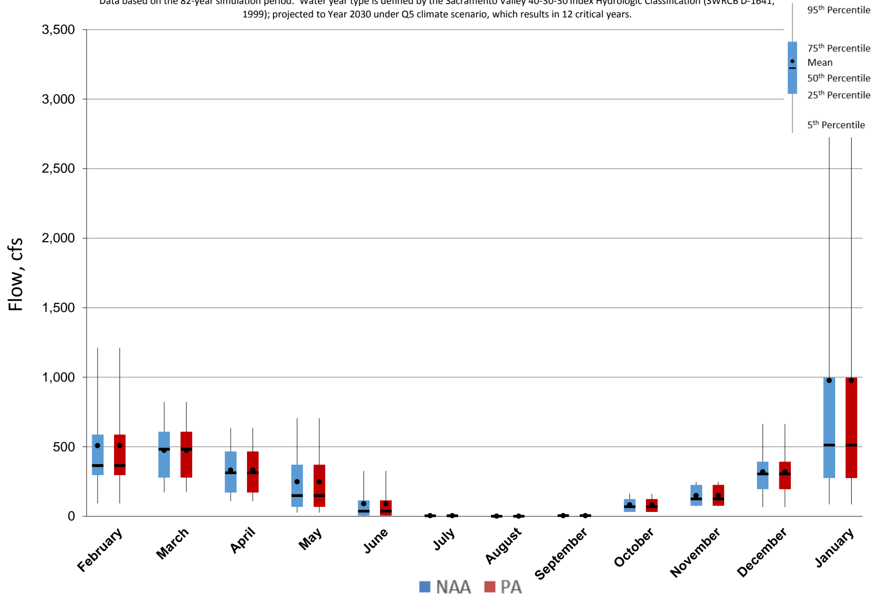
Figure 5.A.6-24-6. Monthly Flow Ranges For Mokelumne and Cosumnes River, Critical Years
