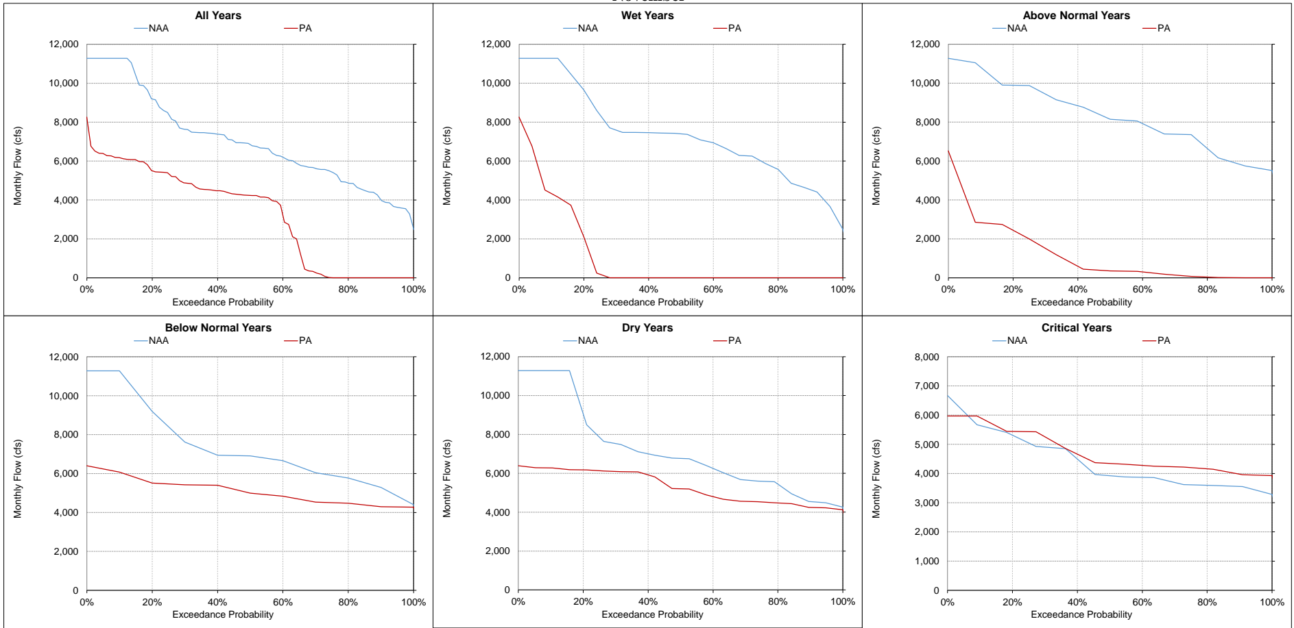
Figure 5.A.6-27-9. South Delta Exports, Monthly Flow November
