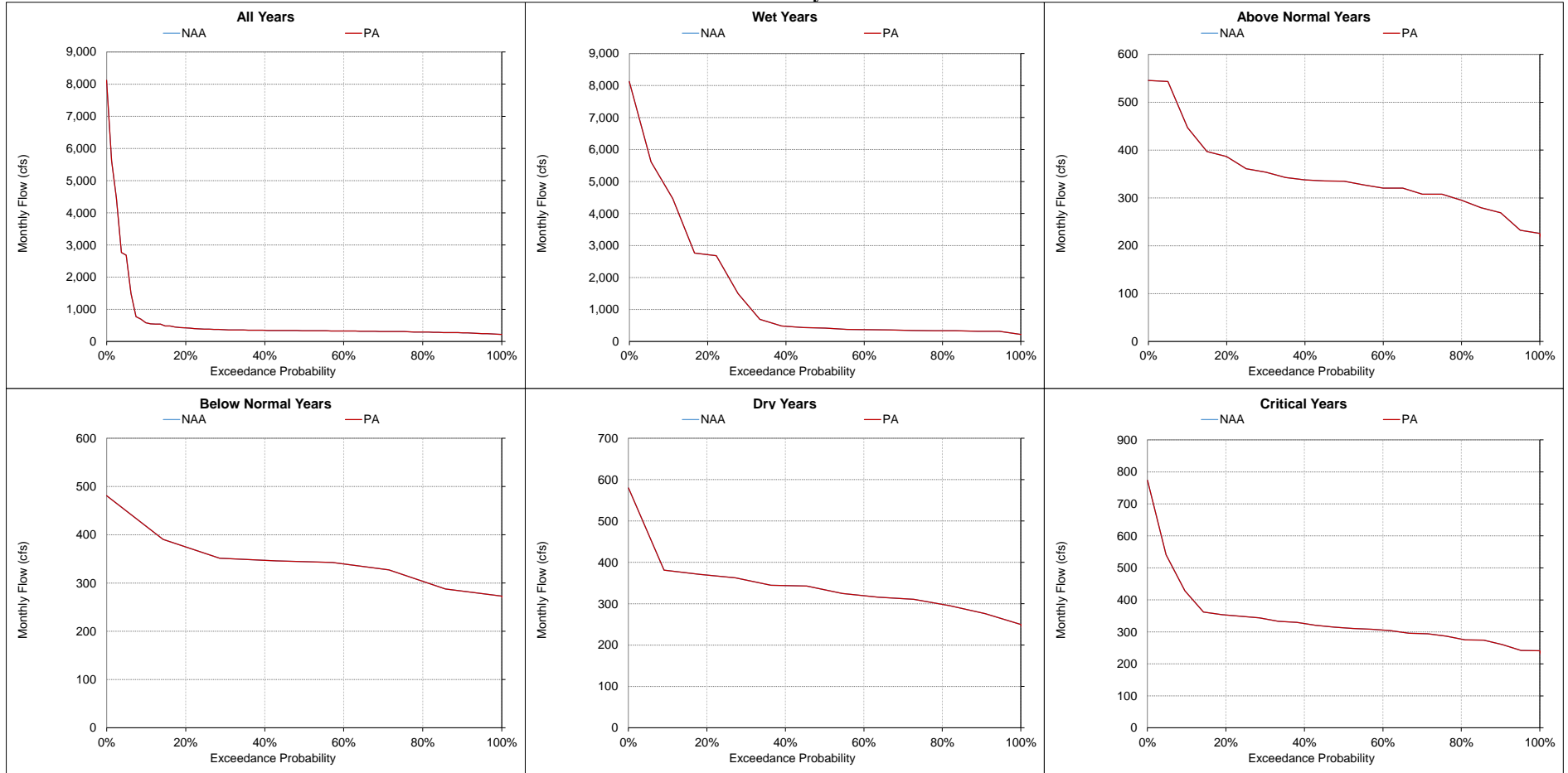
Figure 5.A.6-22-11. Stanislaus River at Mouth, Monthly Flow
