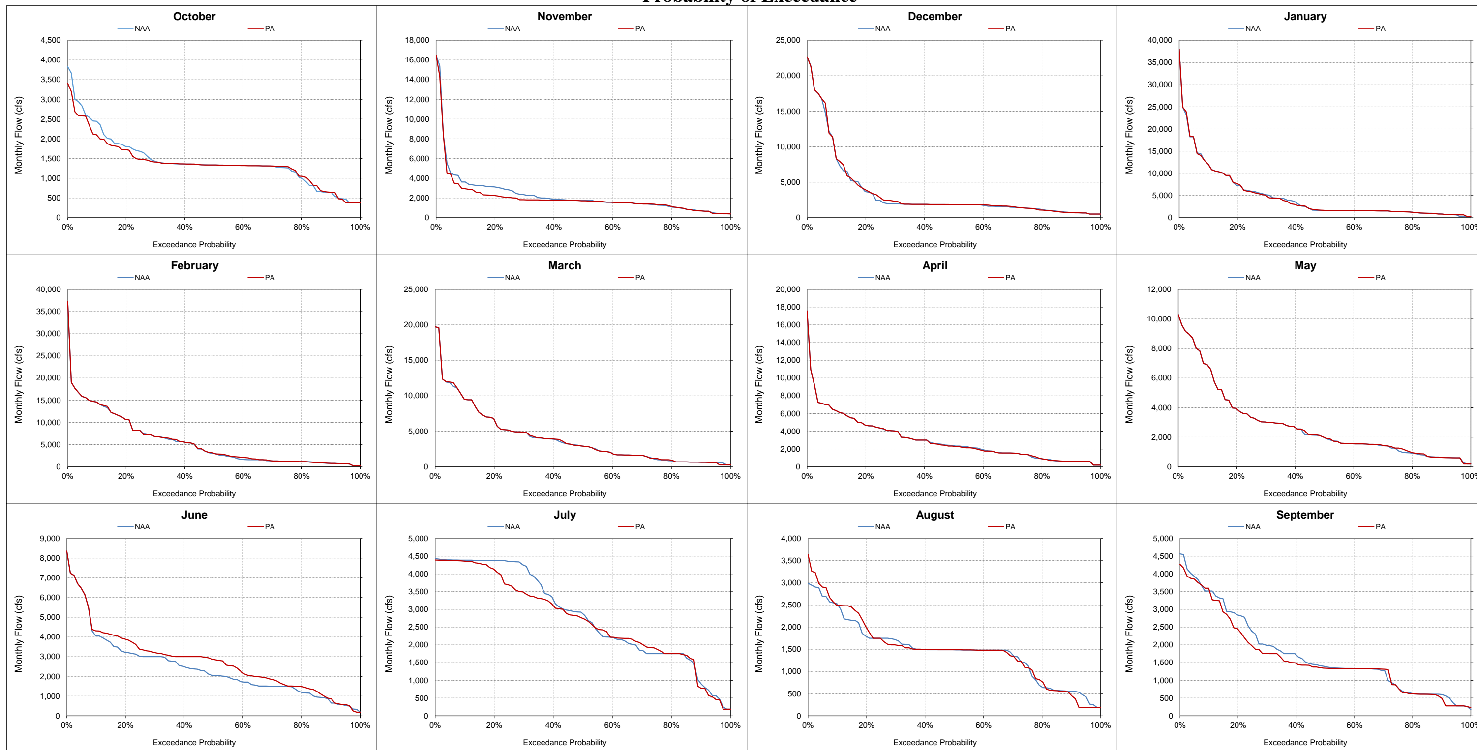
Figure 5.A.6-17-7. American River at Sacramento River Confluence, Monthly Flow Probability of Exceedance
