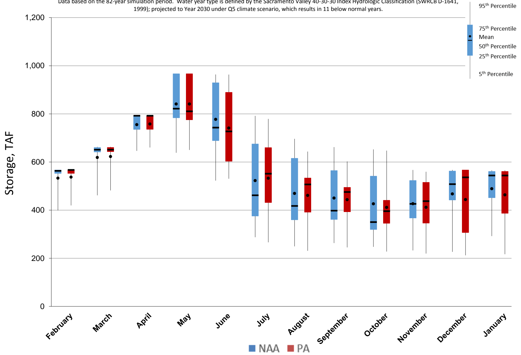
Figure 5.A.6-5-4. End of Month Storage Ranges For Folsom Lake, Below Normal Years
