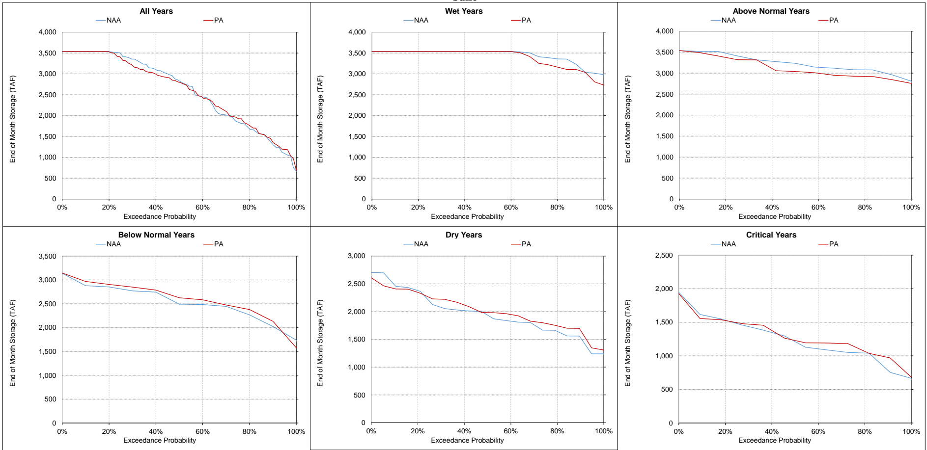
Figure 5.A.6-4-16. Lake Oroville, End of Month Storage June
