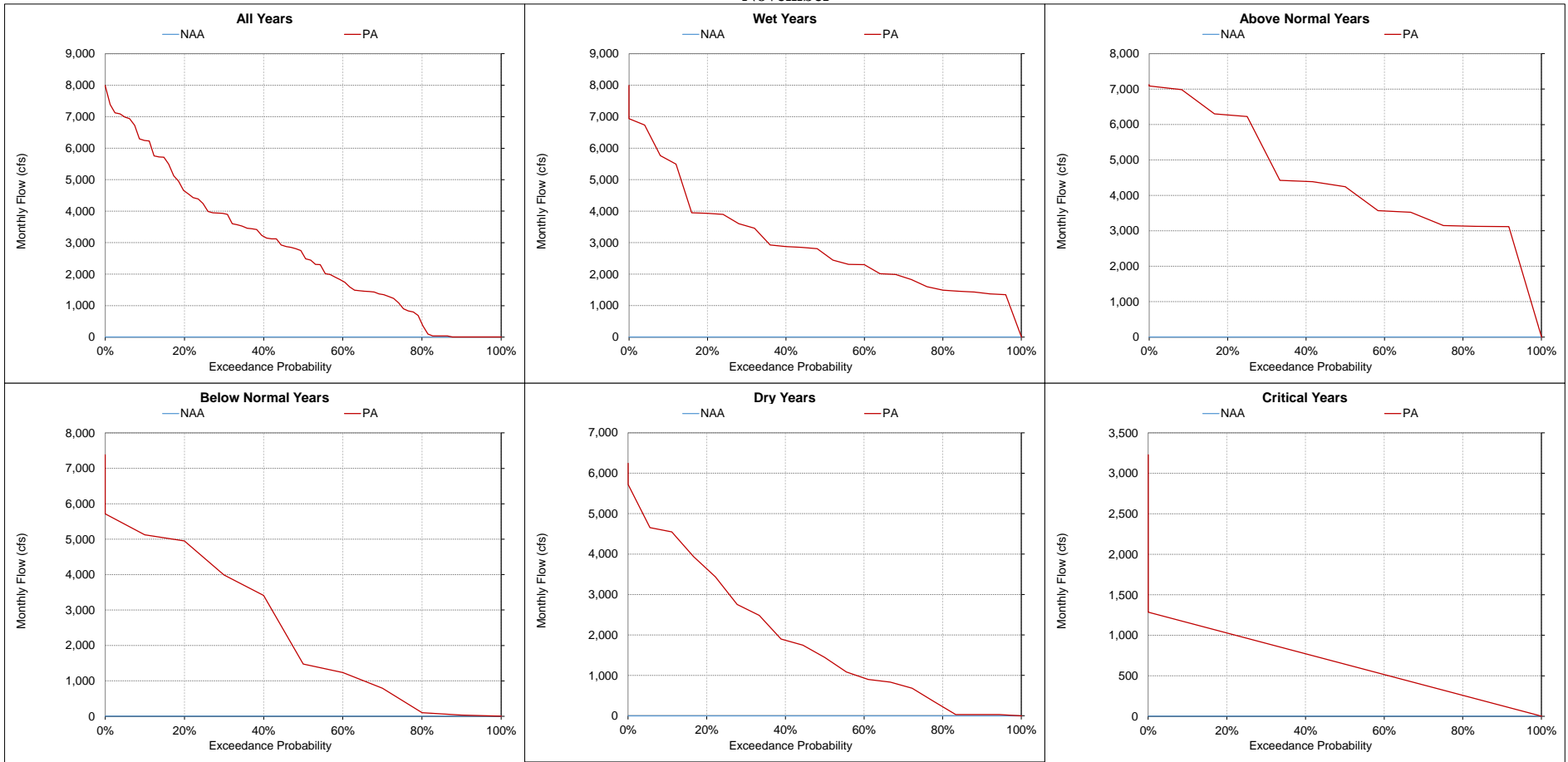
Figure 5.A.6-19-9. North Delta Diversions near Hood, Monthly Flow November
