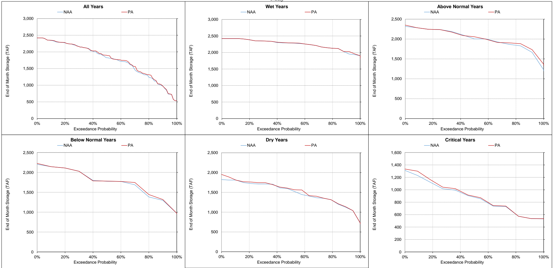
Figure 5.A.6-1-15. Trinity Lake, End of Month Storage May
