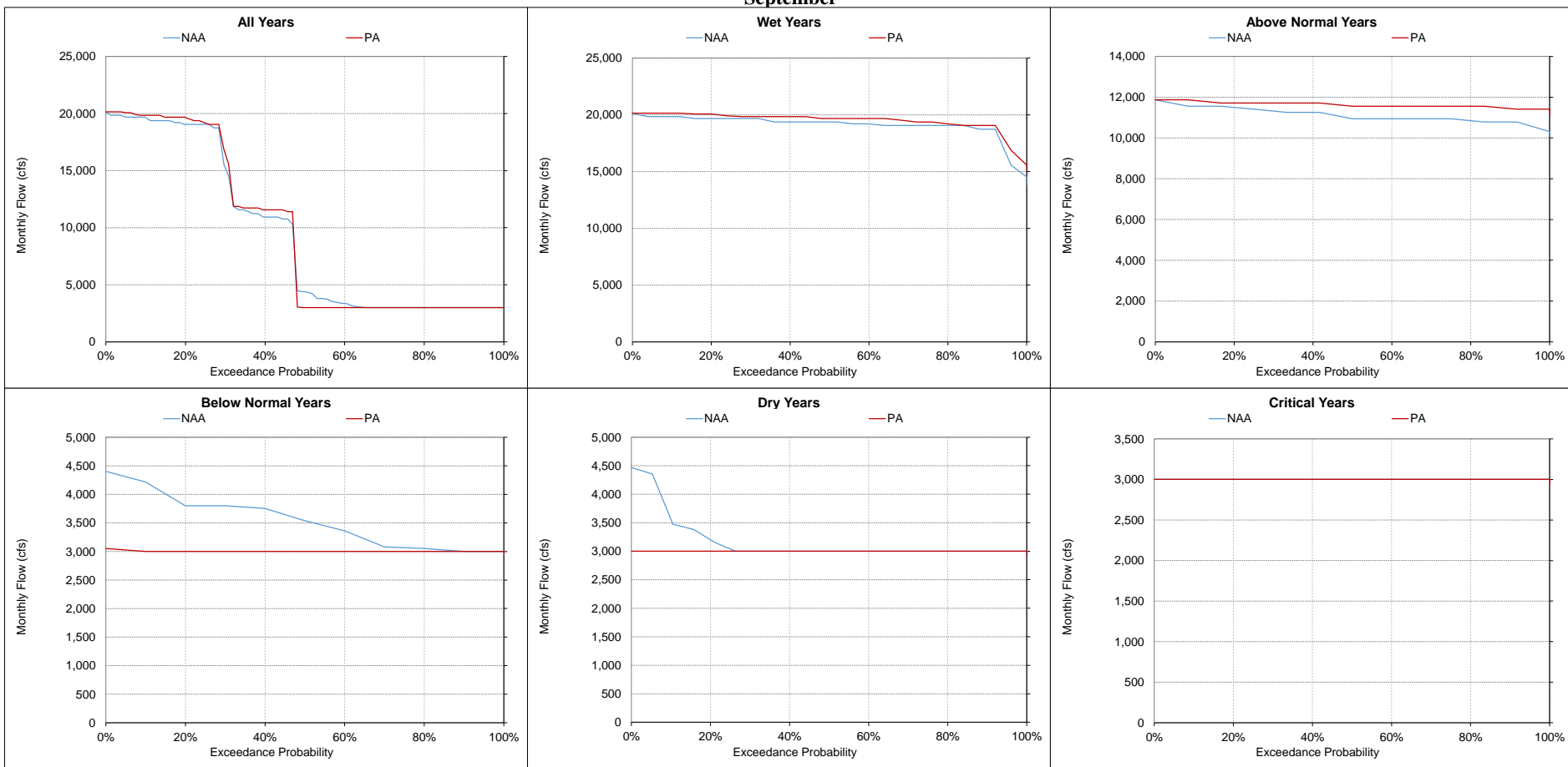
Figure 5.A.6-26-19. Delta Outflow, Monthly Flow September
