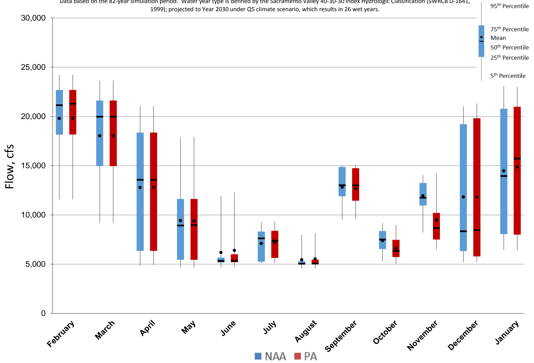
Figure 5.A.6-11-2. Monthly Flow Ranges For Sacramento River at Bend Bridge, Wet Years
