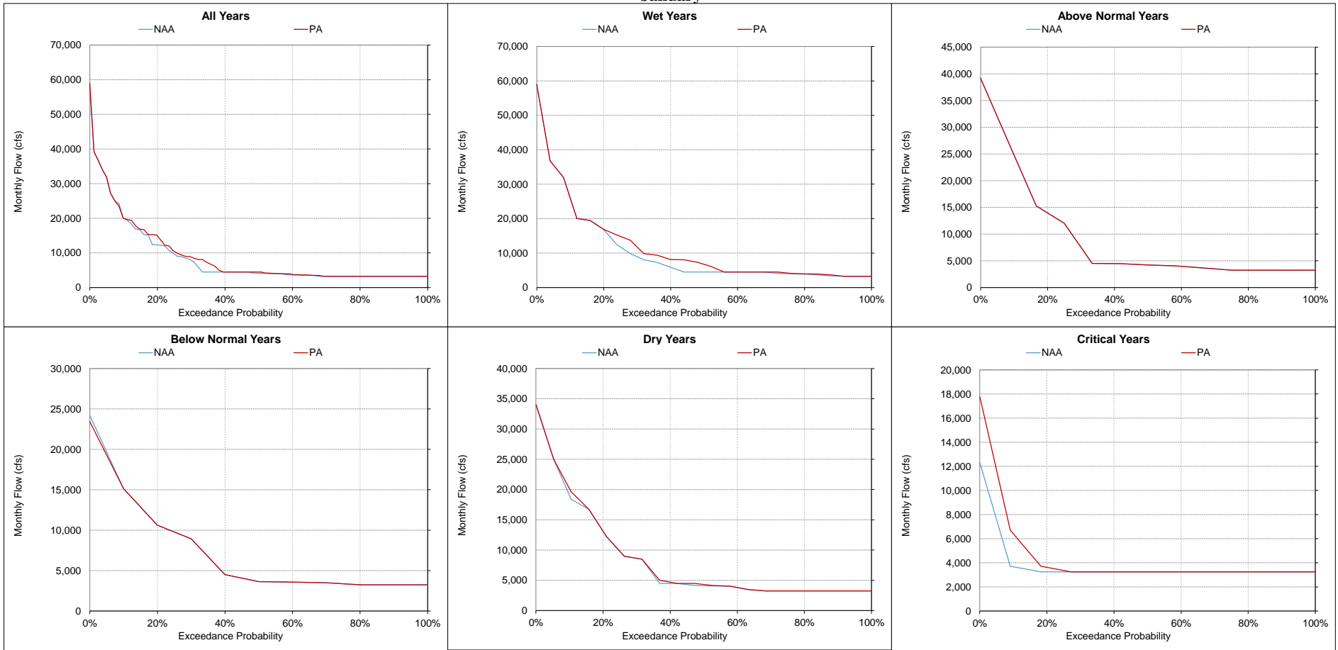
Figure 5.A.6-10-11. Sacramento River below Keswick Dam, Monthly Flow January
