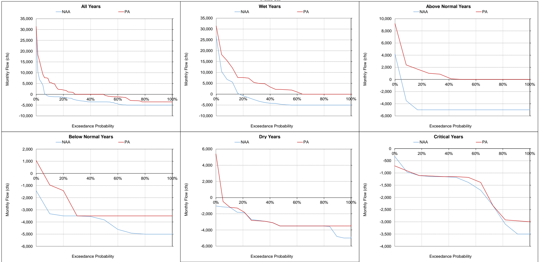
Figure 5.A.6-25-13. Old and Middle River, Monthly Flow March
