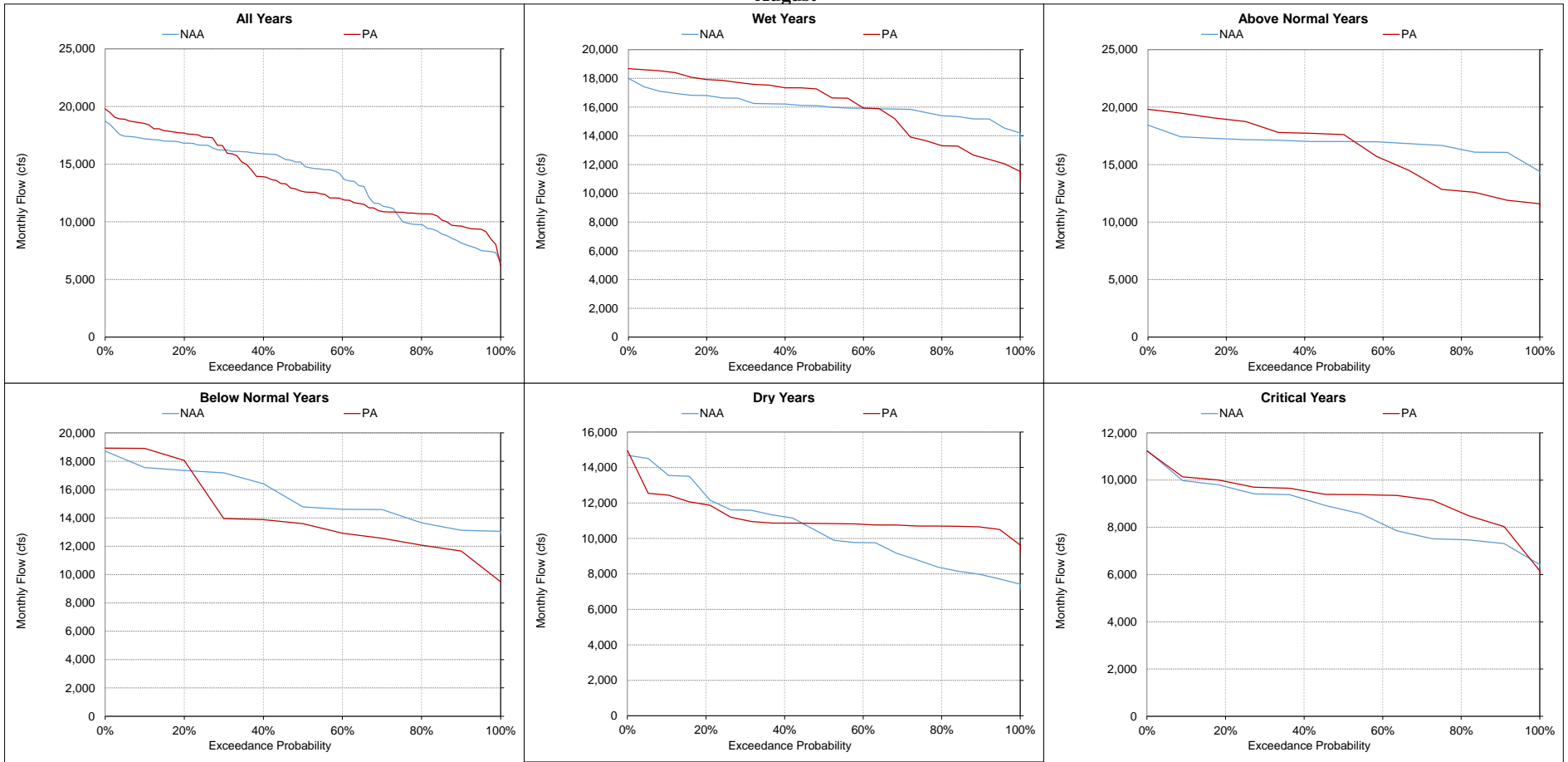
Figure 5.A.6-18-18. Sacramento River at Freeport, Monthly Flow August
