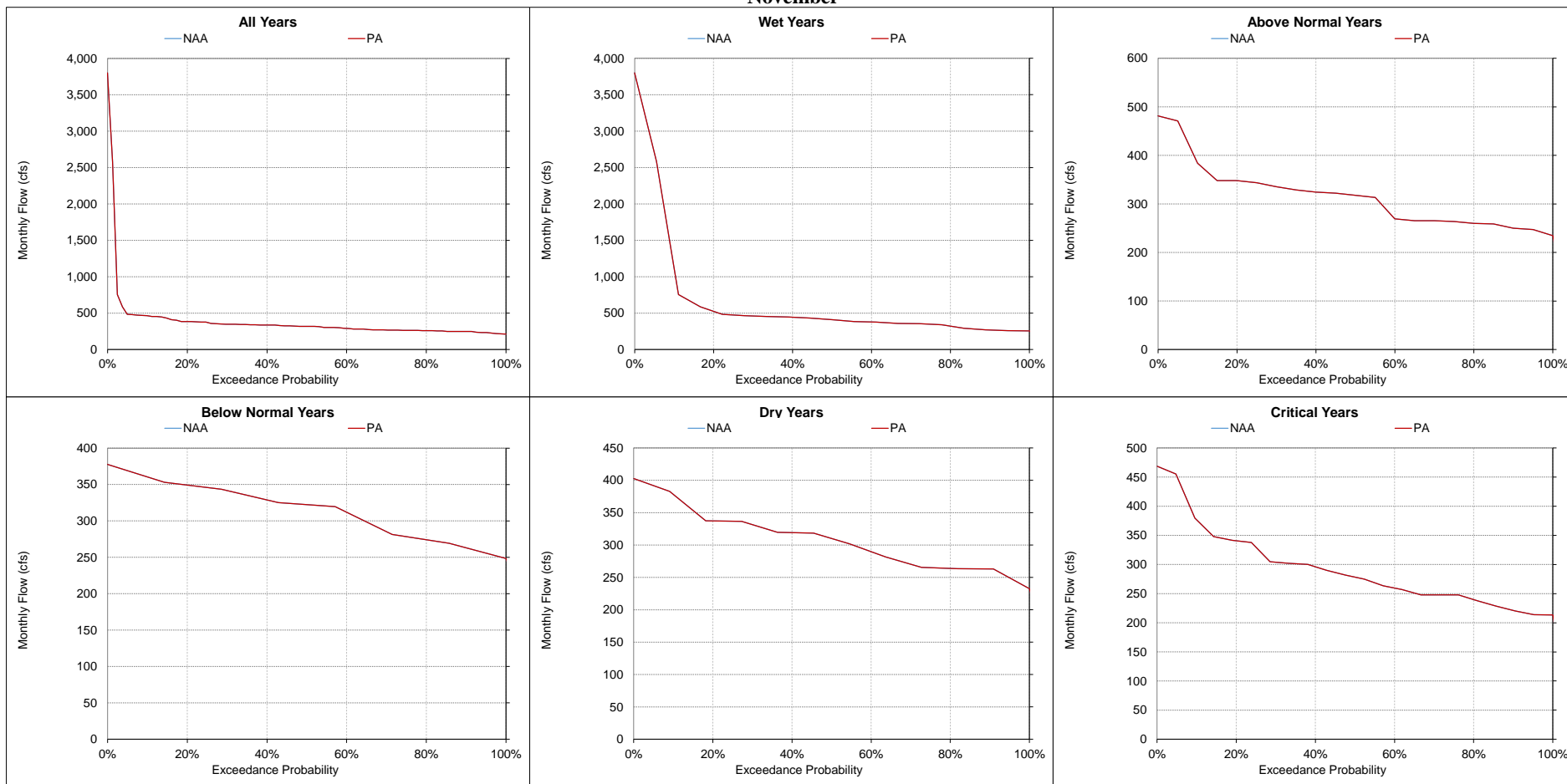
Figure 5.A.6-22-9. Stanislaus River at Mouth, Monthly Flow November
