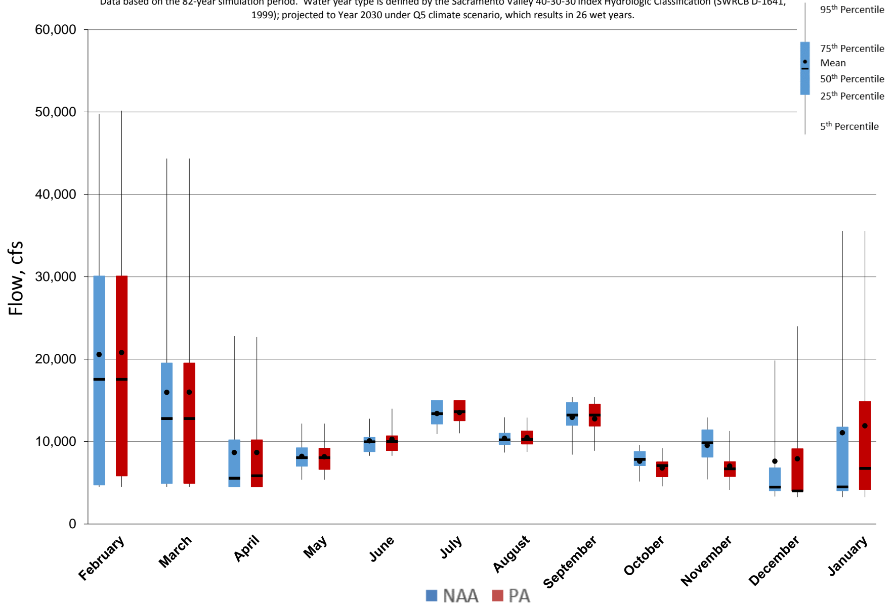
Figure 5.A.6-10-2. Monthly Flow Ranges For Sacramento River below Keswick Dam, Wet Years
