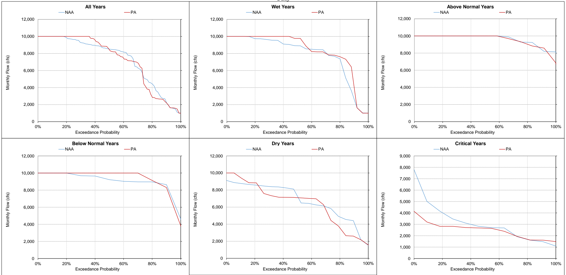
Figure 5.A.6-12-17. Feather River below Thermalito Diversion Dam, Monthly Flow July
