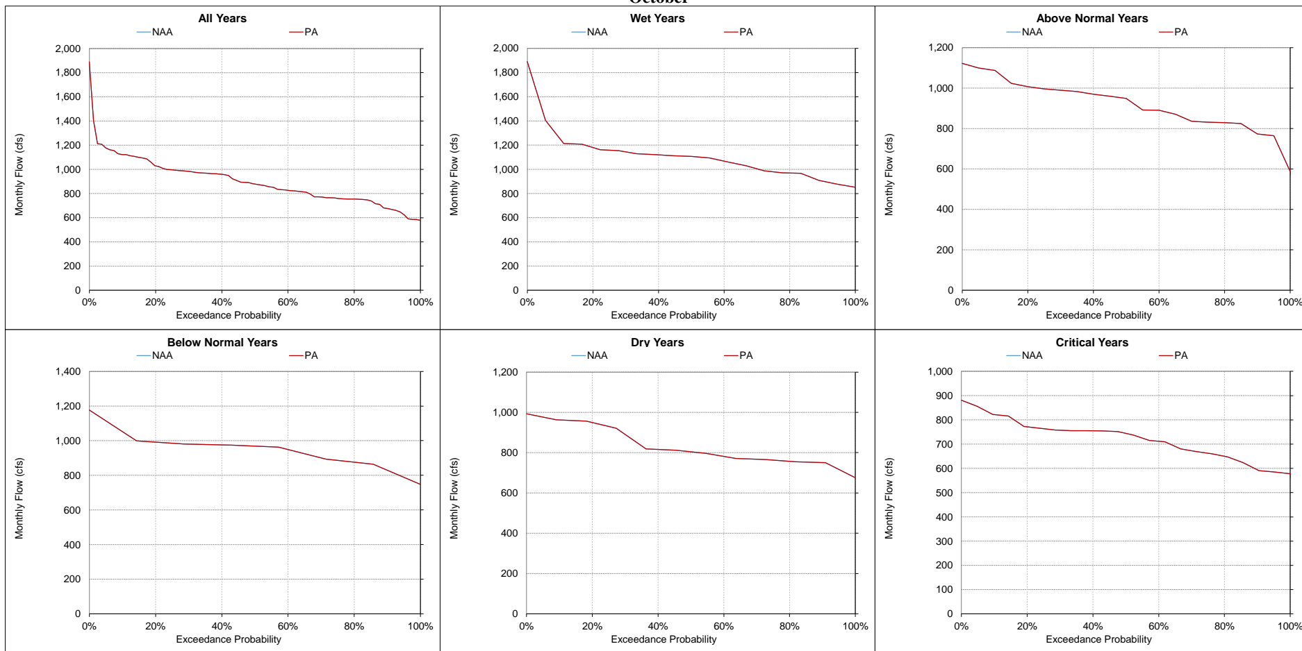
Figure 5.A.6-22-8. Stanislaus River at Mouth, Monthly Flow October
