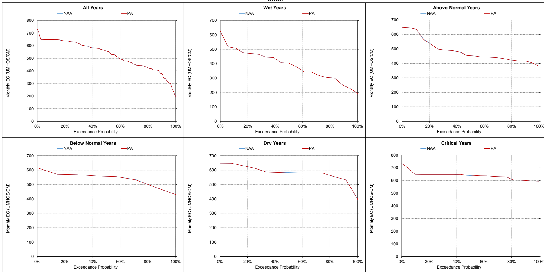
Figure 5.A.6-30-16. San Joaquin River at Vernalis, Monthly EC
