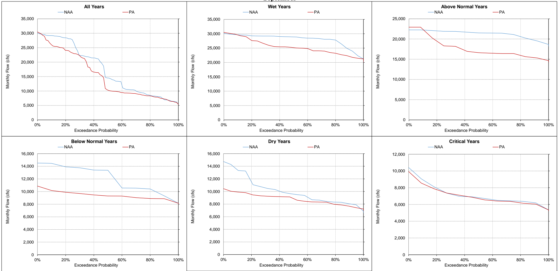
Figure 5.A.6-18-19. Sacramento River at Freeport, Monthly Flow September
