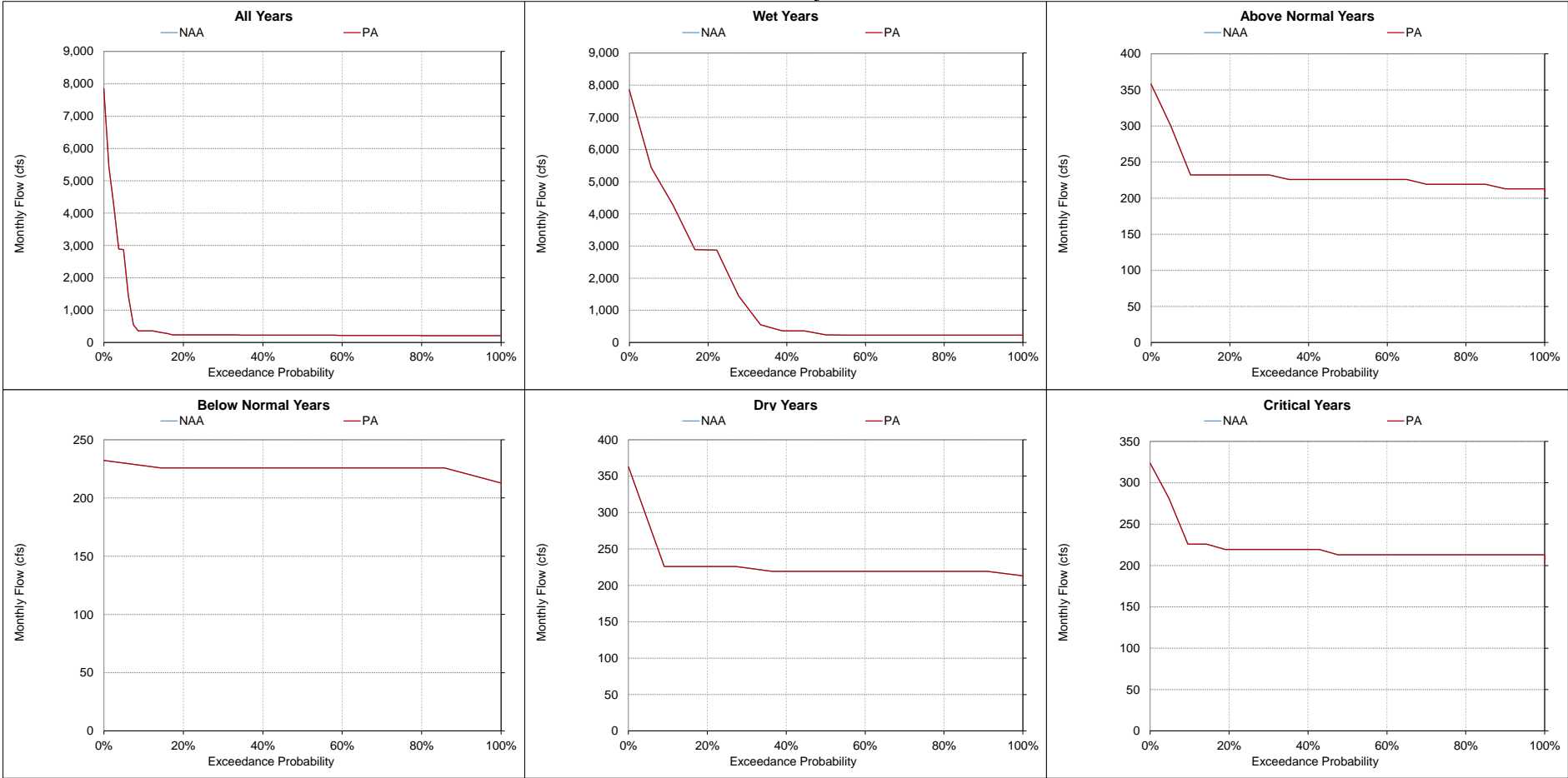
Figure 5.A.6-21-11. Stanislaus River at Ripon, Monthly Flow
