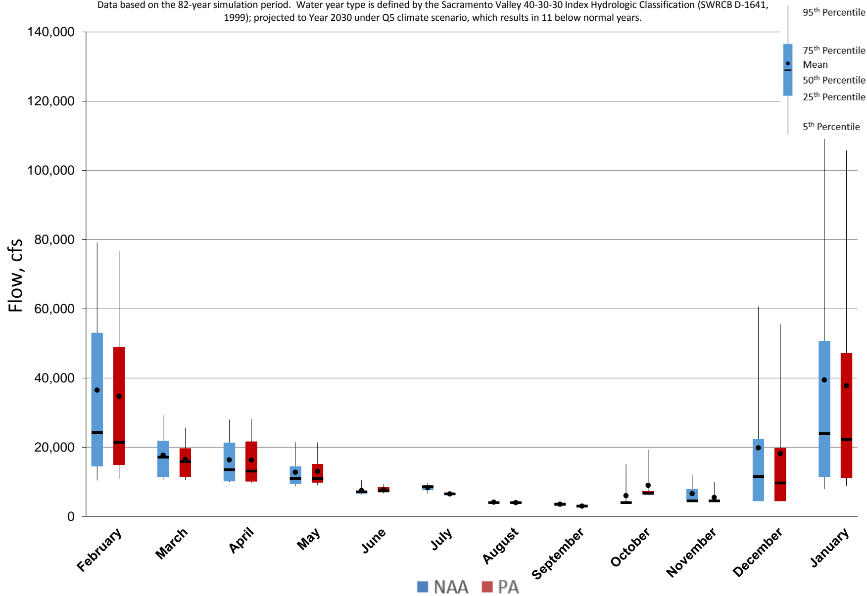
Figure 5.A.6-26-4. Monthly Flow Ranges For Delta Outflow, Below Normal Years
