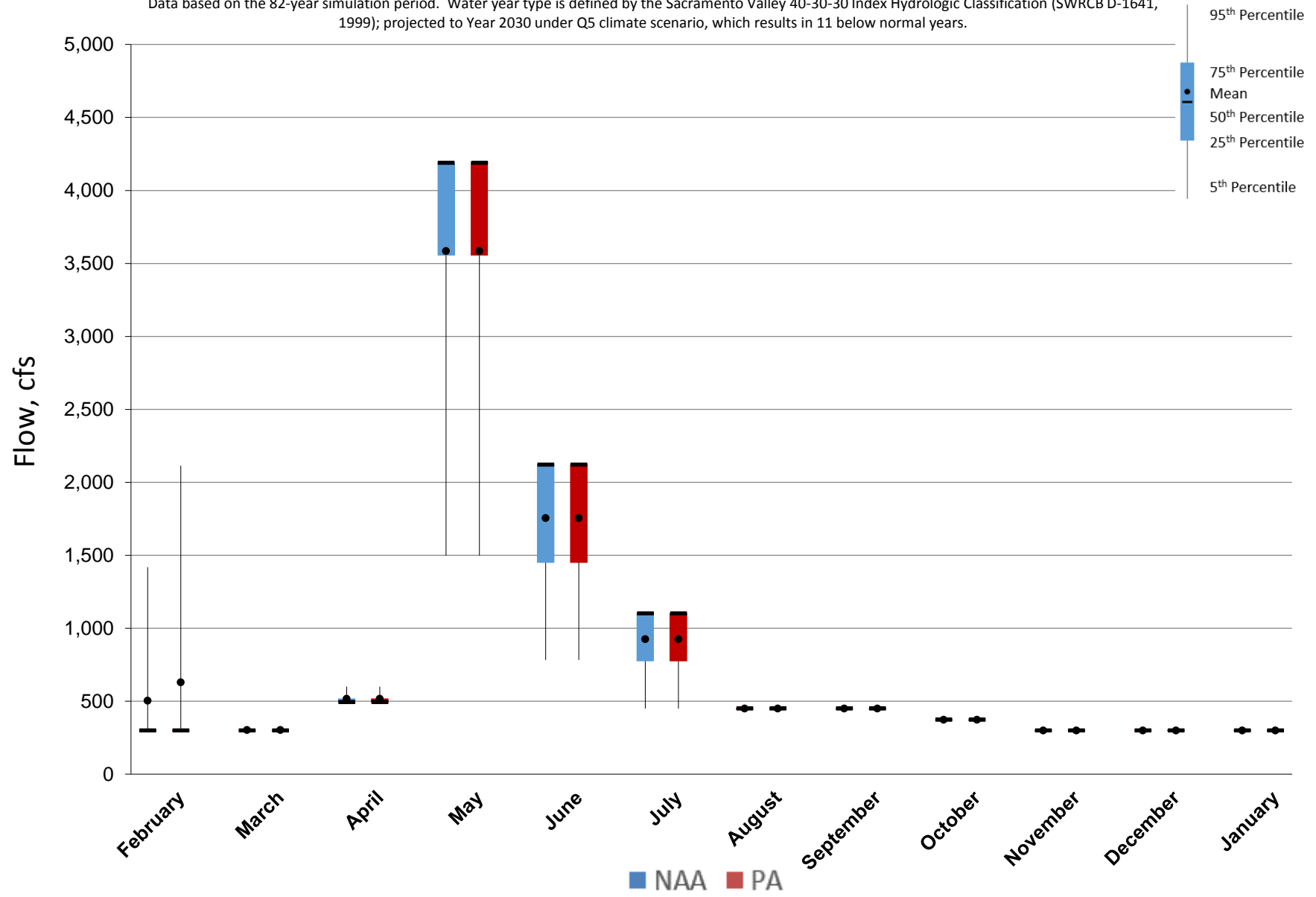
Figure 5.A.6-7-4. Monthly Flow Ranges For Trinity River below Lewiston Dam, Below Normal Years
