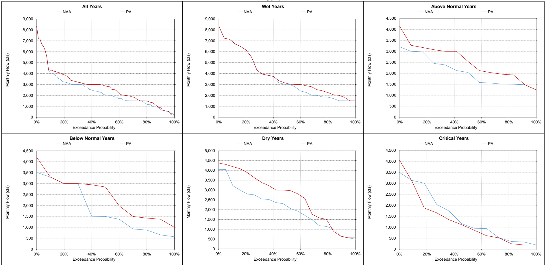
Figure 5.A.6-17-16. American River at Sacramento River Confluence, Monthly Flow June
