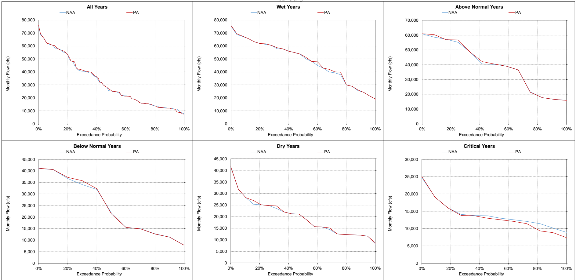
Figure 5.A.6-14-12. Sacramento River at Verona, Monthly Flow February
