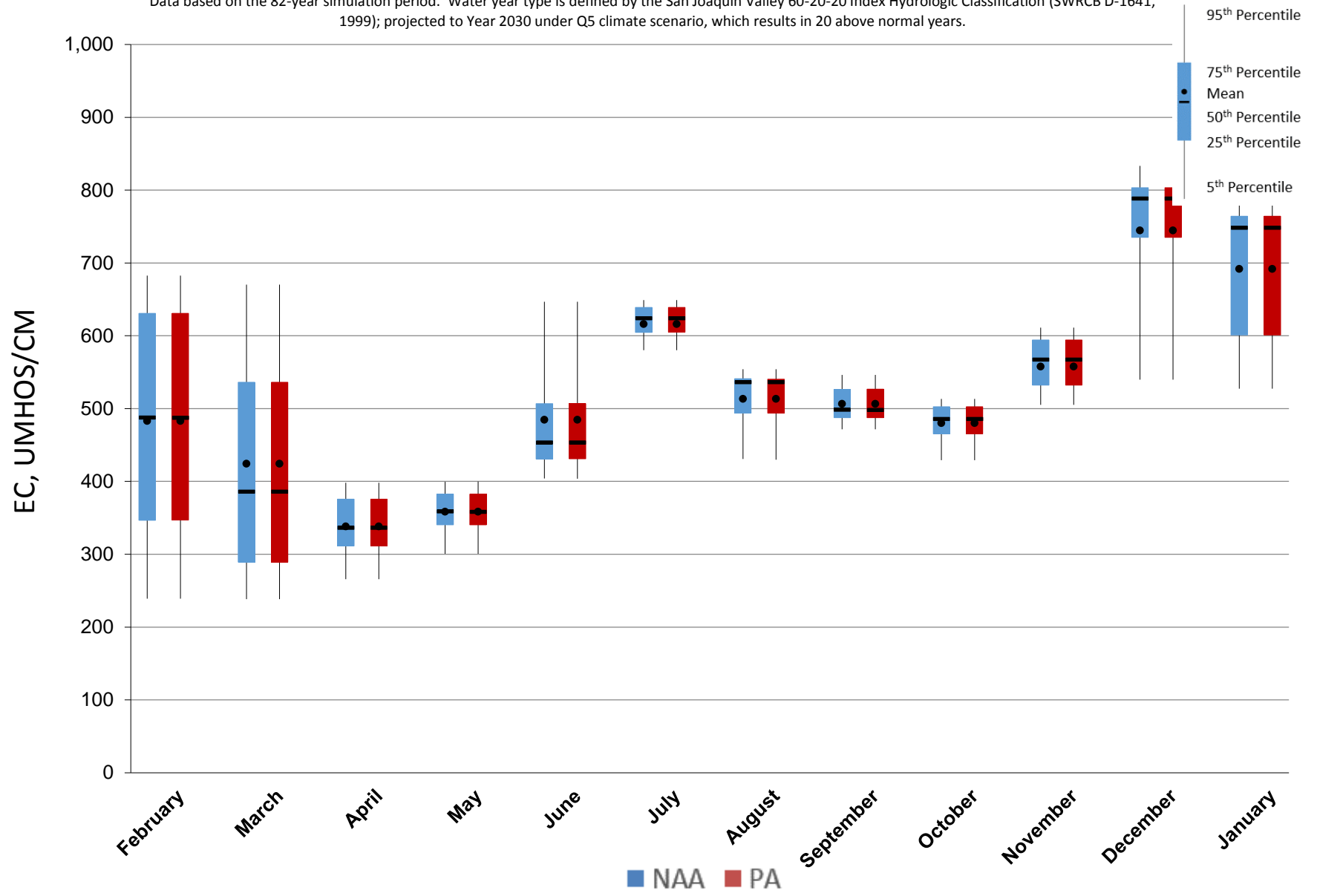
Figure 5.A.6-30-3. Monthly EC Ranges for San Joaquin River at Vernalis, Above Normal Years
