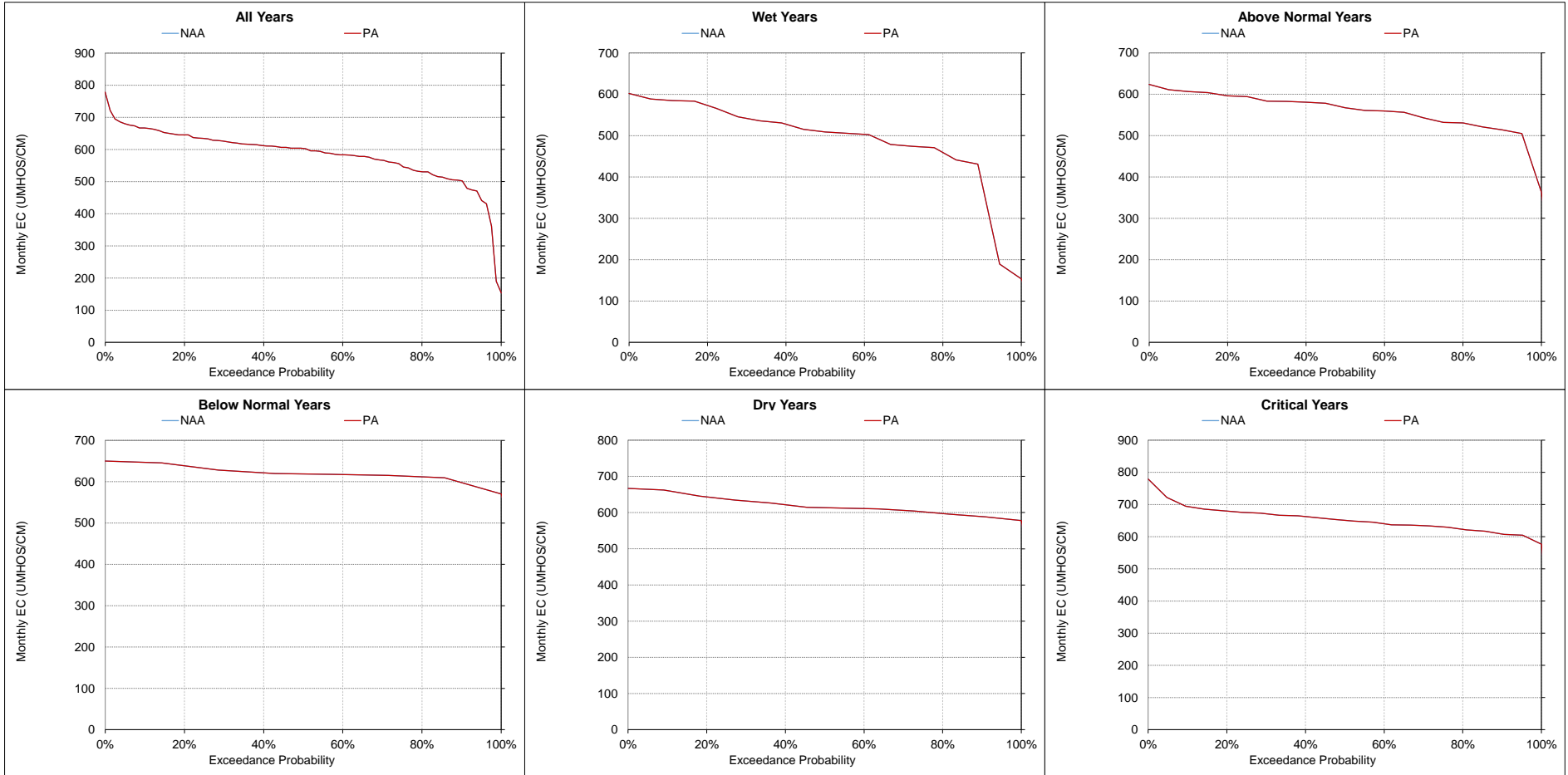
Figure 5.A.6-30-9. San Joaquin River at Vernalis, Monthly EC November
