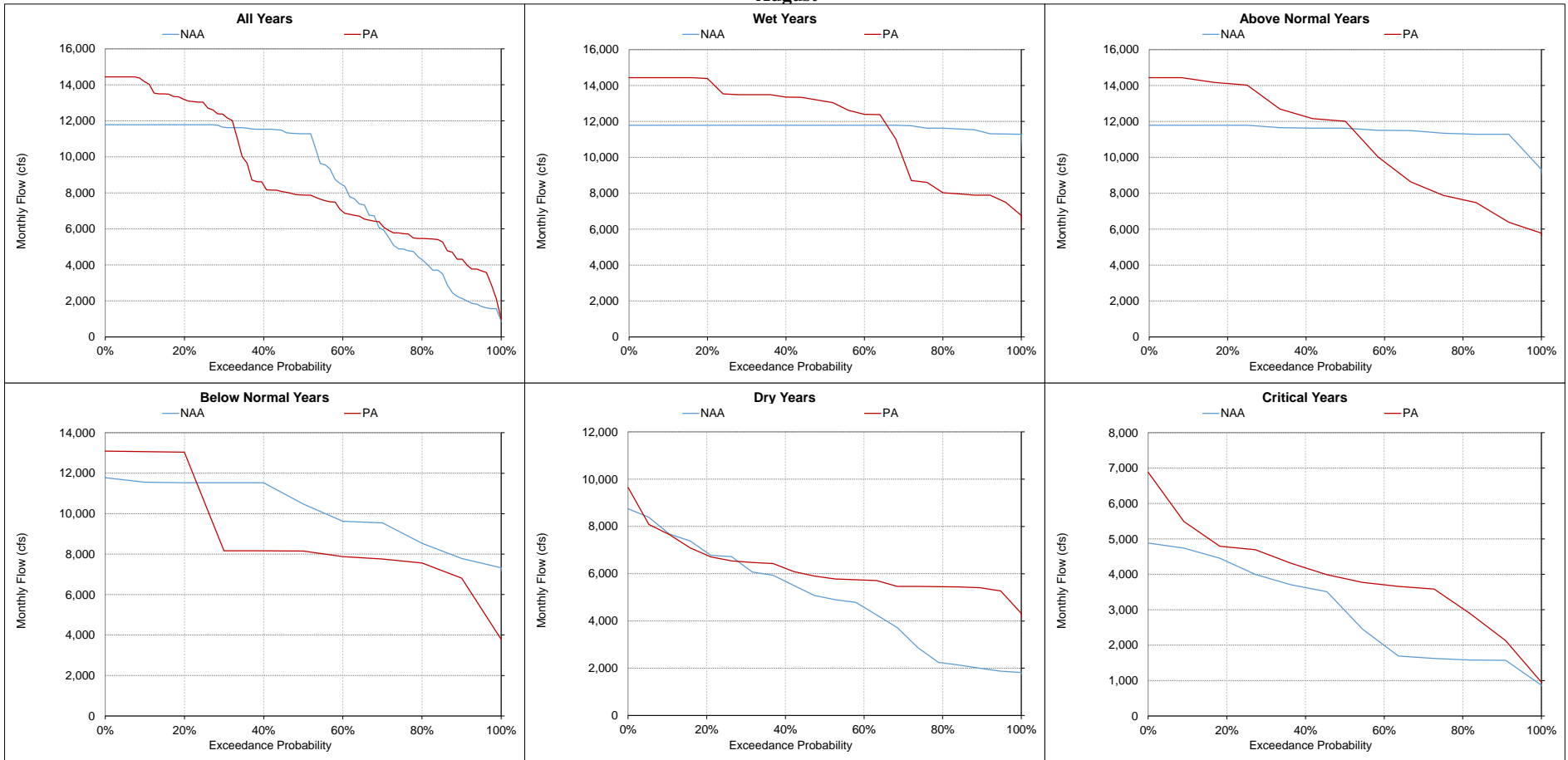
Figure 5.A.6-28-18. Total Delta Exports, Monthly Flow August
