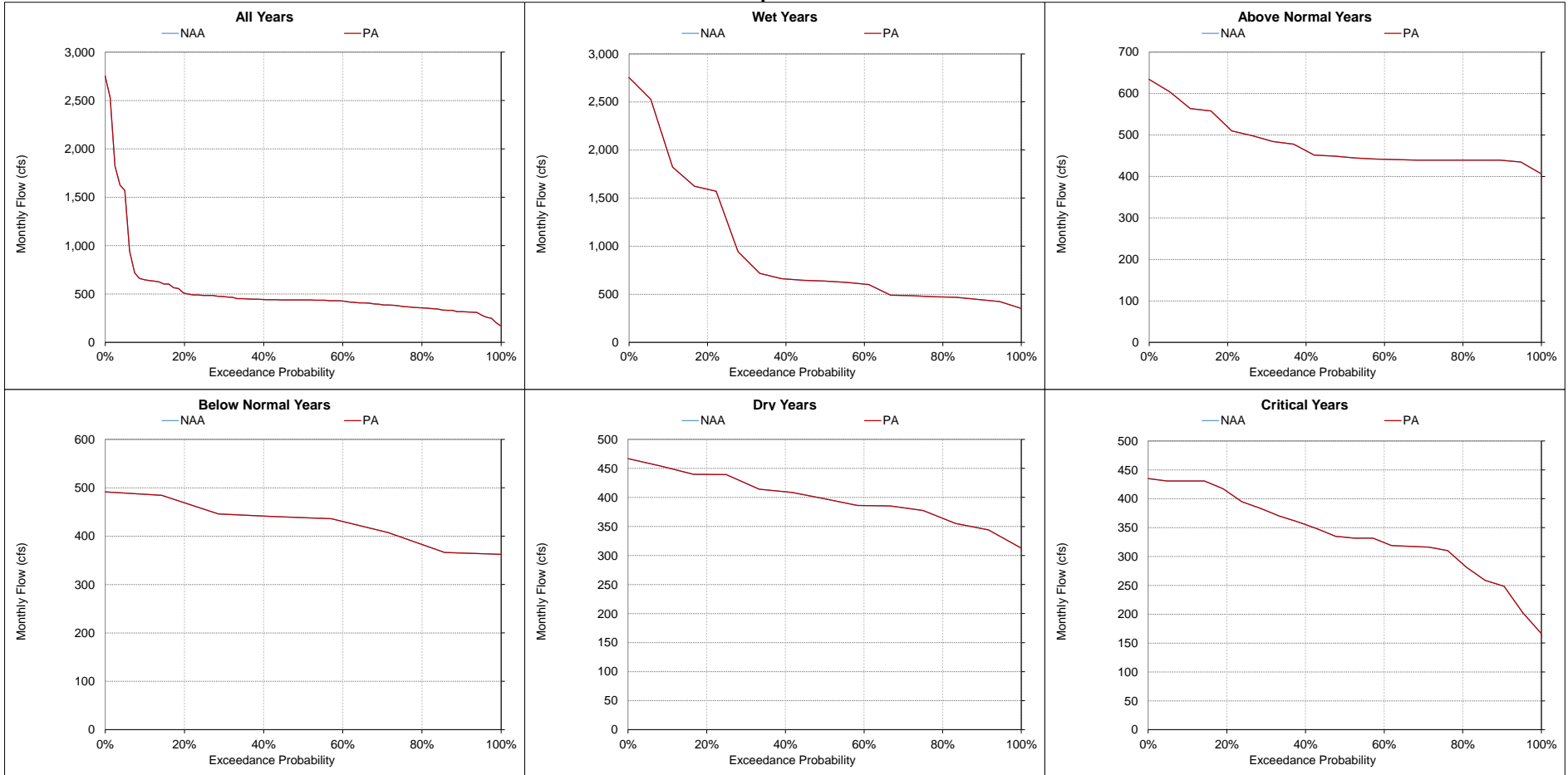
Figure 5.A.6-22-19. Stanislaus River at Mouth, Monthly Flow September
