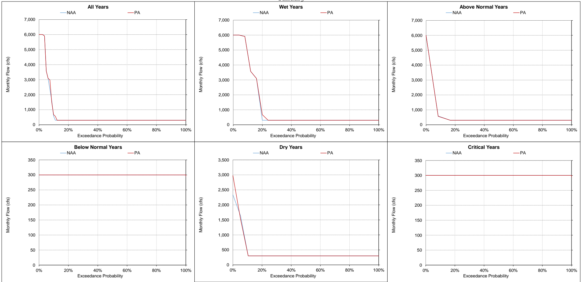
Figure 5.A.6-7-11. Trinity River below Lewiston Dam, Monthly Flow January
