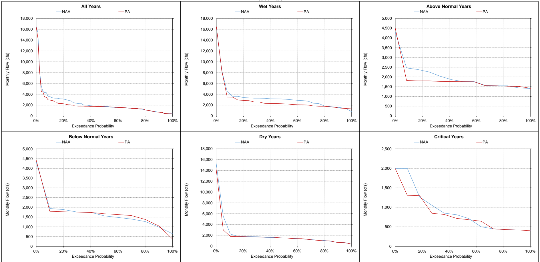
Figure 5.A.6-17-9. American River at Sacramento River Confluence, Monthly Flow November
