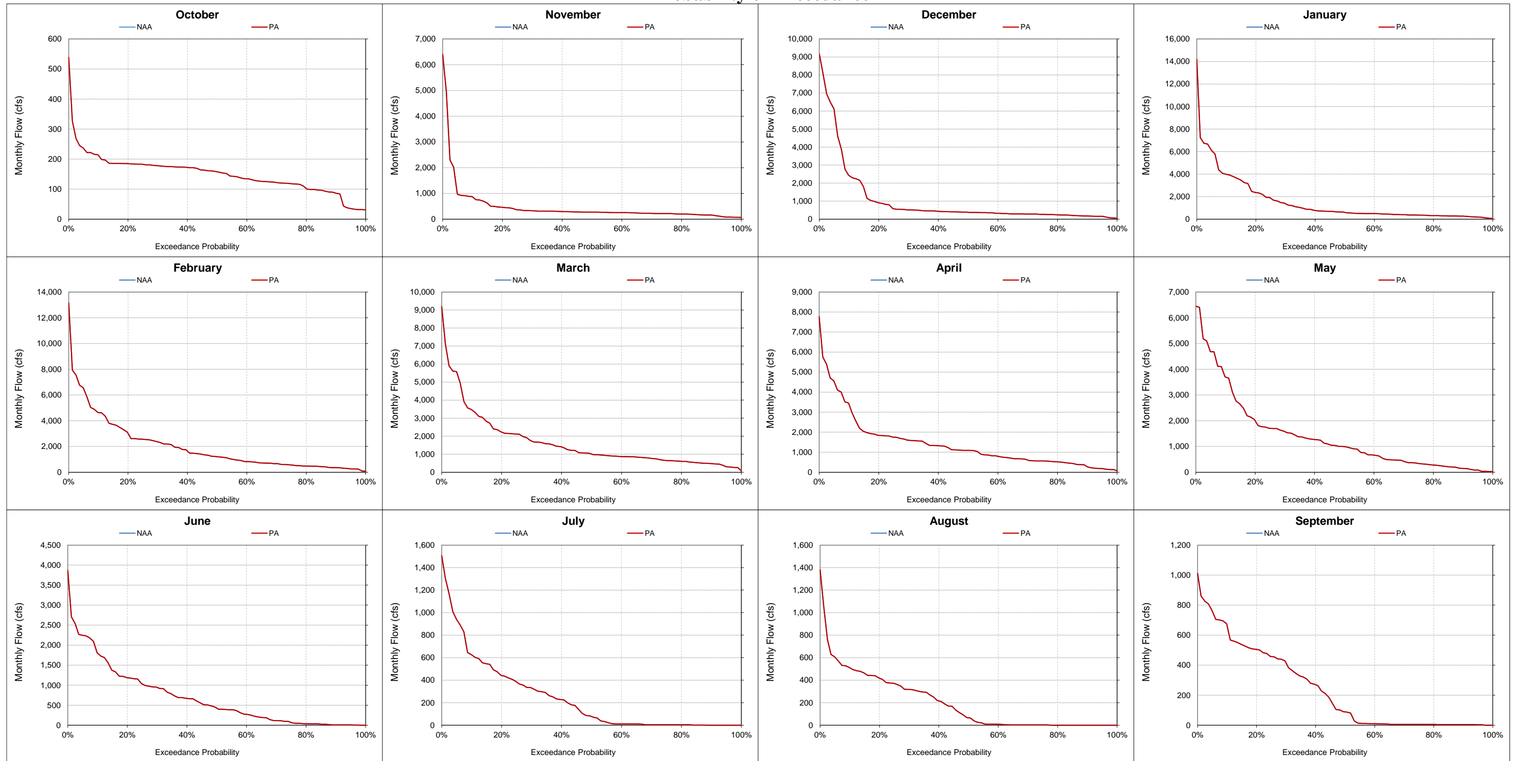
Figure 5.A.6-24-7. Mokelumne and Cosumnes River, Monthly Flow Probability of Exceedance
