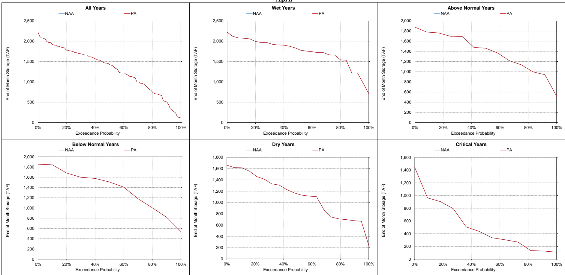
Figure 5.A.6-14. New Melones Lake, End of Month Storage April
