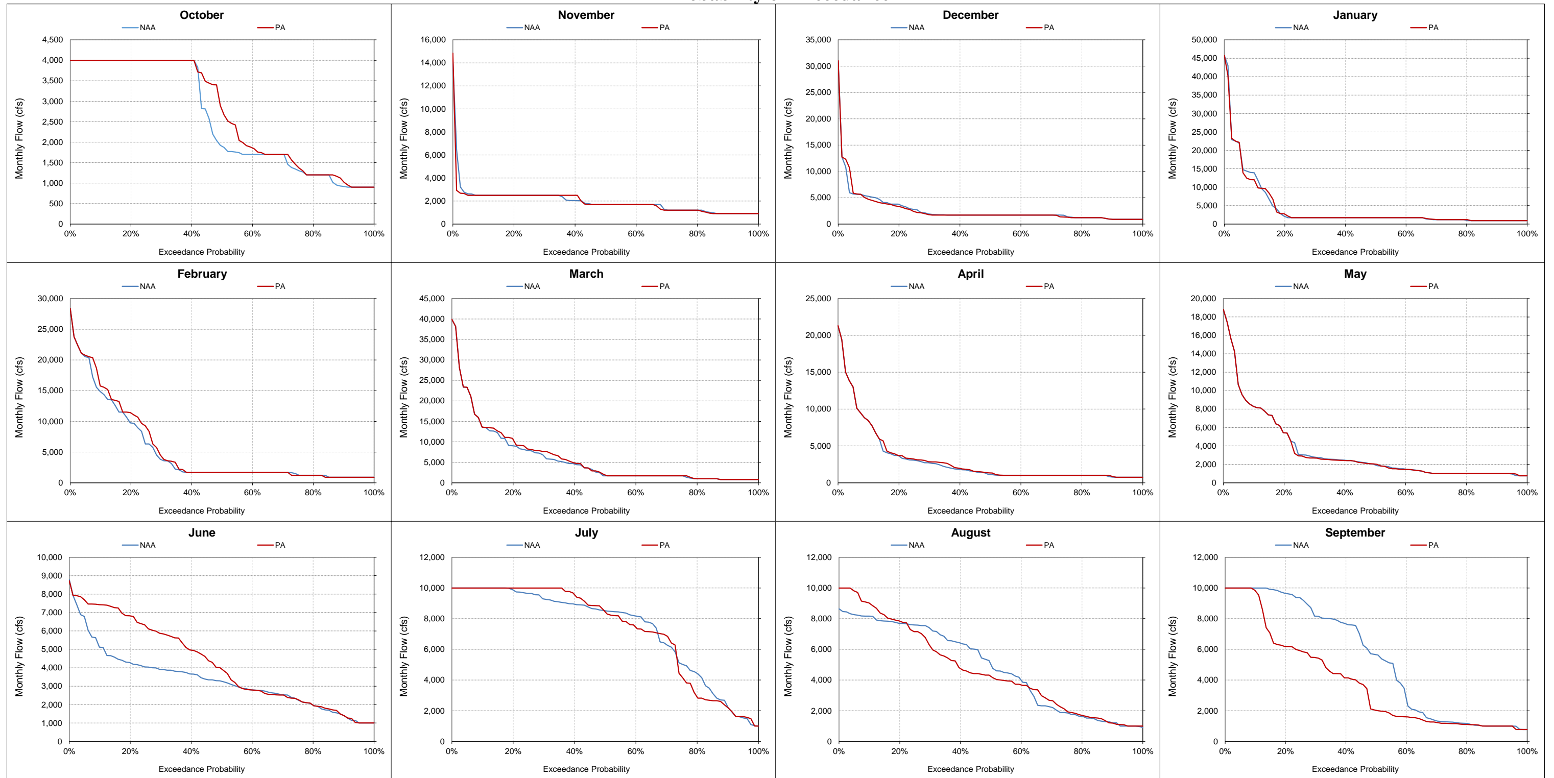
Figure 5.A.6-12-7. Feather River below Thermalito Diversion Dam, Monthly Flow Probability of Exceedance
