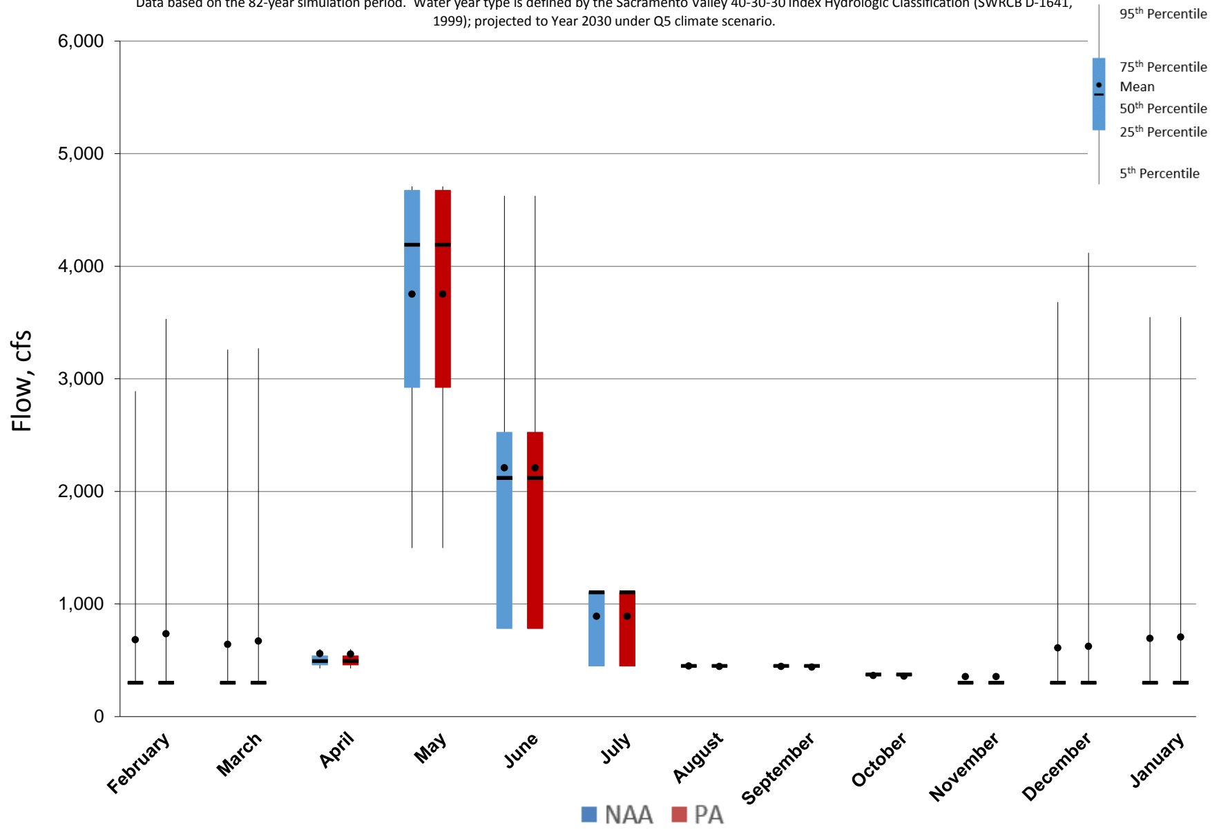
Figure 5.A.6-7-1. Monthly Flow Ranges For Trinity River below Lewiston Dam, All Years
