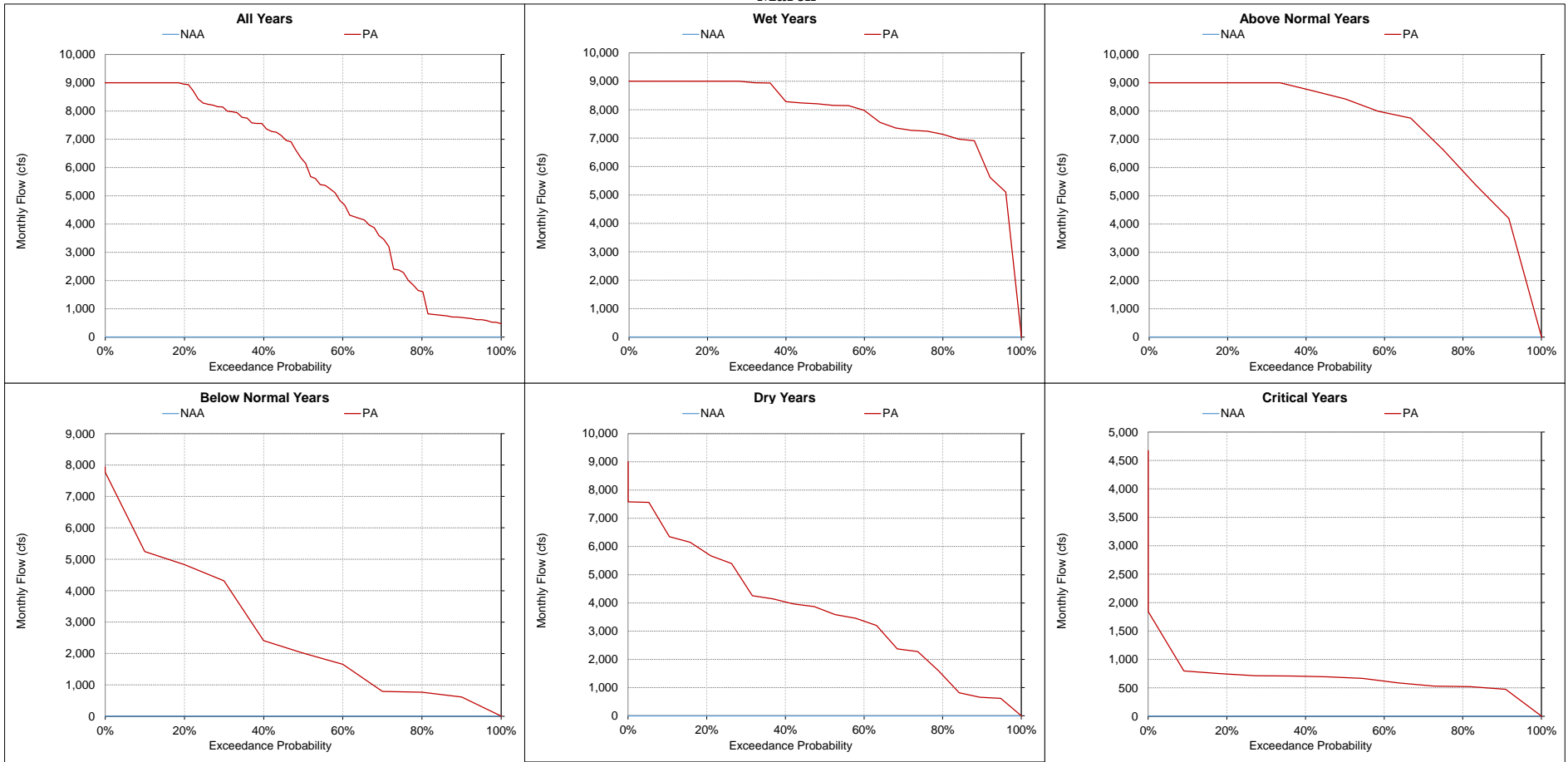
Figure 5.A.6-19-13. North Delta Diversions near Hood, Monthly Flow March
