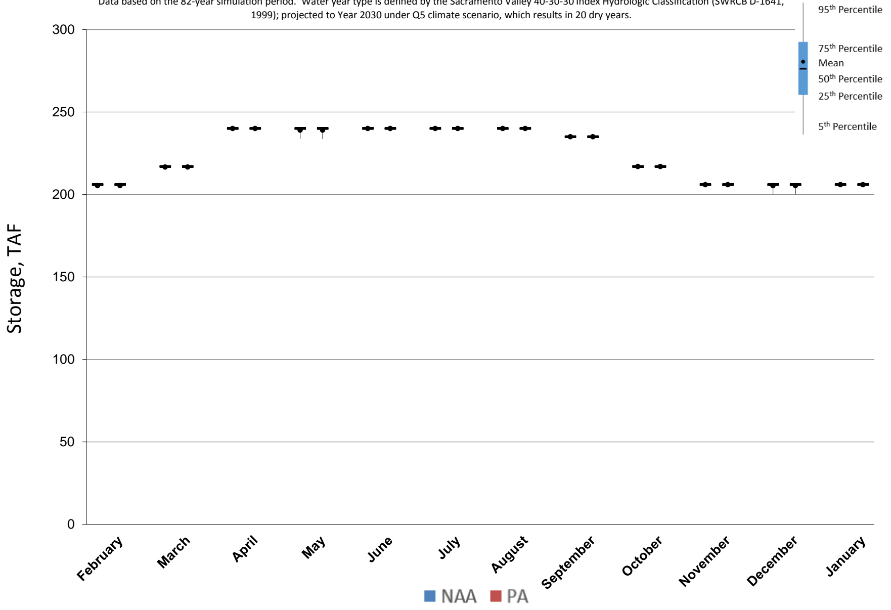
Figure 5.A.6-2-5. End of Month Storage Ranges For Whiskeytown Reservoir, Dry Years
