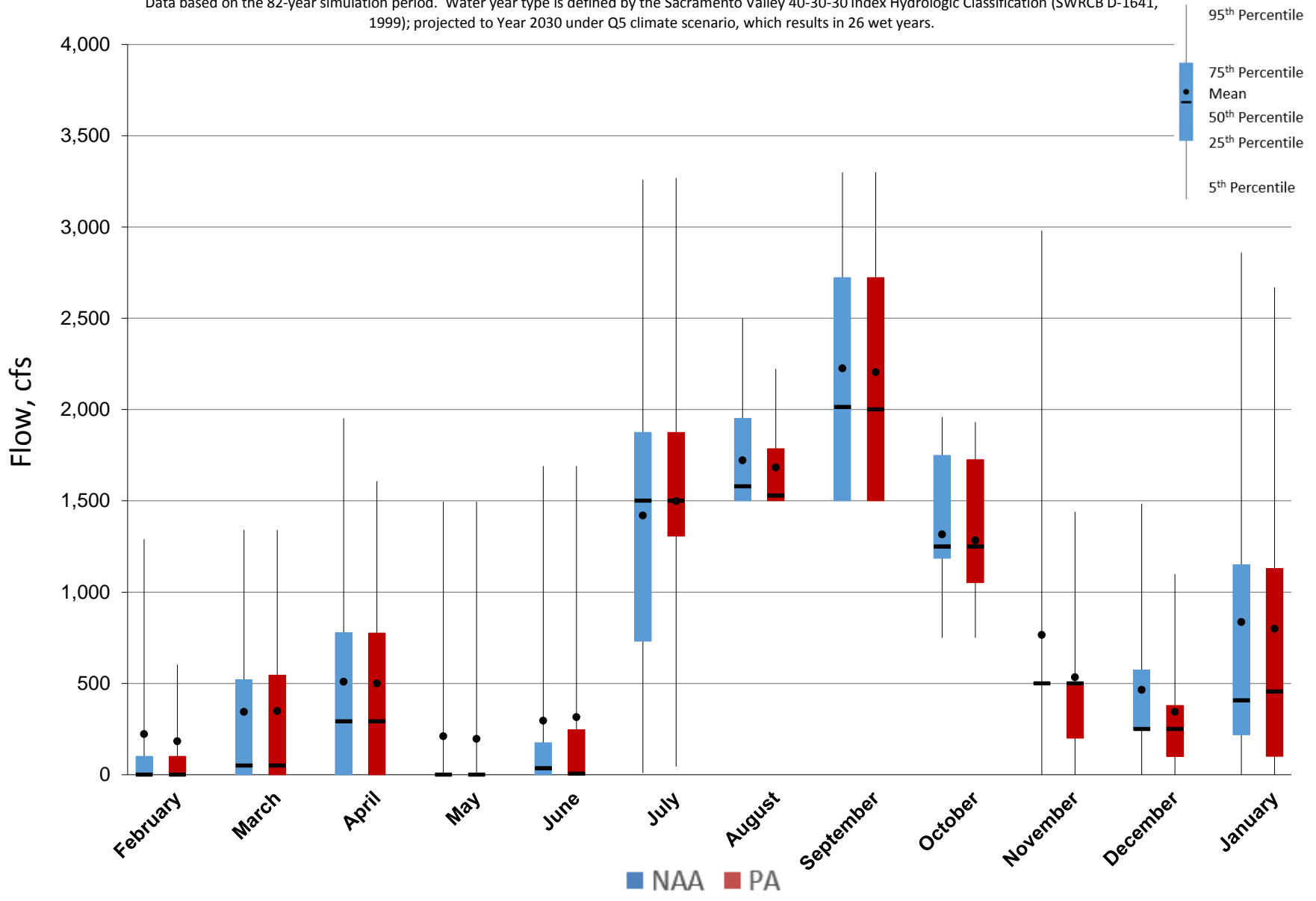
Figure 5.A.6-8-2. Monthly Flow Ranges For Clear Creek Tunnel Flow, Wet Years
