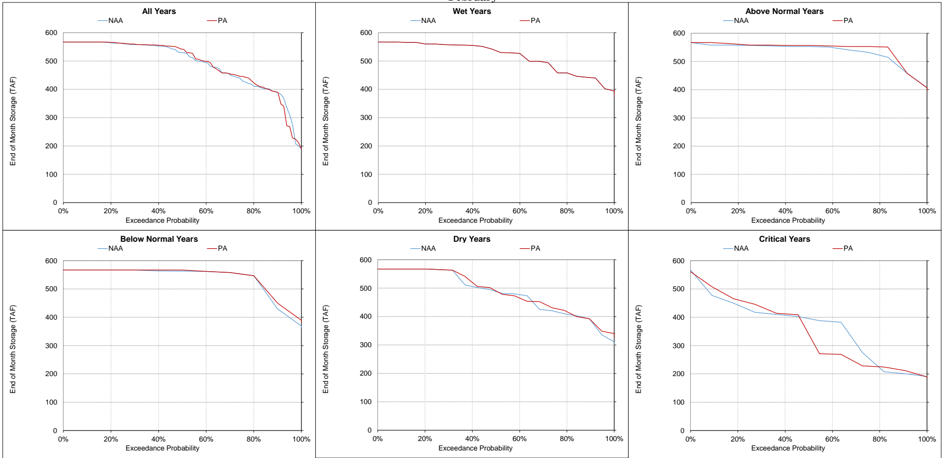
Figure 5.A.6-5-12. Folsom Lake, End of Month Storage February
