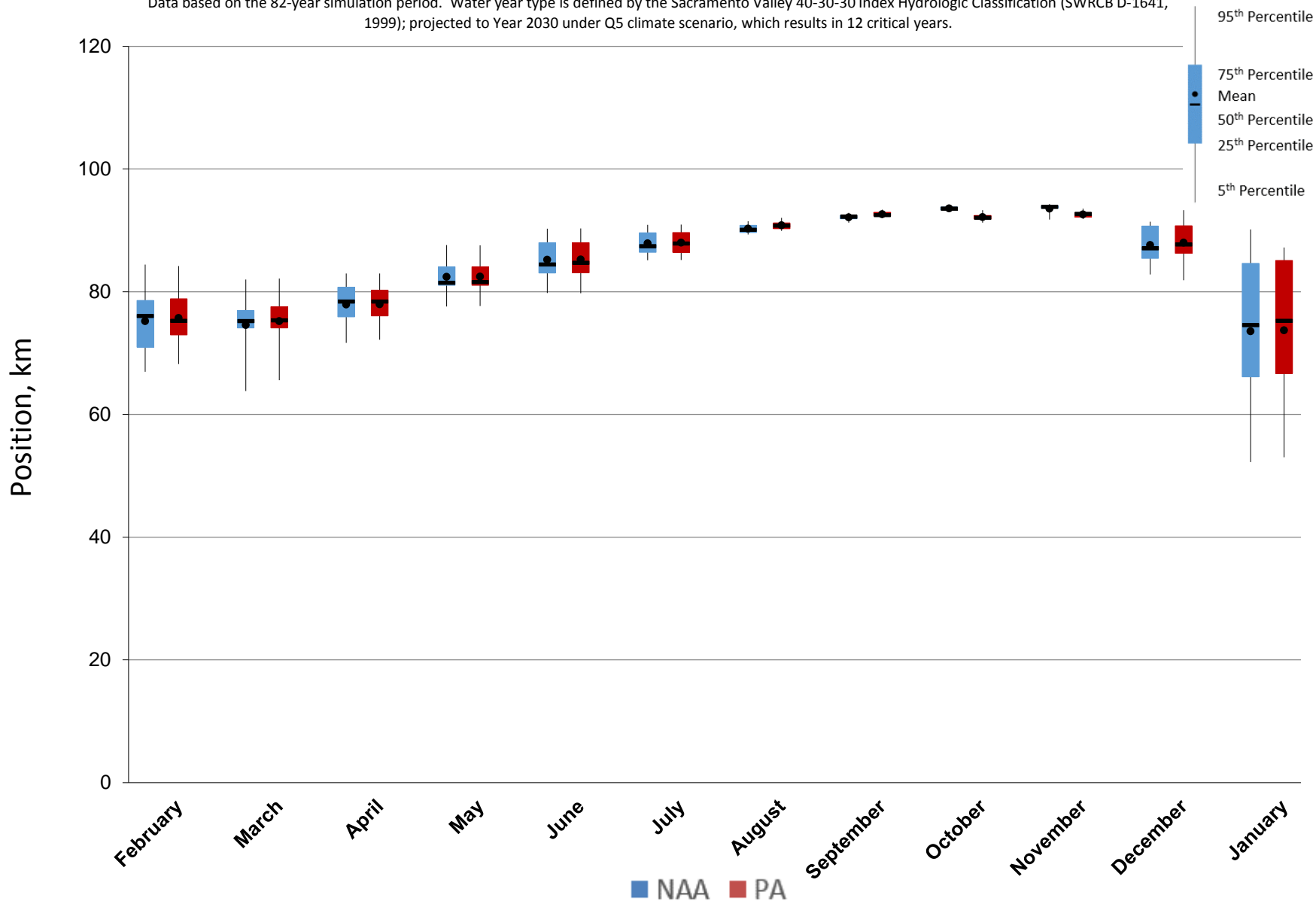
Figure 5.A.6-29-6. End of Month Position Ranges For X2, Critical Years
