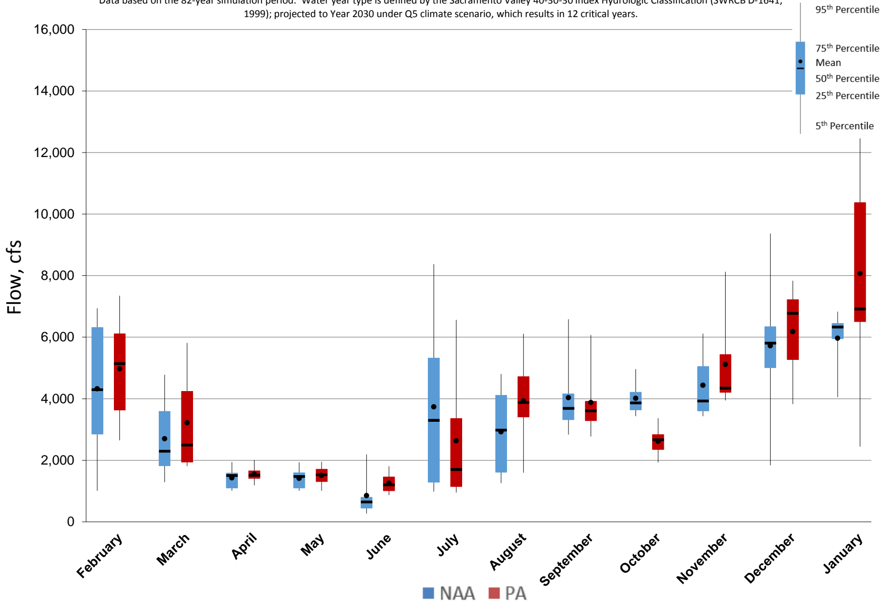
Figure 5.A.6-28-6. Monthly Flow Ranges For Total Delta Exports, Critical Years
