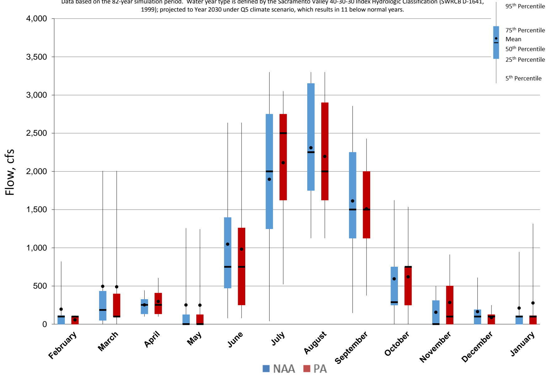
Figure 5.A.6-8-4. Monthly Flow Ranges For Clear Creek Tunnel Flow, Below Normal Years
