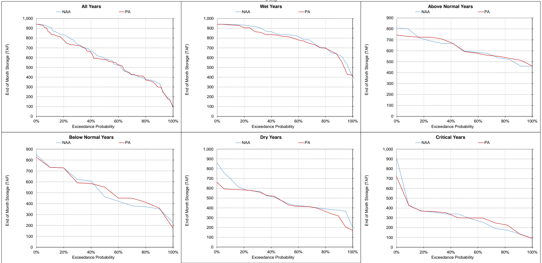
Figure 5.A.6-5-17. Folsom Lake, End of Month Storage July
