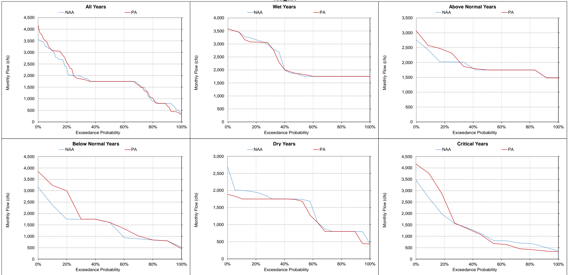
Figure 5.A.6-16-18. American River below Nimbus Dam, Monthly Flow August
