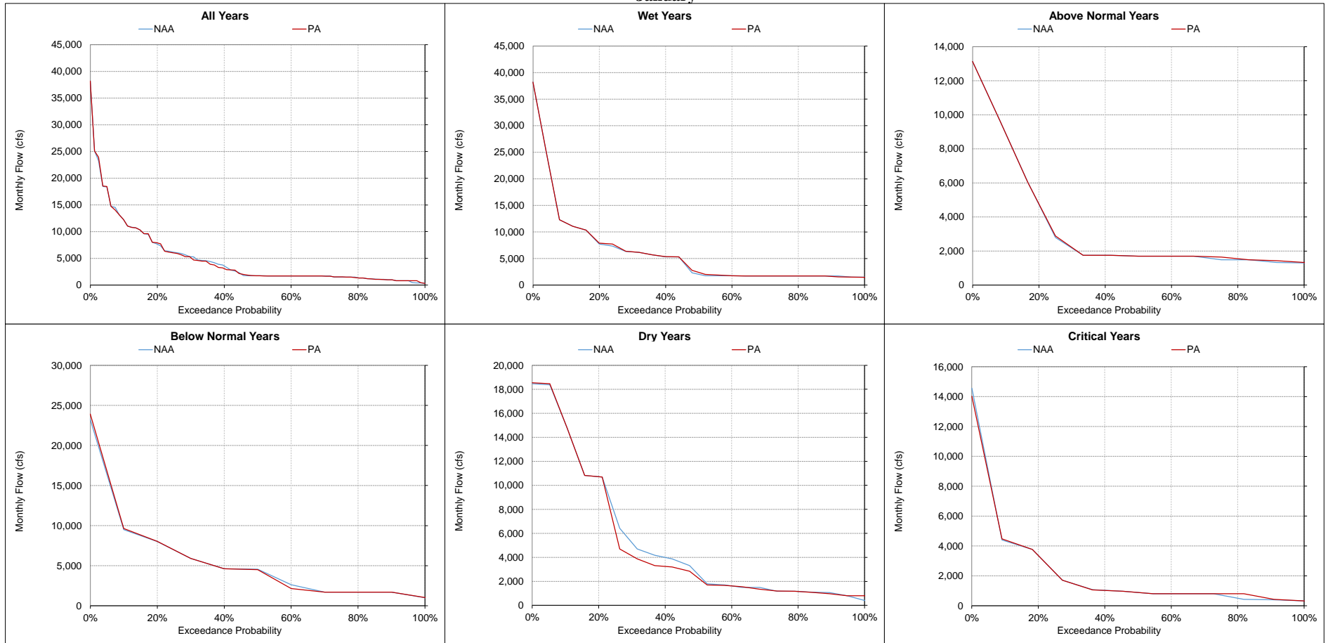
Figure 5.A.6-16-11. American River below Nimbus Dam, Monthly Flow January
