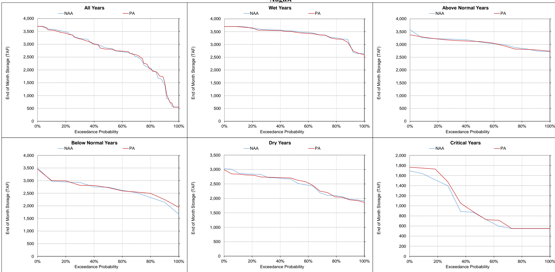
Figure 5.A.6-3-18. Shasta Lake, End of Month Storage August
