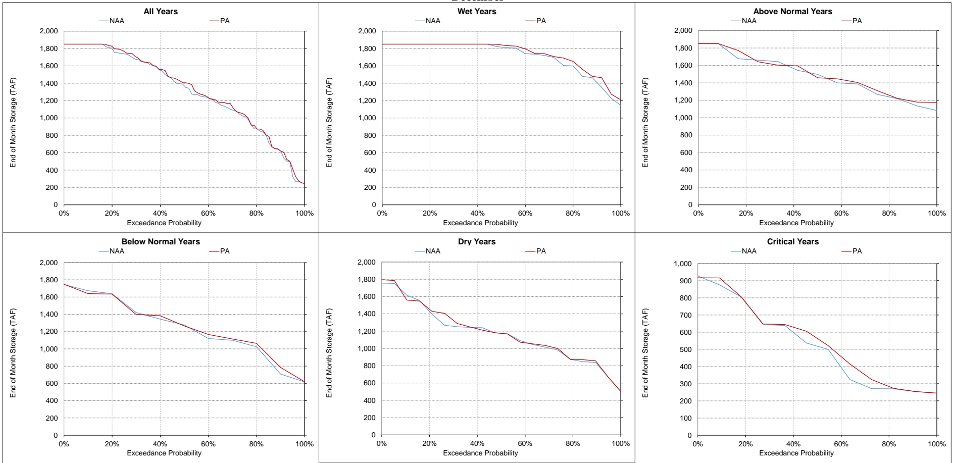
Figure 5.A.6-1-10. Trinity Lake, End of Month Storage December
