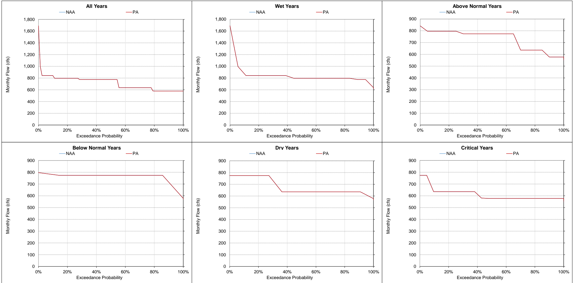
Figure 5.A.6-21-8. Stanislaus River at Ripon, Monthly Flow October
