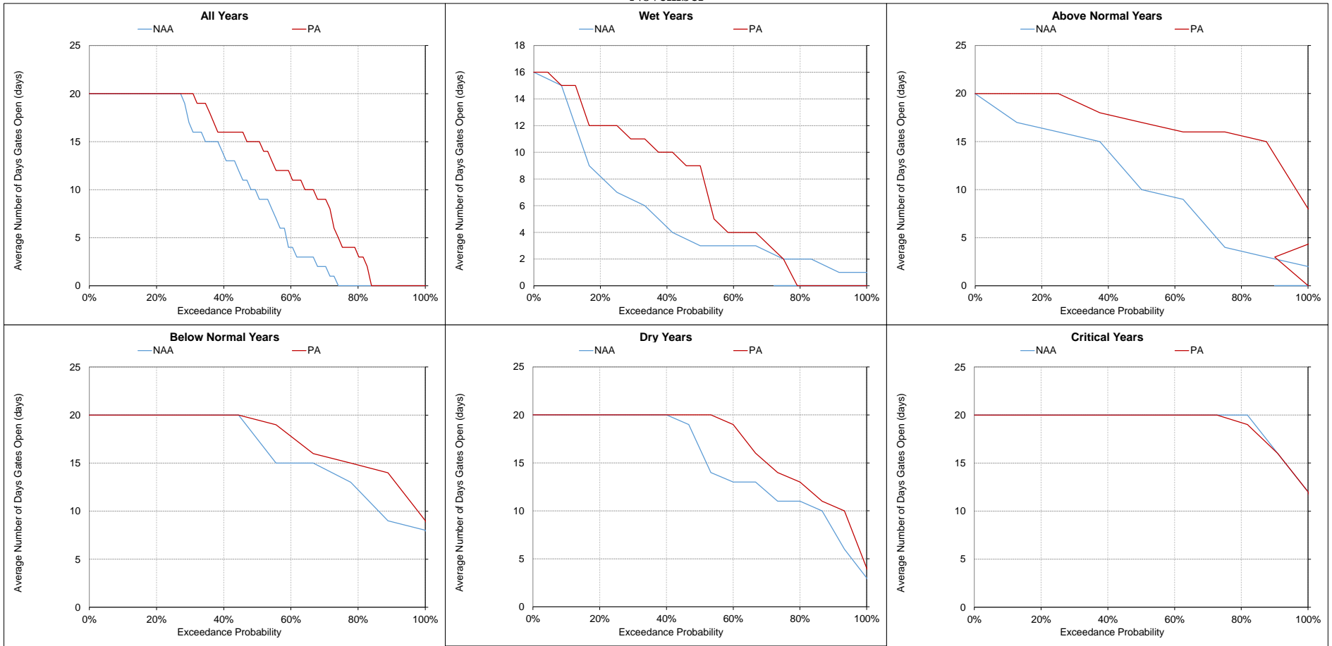
Figure 5.A.6-31-9. Delta Cross Channel, Average Number of Days Gates Open November
