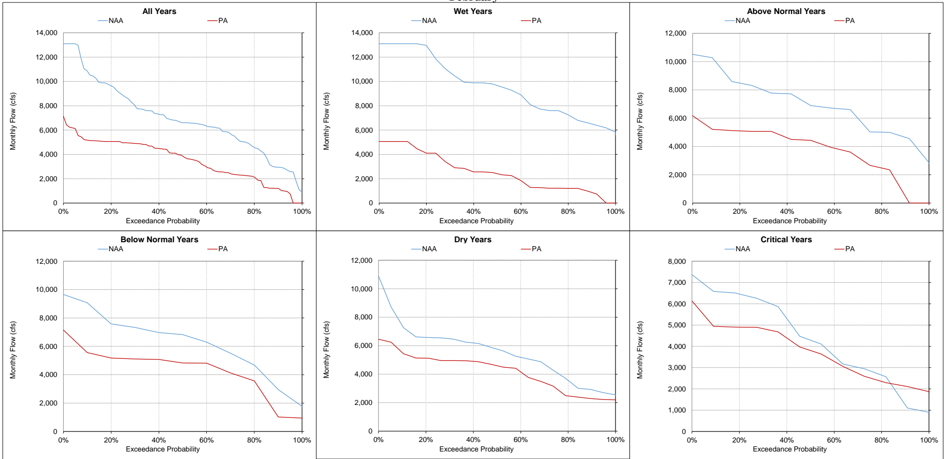
Figure 5.A.6-27-12. South Delta Exports, Monthly Flow February
