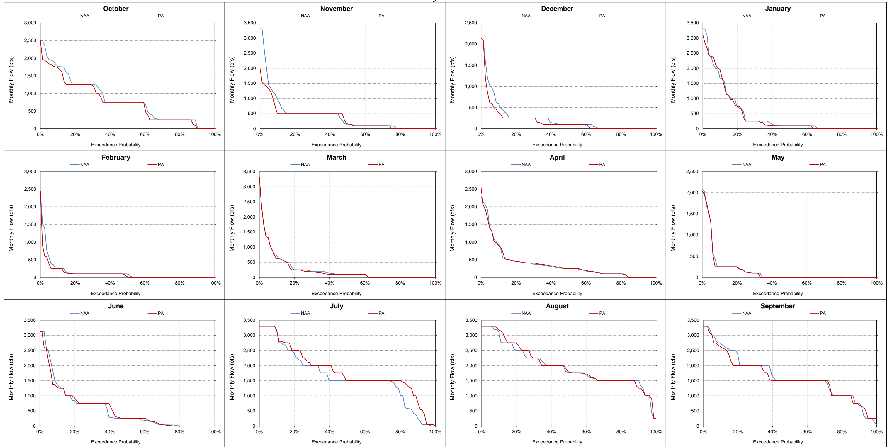
Figure 5.A.6-8-7. Clear Creek Tunnel Flow, Monthly Flow Probability of Exceedance
