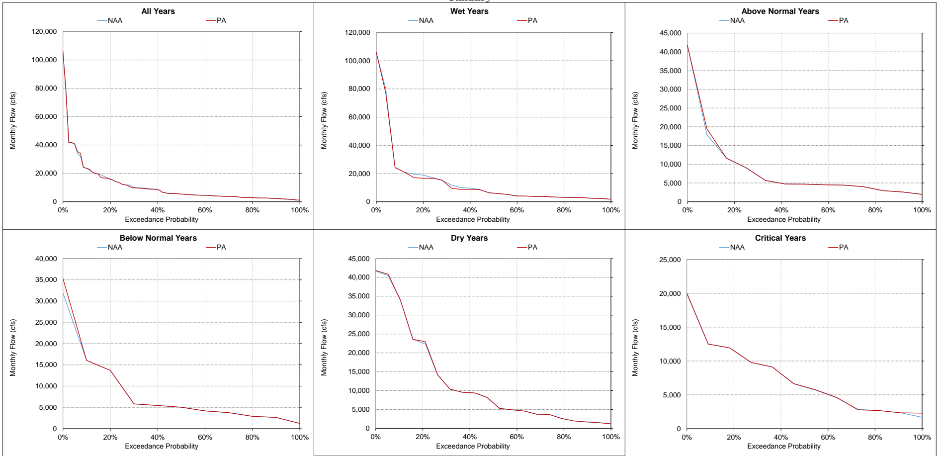
Figure 5.A.6-13-11. Feather River at Sacramento River Confluence, Monthly Flow January
