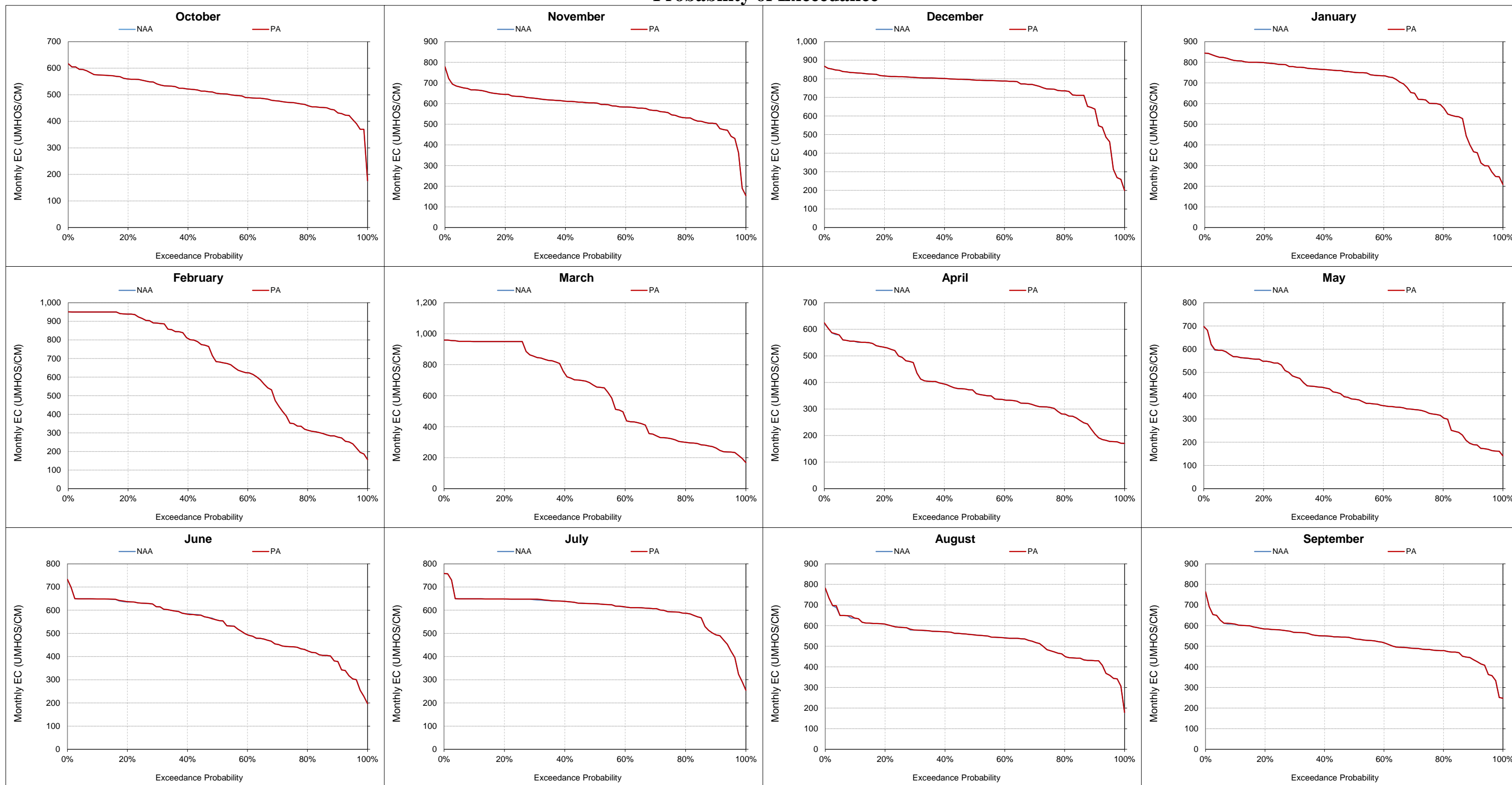
Figure 5.A.6-30-7. San Joaquin River at Vernalis, Monthly EC Probability of Exceedance
