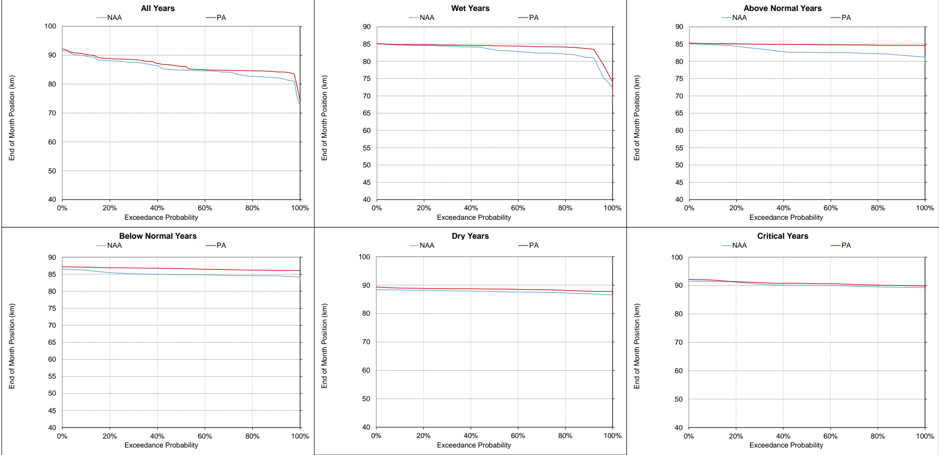
Figure 5.A.6-29-18. X2, End of Month Position August
