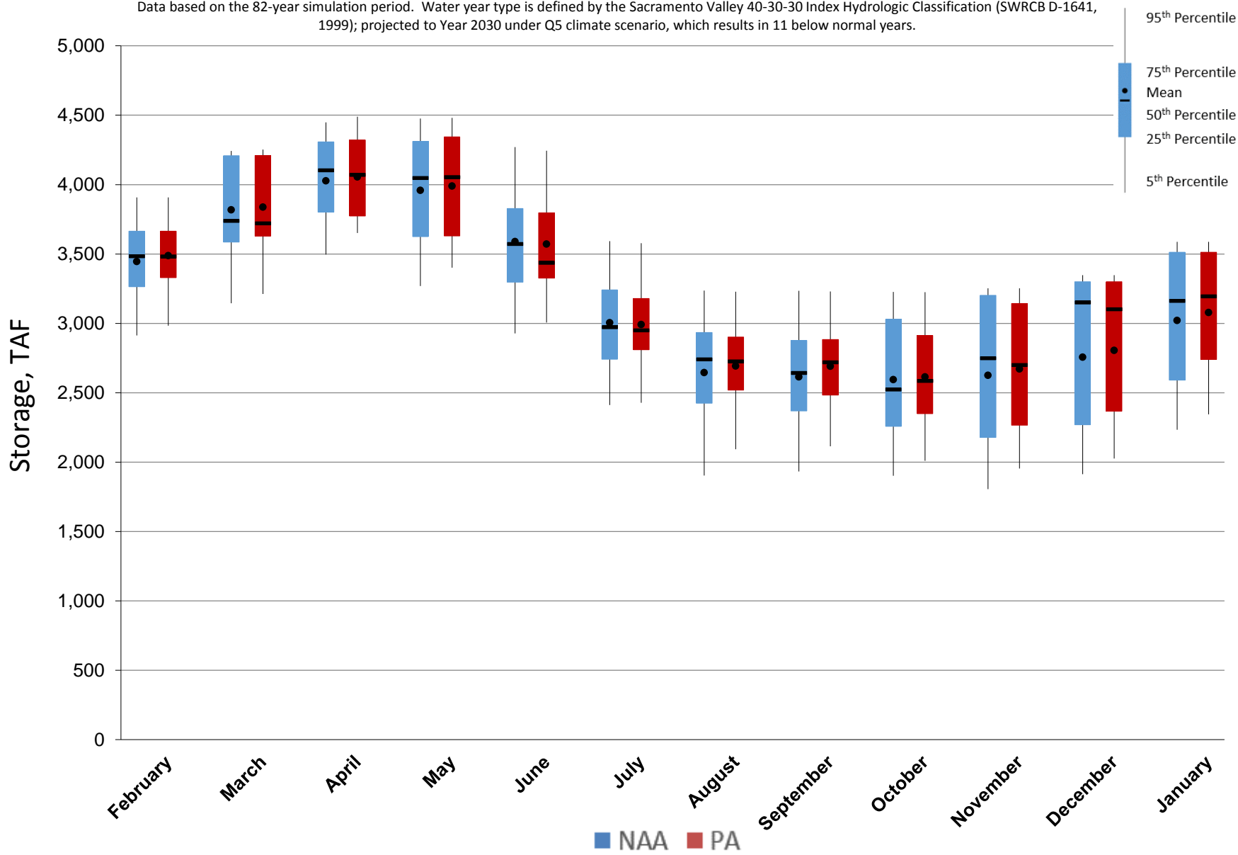
Figure 5.A.6-3-4. End of Month Storage Ranges For Shasta Lake, Below Normal Years
