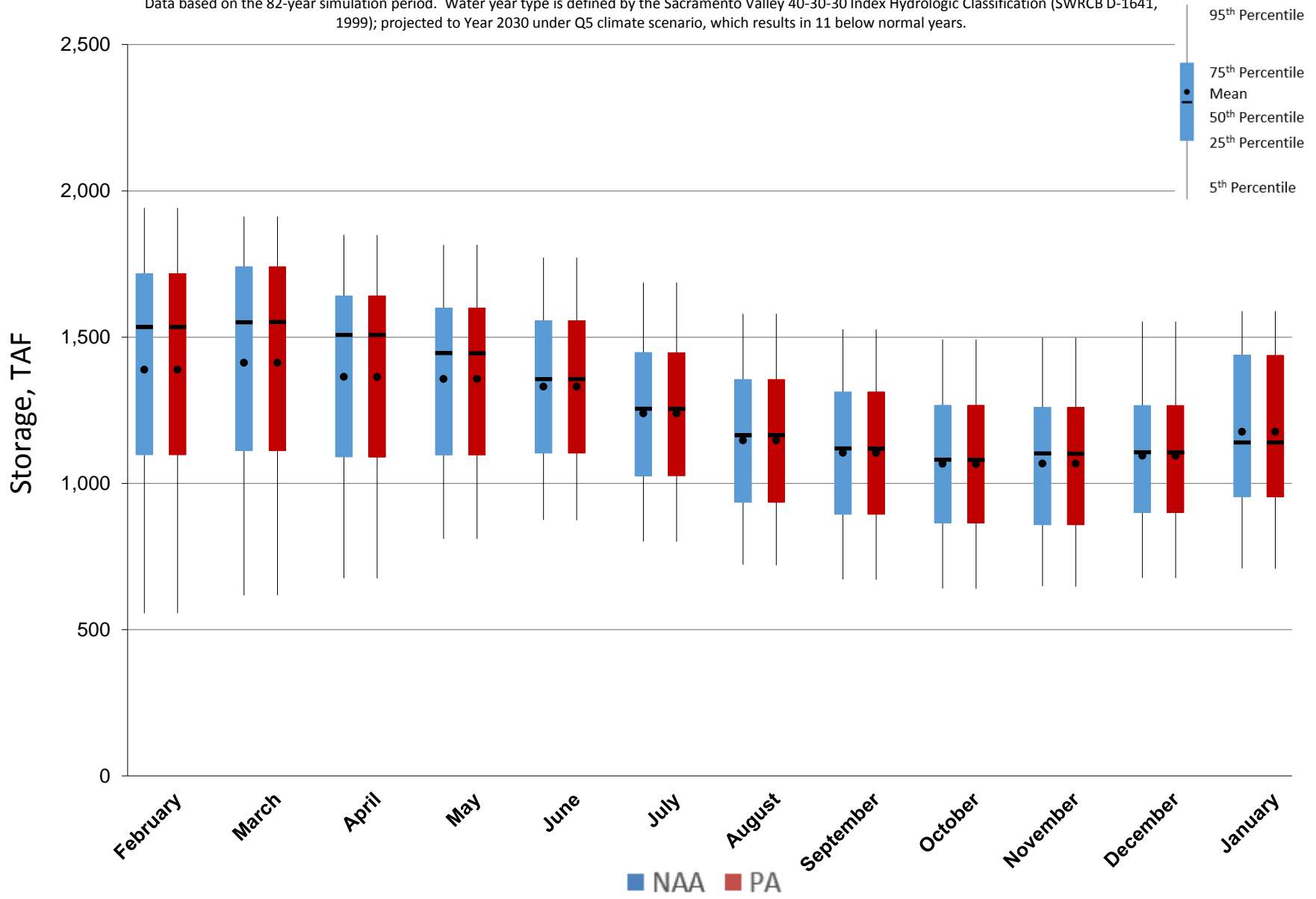
Figure 5.A.6-6-4. End of Month Storage Ranges For New Melones Lake, Below Normal Years
