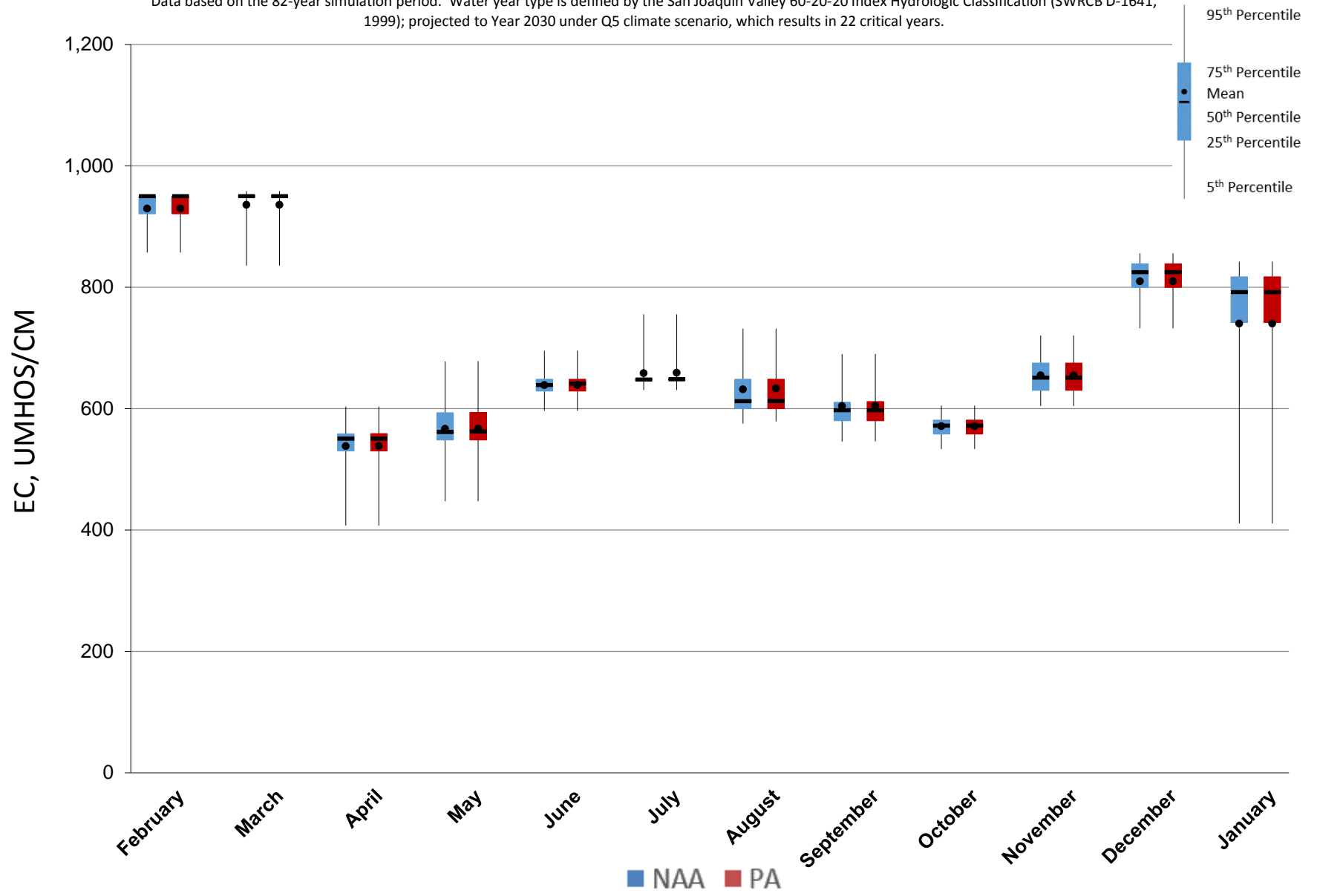
Figure 5.A.6-30-6. Monthly EC Ranges for San Joaquin River at Vernalis, Critical Years
