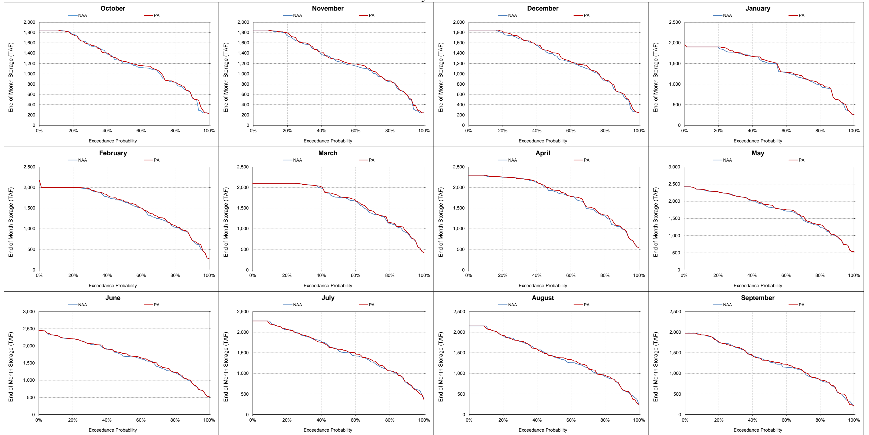
Figure 5.A.6-1-7. Trinity Lake, End of Month Storage Probability of Exceedance
