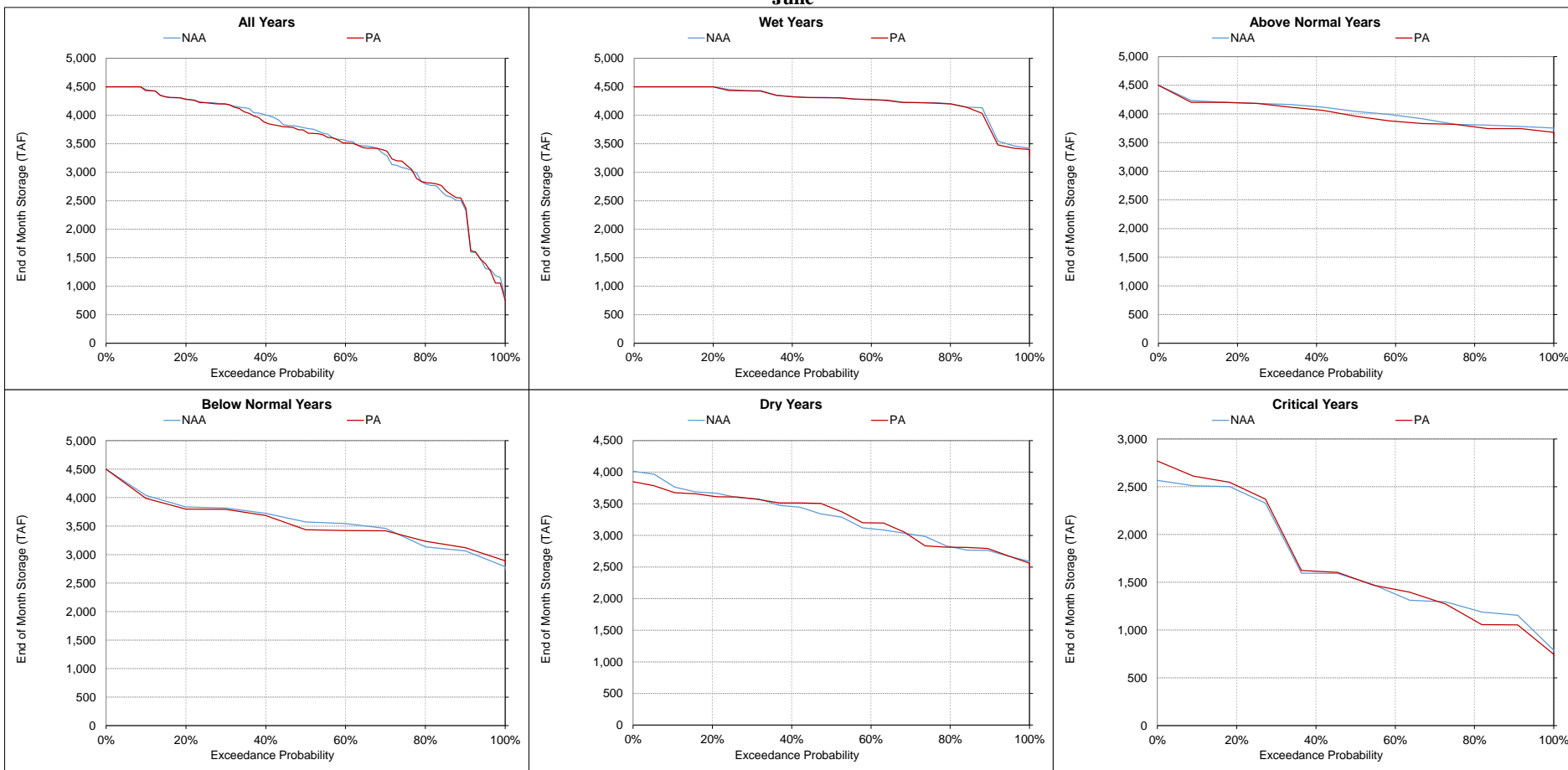
Figure 5.A.6-3-16. Shasta Lake, End of Month Storage June
