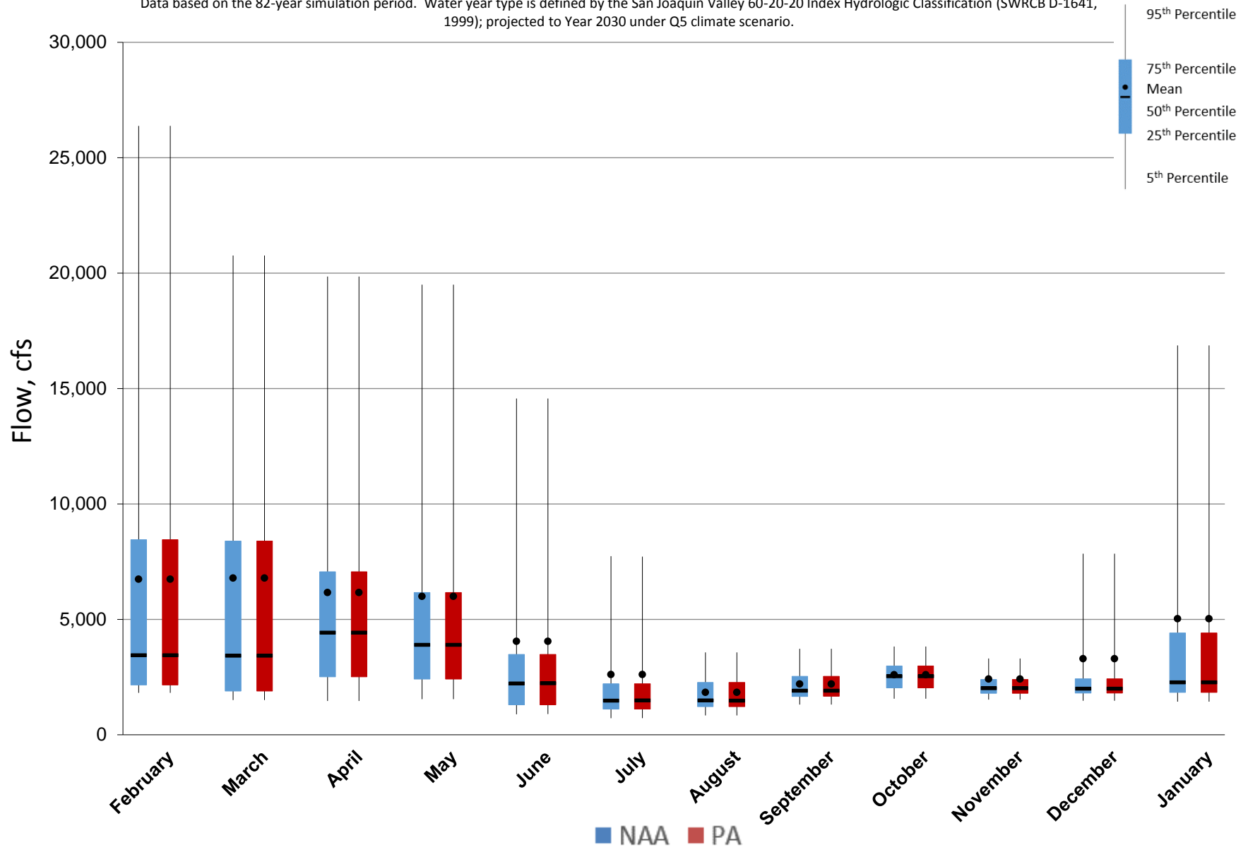
Figure 5.A.6-23-1. Monthly Flow Ranges for San Joaquin River at Vernalis, All Years
