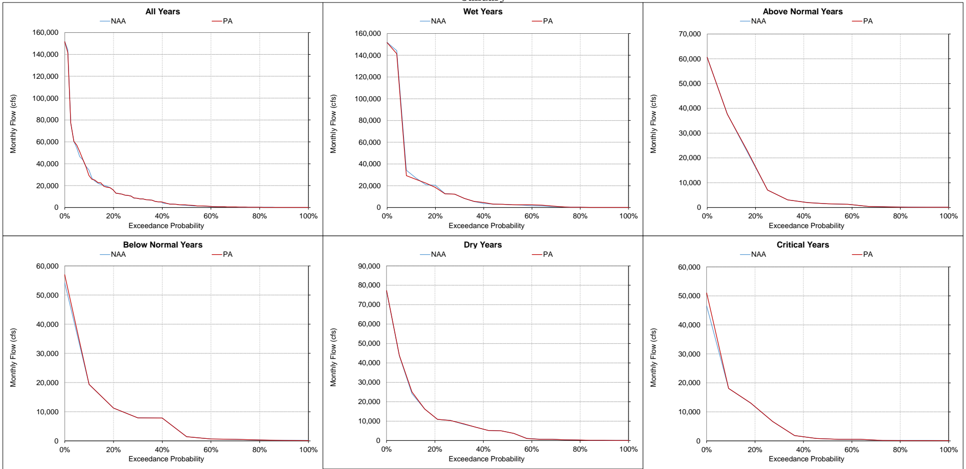
Figure 5.A.6-20-11. Yolo Bypass, Monthly Flow January
