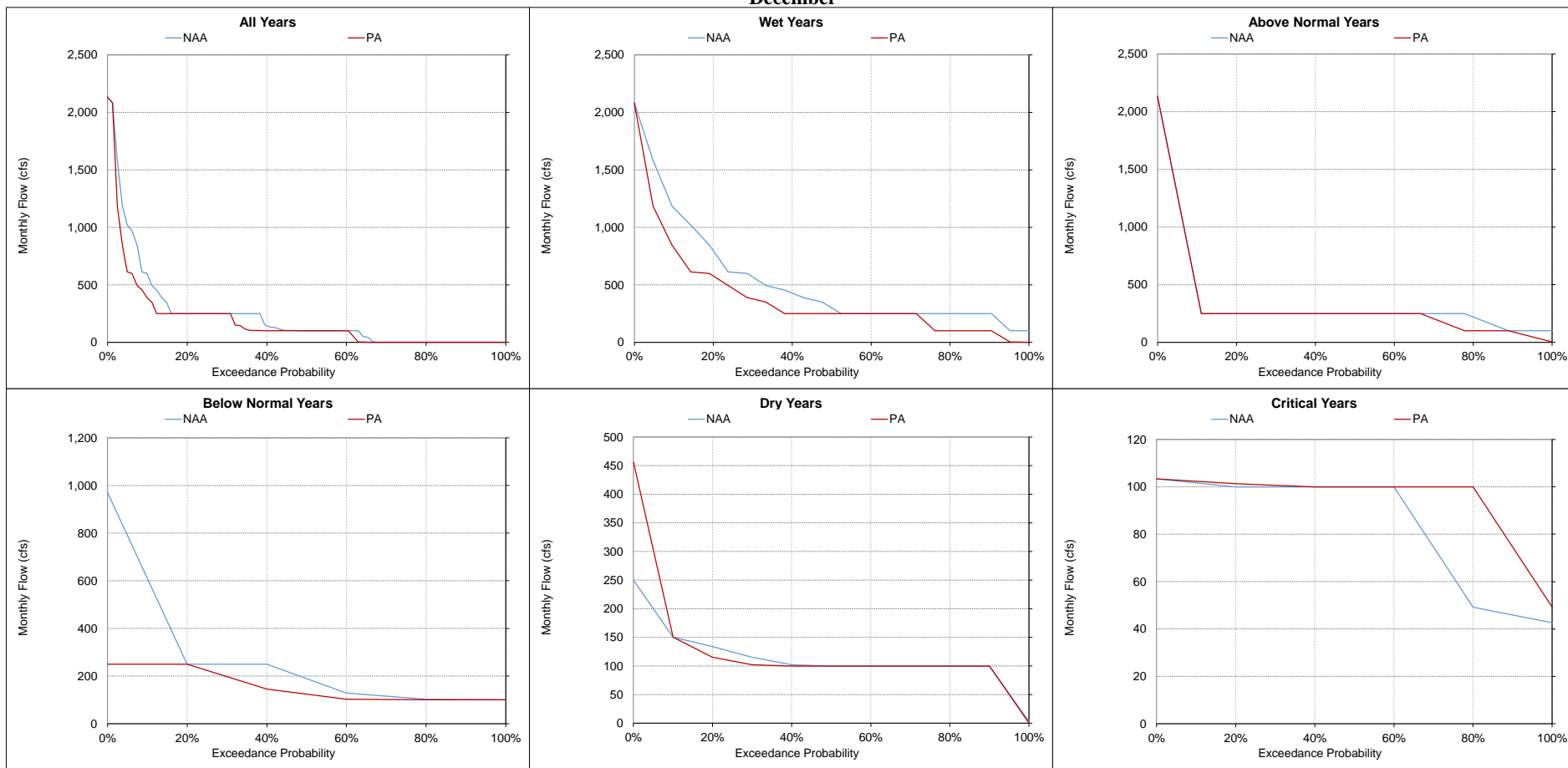
Figure 5.A.6-8-10. Clear Creek Tunnel Flow, Monthly Flow December
