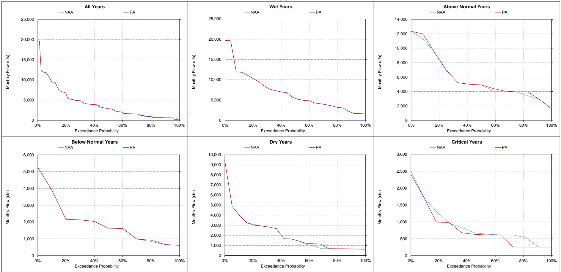
Figure 5.A.6-17-13. American River at Sacramento River Confluence, Monthly Flow March
