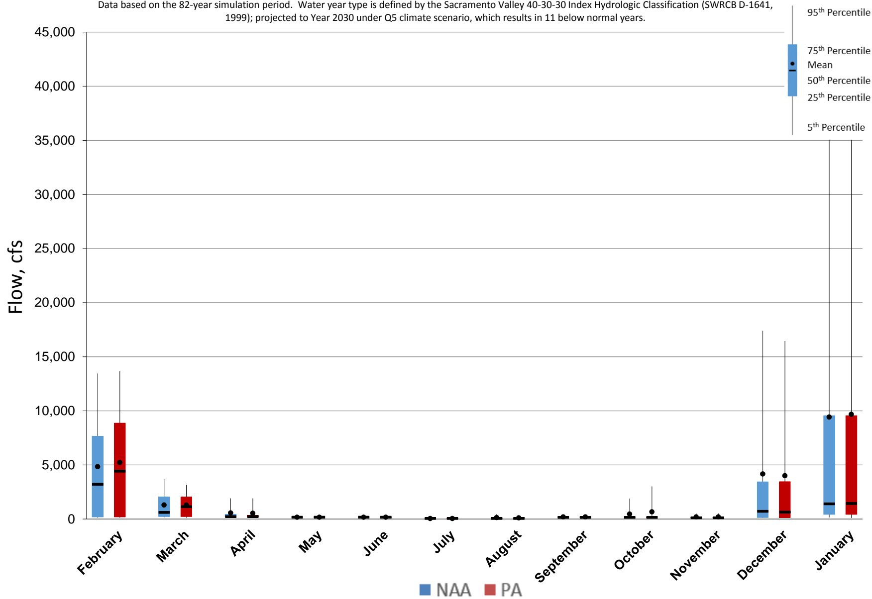
Figure 5.A.6-20-4. Monthly Flow Ranges For Yolo Bypass, Below Normal Years
