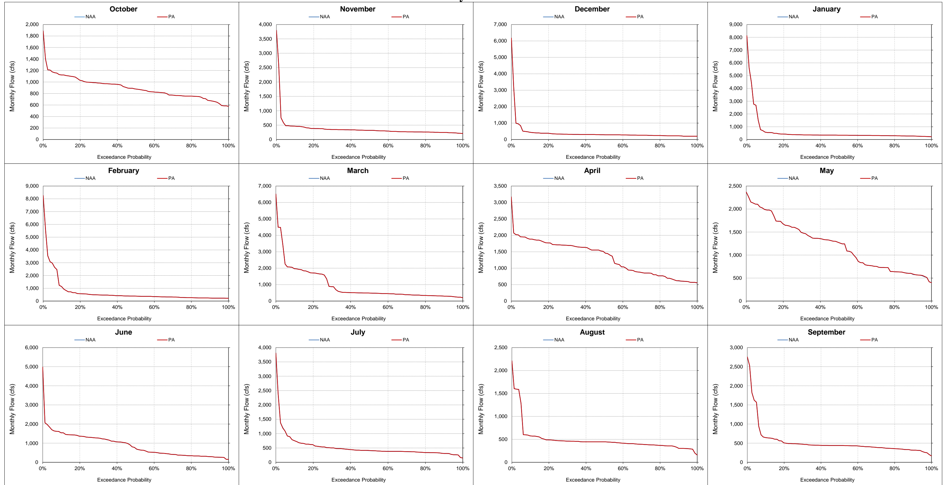
Figure 5.A.6-22-7. Stanislaus River at Mouth, Monthly Flow Probability of Exceedance
