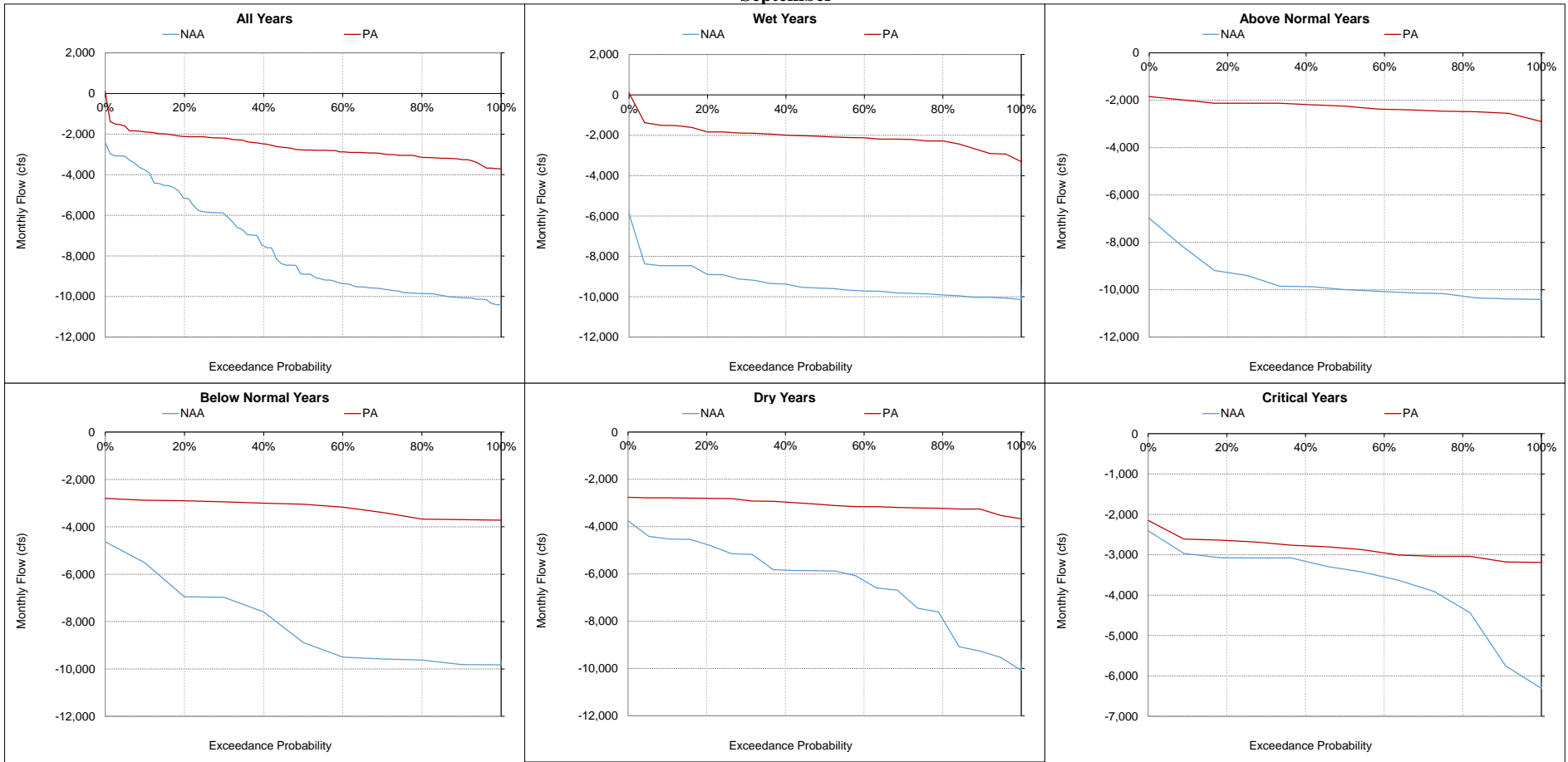
Figure 5.A.6-25-19. Old and Middle River, Monthly Flow September
