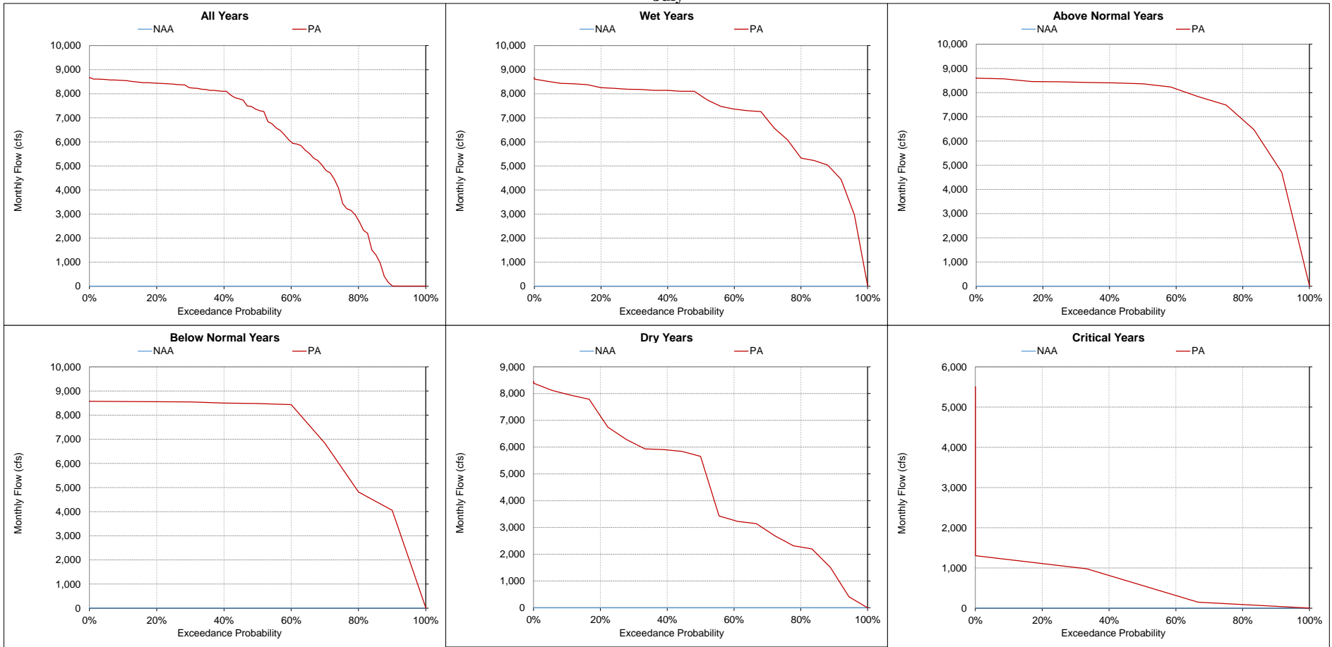
Figure 5.A.6-19-17. North Delta Diversions near Hood, Monthly Flow July
