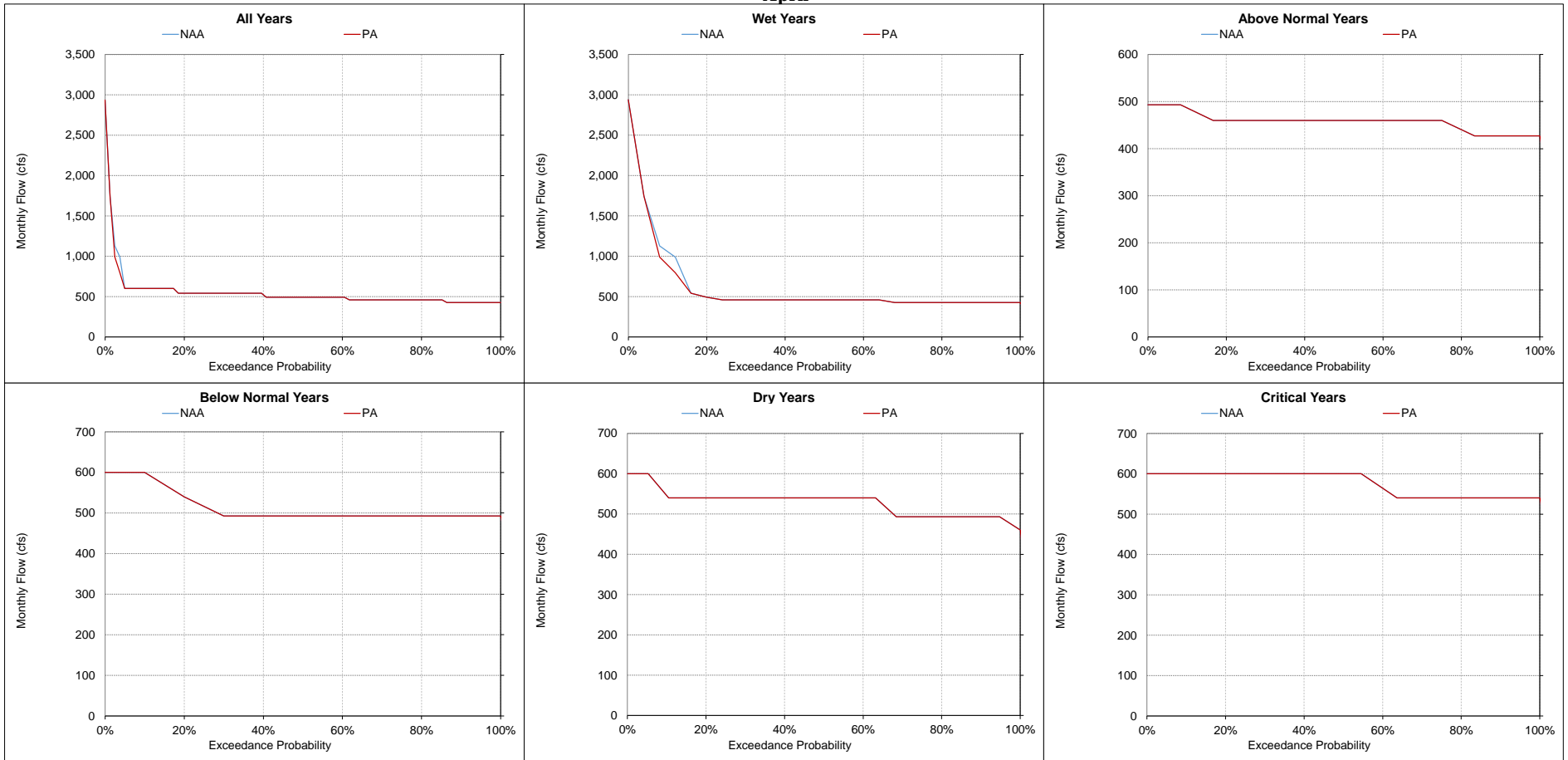
Figure 5.A.6-7-14. Trinity River below Lewiston Dam, Monthly Flow April
