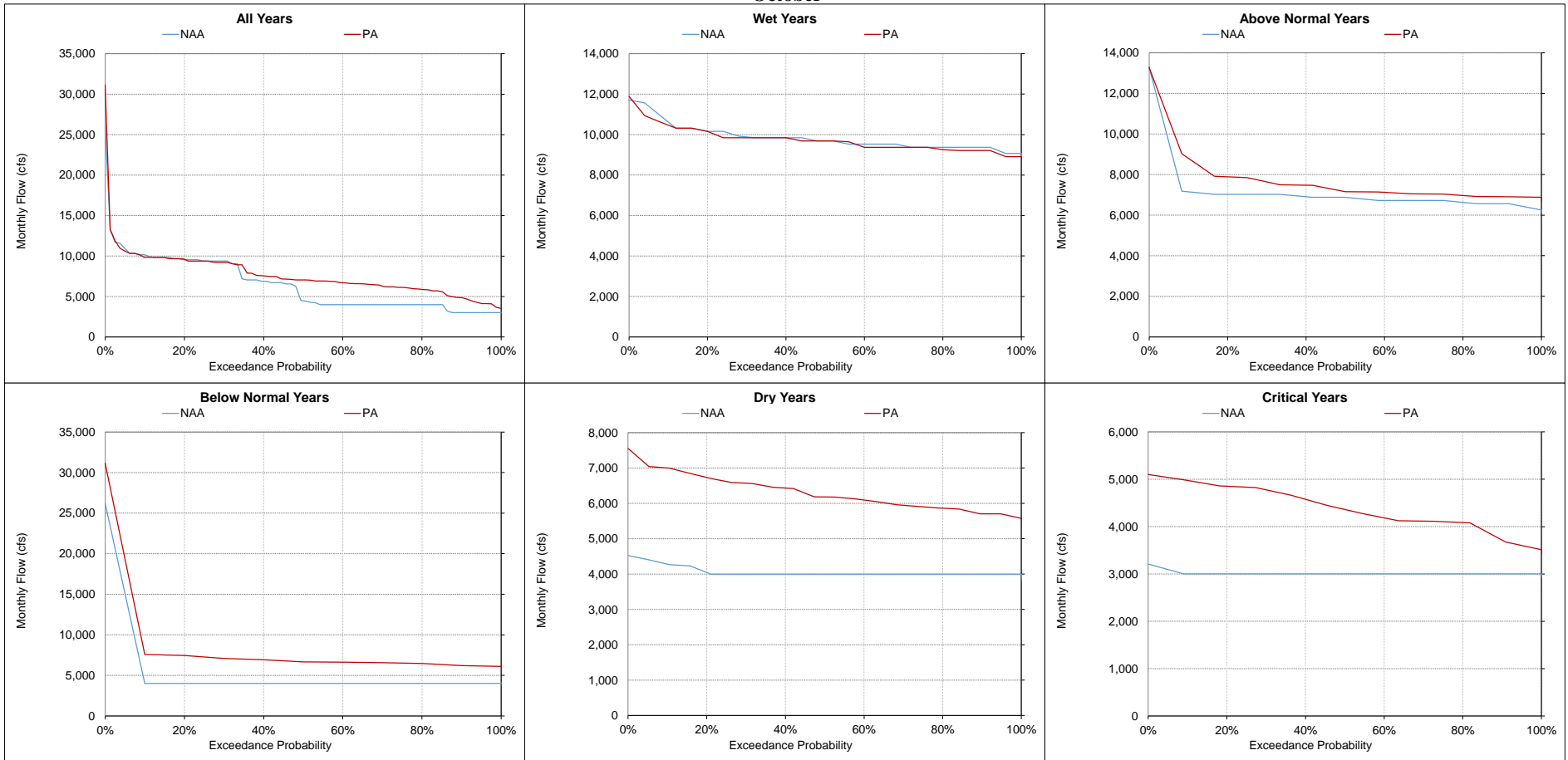
Figure 5.A.6-26-8. Delta Outflow, Monthly Flow October
