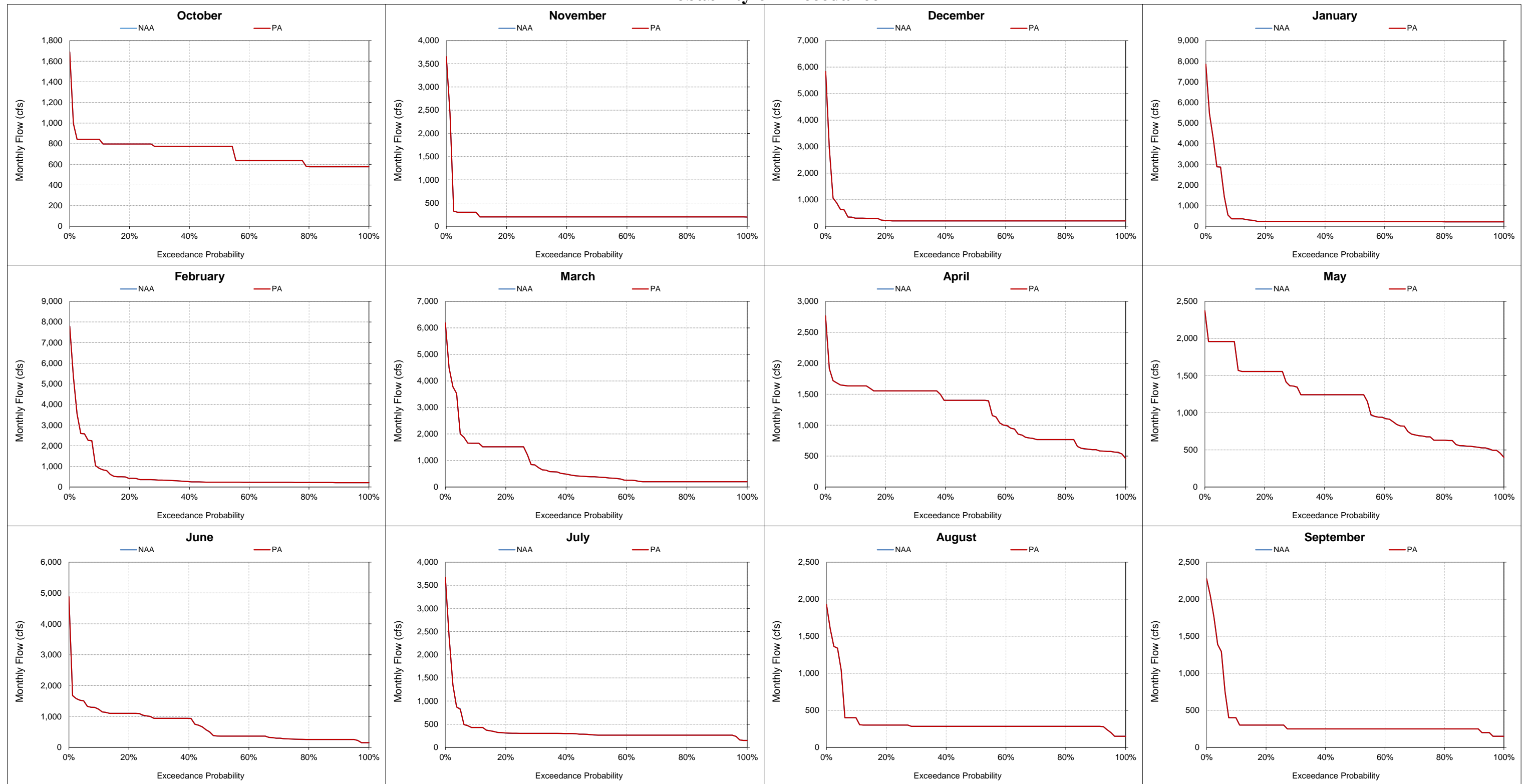
Figure 5.A.6-21-7. Stanislaus River at Ripon, Monthly Flow Probability of Exceedance
