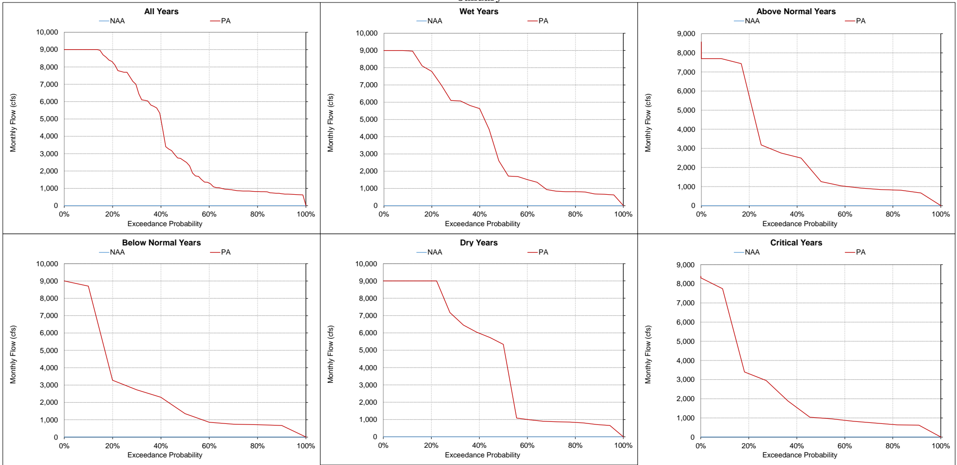
Figure 5.A.6-19-11. North Delta Diversions near Hood, Monthly Flow January
