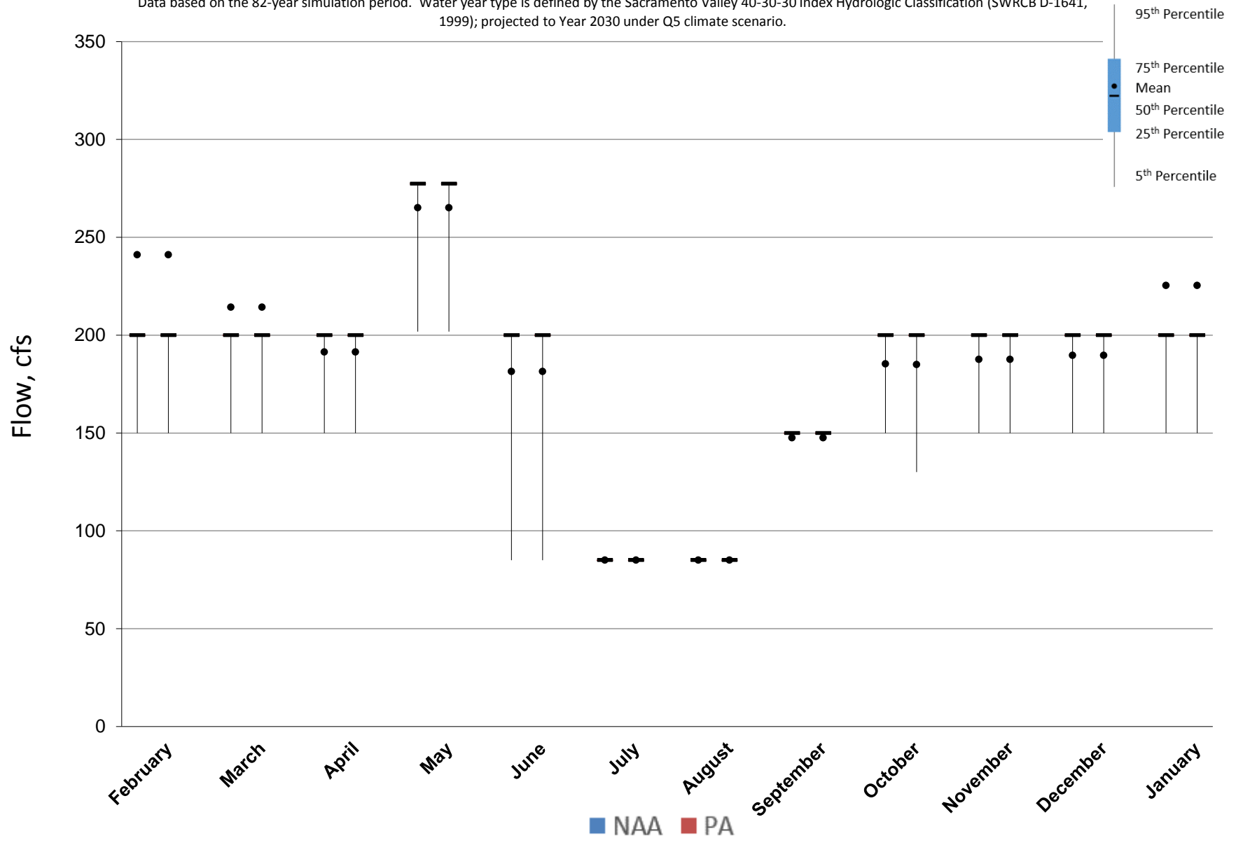
Figure 5.A.6-9-1. Monthly Flow Ranges For Clear Creek below Whiskeytown Dam, All Years
