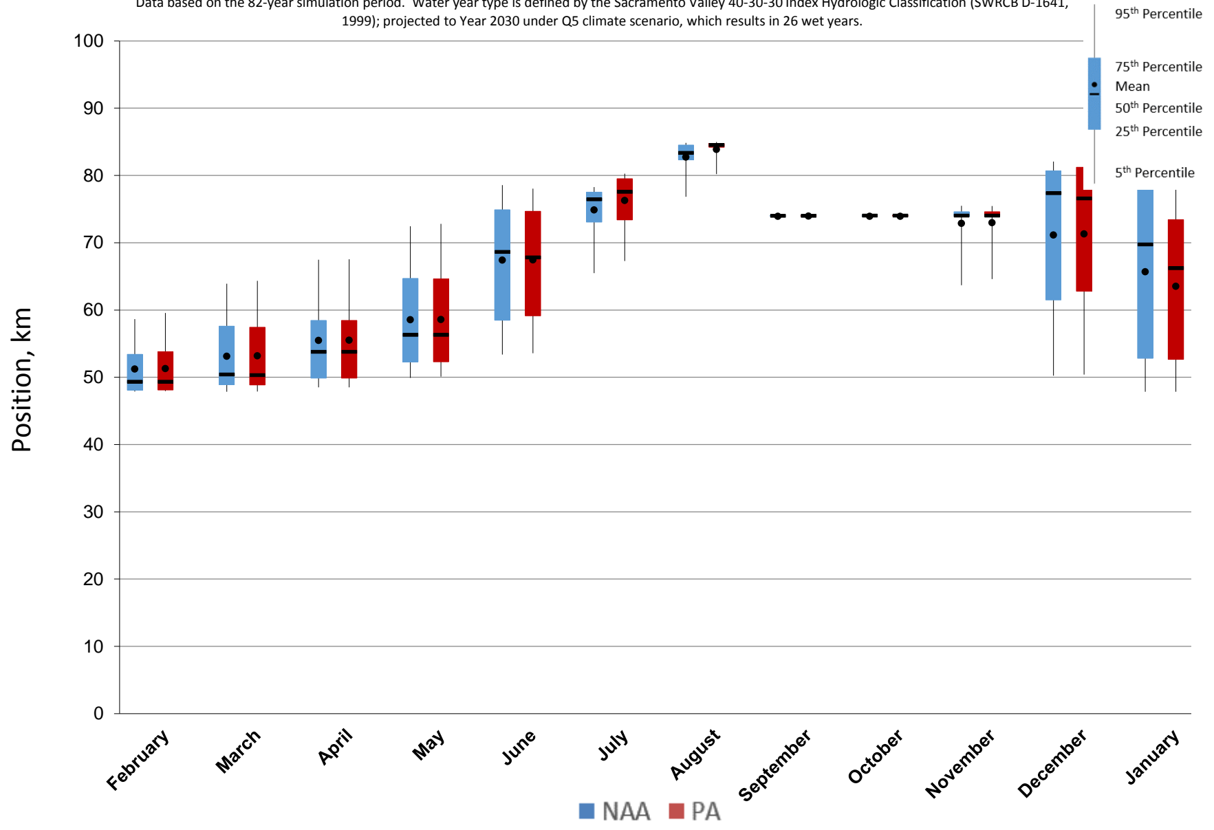
Figure 5.A.6-29-2. End of Month Position Ranges For X2, Wet Years
