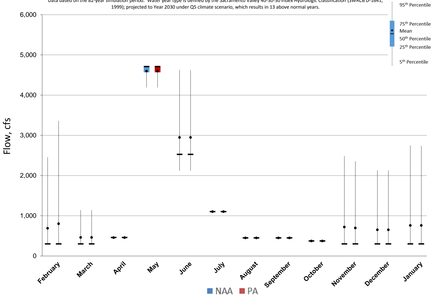
Figure 5.A.6-7-3. Monthly Flow Ranges For Trinity River below Lewiston Dam, Above Normal Years
