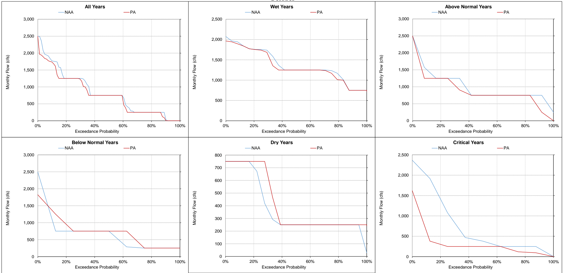
Figure 5.A.6-8-8. Clear Creek Tunnel Flow, Monthly Flow October
