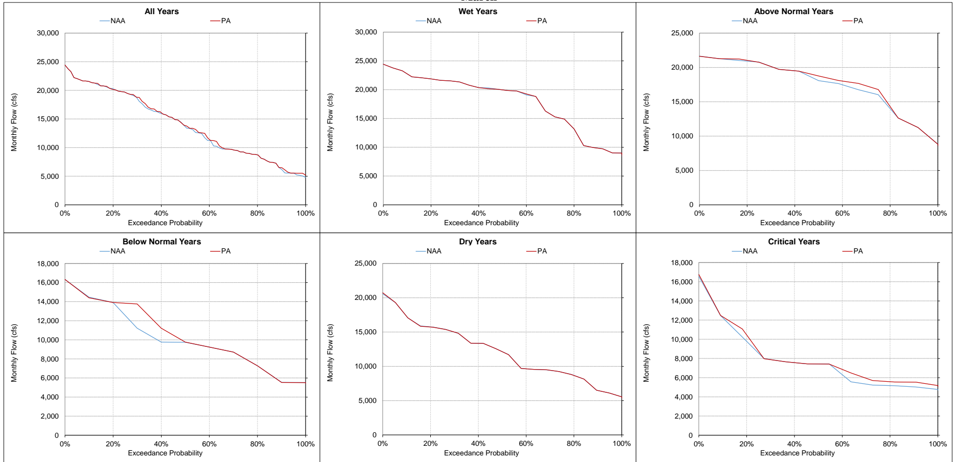
Figure 5.A.6-11-13. Sacramento River at Bend Bridge, Monthly Flow March
