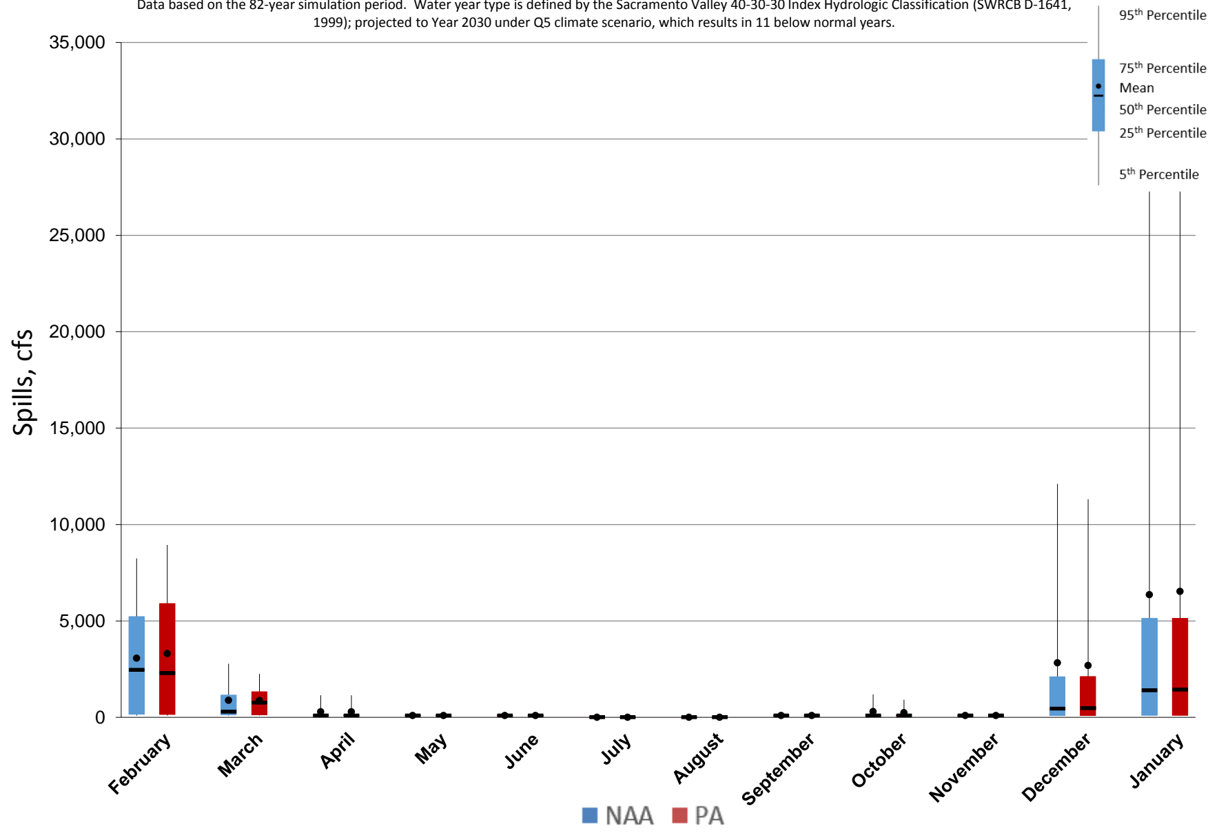
Figure 5.A.6-15-4. Monthly Spills Ranges For Fremont Weir, Below Normal Years
