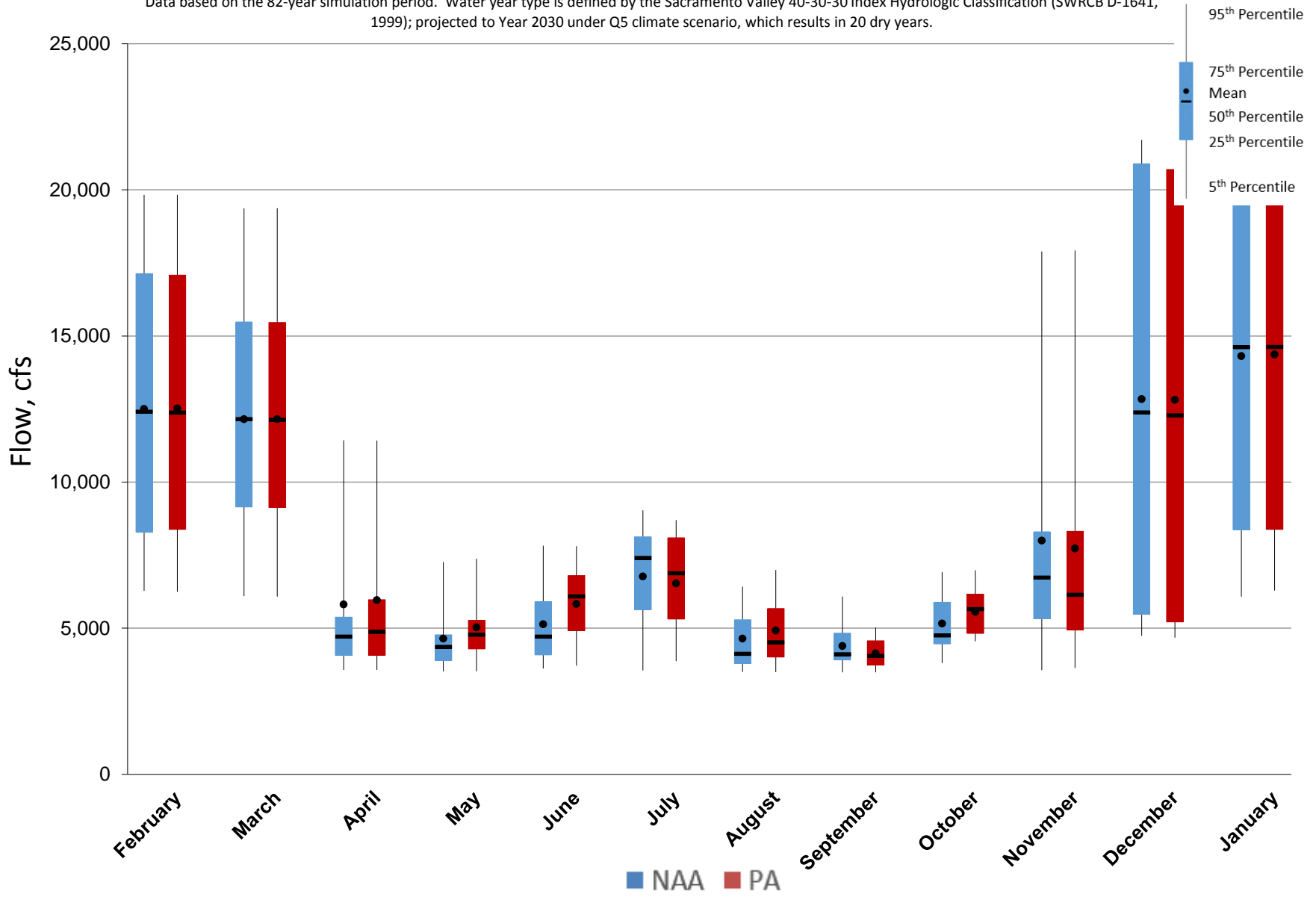
Figure 5.A.6-11-5. Monthly Flow Ranges For Sacramento River at Bend Bridge, Dry Years
