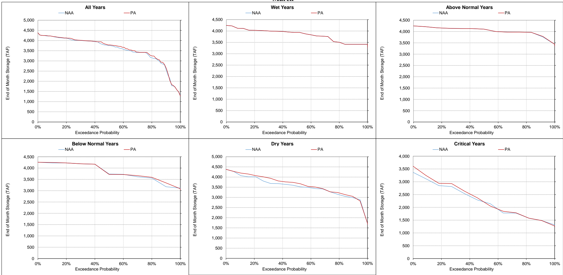
Figure 5.A.6-3-13. Shasta Lake, End of Month Storage March
