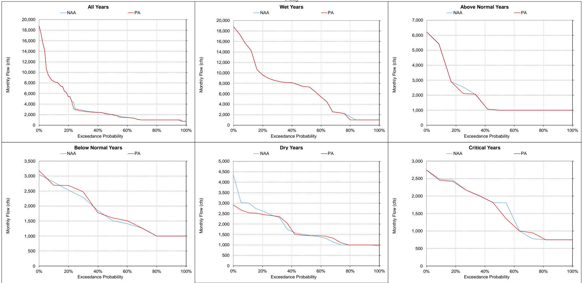
Figure 5.A.6-12-15. Feather River below Thermalito Diversion Dam, Monthly Flow May
