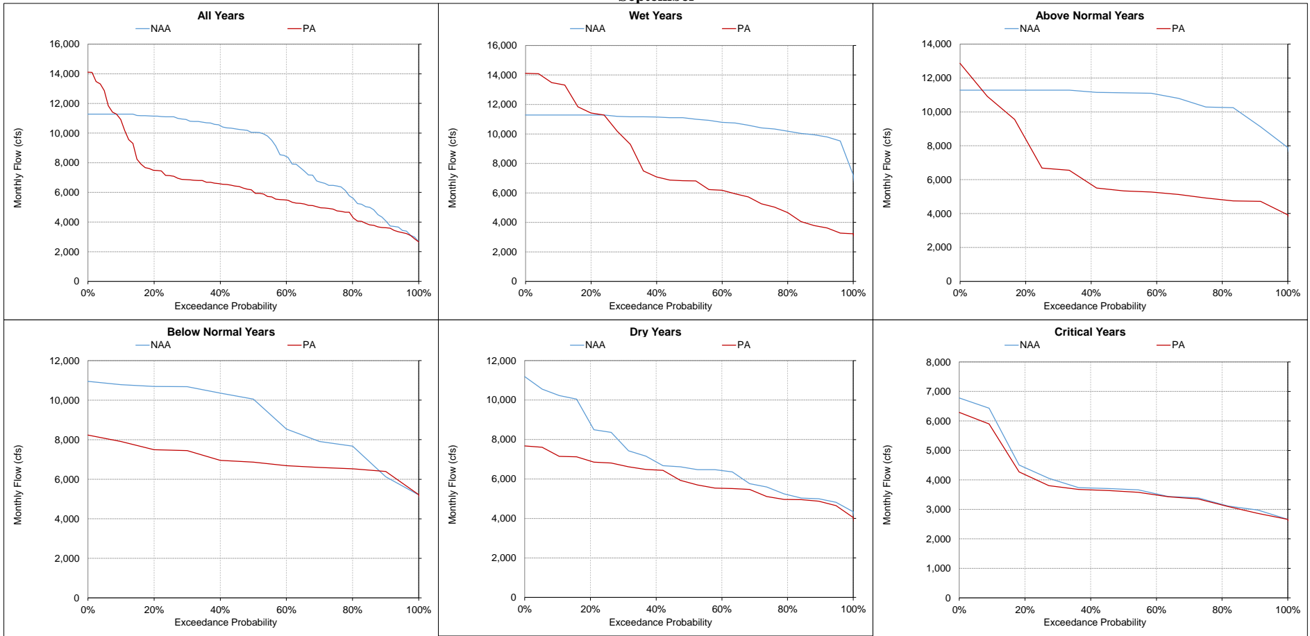
Figure 5.A.6-28-19. Total Delta Exports, Monthly Flow September
