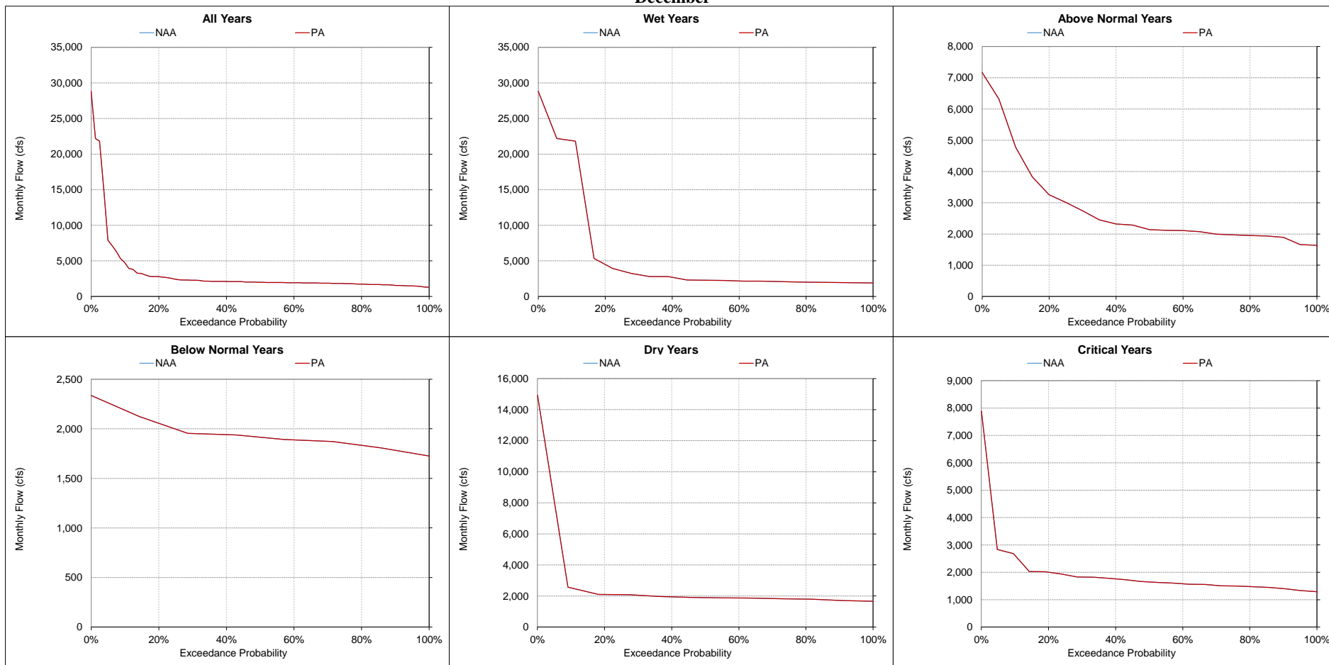
Figure 5.A.6-23-10. San Joaquin River at Vernalis, Monthly Flow December
