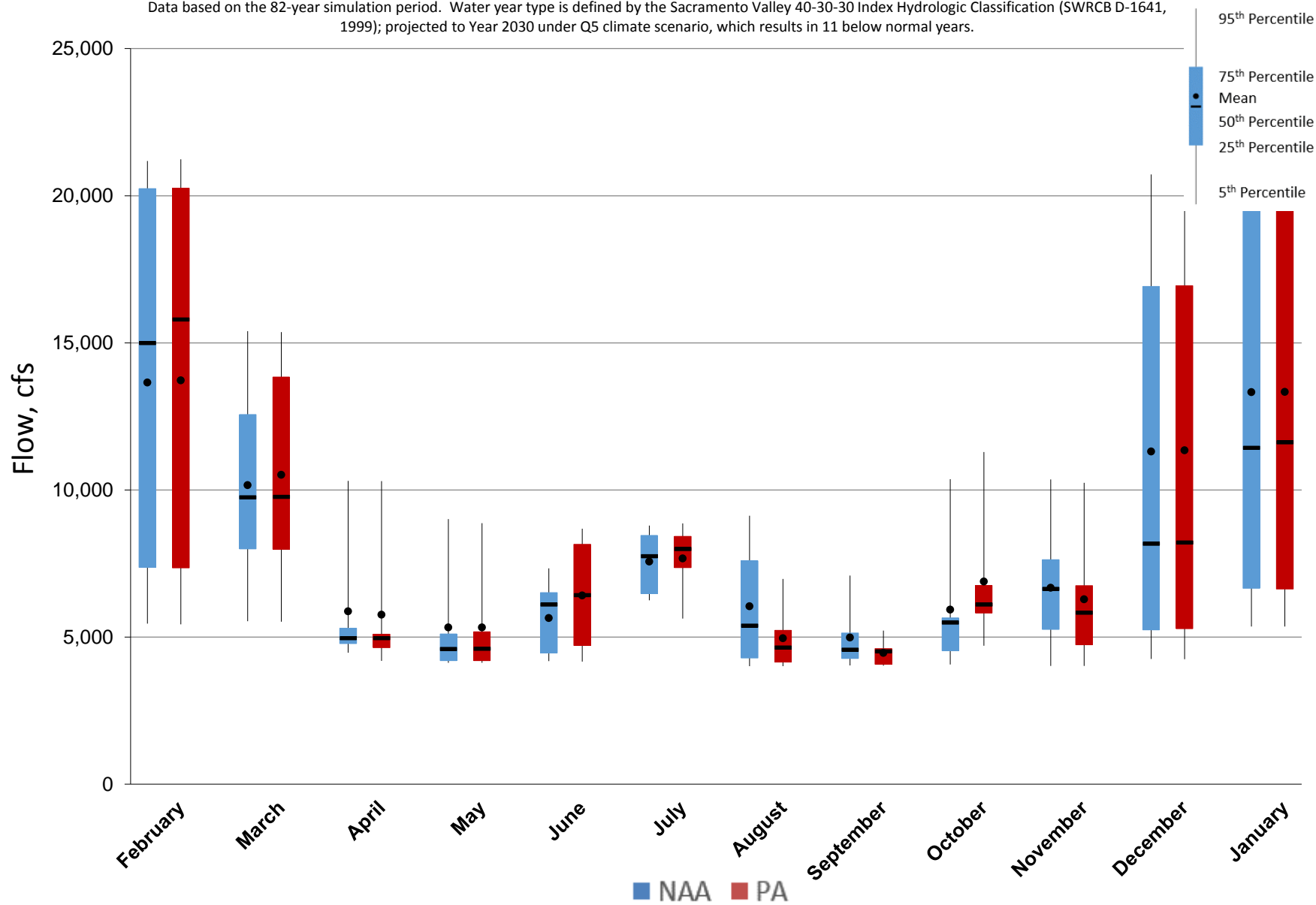
Figure 5.A.6-11-4. Monthly Flow Ranges For Sacramento River at Bend Bridge, Below Normal Years
