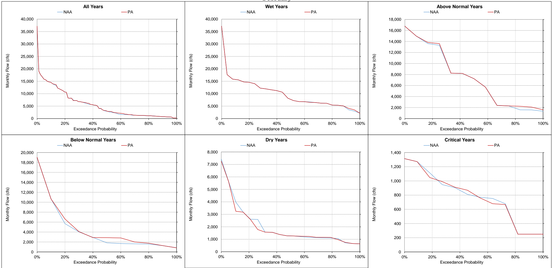
Figure 5.A.6-17-12. American River at Sacramento River Confluence, Monthly Flow February
