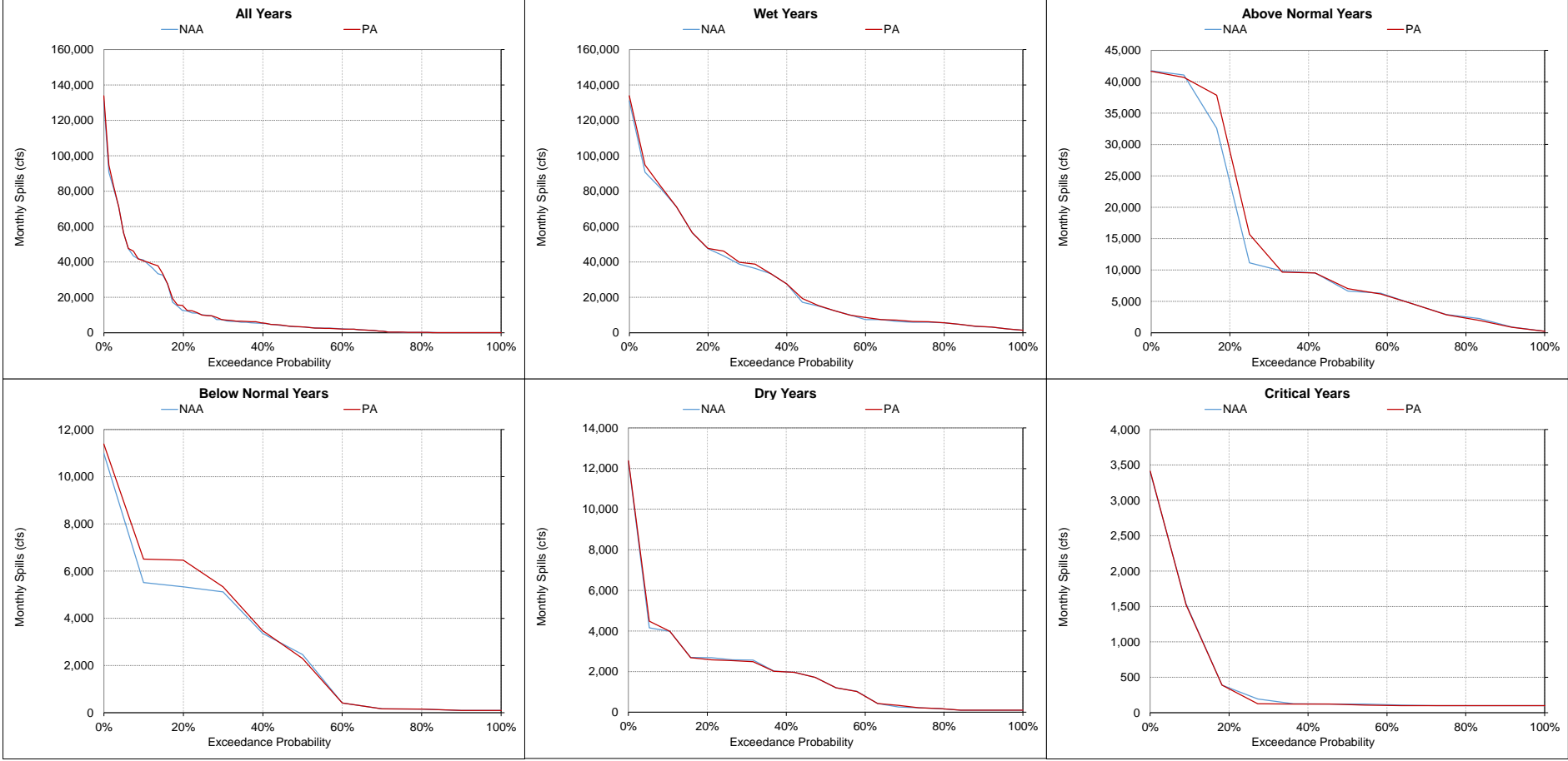
Figure 5.A.6-15-12. Fremont Weir, Monthly Spills February
