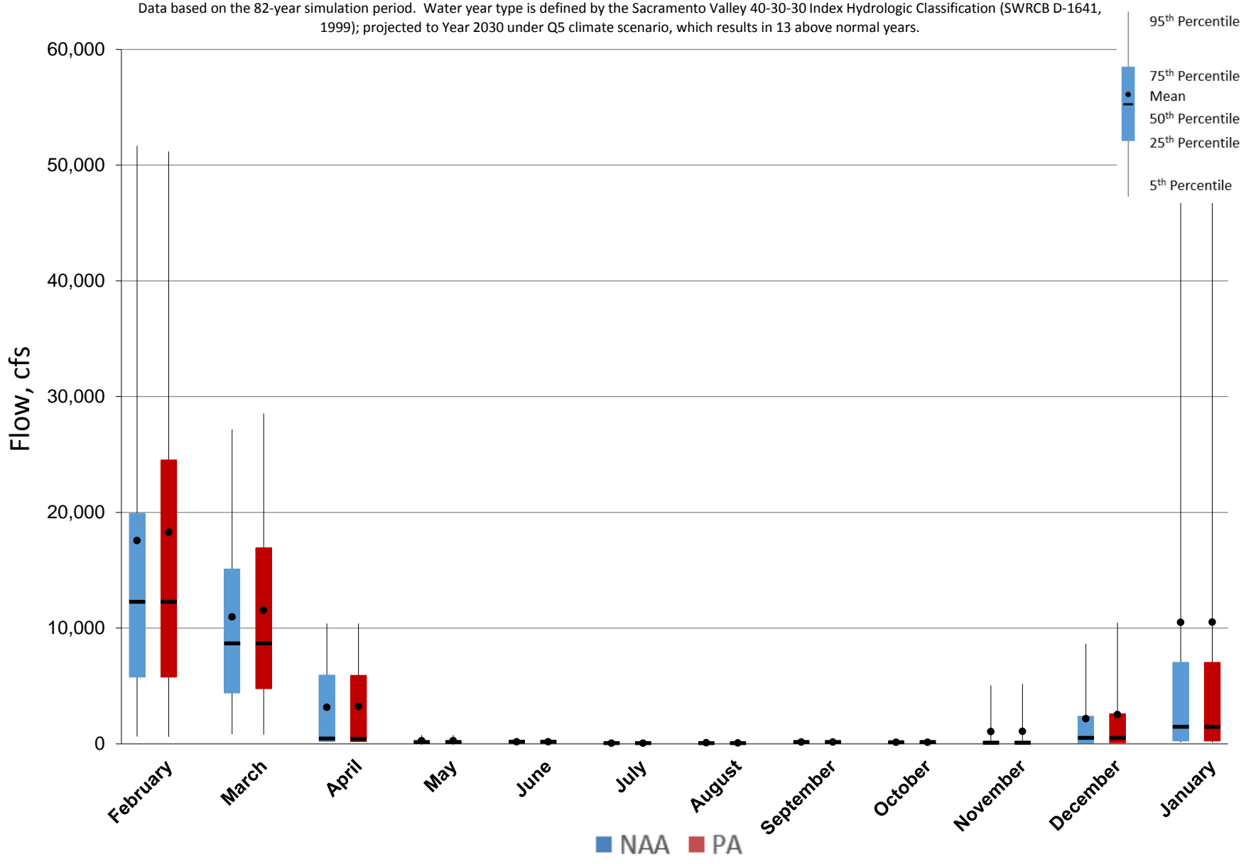
Figure 5.A.6-20-3. Monthly Flow Ranges For Yolo Bypass, Above Normal Years
