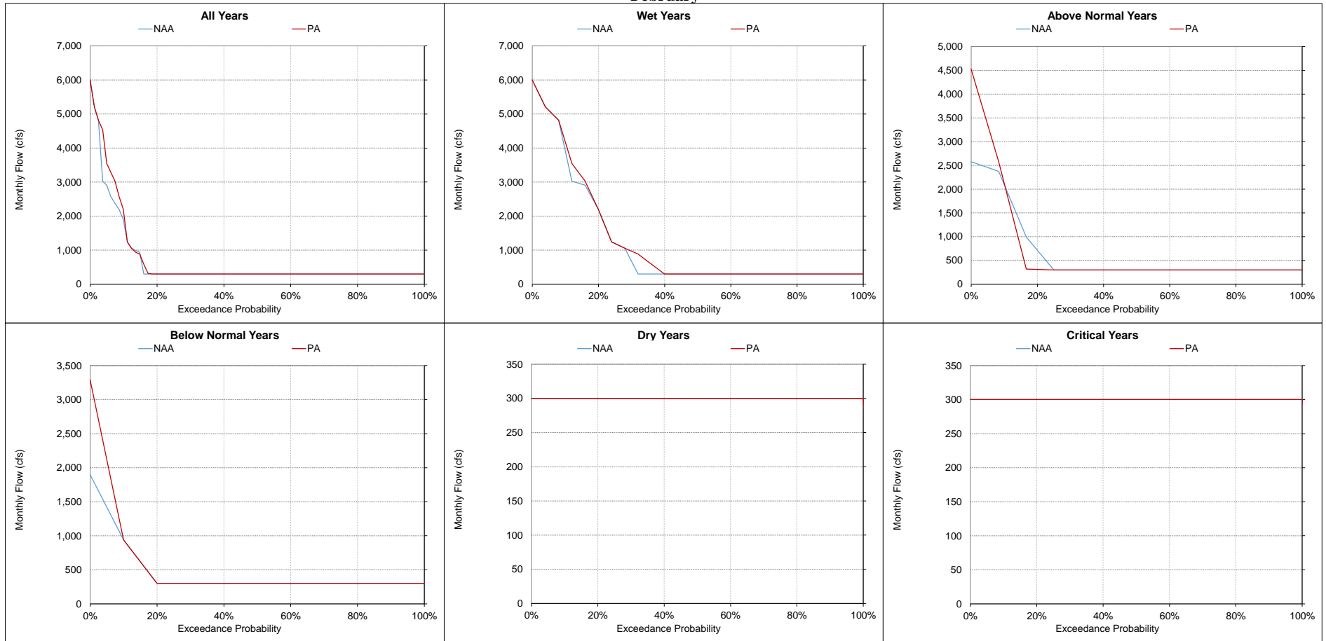
Figure 5.A.6-7-12. Trinity River below Lewiston Dam, Monthly Flow February
