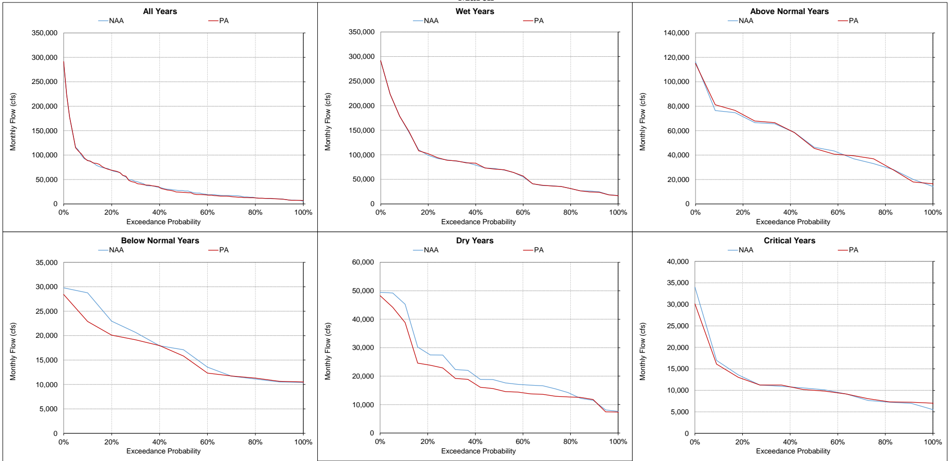
Figure 5.A.6-26-13. Delta Outflow, Monthly Flow March
