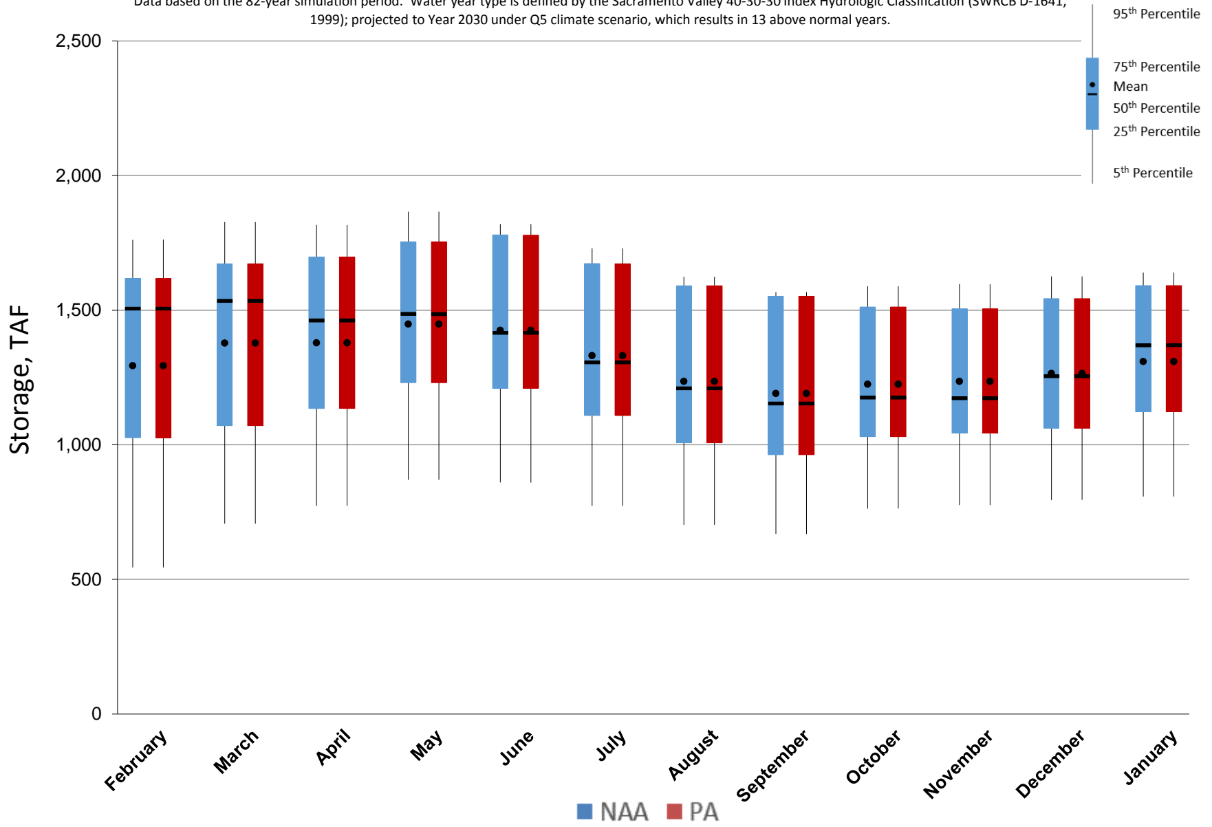
Figure 5.A.6-6-3. End of Month Storage Ranges For New Melones Lake, Above Normal Years
