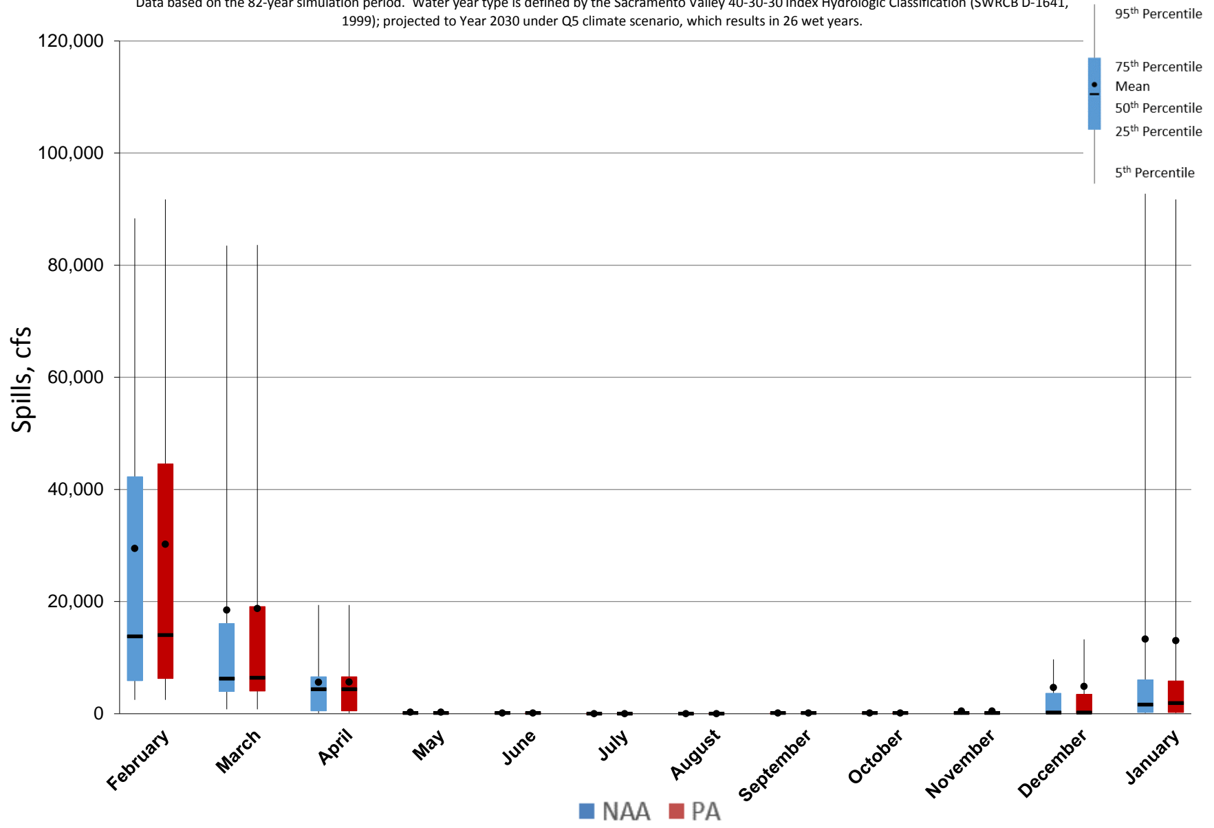
Figure 5.A.6-15-2. Monthly Spills Ranges For Fremont Weir, Wet Years
