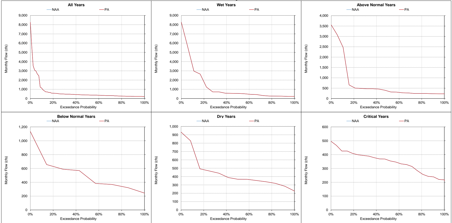
Figure 5.A.6-22-12. Stanislaus River at Mouth, Monthly Flow February
