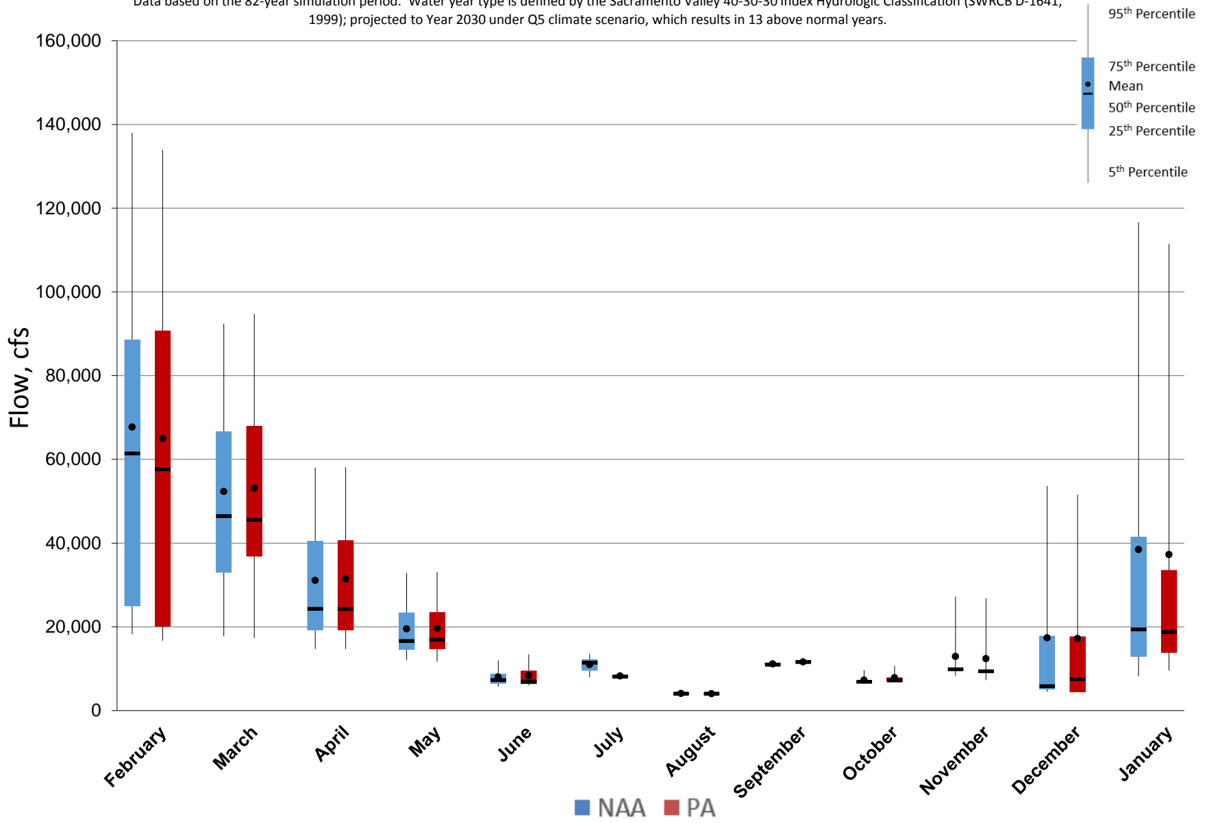
Figure 5.A.6-26-3. Monthly Flow Ranges For Delta Outflow, Above Normal Years
