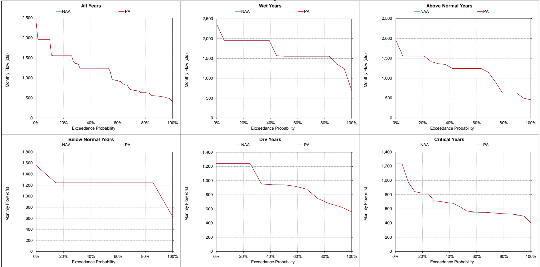
Figure 5.A.6-21-15. Stanislaus River at Ripon, Monthly Flow May
