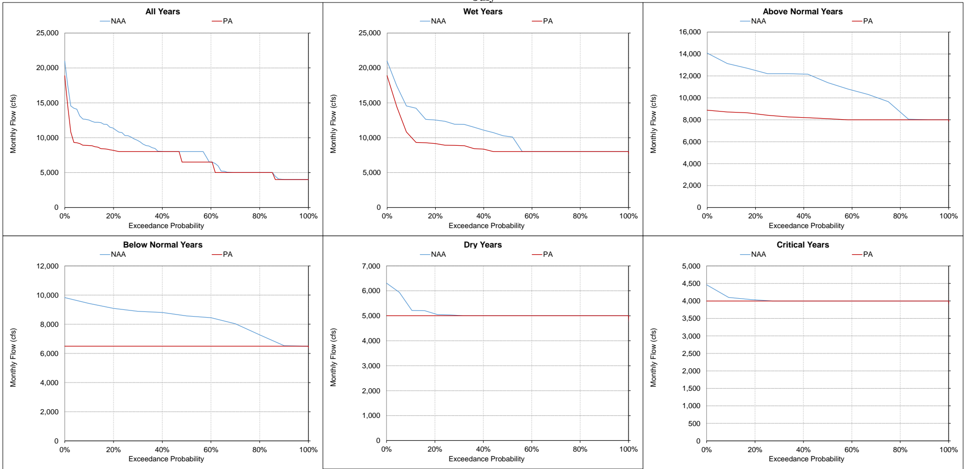
Figure 5.A.6-26-17. Delta Outflow, Monthly Flow July
