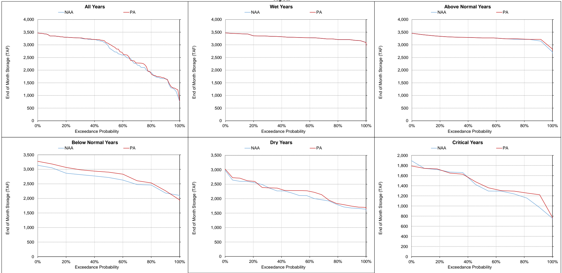
Figure 5.A.6-4-14. Lake Oroville, End of Month Storage April
