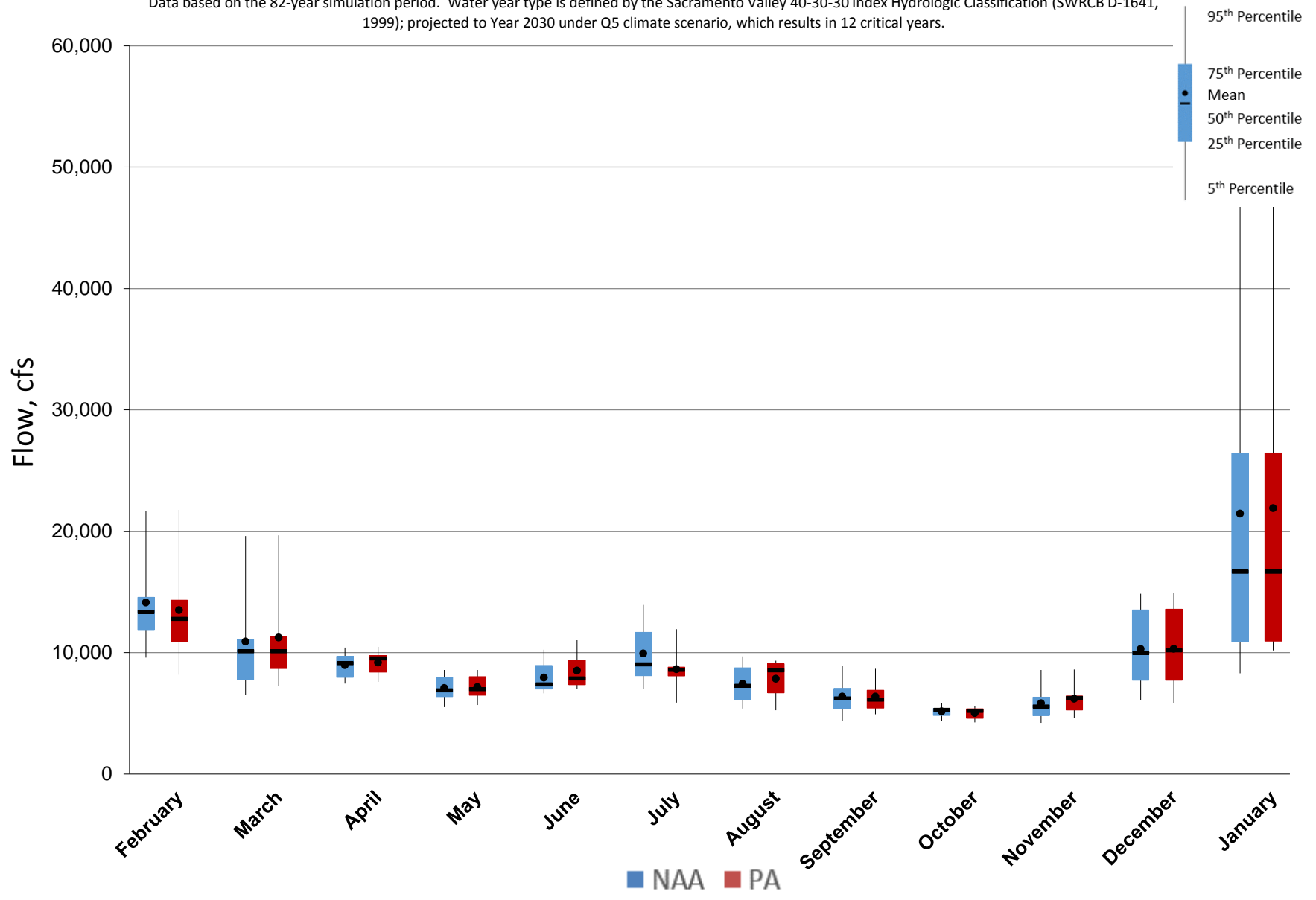
Figure 5.A.6-14-6. Monthly Flow Ranges For Sacramento River at Verona, Critical Years
