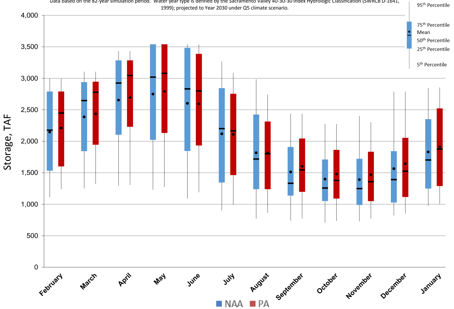
Figure 5.A.6-4-1. End of Month Storage Ranges For Lake Oroville, All Years
