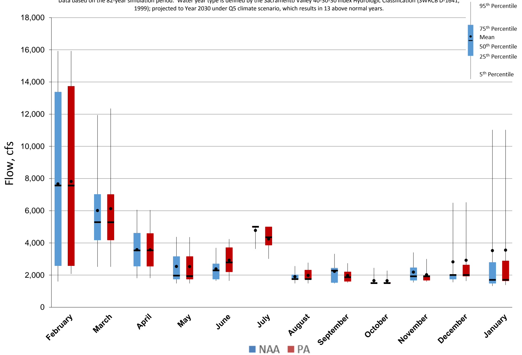
Figure 5.A.6-16-3. Monthly Flow Ranges For American River below Nimbus Dam, Above Normal Years
