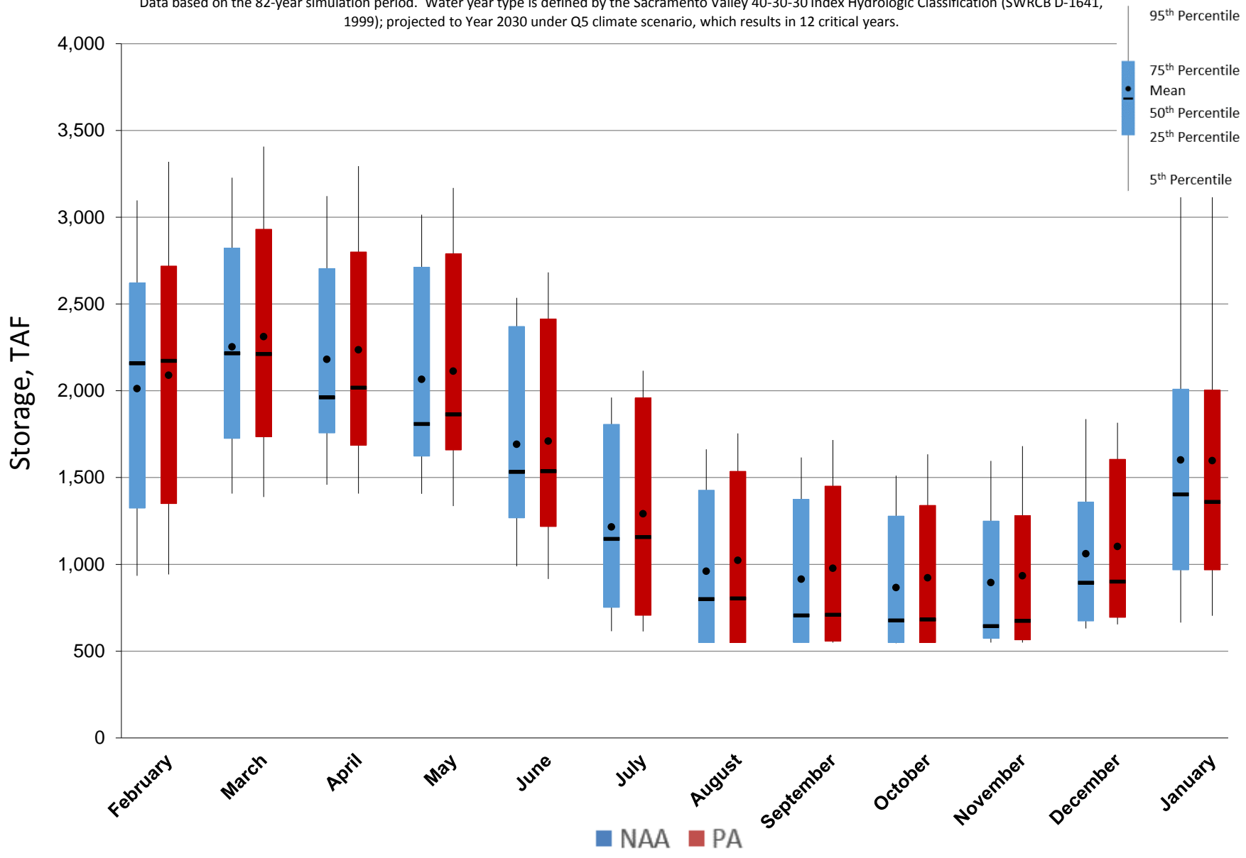
Figure 5.A.6-3-6. End of Month Storage Ranges For Shasta Lake, Critical Years
