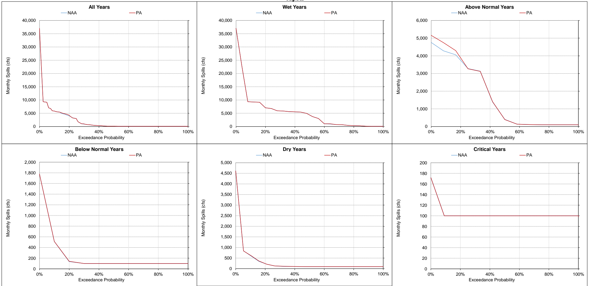
Figure 5.A.6-15-14. Fremont Weir, Monthly Spills April
