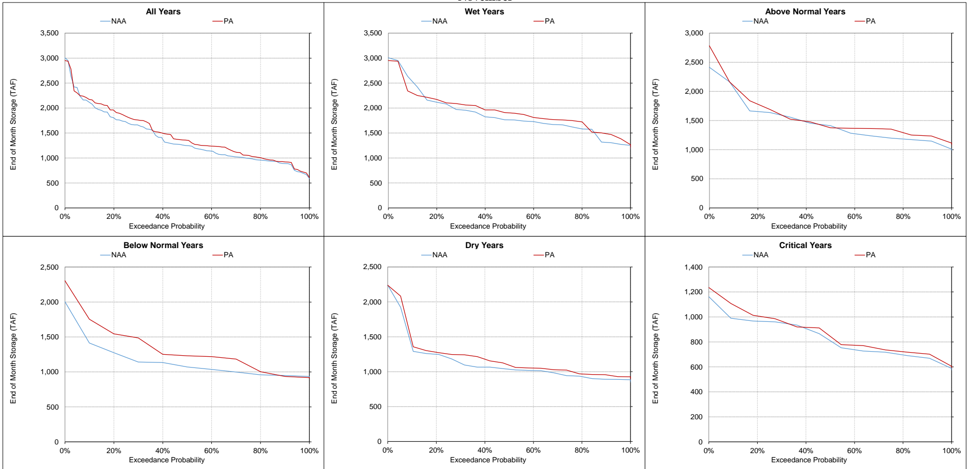
Figure 5.A.6-4-9. Lake Oroville, End of Month Storage November
