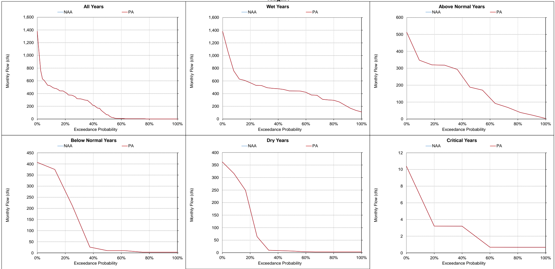
Figure 5.A.6-24-18. Mokelumne and Cosumnes River, Monthly Flow August
