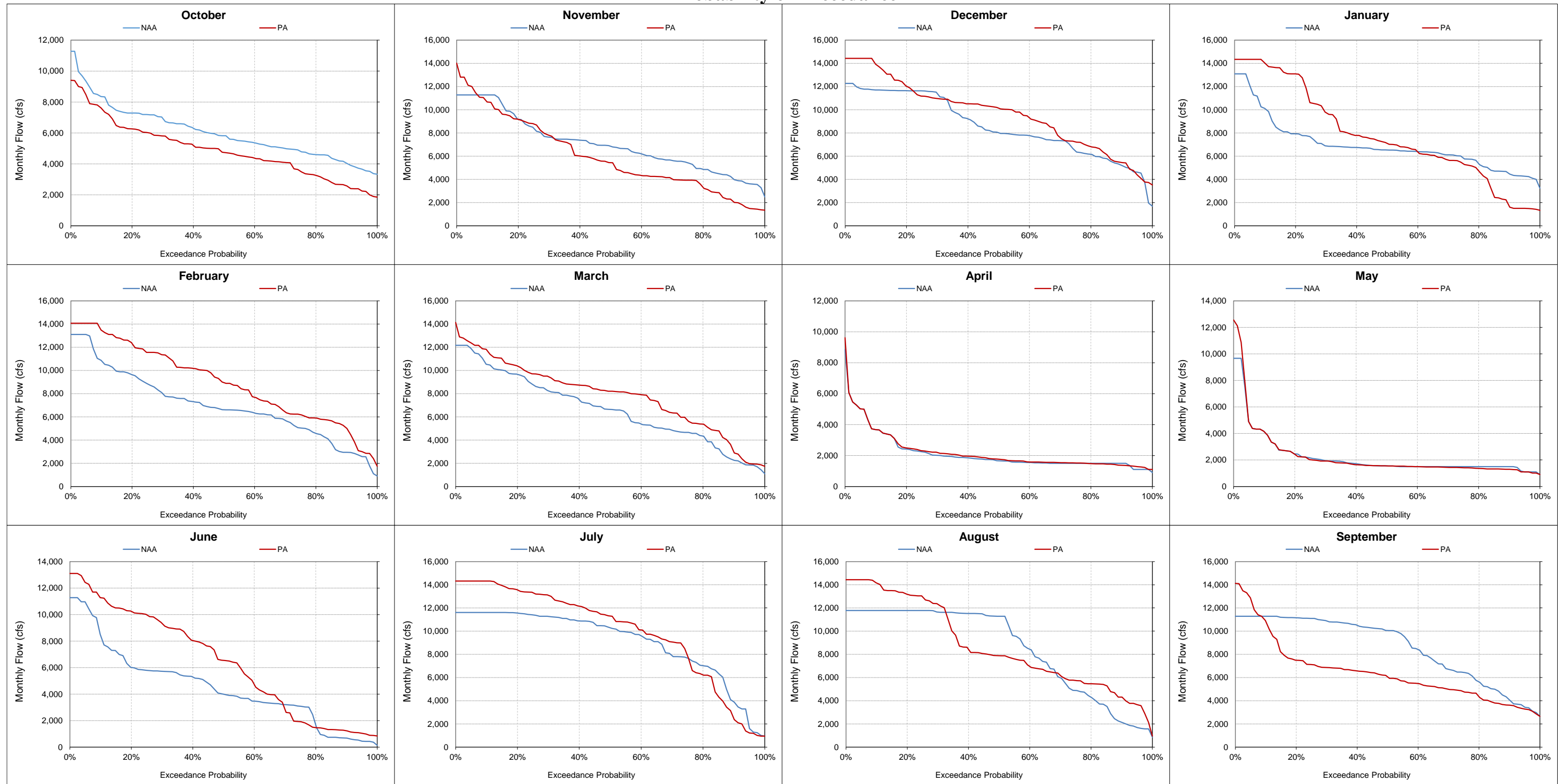
Figure 5.A.6-28-7. Total Delta Exports, Monthly Flow Probability of Exceedance
