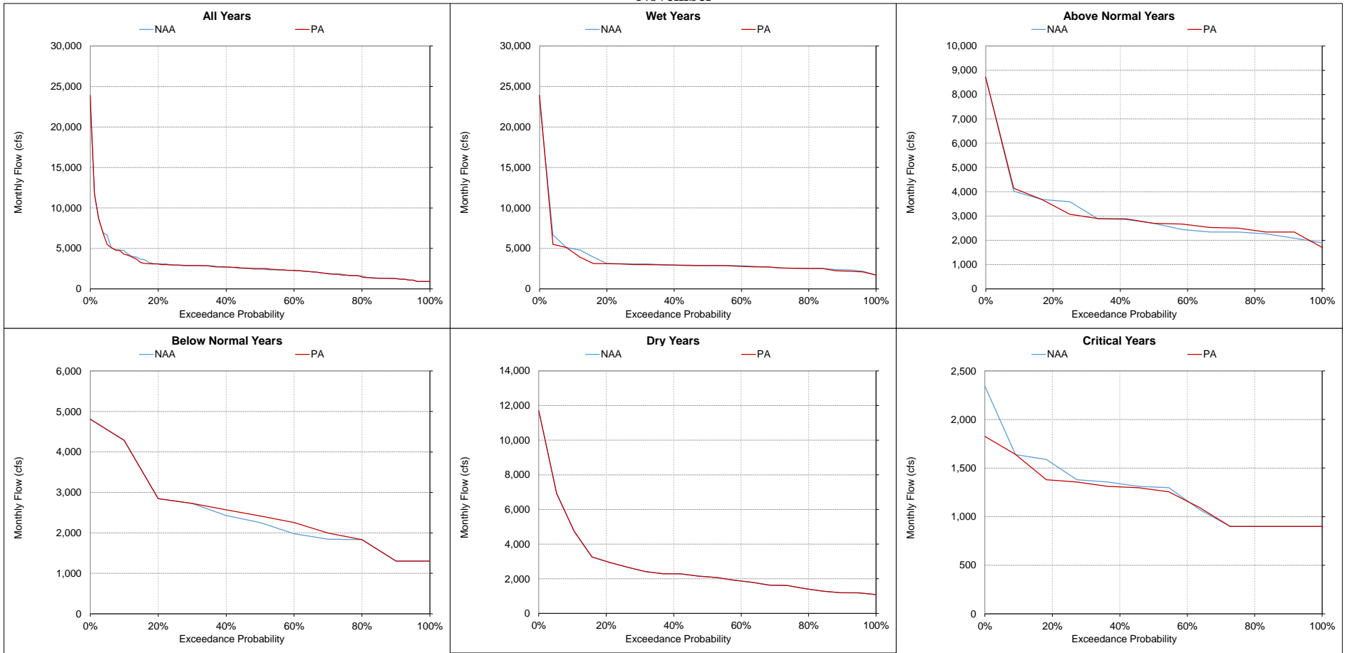
Figure 5.A.6-13-9. Feather River at Sacramento River Confluence, Monthly Flow November
