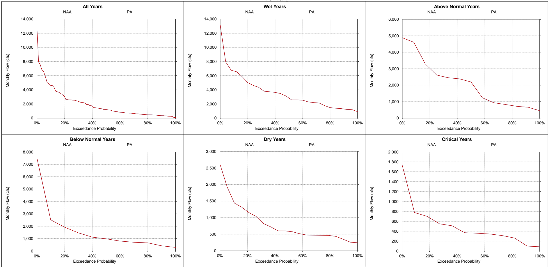
Figure 5.A.6-24-12. Mokelumne and Cosumnes River, Monthly Flow February
