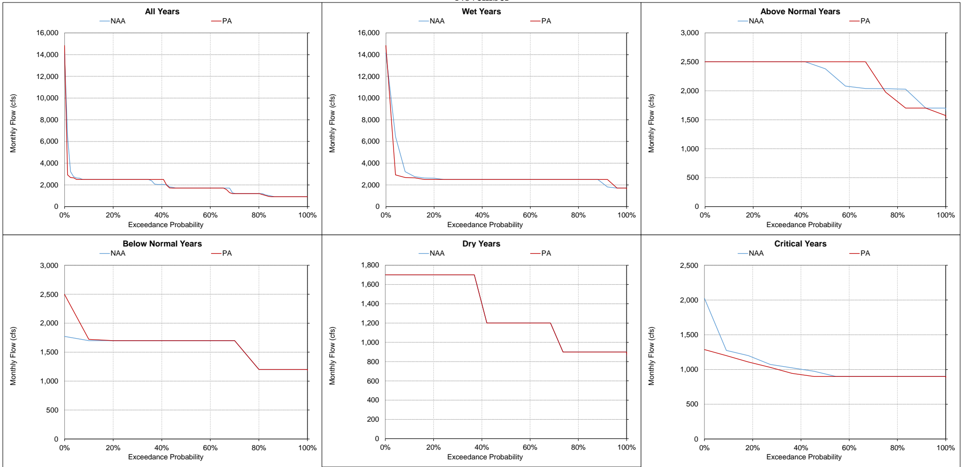
Figure 5.A.6-12-9. Feather River below Thermalito Diversion Dam, Monthly Flow November
