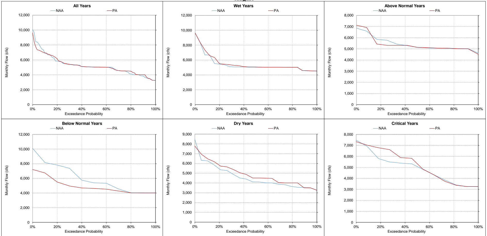
Figure 5.A.6-11-18. Sacramento River at Bend Bridge, Monthly Flow August
