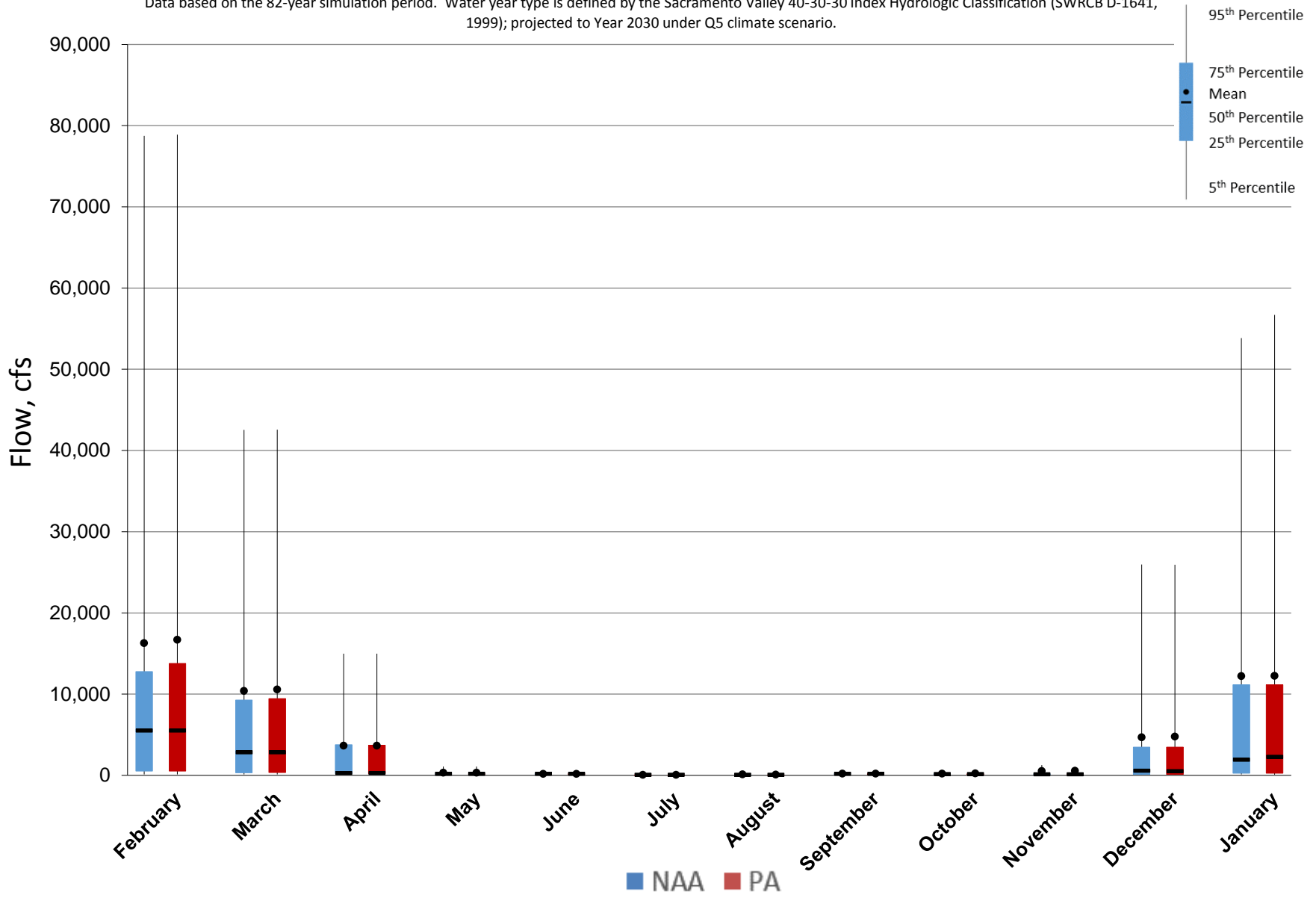
Figure 5.A.6-20-1. Monthly Flow Ranges For Yolo Bypass, All Years
