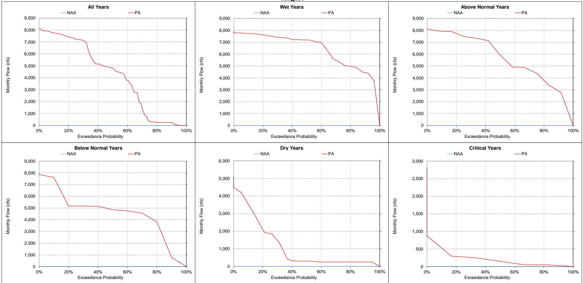
Figure 5.A.6-19-18. North Delta Diversions near Hood, Monthly Flow August
