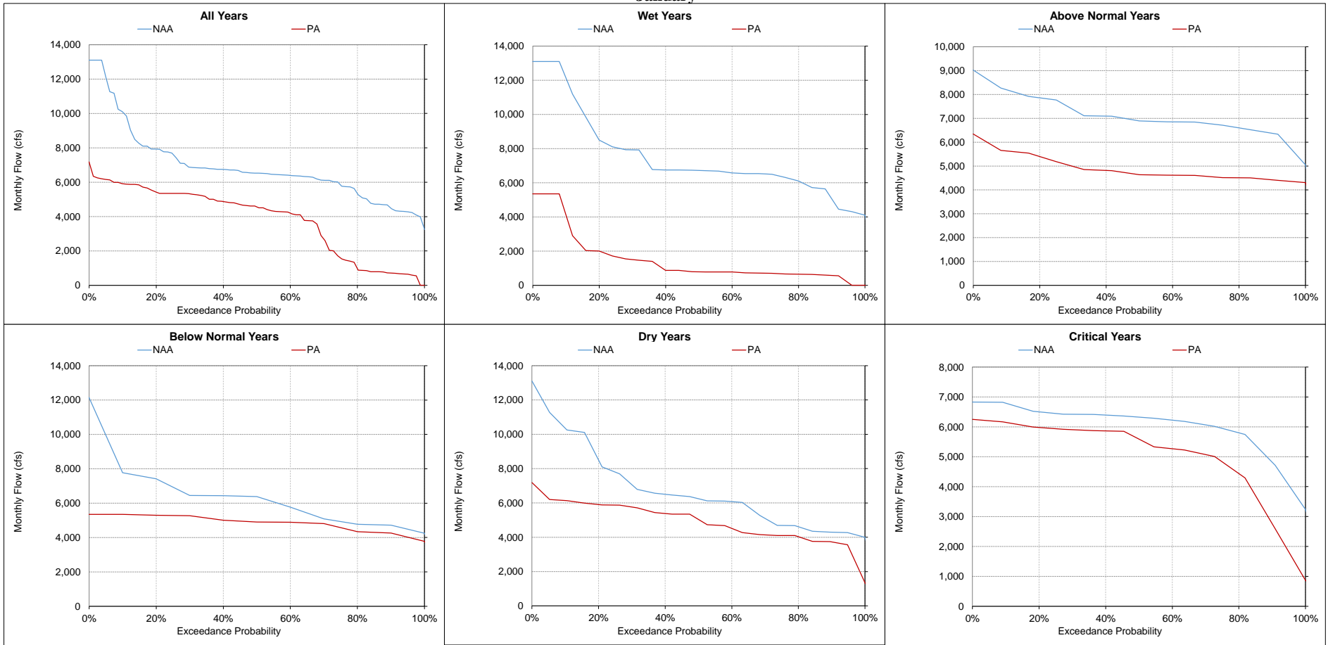
Figure 5.A.6-27-11. South Delta Exports, Monthly Flow January
