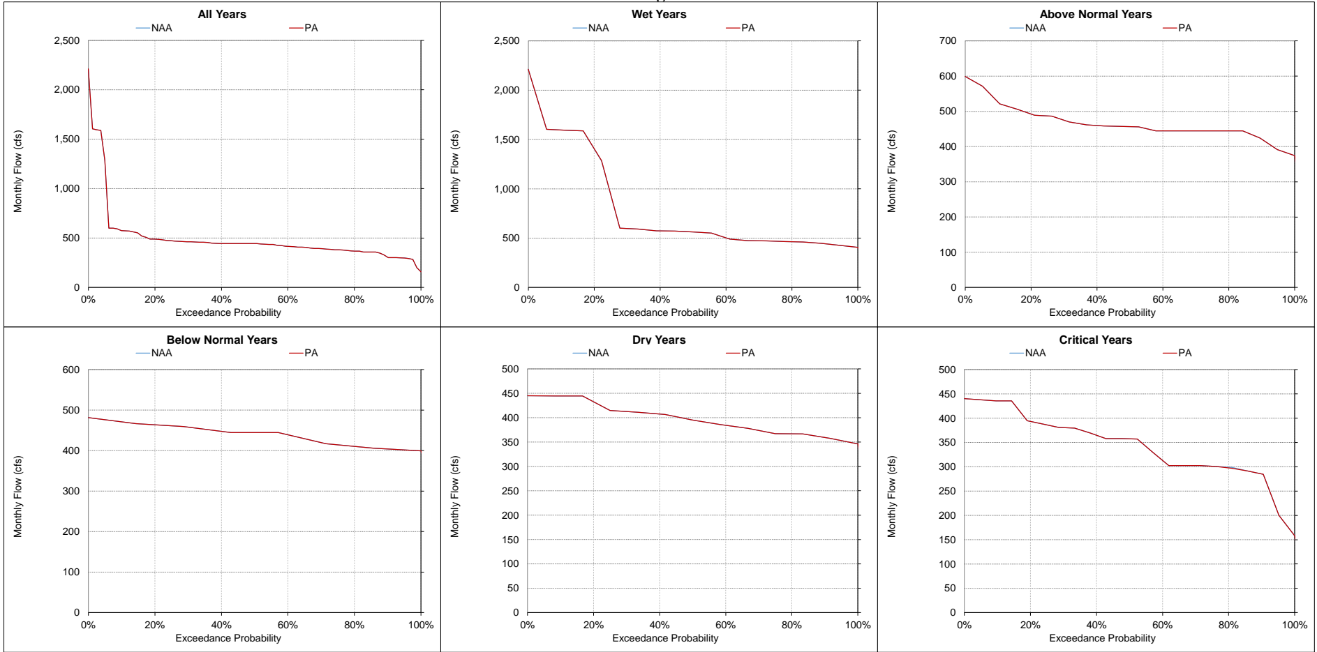
Figure 5.A.6-22-18. Stanislaus River at Mouth, Monthly Flow
