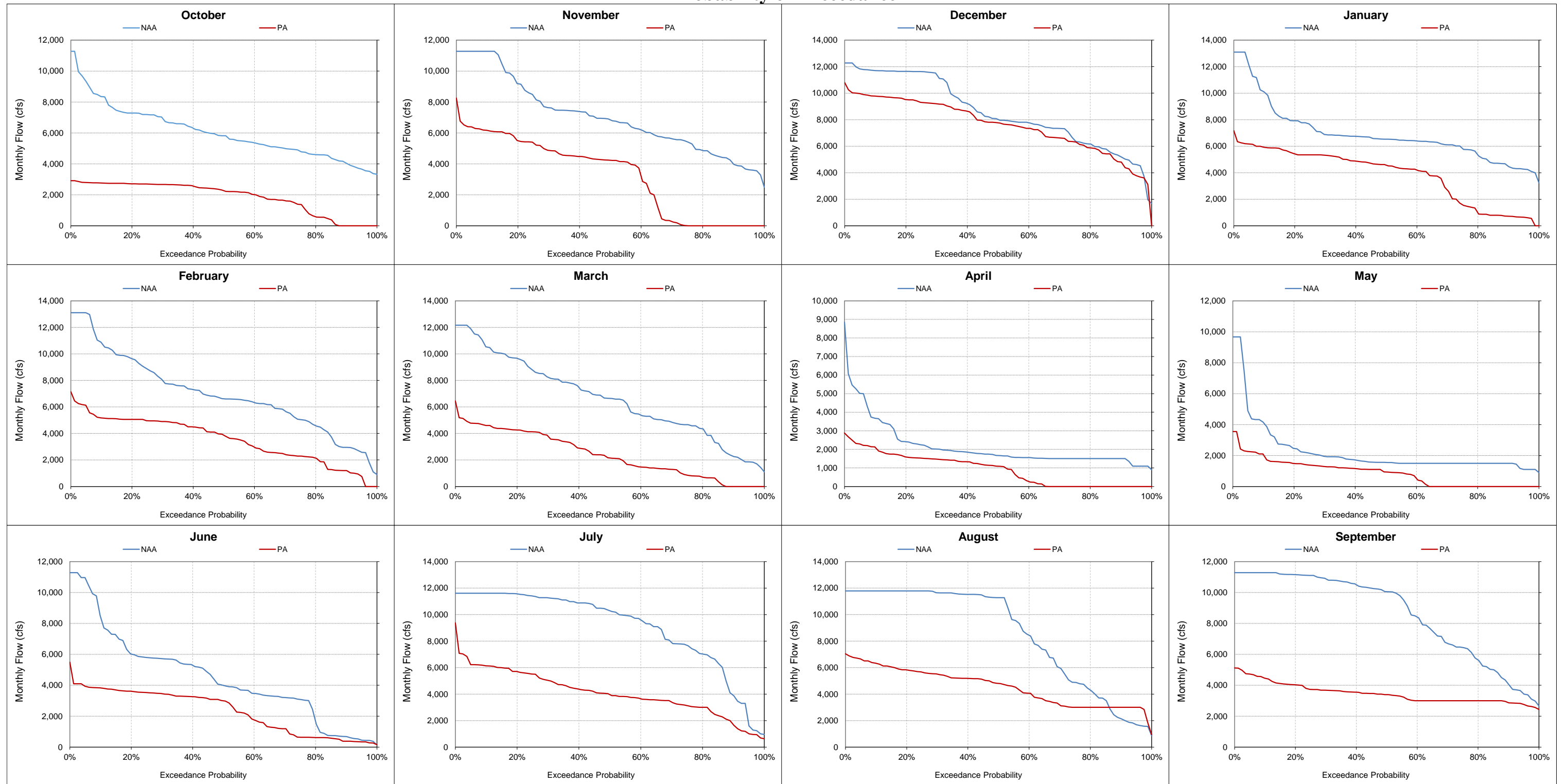
Figure 5.A.6-27-7. South Delta Exports, Monthly Flow Probability of Exceedance
