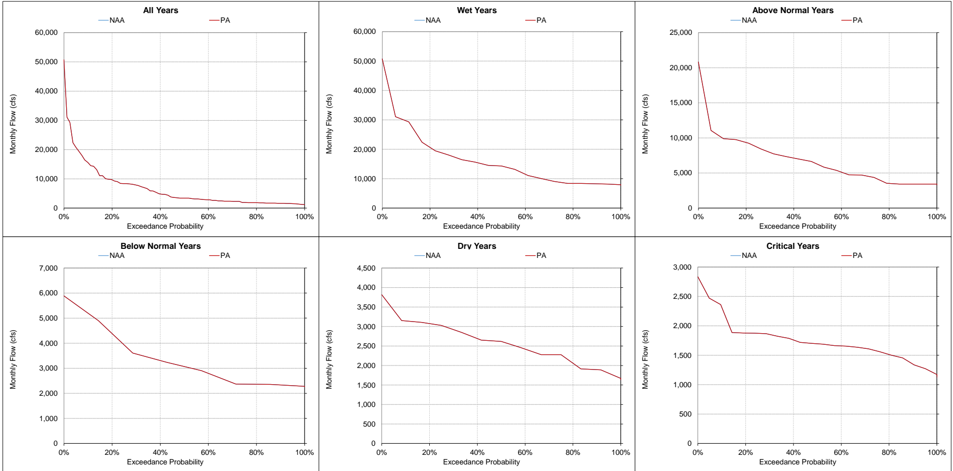
Figure 5.A.6-23-13. San Joaquin River at Vernalis, Monthly Flow March
