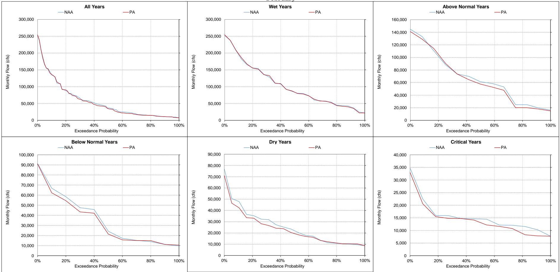
Figure 5.A.6-26-12. Delta Outflow, Monthly Flow February
