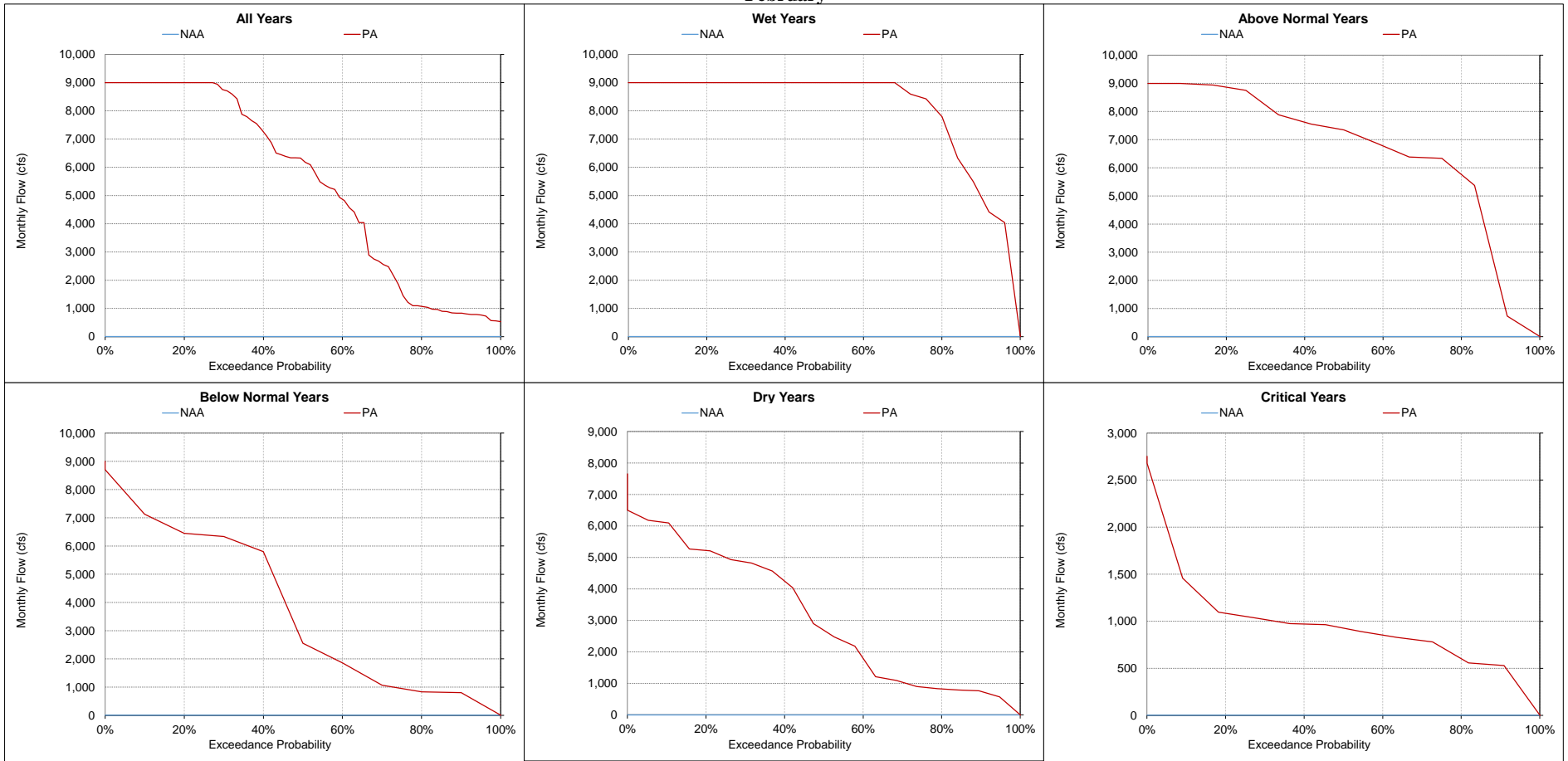
Figure 5.A.6-19-12. North Delta Diversions near Hood, Monthly Flow February
