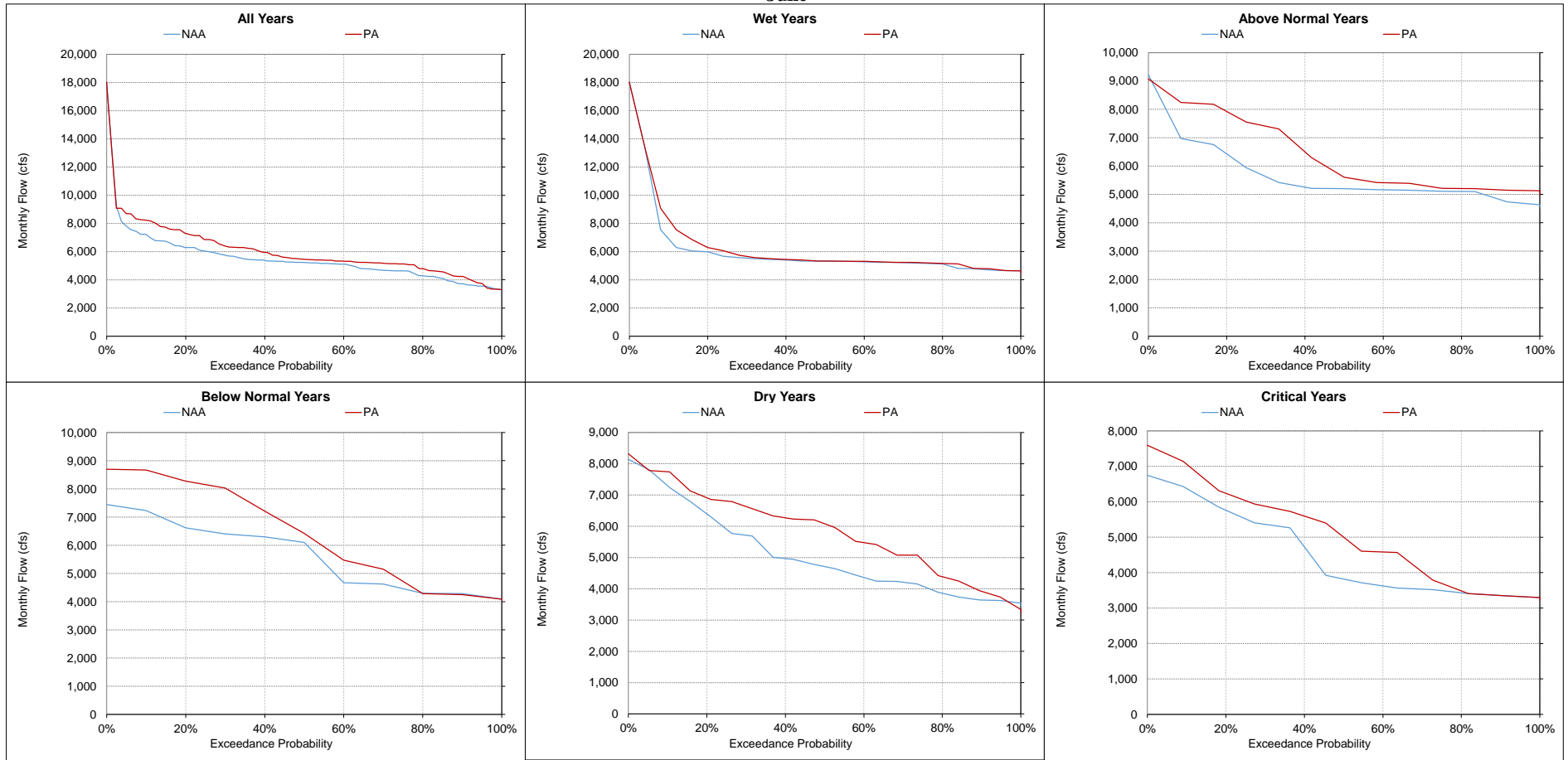
Figure 5.A.6-11-16. Sacramento River at Bend Bridge, Monthly Flow June
