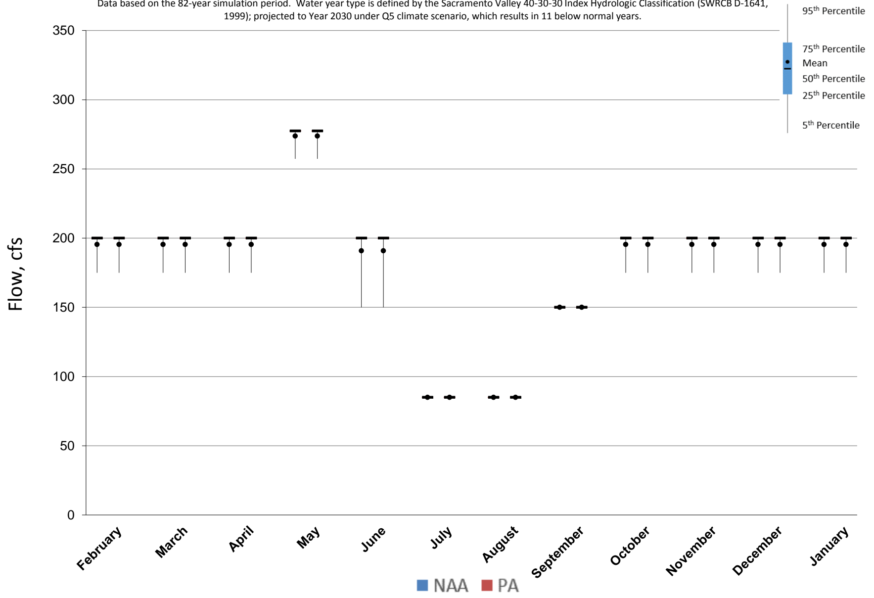
Figure 5.A.6-9-4. Monthly Flow Ranges For Clear Creek below Whiskeytown Dam, Below Normal Years
