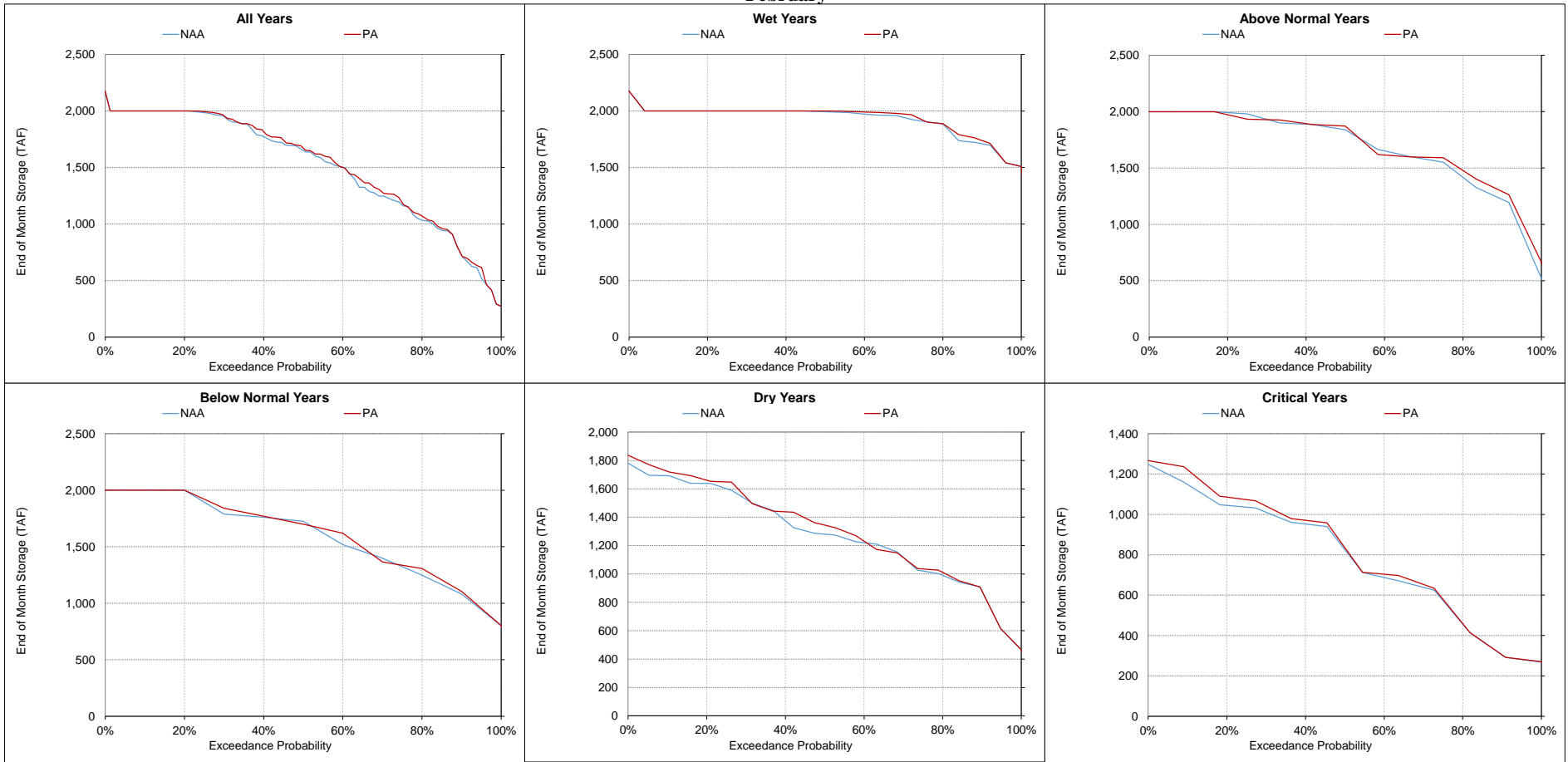
Figure 5.A.6-1-12. Trinity Lake, End of Month Storage February
