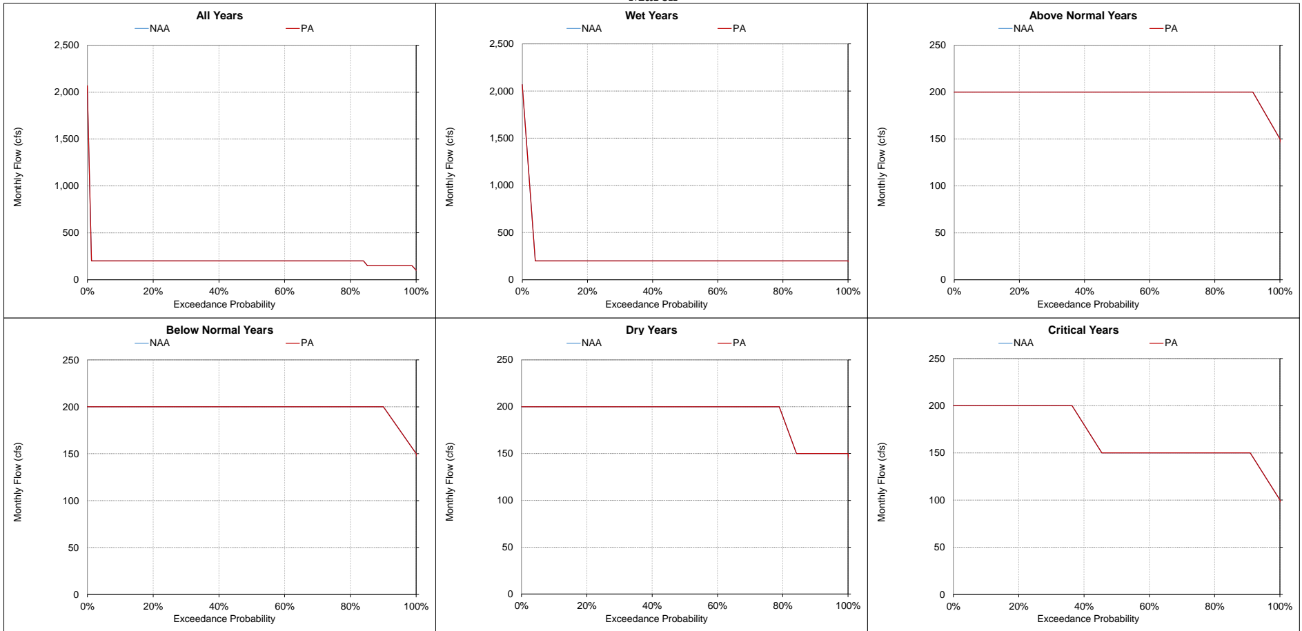
Figure 5.A.6-9-13. Clear Creek below Whiskeytown Dam, Monthly Flow March
