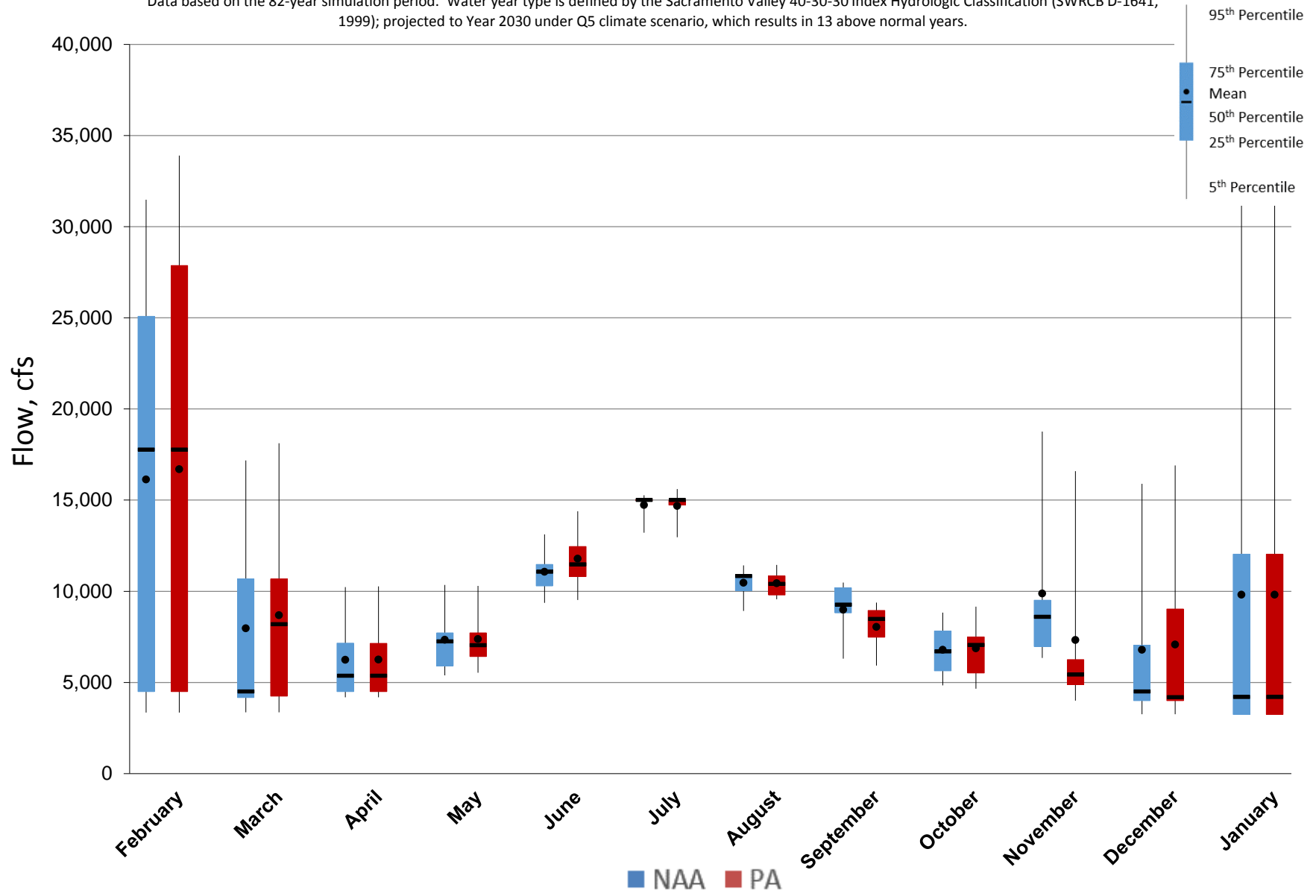
Figure 5.A.6-10-3. Monthly Flow Ranges For Sacramento River below Keswick Dam, Above Normal Years
