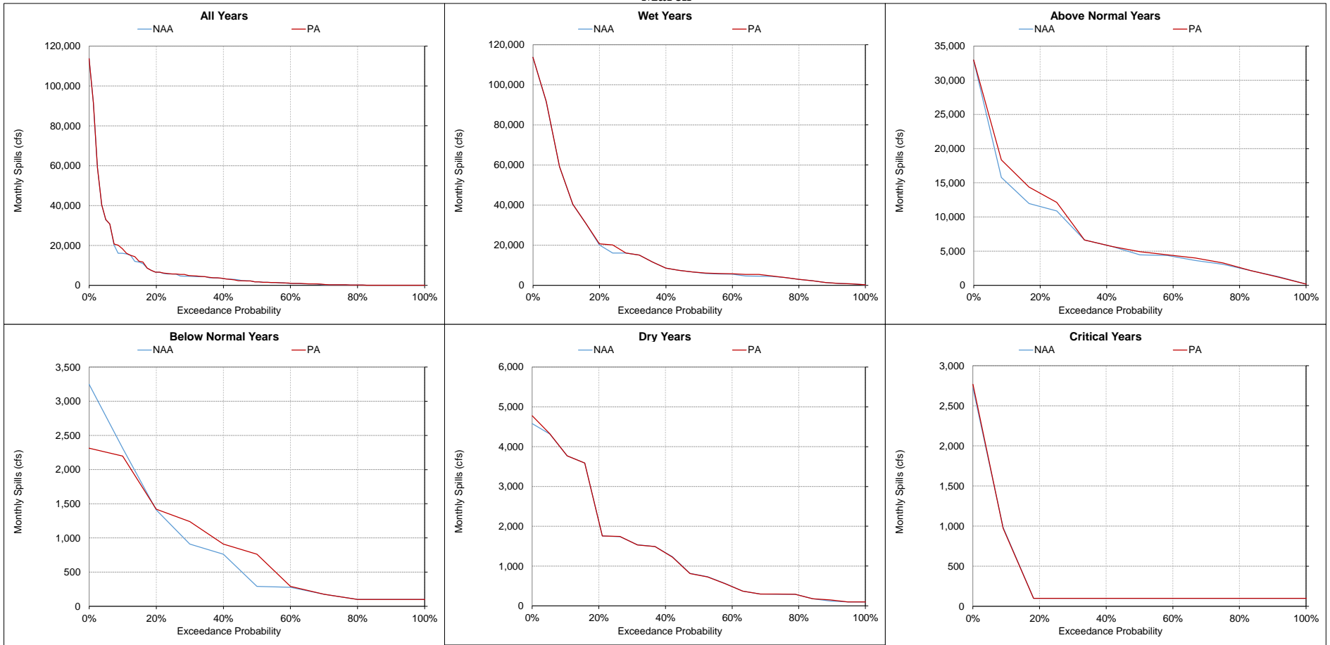
Figure 5.A.6-15-13. Fremont Weir, Monthly Spills March
