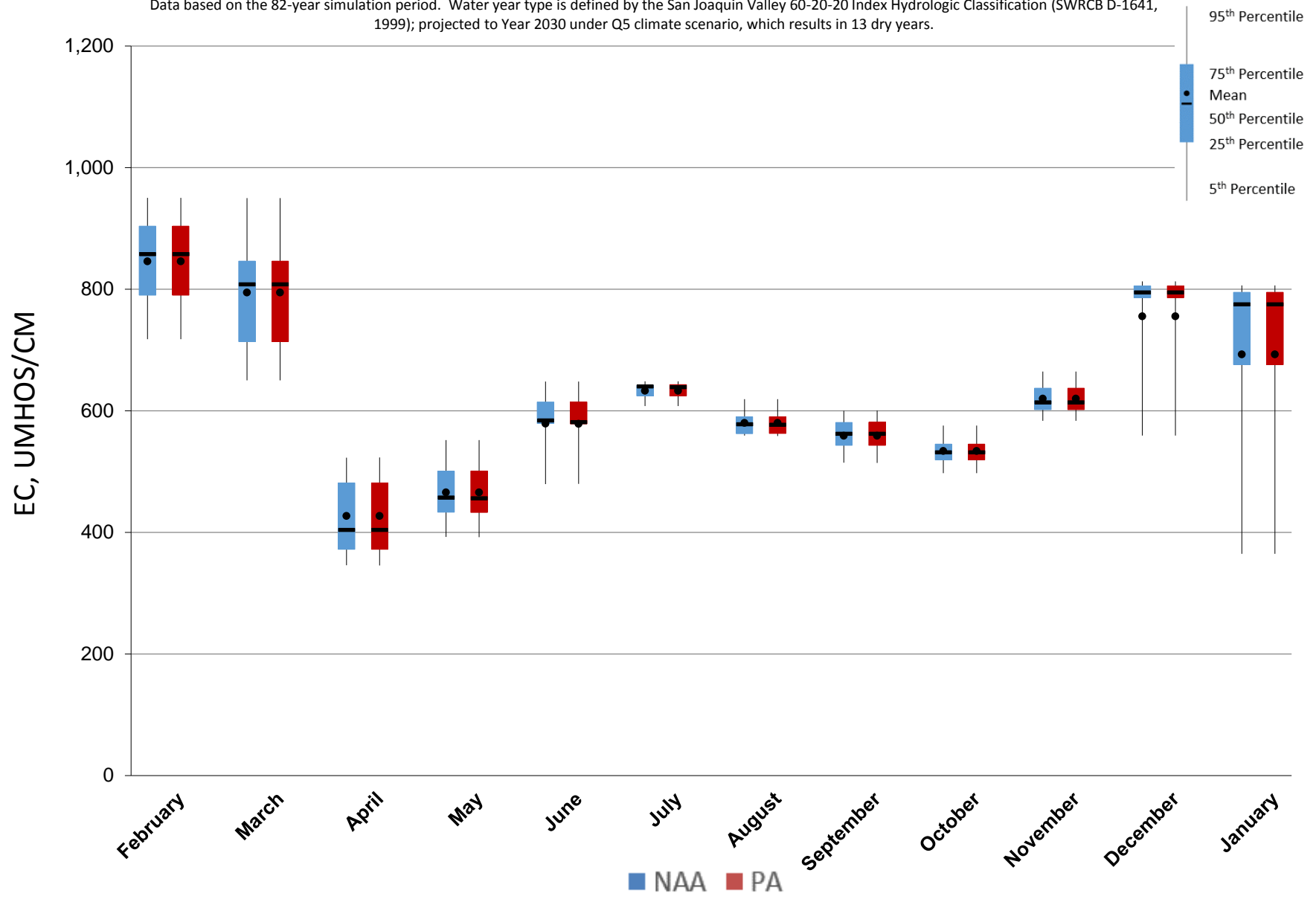
Figure 5.A.6-30-5. Monthly EC Ranges for San Joaquin River at Vernalis, Dry Years
