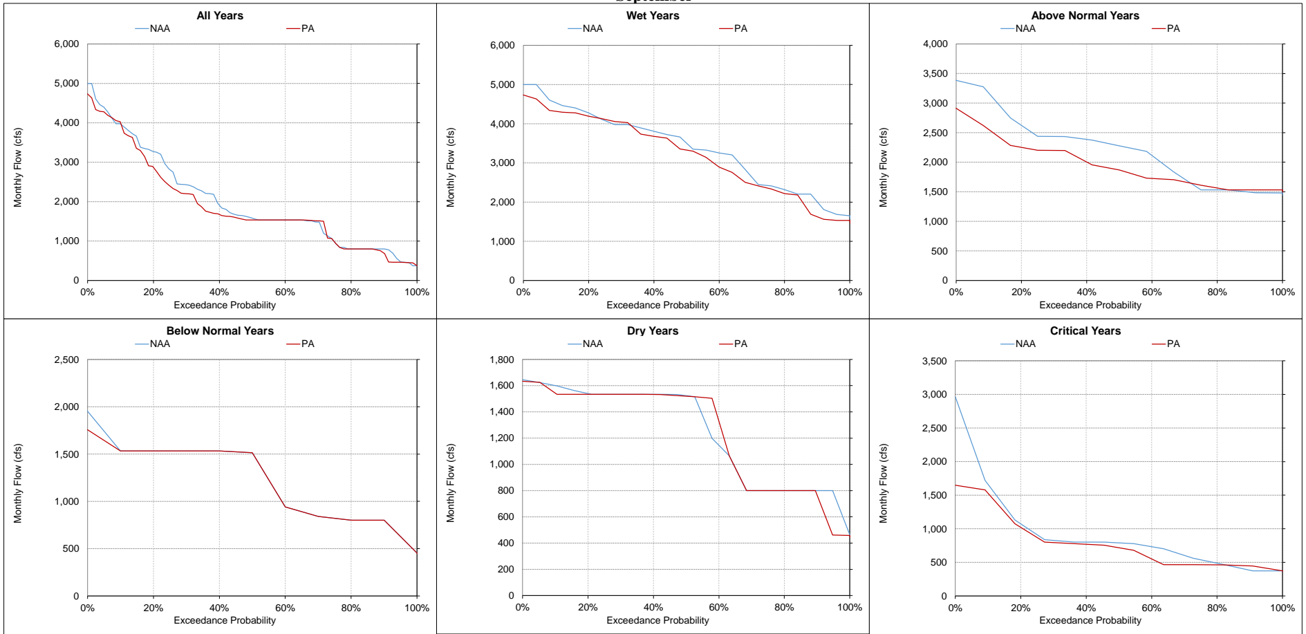
Figure 5.A.6-16-19. American River below Nimbus Dam, Monthly Flow September
