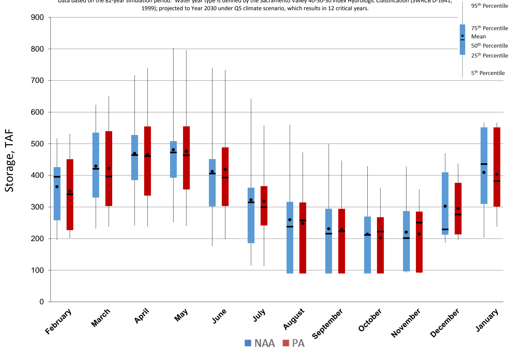
Figure 5.A.6-5-6. End of Month Storage Ranges For Folsom Lake, Critical Years
