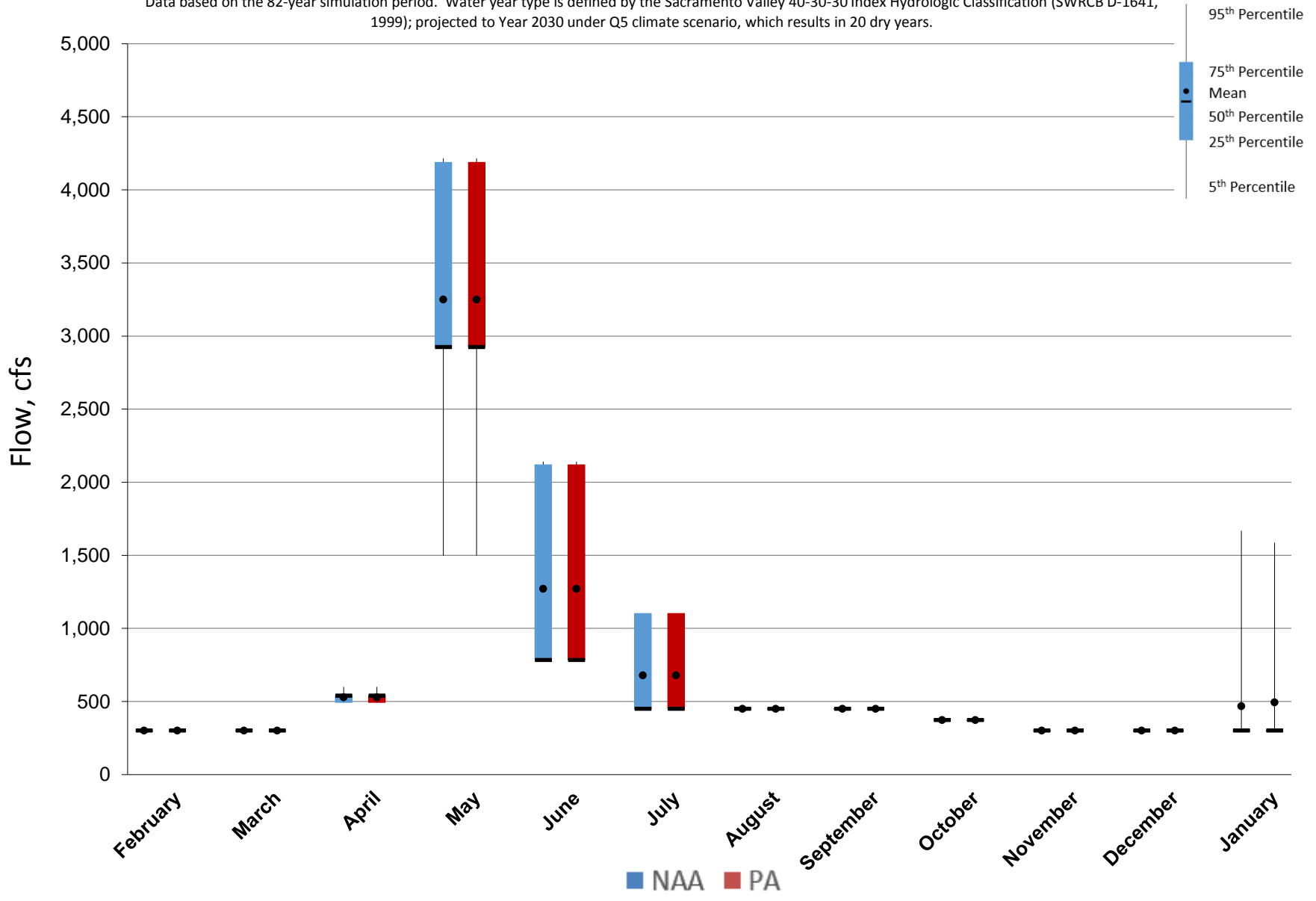
Figure 5.A.6-7-5. Monthly Flow Ranges For Trinity River below Lewiston Dam, Dry Years
