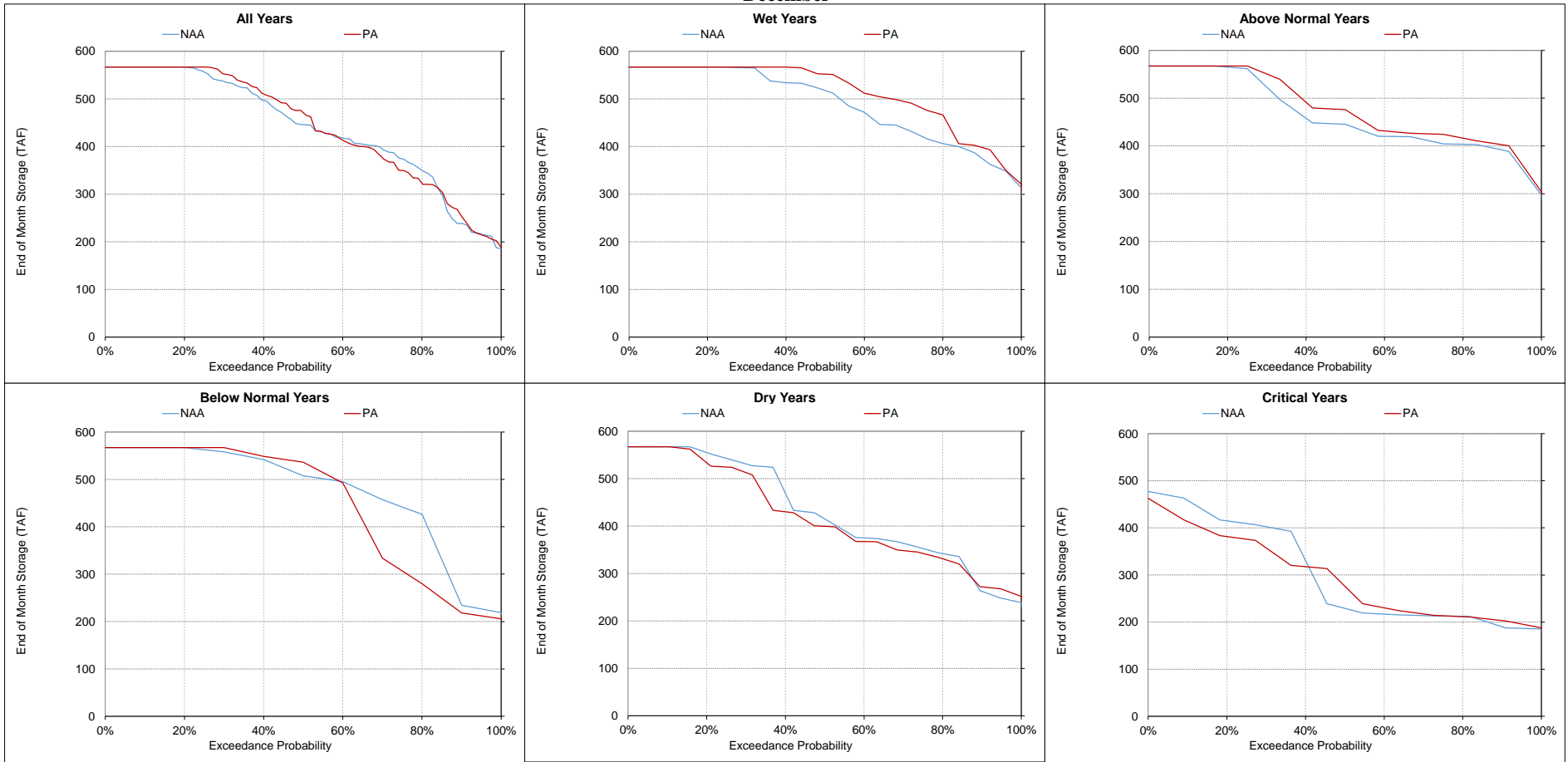
Figure 5.A.6-5-10. Folsom Lake, End of Month Storage December
