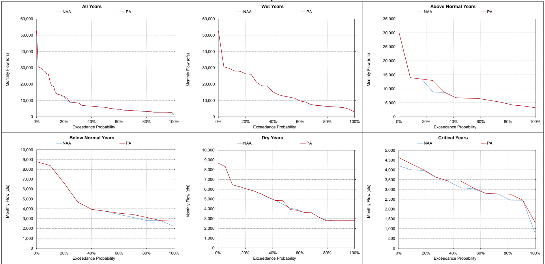
Figure 5.A.6-13-14. Feather River at Sacramento River Confluence, Monthly Flow April
