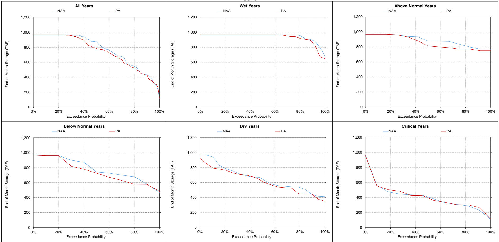
Figure 5.A.6-5-16. Folsom Lake, End of Month Storage June
