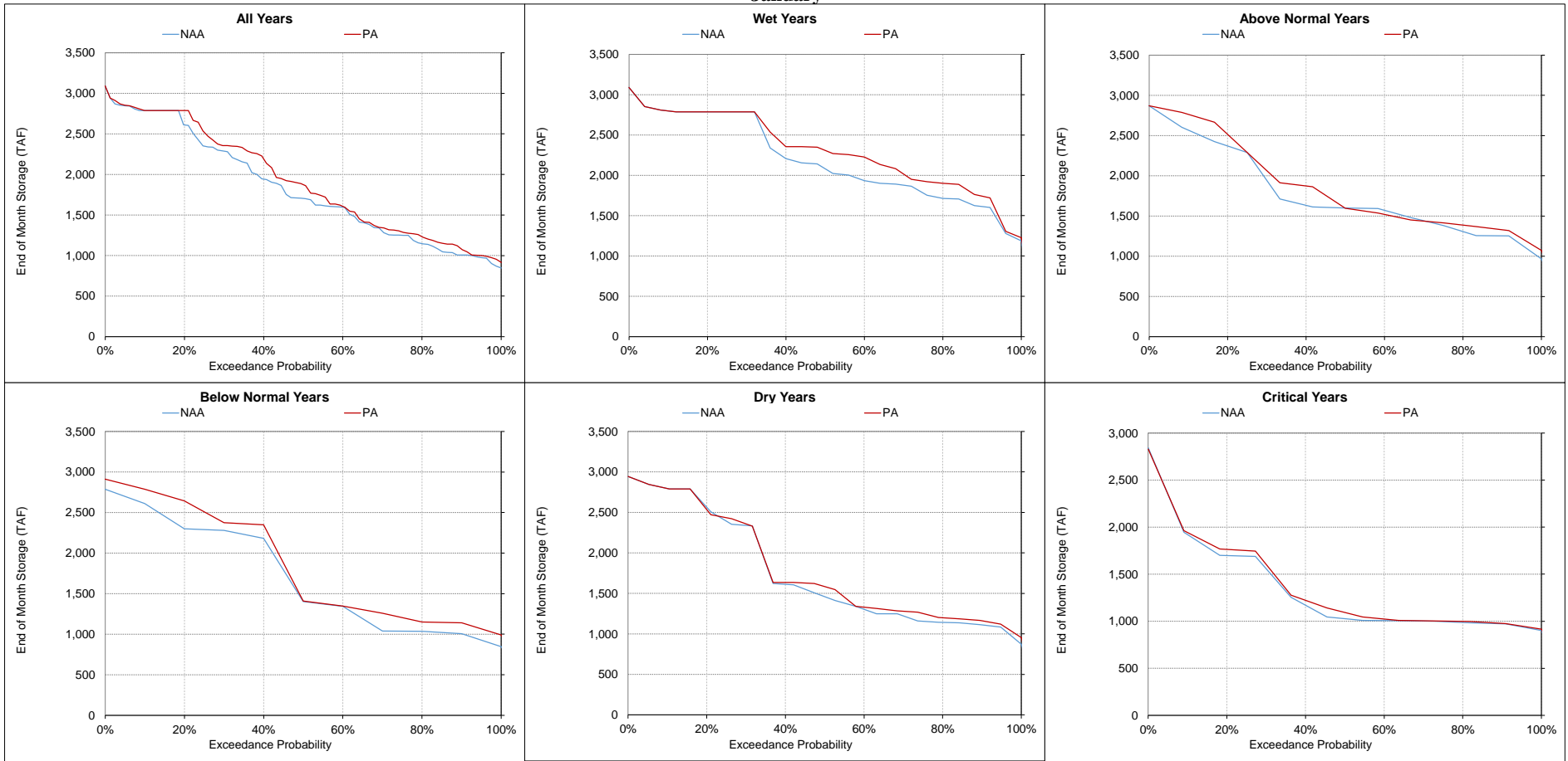
Figure 5.A.6-4-11. Lake Oroville, End of Month Storage January
