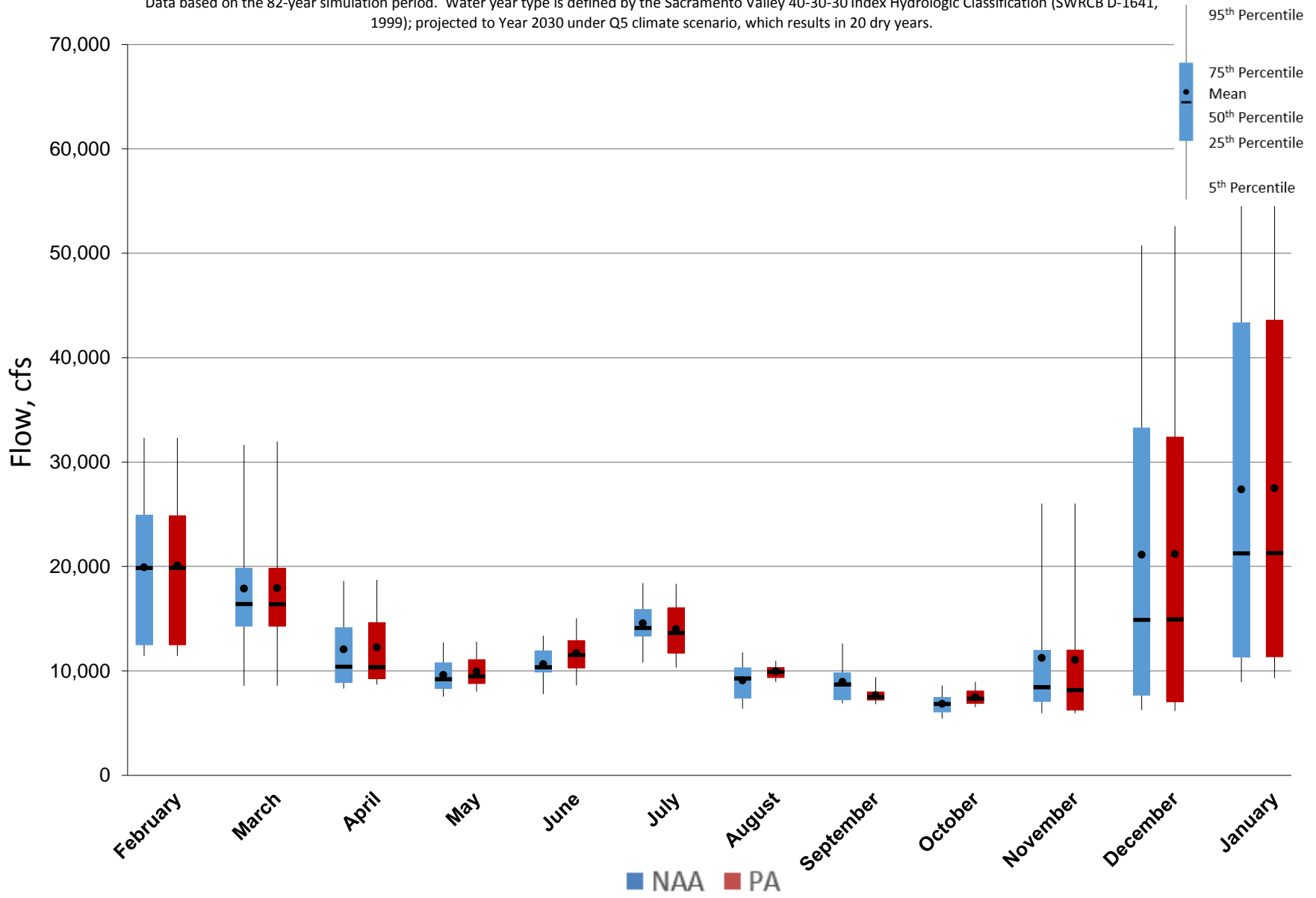
Figure 5.A.6-14-5. Monthly Flow Ranges For Sacramento River at Verona, Dry Years
