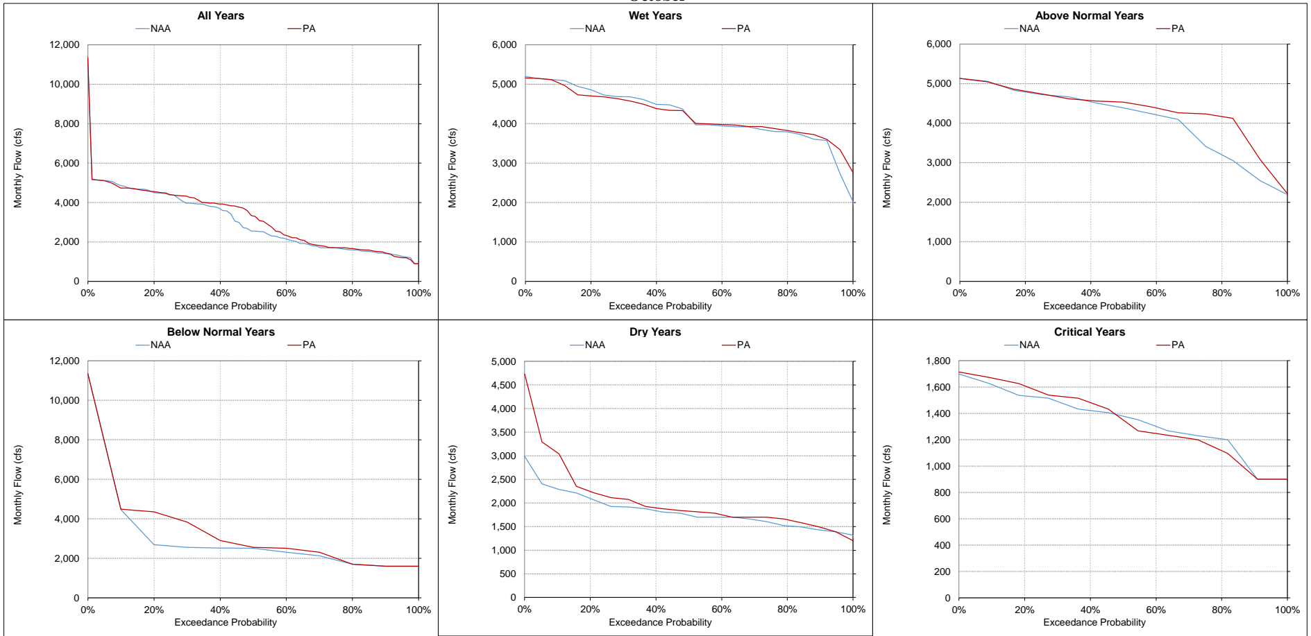
Figure 5.A.6-13-8. Feather River at Sacramento River Confluence, Monthly Flow October
