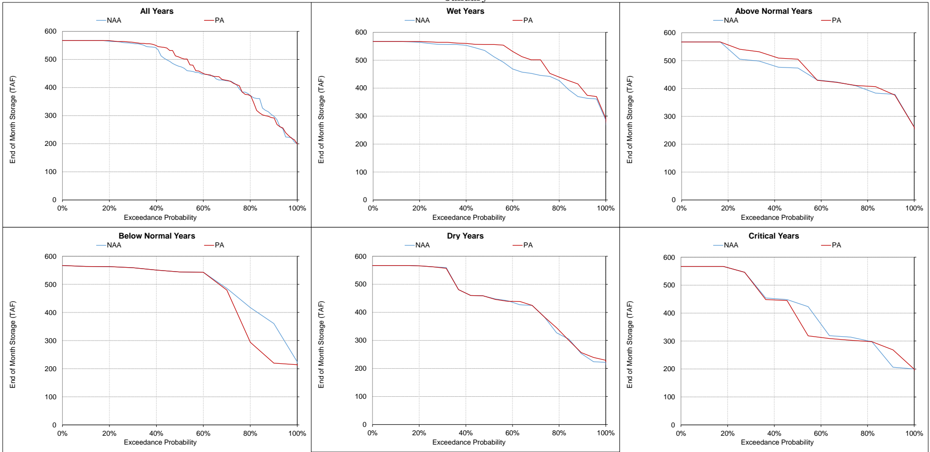
Figure 5.A.6-5-11. Folsom Lake, End of Month Storage January
