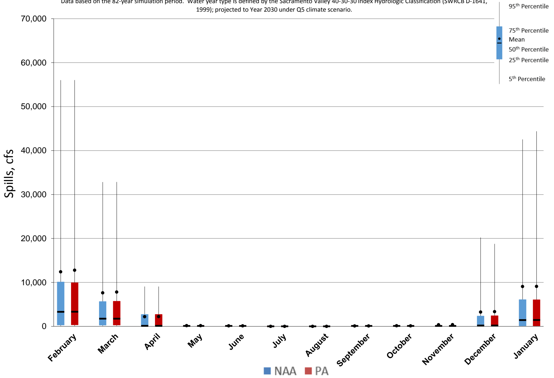
Figure 5.A.6-15-1. Monthly Spills Ranges For Fremont Weir, All Years
