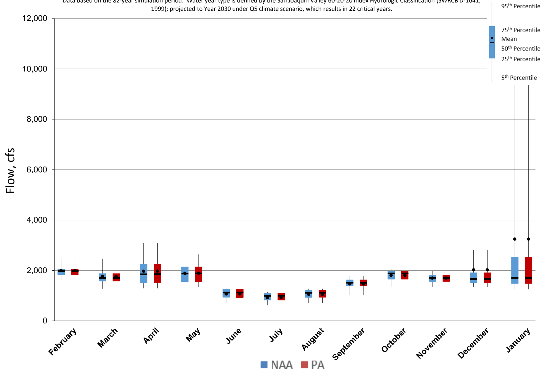
Figure 5.A.6-23-6. Monthly Flow Ranges for San Joaquin River at Vernalis, Critical Years
