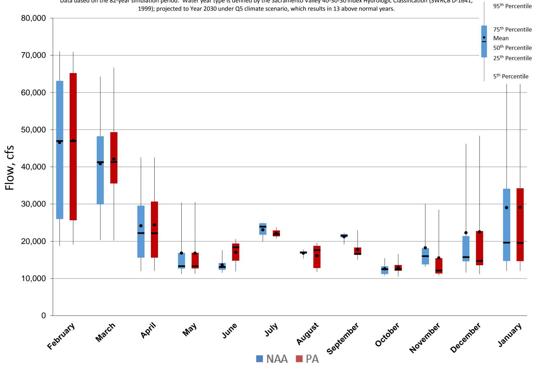
Figure 5.A.6-18-3. Monthly Flow Ranges For Sacramento River at Freeport, Above Normal Years
