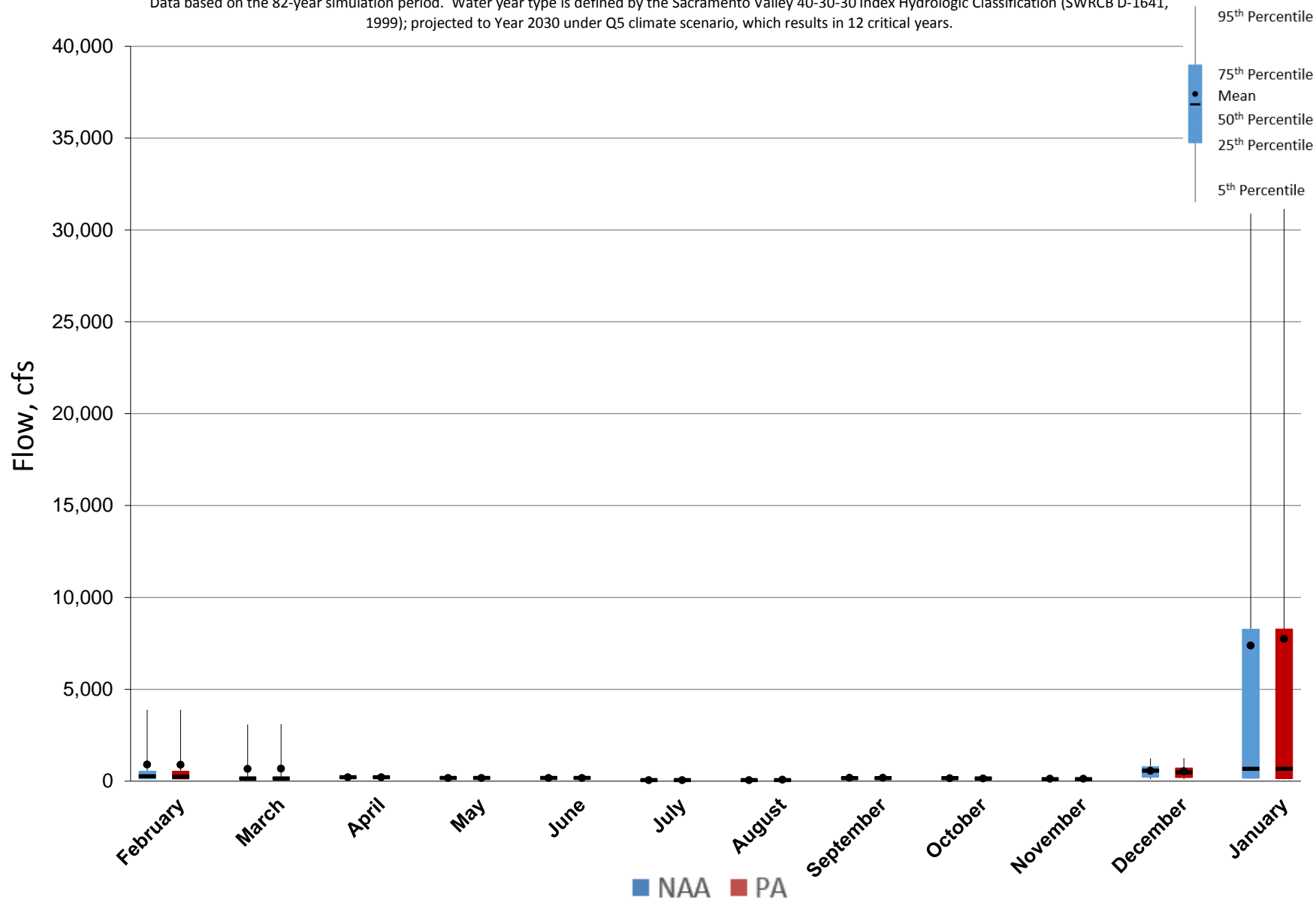
Figure 5.A.6-20-6. Monthly Flow Ranges For Yolo Bypass, Critical Years
