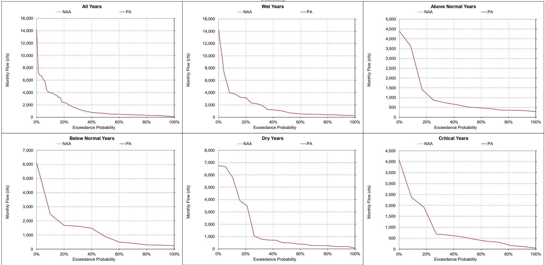
Figure 5.A.6-24-11. Mokelumne and Cosumnes River, Monthly Flow January
