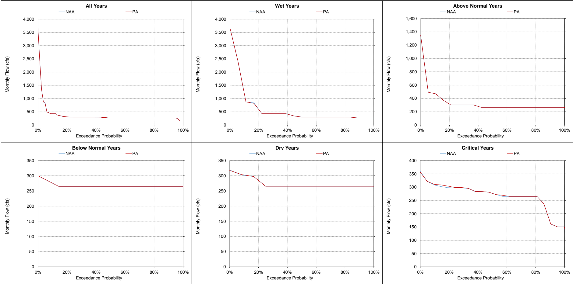
Figure 5.A.6-21-17. Stanislaus River at Ripon, Monthly Flow
