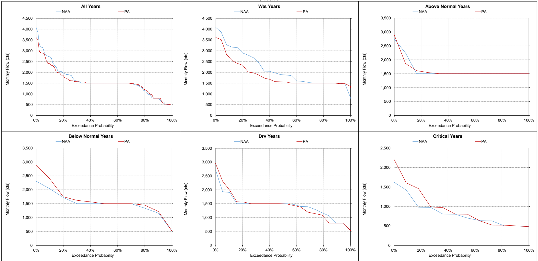
Figure 5.A.6-16-8. American River below Nimbus Dam, Monthly Flow October
