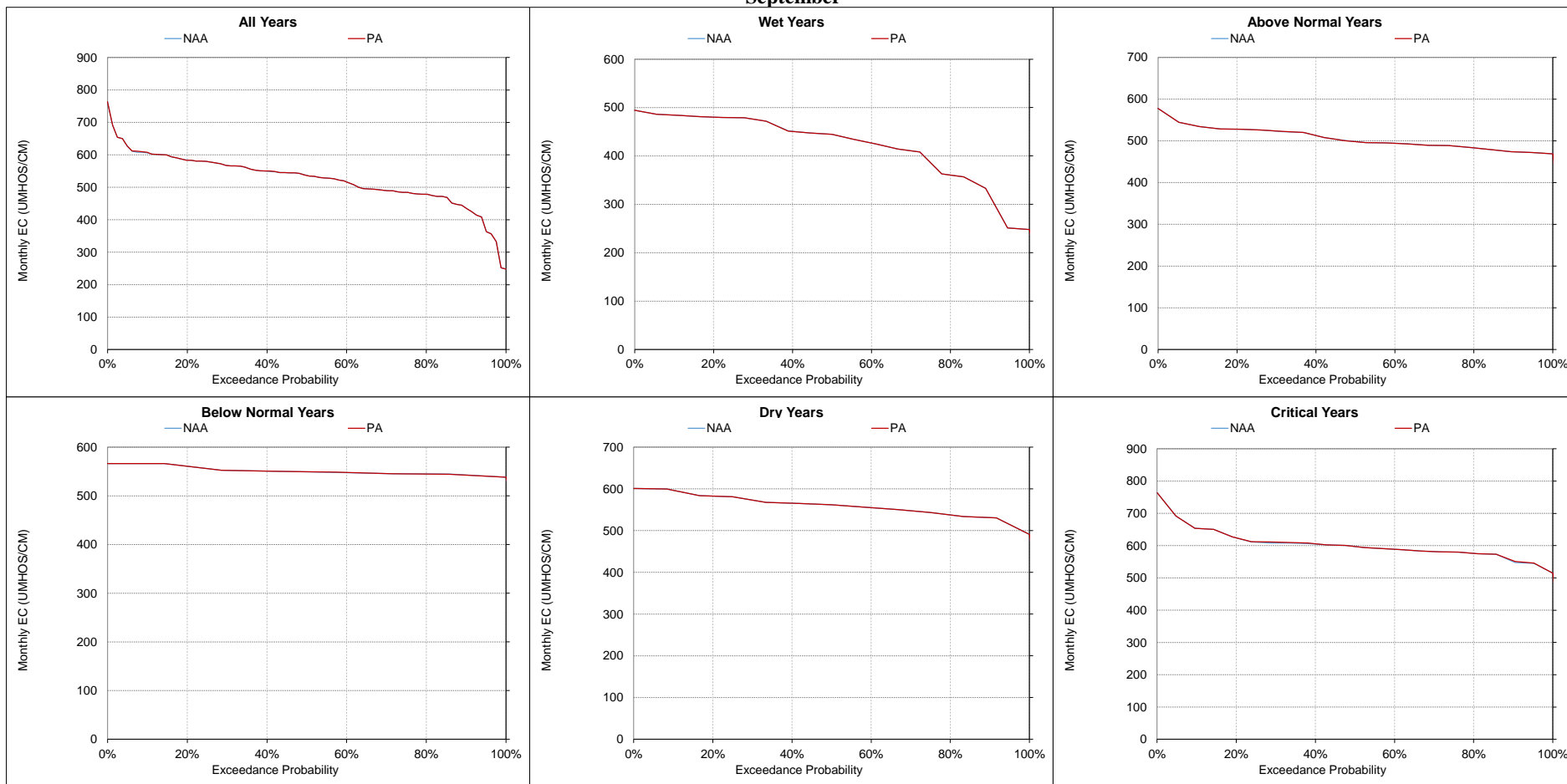
Figure 5.A.6-30-19. San Joaquin River at Vernalis, Monthly EC September
