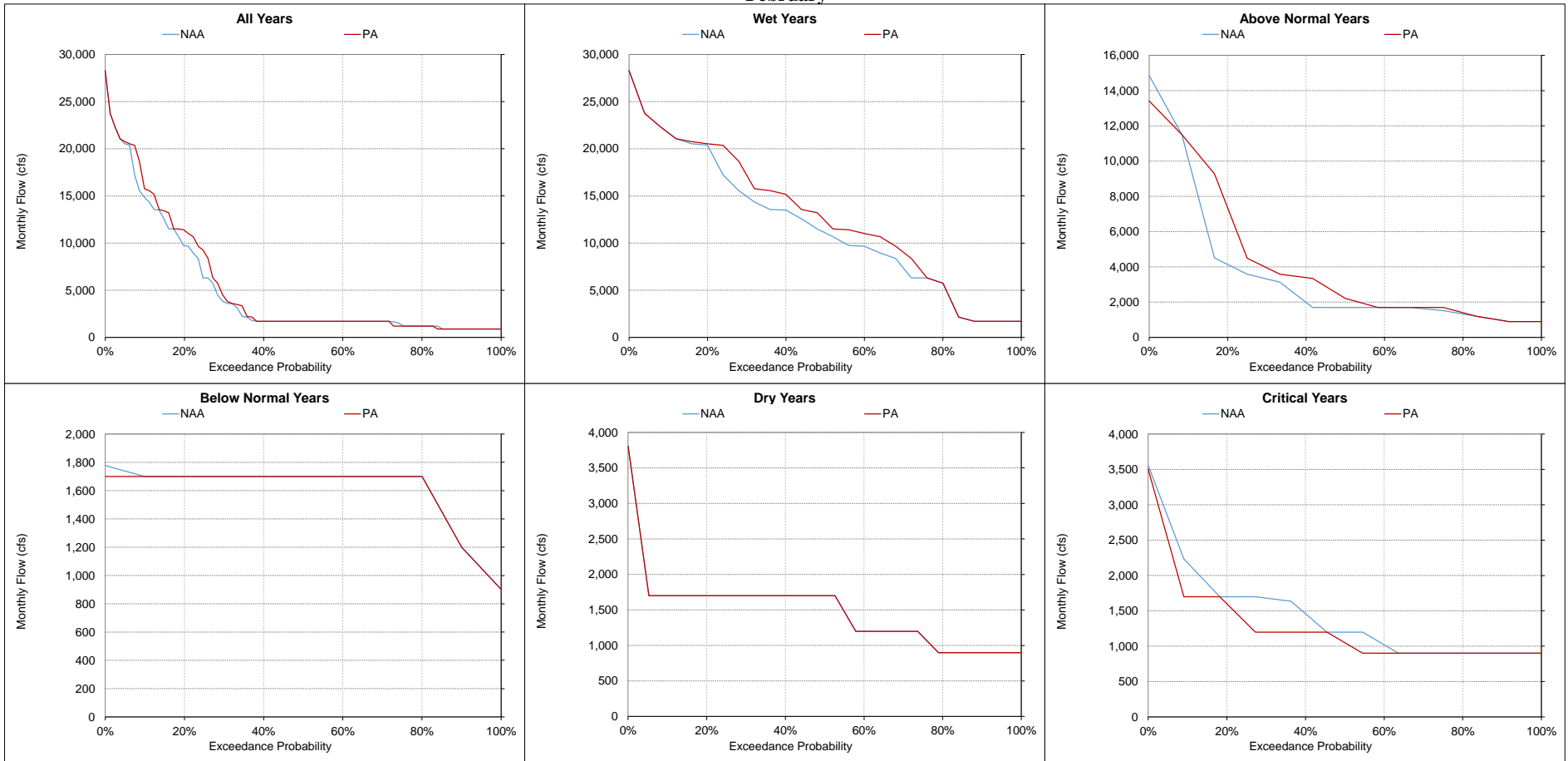
Figure 5.A.6-12-12. Feather River below Thermalito Diversion Dam, Monthly Flow February
