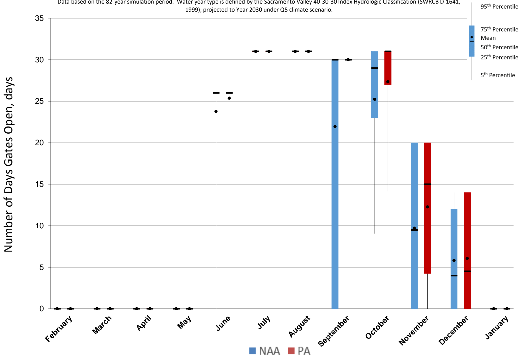
Figure 5.A.6-31-1. Average Number of Days Gates Open Ranges For Delta Cross Channel, All Years
