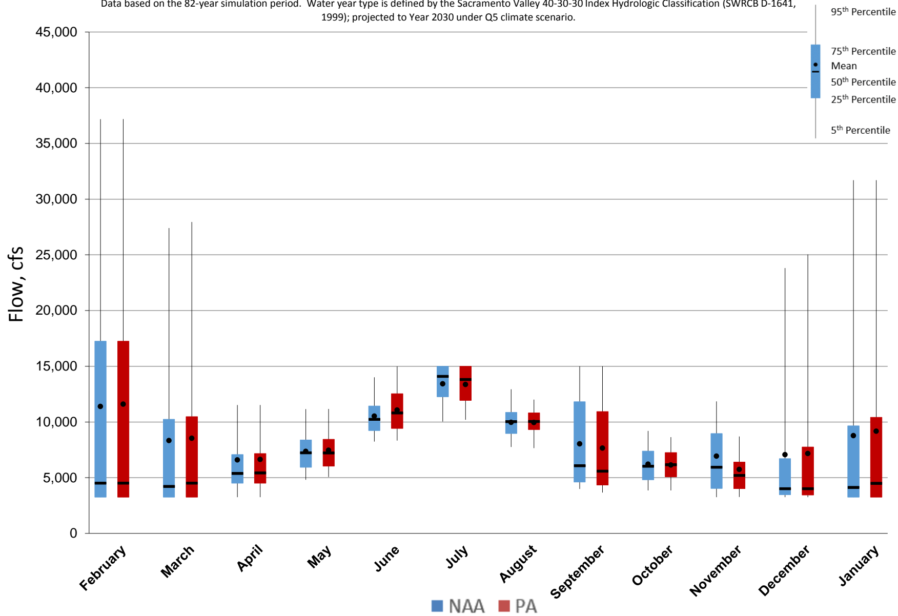
Figure 5.A.6-10-1. Monthly Flow Ranges For Sacramento River below Keswick Dam, All Years
