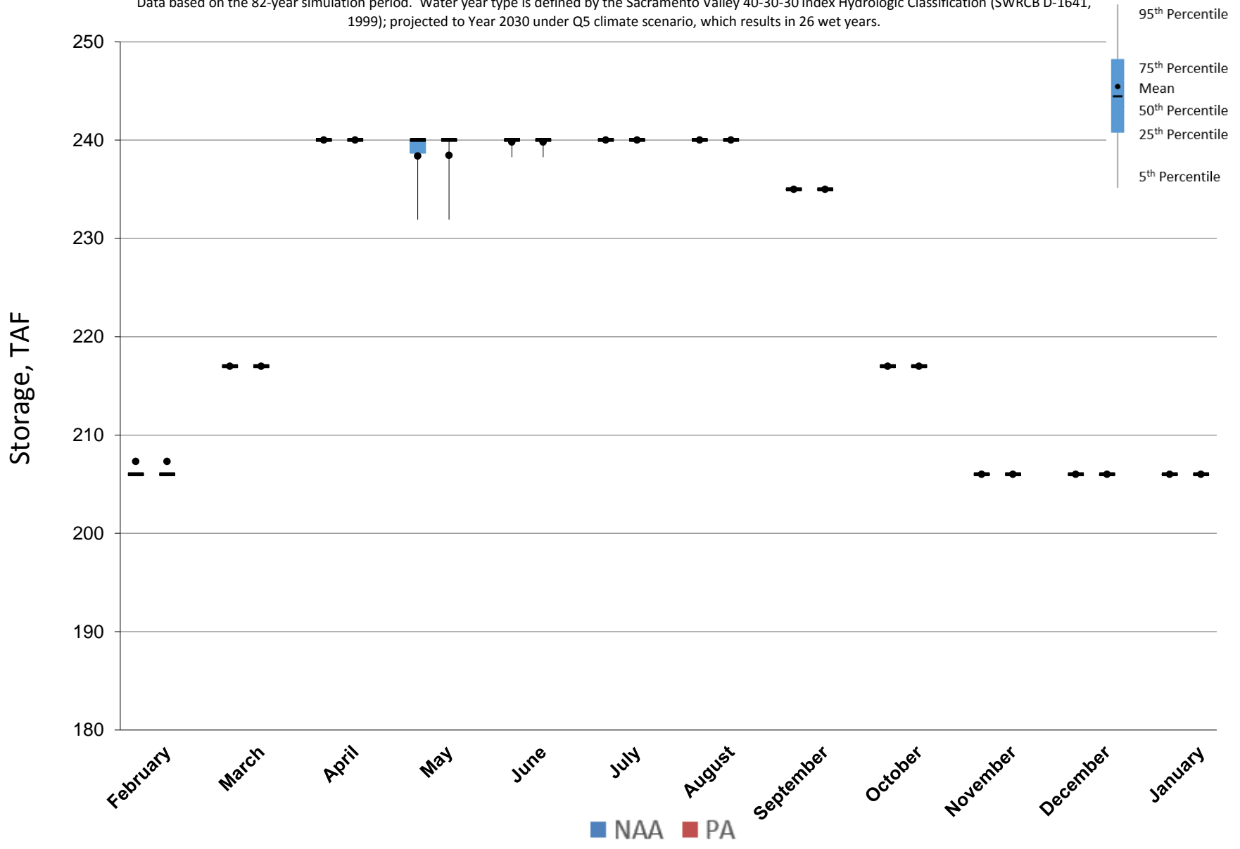
Figure 5.A.6-2-2. End of Month Storage Ranges For Whiskeytown Reservoir, Wet Years
