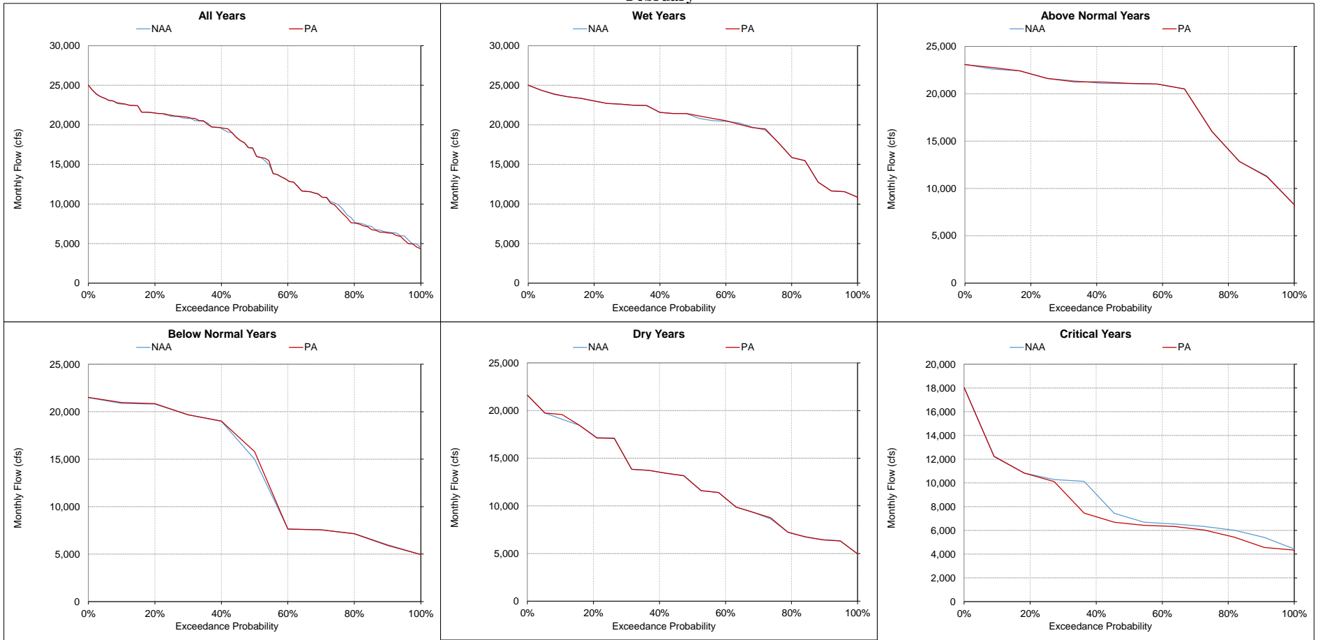
Figure 5.A.6-11-12. Sacramento River at Bend Bridge, Monthly Flow February
