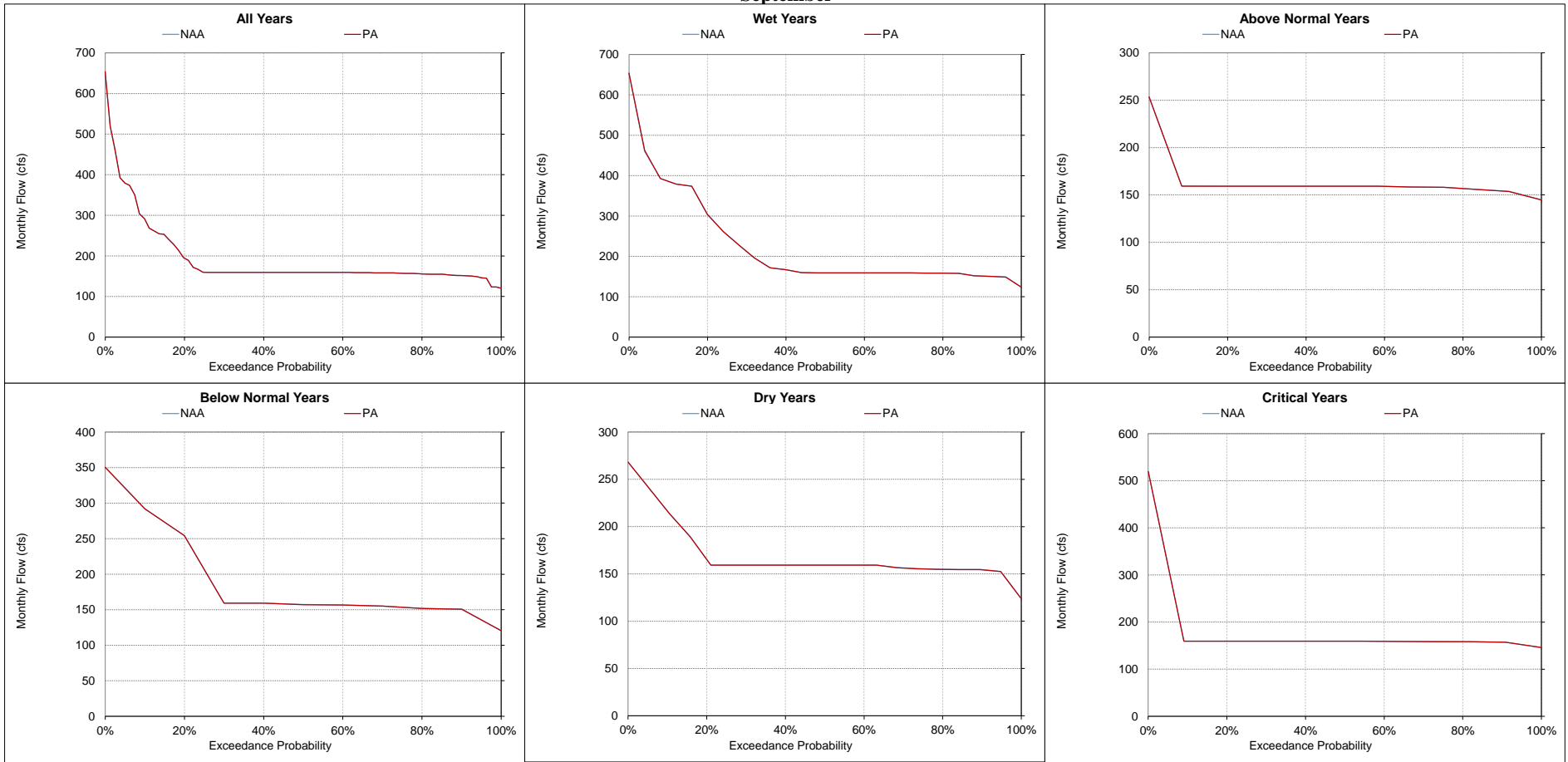
Figure 5.A.6-20-19. Yolo Bypass, Monthly Flow September
