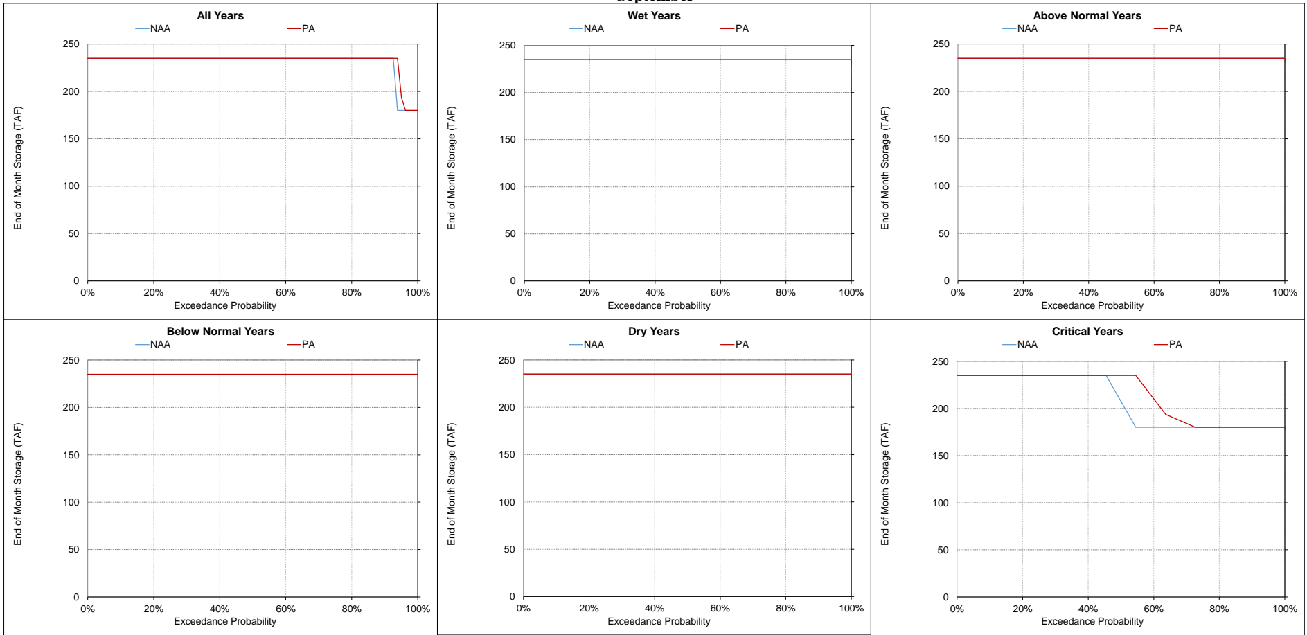
Figure 5.A.6-2-19. Whiskeytown Reservoir, End of Month Storage September
