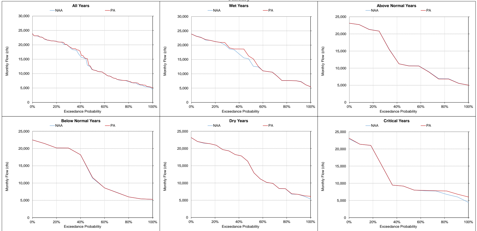
Figure 5.A.6-11-11. Sacramento River at Bend Bridge, Monthly Flow January
