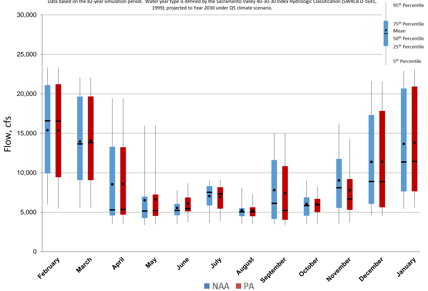
Figure 5.A.6-11-1. Monthly Flow Ranges For Sacramento River at Bend Bridge, All Years
