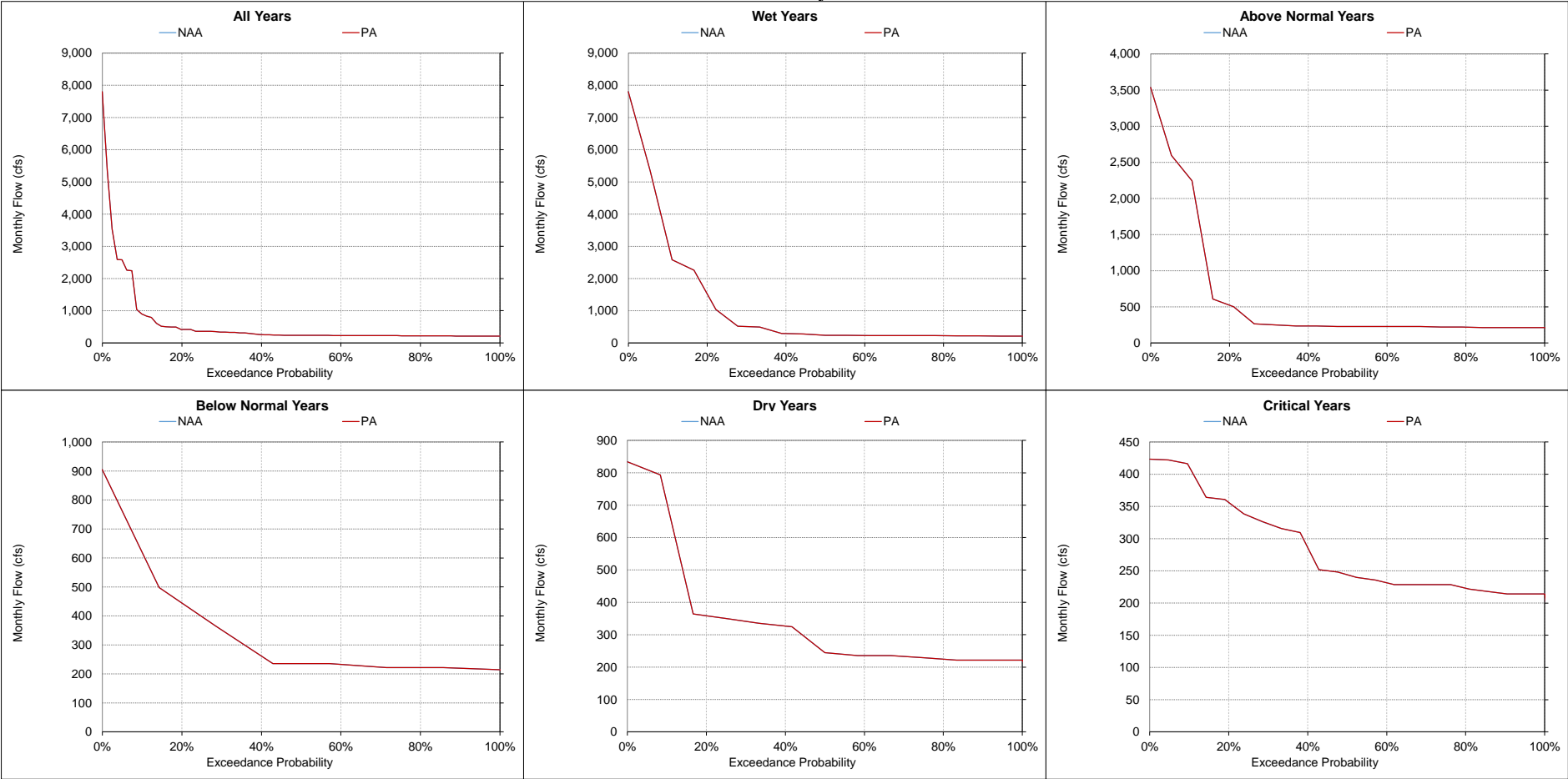
Figure 5.A.6-21-12. Stanislaus River at Ripon, Monthly Flow February
