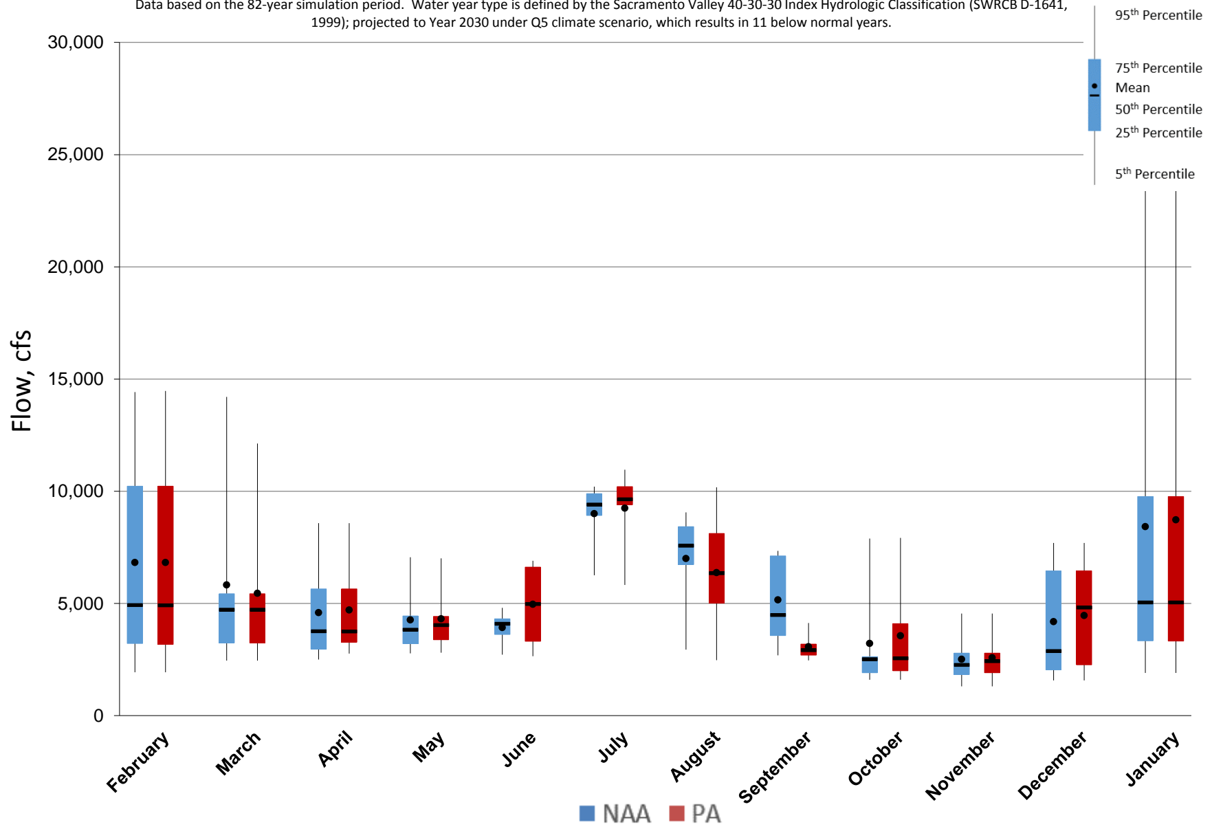
Figure 5.A.6-13-4. Monthly Flow Ranges For Feather River at Sacramento River Confluence, Below Normal Years
