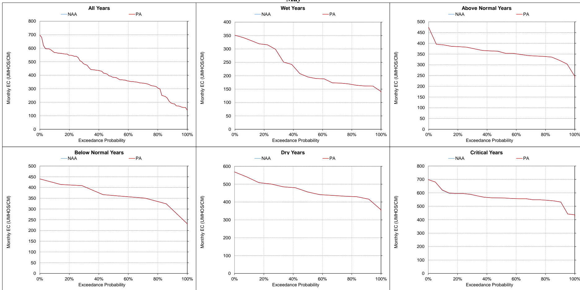
Figure 5.A.6-30-15. San Joaquin River at Vernalis, Monthly EC May
