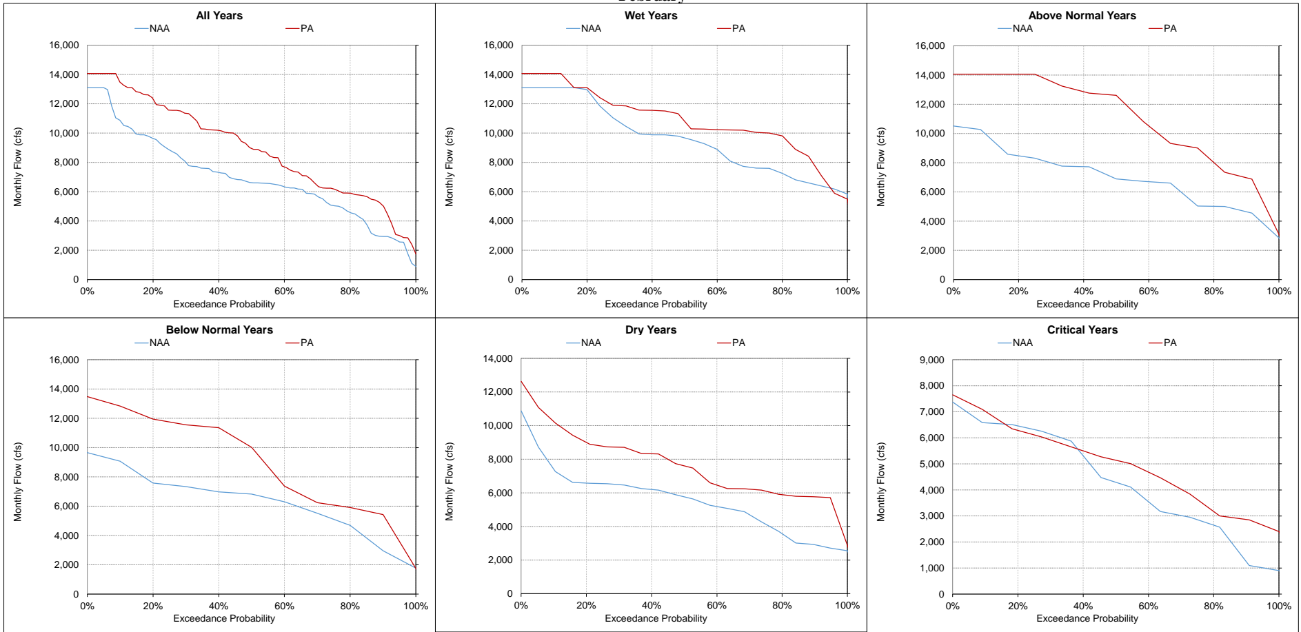
Figure 5.A.6-28-12. Total Delta Exports, Monthly Flow February
