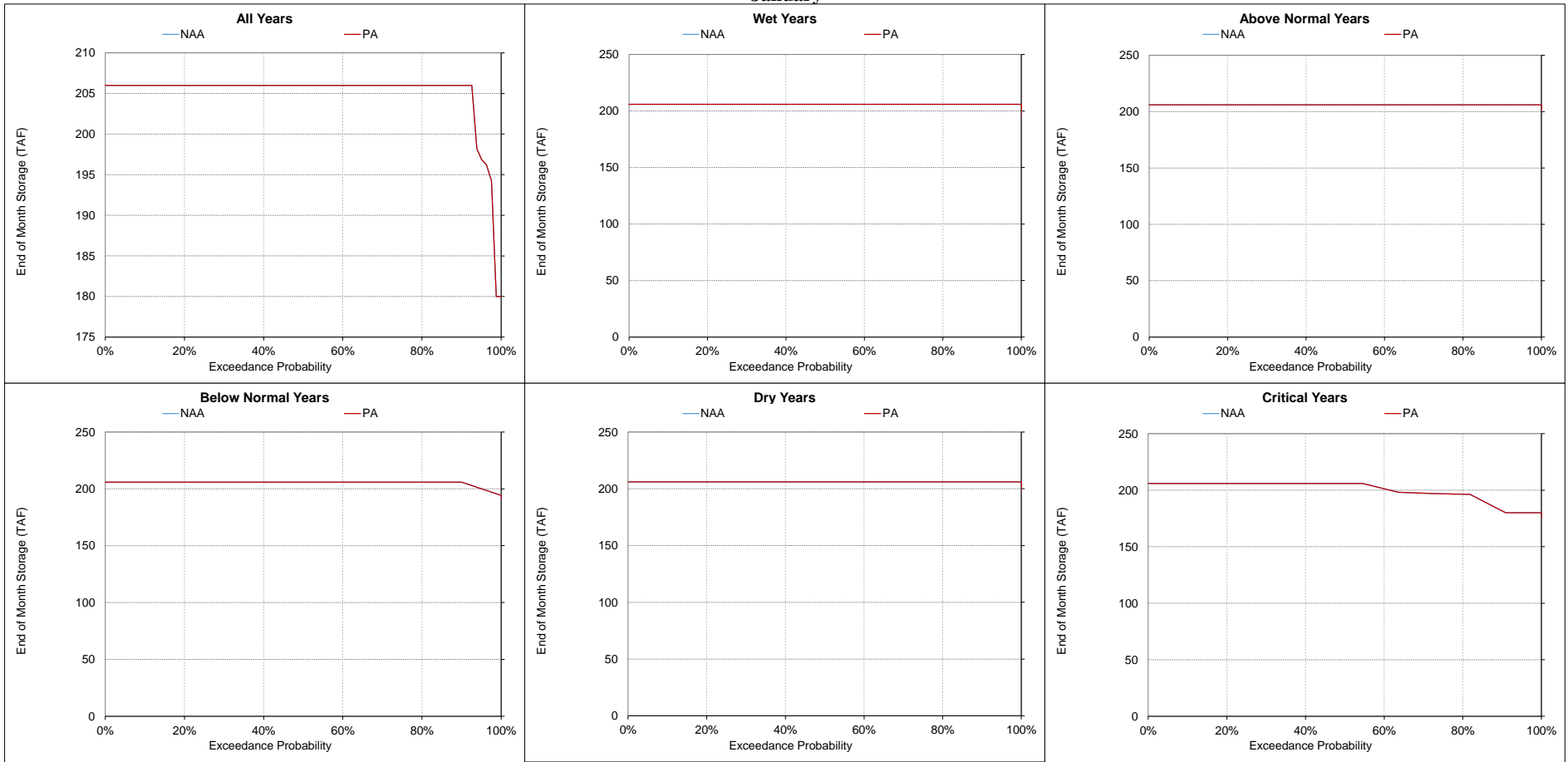
Figure 5.A.6-2-11. Whiskeytown Reservoir, End of Month Storage January
