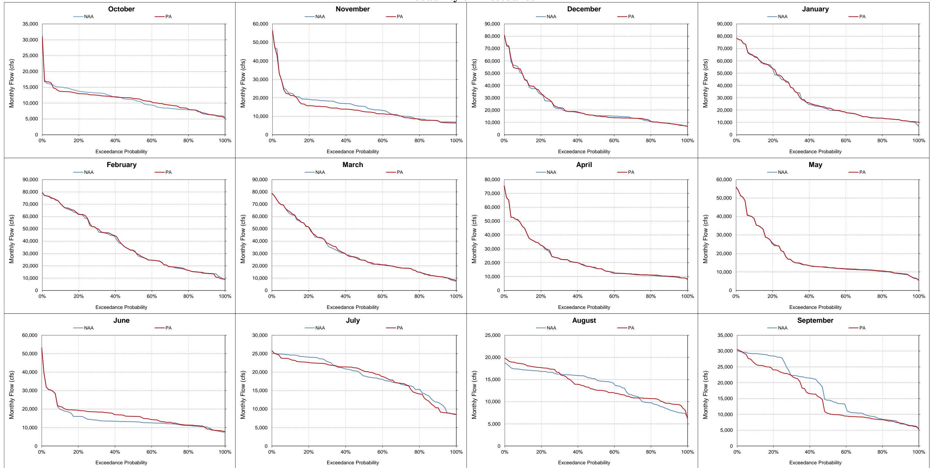
Figure 5.A.6-18-7. Sacramento River at Freeport, Monthly Flow Probability of Exceedance
