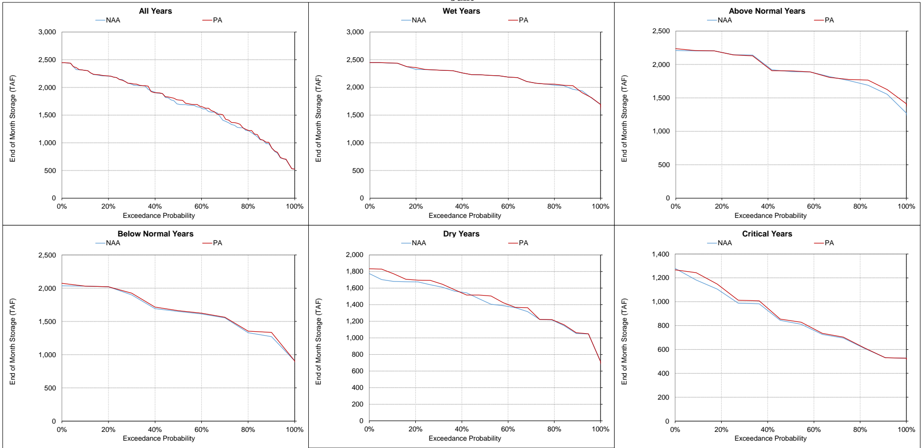
Figure 5.A.6-1-16. Trinity Lake, End of Month Storage June
