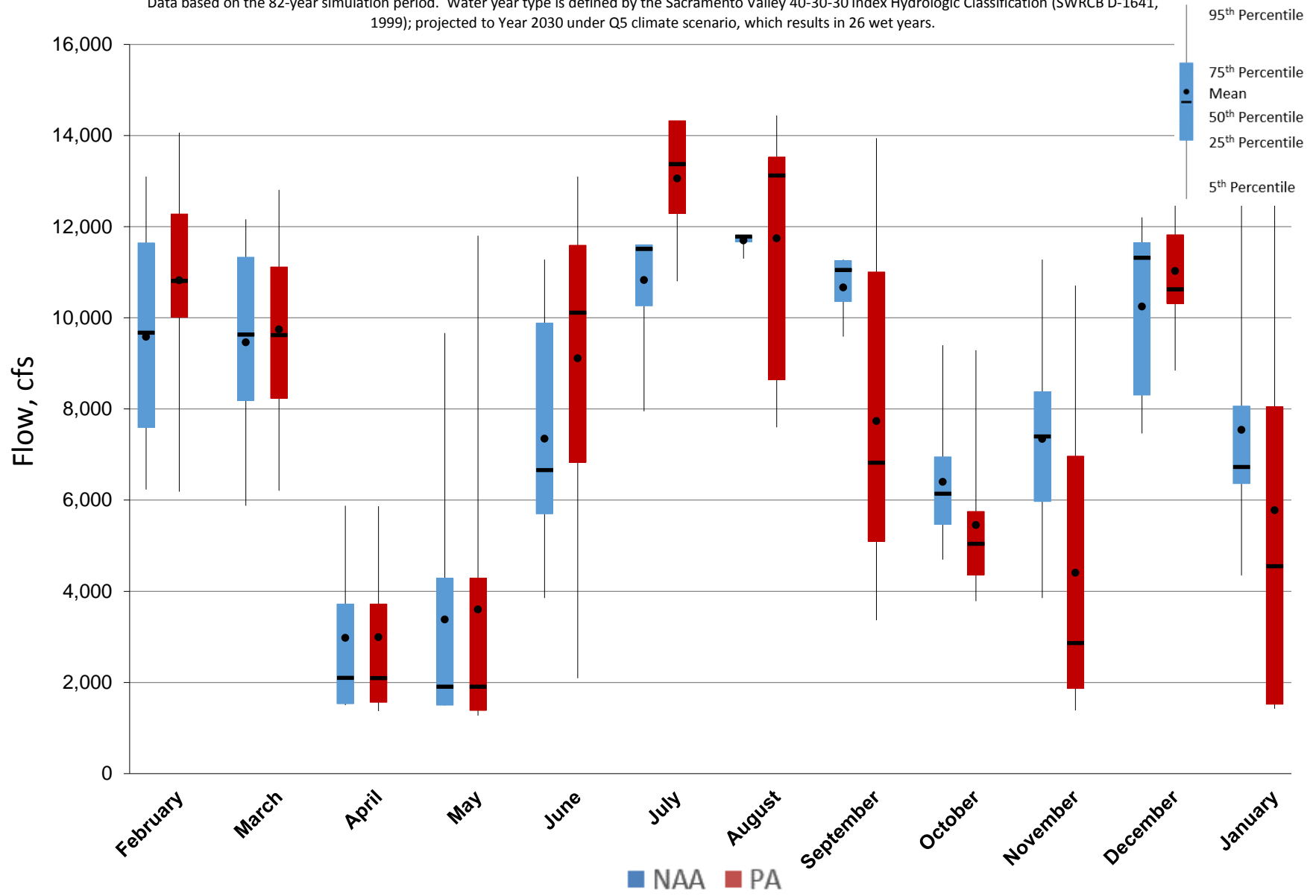
Figure 5.A.6-28-2. Monthly Flow Ranges For Total Delta Exports, Wet Years
