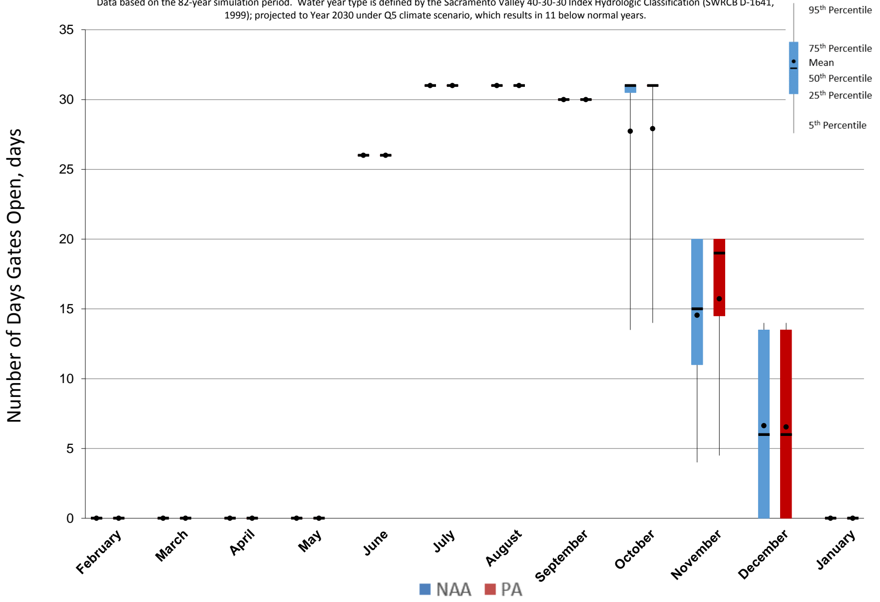
Figure 5.A.6-31-4. Average Number of Days Gates Open Ranges For Delta Cross Channel, Below Normal Years
