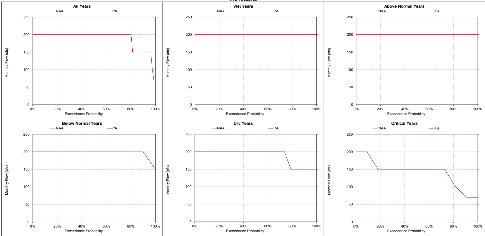
Figure 5.A.6-9-9. Clear Creek below Whiskeytown Dam, Monthly Flow November
