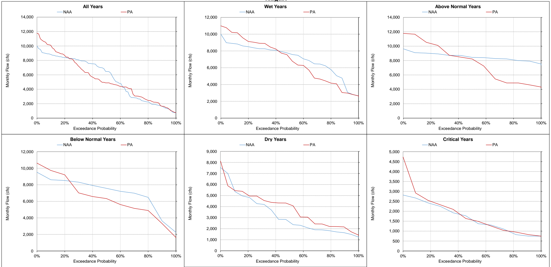
Figure 5.A.6-13-18. Feather River at Sacramento River Confluence, Monthly Flow August
