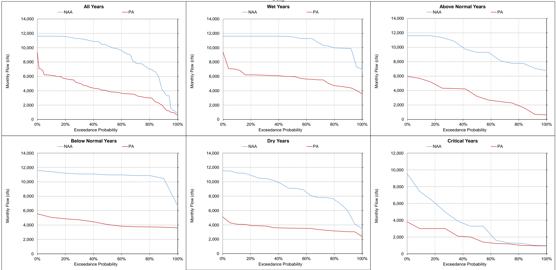
Figure 5.A.6-27-17. South Delta Exports, Monthly Flow July
