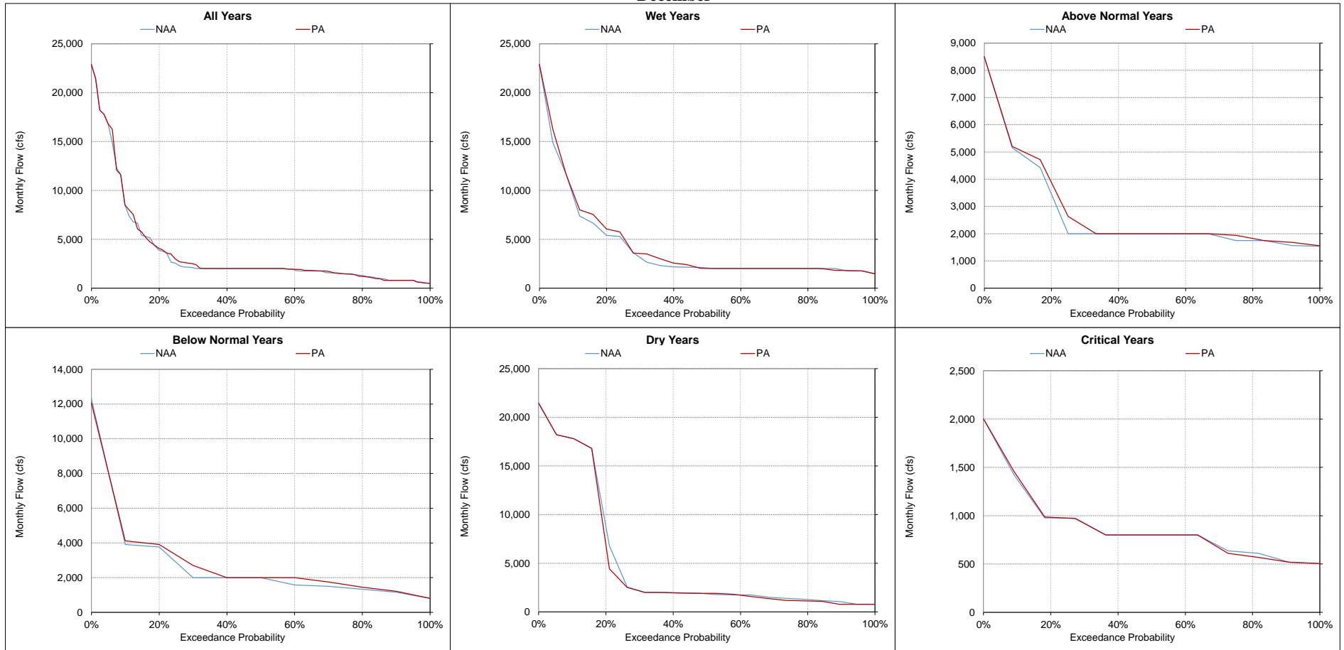
Figure 5.A.6-16-10. American River below Nimbus Dam, Monthly Flow December
