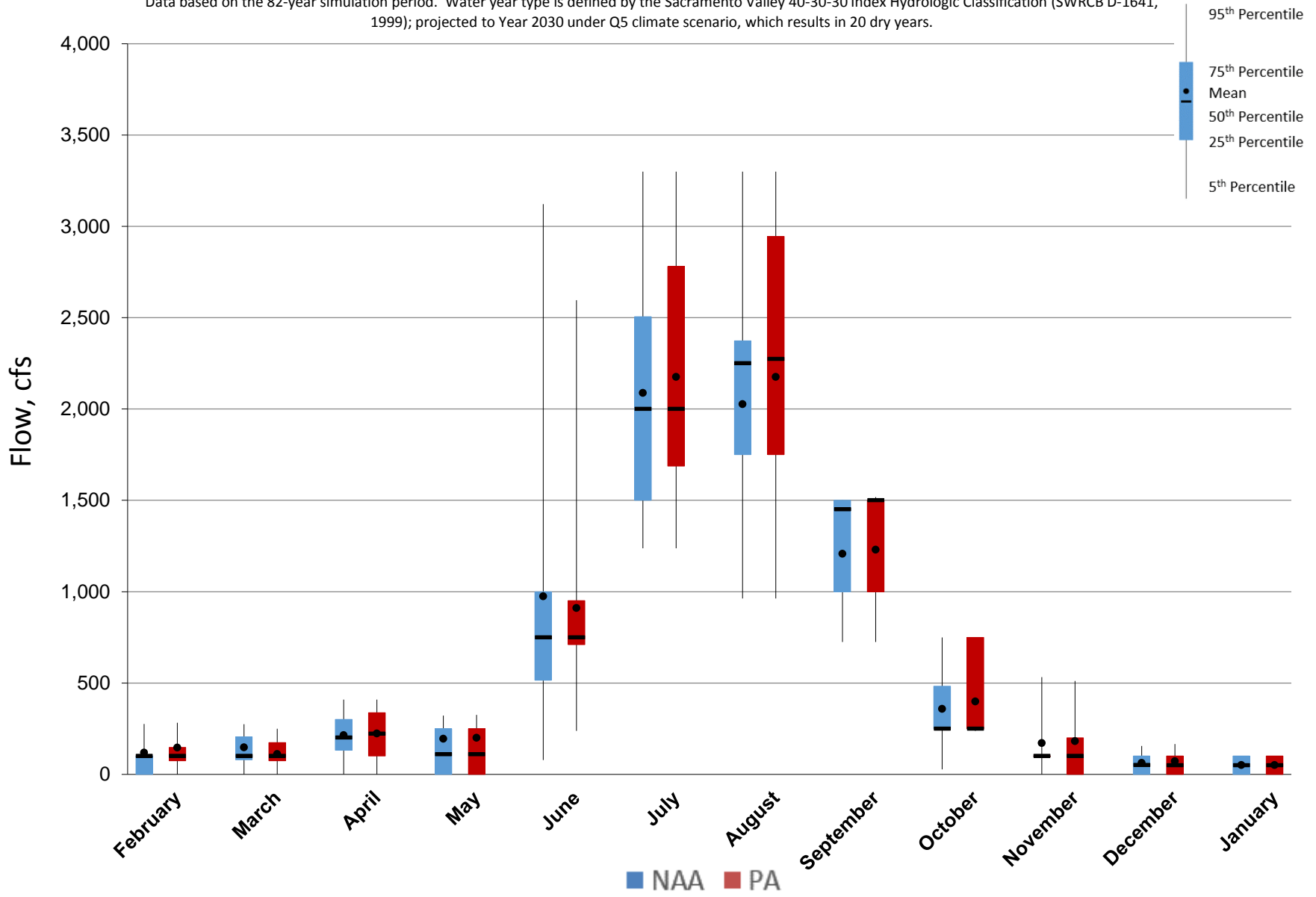
Figure 5.A.6-8-5. Monthly Flow Ranges For Clear Creek Tunnel Flow, Dry Years
