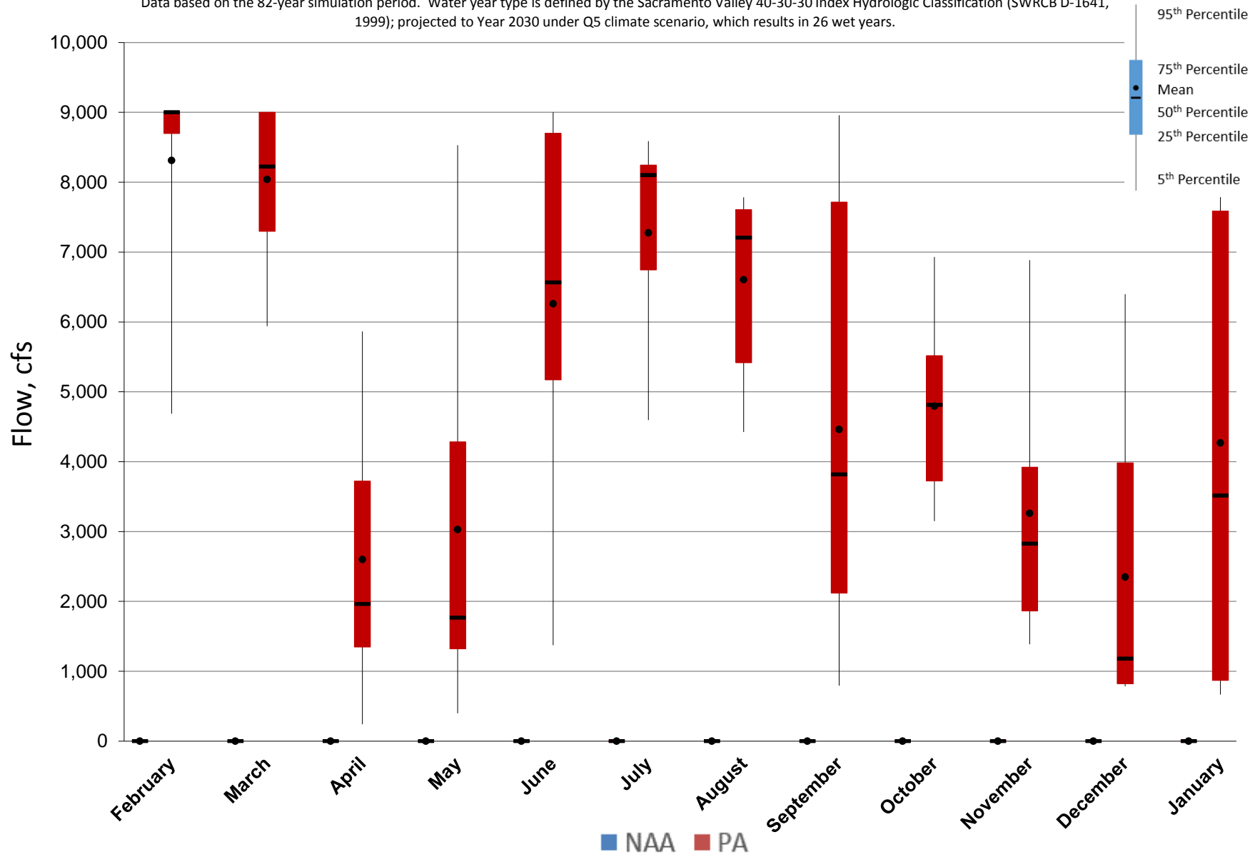
Figure 5.A.6-19-2. Monthly Flow Ranges For North Delta Diversions near Hood, Wet Years
