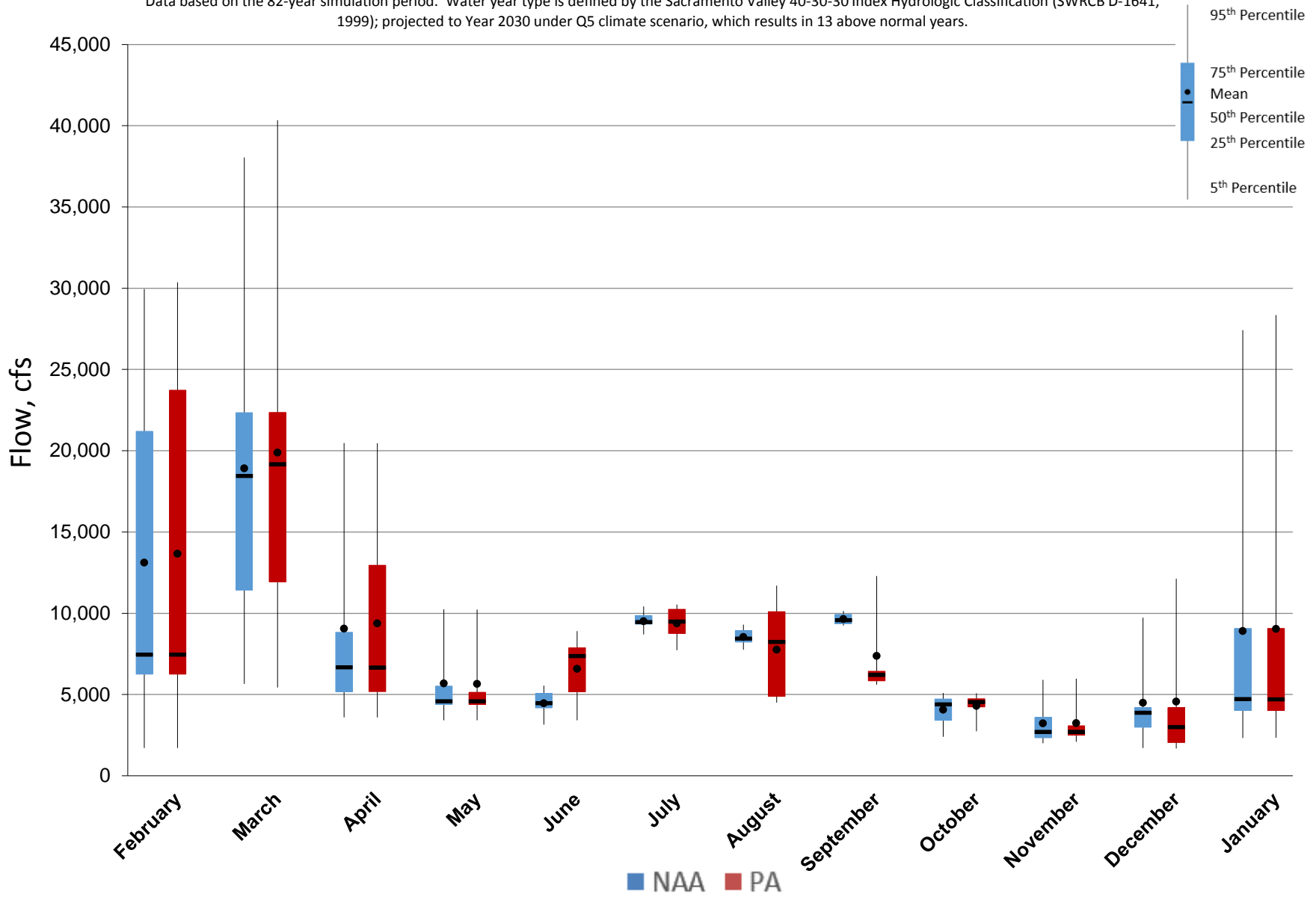
Figure 5.A.6-13-3. Monthly Flow Ranges For Feather River at Sacramento River Confluence, Above Normal Years
