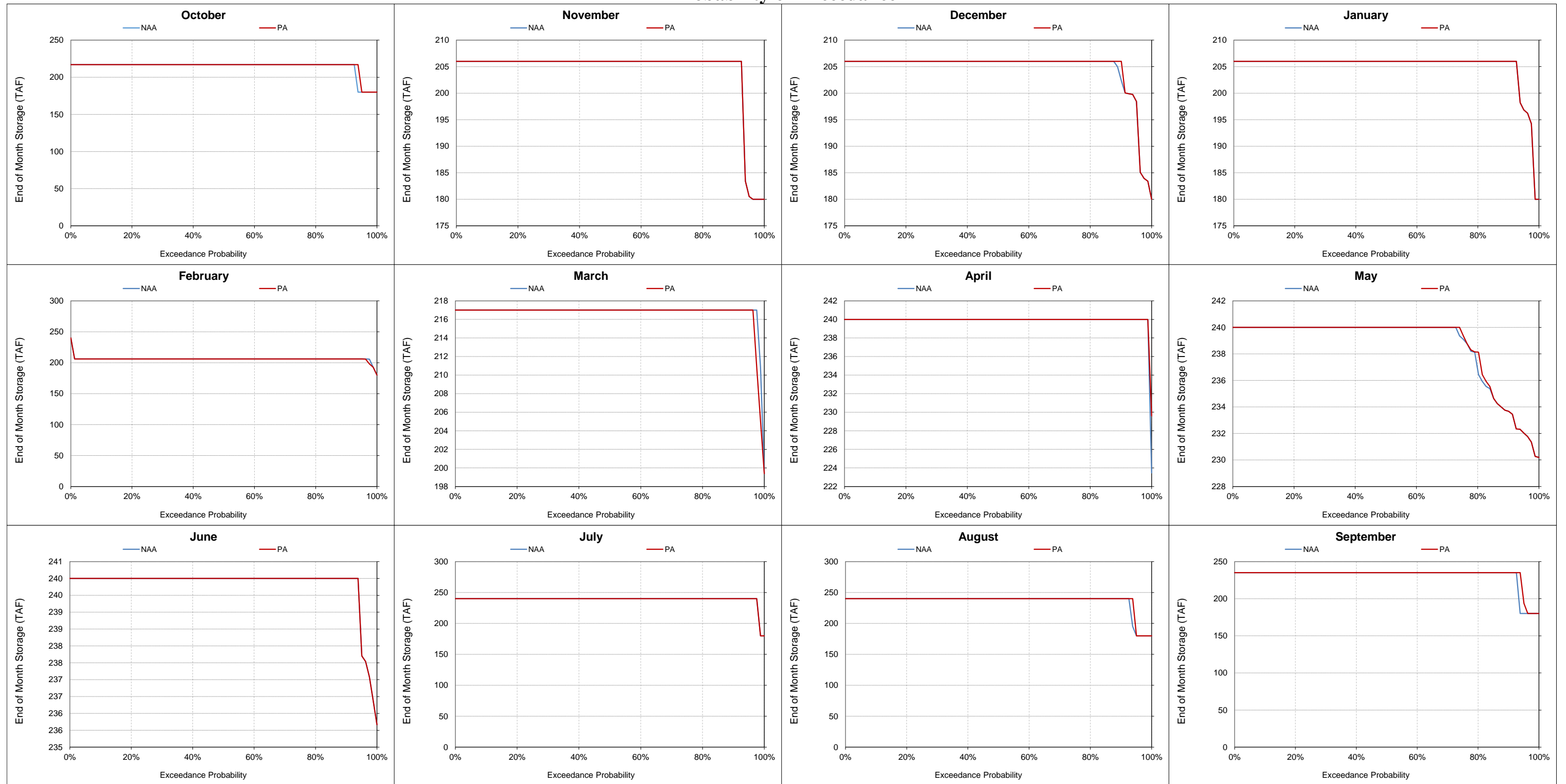
Figure 5.A.6-2-7. Whiskeytown Reservoir, End of Month Storage Probability of Exceedance
