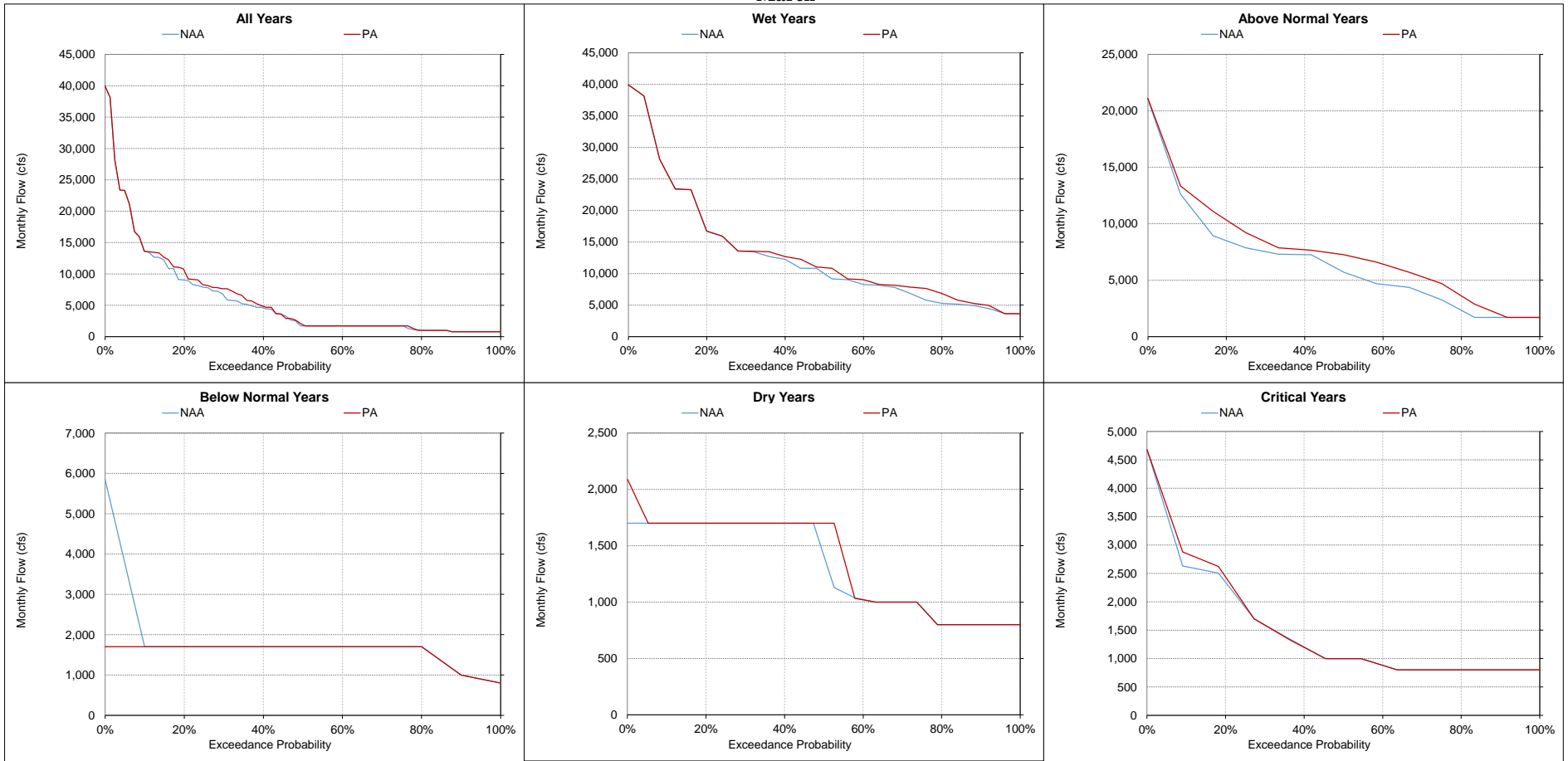
Figure 5.A.6-12-13. Feather River below Thermalito Diversion Dam, Monthly Flow March
