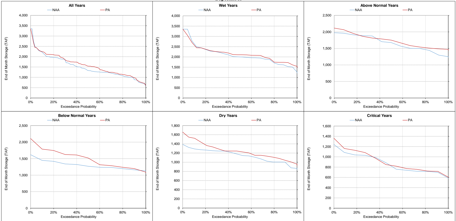
Figure 5.A.6-4-19. Lake Oroville, End of Month Storage September
