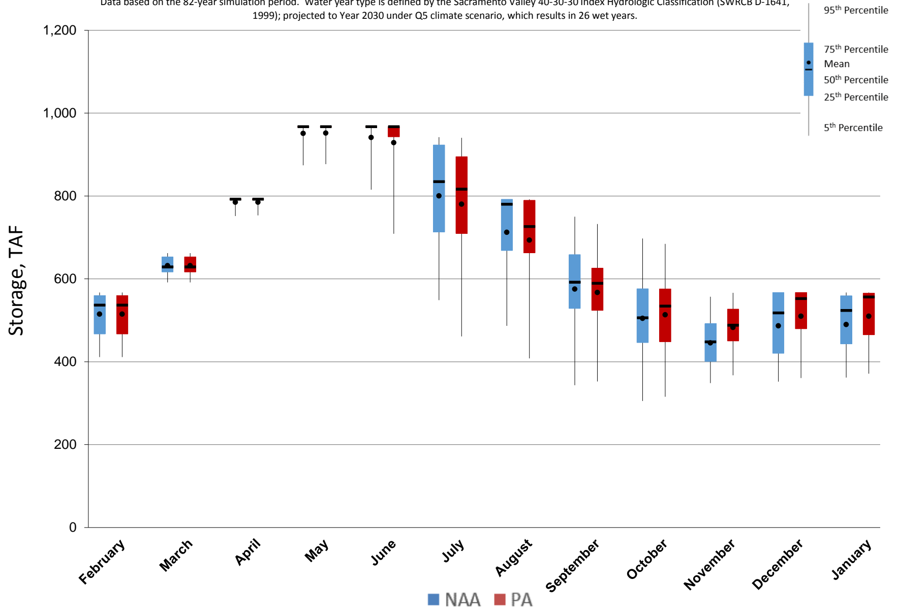
Figure 5.A.6-5-2. End of Month Storage Ranges For Folsom Lake, Wet Years
