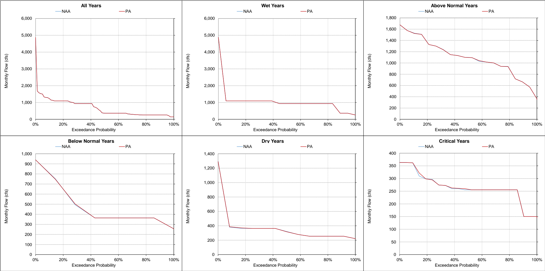
Figure 5.A.6-21-16. Stanislaus River at Ripon, Monthly Flow
