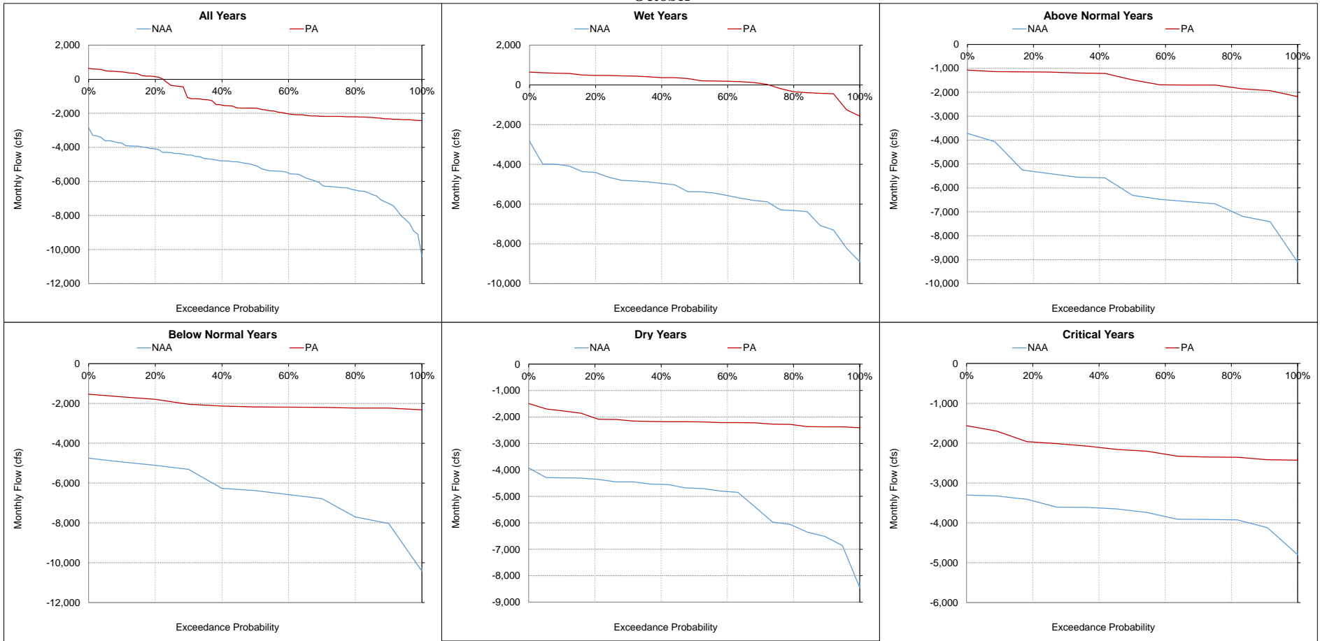
Figure 5.A.6-25-8. Old and Middle River, Monthly Flow October
