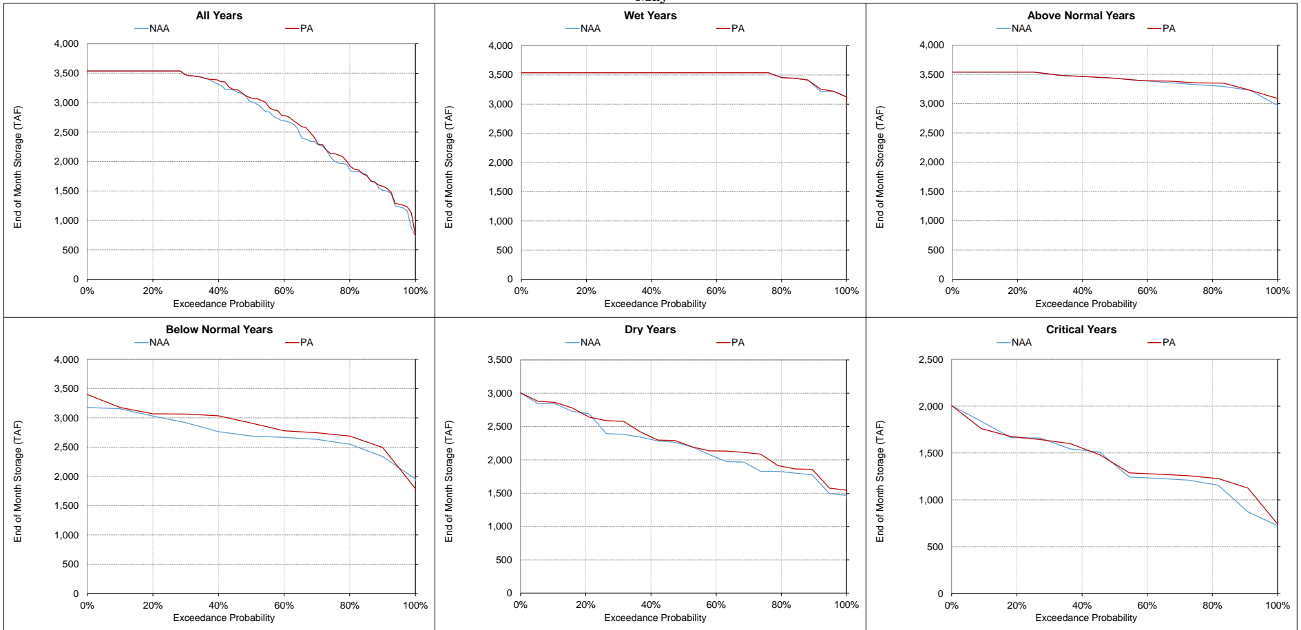
Figure 5.A.6-4-15. Lake Oroville, End of Month Storage May
