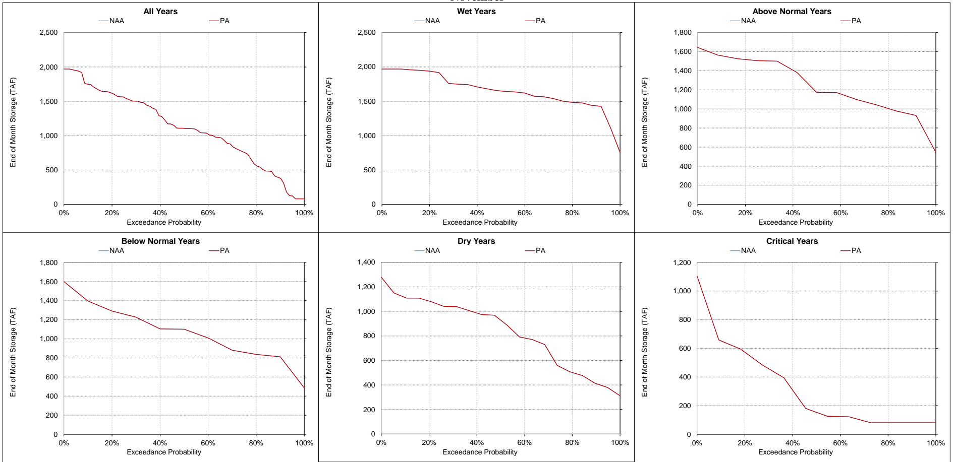
Figure 5.A.6-9. New Melones Lake, End of Month Storage November
