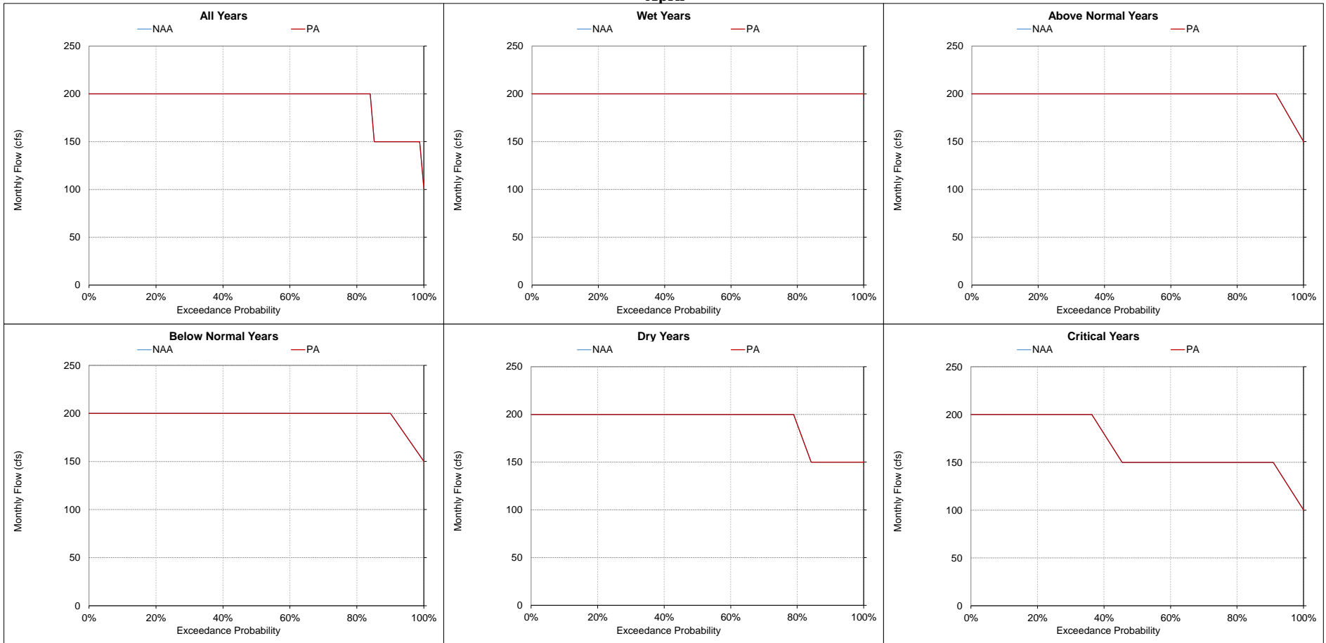
Figure 5.A.6-9-14. Clear Creek below Whiskeytown Dam, Monthly Flow April
