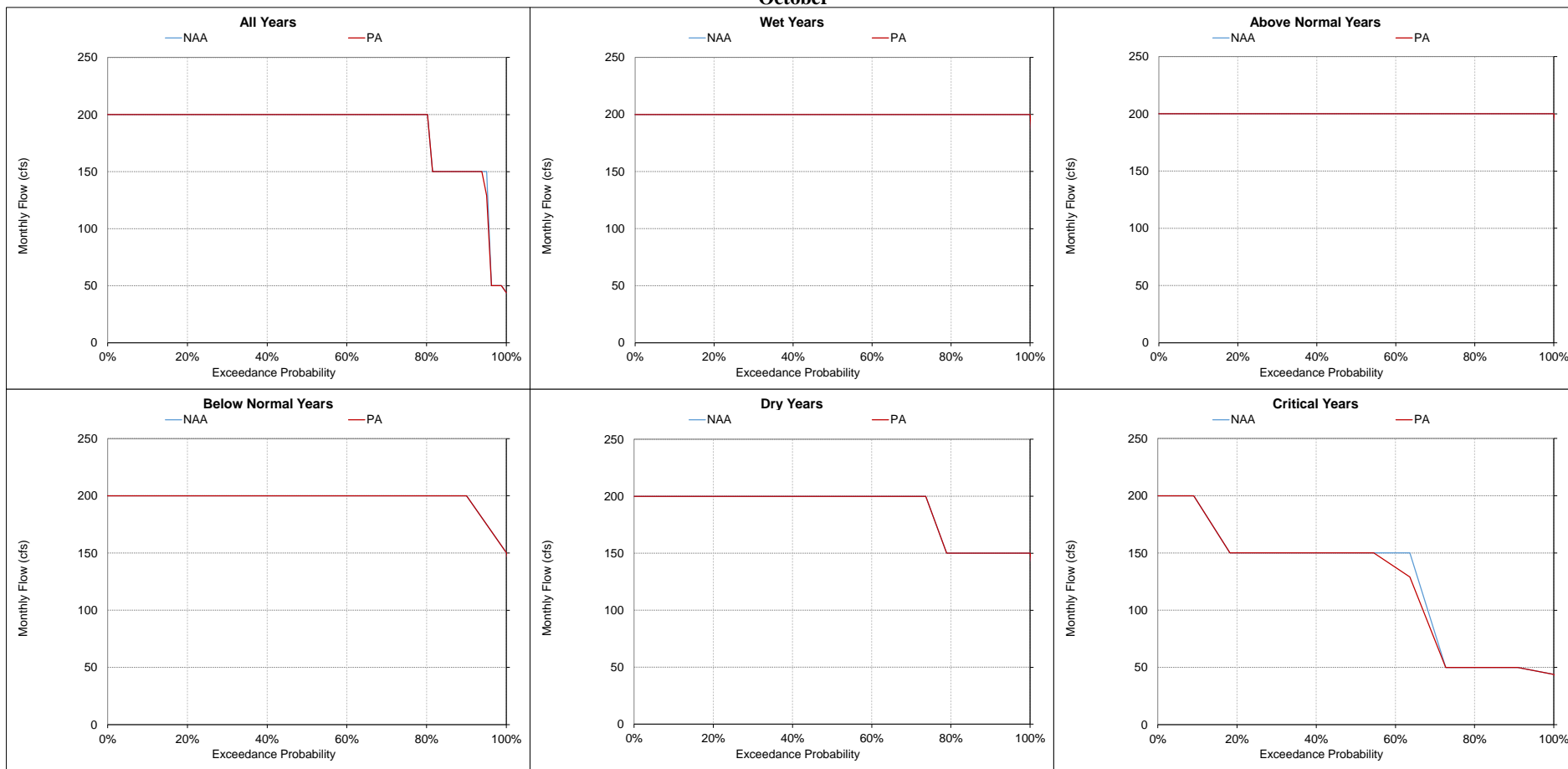
Figure 5.A.6-9-8. Clear Creek below Whiskeytown Dam, Monthly Flow October
