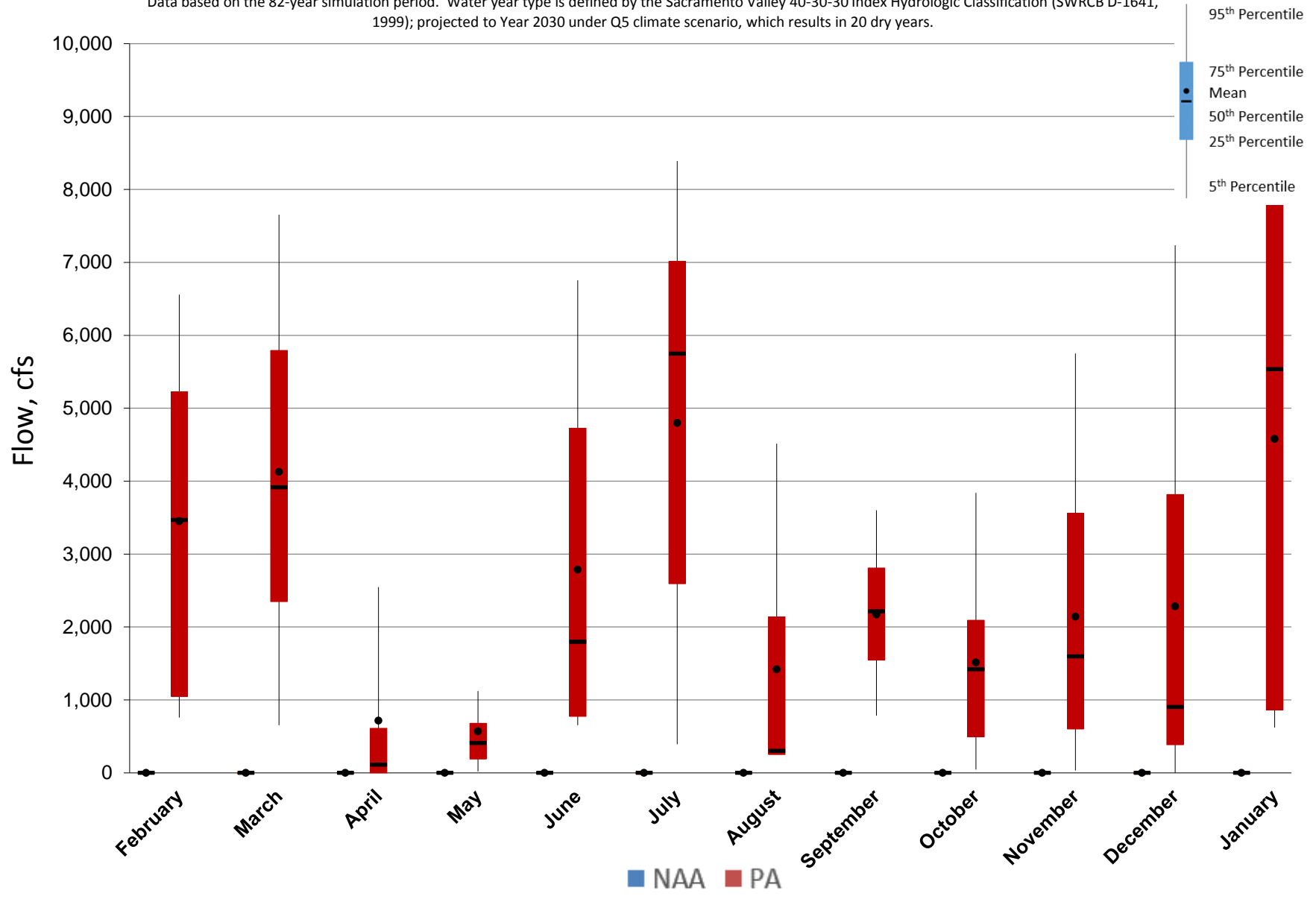
Figure 5.A.6-19-5. Monthly Flow Ranges For North Delta Diversions near Hood, Dry Years
