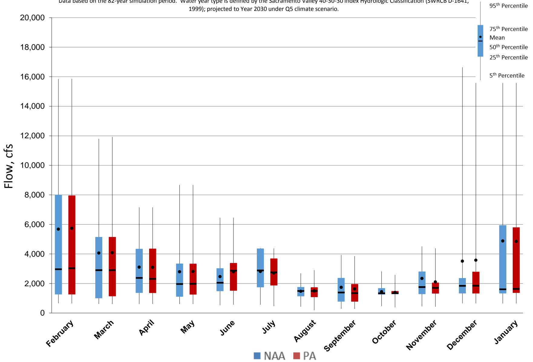
Figure 5.A.6-17-1. Monthly Flow Ranges For American River at Sacramento River Confluence, All Years
