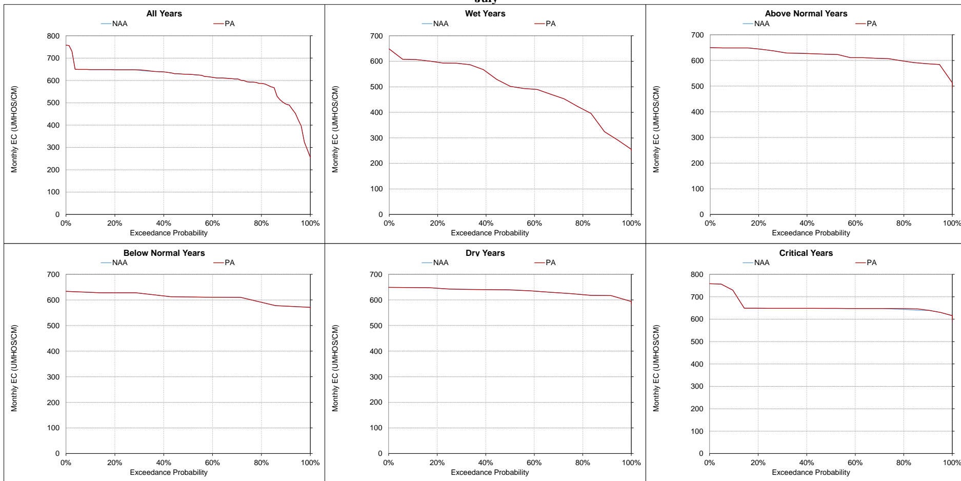
Figure 5.A.6-30-17. San Joaquin River at Vernalis, Monthly EC July
