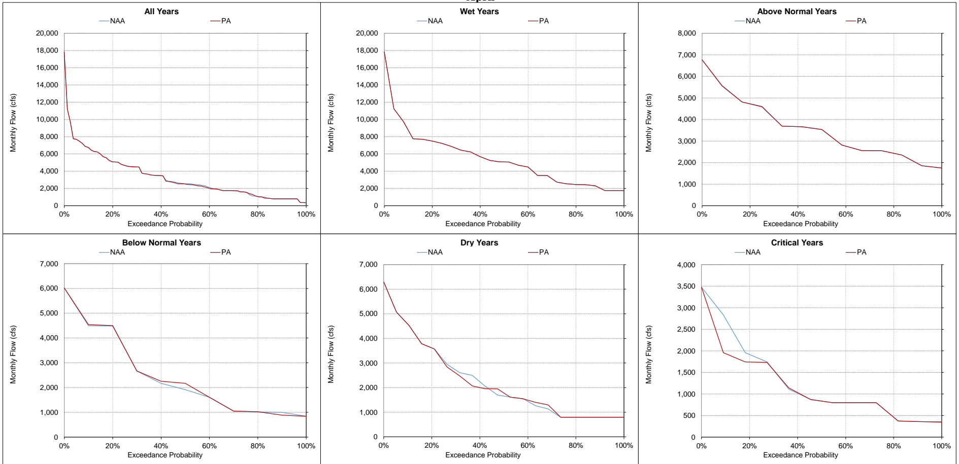
Figure 5.A.6-16-14. American River below Nimbus Dam, Monthly Flow April
