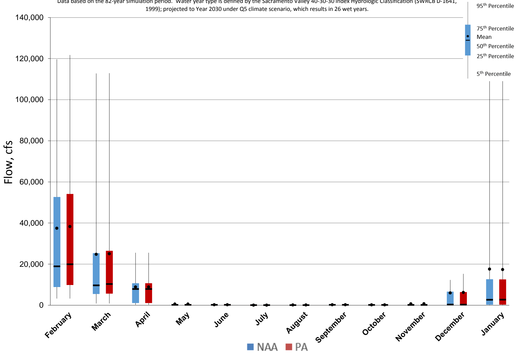
Figure 5.A.6-20-2. Monthly Flow Ranges For Yolo Bypass, Wet Years
