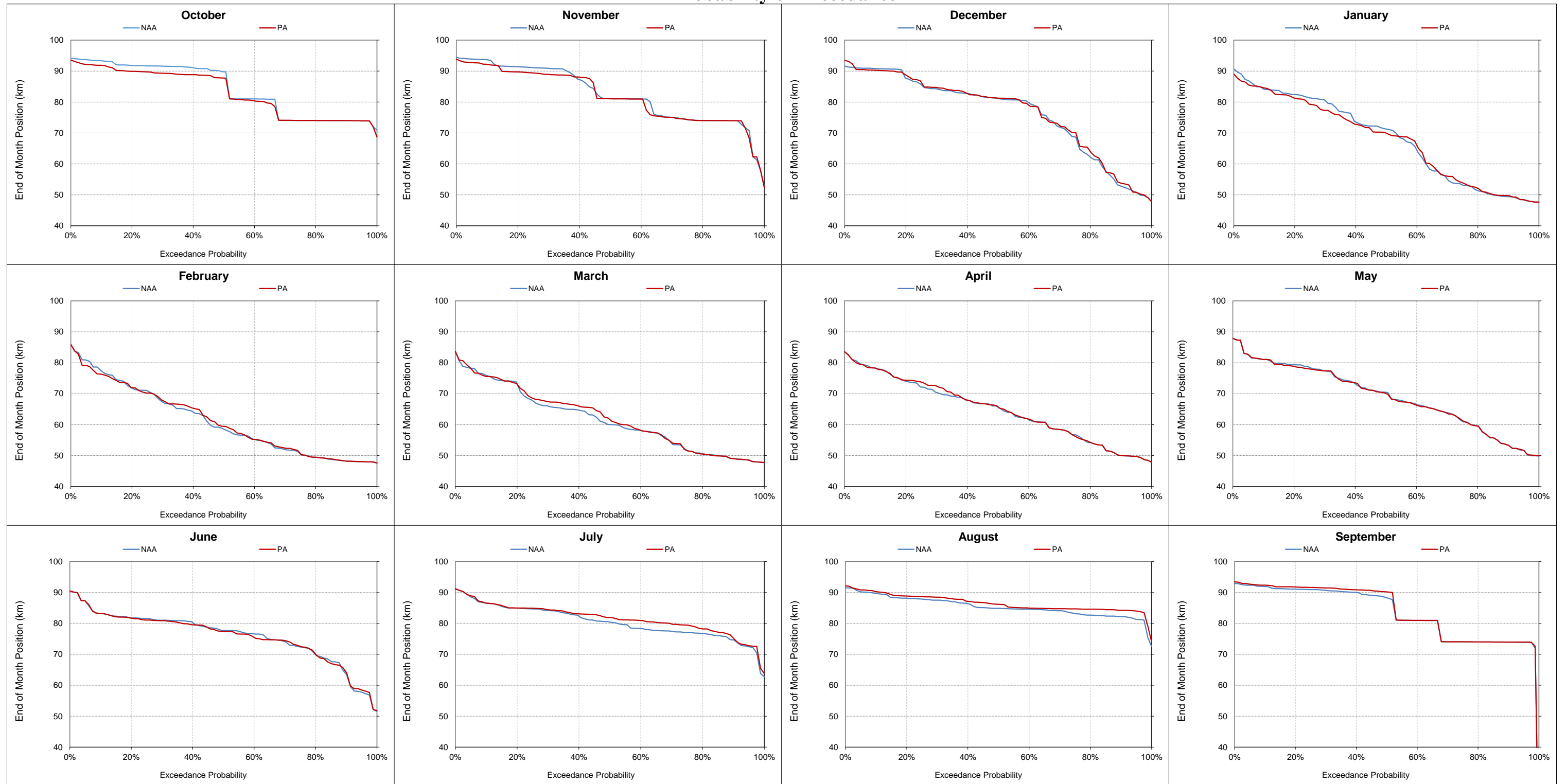
Figure 5.A.6-29-7. X2, End of Month Position Probability of Exceedance
