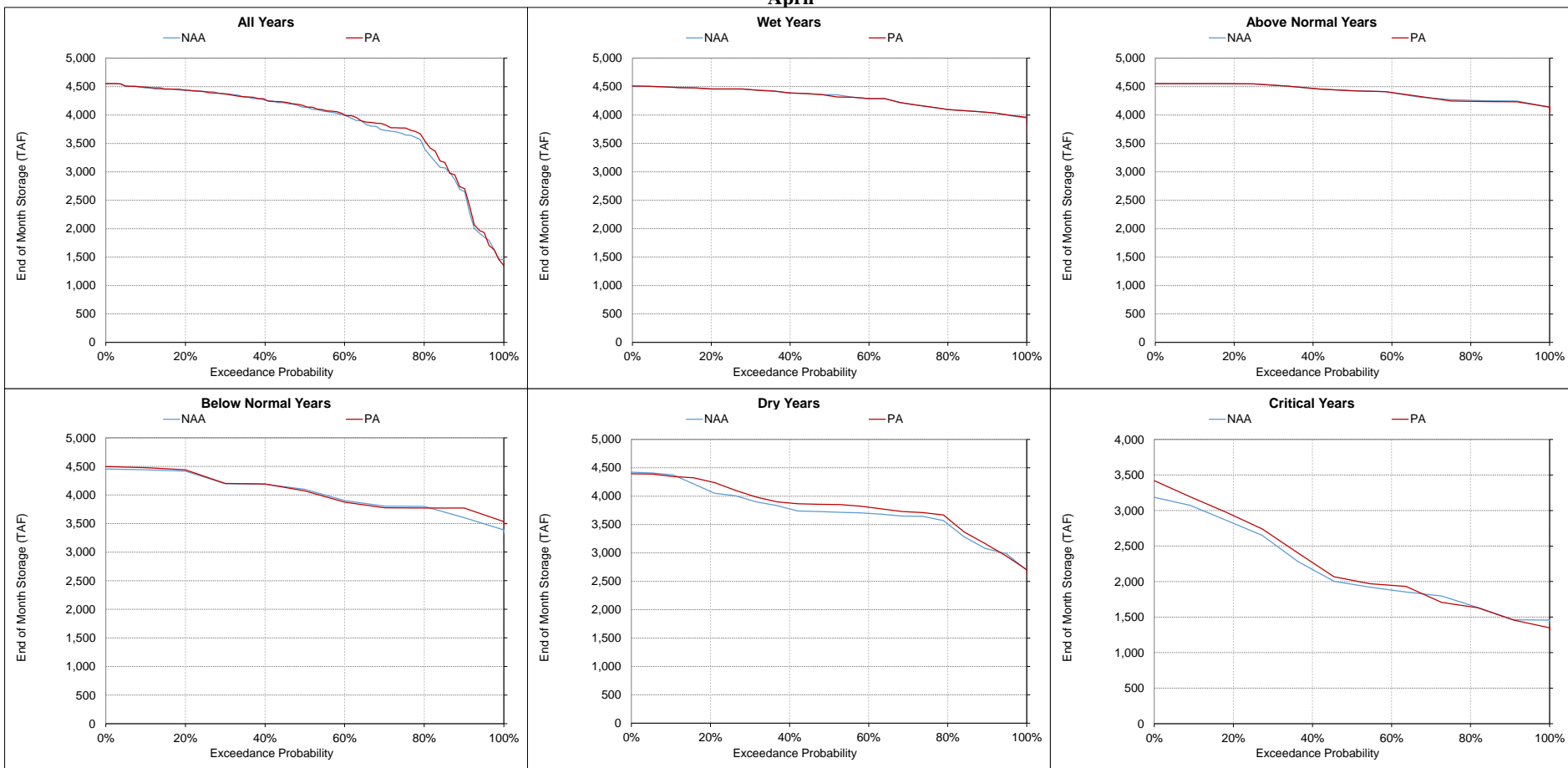
Figure 5.A.6-3-14. Shasta Lake, End of Month Storage April
