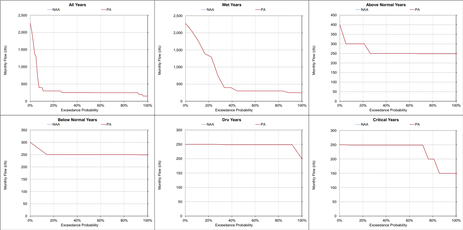
Figure 5.A.6-21-19. Stanislaus River at Ripon, Monthly Flow September
