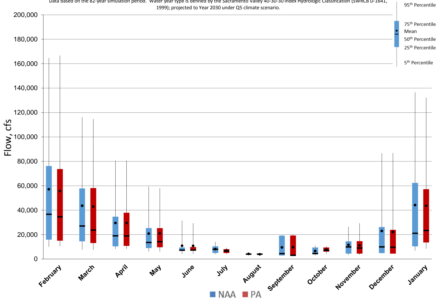
Figure 5.A.6-26-1. Monthly Flow Ranges For Delta Outflow, All Years
