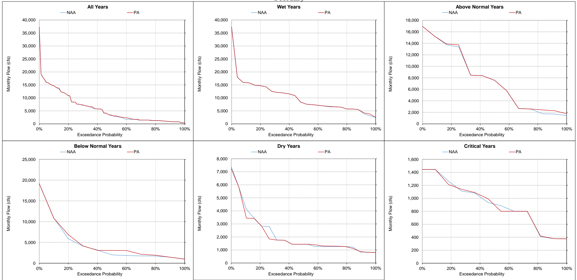
Figure 5.A.6-16-12. American River below Nimbus Dam, Monthly Flow February
