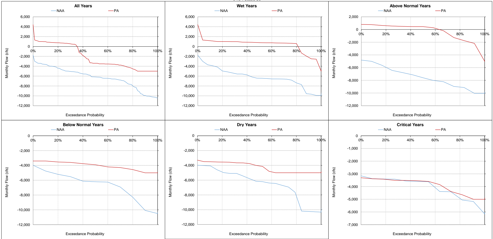
Figure 5.A.6-25-9. Old and Middle River, Monthly Flow November
