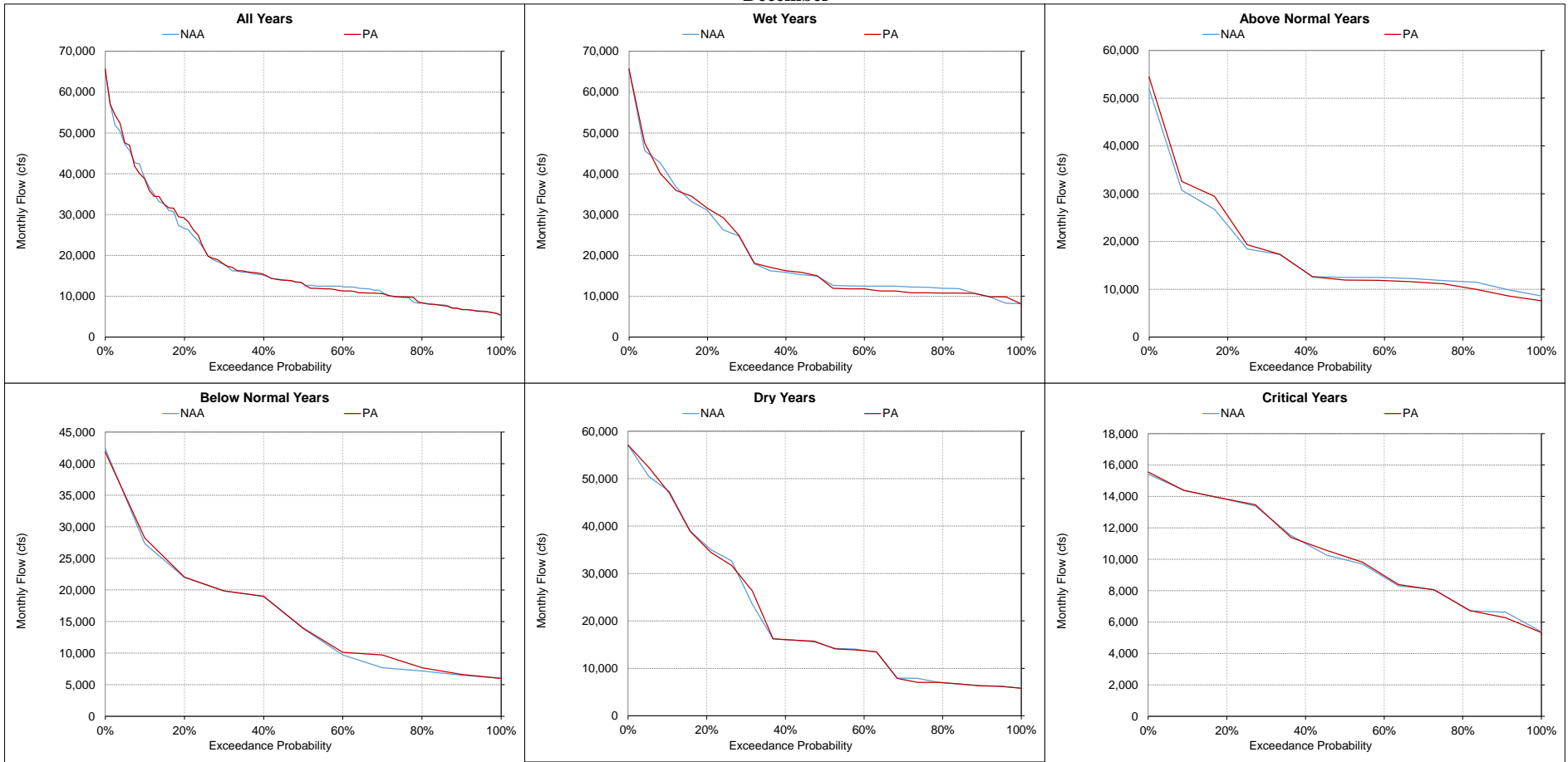
Figure 5.A.6-14-10. Sacramento River at Verona, Monthly Flow December
