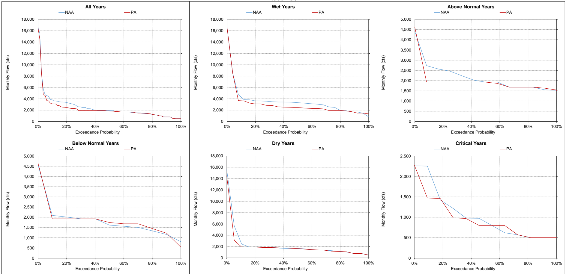
Figure 5.A.6-16-9. American River below Nimbus Dam, Monthly Flow November
