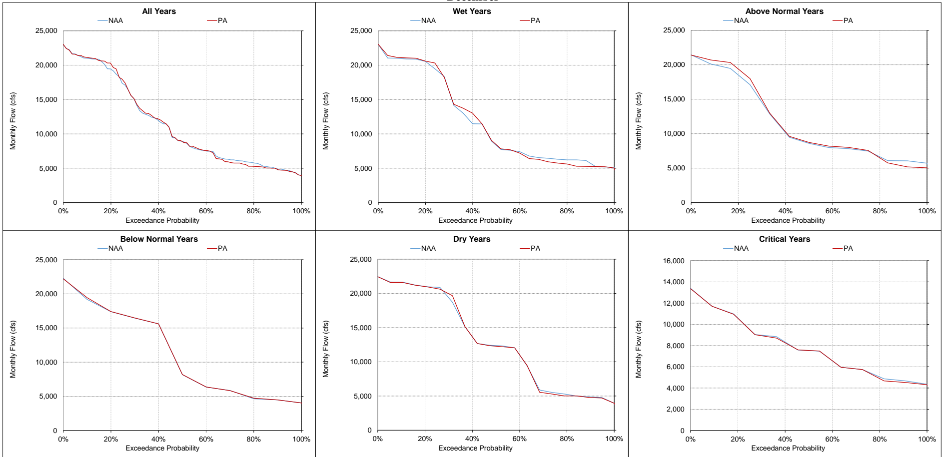
Figure 5.A.6-11-10. Sacramento River at Bend Bridge, Monthly Flow December
