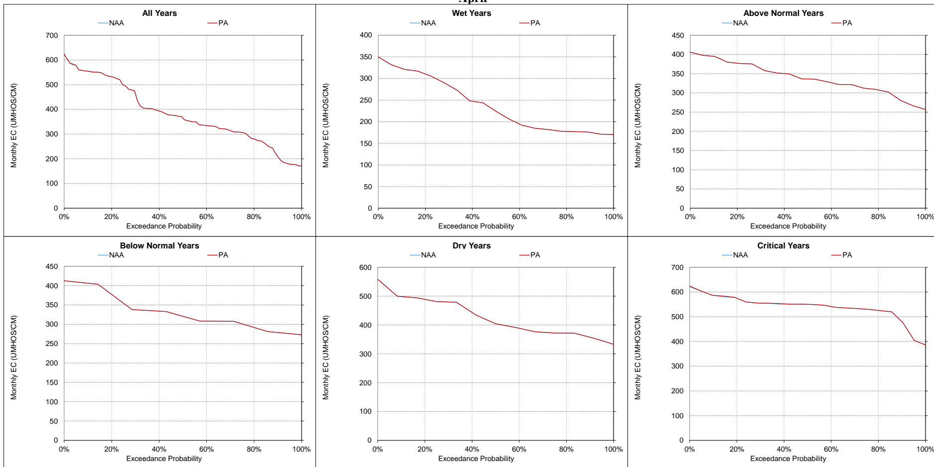
Figure 5.A.6-30-14. San Joaquin River at Vernalis, Monthly EC April
