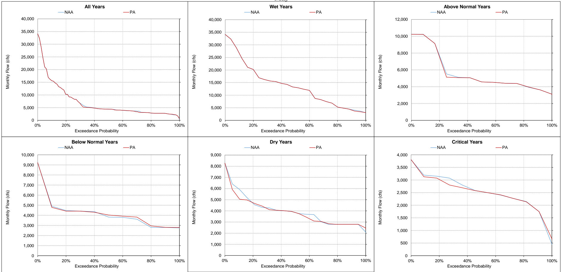
Figure 5.A.6-13-15. Feather River at Sacramento River Confluence, Monthly Flow May
