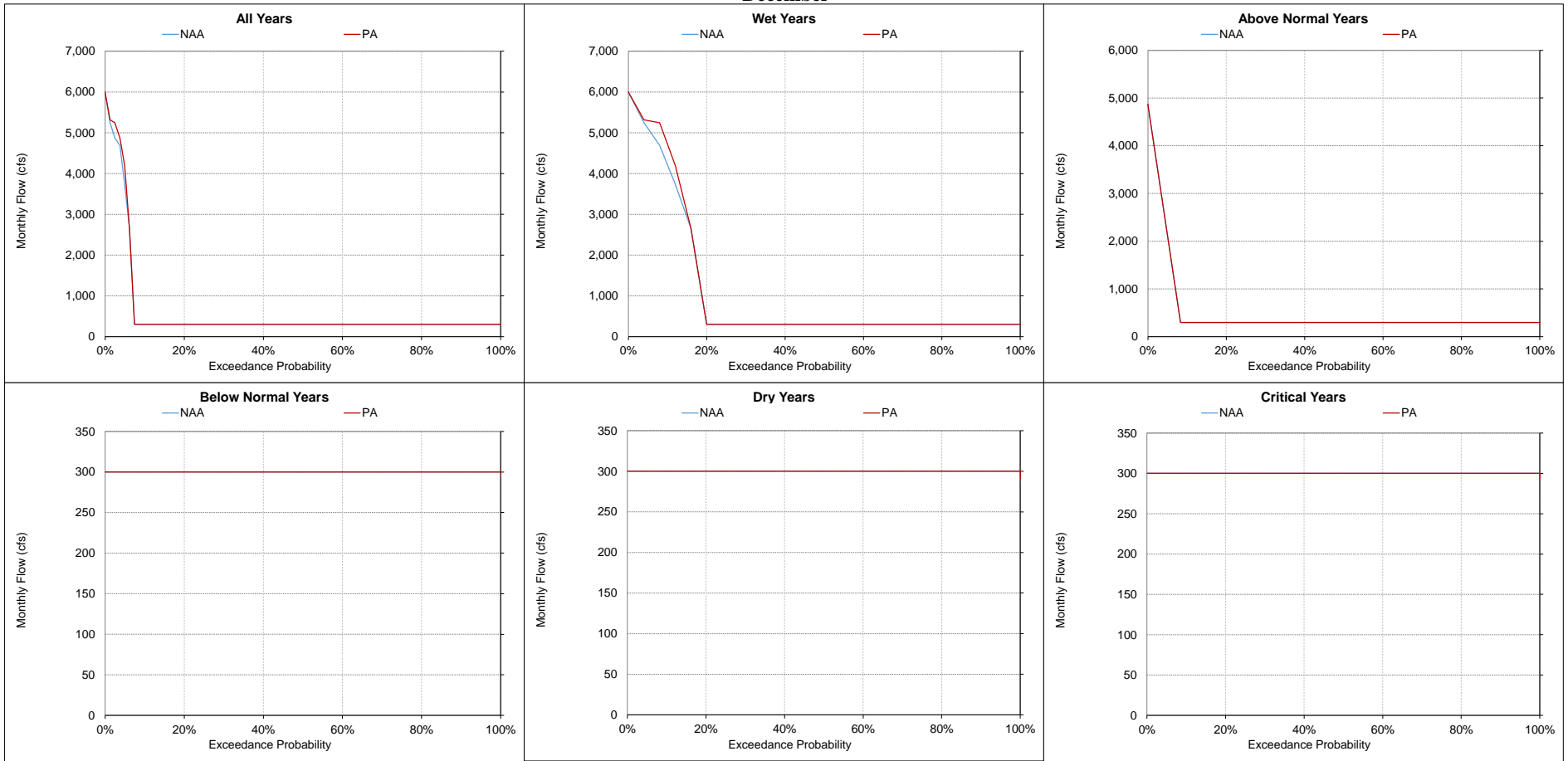
Figure 5.A.6-7-10. Trinity River below Lewiston Dam, Monthly Flow December
