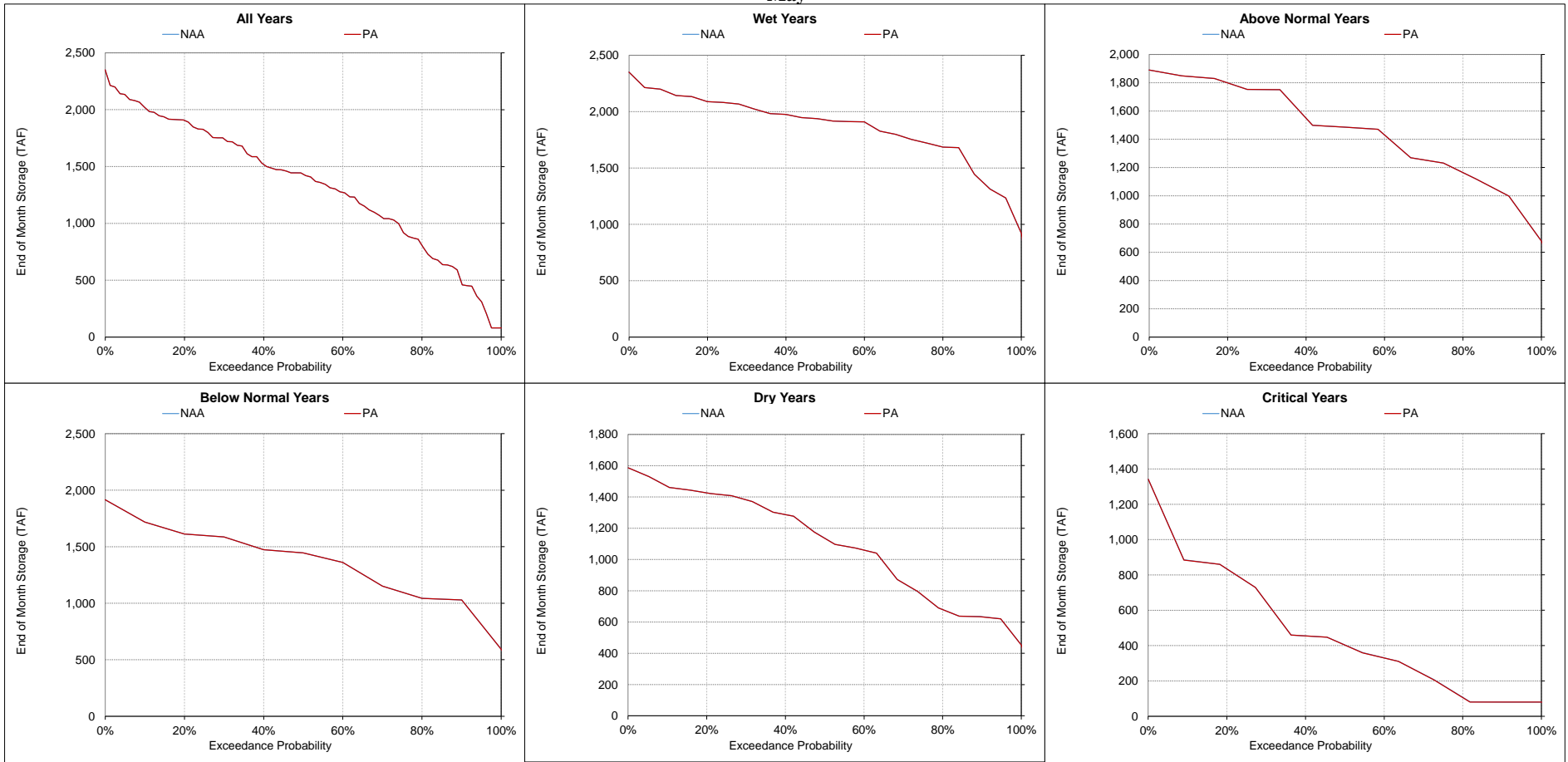
Figure 5.A.6-15. New Melones Lake, End of Month Storage May
