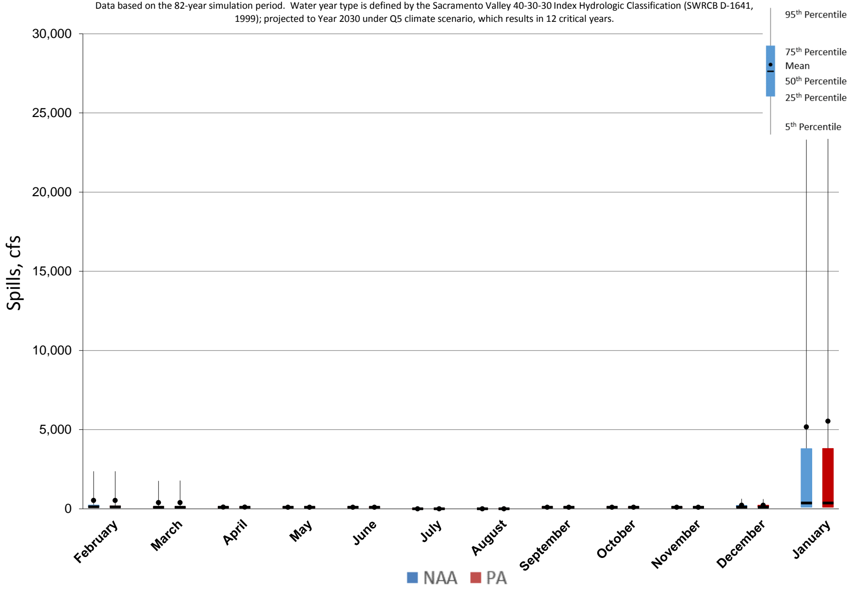
Figure 5.A.6-15-6. Monthly Spills Ranges For Fremont Weir, Critical Years
