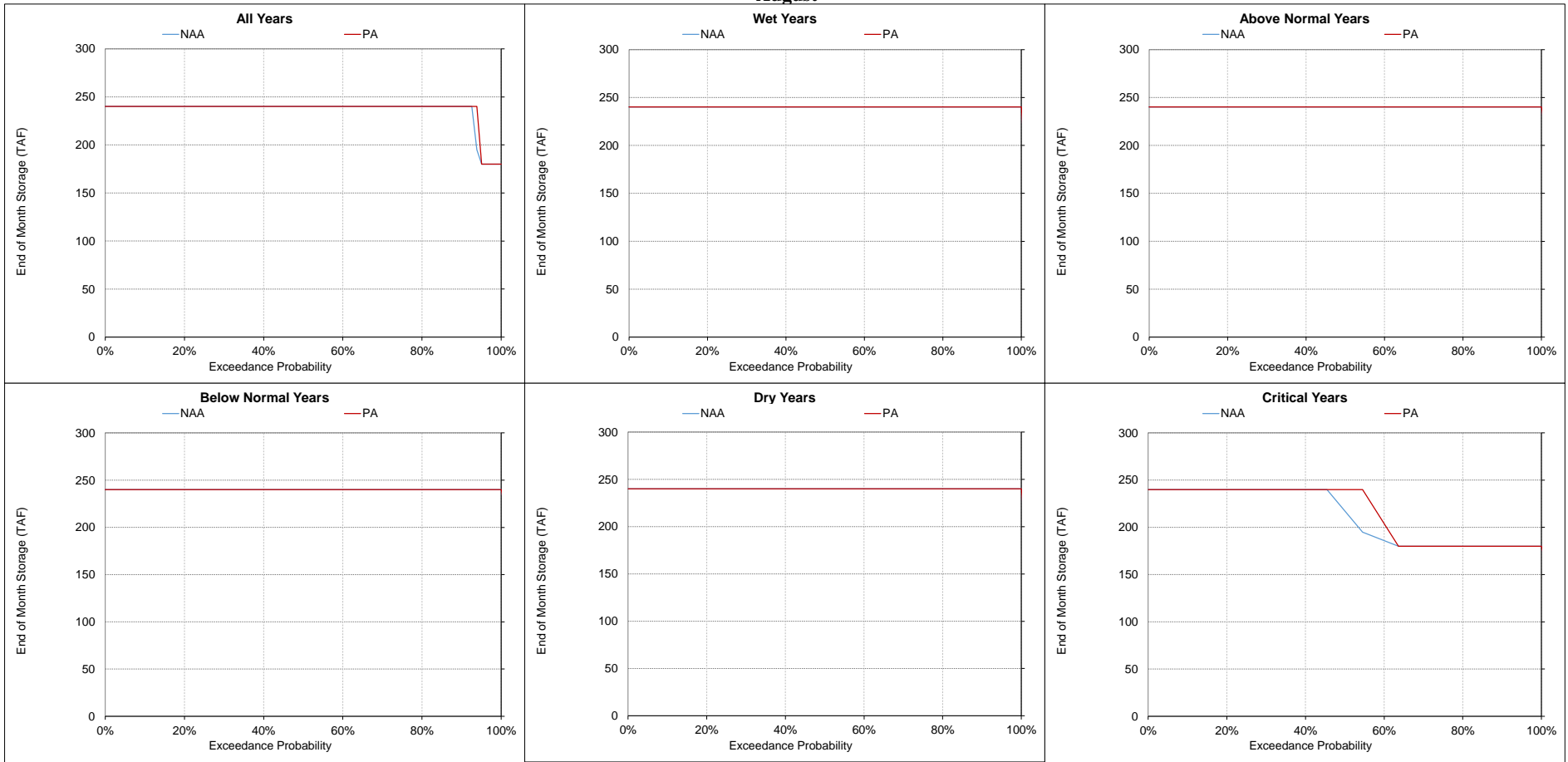
Figure 5.A.6-2-18. Whiskeytown Reservoir, End of Month Storage August
