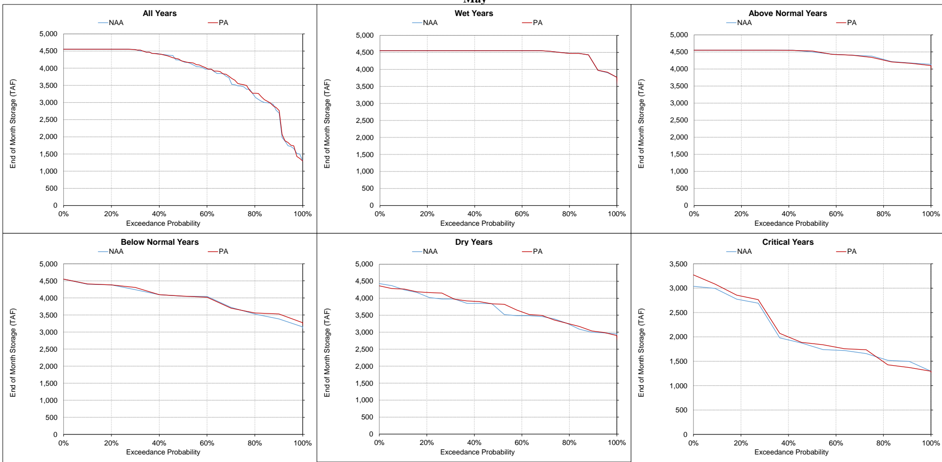
Figure 5.A.6-3-15. Shasta Lake, End of Month Storage May
