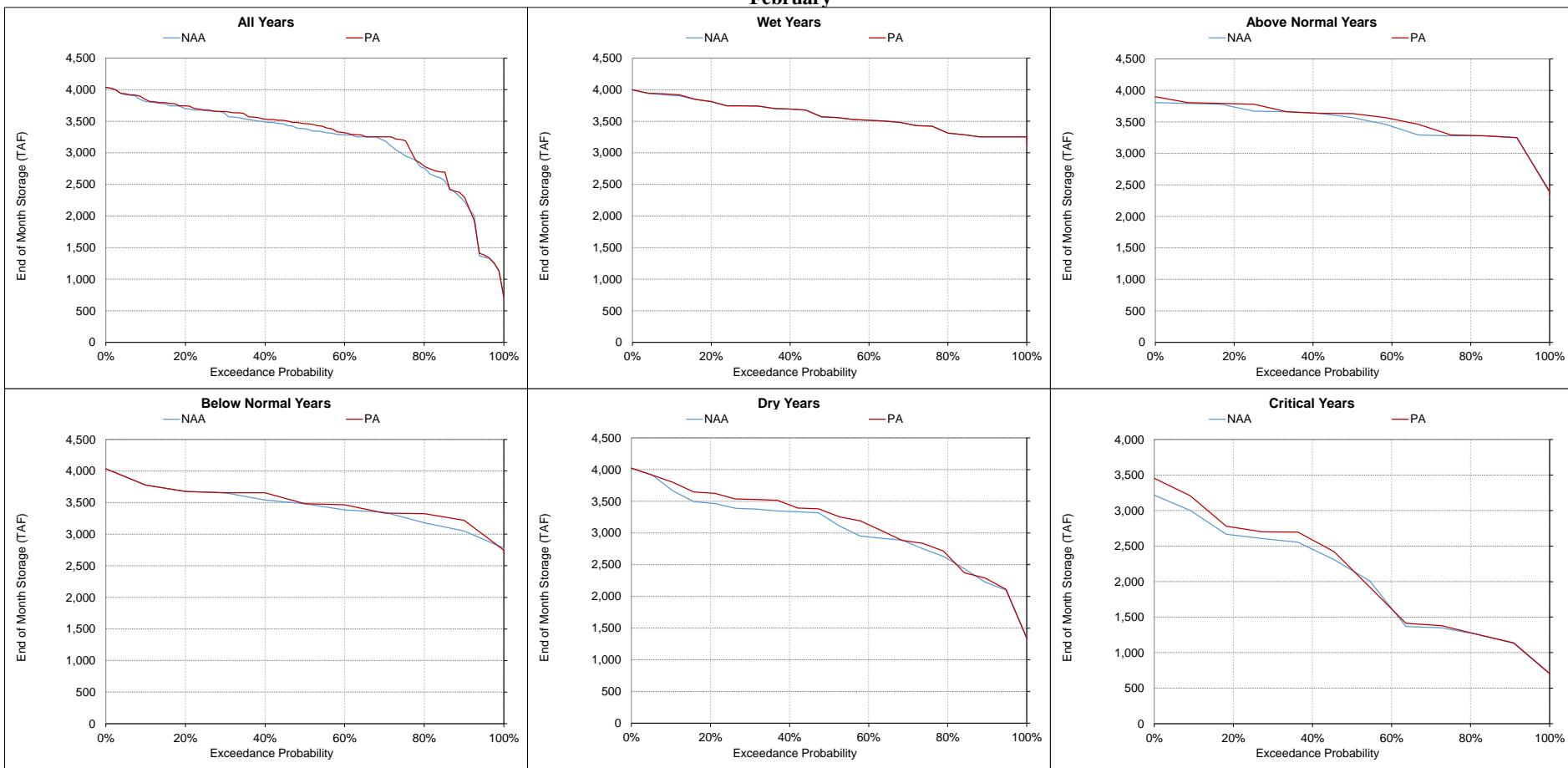
Figure 5.A.6-3-12. Shasta Lake, End of Month Storage February
