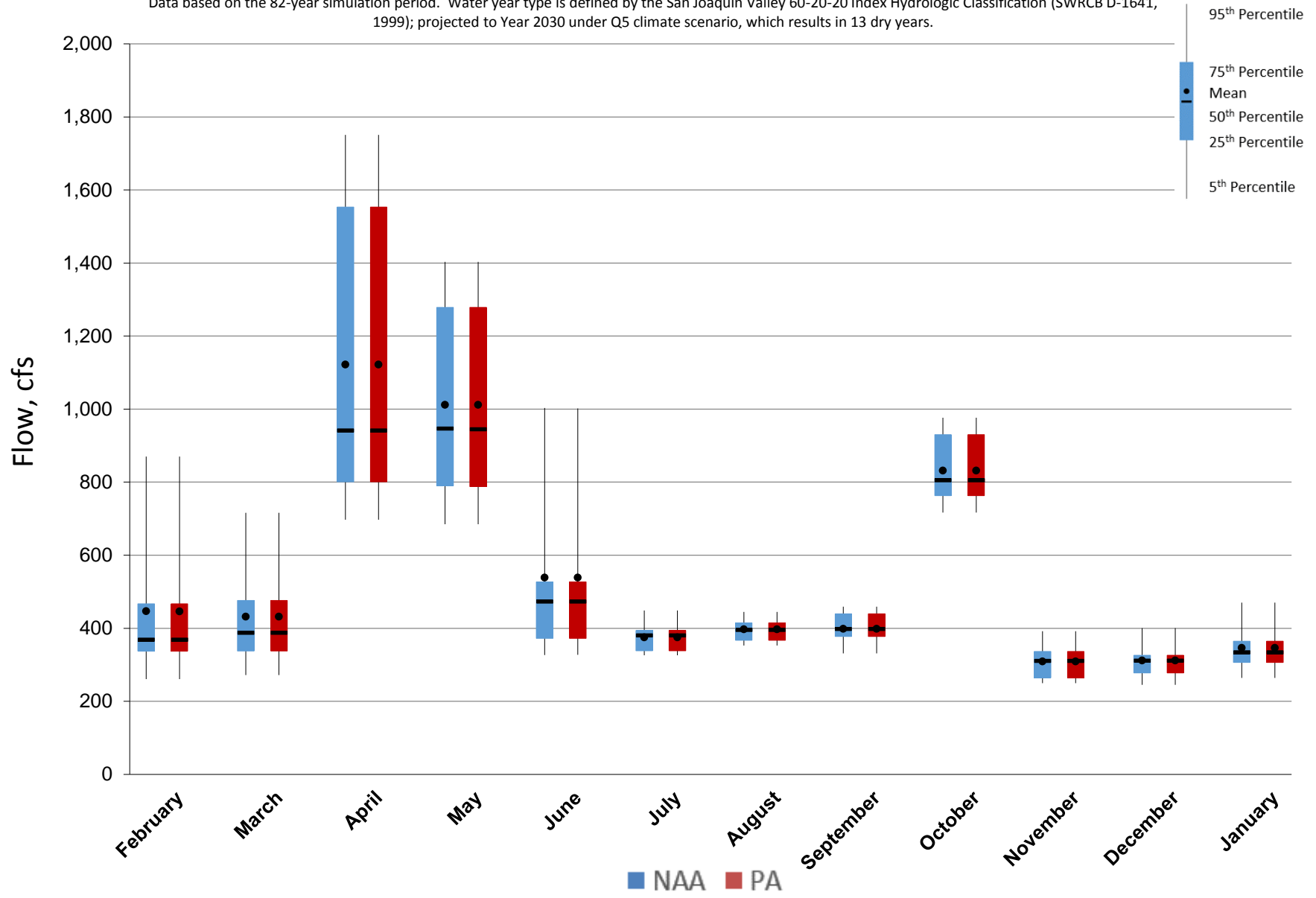
Figure 5.A.6-22-5. Monthly Flow Ranges for Stanislaus River at Mouth, Dry Years
