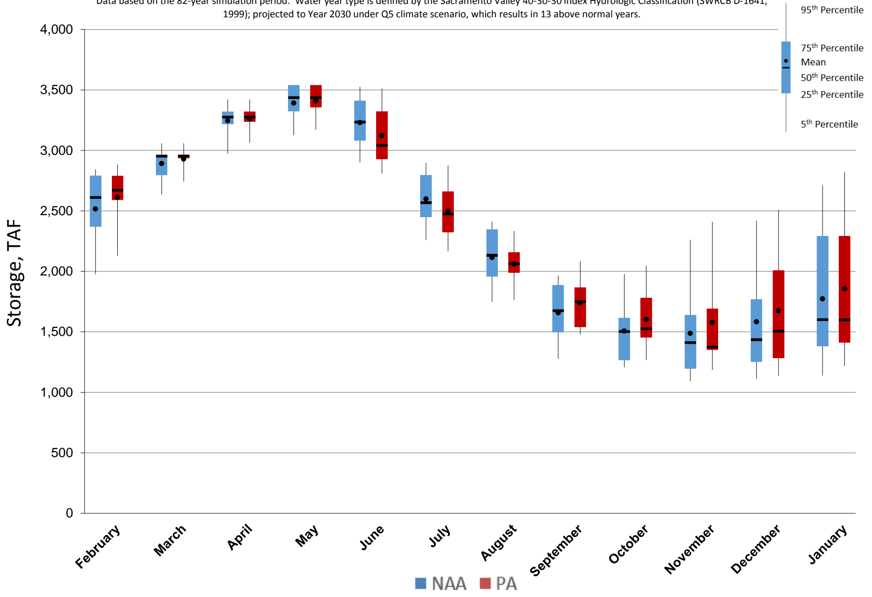
Figure 5.A.6-4-3. End of Month Storage Ranges For Lake Oroville, Above Normal Years
