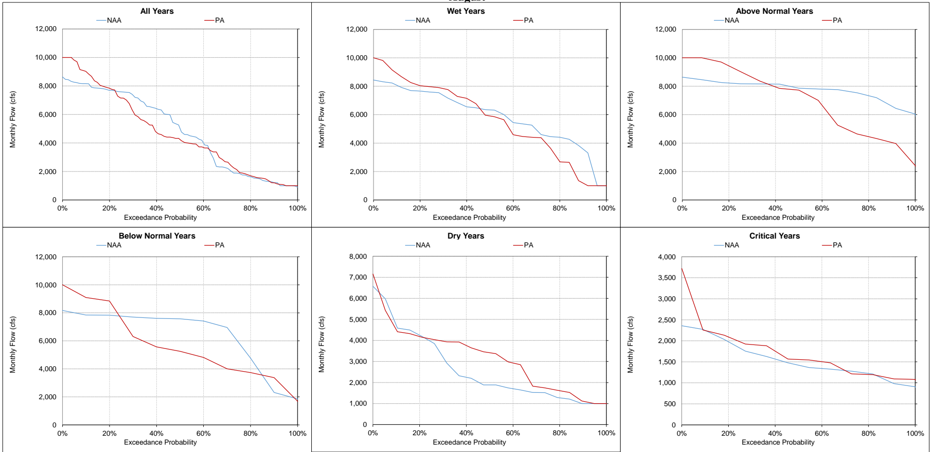
Figure 5.A.6-12-18. Feather River below Thermalito Diversion Dam, Monthly Flow August
