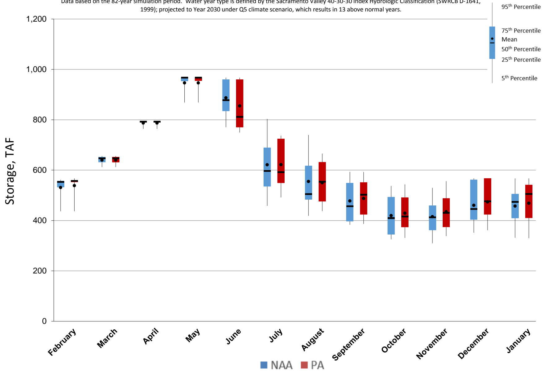
Figure 5.A.6-5-3. End of Month Storage Ranges For Folsom Lake, Above Normal Years
