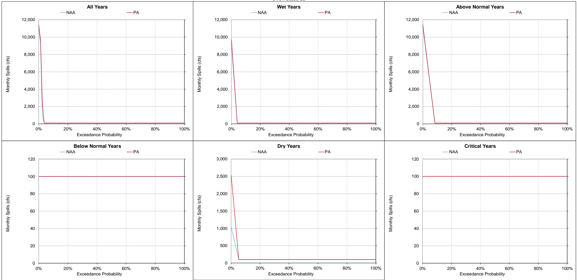
Figure 5.A.6-15-9. Fremont Weir, Monthly Spills November
