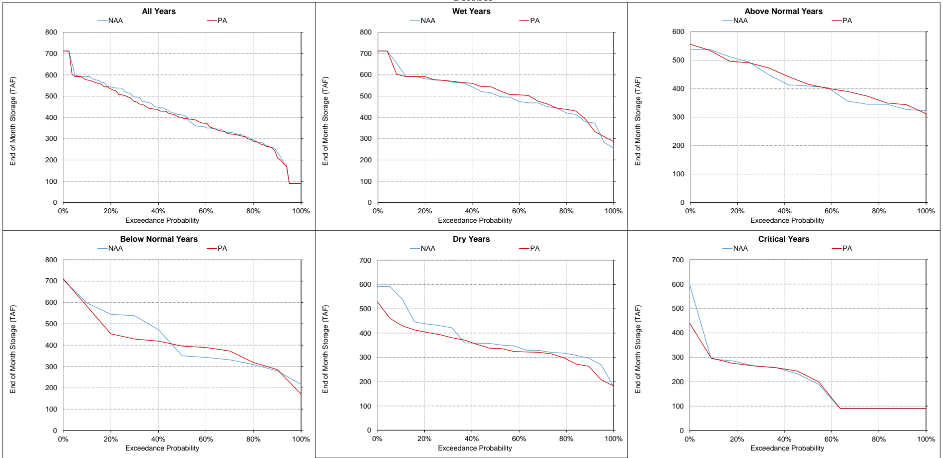
Figure 5.A.6-5-8. Folsom Lake, End of Month Storage October
