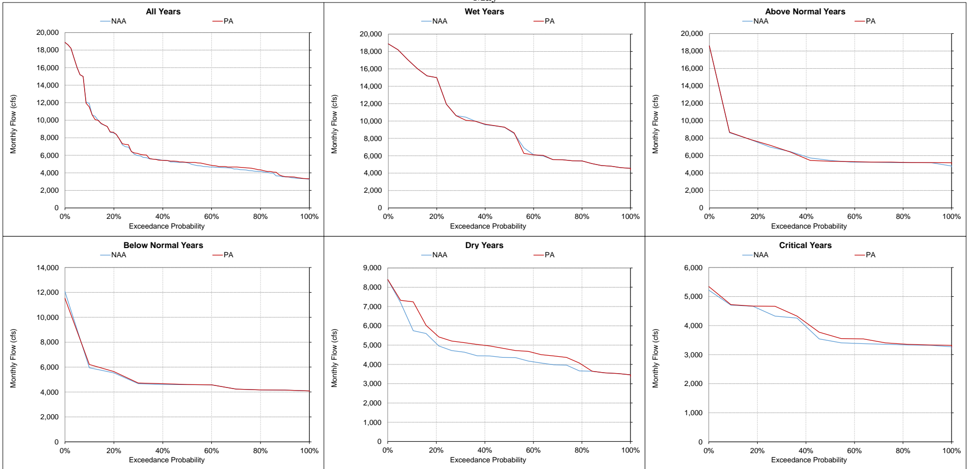
Figure 5.A.6-11-15. Sacramento River at Bend Bridge, Monthly Flow May
