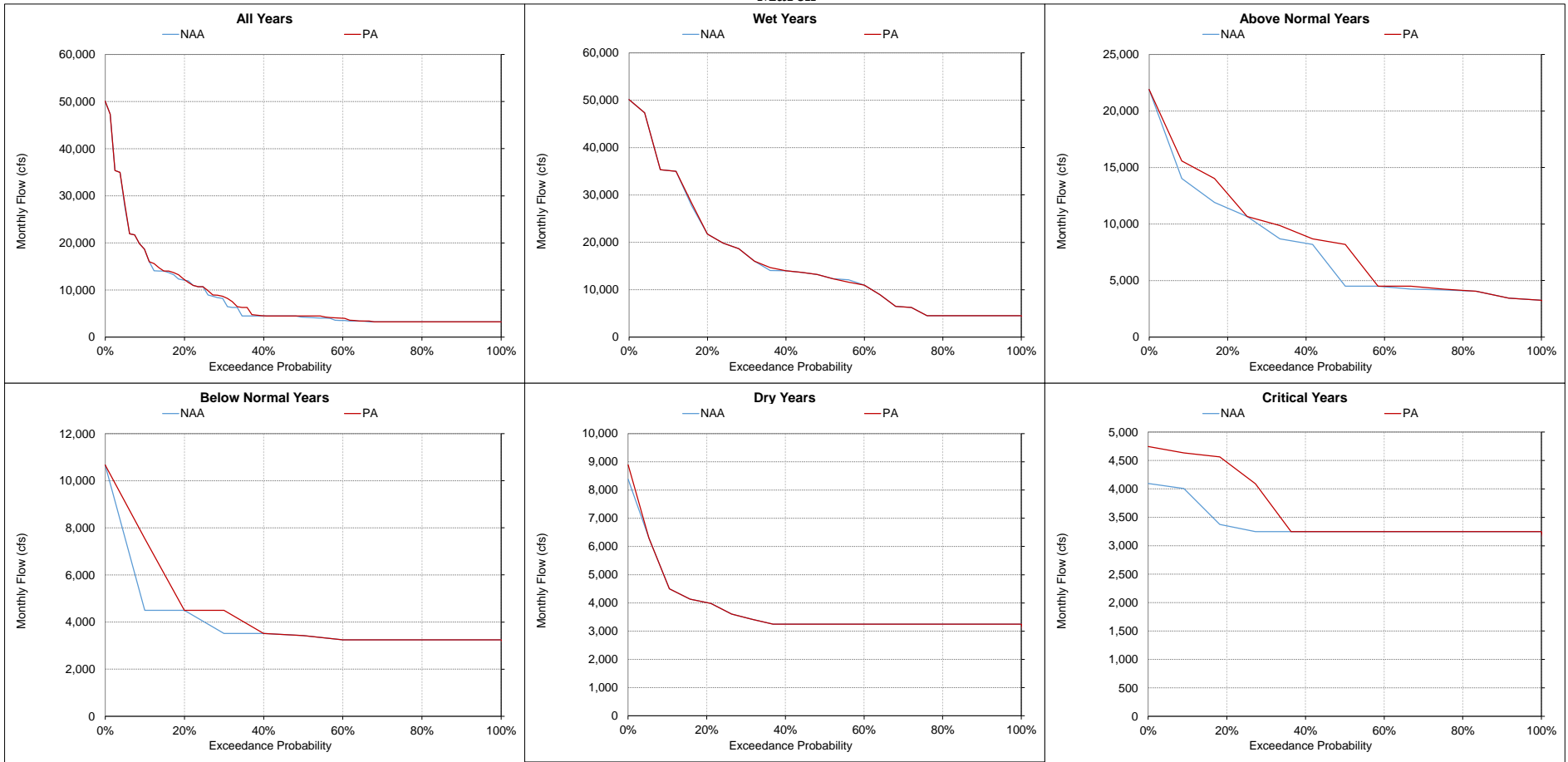
Figure 5.A.6-10-13. Sacramento River below Keswick Dam, Monthly Flow March
