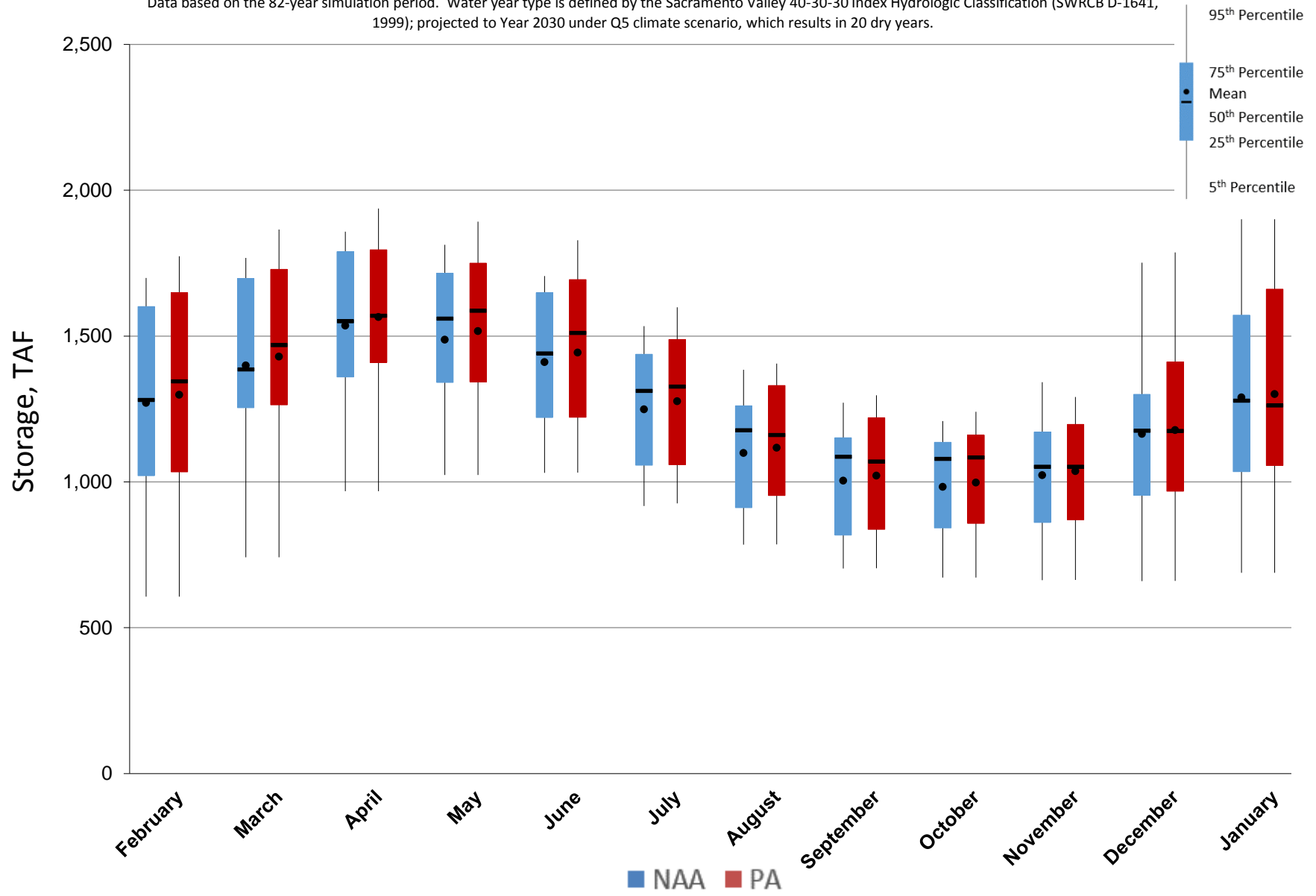
Figure 5.A.6-1-5. End of Month Storage Ranges For Trinity Lake, Dry Years
