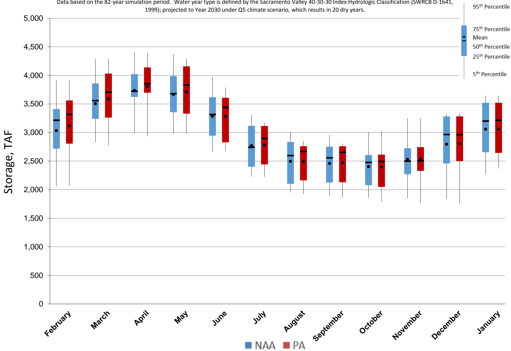
Figure 5.A.6-3-5. End of Month Storage Ranges For Shasta Lake, Dry Years
