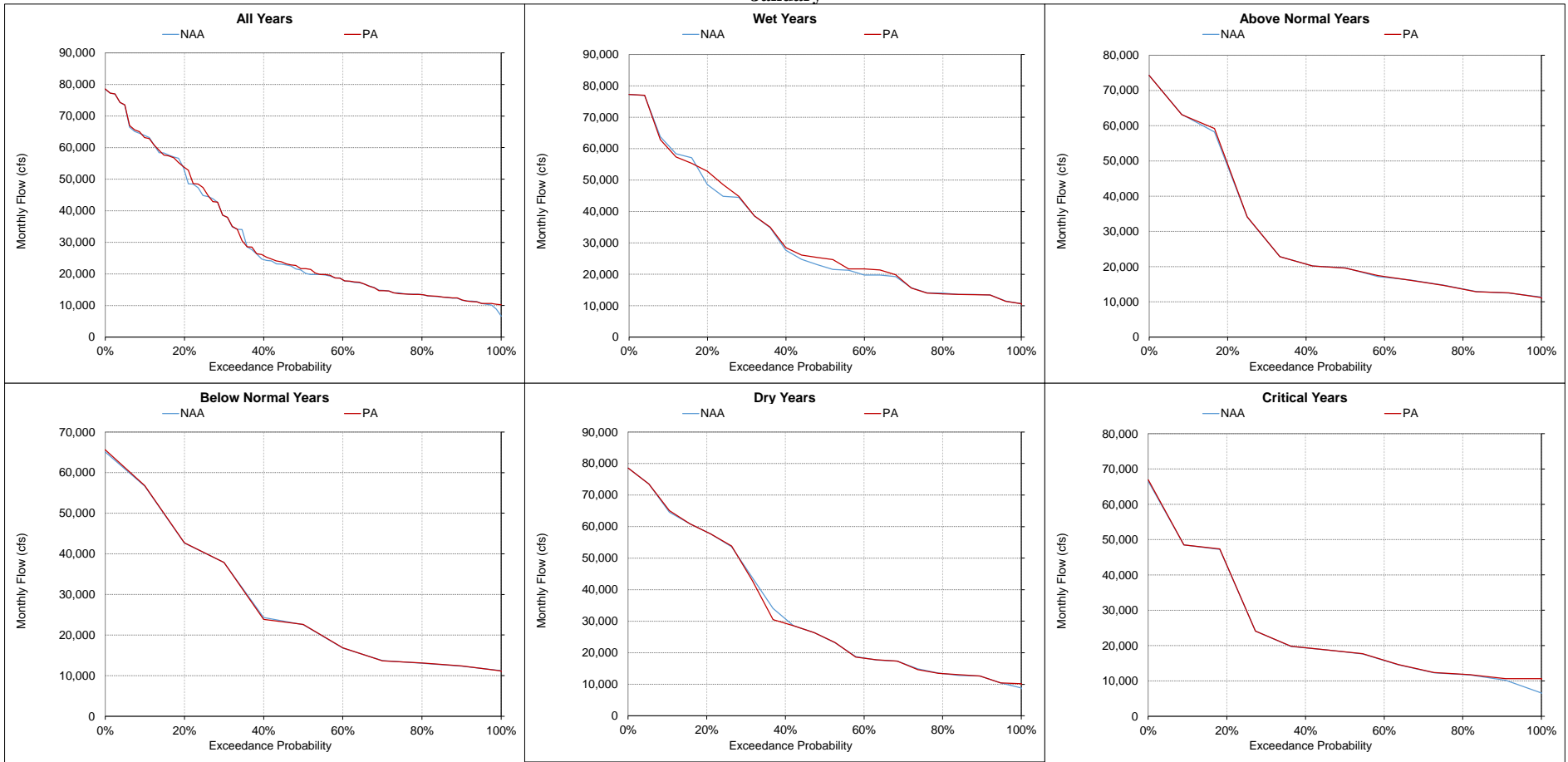
Figure 5.A.6-18-11. Sacramento River at Freeport, Monthly Flow January
