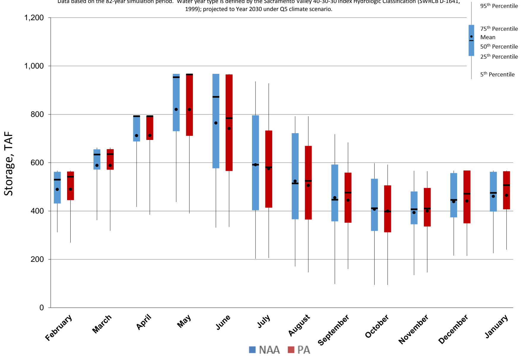
Figure 5.A.6-5-1. End of Month Storage Ranges For Folsom Lake, All Years
