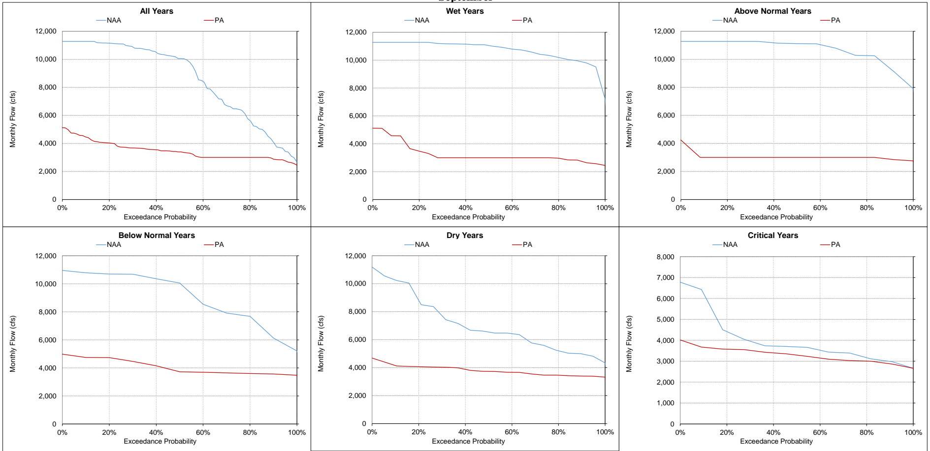
Figure 5.A.6-27-19. South Delta Exports, Monthly Flow September
