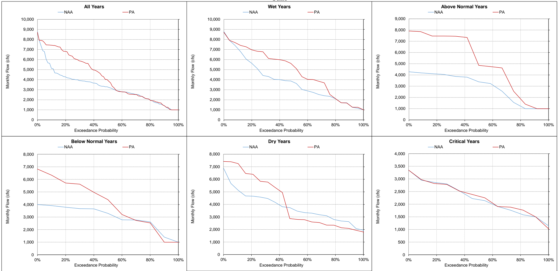
Figure 5.A.6-12-16. Feather River below Thermalito Diversion Dam, Monthly Flow June
