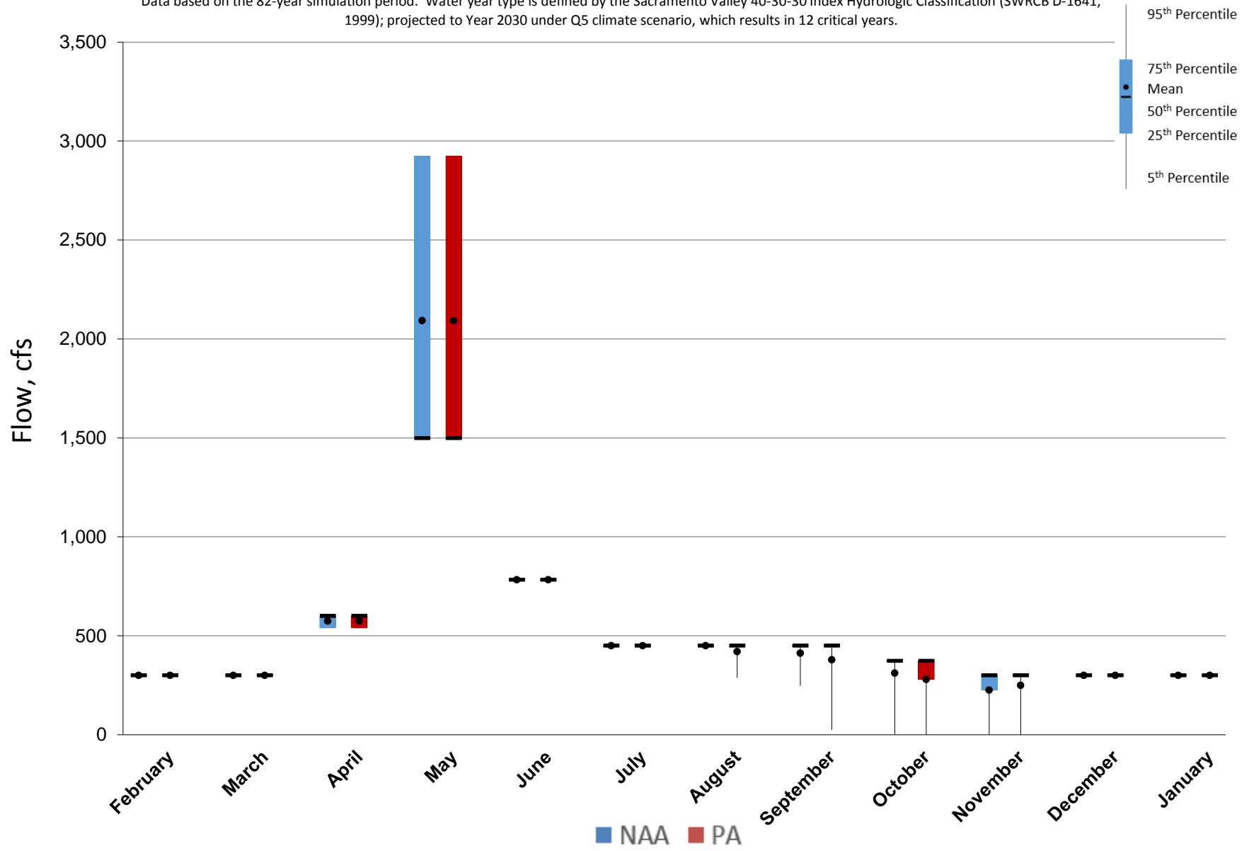
Figure 5.A.6-7-6. Monthly Flow Ranges For Trinity River below Lewiston Dam, Critical Years
