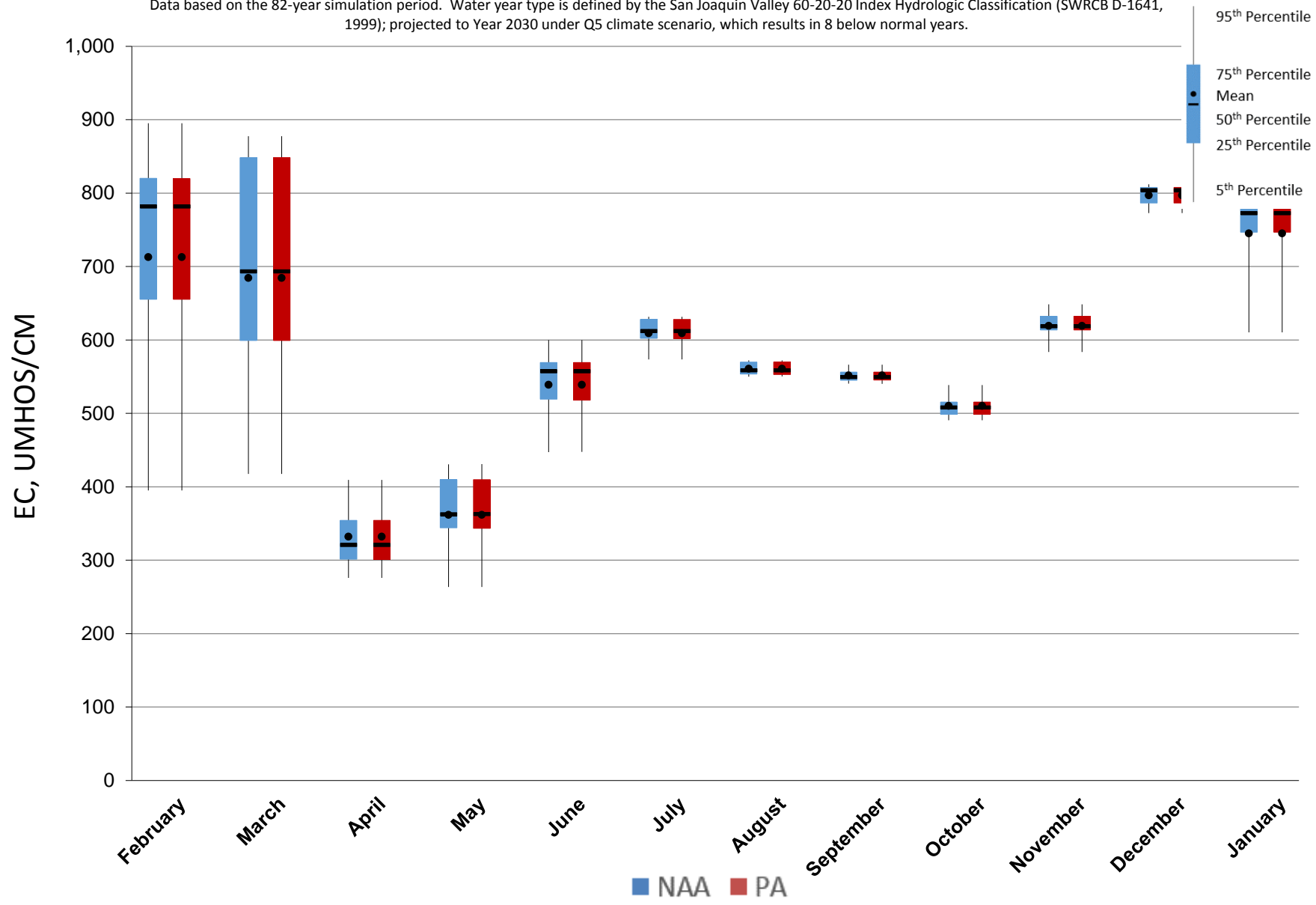
Figure 5.A.6-30-4. Monthly EC Ranges for San Joaquin River at Vernalis, Below Normal Years
