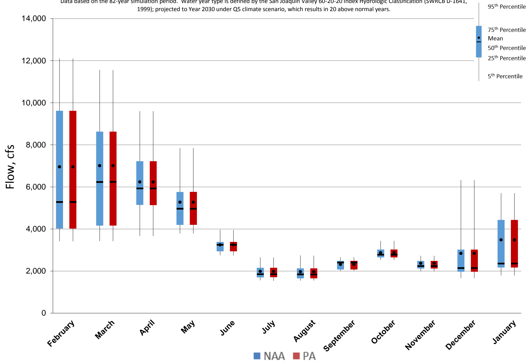
Figure 5.A.6-23-3. Monthly Flow Ranges for San Joaquin River at Vernalis, Above Normal Years
