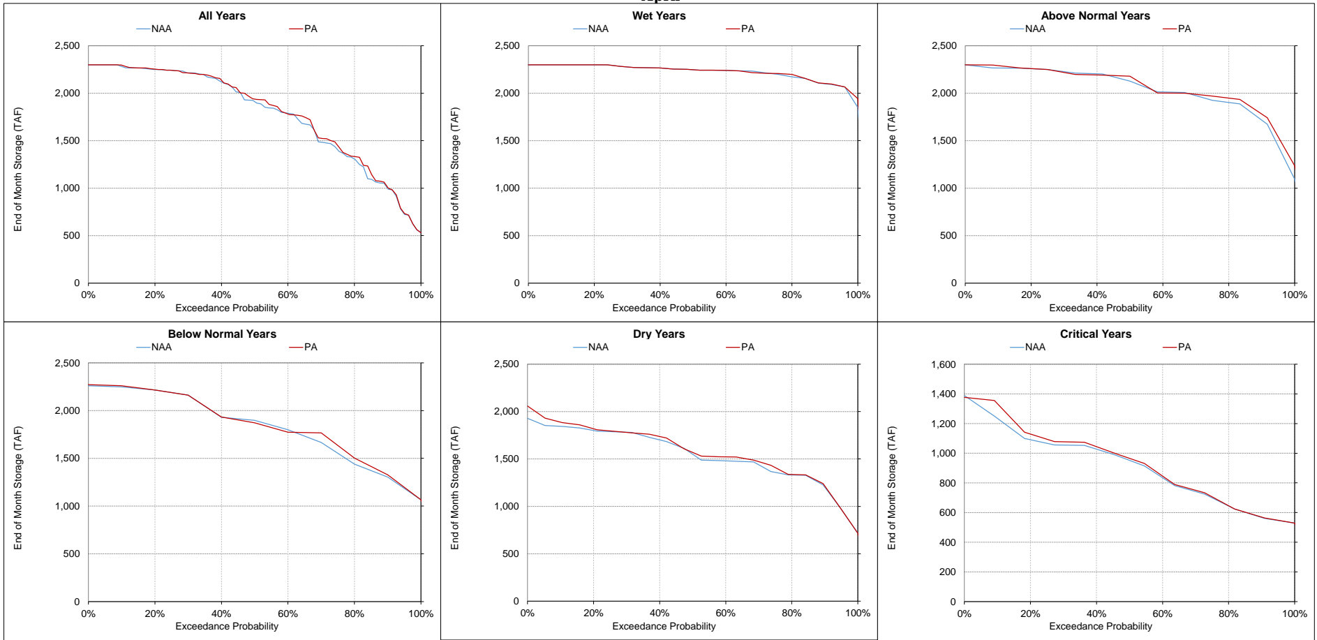
Figure 5.A.6-1-14. Trinity Lake, End of Month Storage April
