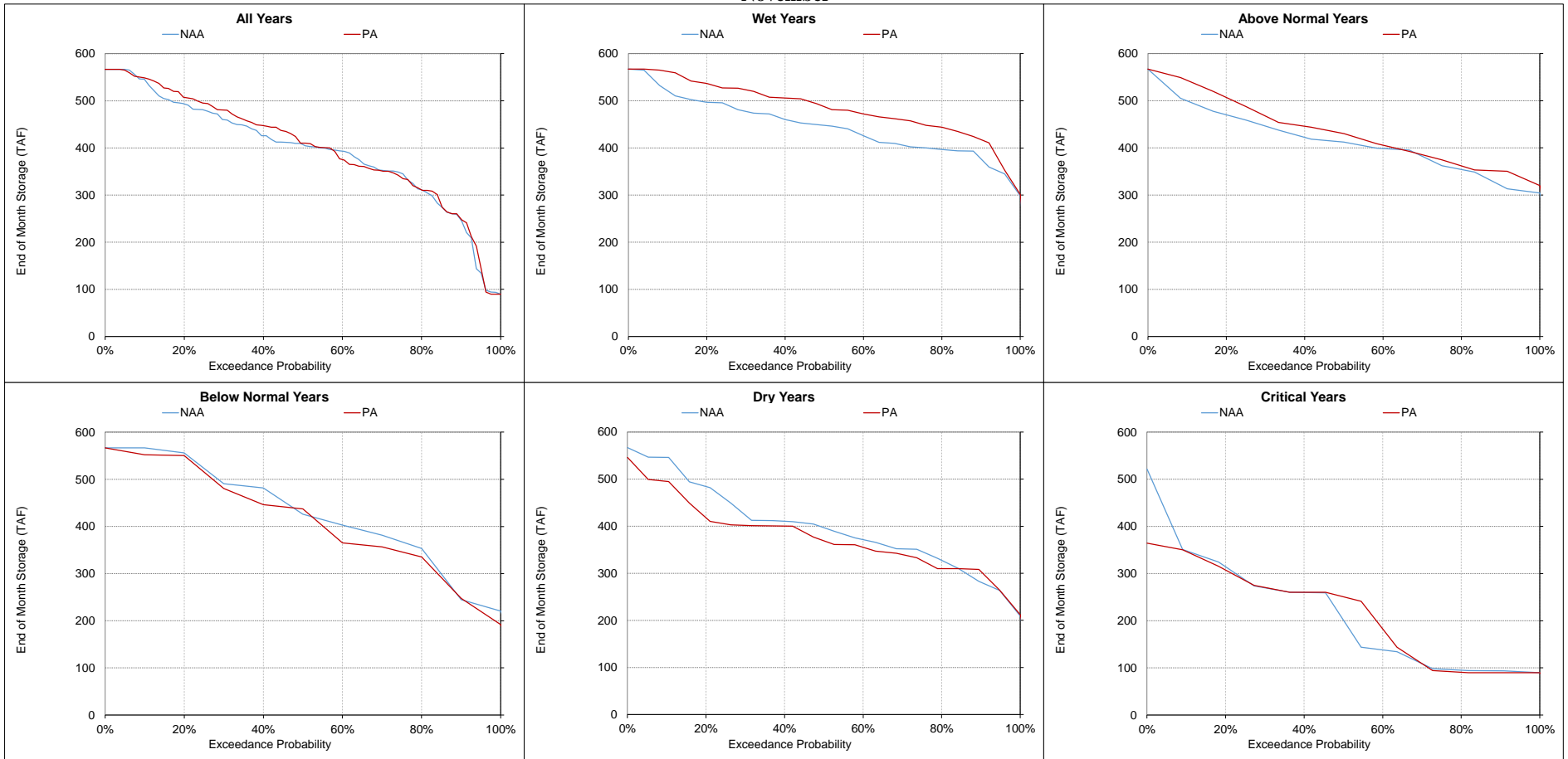
Figure 5.A.6-5-9. Folsom Lake, End of Month Storage November
