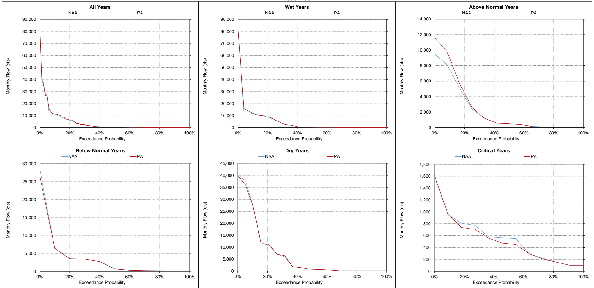
Figure 5.A.6-20-10. Yolo Bypass, Monthly Flow December
