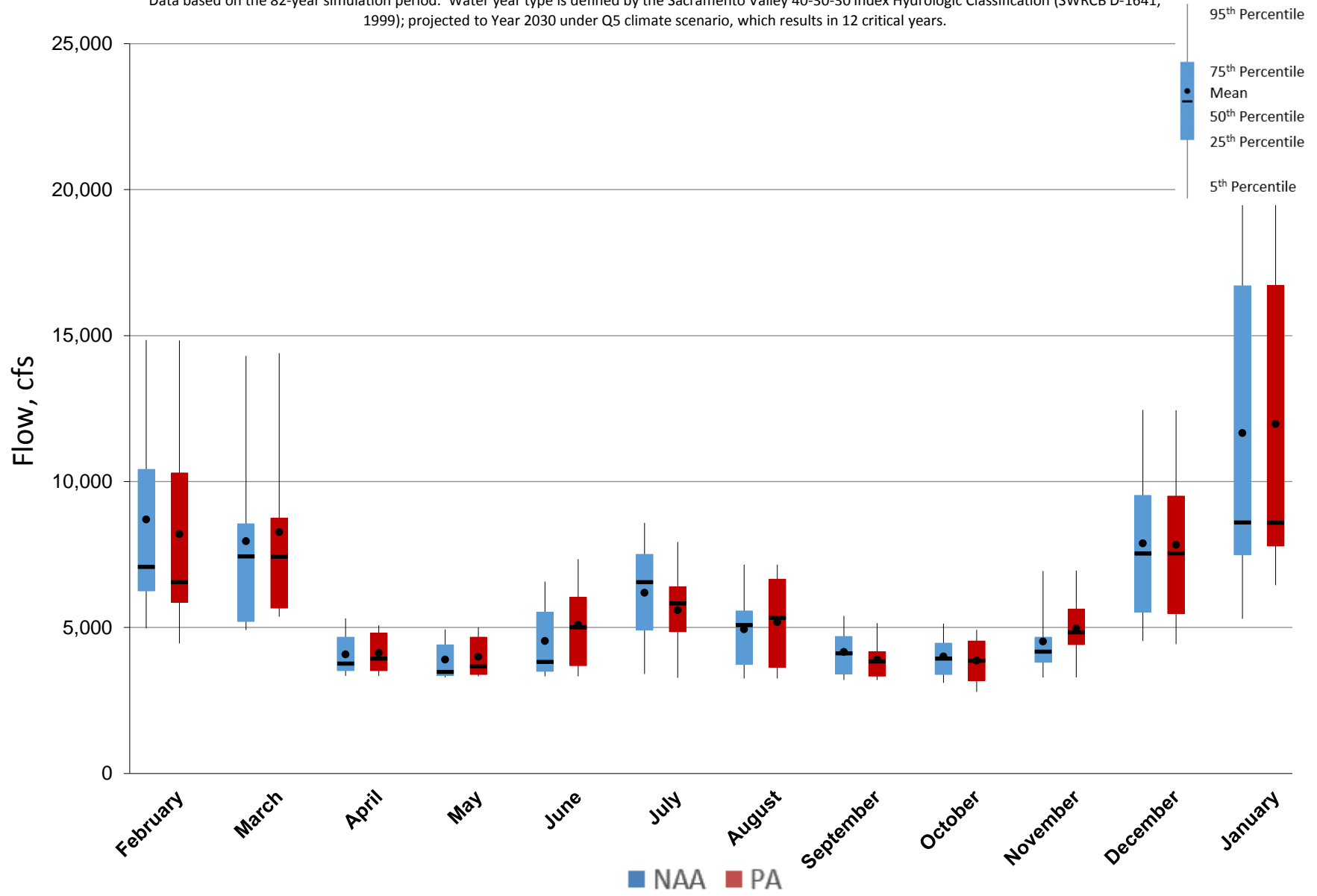
Figure 5.A.6-11-6. Monthly Flow Ranges For Sacramento River at Bend Bridge, Critical Years
