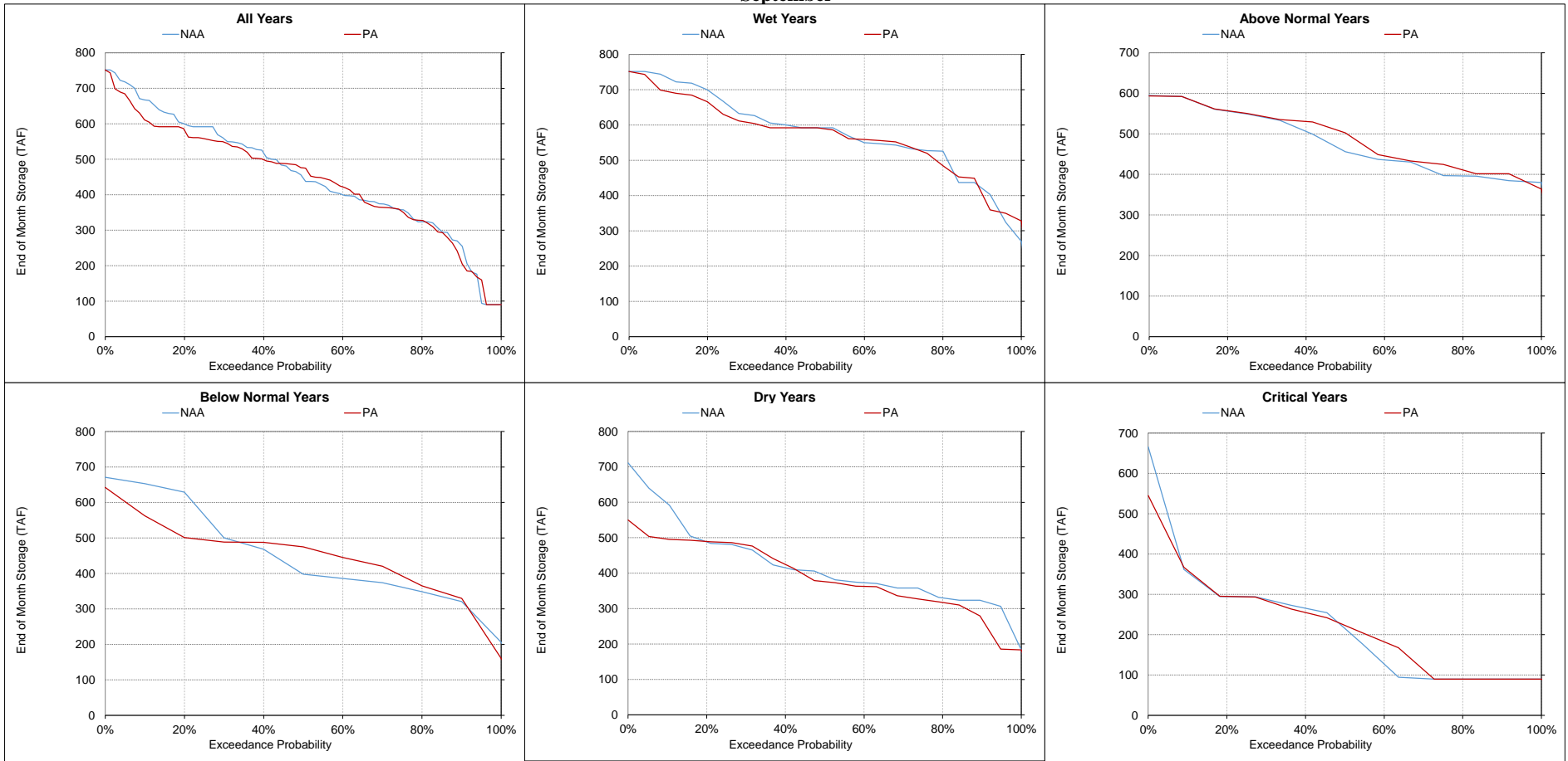
Figure 5.A.6-5-19. Folsom Lake, End of Month Storage September
