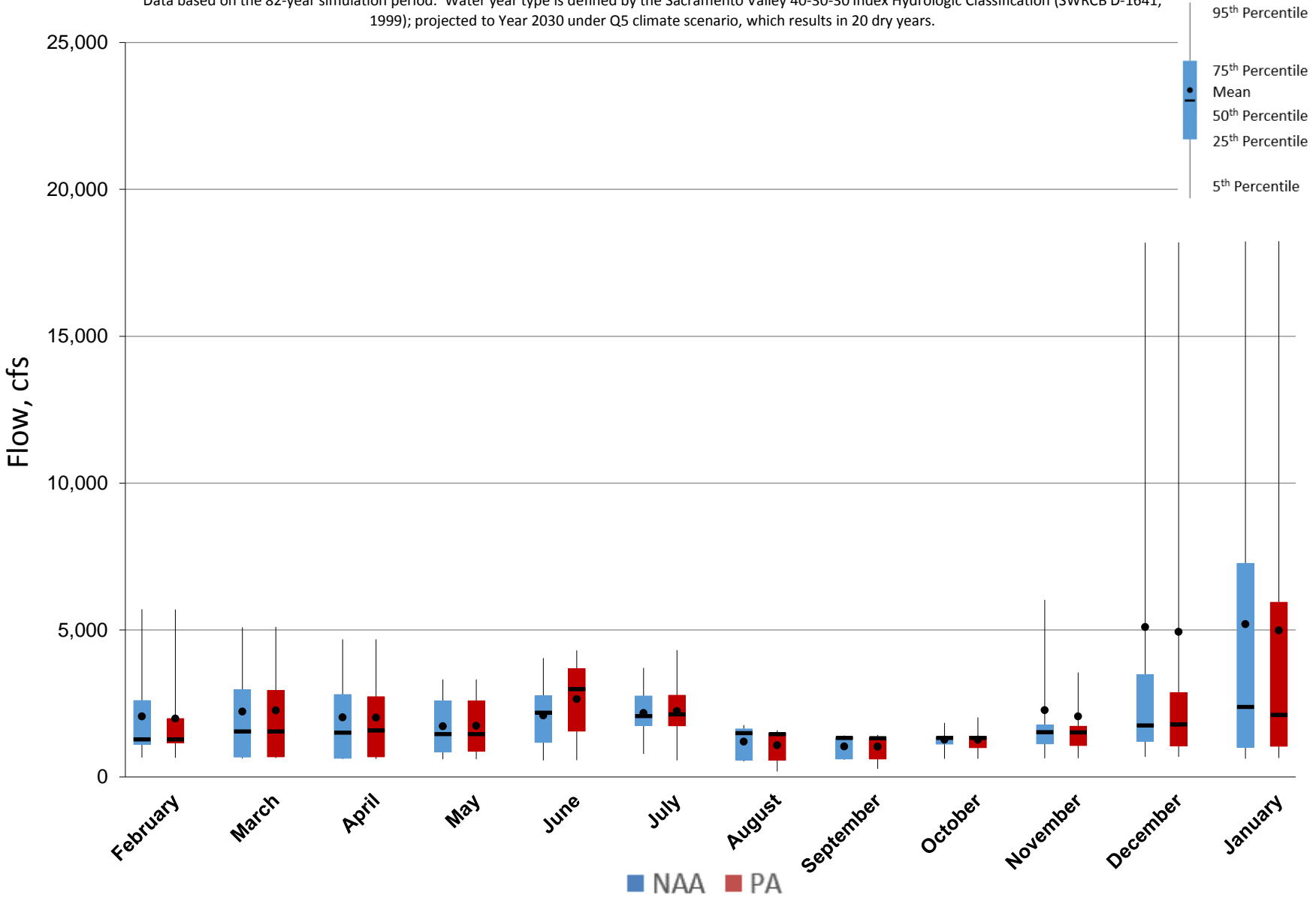
Figure 5.A.6-17-5. Monthly Flow Ranges For American River at Sacramento River Confluence, Dry Years
