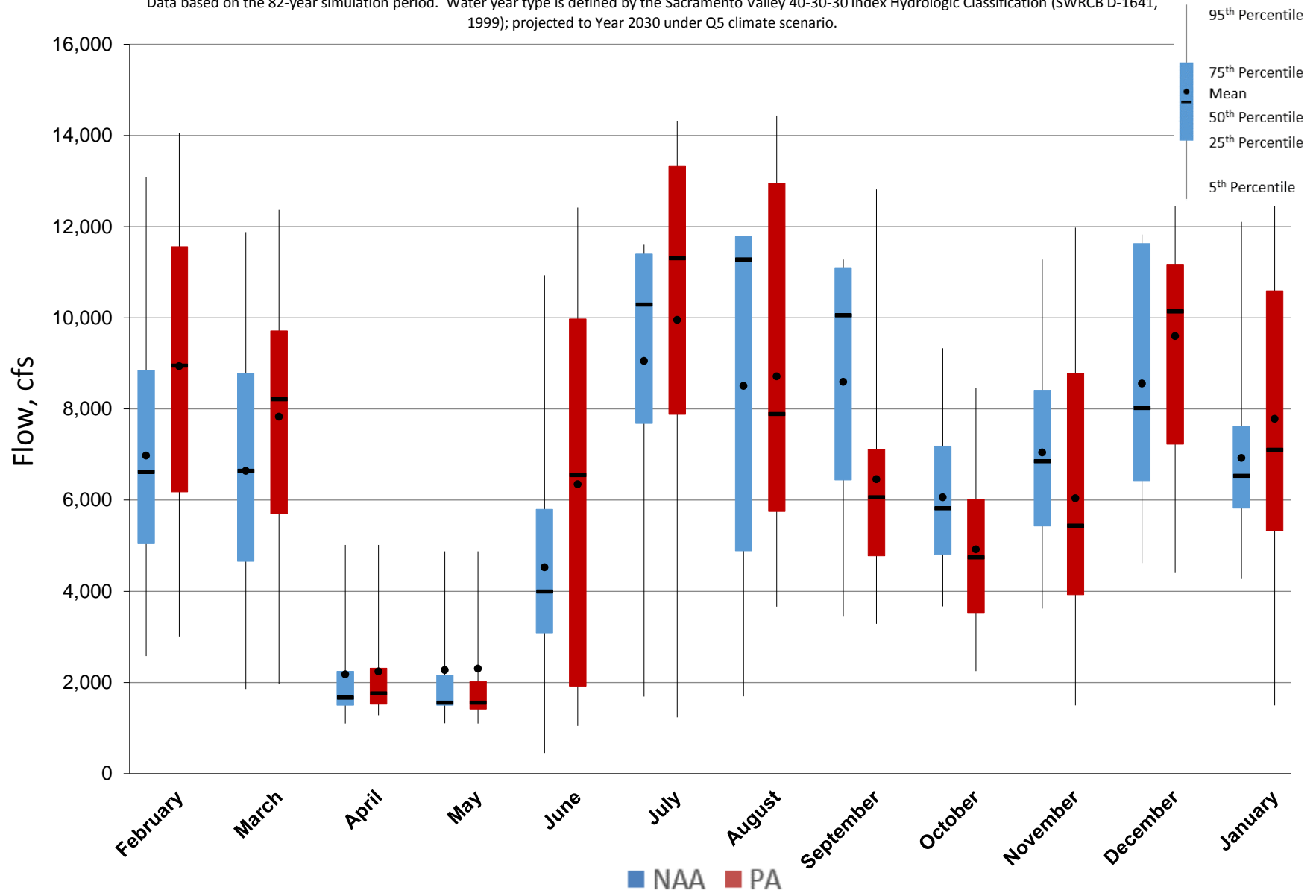
Figure 5.A.6-28-1. Monthly Flow Ranges For Total Delta Exports, All Years
