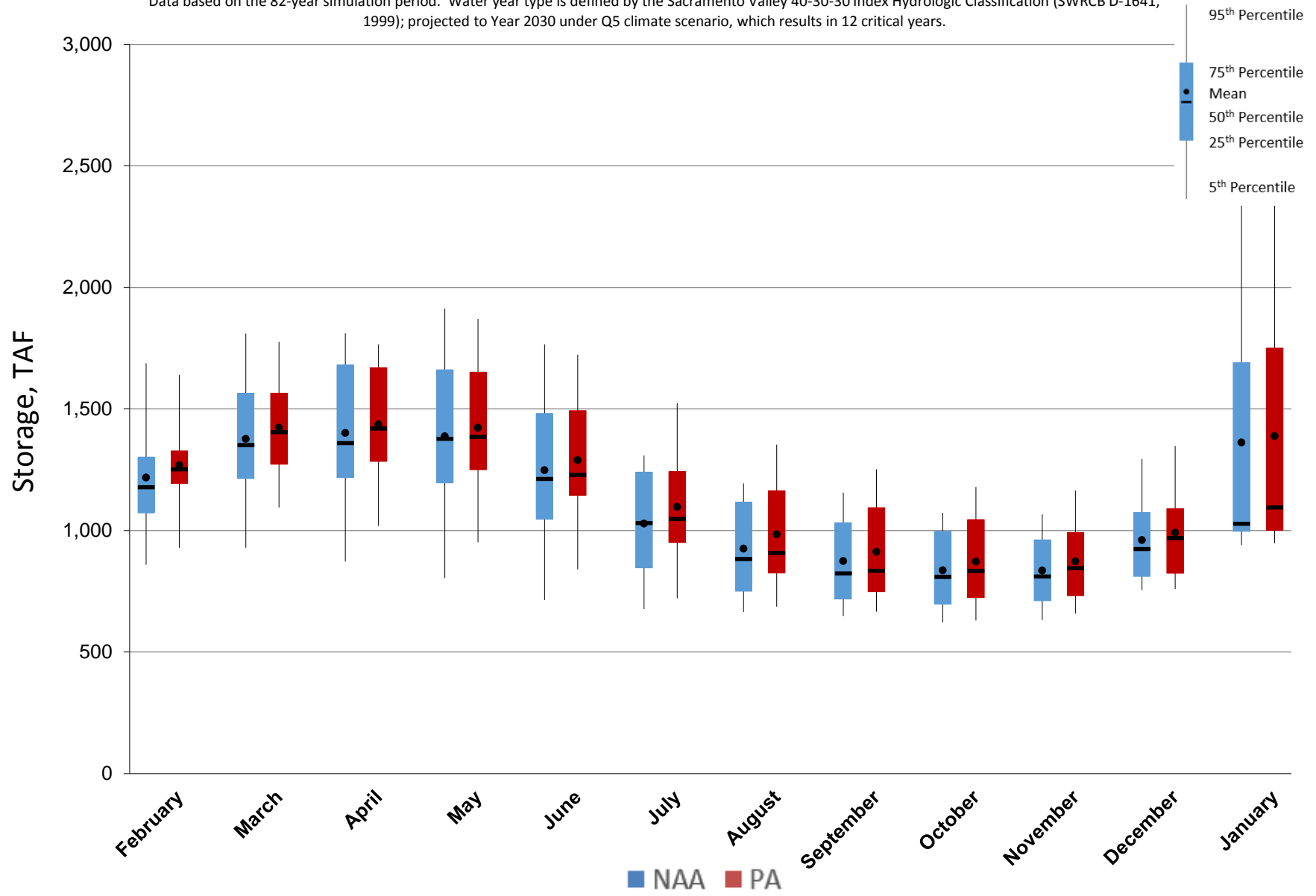
Figure 5.A.6-4-6. End of Month Storage Ranges For Lake Oroville, Critical Years
