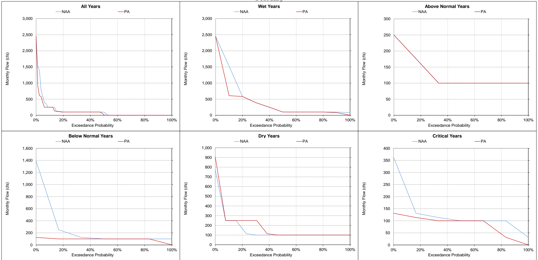
Figure 5.A.6-8-12. Clear Creek Tunnel Flow, Monthly Flow February
