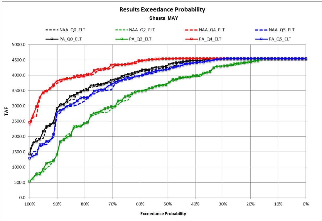
Figure 5.A.A.3-1 Shasta End of May Storage for the NAA and the PA Scenarios under Q0, Q2, Q4 and Q5 climate scenarios at Year 2030
