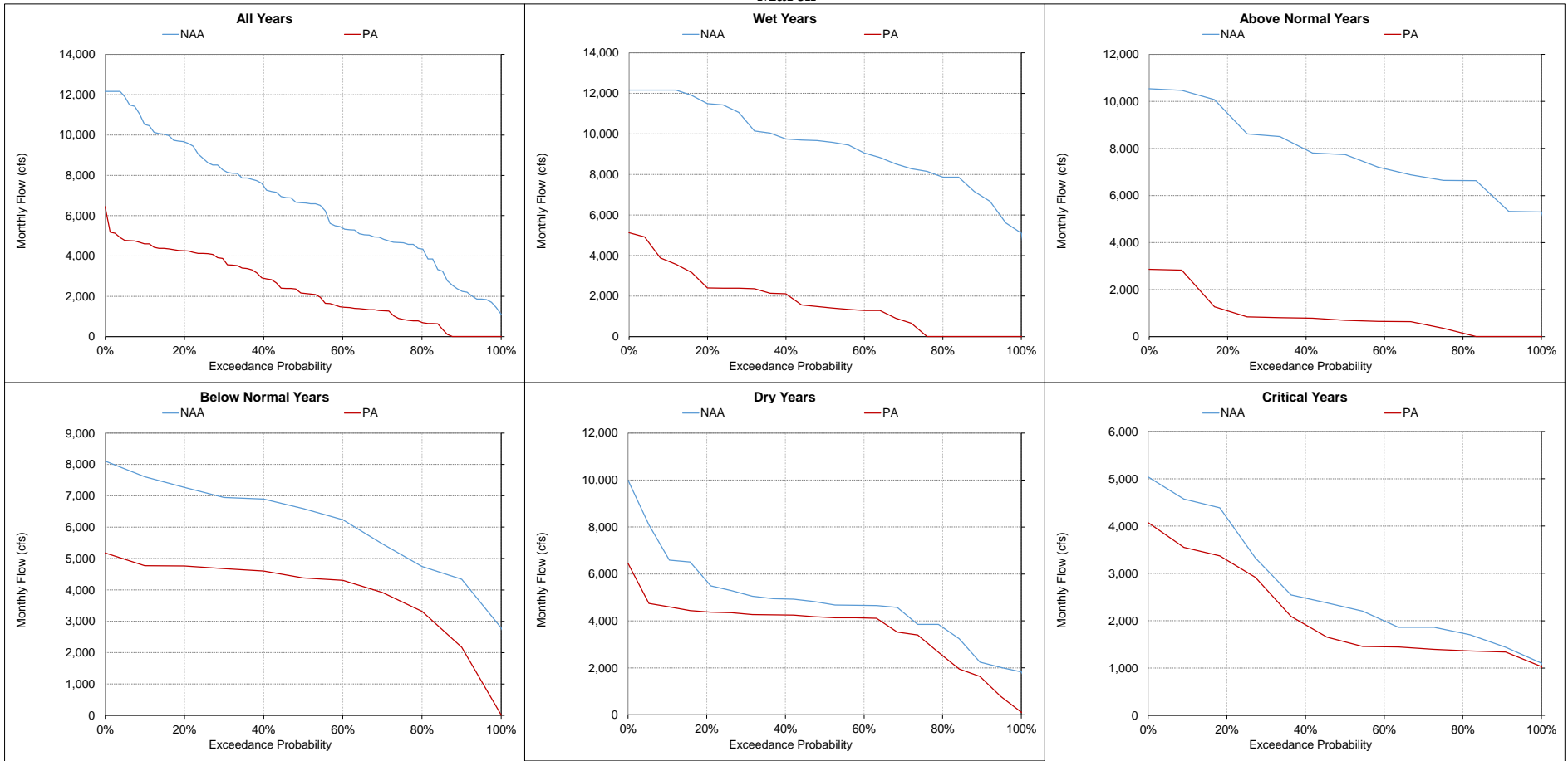
Figure 5.A.6-27-13. South Delta Exports, Monthly Flow March
