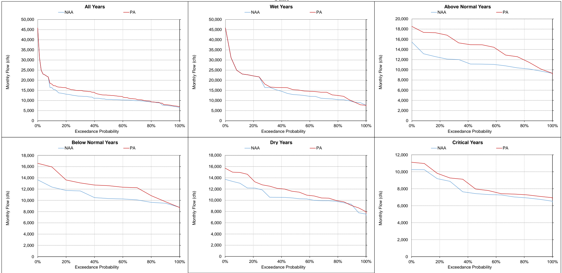
Figure 5.A.6-14-16. Sacramento River at Verona, Monthly Flow June
