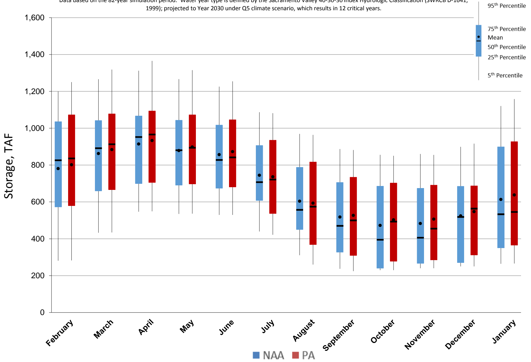
Figure 5.A.6-1-6. End of Month Storage Ranges For Trinity Lake, Critical Years
