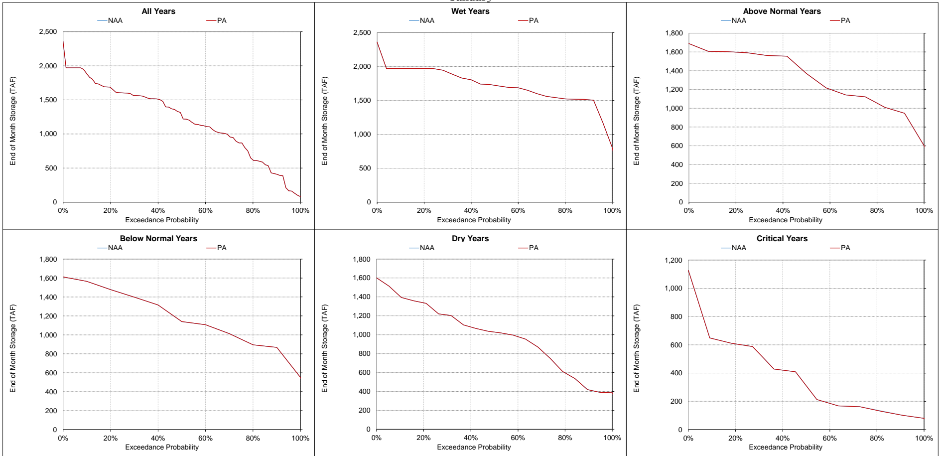
Figure 5.A.6-11. New Melones Lake, End of Month Storage January
