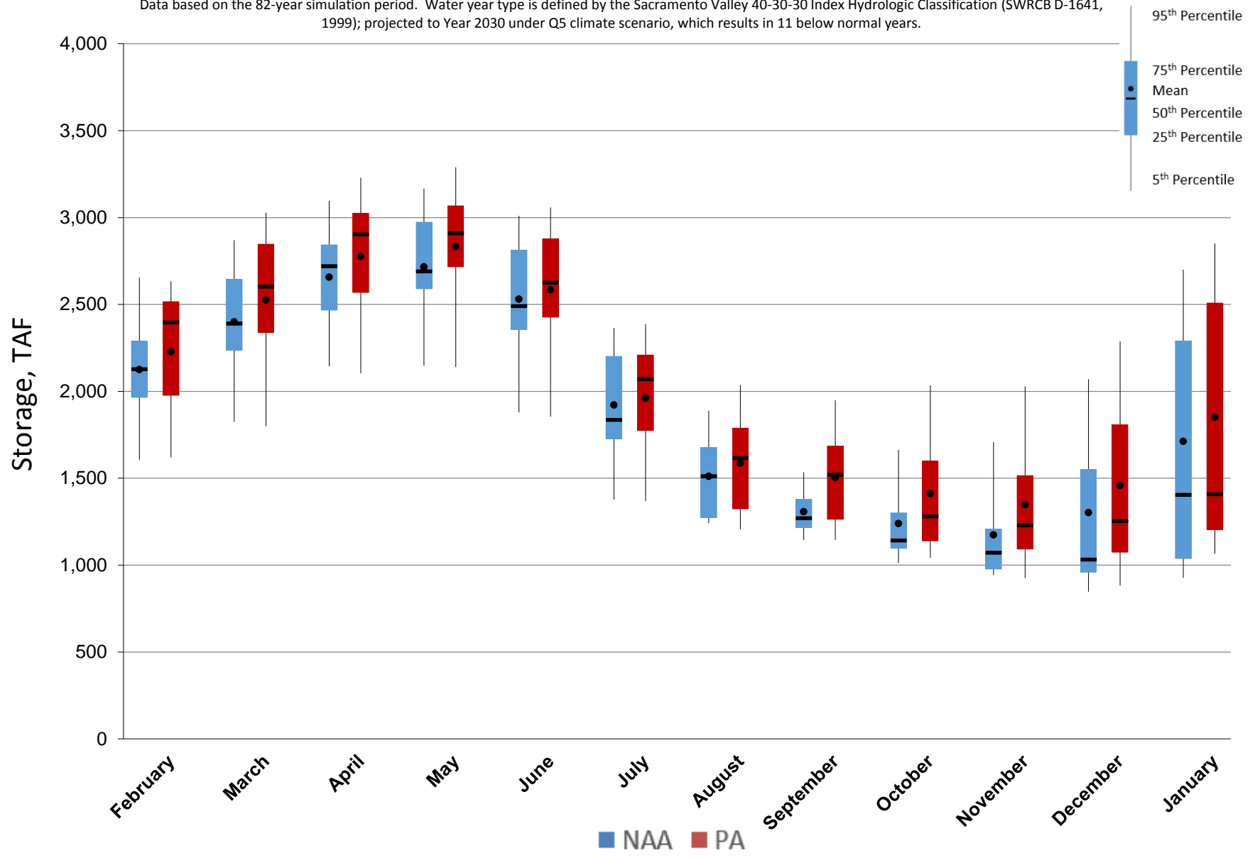
Figure 5.A.6-4-4. End of Month Storage Ranges For Lake Oroville, Below Normal Years
