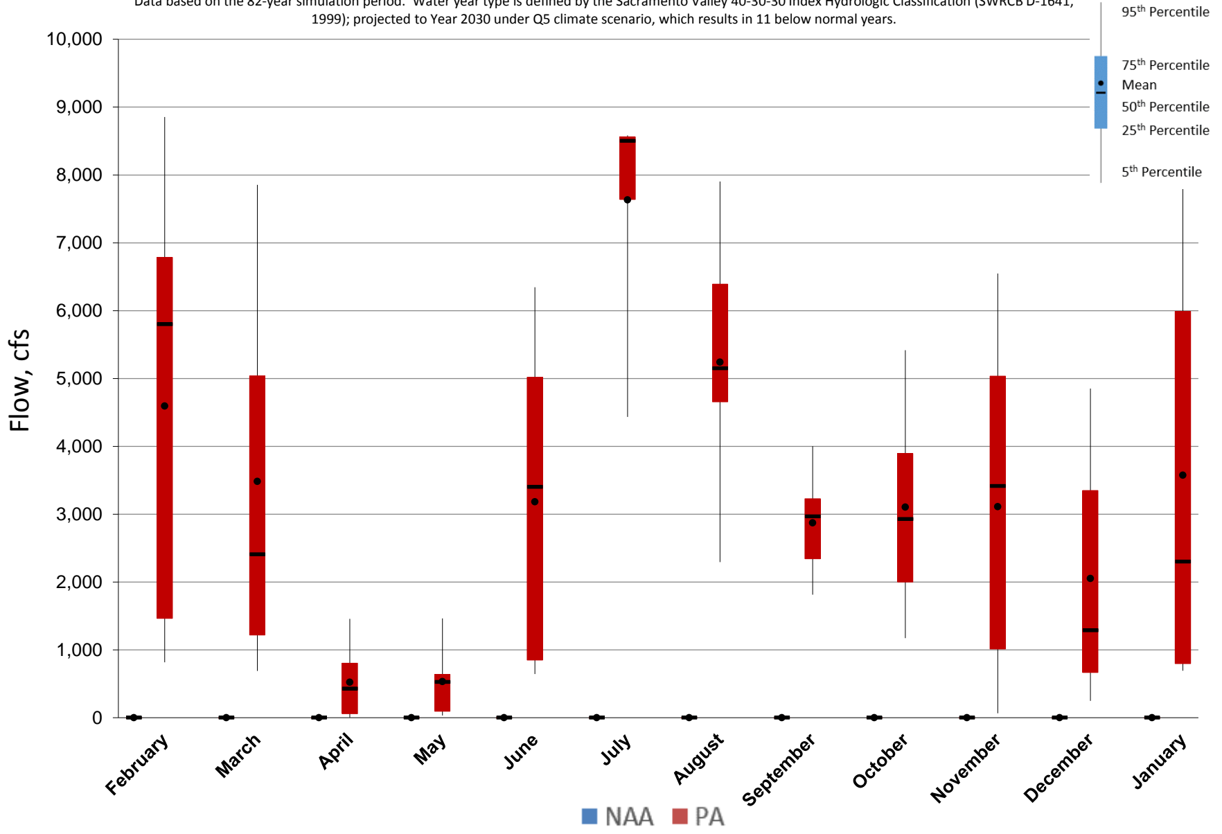
Figure 5.A.6-19-4. Monthly Flow Ranges For North Delta Diversions near Hood, Below Normal Years
