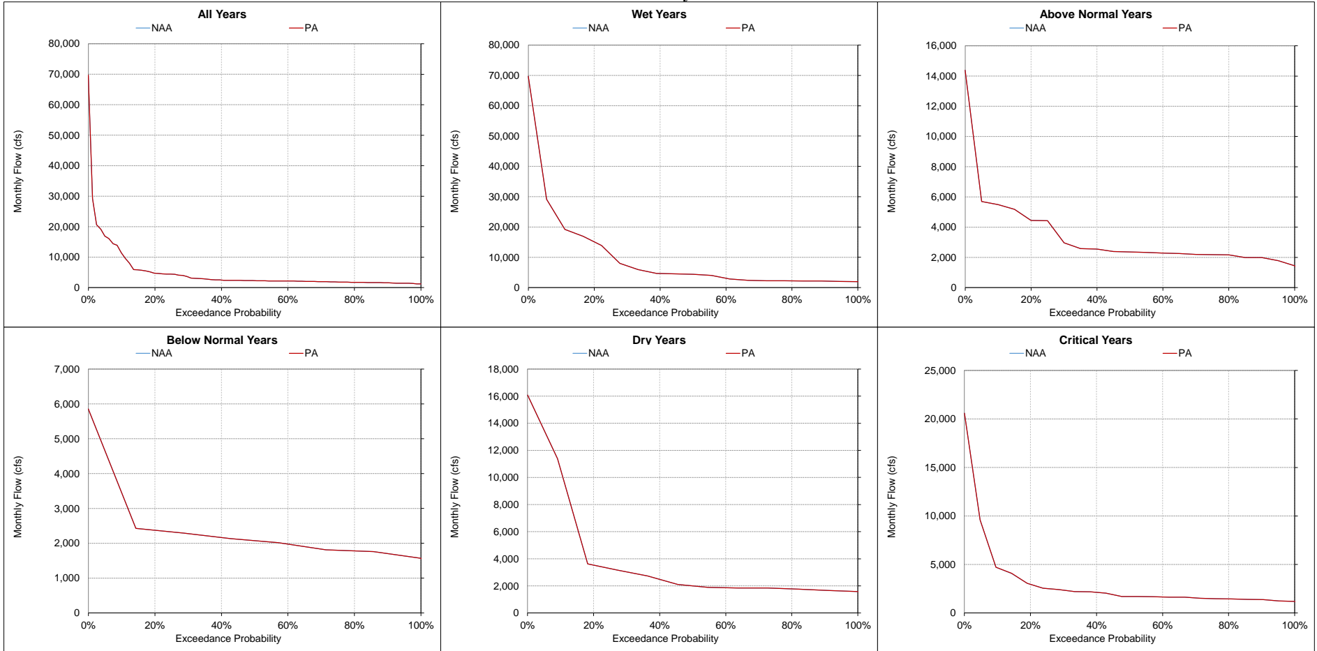
Figure 5.A.6-23-11. San Joaquin River at Vernalis, Monthly Flow
