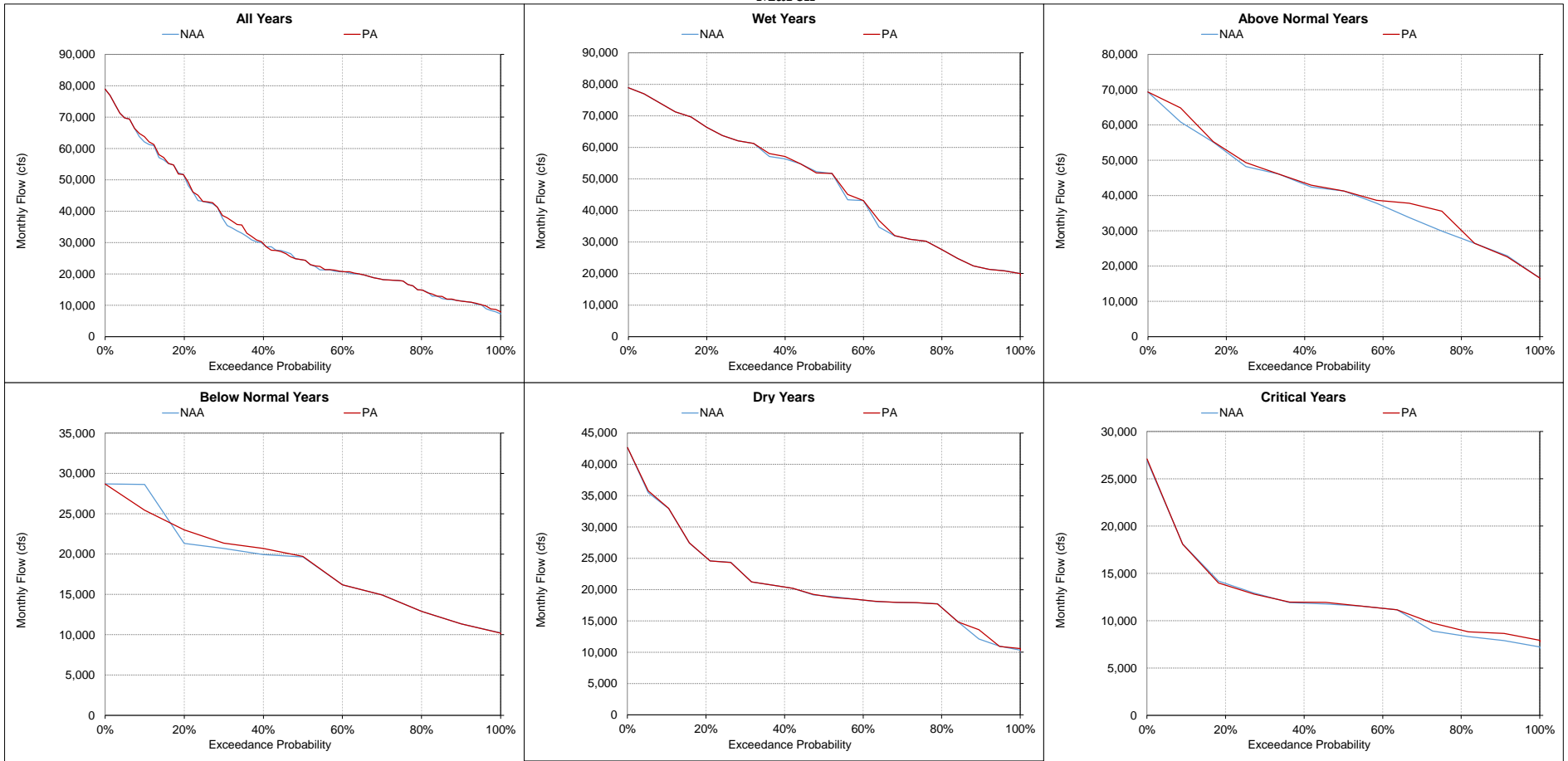
Figure 5.A.6-18-13. Sacramento River at Freeport, Monthly Flow March
