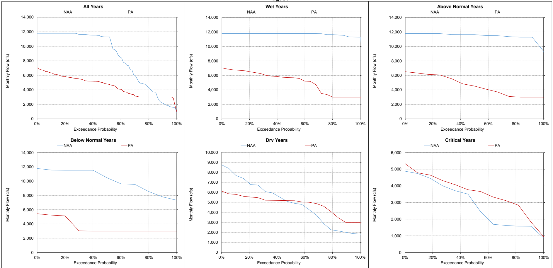
Figure 5.A.6-27-18. South Delta Exports, Monthly Flow August
