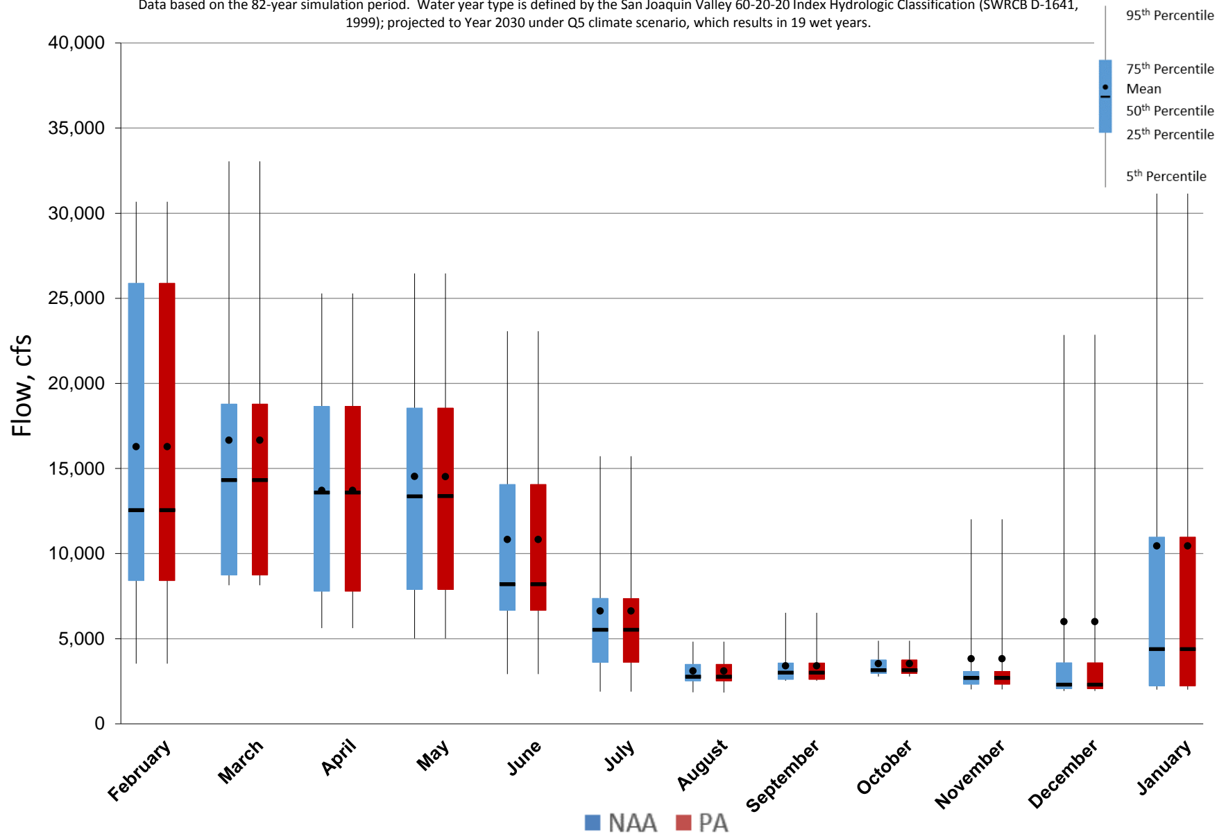
Figure 5.A.6-23-2. Monthly Flow Ranges for San Joaquin River at Vernalis, Wet Years
