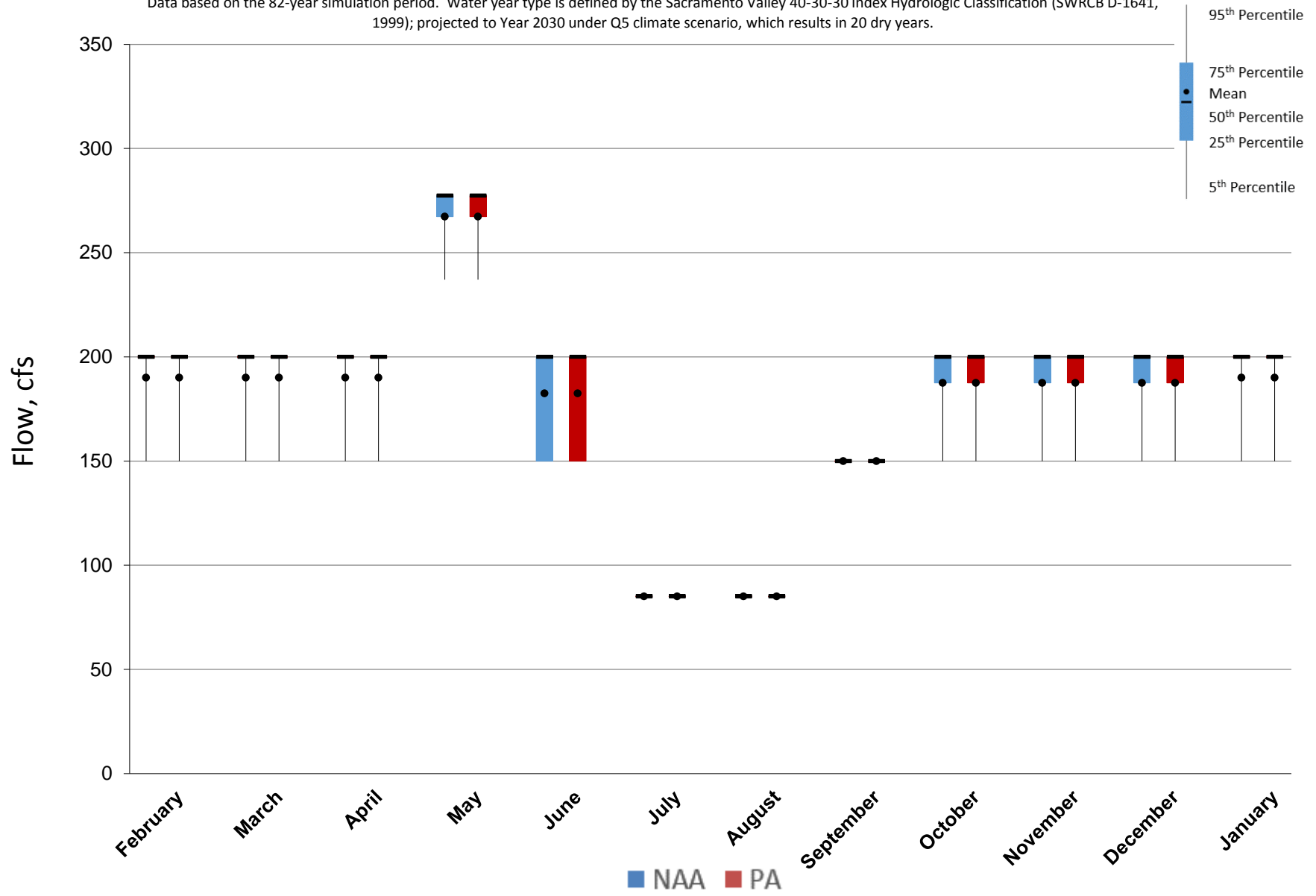
Figure 5.A.6-9-5. Monthly Flow Ranges For Clear Creek below Whiskeytown Dam, Dry Years
