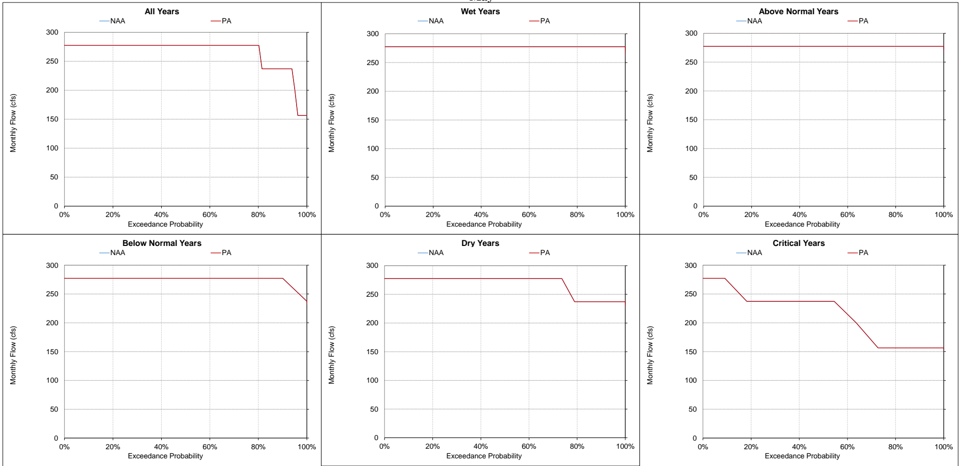
Figure 5.A.6-9-15. Clear Creek below Whiskeytown Dam, Monthly Flow May
