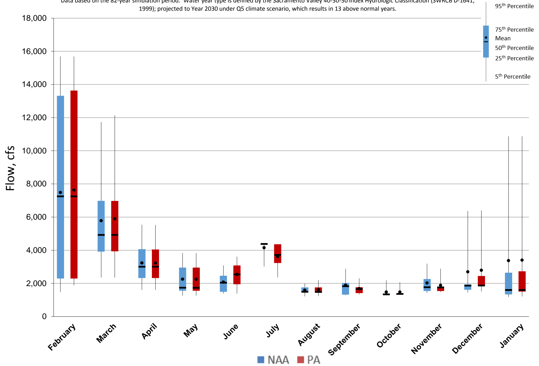
Figure 5.A.6-17-3. Monthly Flow Ranges For American River at Sacramento River Confluence, Above Normal Years
