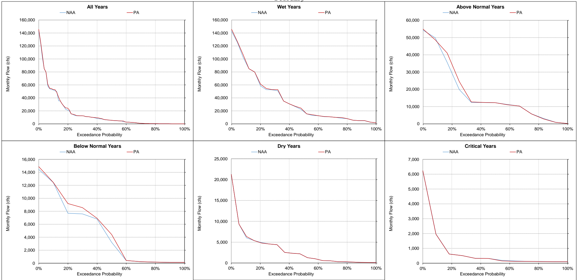
Figure 5.A.6-20-12. Yolo Bypass, Monthly Flow February
