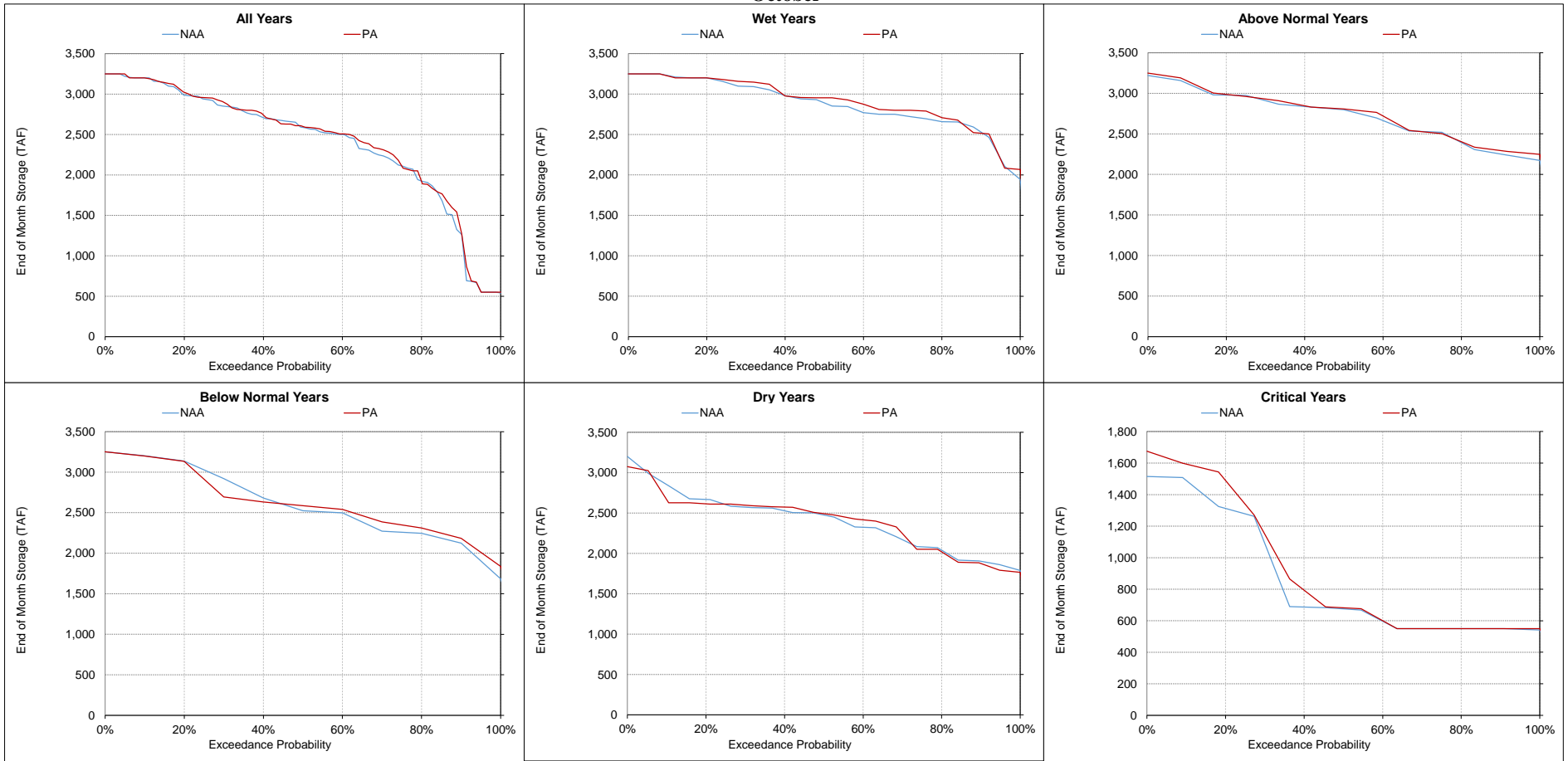
Figure 5.A.6-3-8. Shasta Lake, End of Month Storage October
