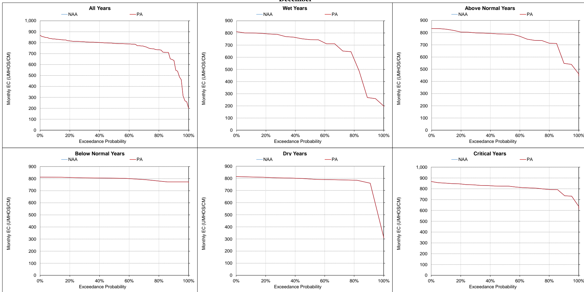
Figure 5.A.6-30-10. San Joaquin River at Vernalis, Monthly EC December
