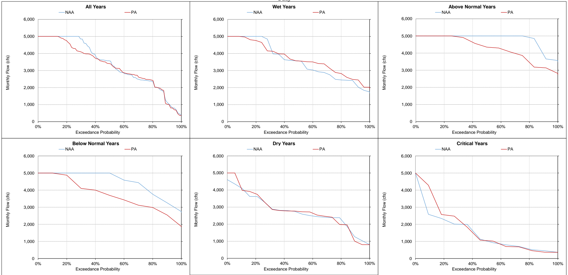
Figure 5.A.6-16-17. American River below Nimbus Dam, Monthly Flow July
