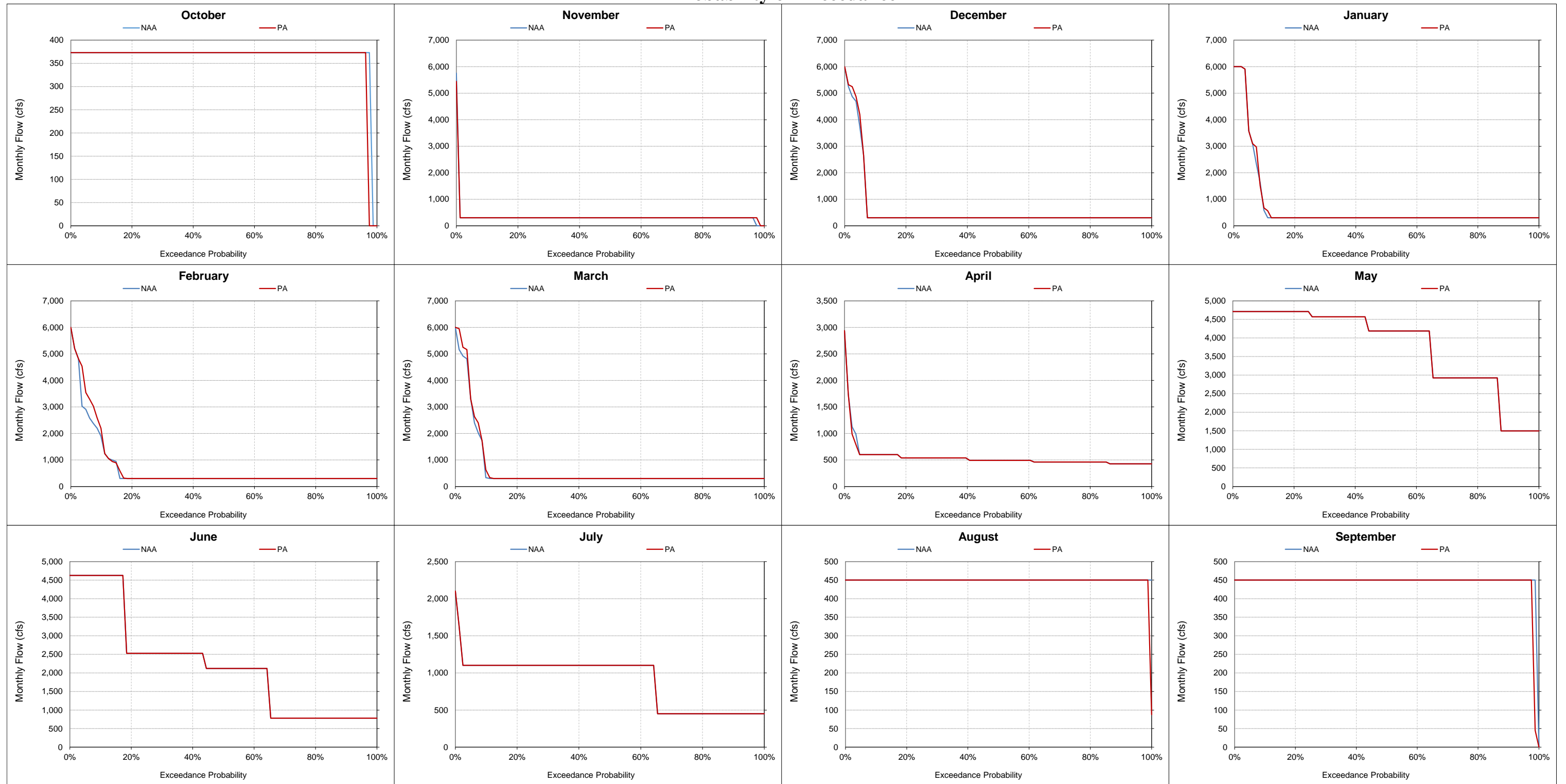
Figure 5.A.6-7-7. Trinity River below Lewiston Dam, Monthly Flow Probability of Exceedance
