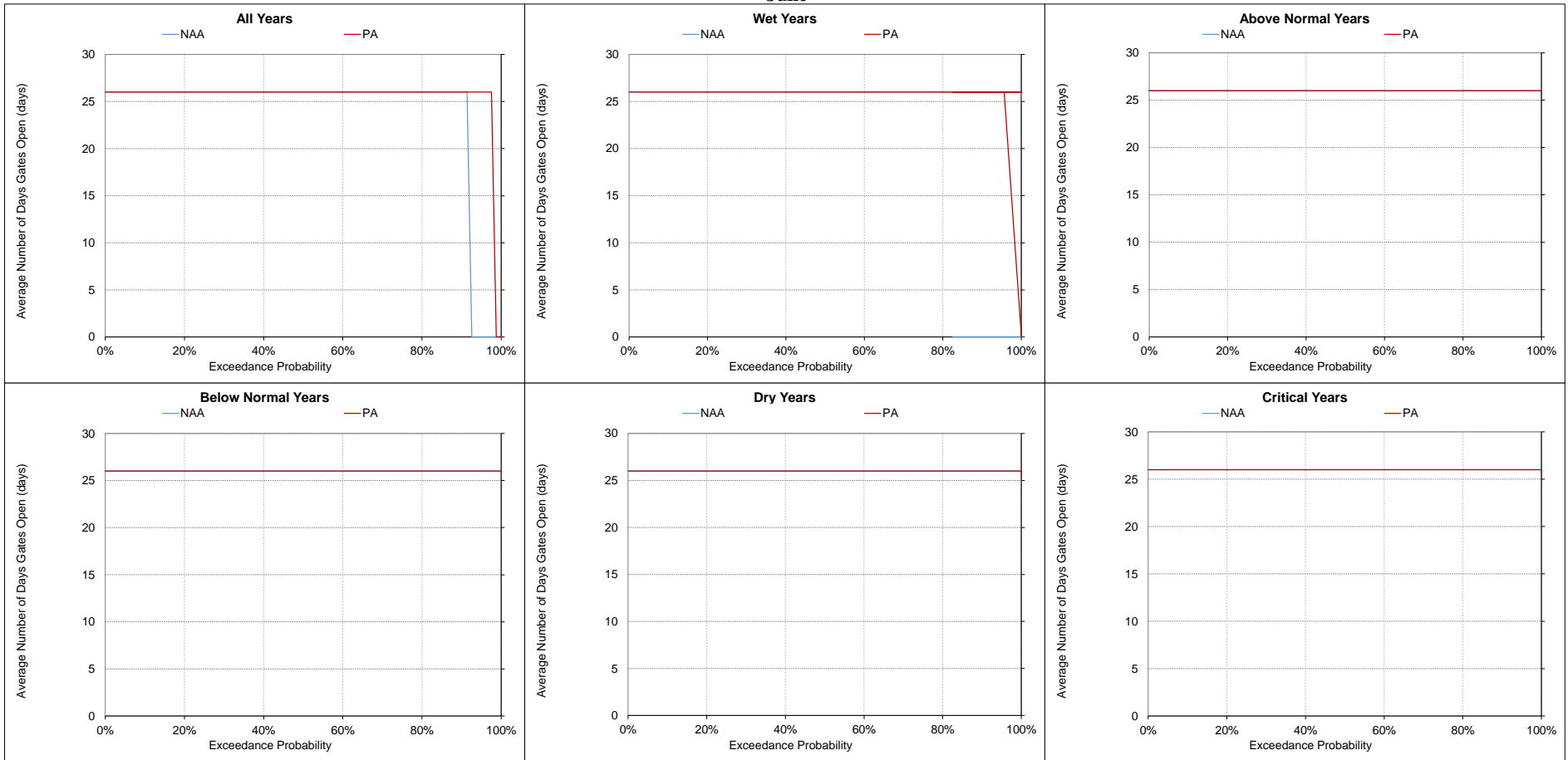
Figure 5.A.6-31-16. Delta Cross Channel, Average Number of Days Gates Open June
