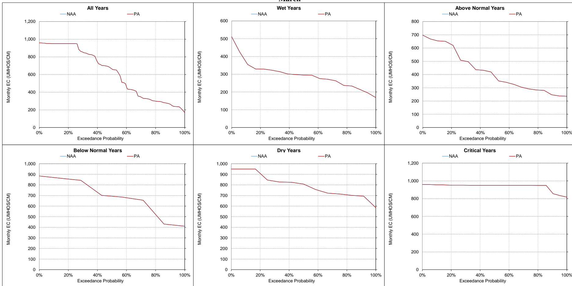
Figure 5.A.6-30-13. San Joaquin River at Vernalis, Monthly EC March
