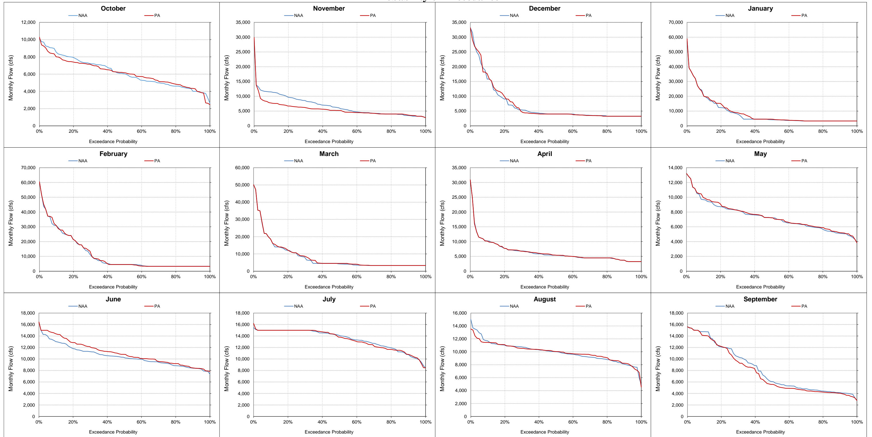
Figure 5.A.6-10-7. Sacramento River below Keswick Dam, Monthly Flow Probability of Exceedance
