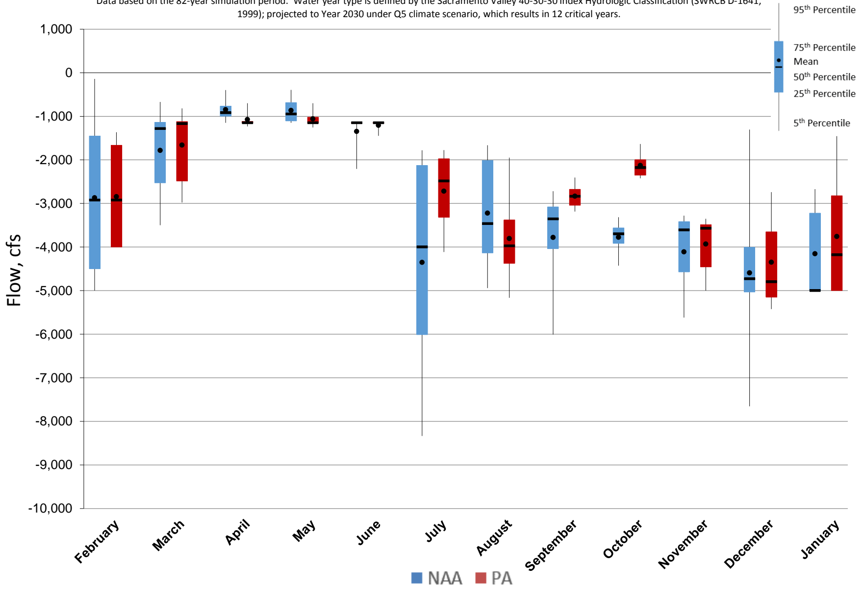
Figure 5.A.6-25-6. Monthly Flow Ranges For Old and Middle River, Critical Years
