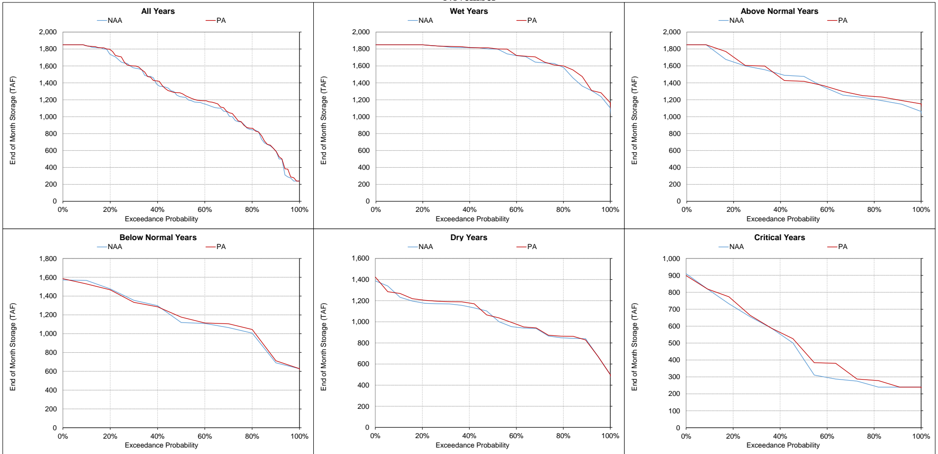
Figure 5.A.6-1-9. Trinity Lake, End of Month Storage November
