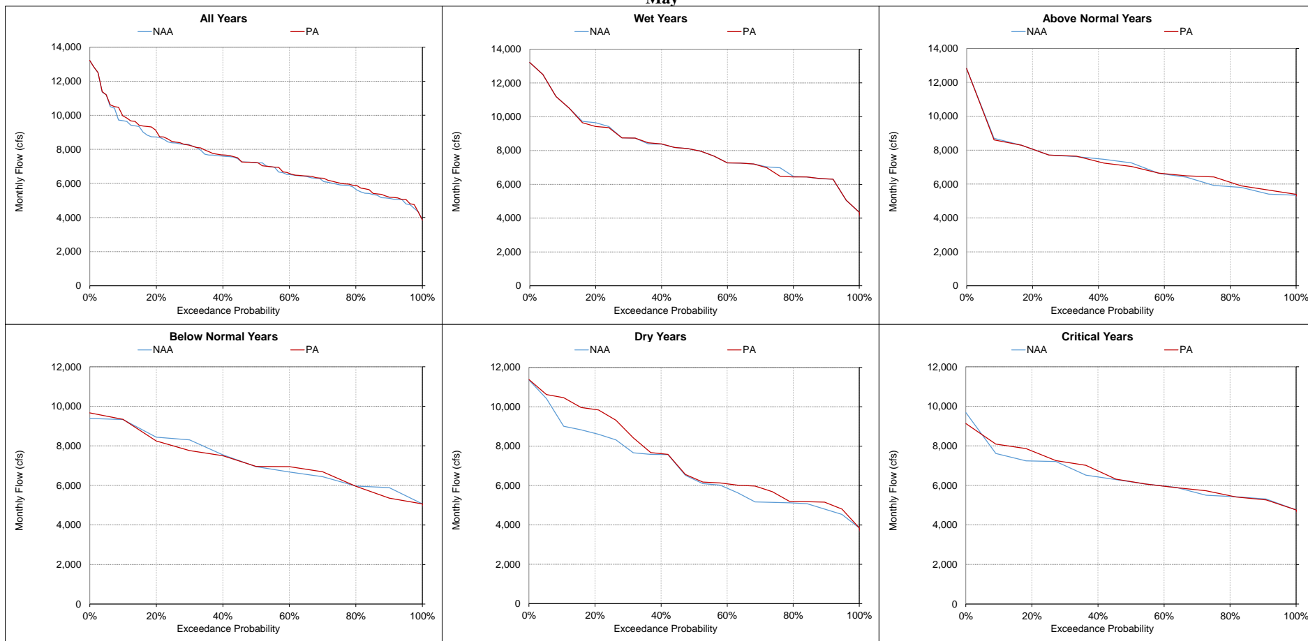
Figure 5.A.6-10-15. Sacramento River below Keswick Dam, Monthly Flow May
