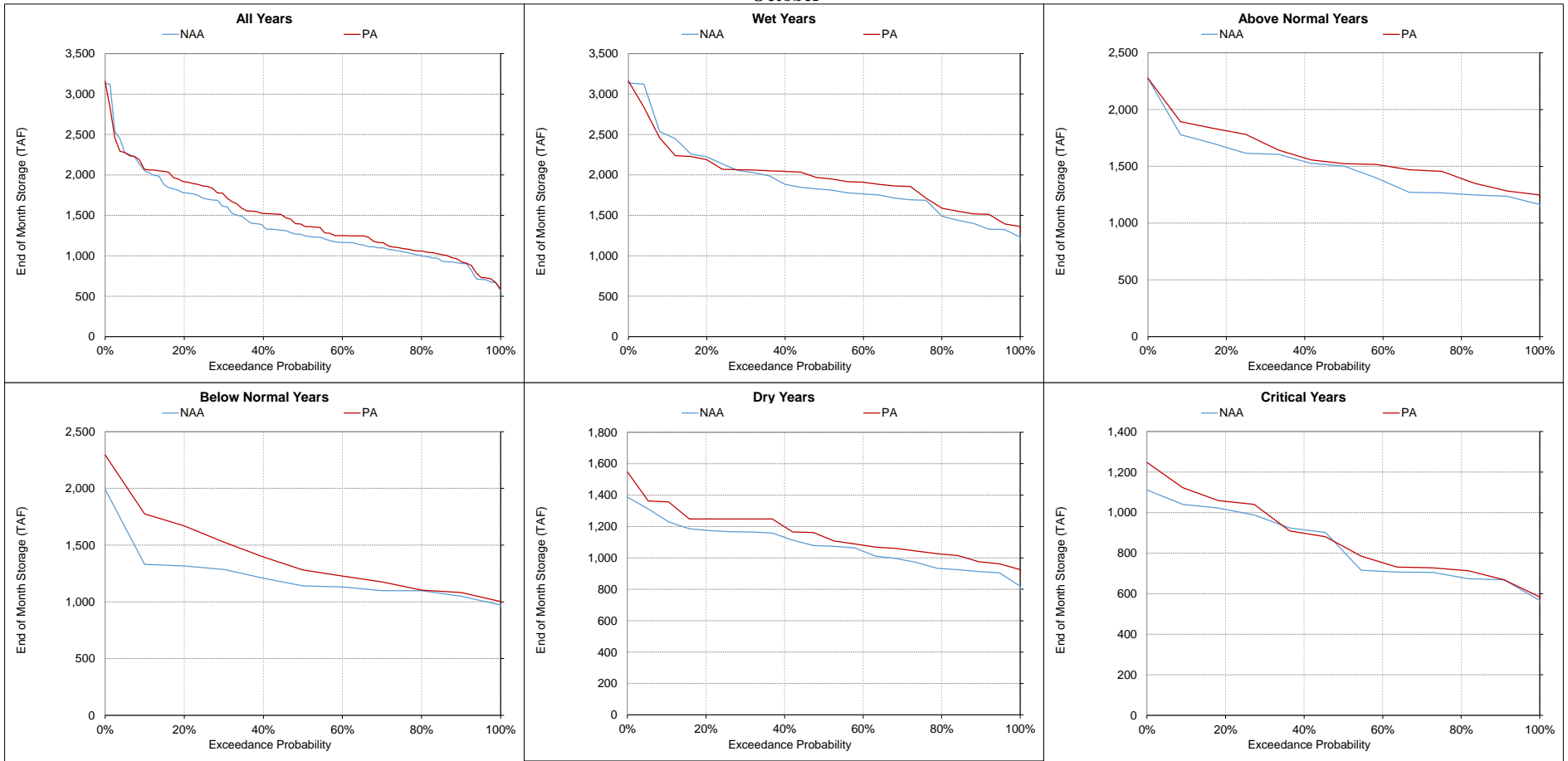
Figure 5.A.6-4-8. Lake Oroville, End of Month Storage October
