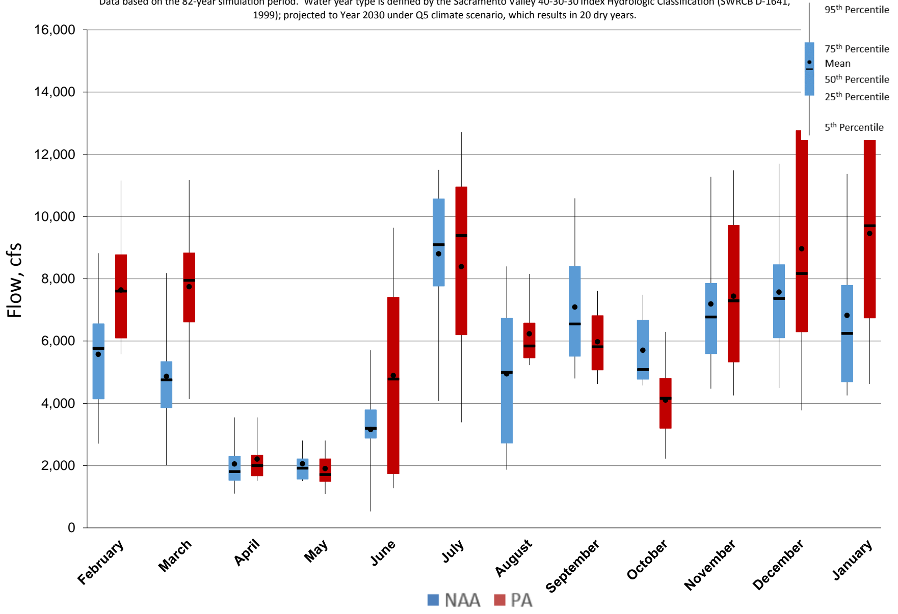
Figure 5.A.6-28-5. Monthly Flow Ranges For Total Delta Exports, Dry Years
