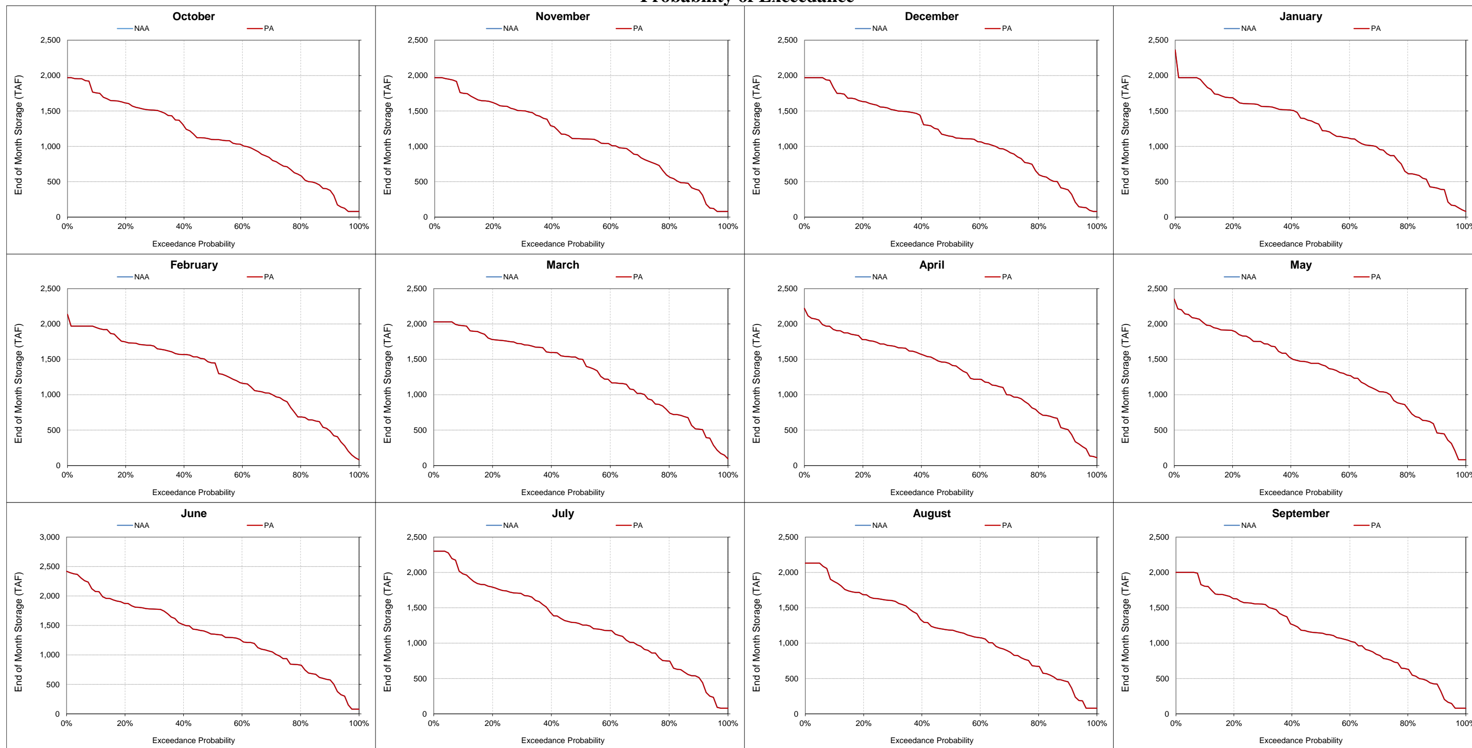
Figure 5.A.6-6-7. New Melones Lake, End of Month Storage Probability of Exceedance
