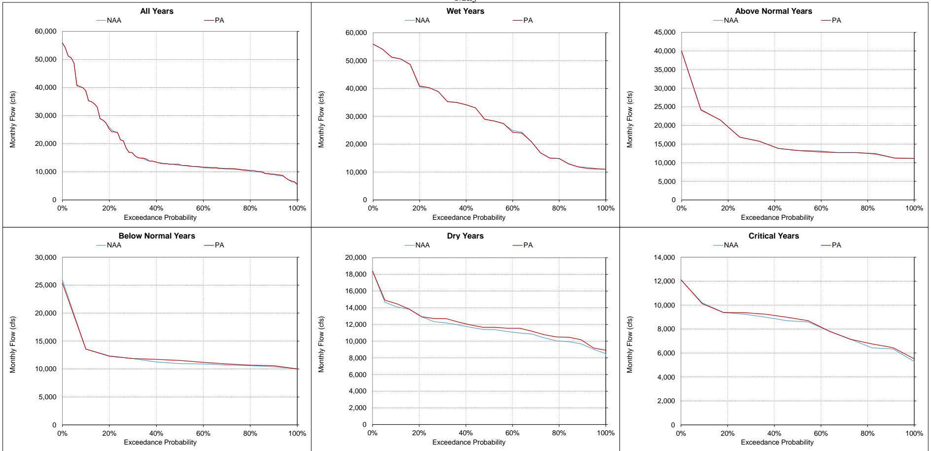
Figure 5.A.6-18-15. Sacramento River at Freeport, Monthly Flow May
