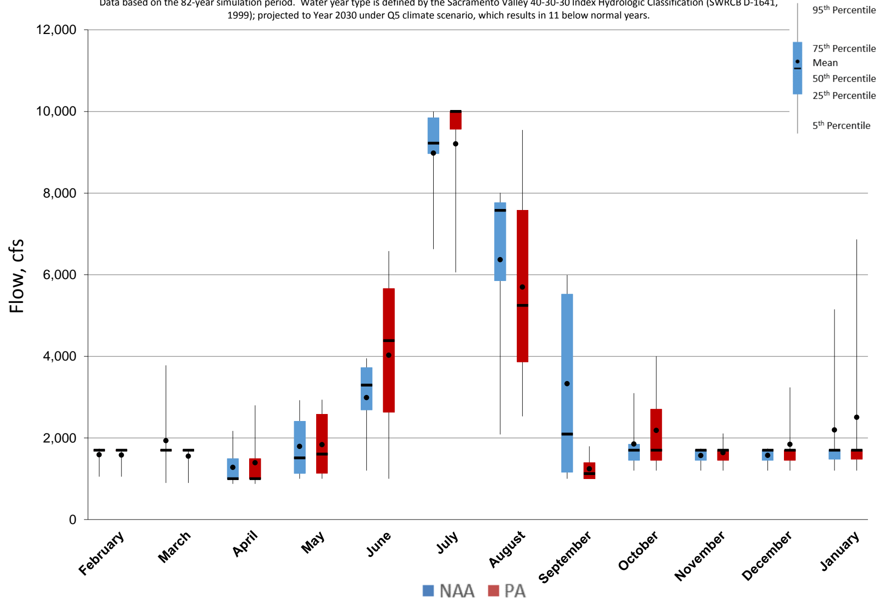
Figure 5.A.6-12-4. Monthly Flow Ranges For Feather River below Thermalito Diversion Dam, Below Normal Years
