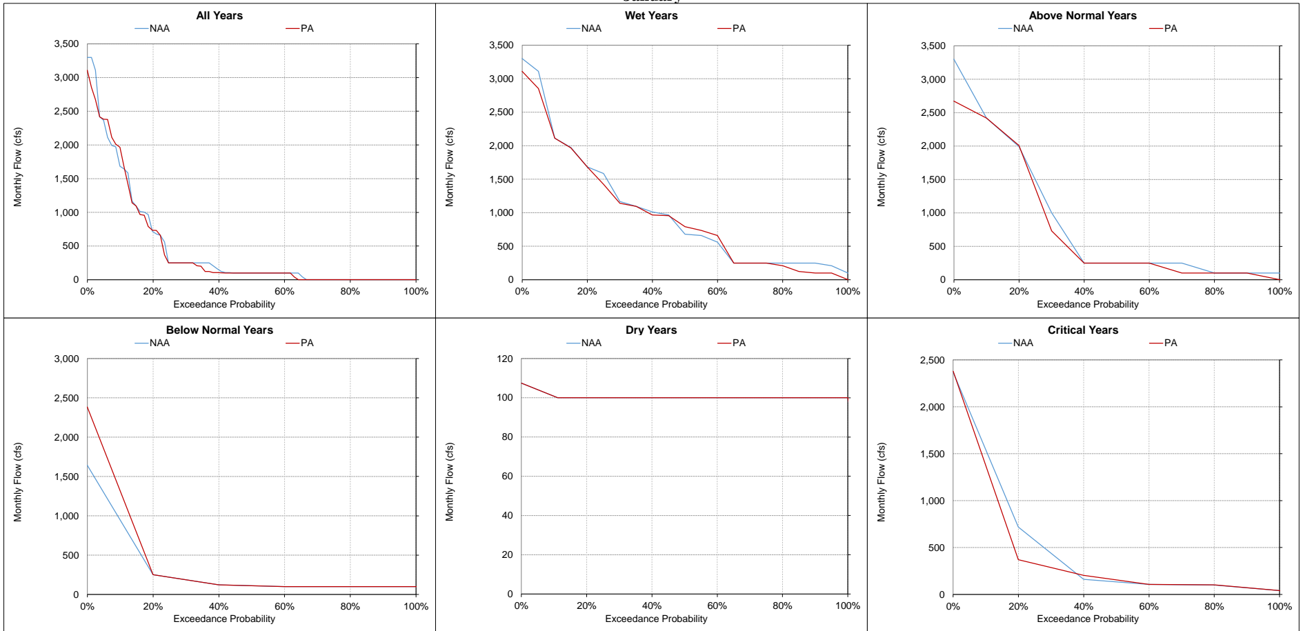
Figure 5.A.6-8-11. Clear Creek Tunnel Flow, Monthly Flow January
