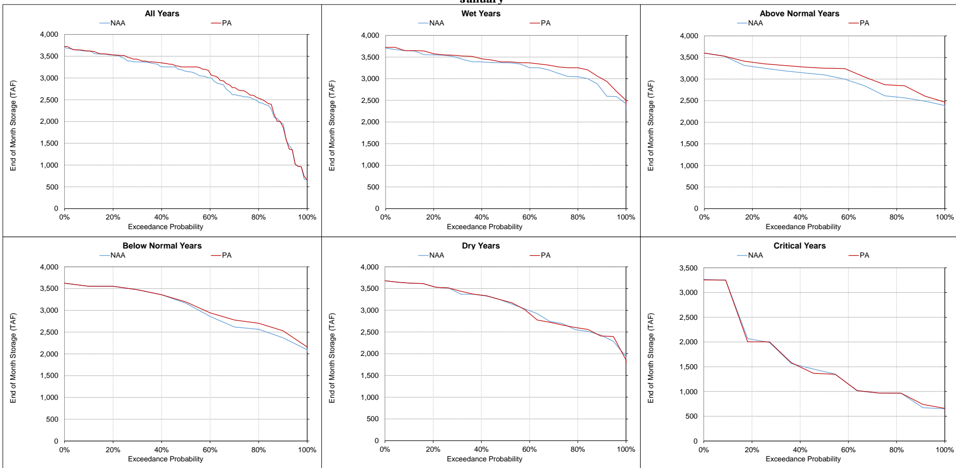
Figure 5.A.6-3-11. Shasta Lake, End of Month Storage January
