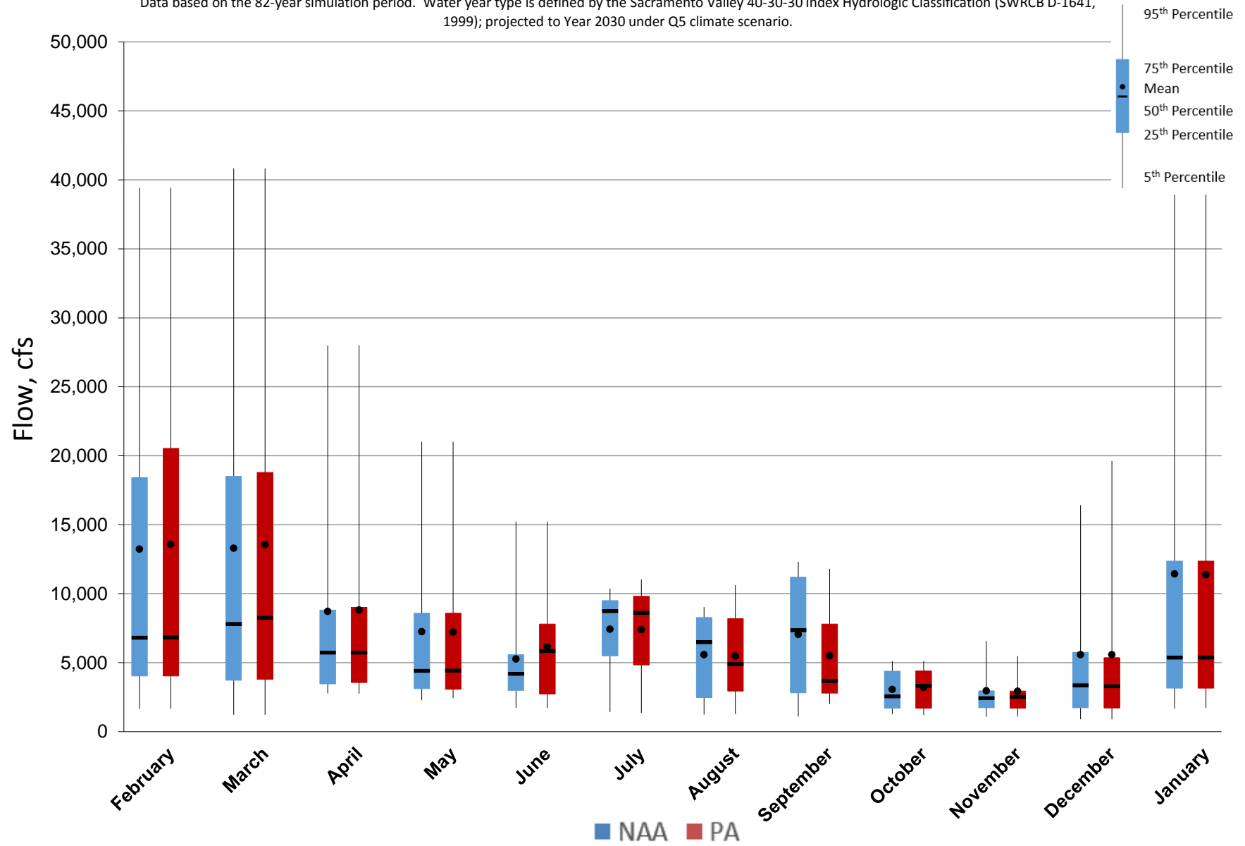
Figure 5.A.6-13-1. Monthly Flow Ranges For Feather River at Sacramento River Confluence, All Years
