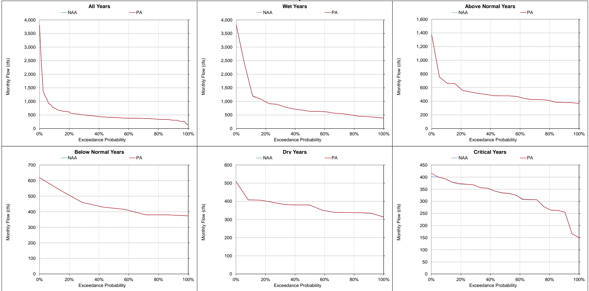
Figure 5.A.6-22-17. Stanislaus River at Mouth, Monthly Flow July
