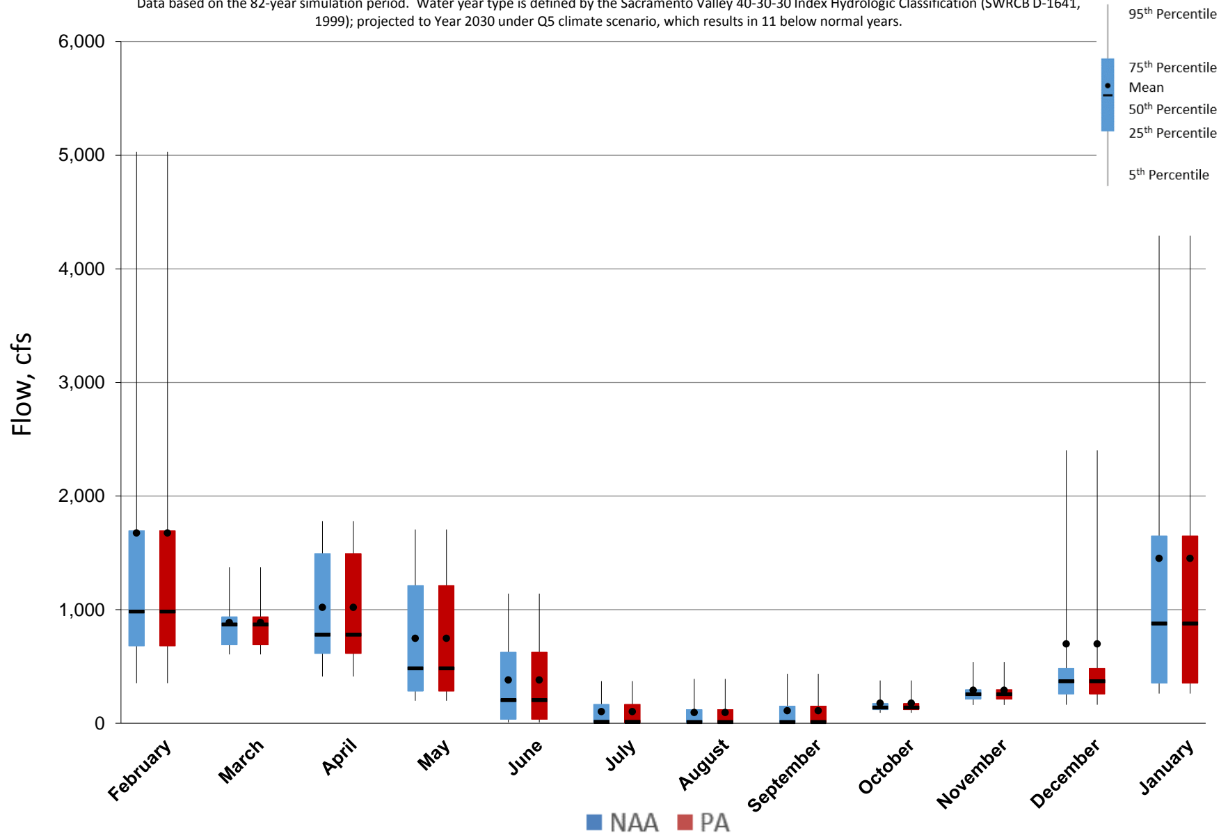
Figure 5.A.6-24-4. Monthly Flow Ranges For Mokelumne and Cosumnes River, Below Normal Years
