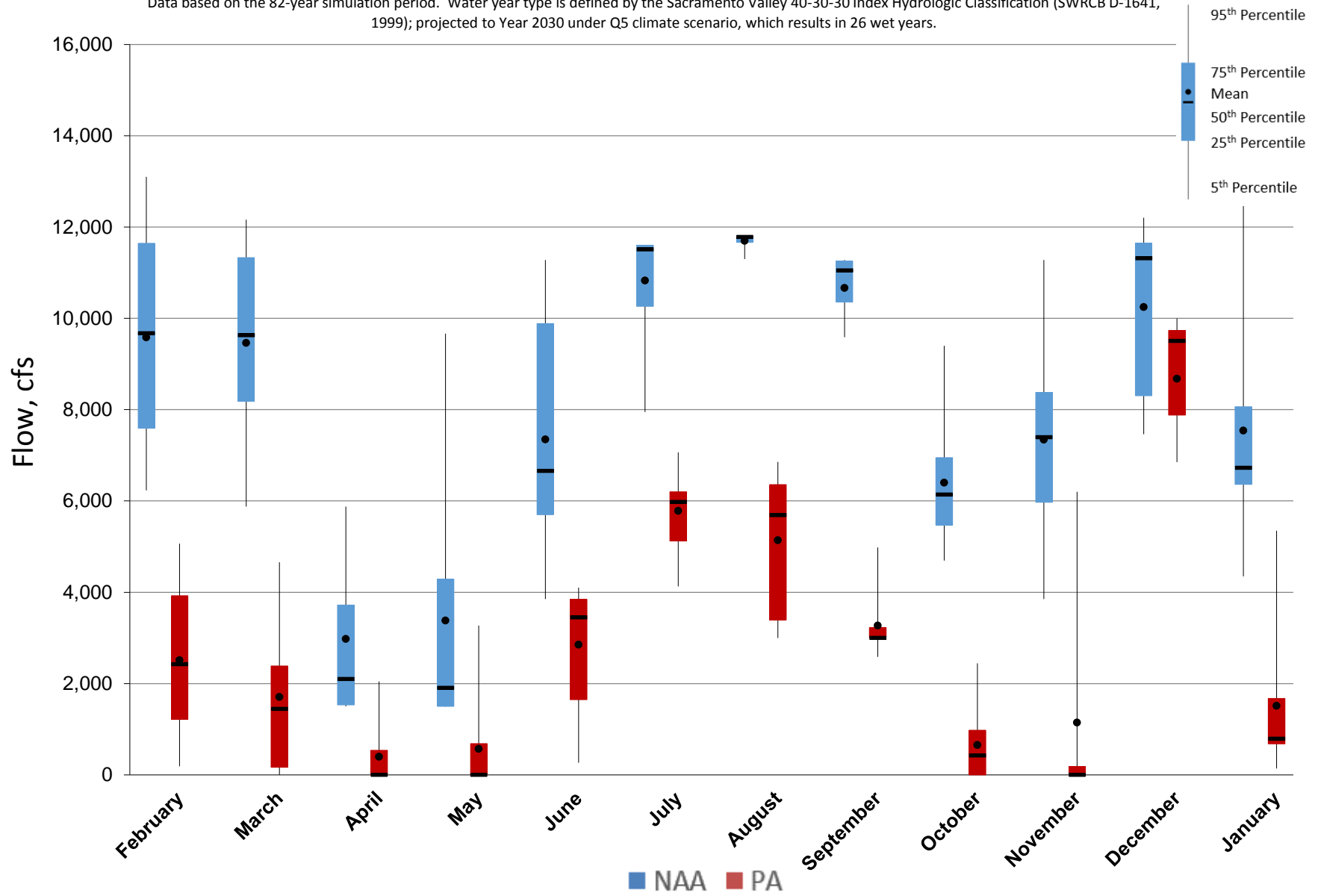
Figure 5.A.6-27-2. Monthly Flow Ranges For South Delta Exports, Wet Years
