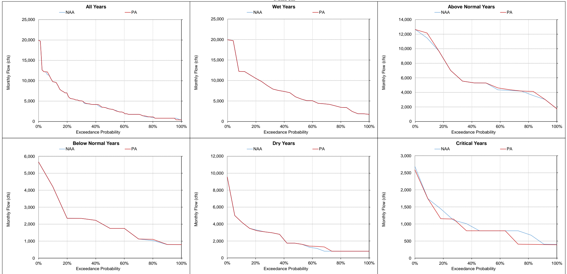
Figure 5.A.6-16-13. American River below Nimbus Dam, Monthly Flow March
