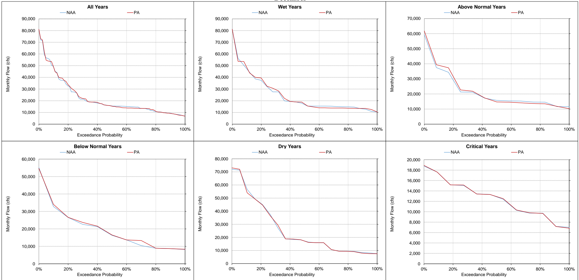
Figure 5.A.6-18-10. Sacramento River at Freeport, Monthly Flow December
