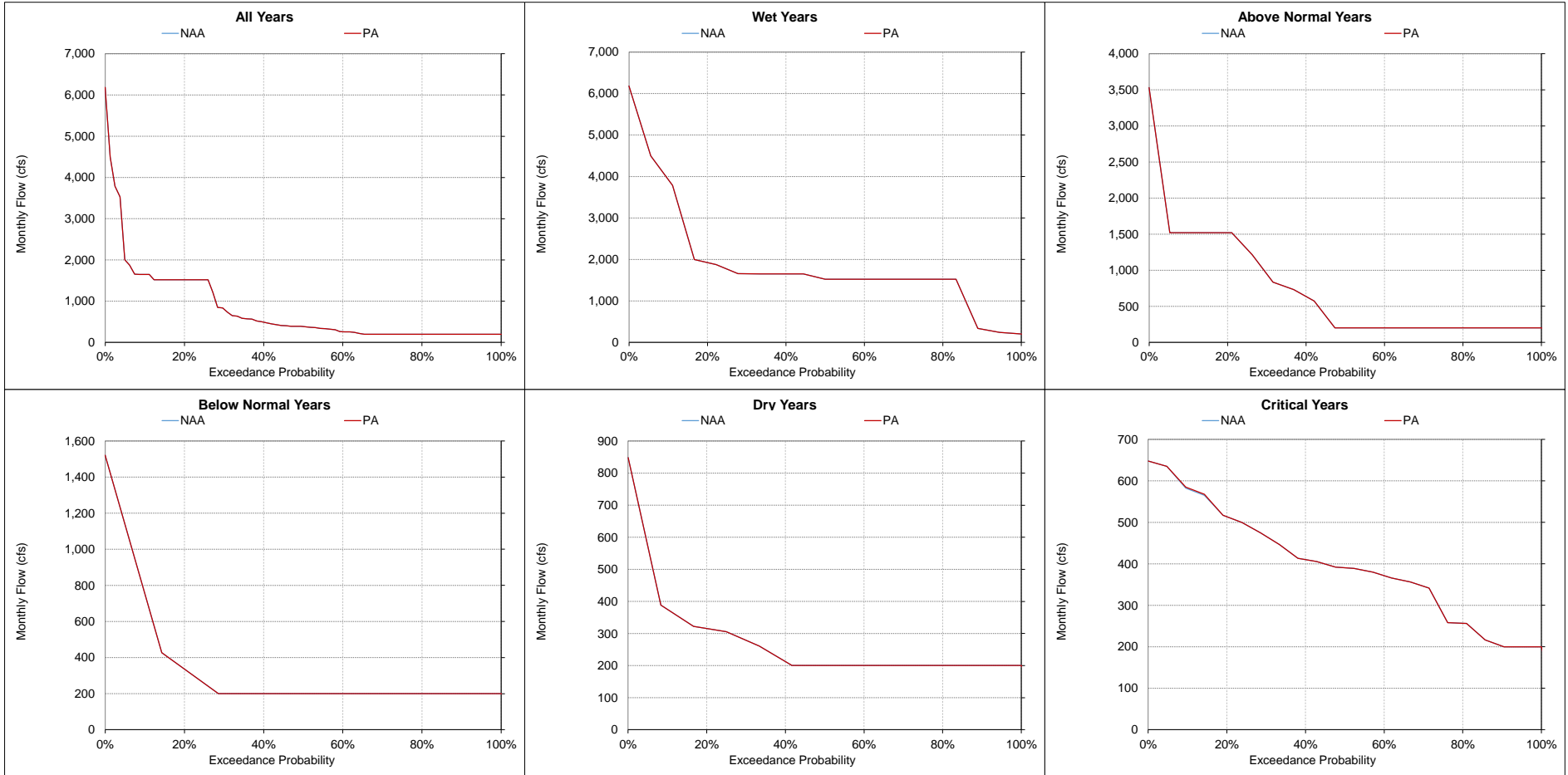
Figure 5.A.6-21-13. Stanislaus River at Ripon, Monthly Flow March
