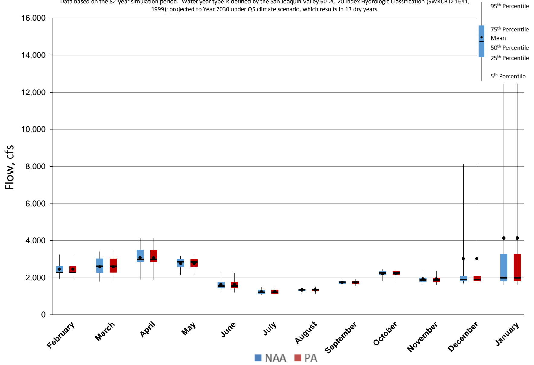
Figure 5.A.6-23-5. Monthly Flow Ranges for San Joaquin River at Vernalis, Dry Years
