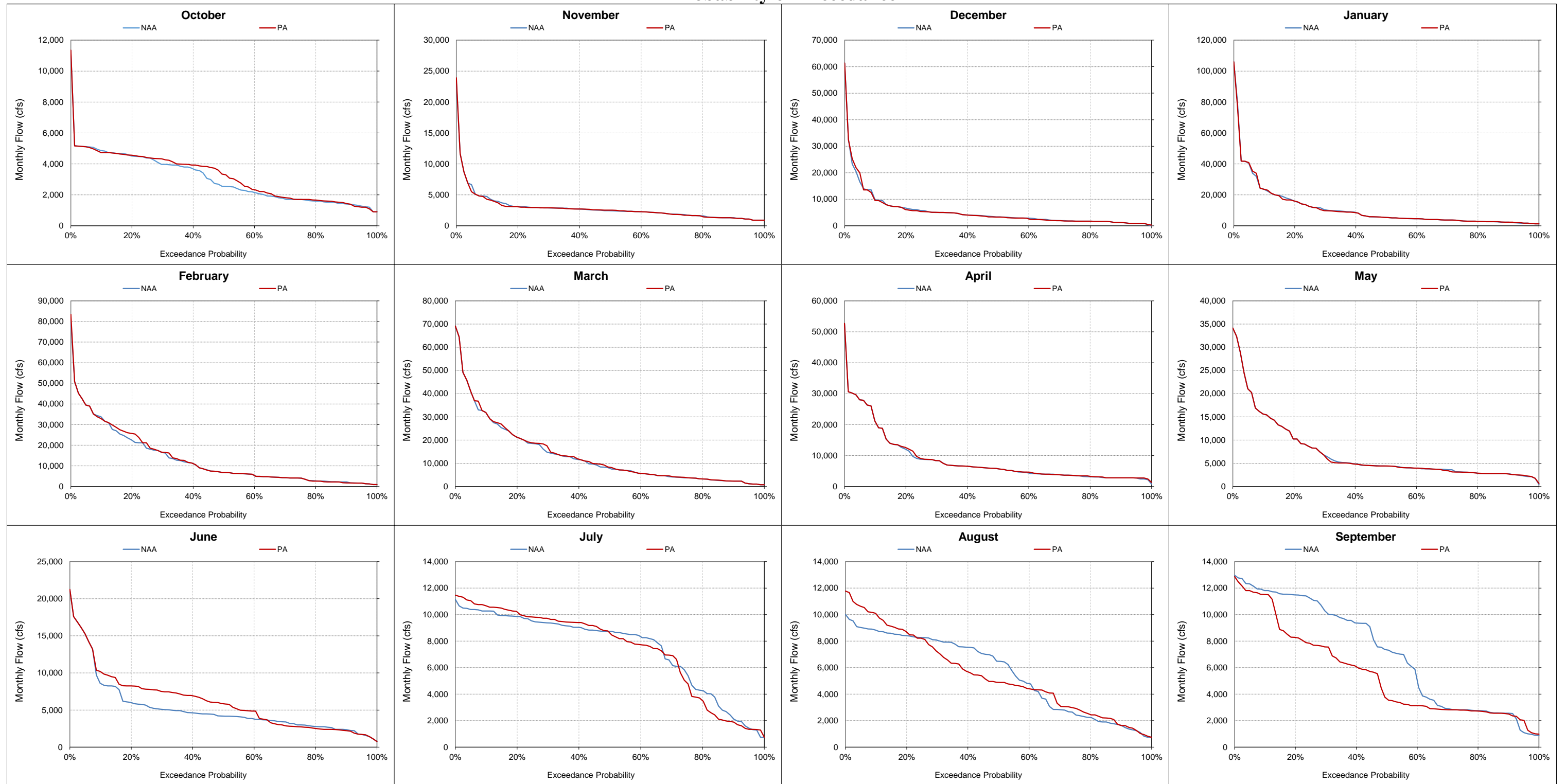
Figure 5.A.6-13-7. Feather River at Sacramento River Confluence, Monthly Flow Probability of Exceedance
