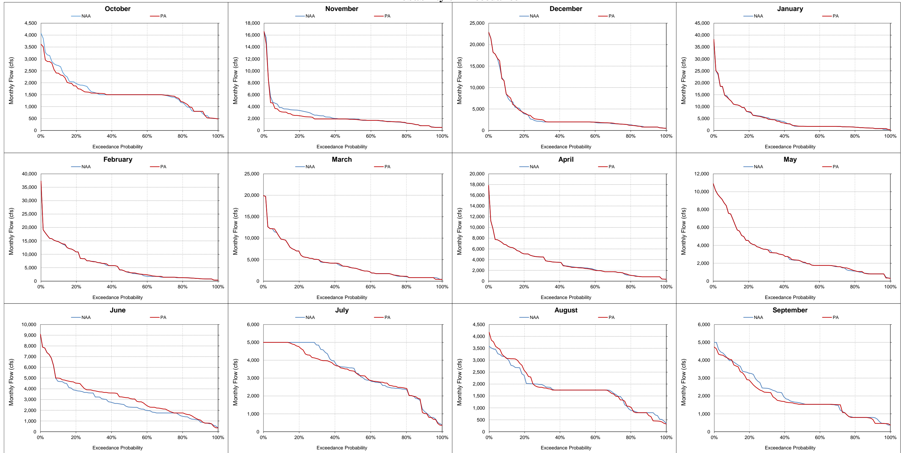
Figure 5.A.6-16-7. American River below Nimbus Dam, Monthly Flow Probability of Exceedance
