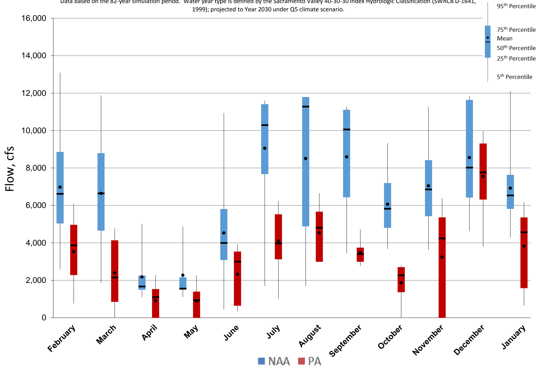
Figure 5.A.6-27-1. Monthly Flow Ranges For South Delta Exports, All Years
