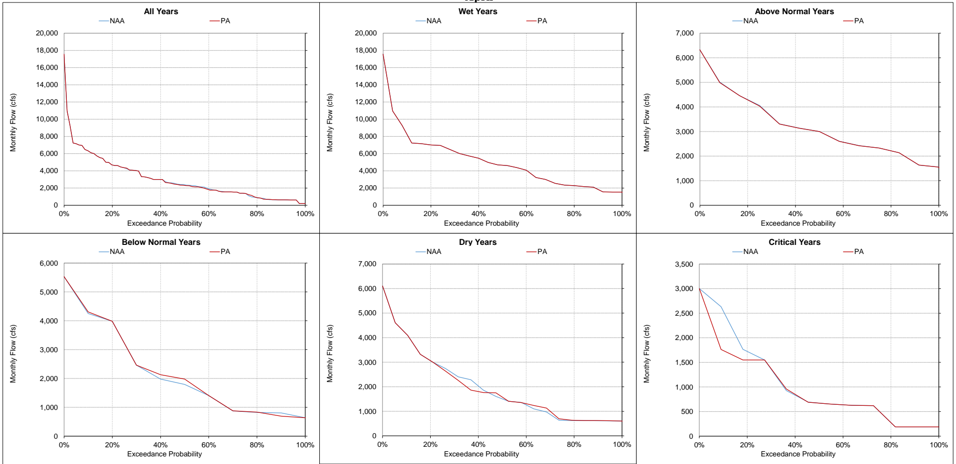
Figure 5.A.6-17-14. American River at Sacramento River Confluence, Monthly Flow April
