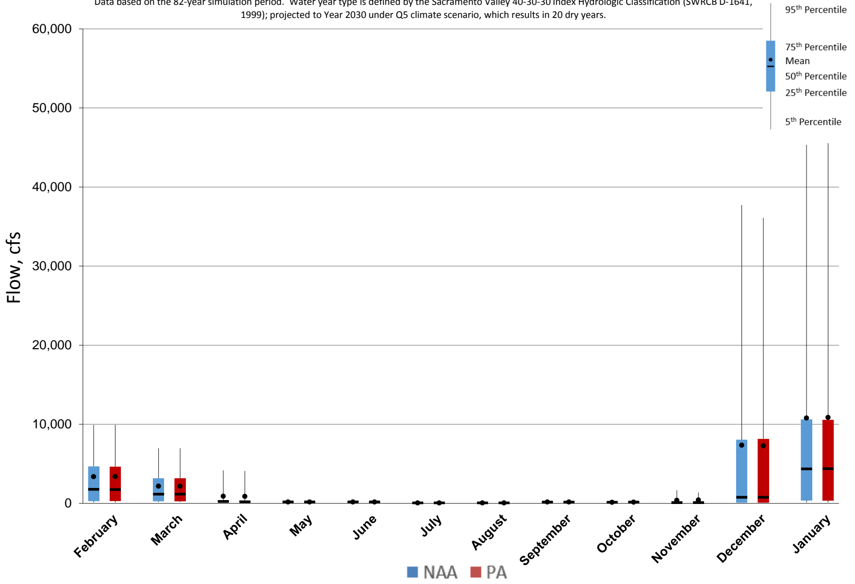
Figure 5.A.6-20-5. Monthly Flow Ranges For Yolo Bypass, Dry Years
