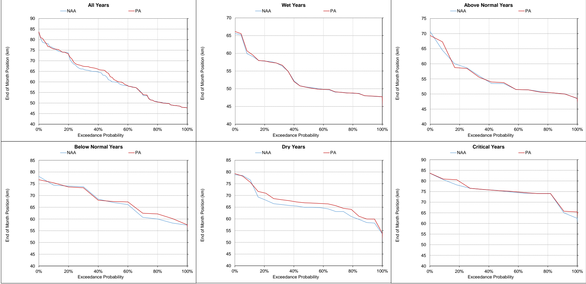
Figure 5.A.6-29-13. X2, End of Month Position March
