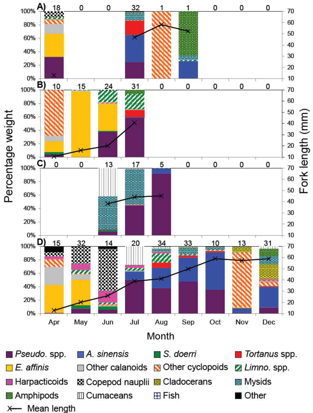
Figure 41. Percentage by weight of prey types found in stomachs of age-0 Delta Smelt collected from 1-6 ppt during April through December in A) 2005, B) 2006, C) 2010, and D) 2011. Number of stomachs examined are shown above the columns. Mean fork length (mm) of Delta Smelt is also shown.
