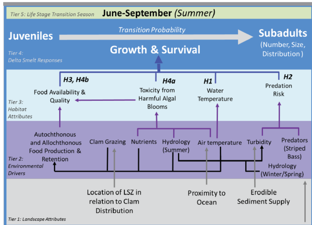
Figure 48. Conceptual model of drivers affecting the transition from Delta Smelt juveniles to subadults. Hypotheses addressed in Chapter 7 are indicated by the “H-number” combinations.
