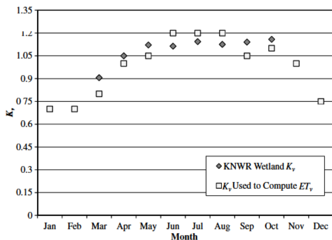
Fig. 4. Comparison of large stand wetland vegetation K_v from literature and computed using the surface energy balance (METRIC) with LandsAT 5 images for wetlands within Kern National Wildlife Refuge from March 2011 through October 2011
