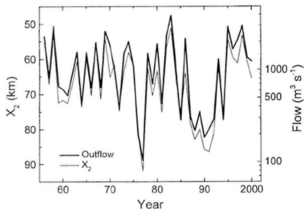
Fig. 3. Time series of X_2 (distance up the axis of the estuary to the 2 psu isohaline, thin line, left axis, scale reversed) and flow (heavy line, right axis, log scale), annual averages for January to June. Flow data from the California Department of Water Resources; X_2 calculated as in Jassby et al. (1995)
