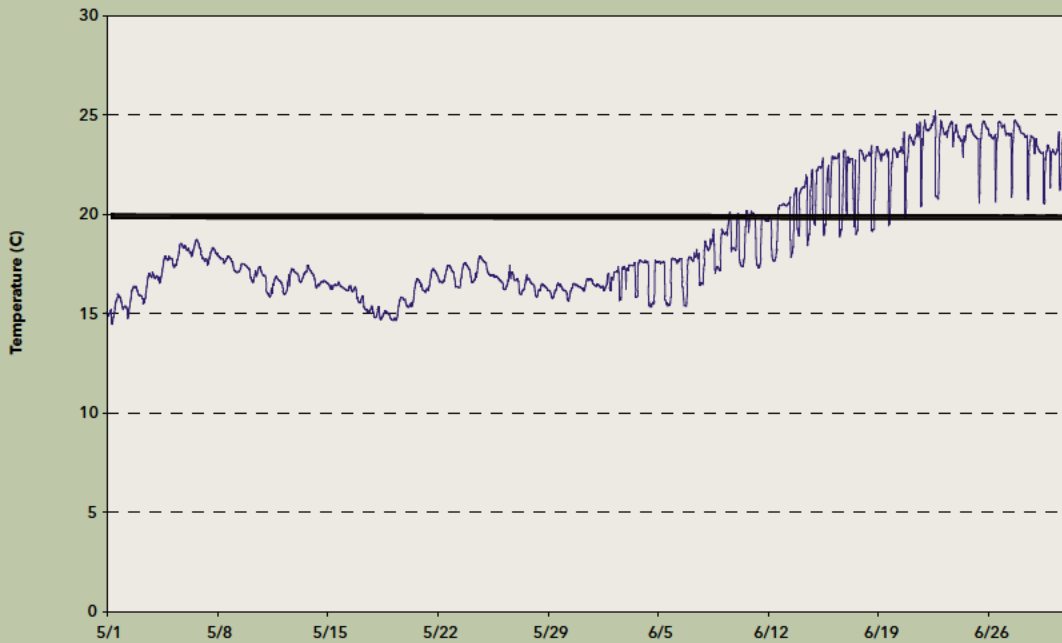
Appendix G, Figure 15 Daily Water Temperature Fluctuations (°C) in the South Delta Near the CCF Radial Gates During the 2011 Vernalis Adaptive Management Program (VAMP)
