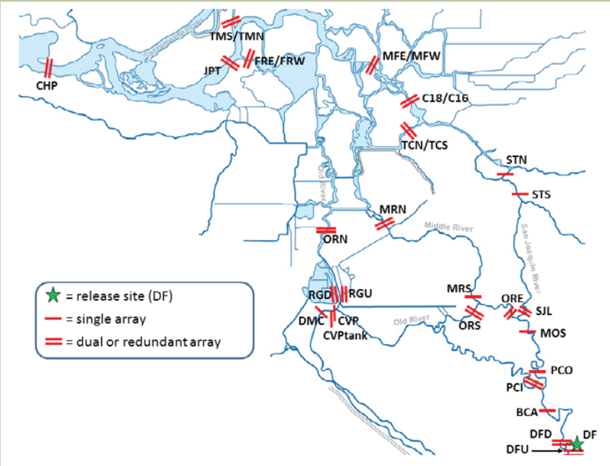
Figure 5-2 Locations of Acoustic Receivers and Release Site Used for the 2011 VAMP Study Including Locations of Acoustic Receivers Deployed by the California Department of Water Resources (DWR) for the South Delta Temporary Barriers Project Study. Site Descriptions, Locations and Codes are Shown in Table 5-6
