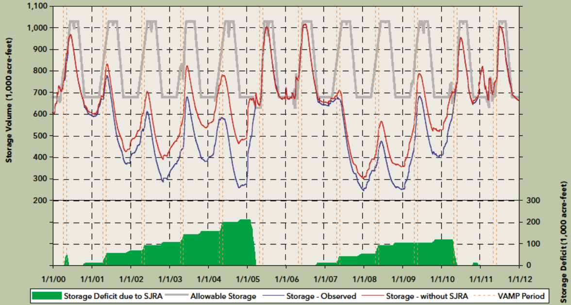
Appendix B, Figure 1 San Joaquin River Agreement (SJRA) Storage Impacts in Acre-Feet on Lake McClure (Merced River) from 2000-2011
