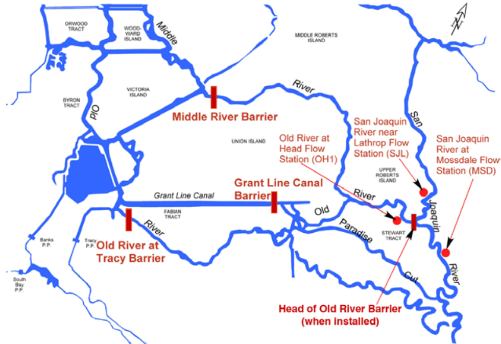
Figure 4-1 Location Map - South Delta Agricultural and Head of Old River Barriers
