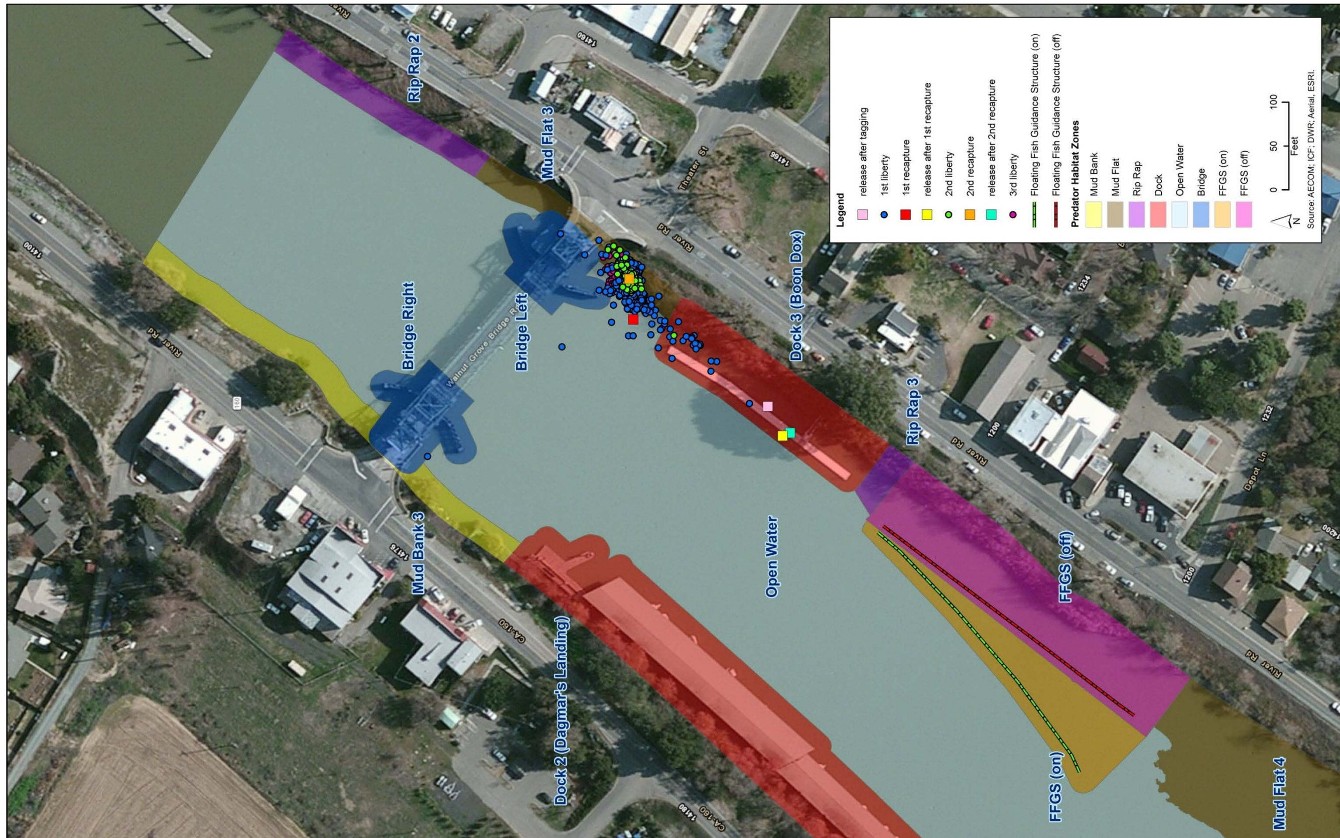
Figure 3.6-25 Detections of Micropterus spp. Tag # 4199
