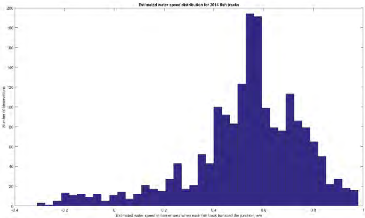
Figure 3.5-31 Estimated Water Speed Distribution for 2014 Study Fish
