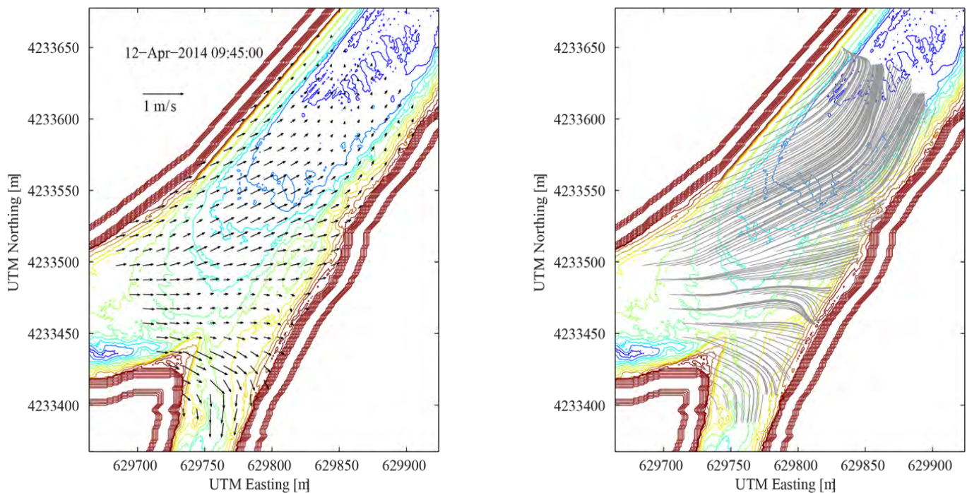
Figure 3.3-18 Plan View Plots during Typical Negative River Discharges—Velocity Vectors (on the left) and Particle Pathlines (on the right)—both Overlain on the Bathymetry Plot
