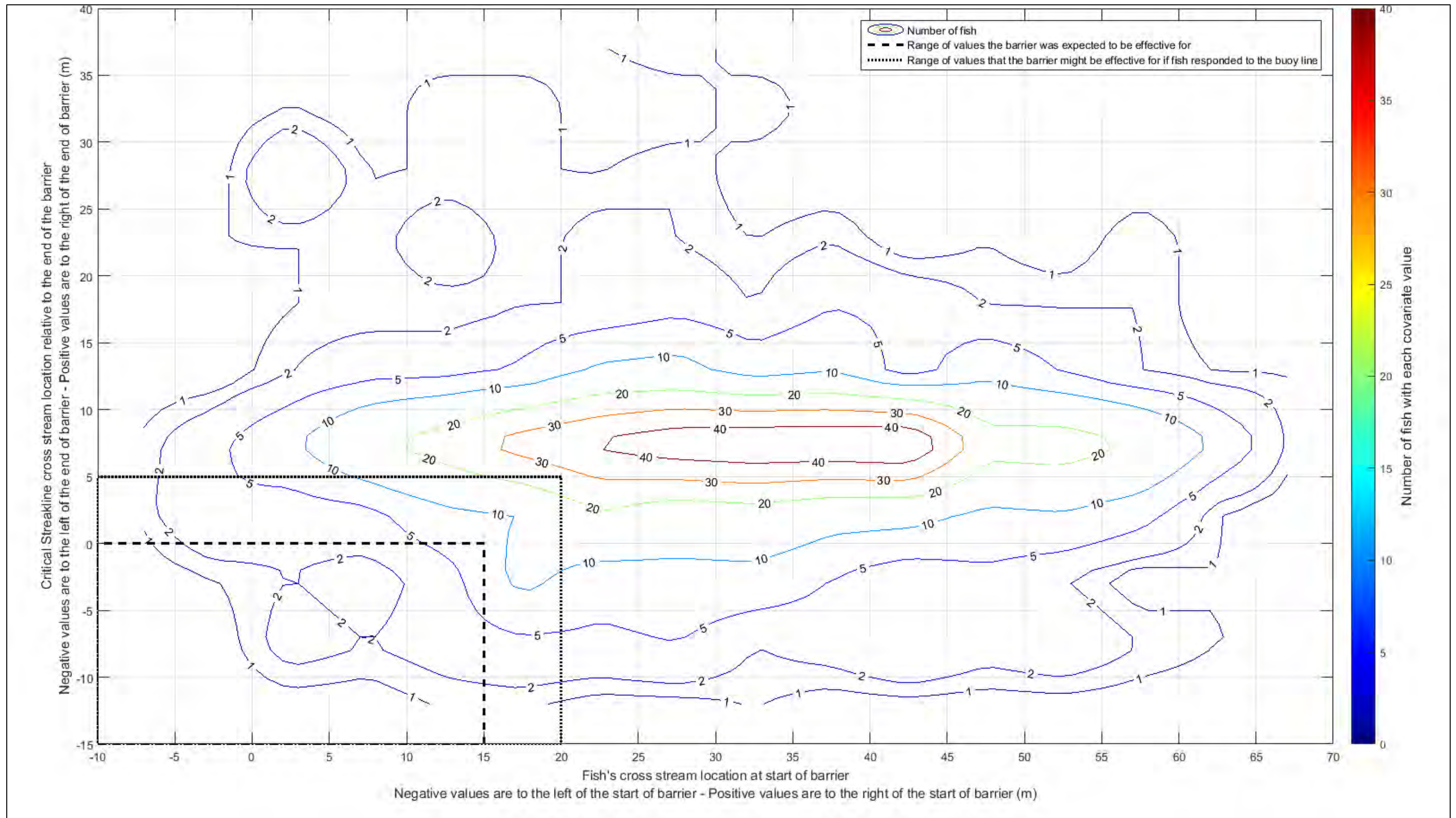
Figure 3.5-1 Contour Plot Showing Distribution of Cross-Stream Location and Critical Streakline Location for Study Fish Passing by the FFGS on Ebb Tides (FFGS On)
