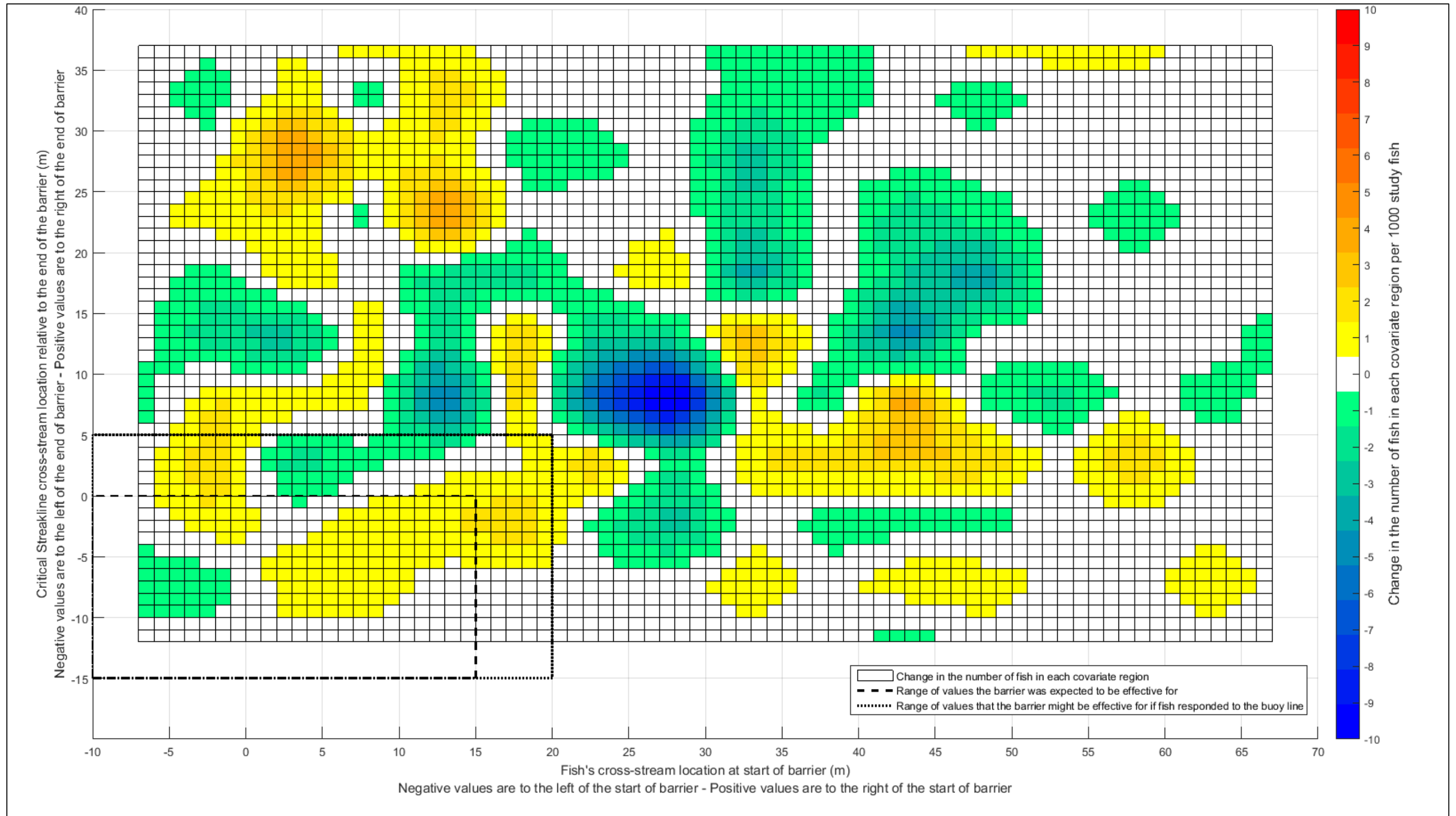
Figure 3.5-7 Flood Plot Showing the Change in the Number of Fish Entrained in Georgiana Slough for Cross-Stream and Critical Streakline Location (FFGS On and FFGS Off)
