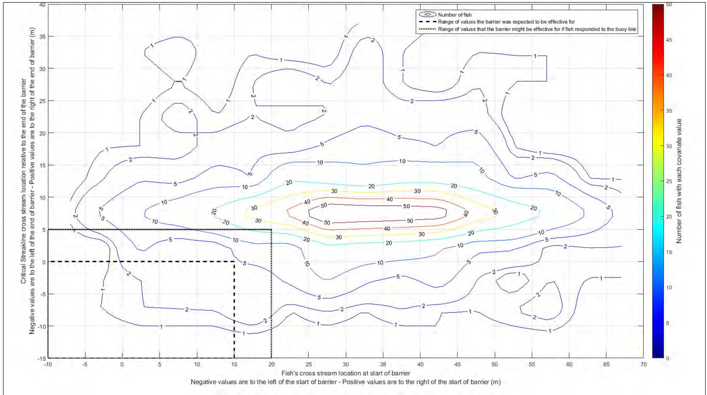
Figure 3.5-2 Contour Plot Showing Distribution of Cross-Stream Location and Critical Streakline Location for Study Fish Passing by the FFGS on Ebb Tides (FFGS Off)
