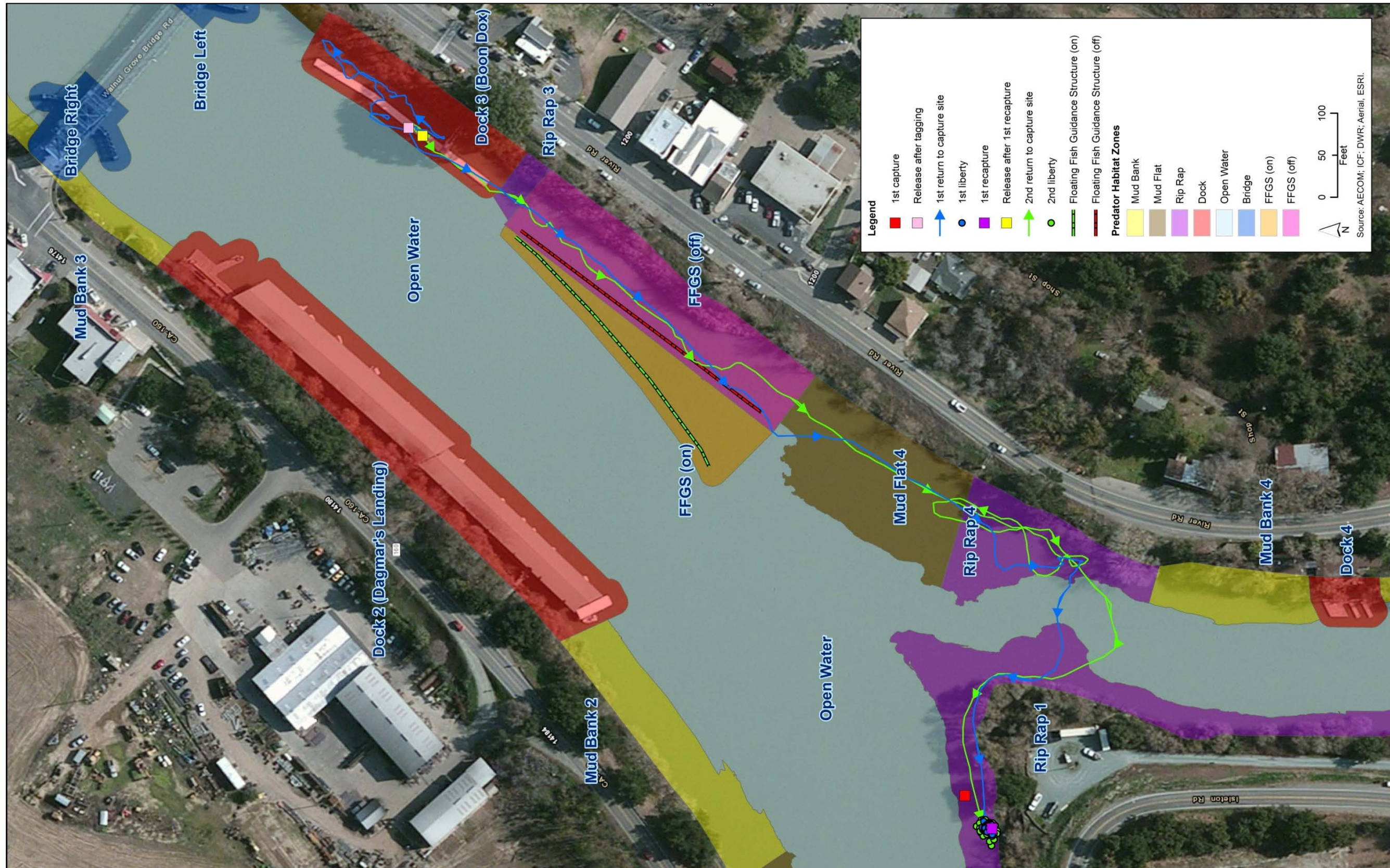
Figure 3.6-26 Detections of Micropterus spp. Tag # 3947
