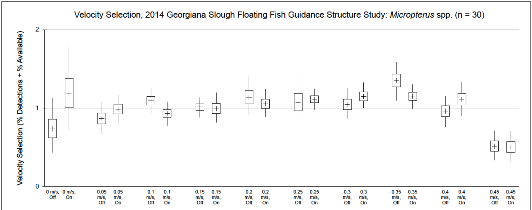
Figure 3.6-23 Micropterus spp.: Velocity Selection with FFGS On/Off
