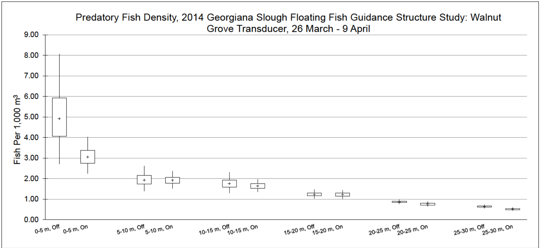
Figure 3.6-43 Predatory Fish Density Estimated by the Walnut Grove Split-Beam Transducer, March 26 to April 9, 2014
