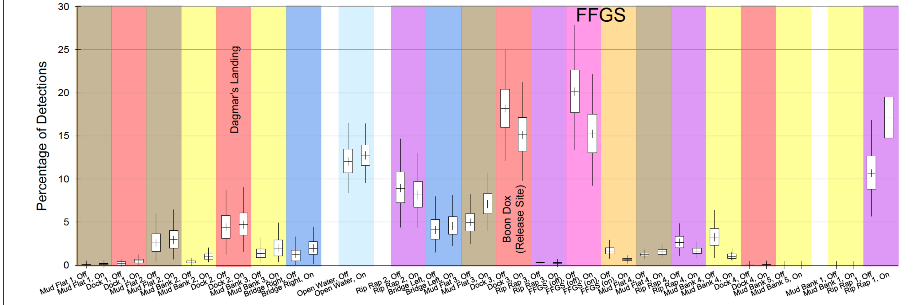
Figure 3.6-20 Micropterus spp.: Percentage of Detections by Habitat Zone with FFGS On/Off
