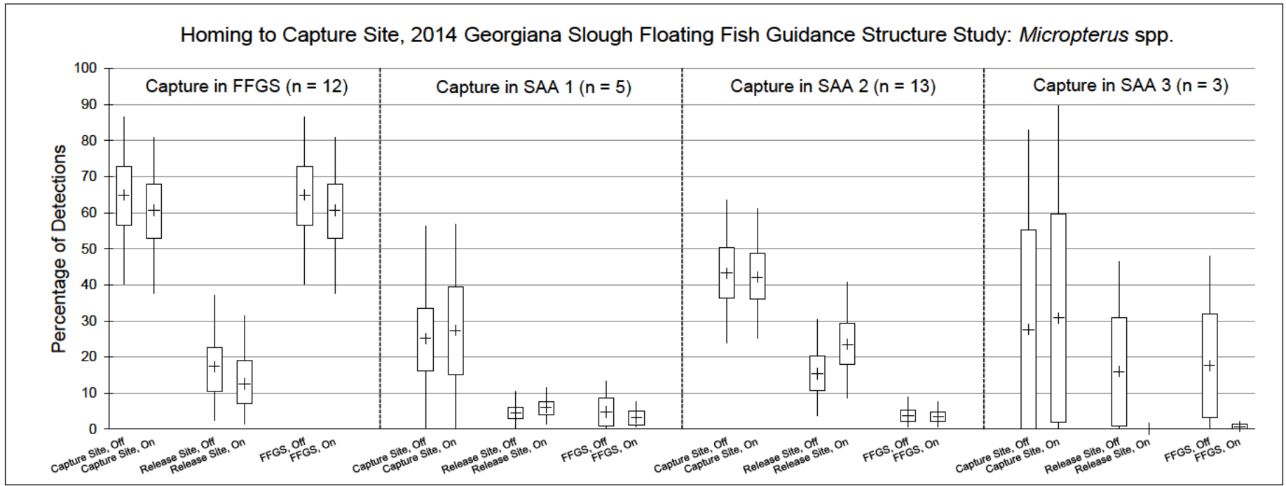
Figure 3.6-24 Micropterus spp.: Percentage of Detections near Capture Site, Release Site, and FFGS with FFGS On/Off
