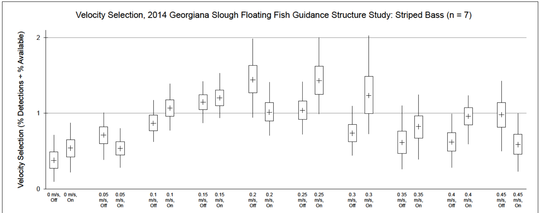
Figure 3.6-22 Striped Bass: Velocity Selection with FFGS On/Off
