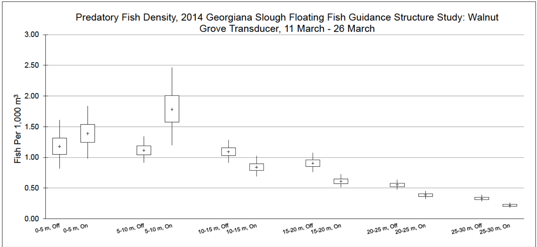
Figure 3.6-42 Predatory Fish Density Estimated by the Walnut Grove Split-Beam Transducer, March 11 to 26, 2014
