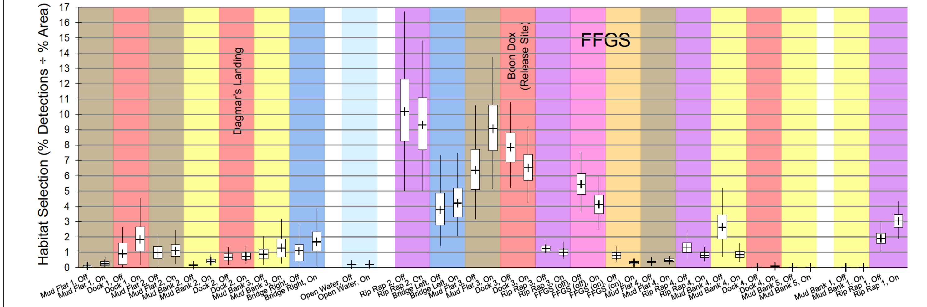
Figure 3.6-21 Micropterus spp.: Habitat Selection with FFGS On/Off
