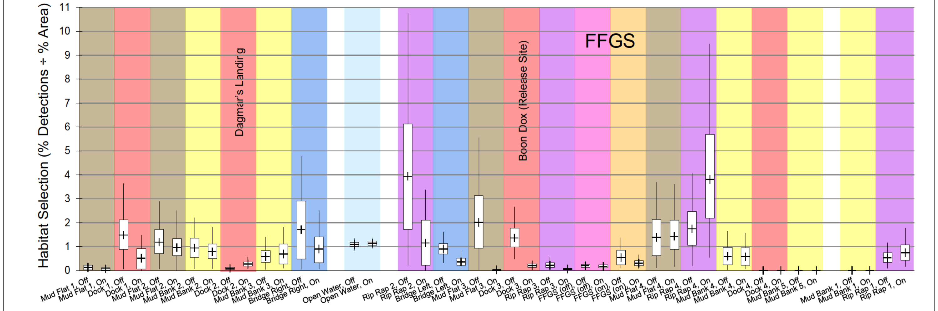
Figure 3.6-19 Striped Bass: Habitat Selection with FFGS On/Off
