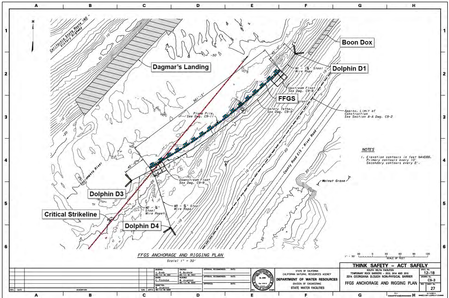
Figure 2-4 2014 Floating Fish Guidance Structure Layout Plan
