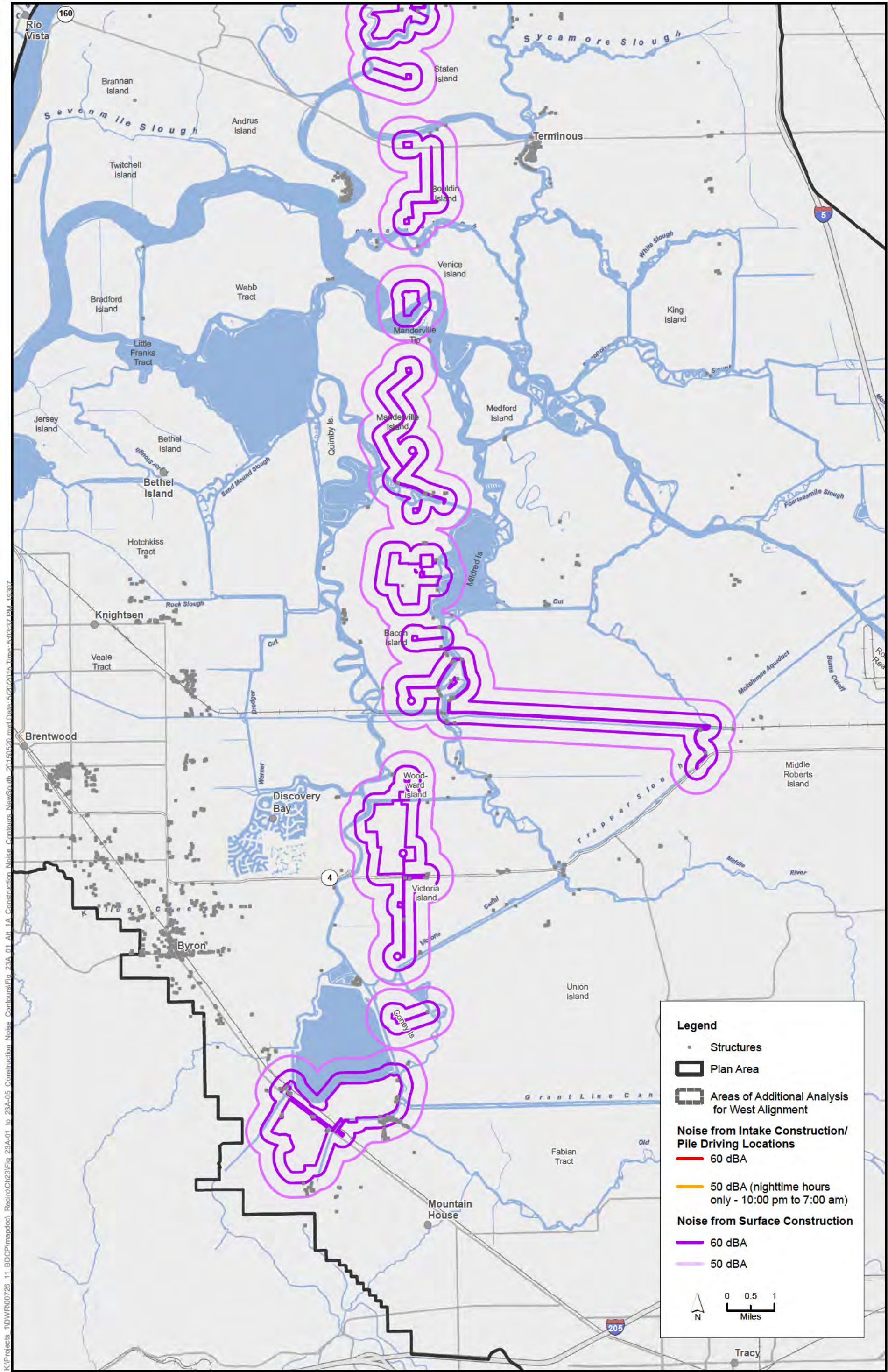
Figure 23A-01 Alternative 1A - Modified Pipeline/Tunnel Option Construction Noise Contours (South)
