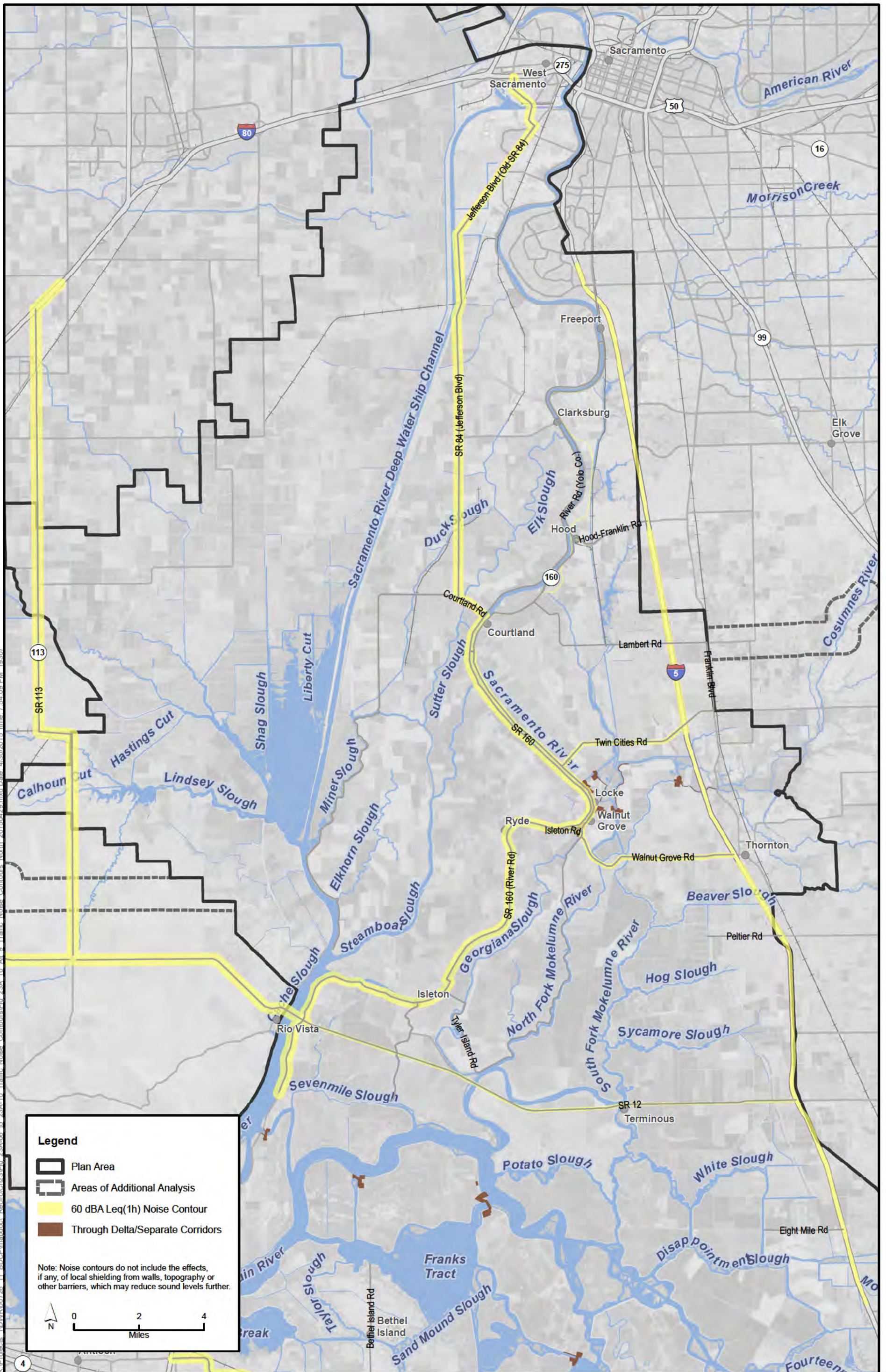
Figure 23A-12 Alternative 9 - Separate Corridors Option Traffic Noise Contours on Worker Commuter Roads and Haul Routes (North)
