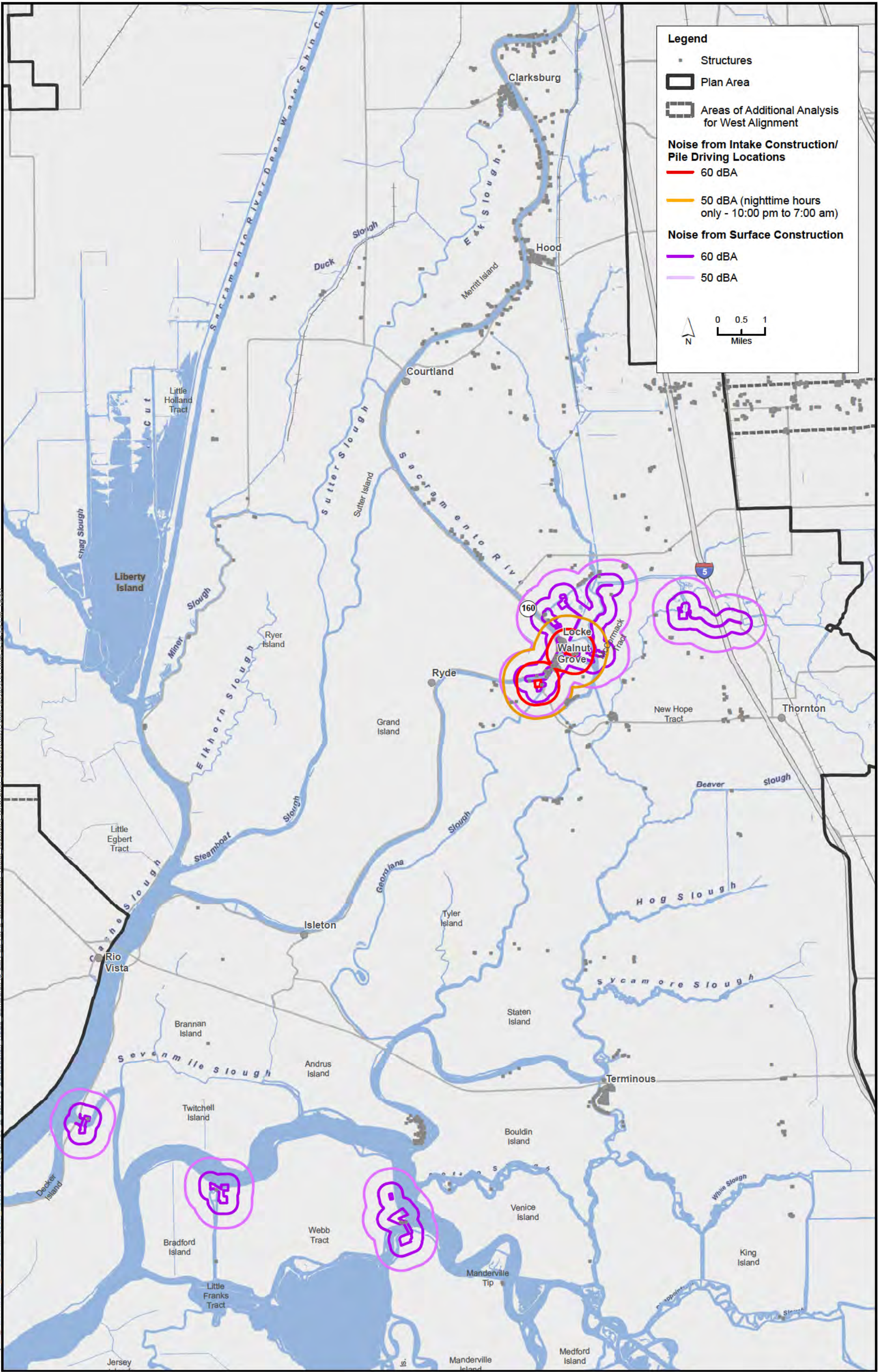
Figure 23A-05 Alternative 9 - Separate Corridors Option Construction Noise Contours (North)
