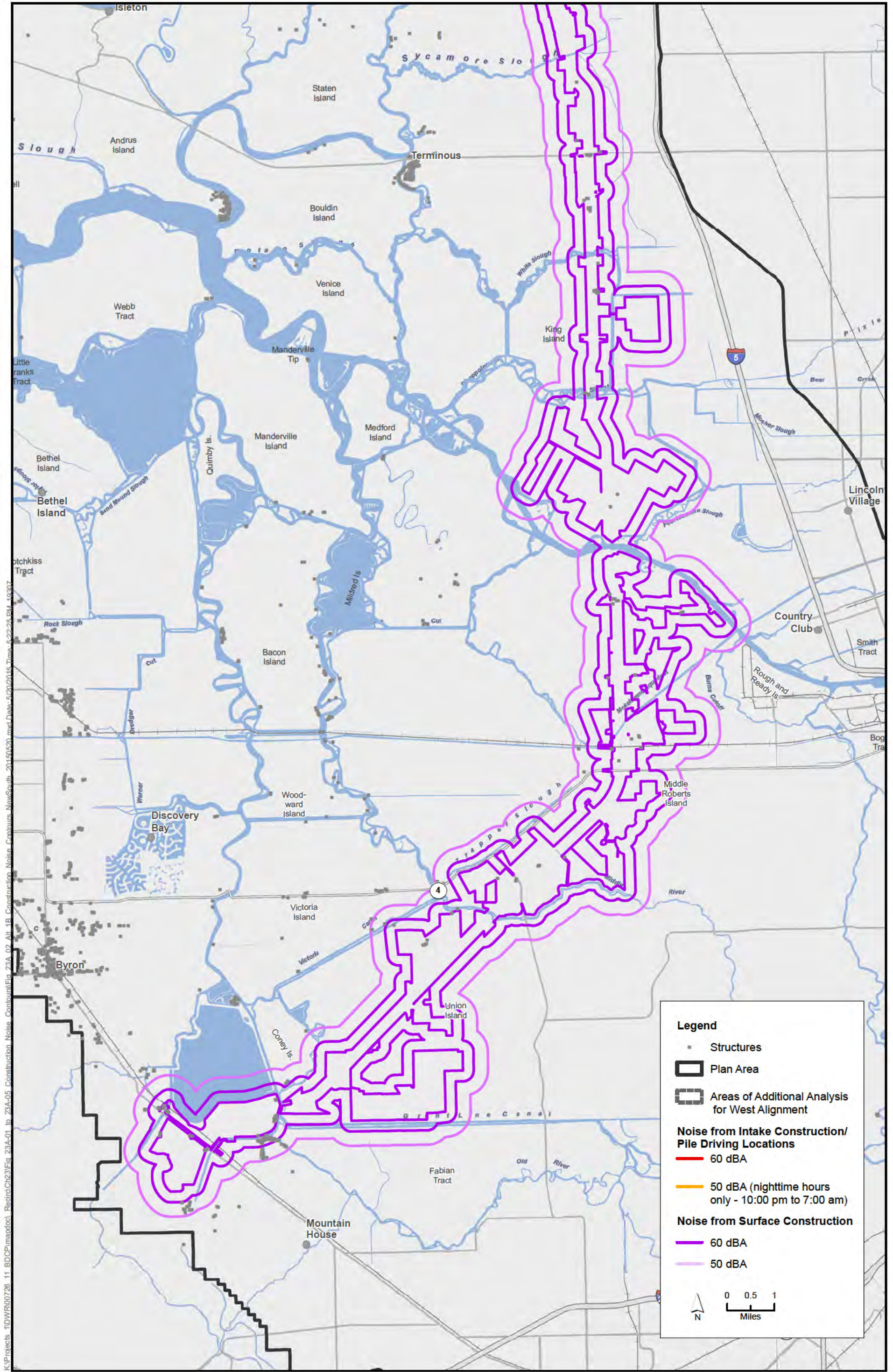
Figure 23A-02 Alternative 1B - East Option Construction Noise Contours (South)
