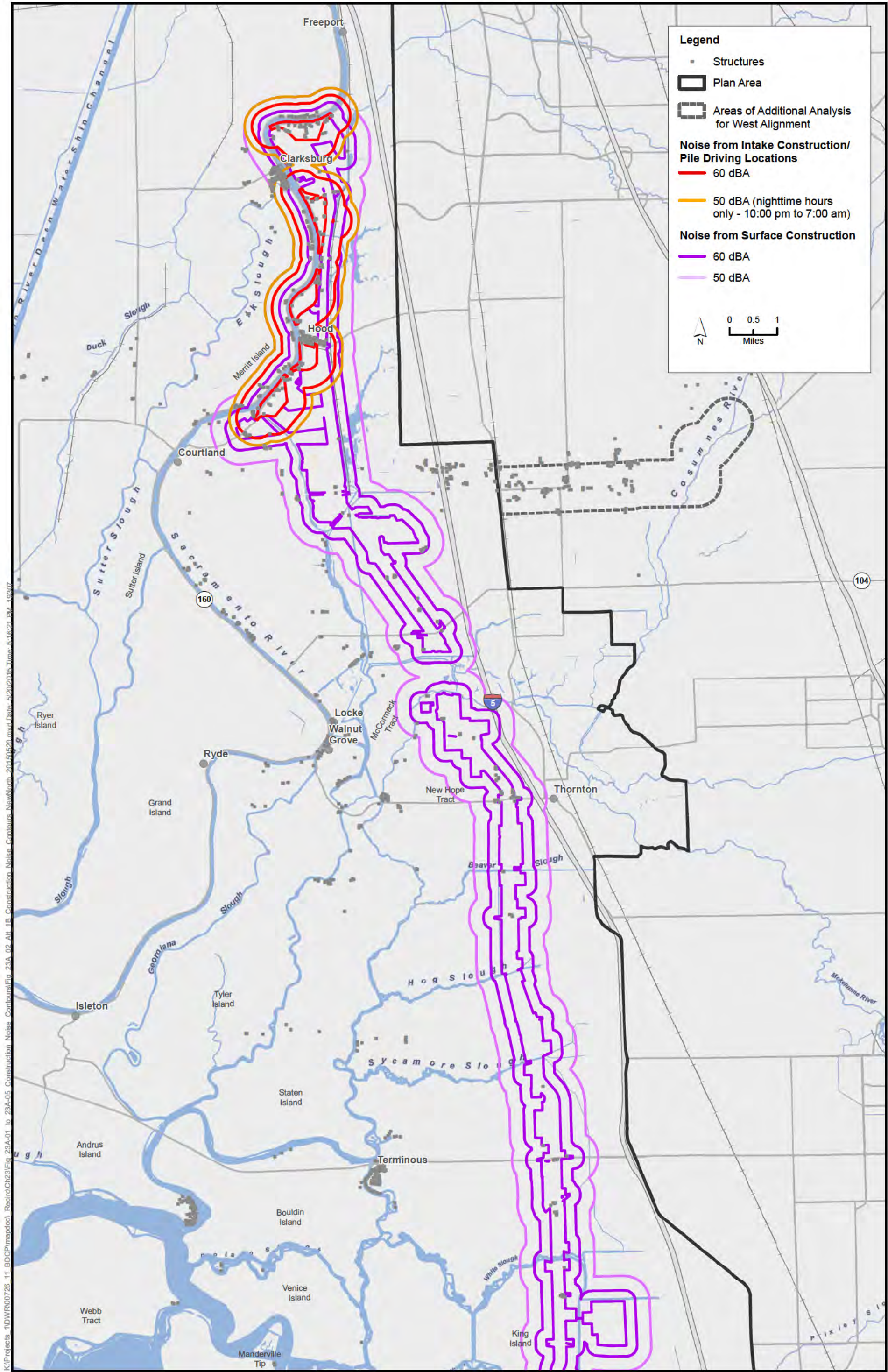
Figure 23A-02 Alternative 1B - East Option Construction Noise Contours (North)
