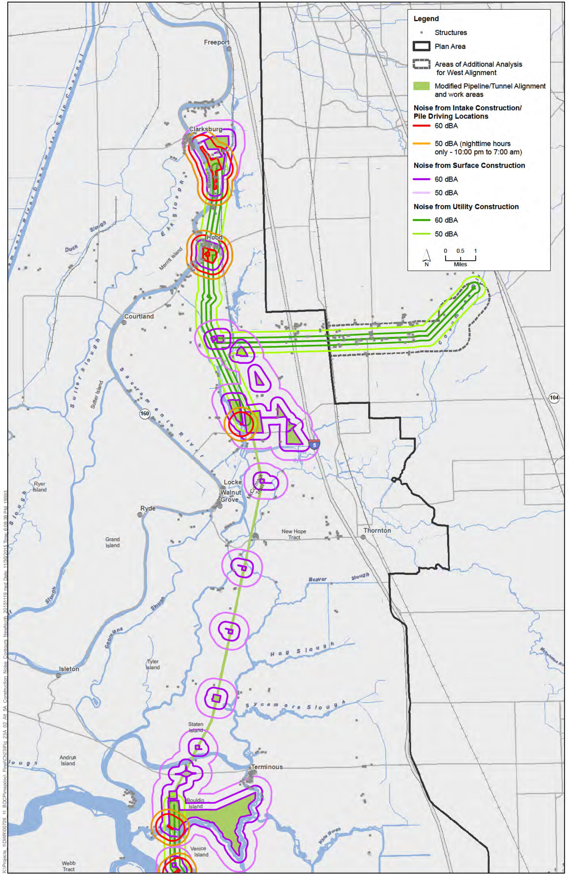
Figure 23A-07 Alternative 5A - Modified Pipeline/Tunnel Option Construction Noise Contours (North)
