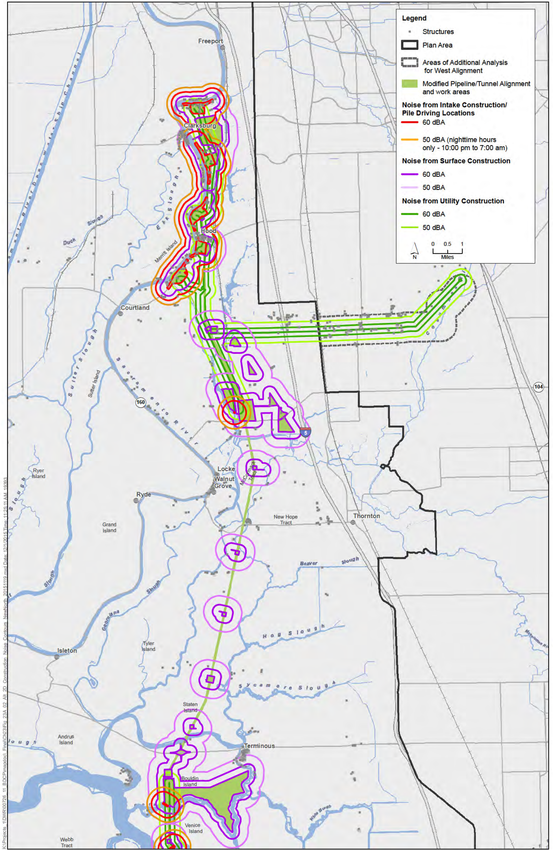
Figure 23A-06 Alternative 2D - Modified Pipeline/Tunnel Option Construction Noise Contours (North)
