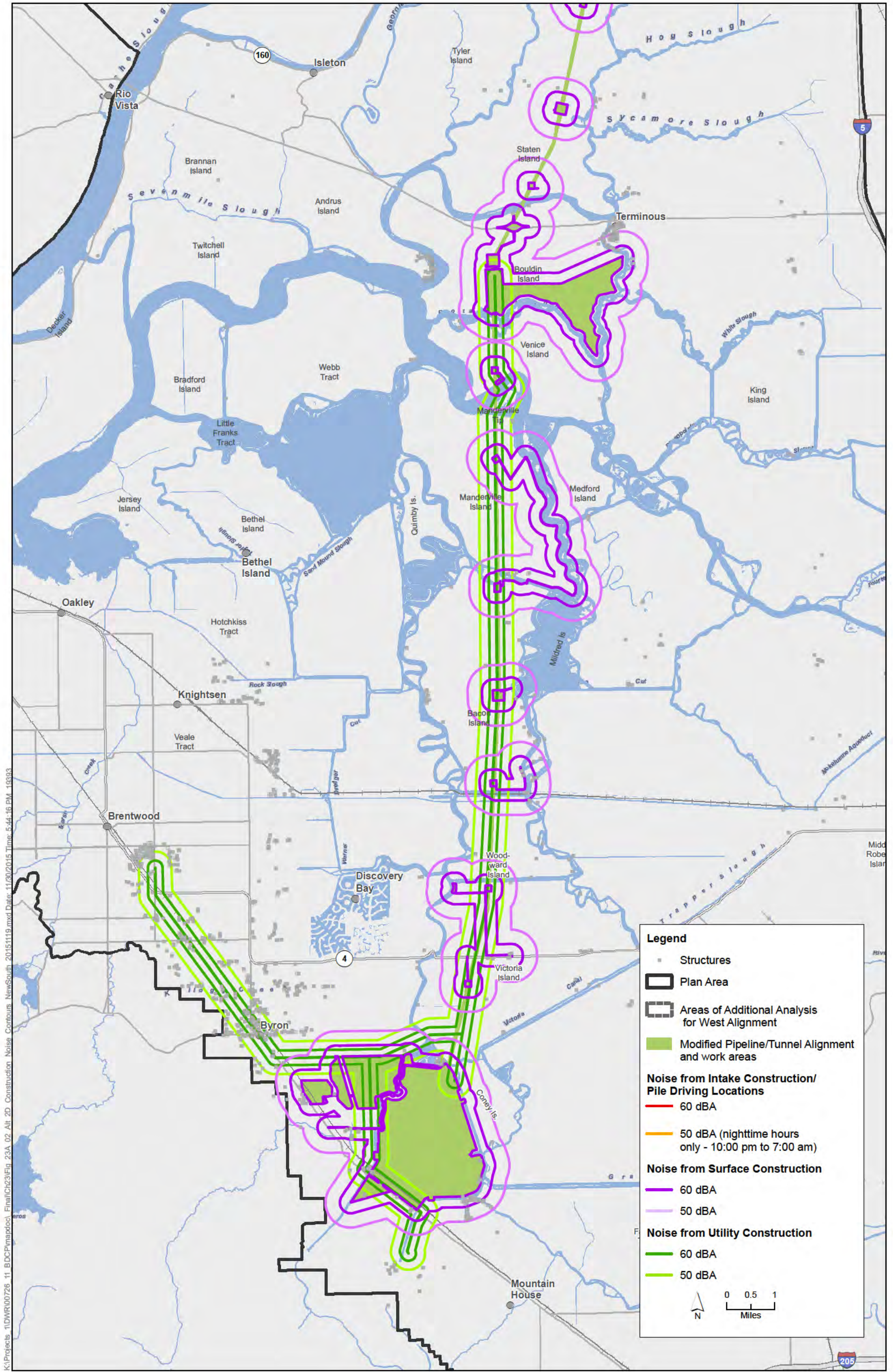
Figure 23A-06 Alternative 2D - Modified Pipeline/Tunnel Option Construction Noise Contours (South)
