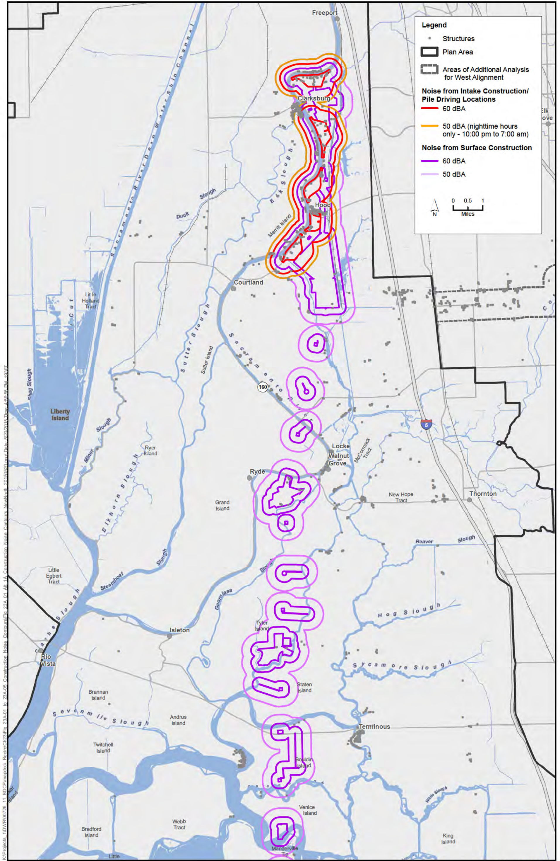
Figure 23A-01 Alternative 1A - Pipeline/Tunnel Option Construction Noise Contours (North)
