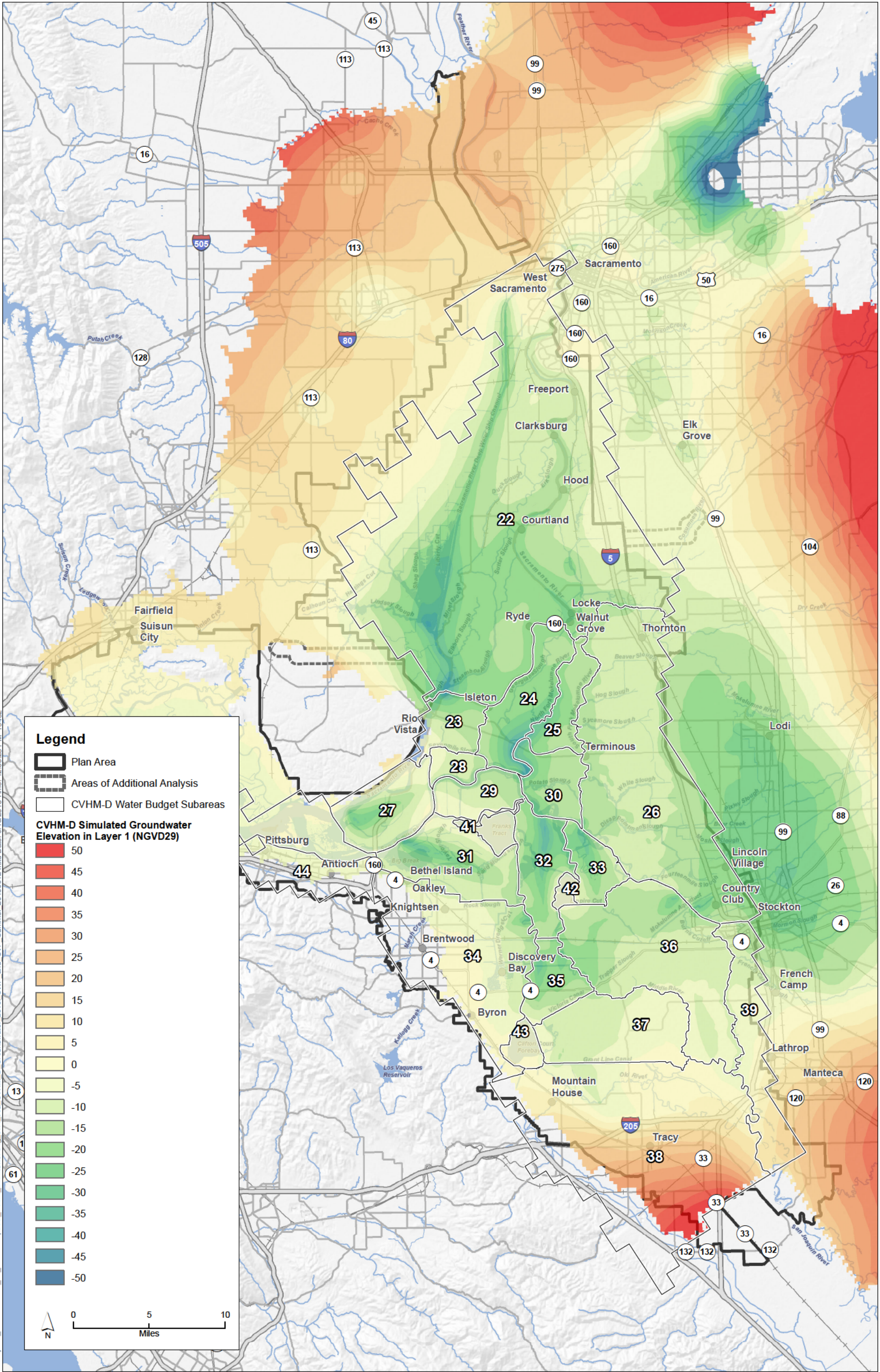
Figure 7A-5a CVHM-D Typical Groundwater Level Contour Map for the Delta Region — Summer
