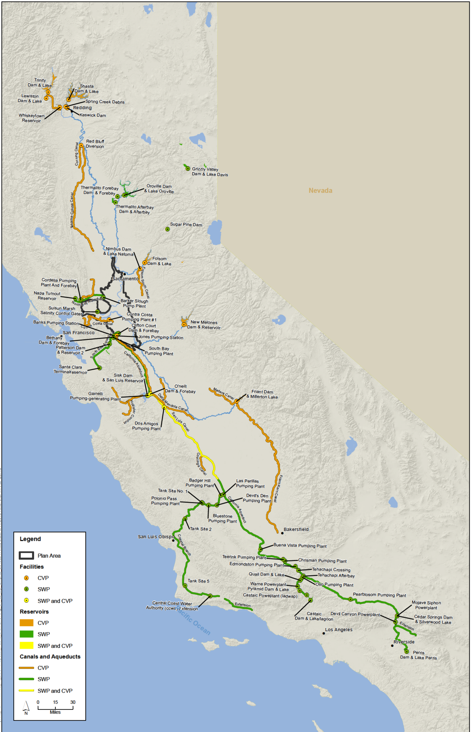
Figure 1-2 Major Components of the SWP and CVP
