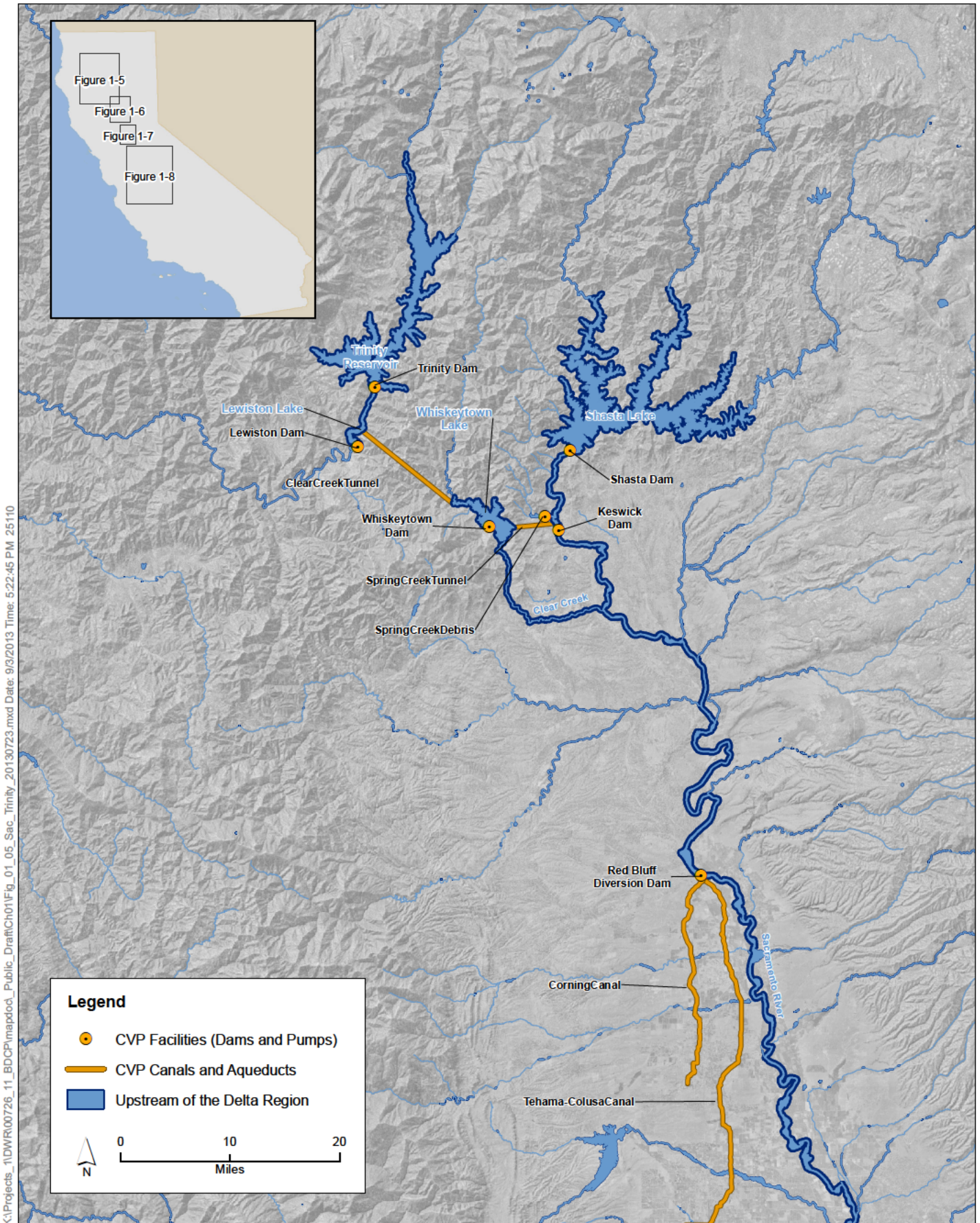
Figure 1-5 Upstream of the Delta Region— Sacramento River and Trinity System (CVP Facilities)
