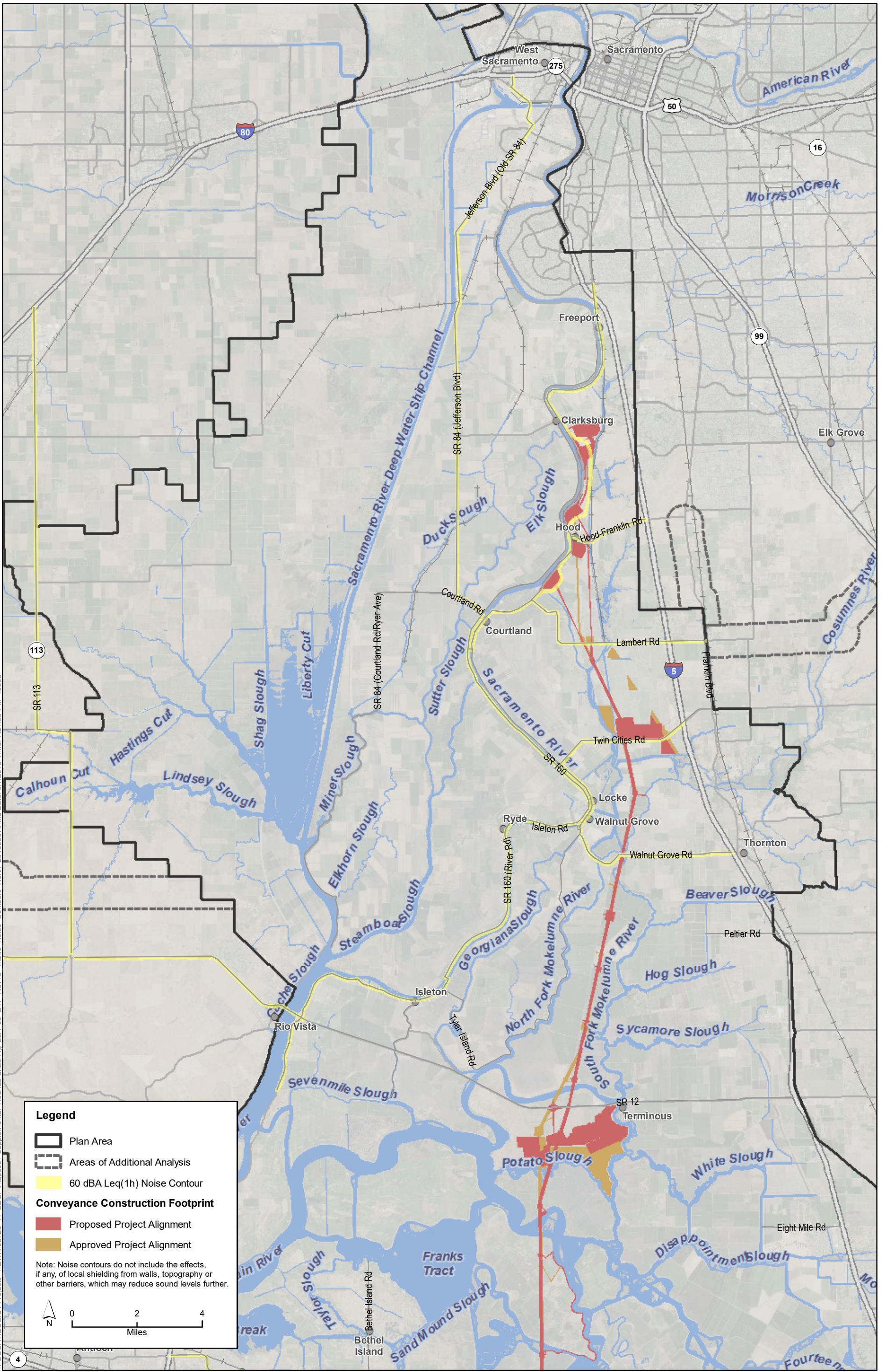
Figure 23A-09 Alternative BTF Rev1e - Project Alignment Traffic Noise Contours on Worker Commuter Roads and Haul Routes (North)
