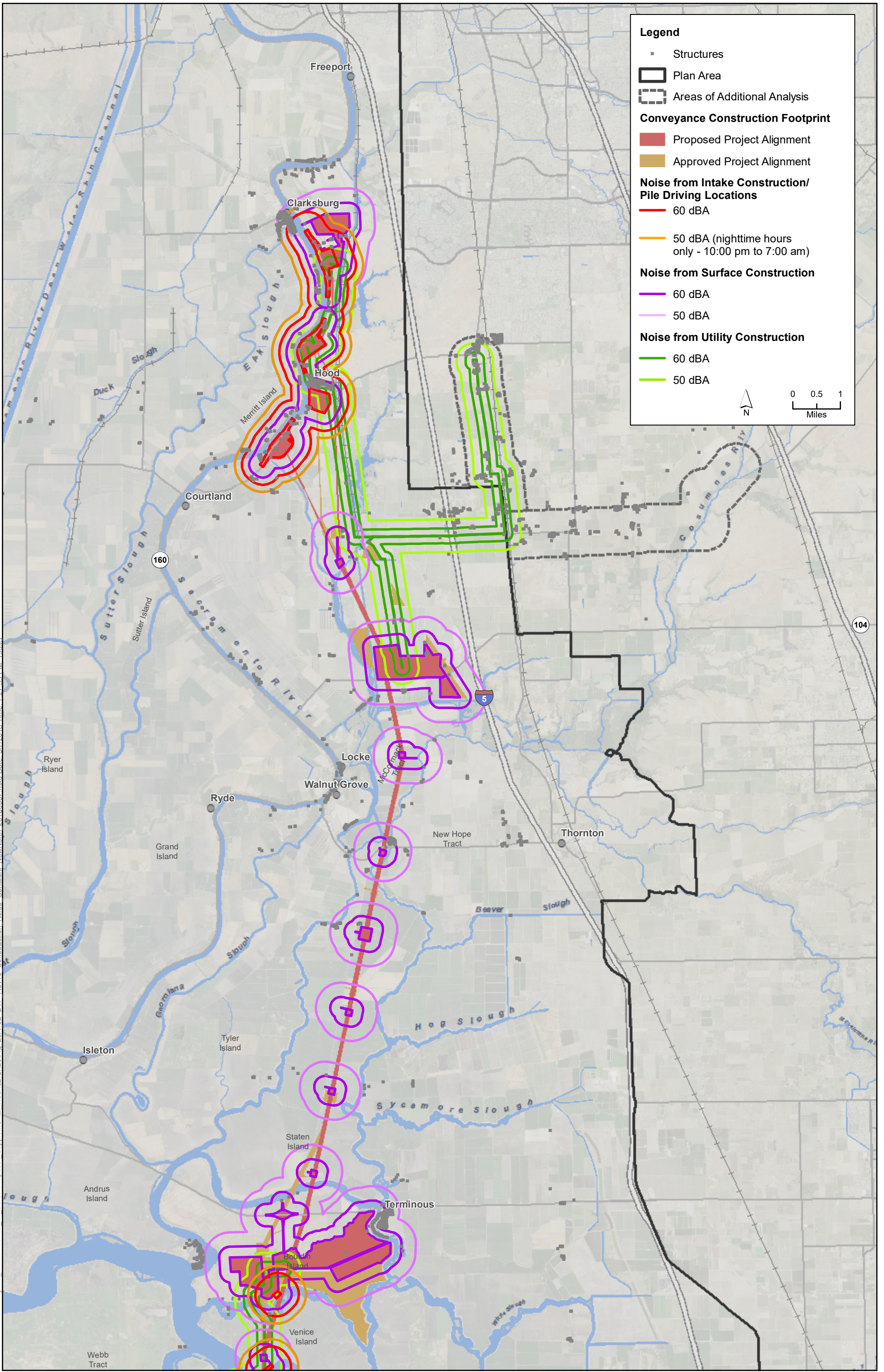
Figure 23A-04 Alternative BTF Rev1e - Project Alignment Construction Noise Contours (North)
