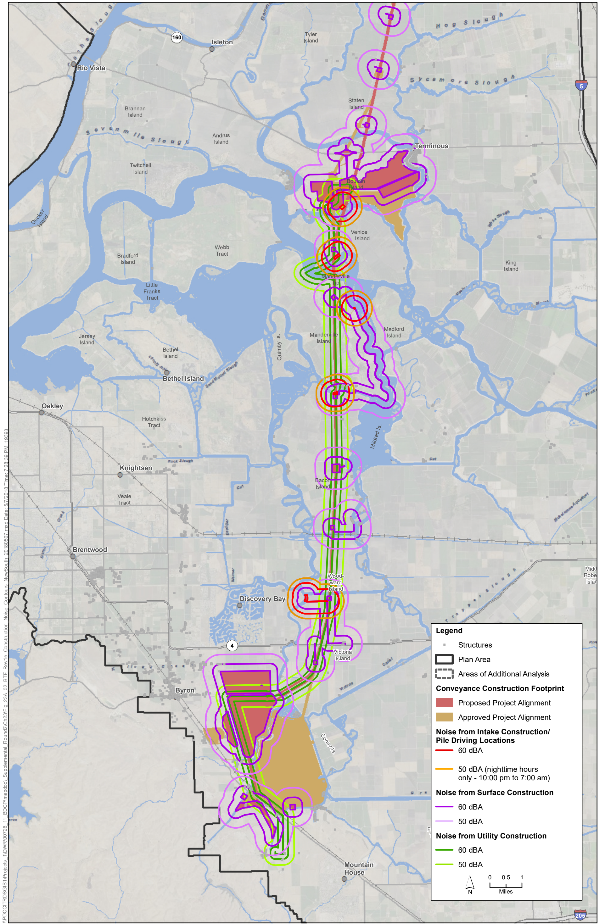
Figure 23A-04 Alternative BTF Rev1e - Project Alignment Construction Noise Contours (South)
