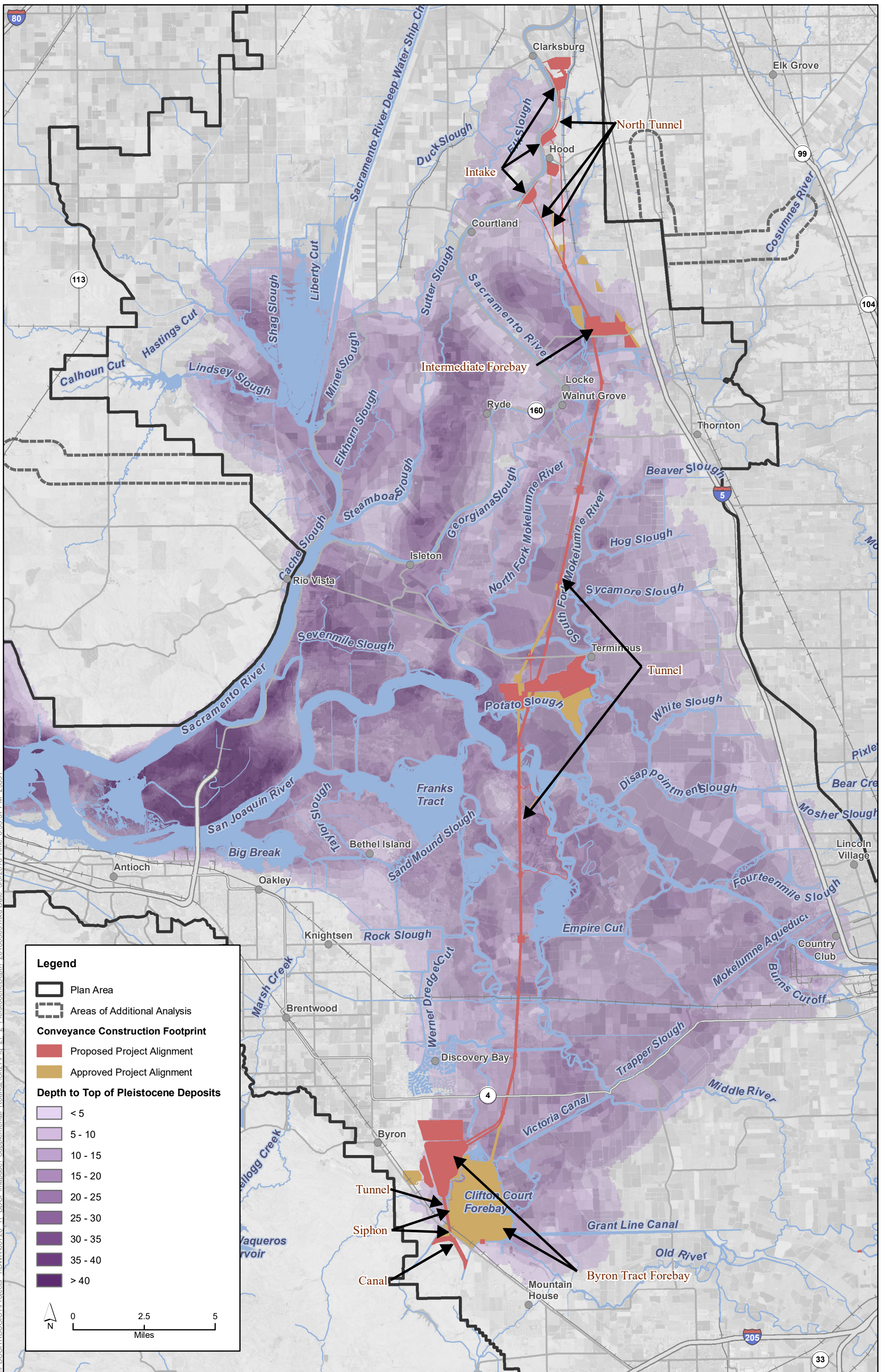
Figure 27-2 Depth to Top of Pleistocene Deposits
