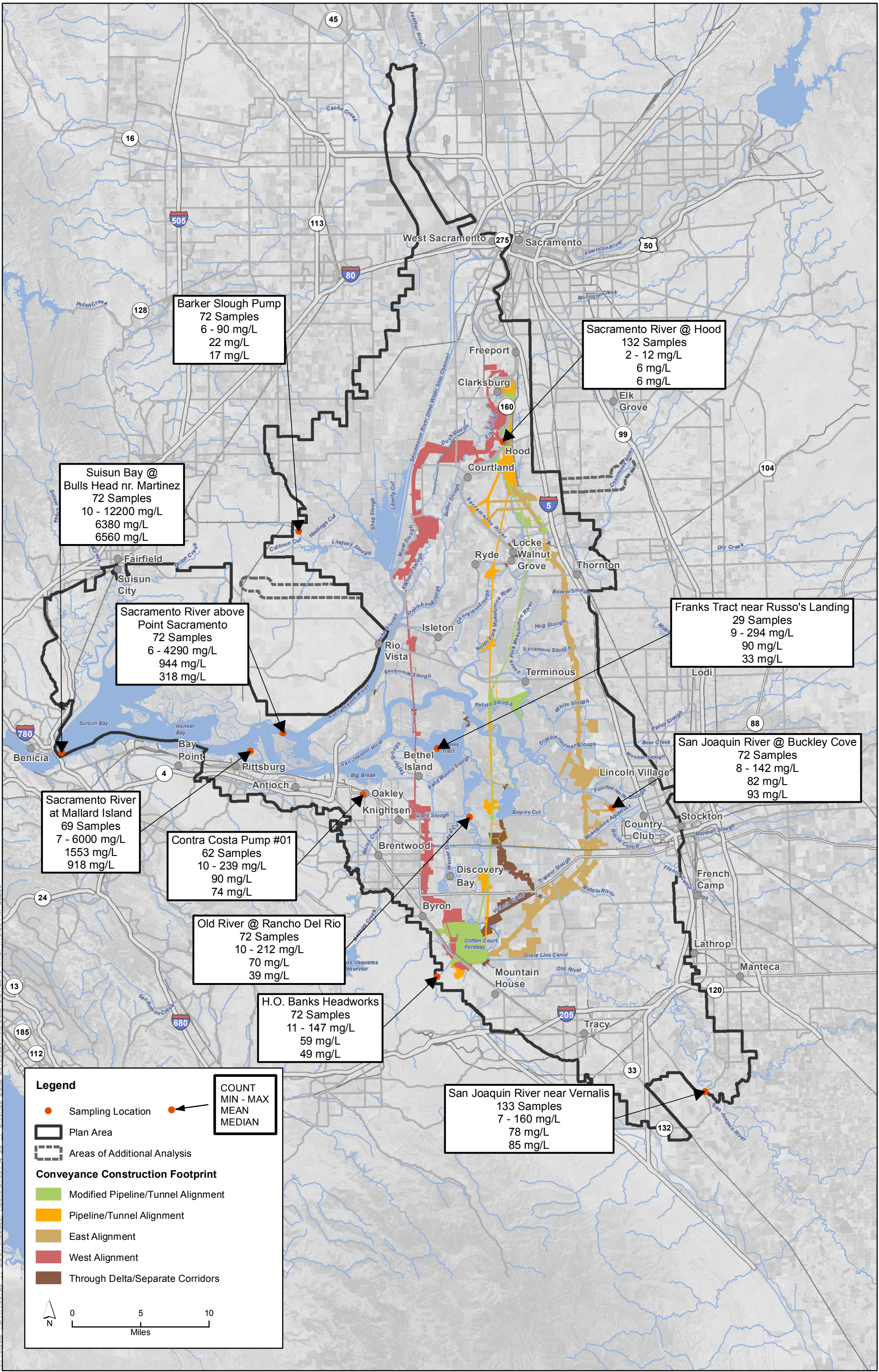
Figure 8-17 Spatial Summary of Chloride Data at Delta Stations (2001 - 2006)
