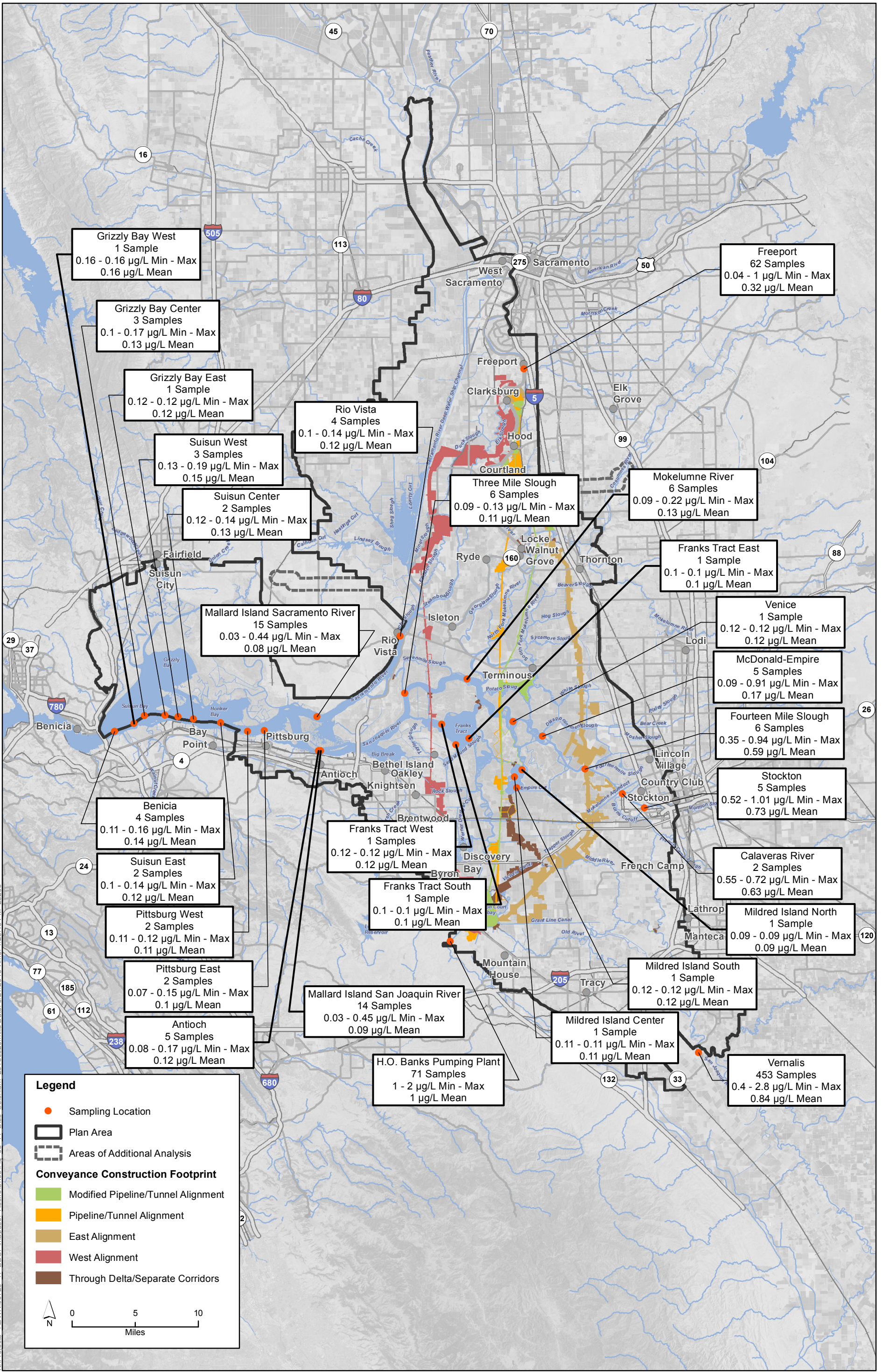
Figure 8-44 Spatial Summary of Dissolved Selenium Data (1999 - 2008)
