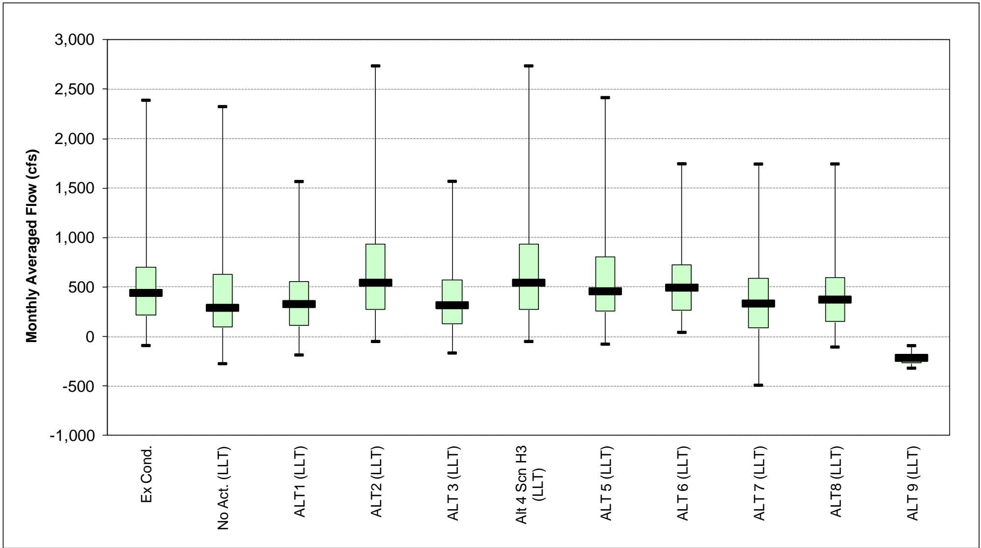
Figure 8-65. Monthly average flow in the San Joaquin River at Stockton for May-October of Dry and Critical water year types for Existing Conditions, No Action Alternative, and Alternatives 1-9. Shown are the maximum, 75th percentile, median, 25th percentile, and minimum flows.
