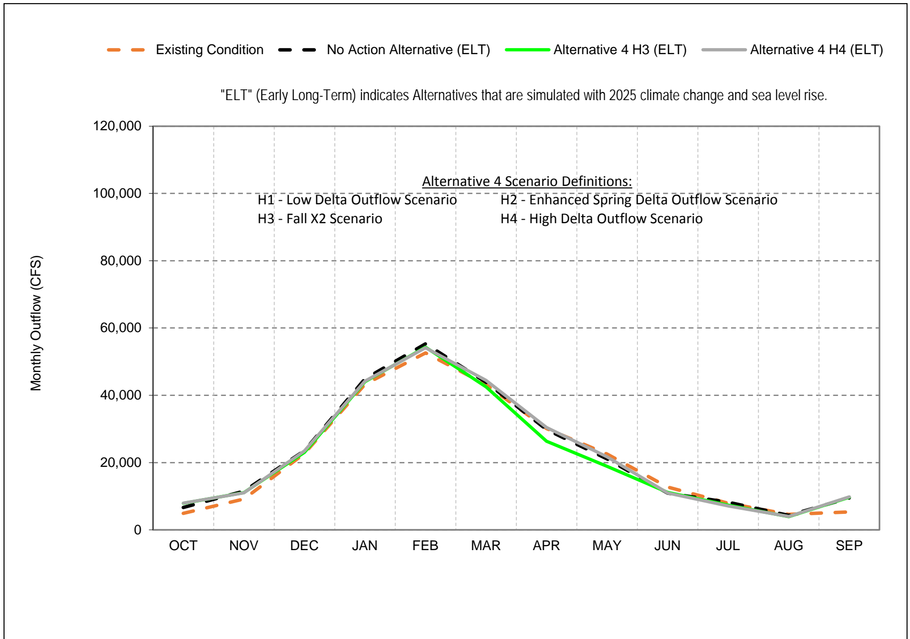
Figure 4.3.1-1 Sacramento/San Joaquin River Monthly Average Delta Outflow for Alternative 4A
