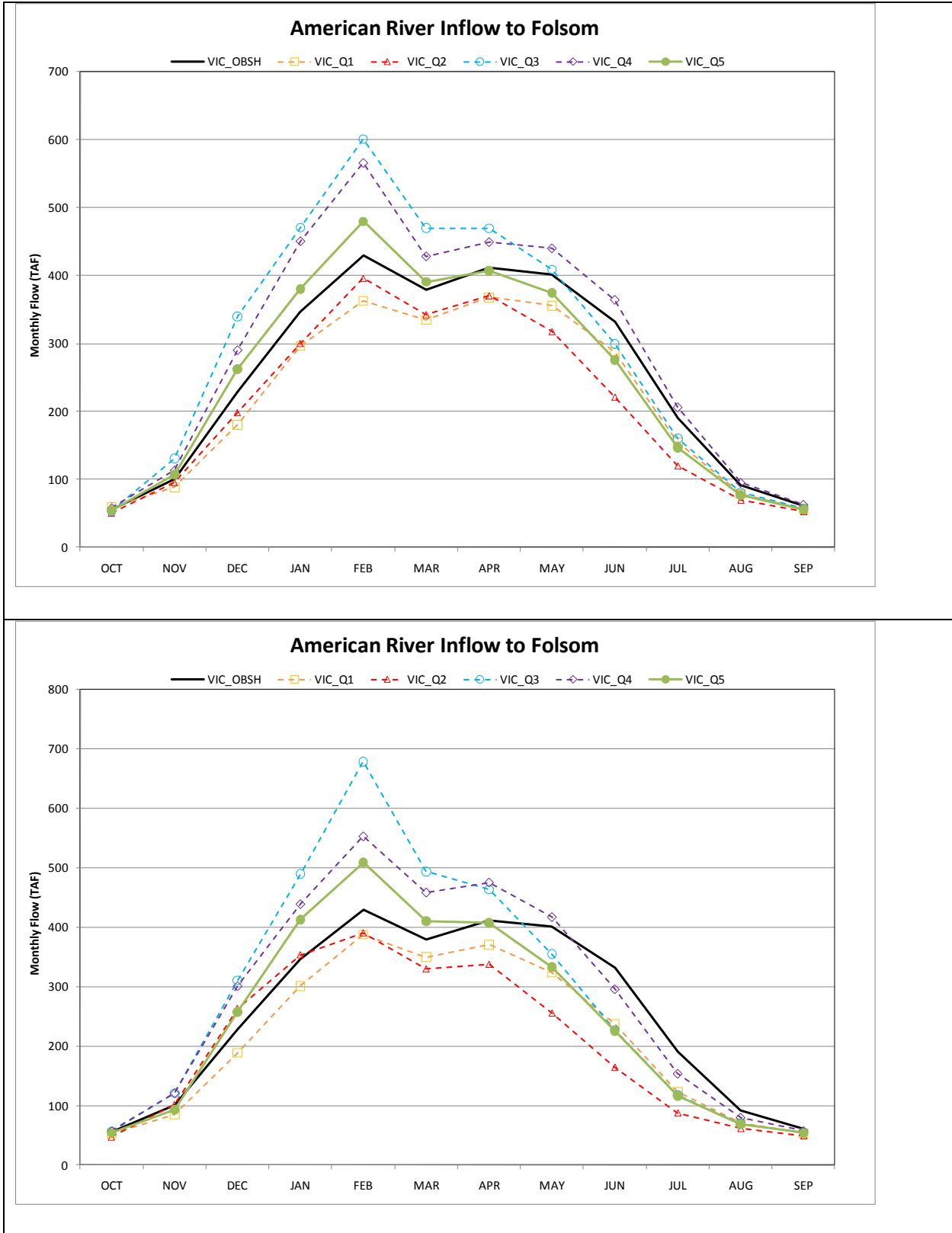
Figure 5.A.A.2-11. Simulated Changes in Monthly Natural Streamflow for American River Inflow to Folsom (top, 2025 changes; bottom, 2060 changes).
