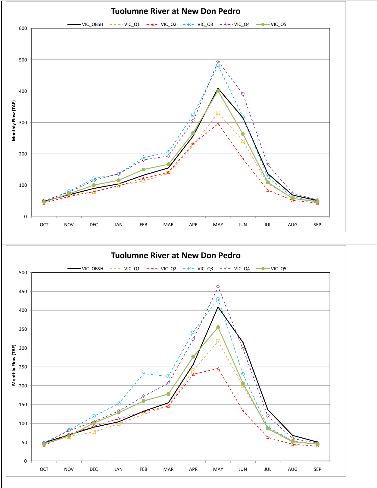
Figure 5.A.A.2-13. Simulated Changes in Monthly Natural Streamflow for Tuolumne River at New Don Pedro (top, 2025 changes; bottom, 2060 changes).
