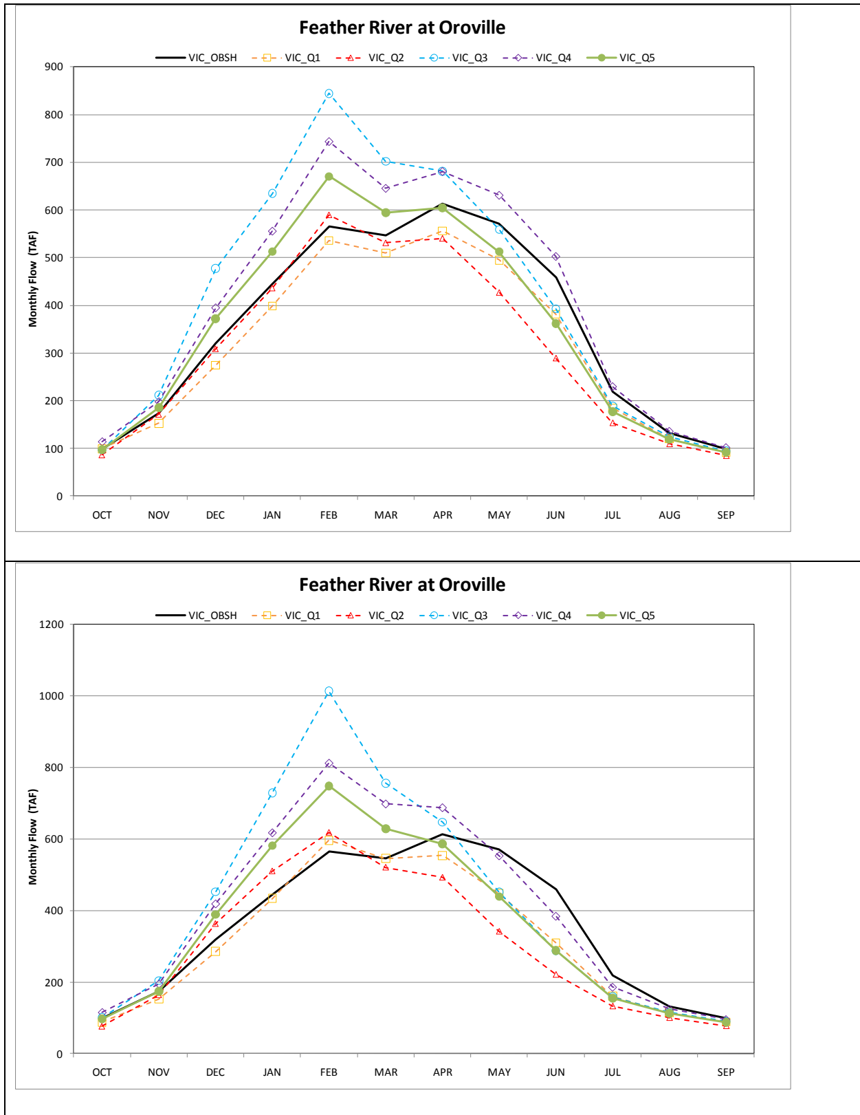
Figure 5.A.A.2-9. Simulated Changes in Monthly Natural Streamflow for Feather River at Oroville (top, 2025 changes; bottom, 2060 changes).
