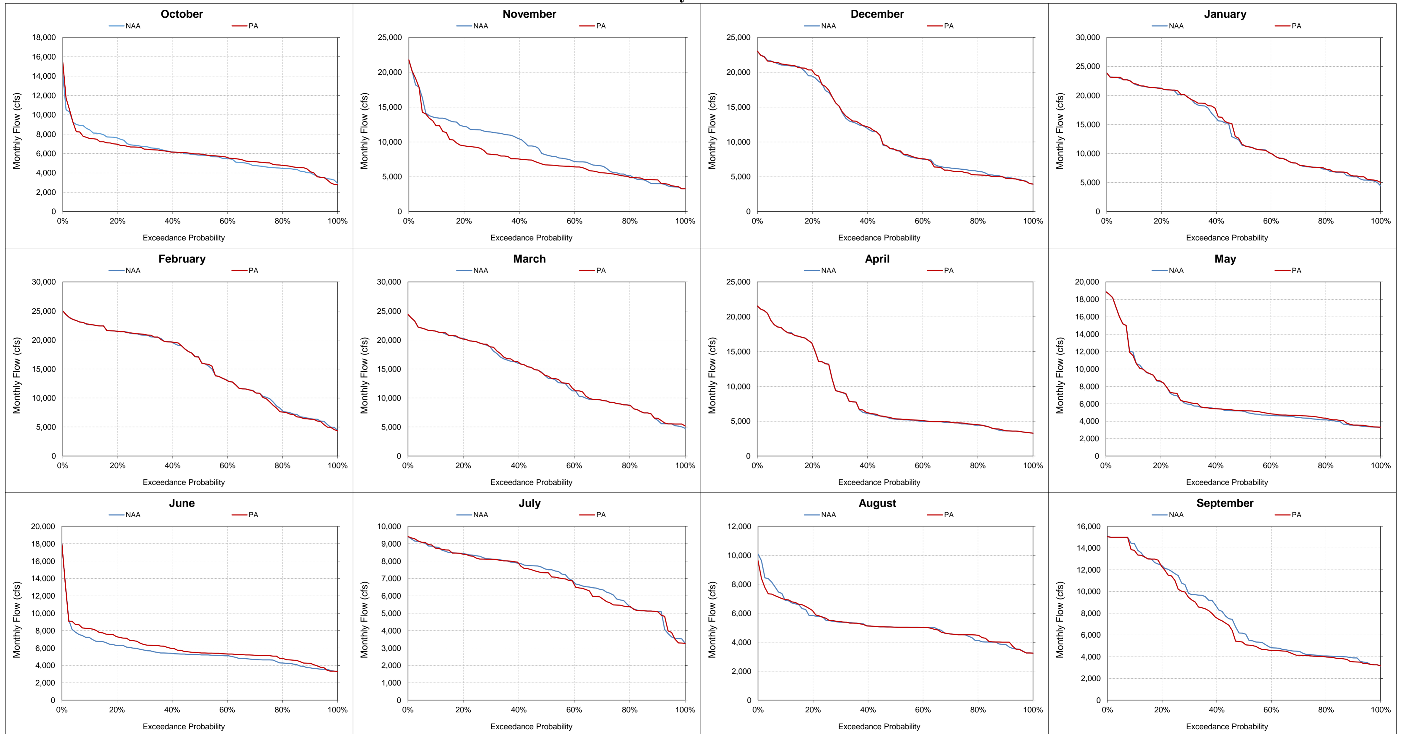
Figure 5.A.6-36-7. Sacramento River at Wilkins Slough, Monthly Flow Probability of Exceedance
