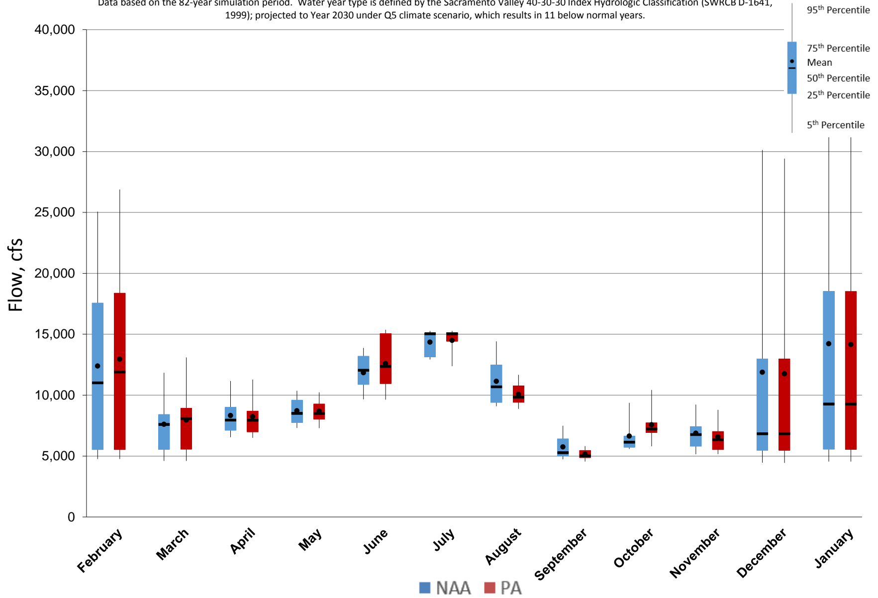
Figure 5.A.6-35-4. Monthly Flow Ranges For Sacramento River above Red Bluff Diversion Dam, Below Normal Years
