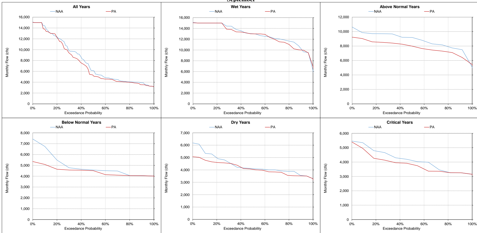
Figure 5.A.6-11-19. Sacramento River at Bend Bridge, Monthly Flow September
