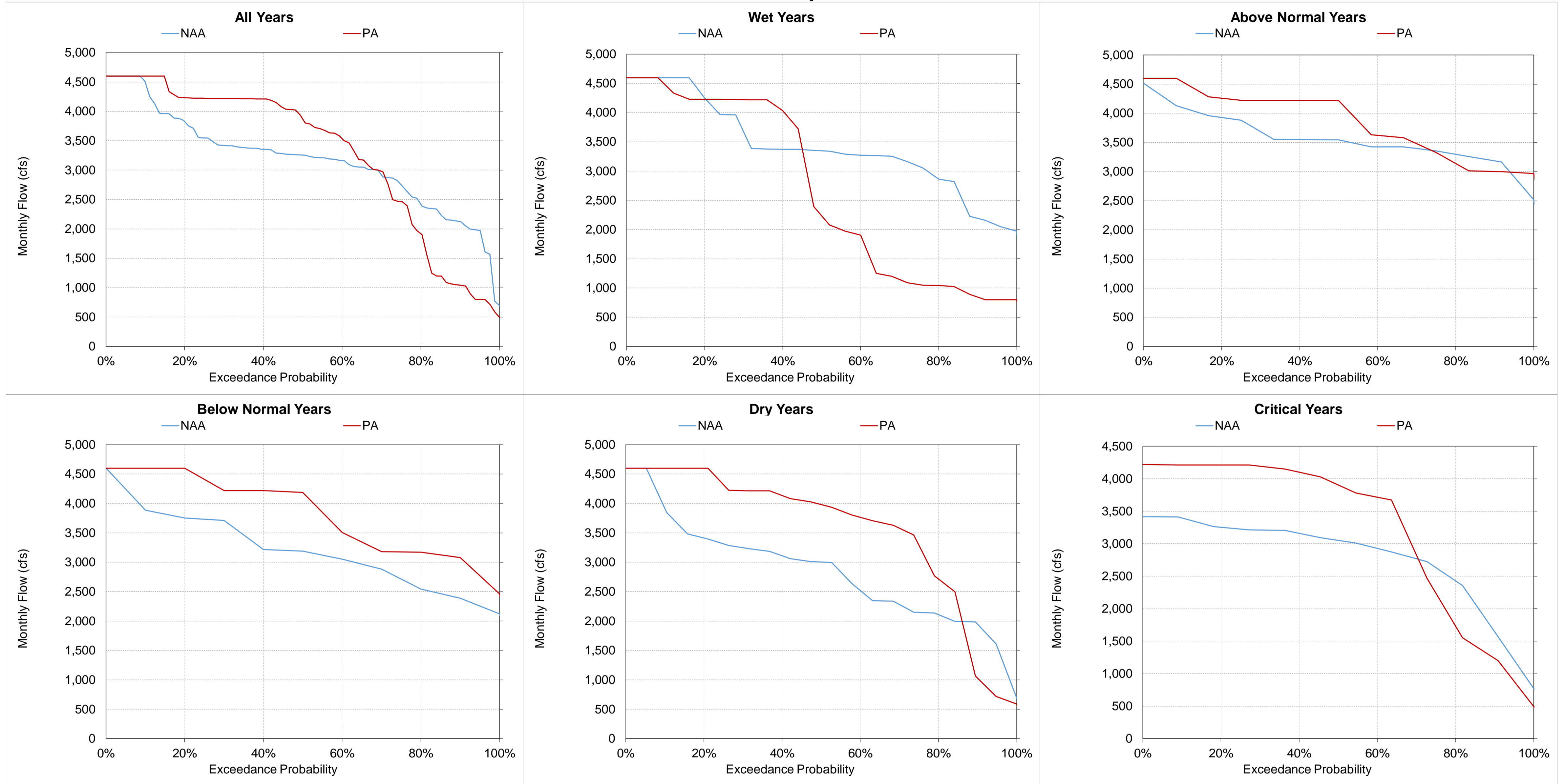
Figure 5.A.6-33-11. Total Jones Pumping Plant Exports, Monthly Flow January
