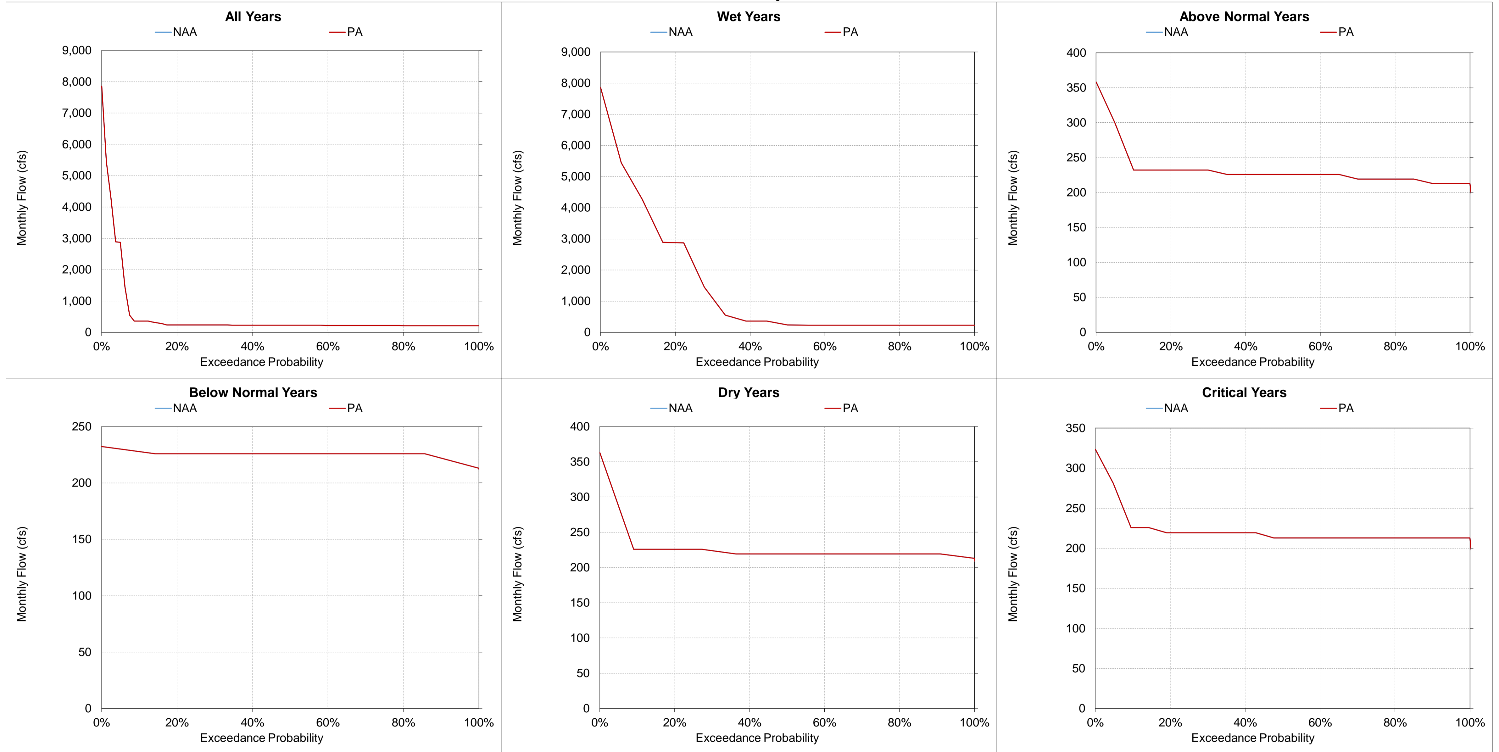
Figure 5.A.6-21-11. Stanislaus River at Goodwin, Monthly Flow January
