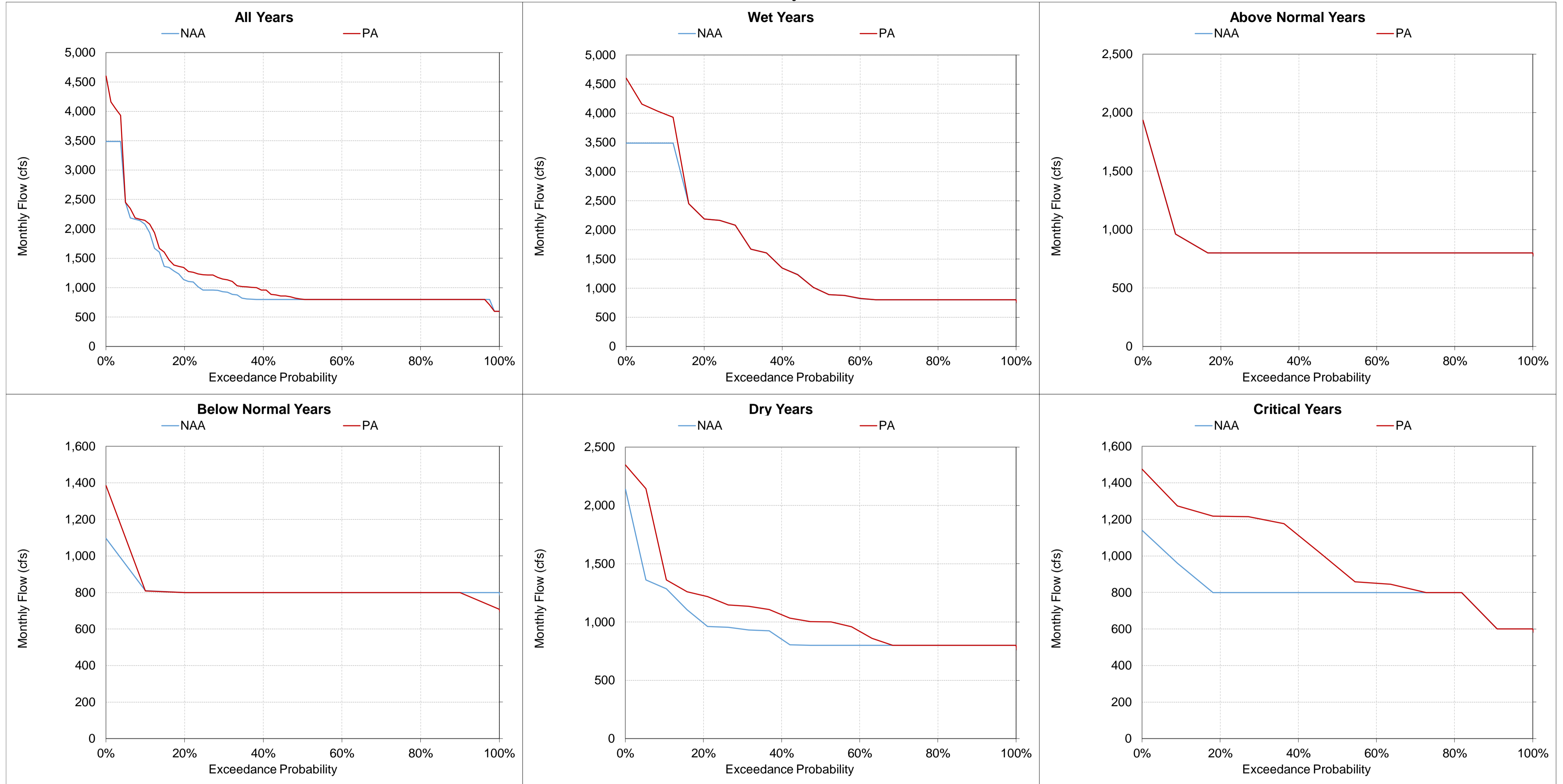
Figure 5.A.6-33-15. Total Jones Pumping Plant Exports, Monthly Flow May
