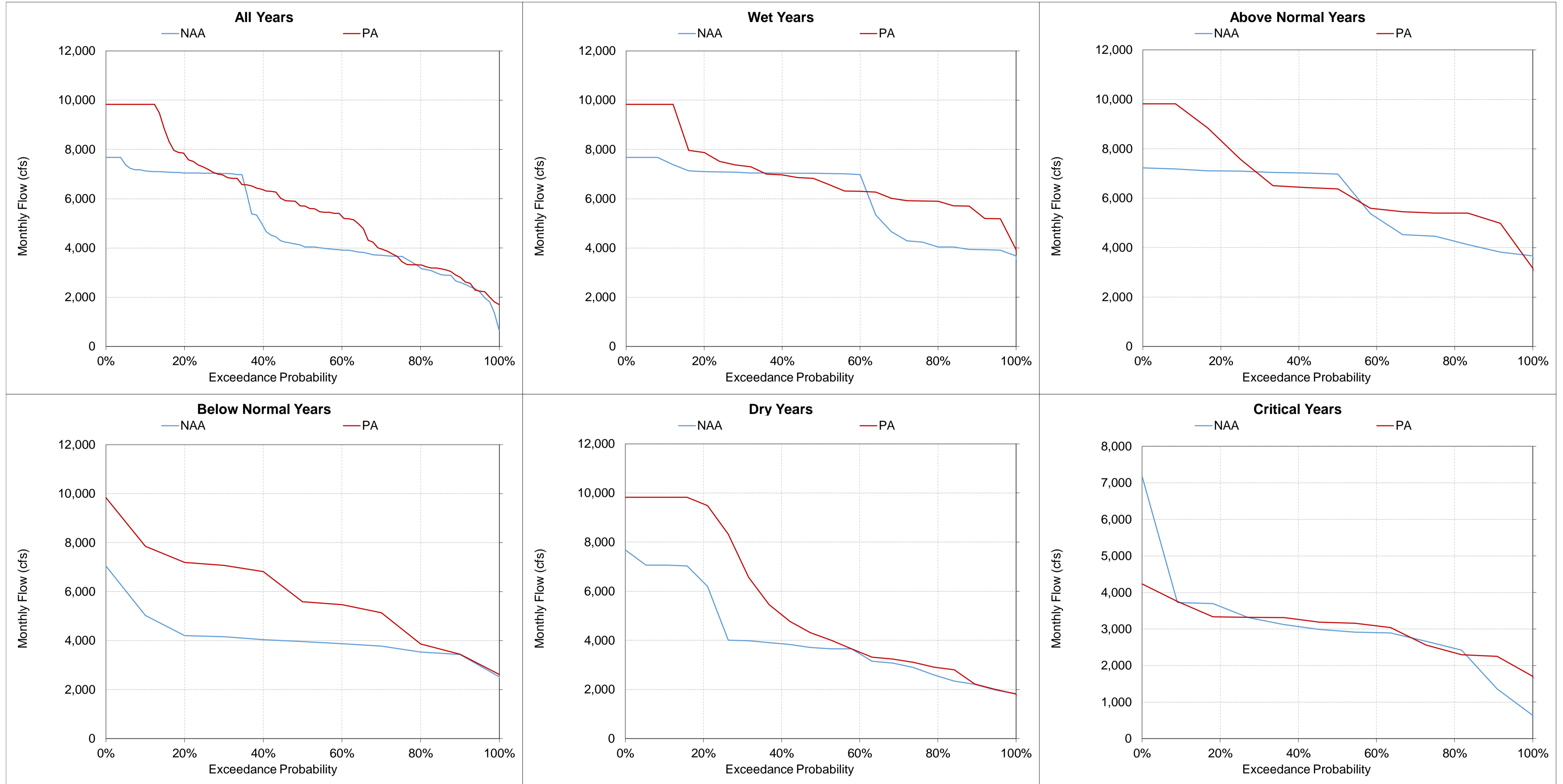
Figure 5.A.6-34-10. Total Banks Pumping Plant Exports, Monthly Flow December
