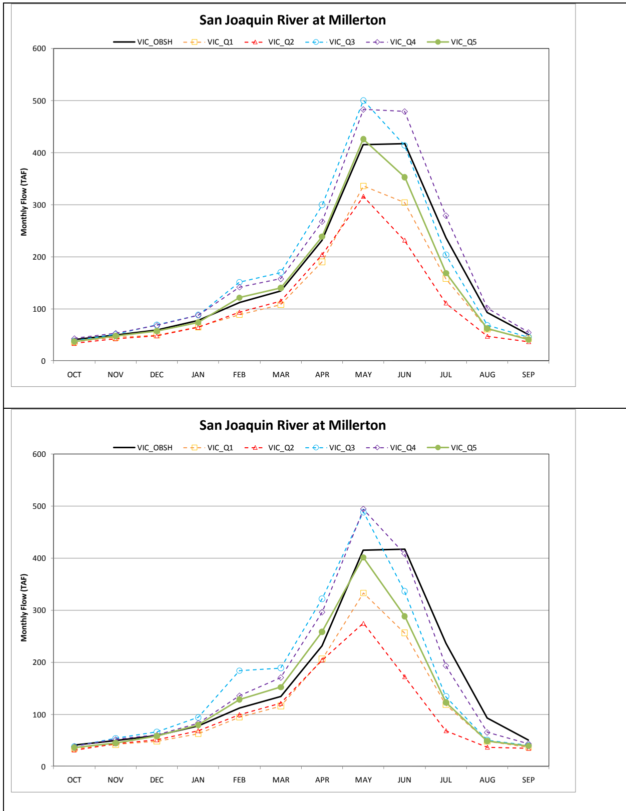
Figure 5.A.A.2-15. Simulated Changes in Monthly Natural Streamflow for San Joaquin River at Millerton (top, 2025 changes; bottom, 2060 changes).
