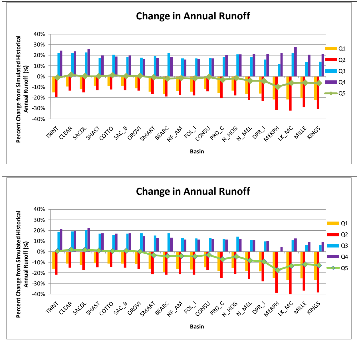
Figure 5.A.A.2-5. Simulated Changes in Natural Streamflow for Each of the VIC Simulations (top, 2025 changes; bottom, 2060 changes).
