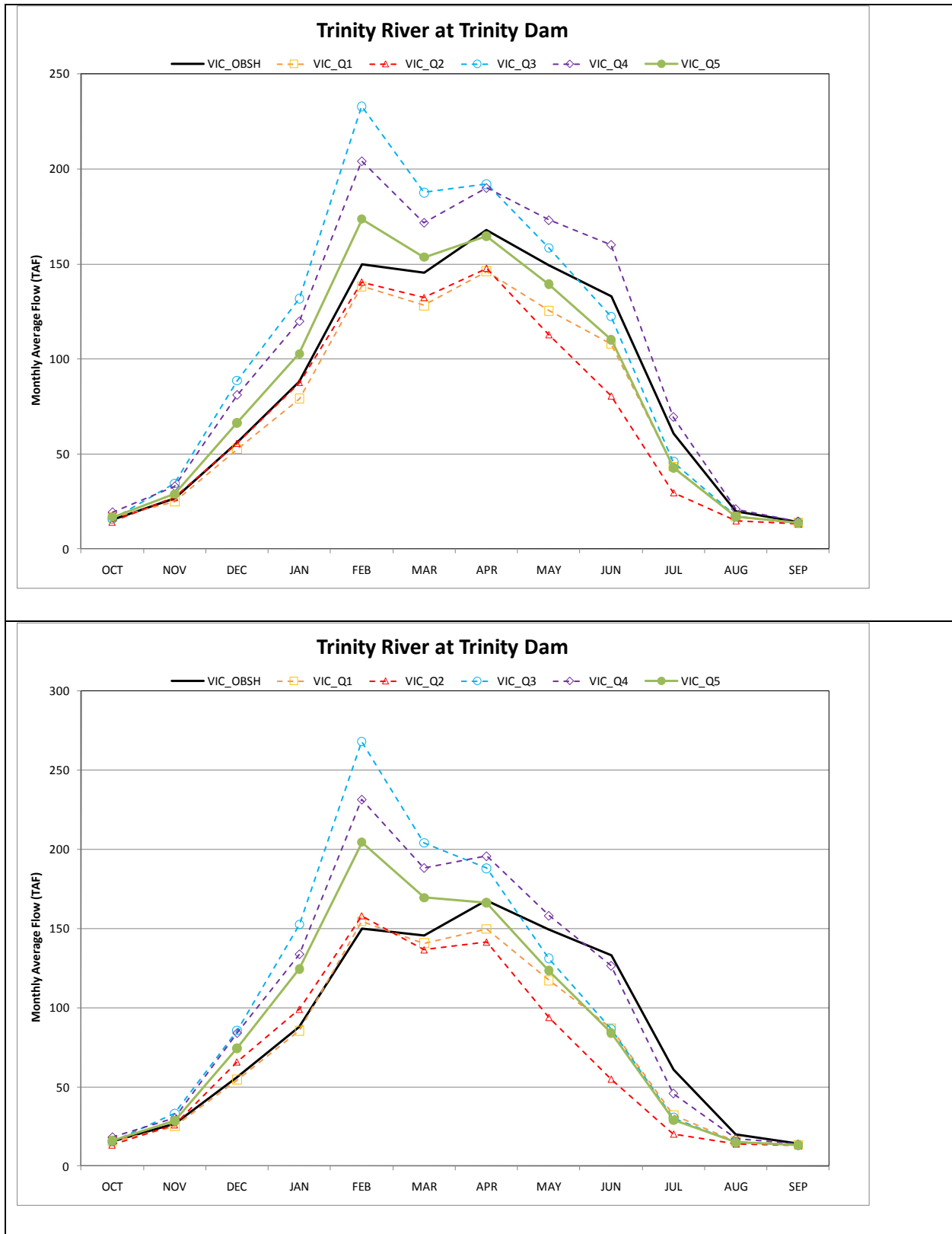
Figure 5.A.A.2-6. Simulated Changes in Monthly Natural Streamflow for Trinity River at Trinity Dam (top, 2025 changes; bottom, 2060 changes).
