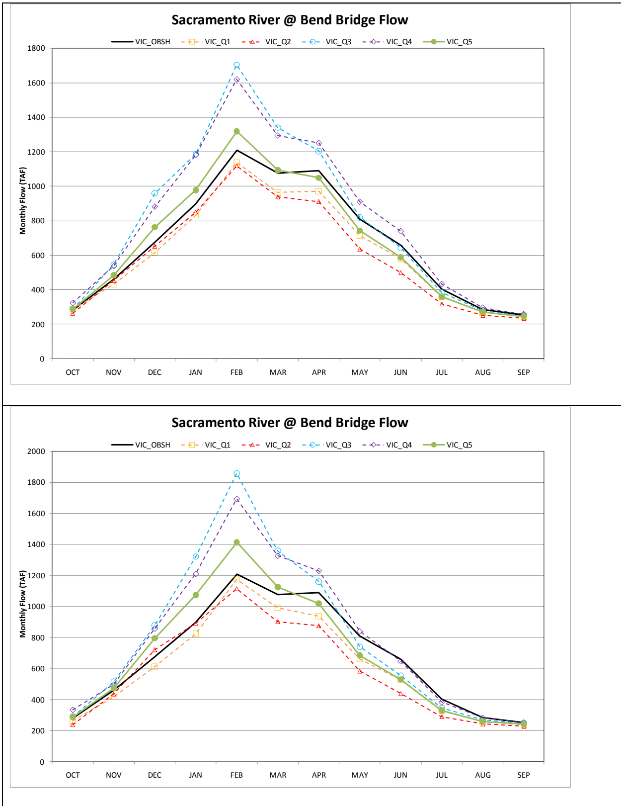
Figure 5.A.A.2-8. Simulated Changes in Monthly Natural Streamflow for Sacramento River at Bend Bridge (top, 2025 changes; bottom, 2060 changes).
