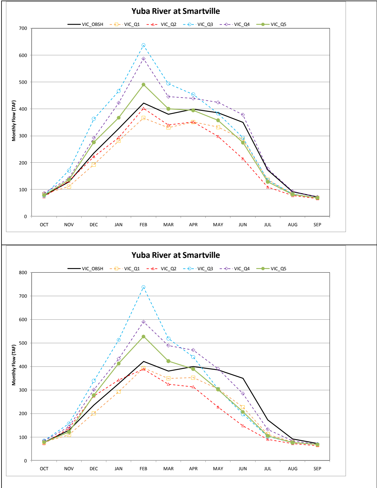
Figure 5.A.A.2-10. Simulated Changes in Monthly Natural Streamflow for Yuba River at Smartville (top, 2025 changes; bottom, 2060 changes).
