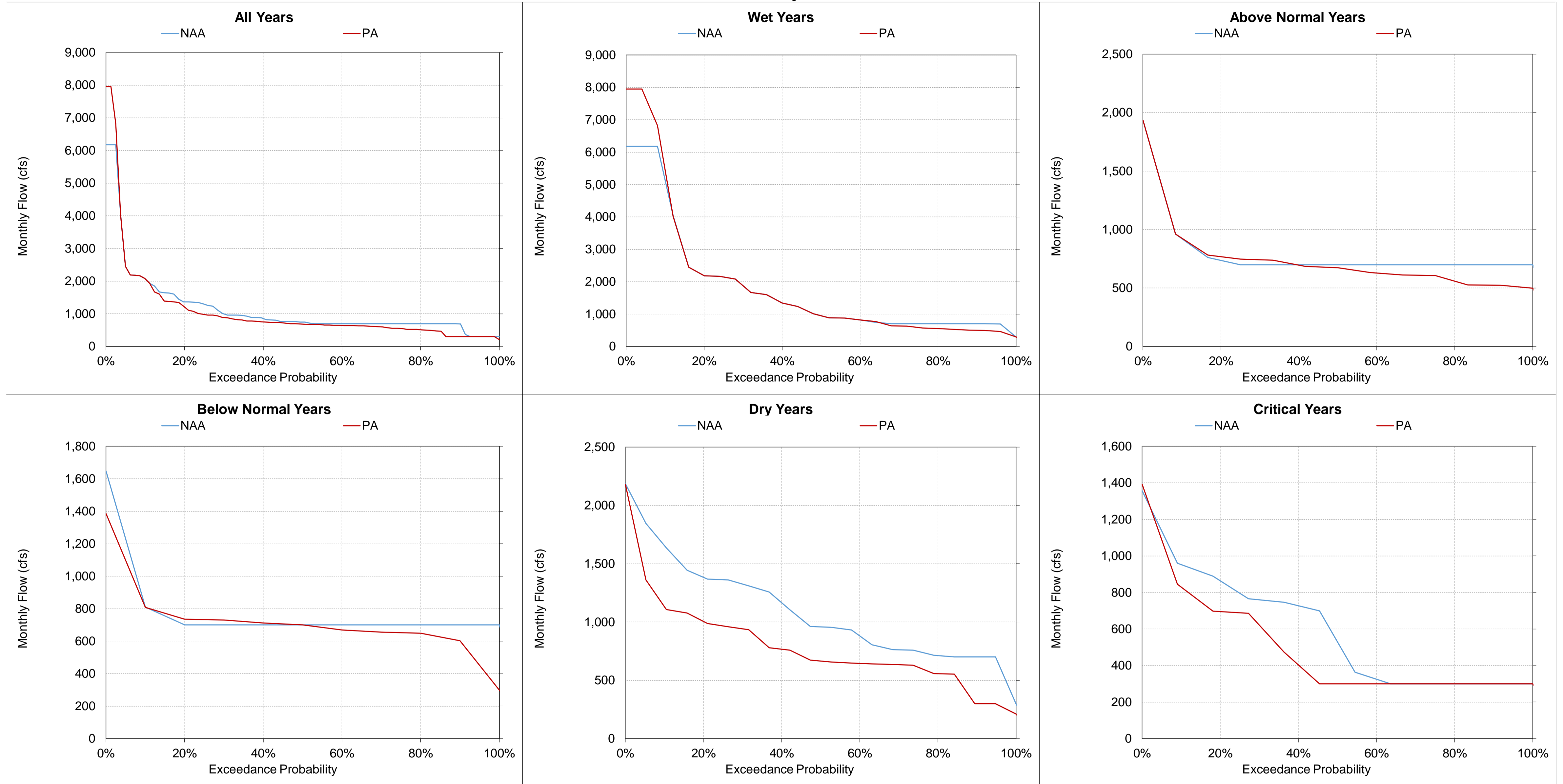
Figure 5.A.6-34-15. Total Banks Pumping Plant Exports, Monthly Flow May
