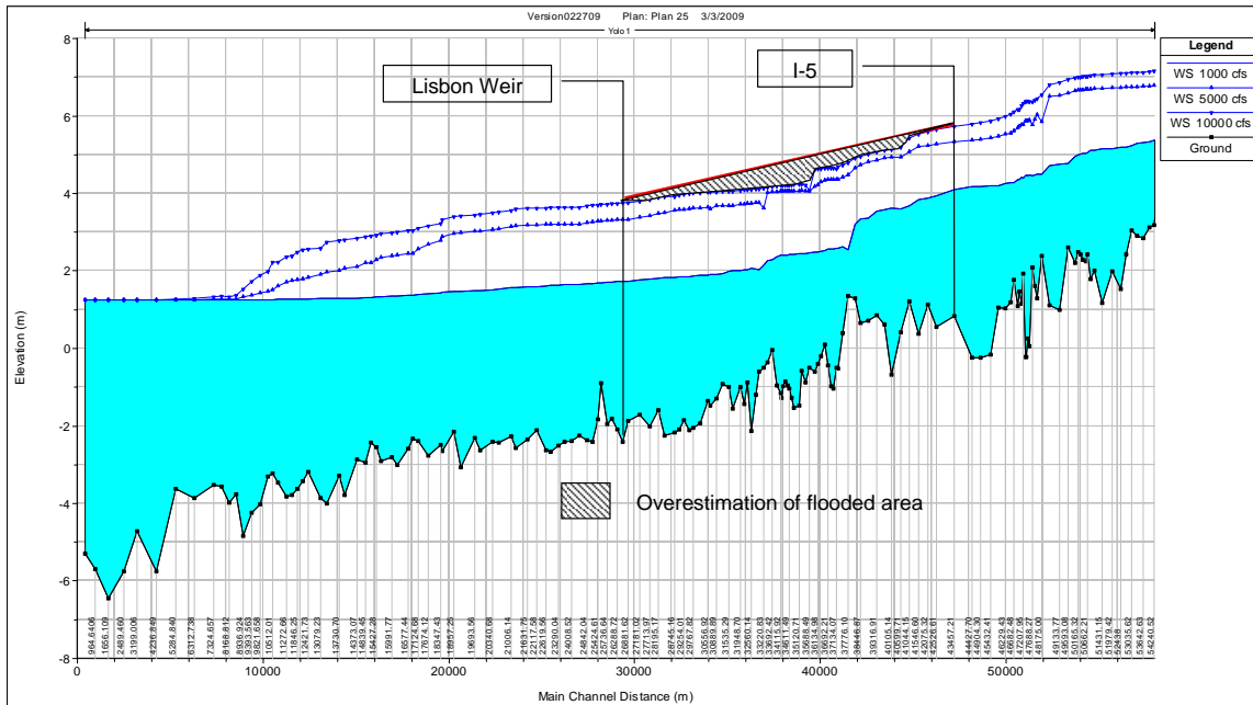
Figure 5.A.A.4-11. Possible overestimation of flooded areas using a linearization of water surface between two stations.
