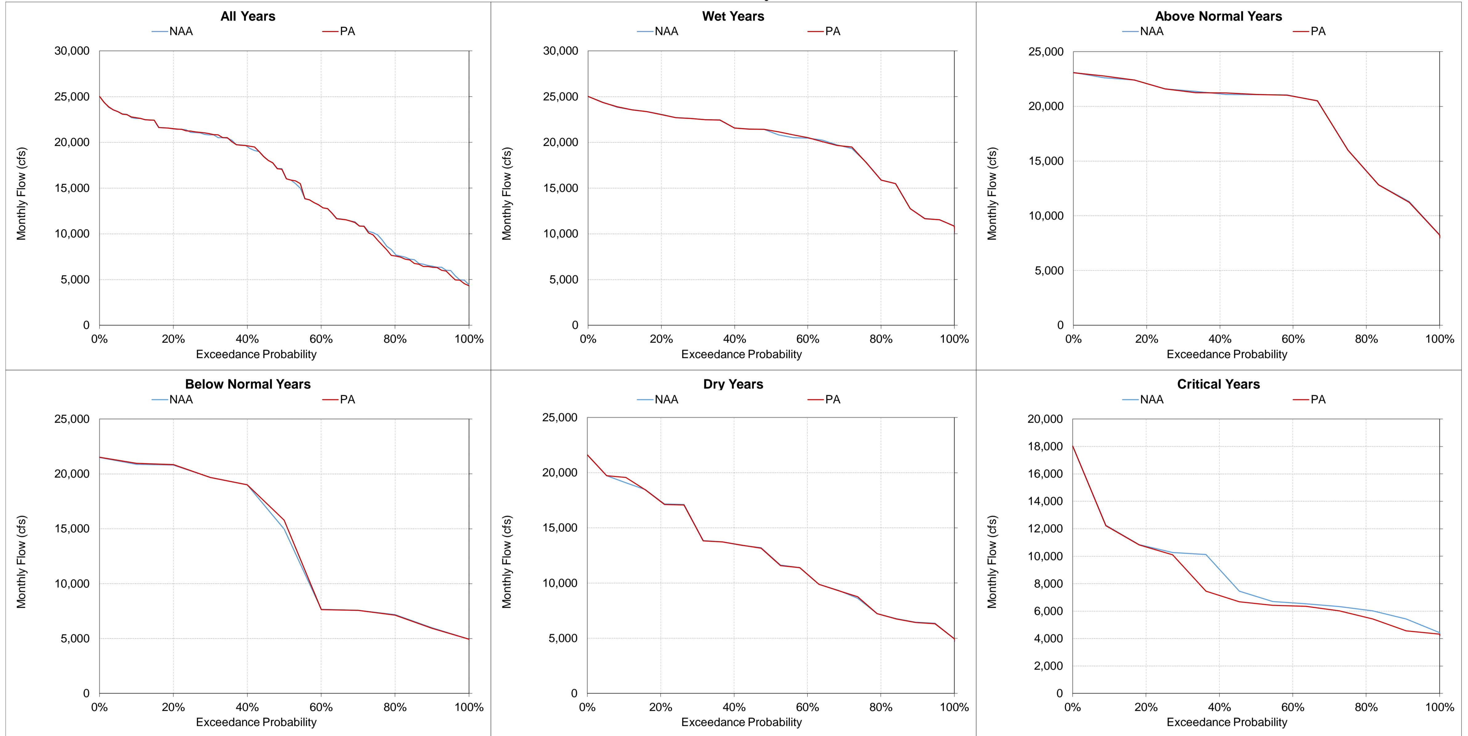
Figure 5.A.6-36-12. Sacramento River at Wilkins Slough, Monthly Flow February
