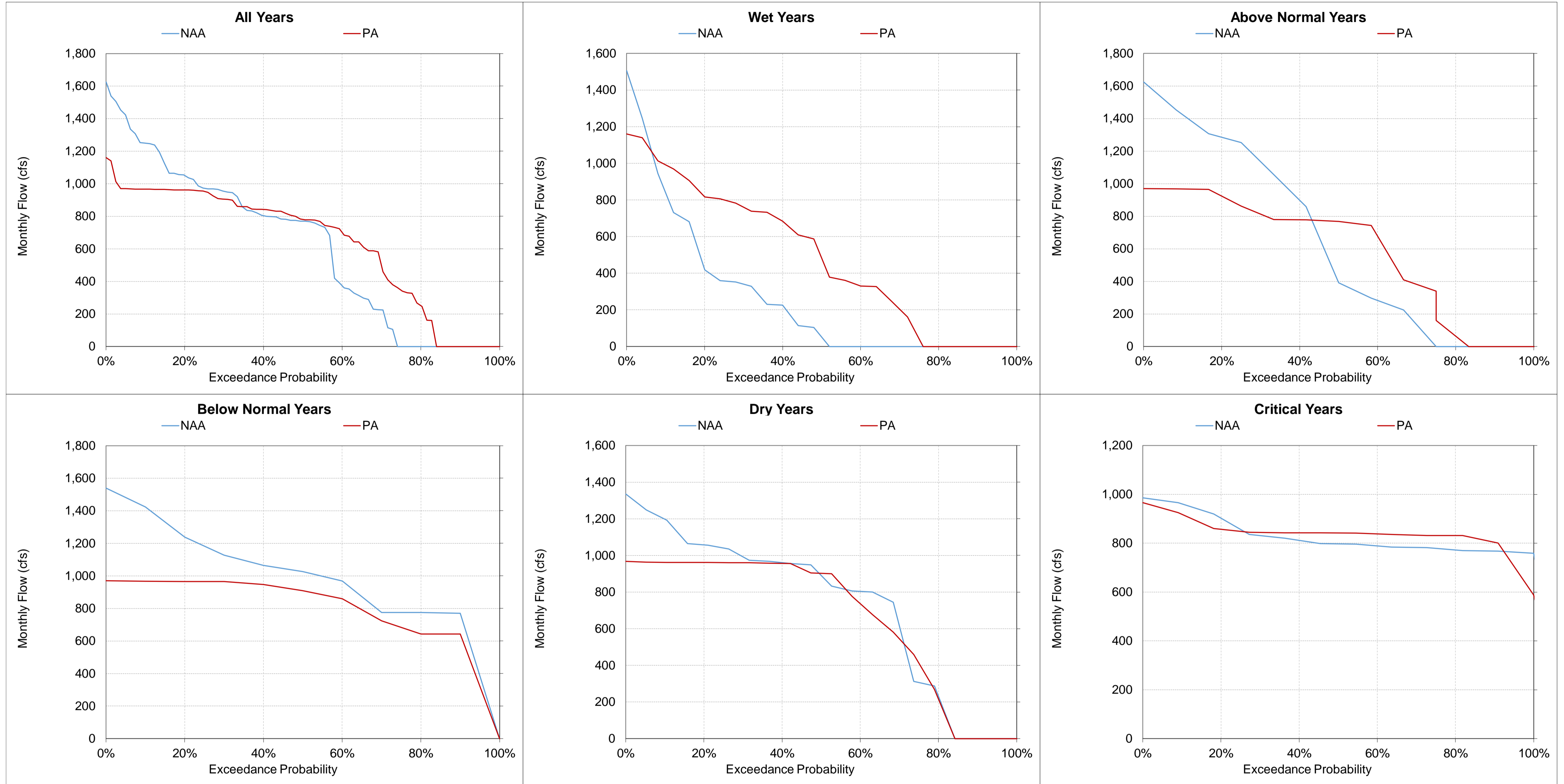
Figure 5.A.6-32-9. Delta Cross Channel, Monthly Flow November
