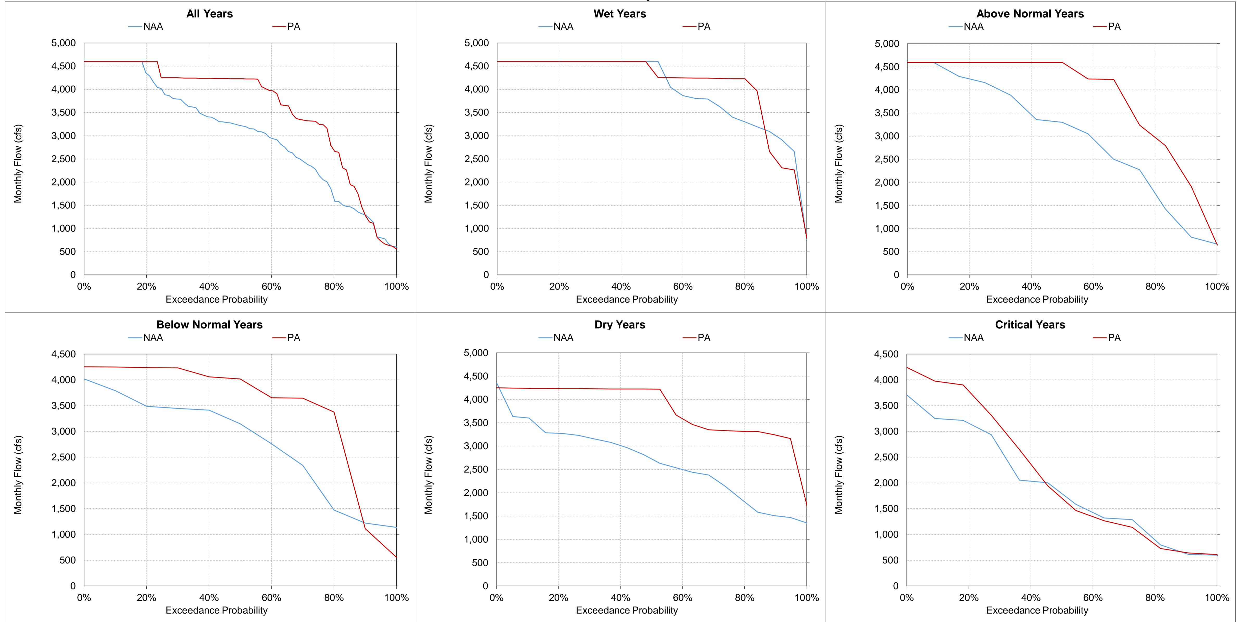
Figure 5.A.6-33-12. Total Jones Pumping Plant Exports, Monthly Flow February
