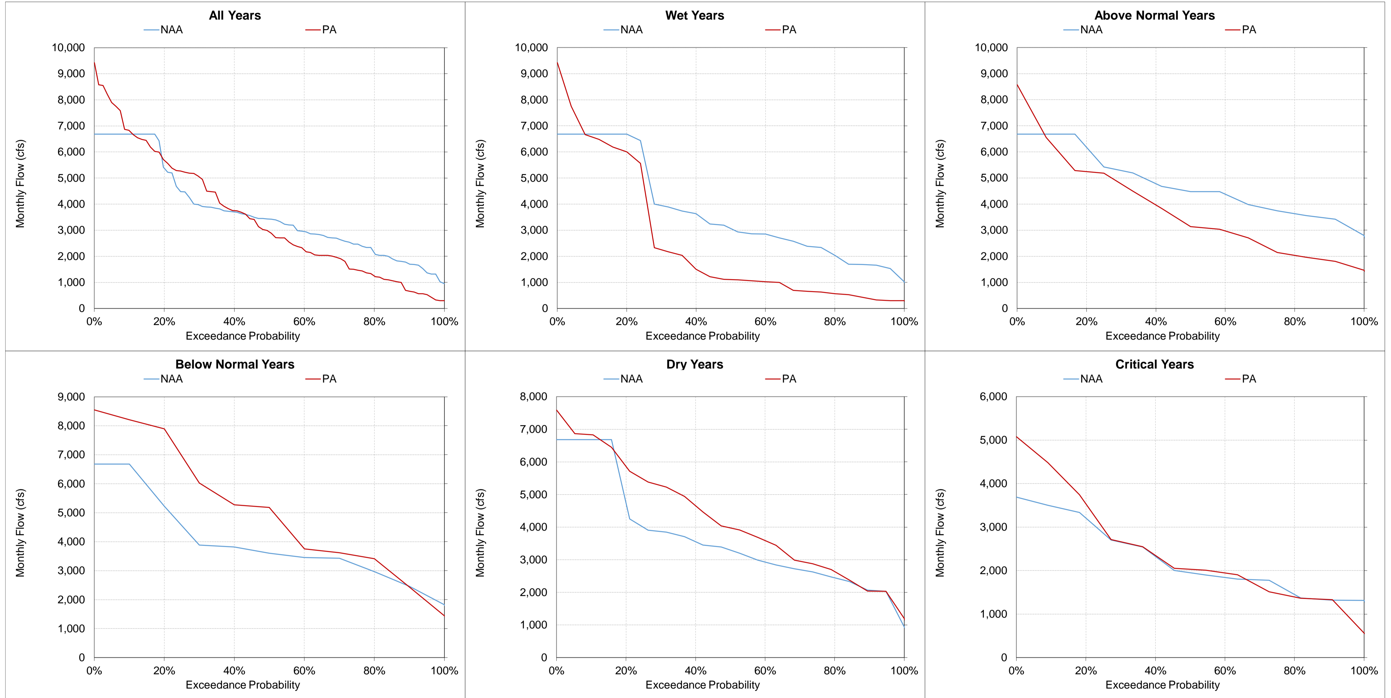
Figure 5.A.6-34-9. Total Banks Pumping Plant Exports, Monthly Flow November
