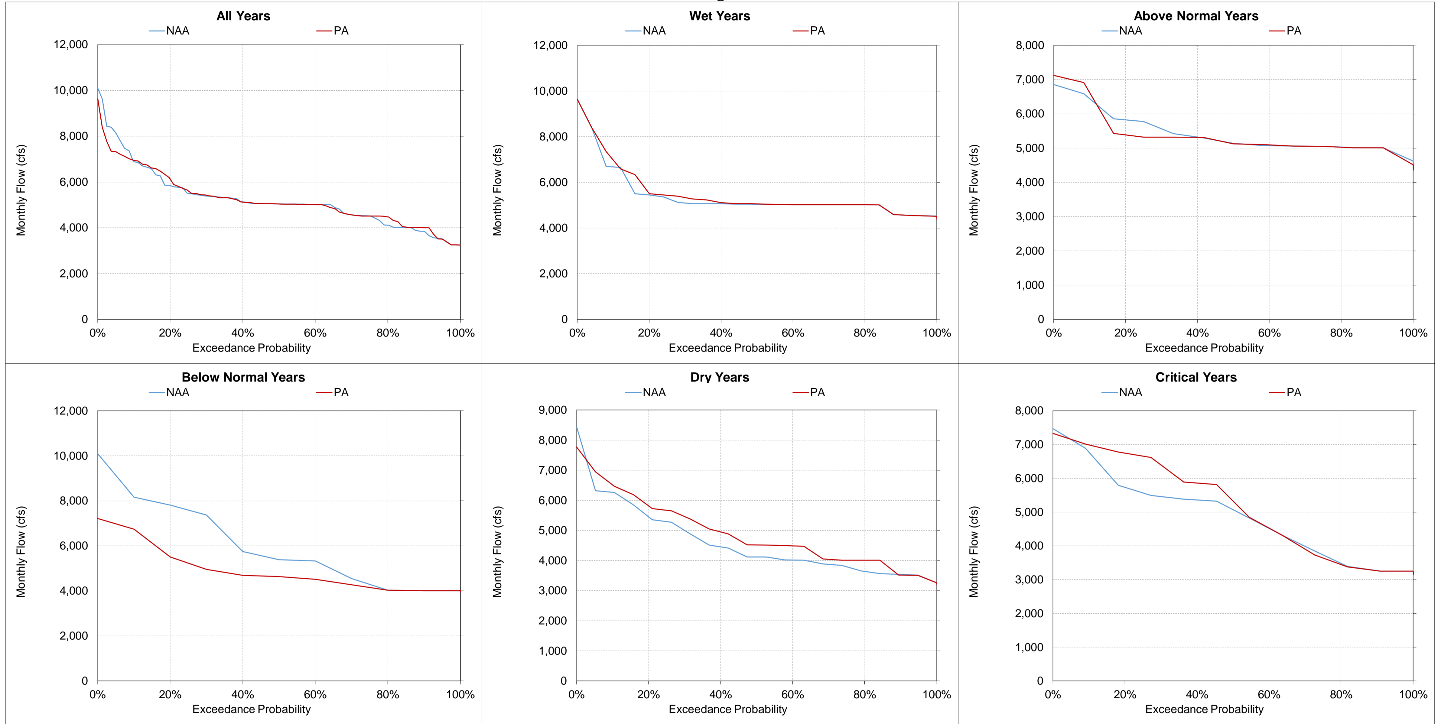
Figure 5.A.6-36-18. Sacramento River at Wilkins Slough, Monthly Flow August
