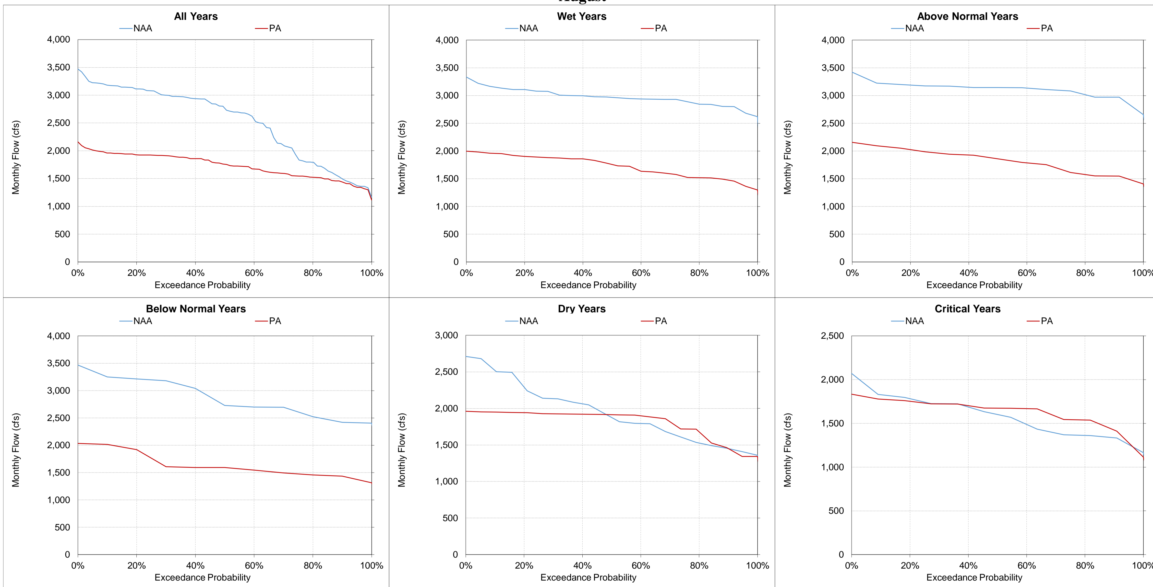
Figure 5.A.6-32-18. Delta Cross Channel, Monthly Flow August
