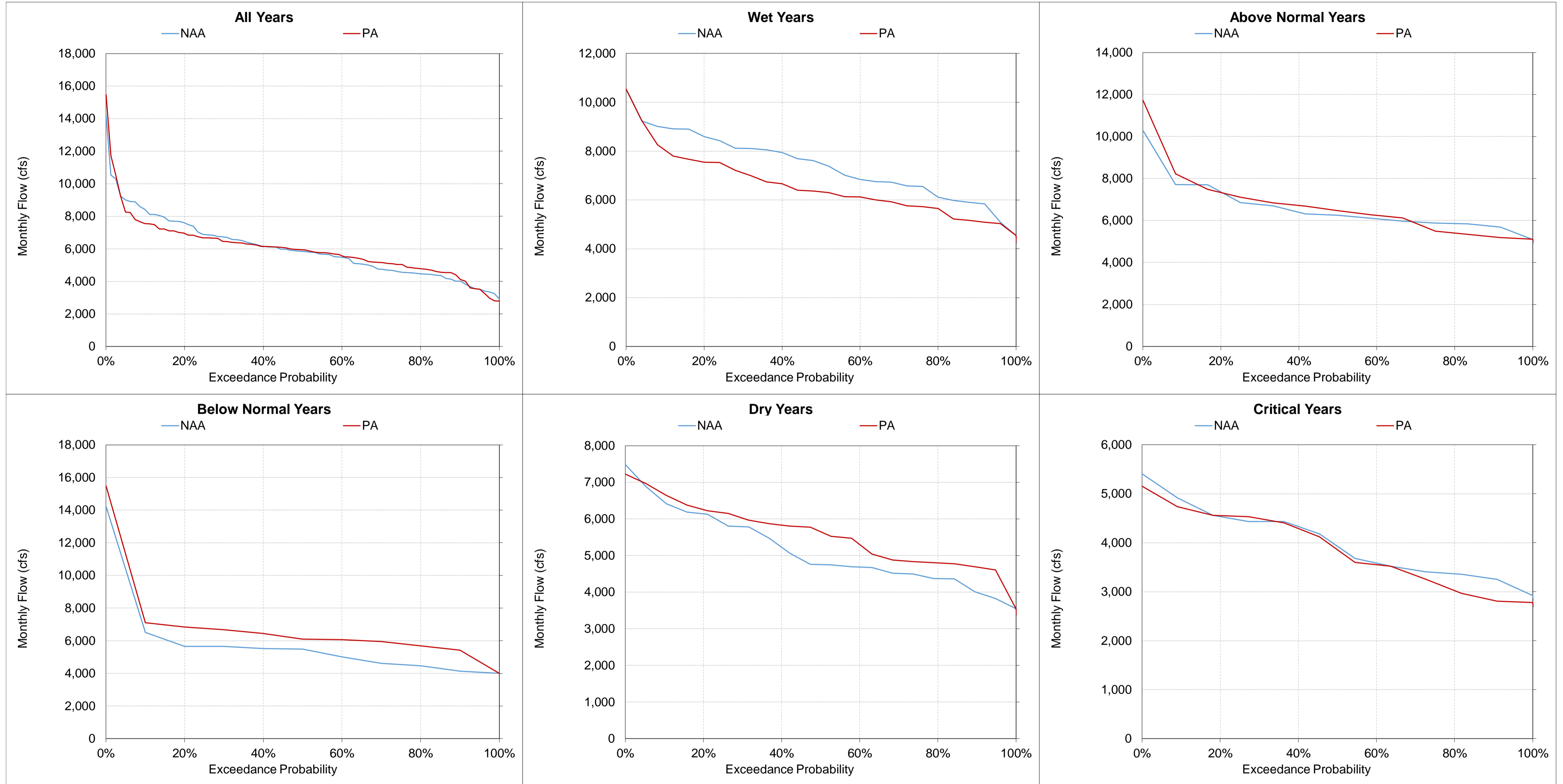
Figure 5.A.6-36-8. Sacramento River at Wilkins Slough, Monthly Flow October
