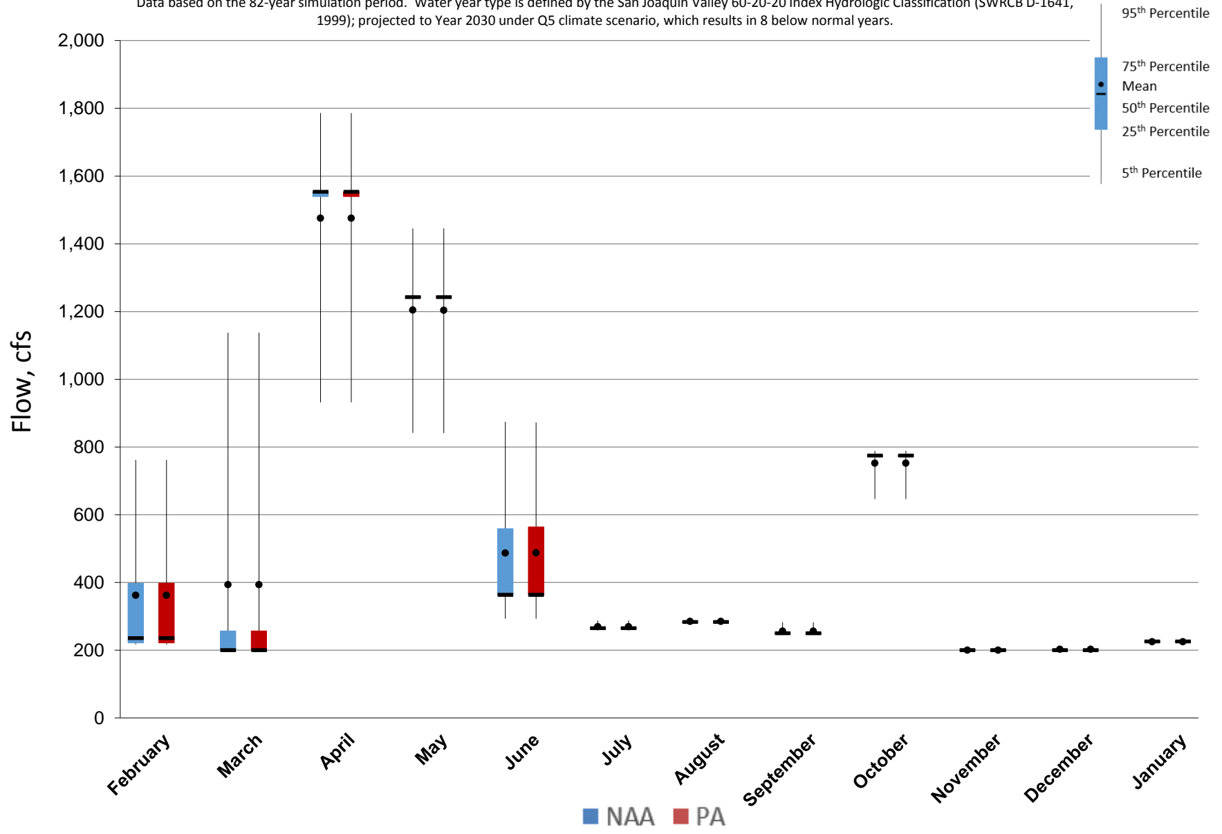
Figure 5.A.6-21-4. Monthly Flow Ranges for Stanislaus River at Goodwin, Below Normal Years
