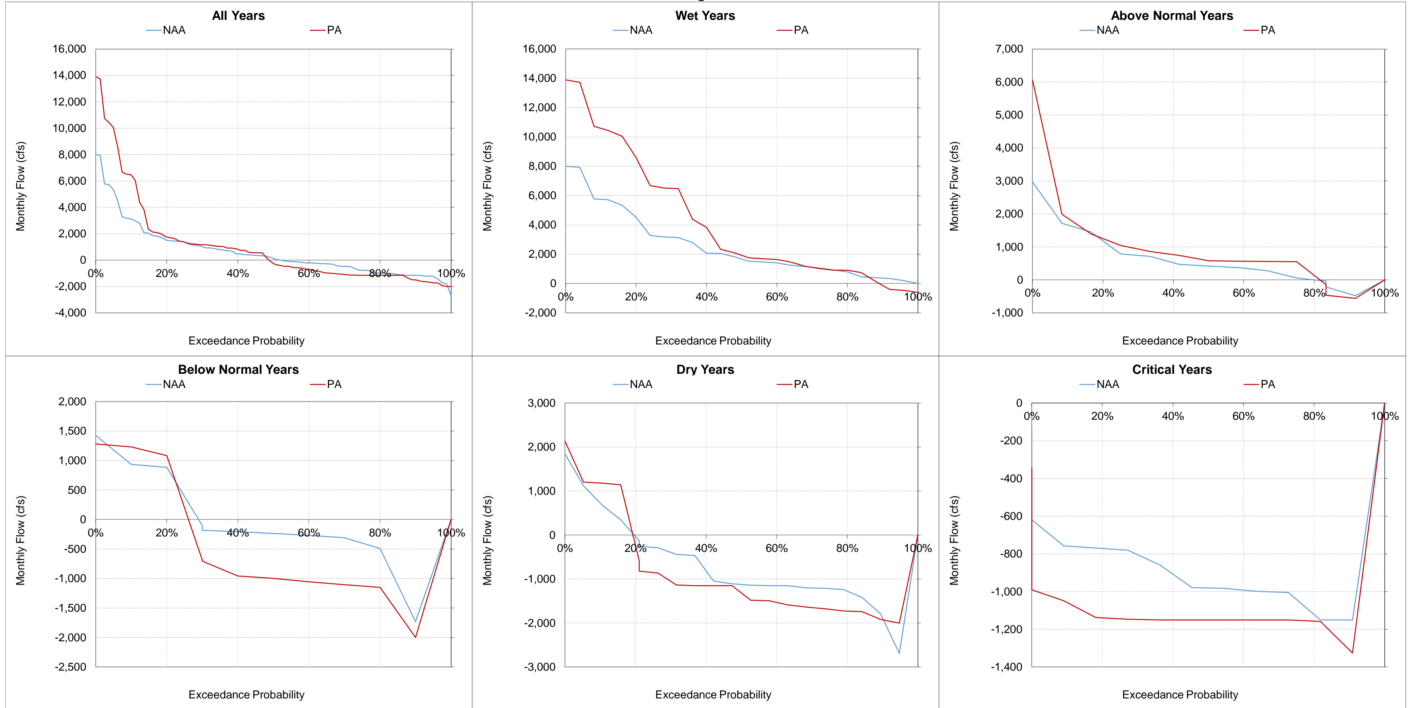
Figure 5.A.6-25-14. Old and Middle River, Monthly Flow April
