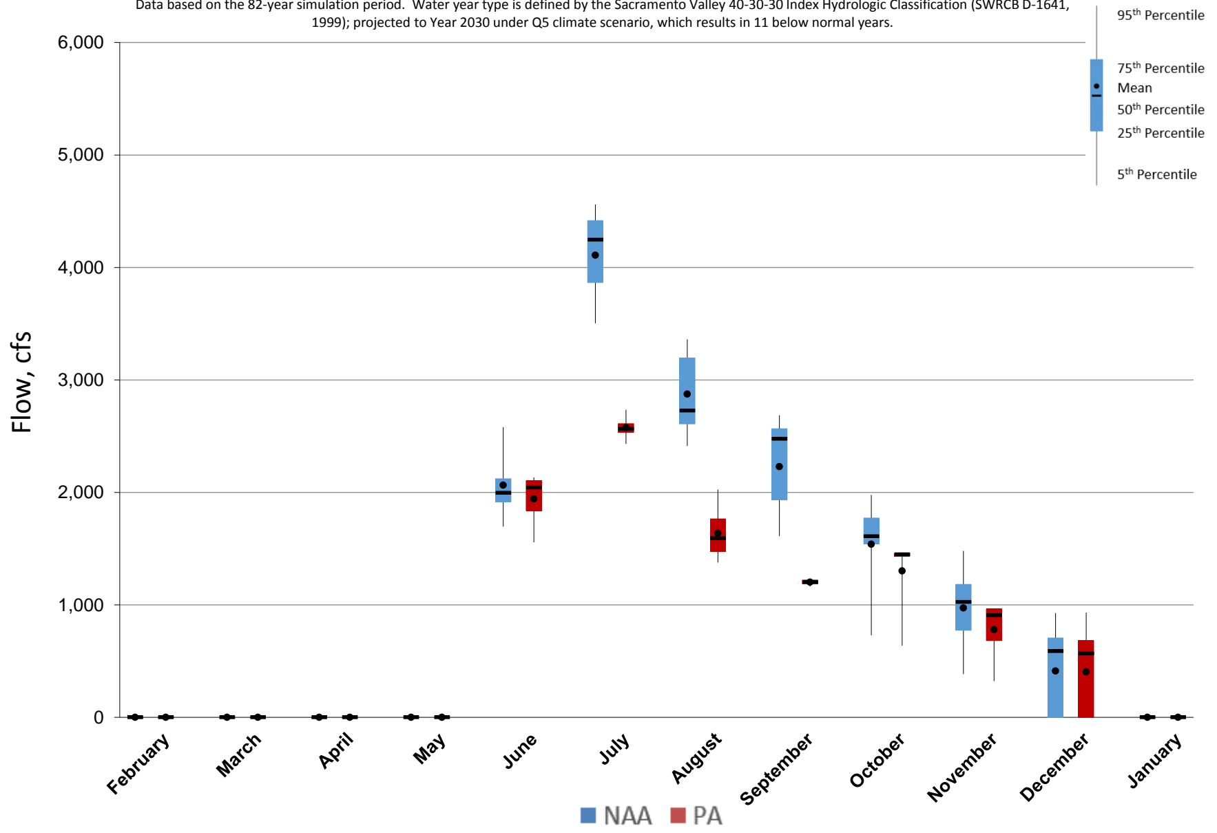
Figure 5.A.6-32-4. Monthly Flow Ranges For Delta Cross Channel, Below Normal Years
