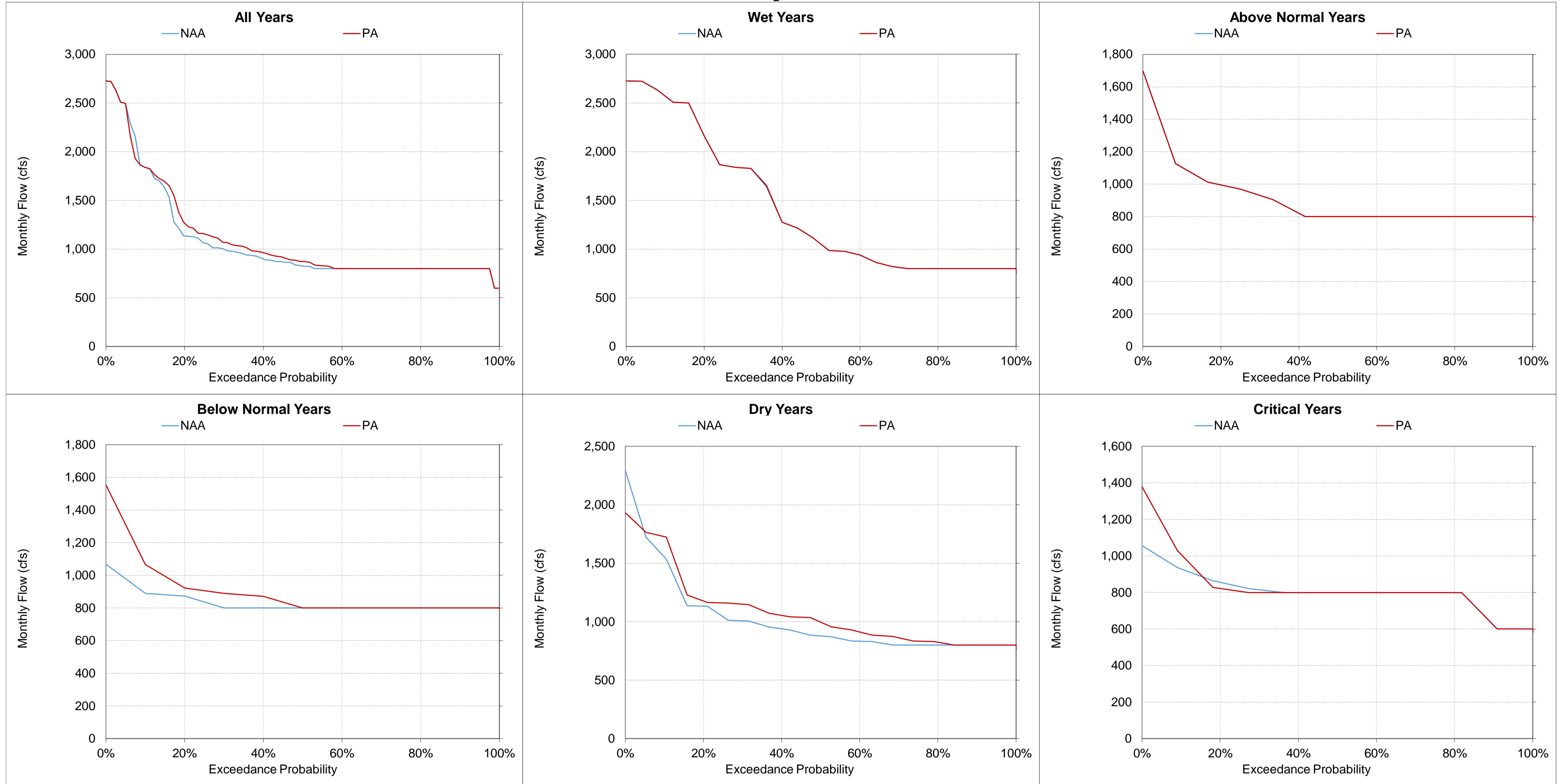
Figure 5.A.6-33-14. Total Jones Pumping Plant Exports, Monthly Flow April
