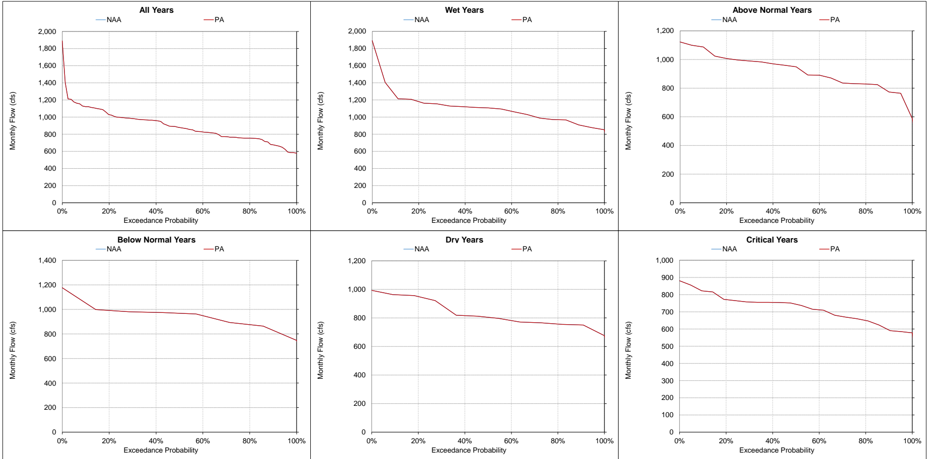
Figure 5.A.6-22-8. Stanislaus River at Mouth, Monthly Flow October
