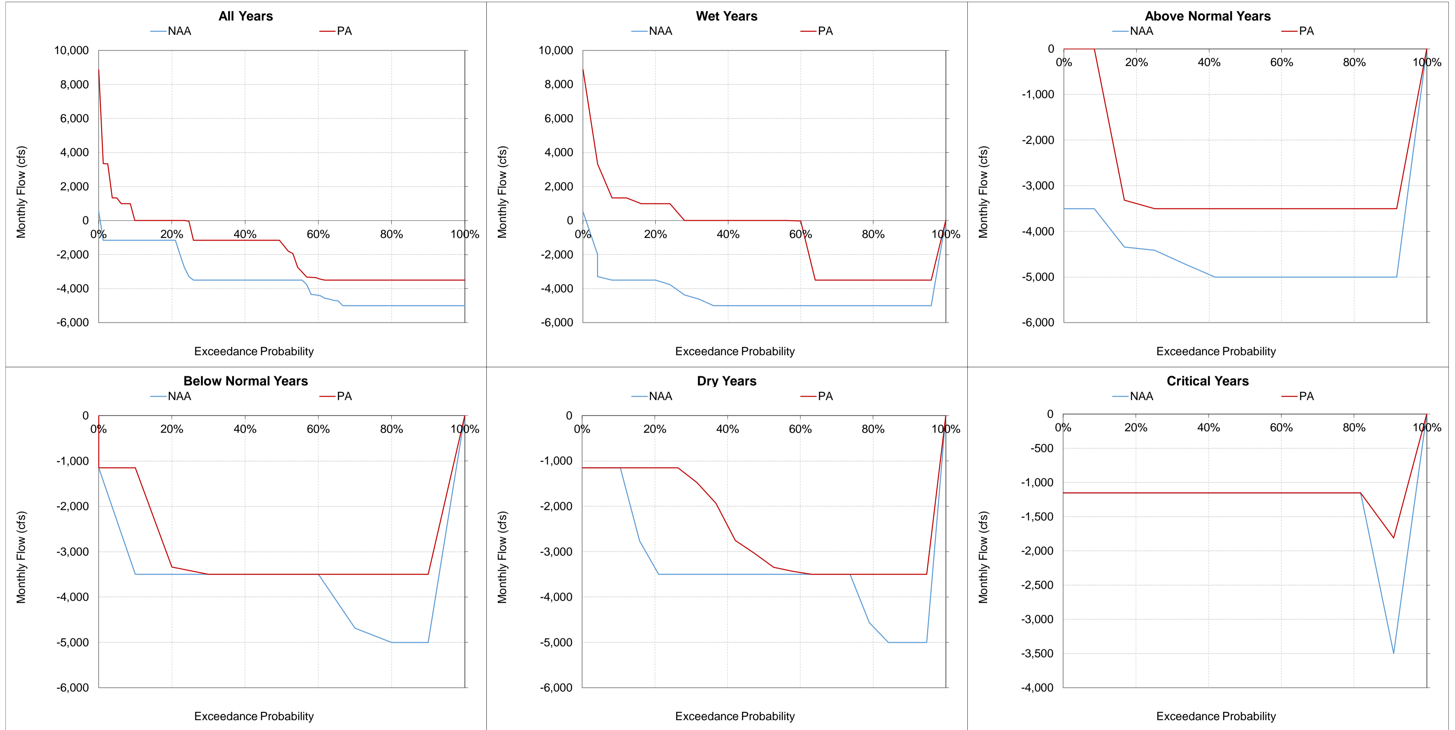
Figure 5.A.6-25-16. Old and Middle River, Monthly Flow June
