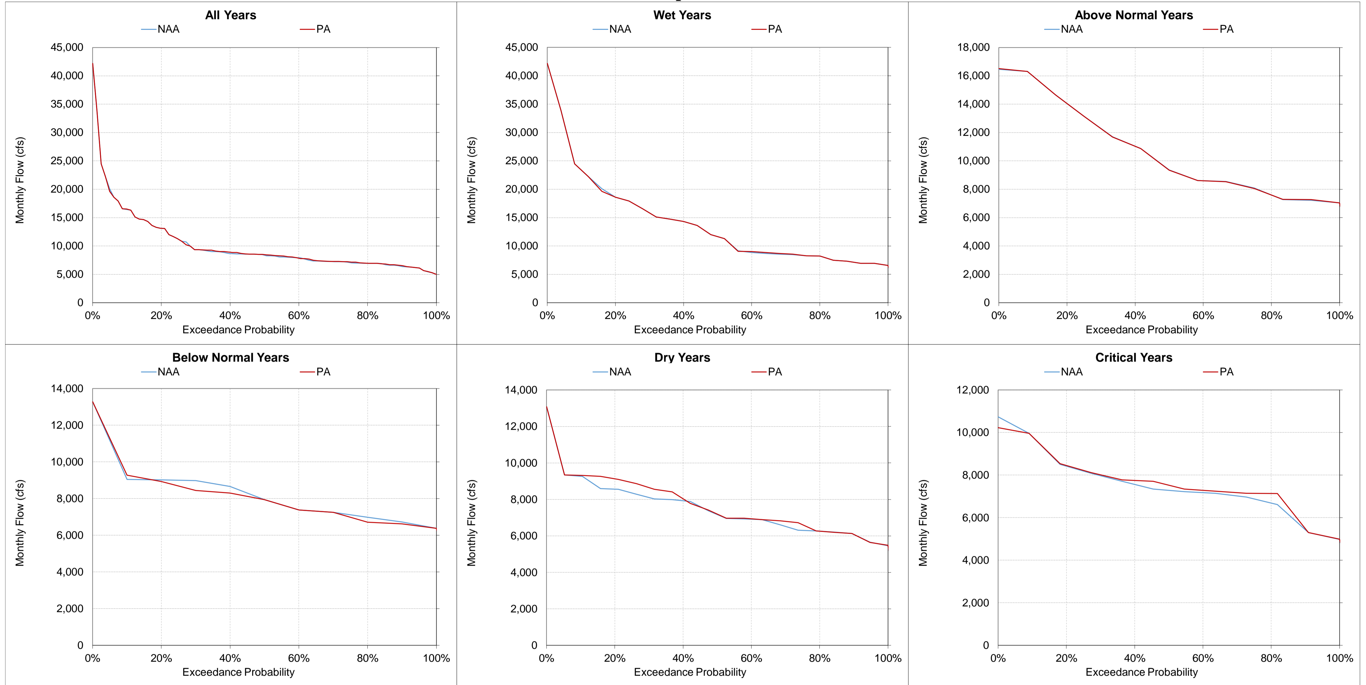
Figure 5.A.6-35-14. Sacramento River above Red Bluff Diversion Dam, Monthly Flow April
