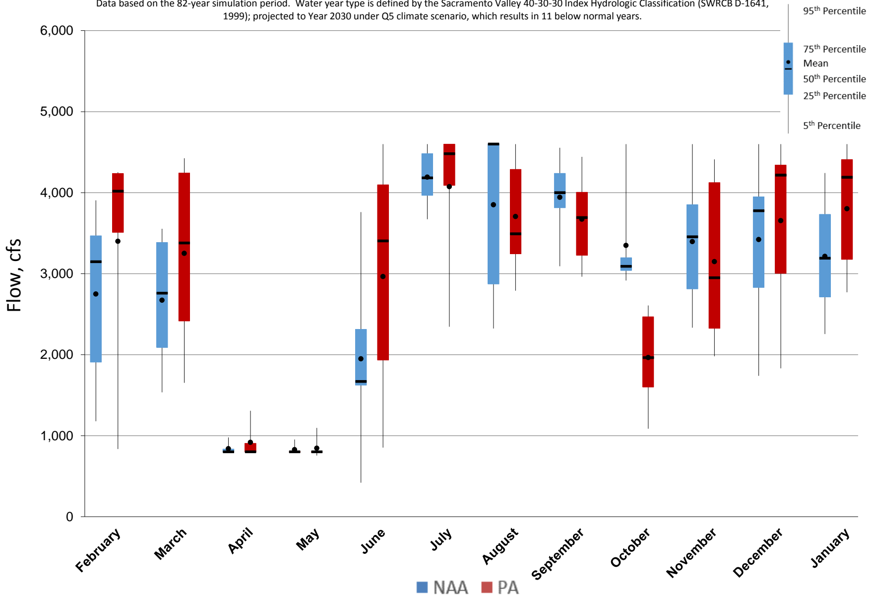
Figure 5.A.6-33-4. Monthly Flow Ranges For Total Jones Pumping Plant Exports, Below Normal Years
