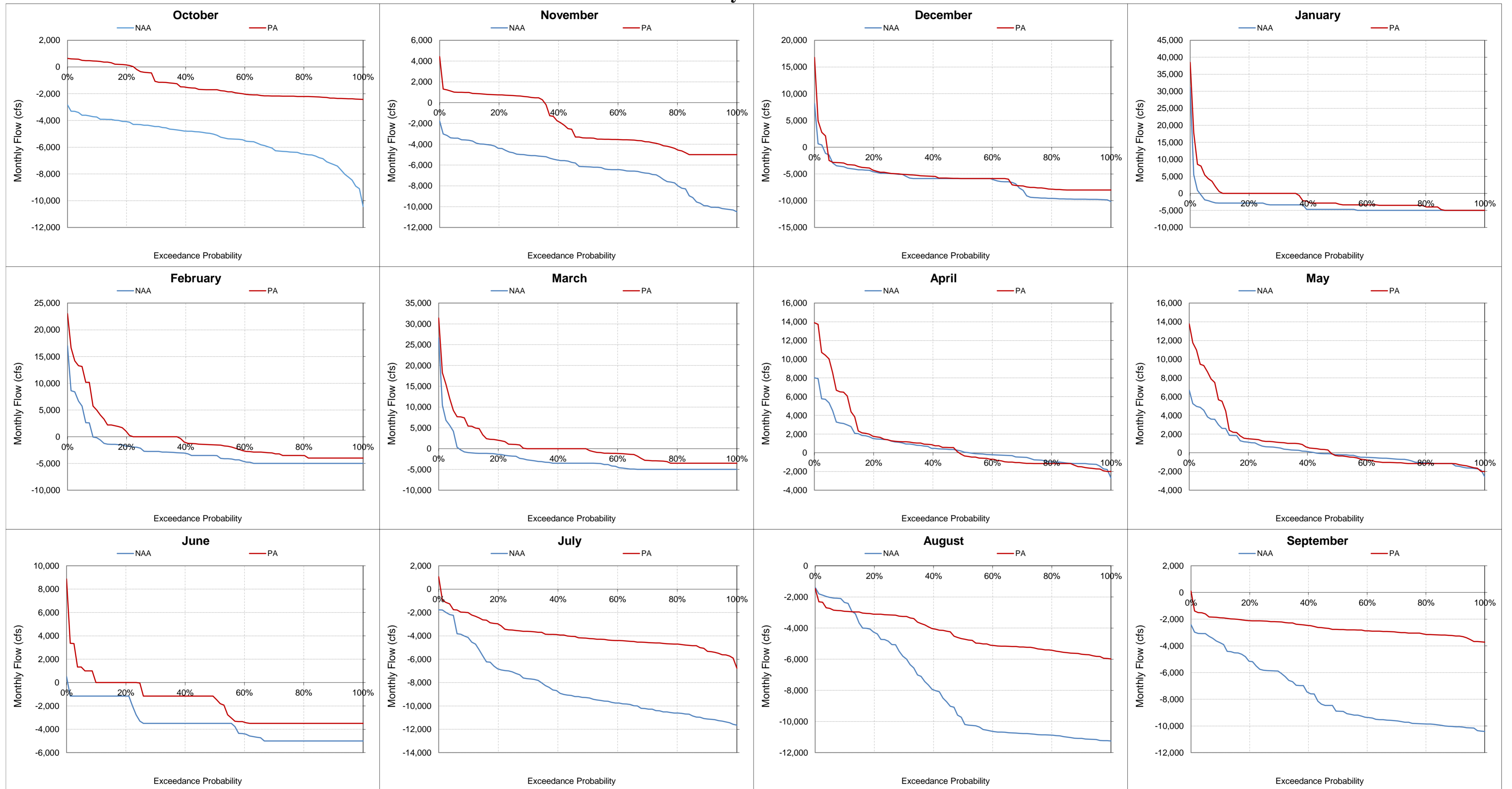
Figure 5.A.6-25-7. Old and Middle River, Monthly Flow Probability of Exceedance
