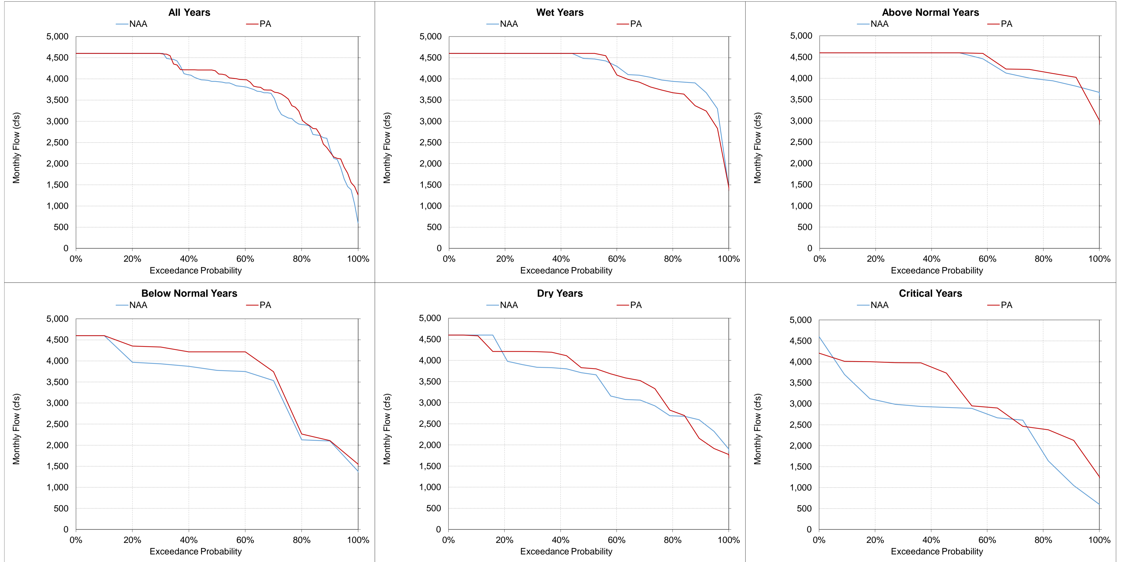
Figure 5.A.6-33-10. Total Jones Pumping Plant Exports, Monthly Flow December
