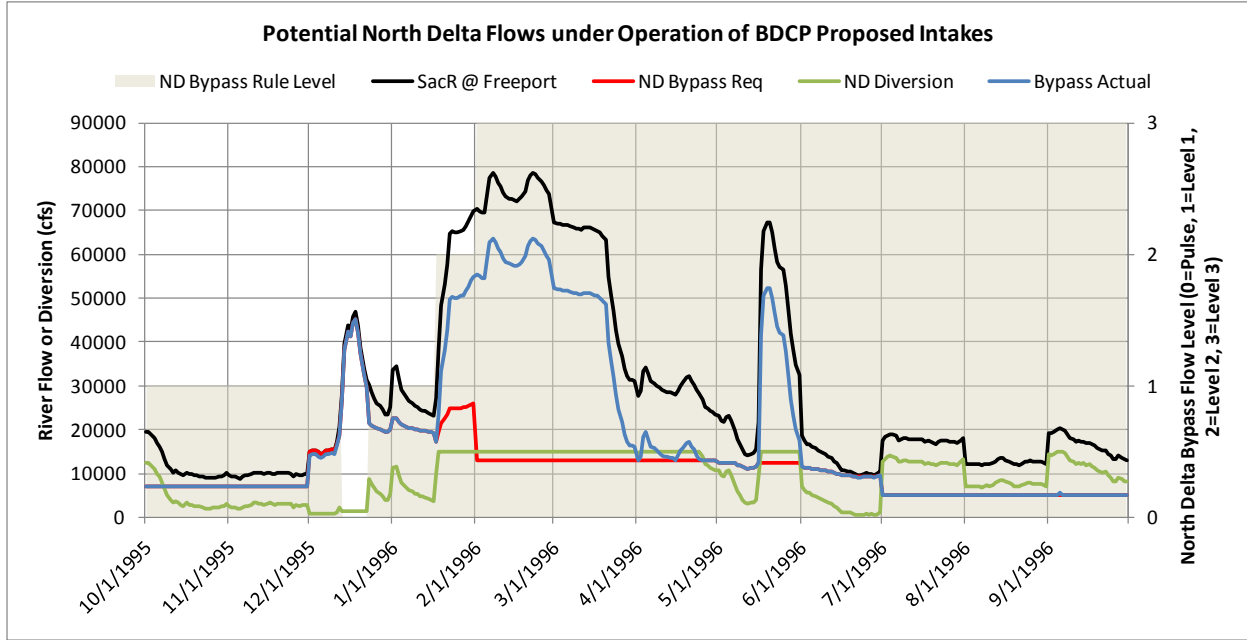
Figure 5.A-8 Example year daily patterns and operation of the north Delta intakes. Note: the grey shading indicates the active bypass rule (0=pulse/low level pumping, 1=level I, 2=level II, and 3=level III).
