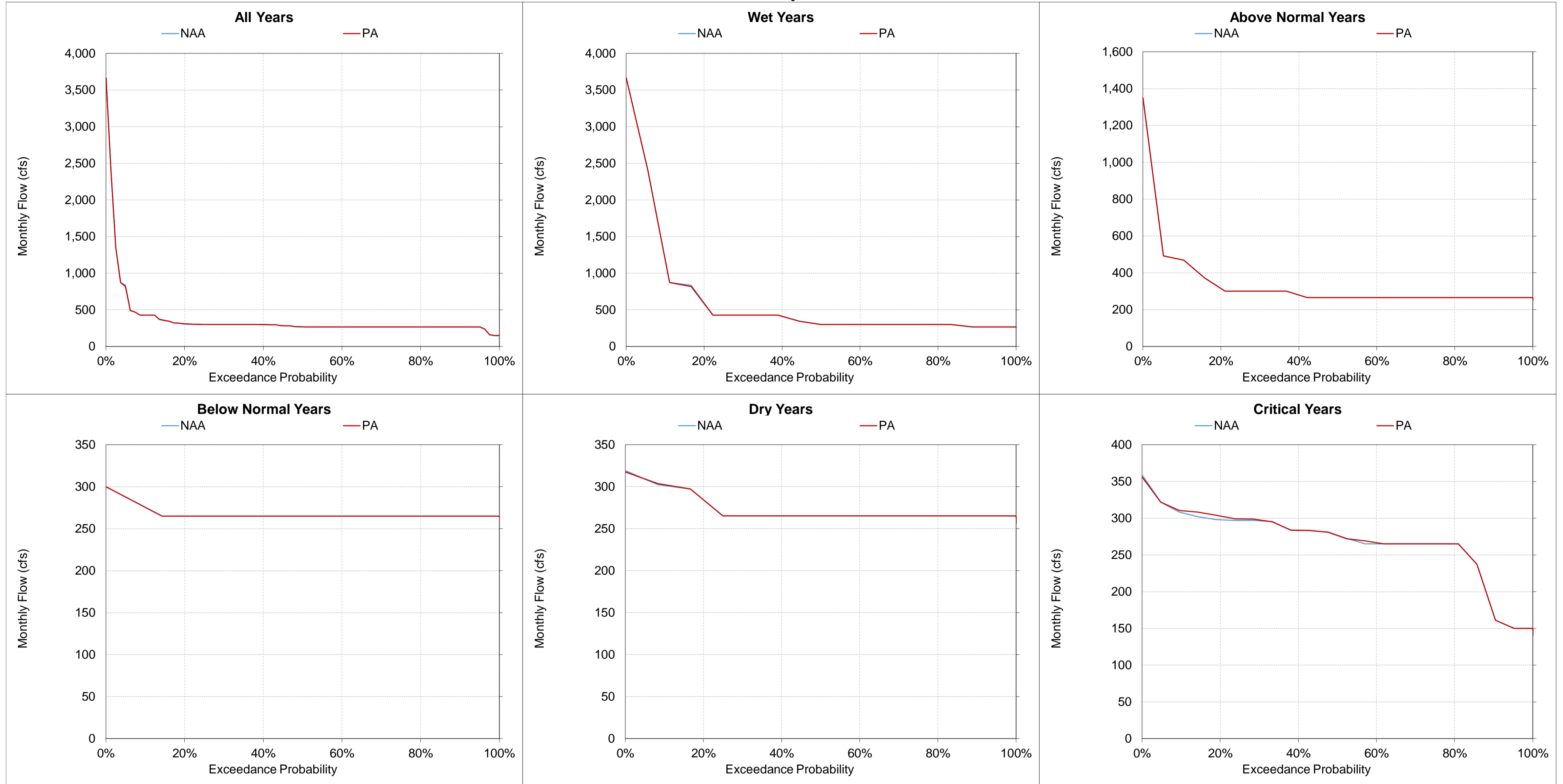
Figure 5.A.6-21-17. Stanislaus River at Goodwin, Monthly Flow July
