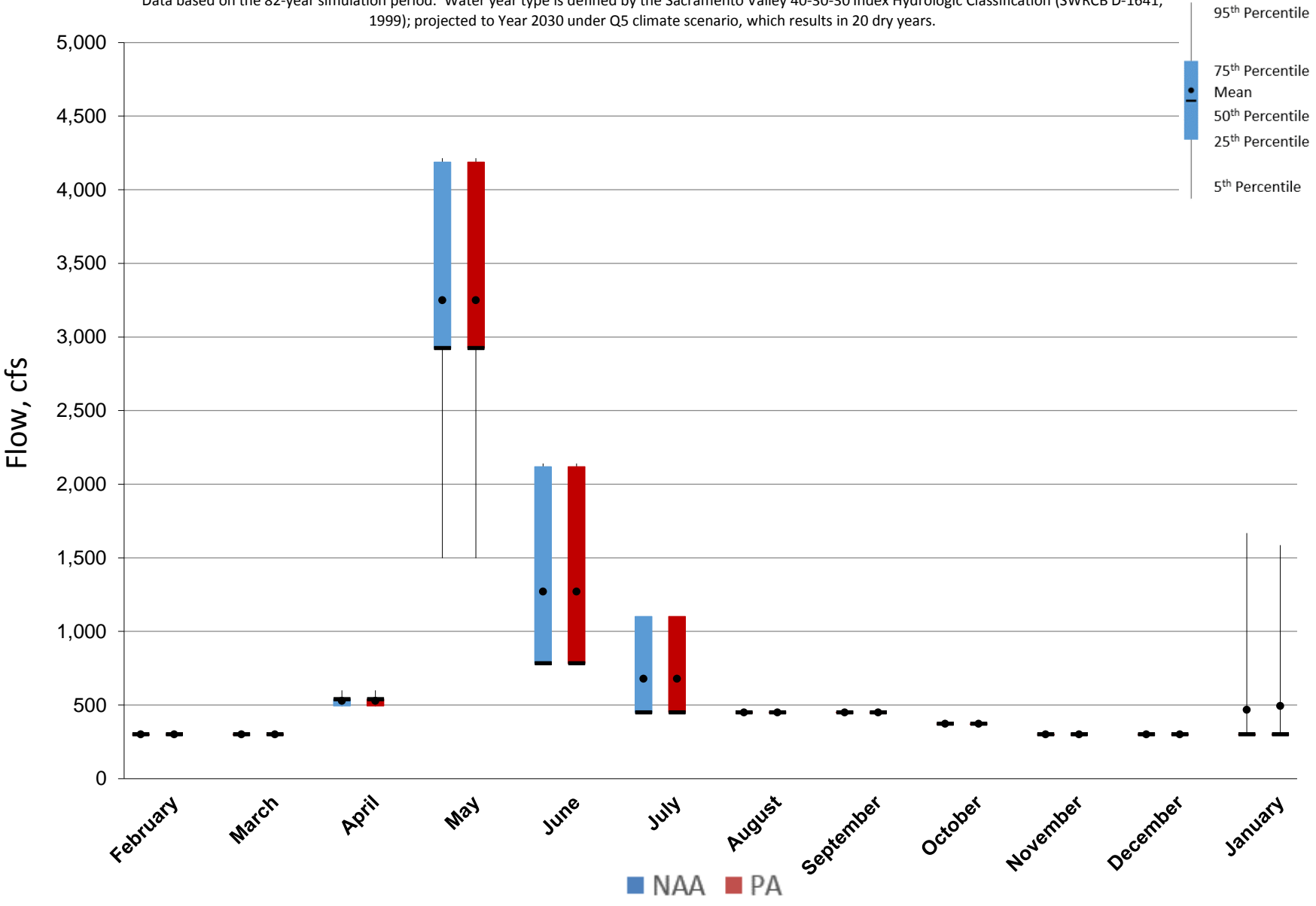
Figure 5.A.6-7-5. Monthly Flow Ranges For Trinity River below Lewiston Dam, Dry Years
