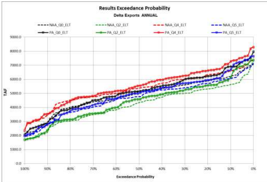
Figure 5.A.A.3-20 Long-term Average Annual Delta Exports at the North Delta Intakes and the South Delta Intakes for the NAA and PA under Q0, Q2, Q4 and Q5 climate scenarios at Year 2030
