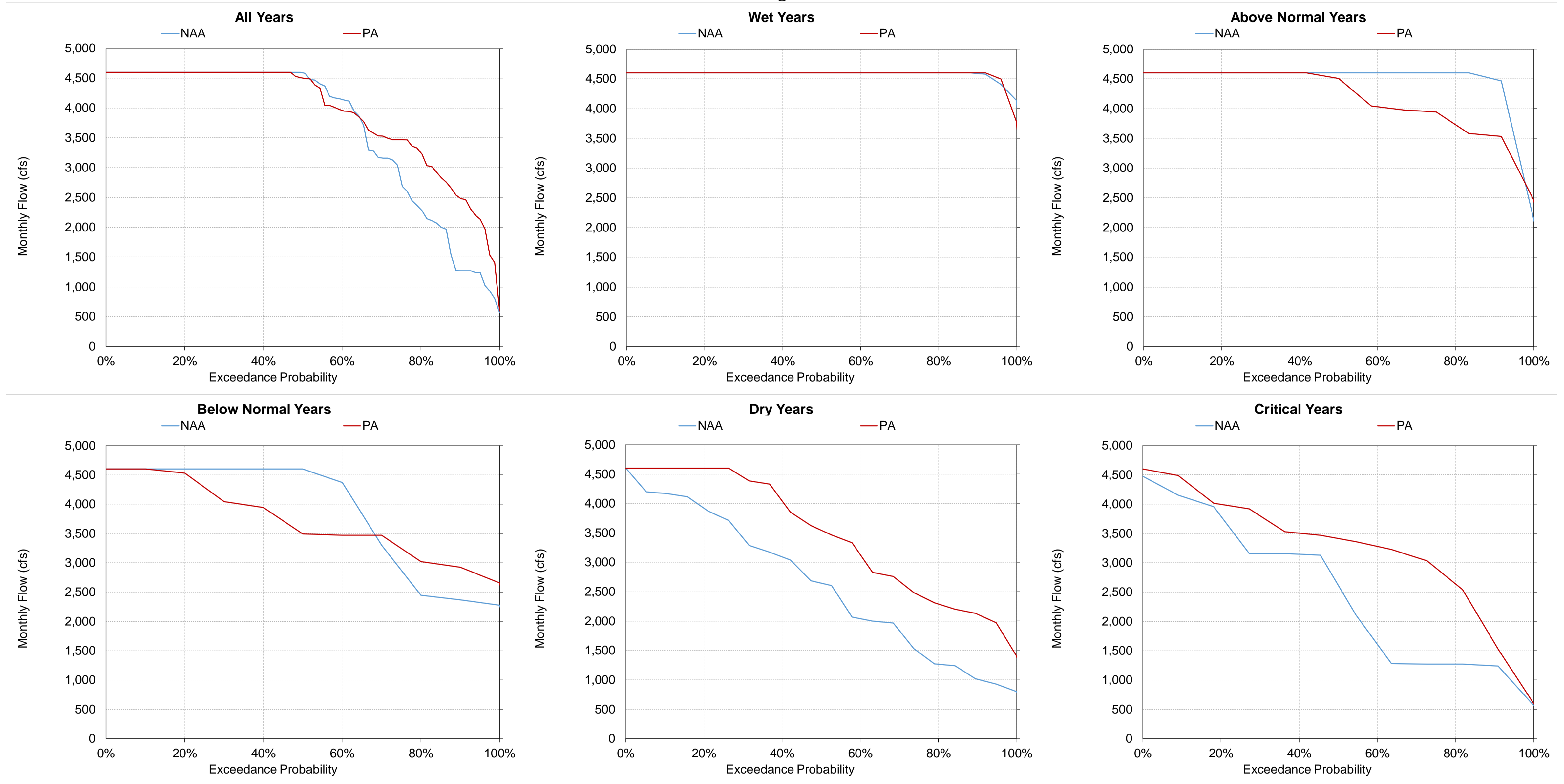
Figure 5.A.6-33-18. Total Jones Pumping Plant Exports, Monthly Flow August
