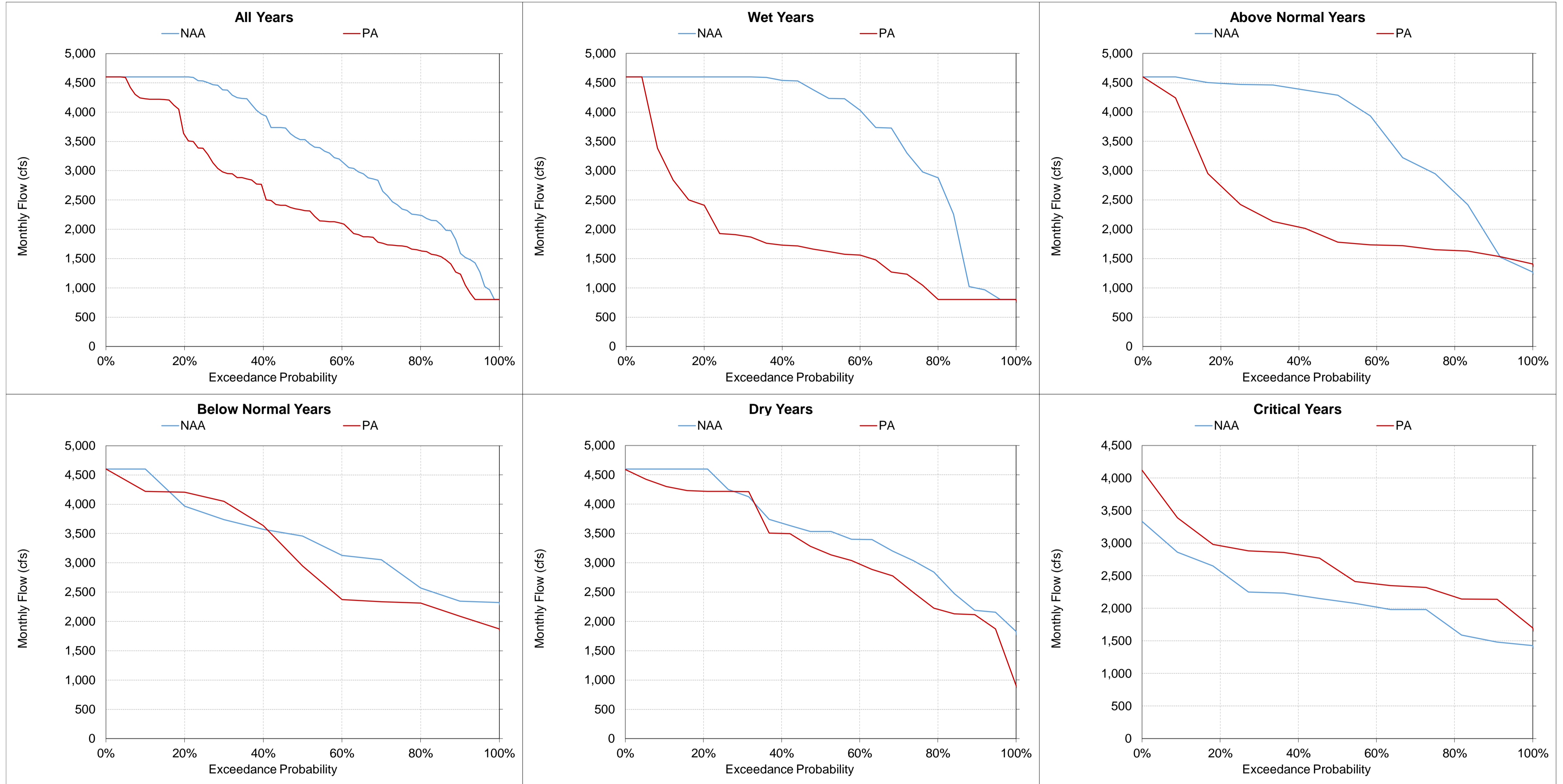
Figure 5.A.6-33-9. Total Jones Pumping Plant Exports, Monthly Flow November
