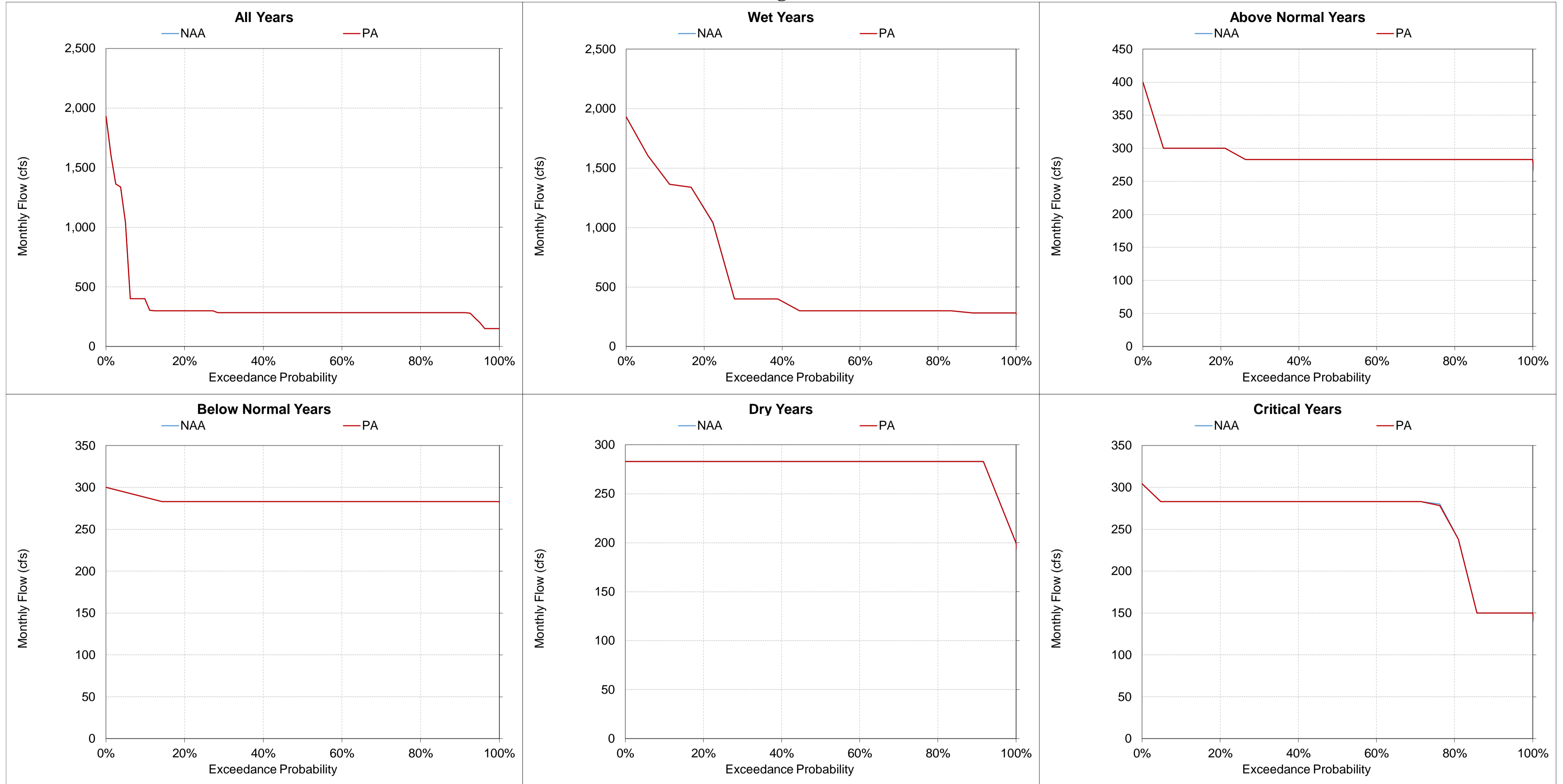
Figure 5.A.6-21-18. Stanislaus River at Goodwin, Monthly Flow August
