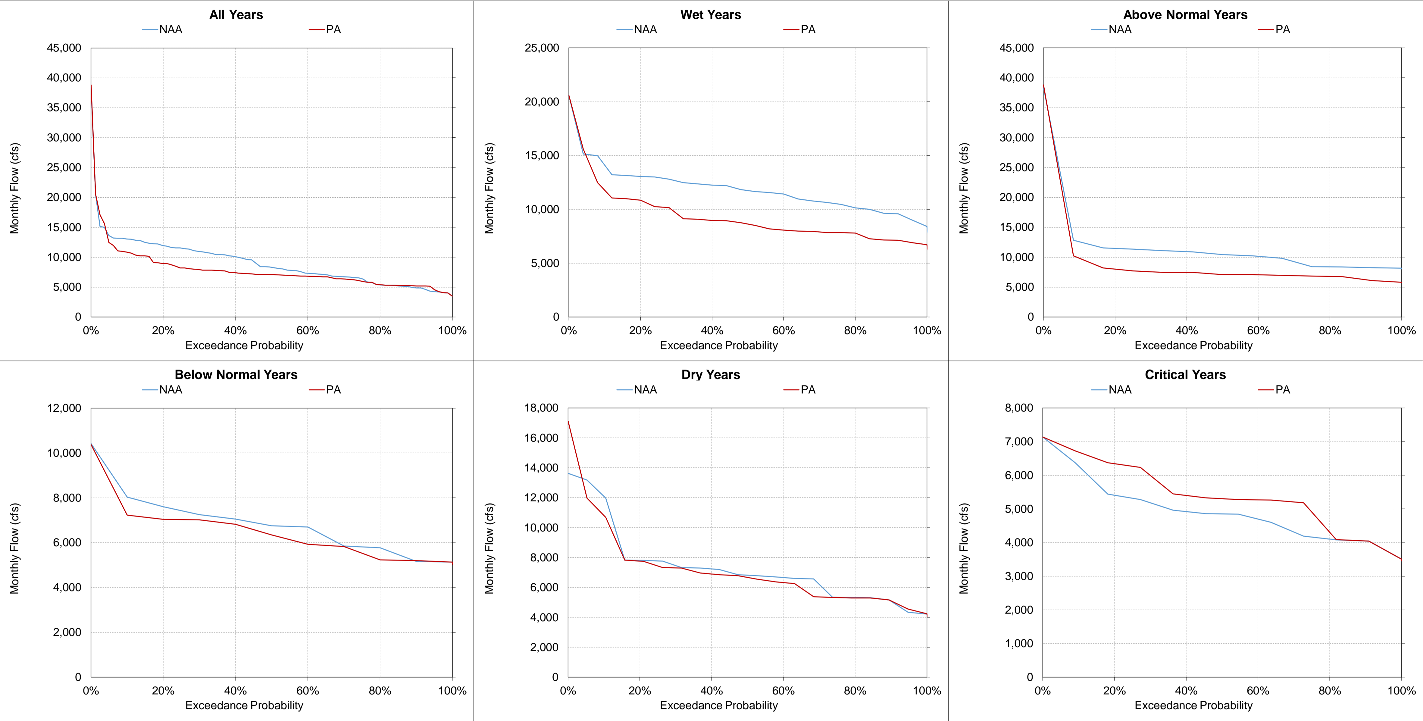
Figure 5.A.6-35-9. Sacramento River above Red Bluff Diversion Dam, Monthly Flow November
