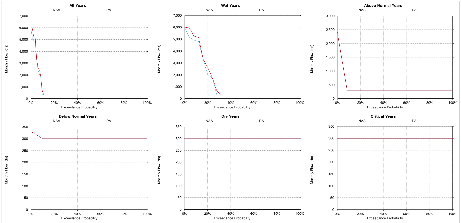
Figure 5.A.6-7-13. Trinity River below Lewiston Dam, Monthly Flow March
