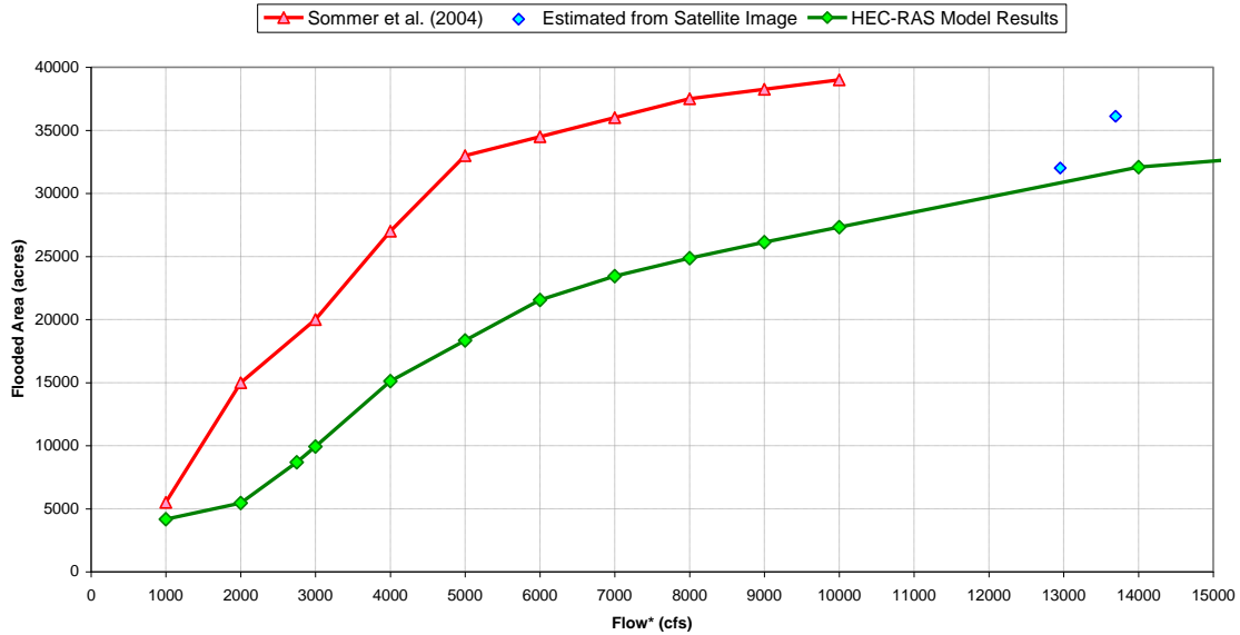
Figure 5.A.A.4-10. Comparison of flooded area for different models and models assumptions.
