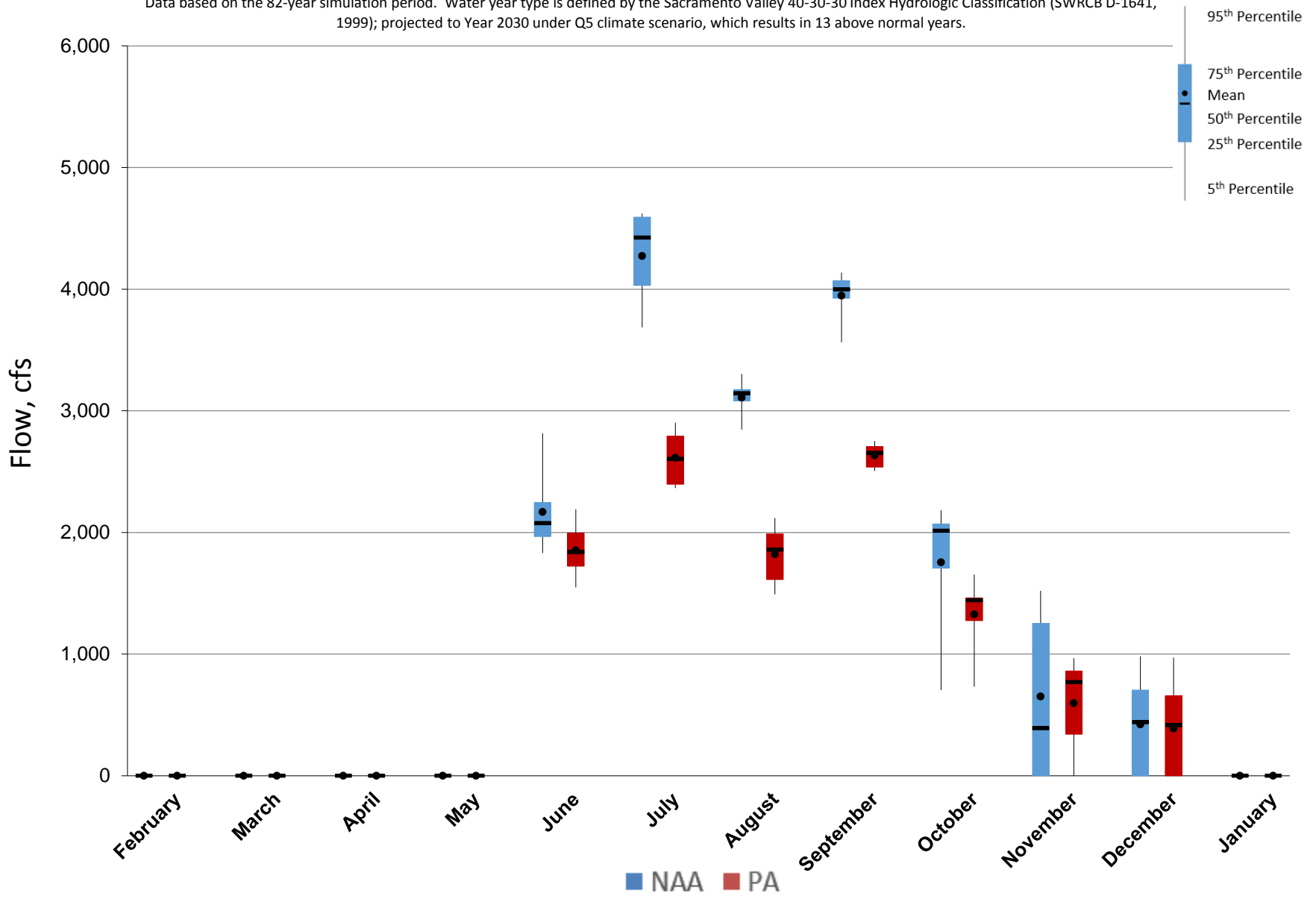
Figure 5.A.6-32-3. Monthly Flow Ranges For Delta Cross Channel, Above Normal Years
