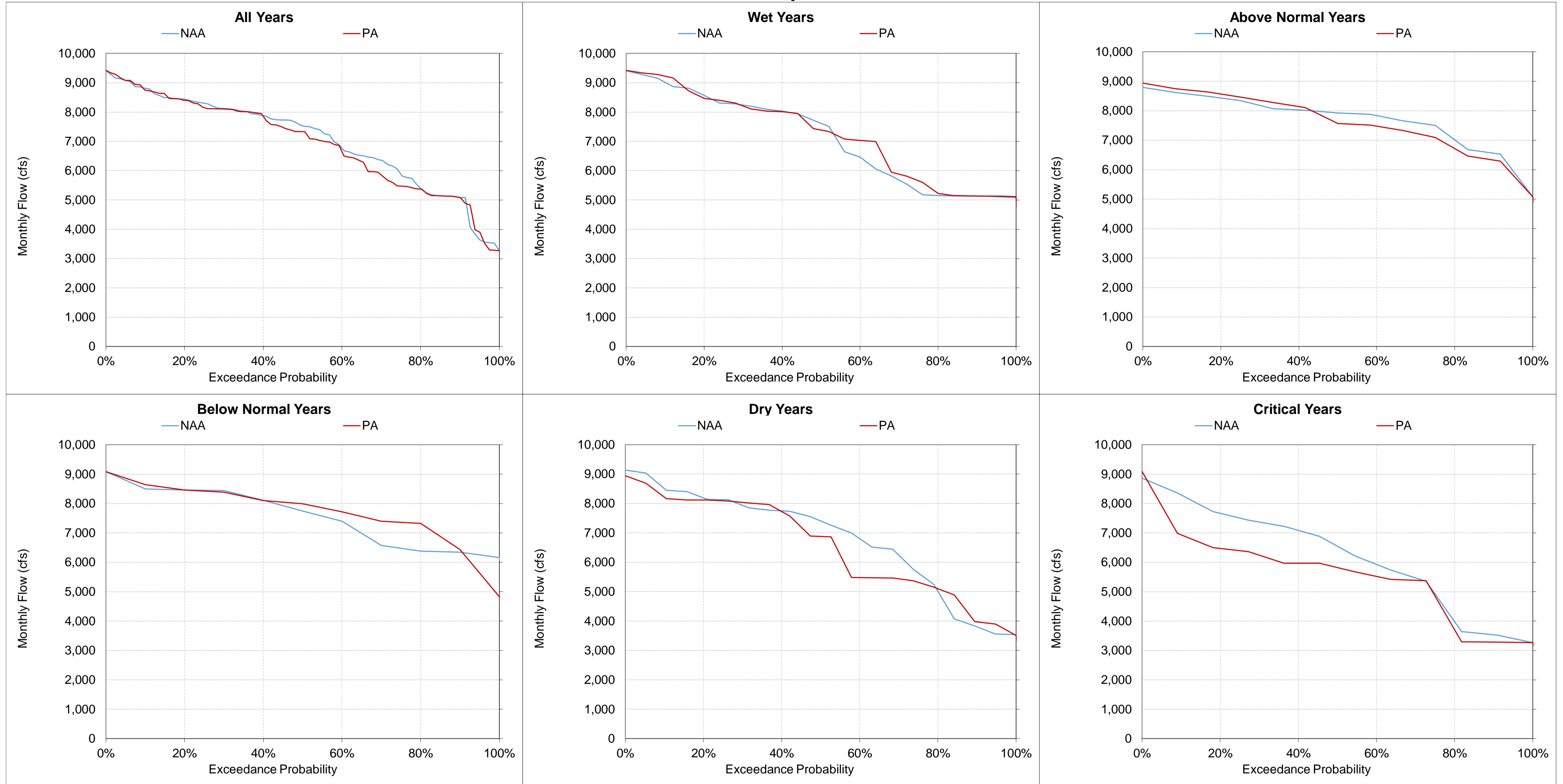
Figure 5.A.6-36-17. Sacramento River at Wilkins Slough, Monthly Flow July
