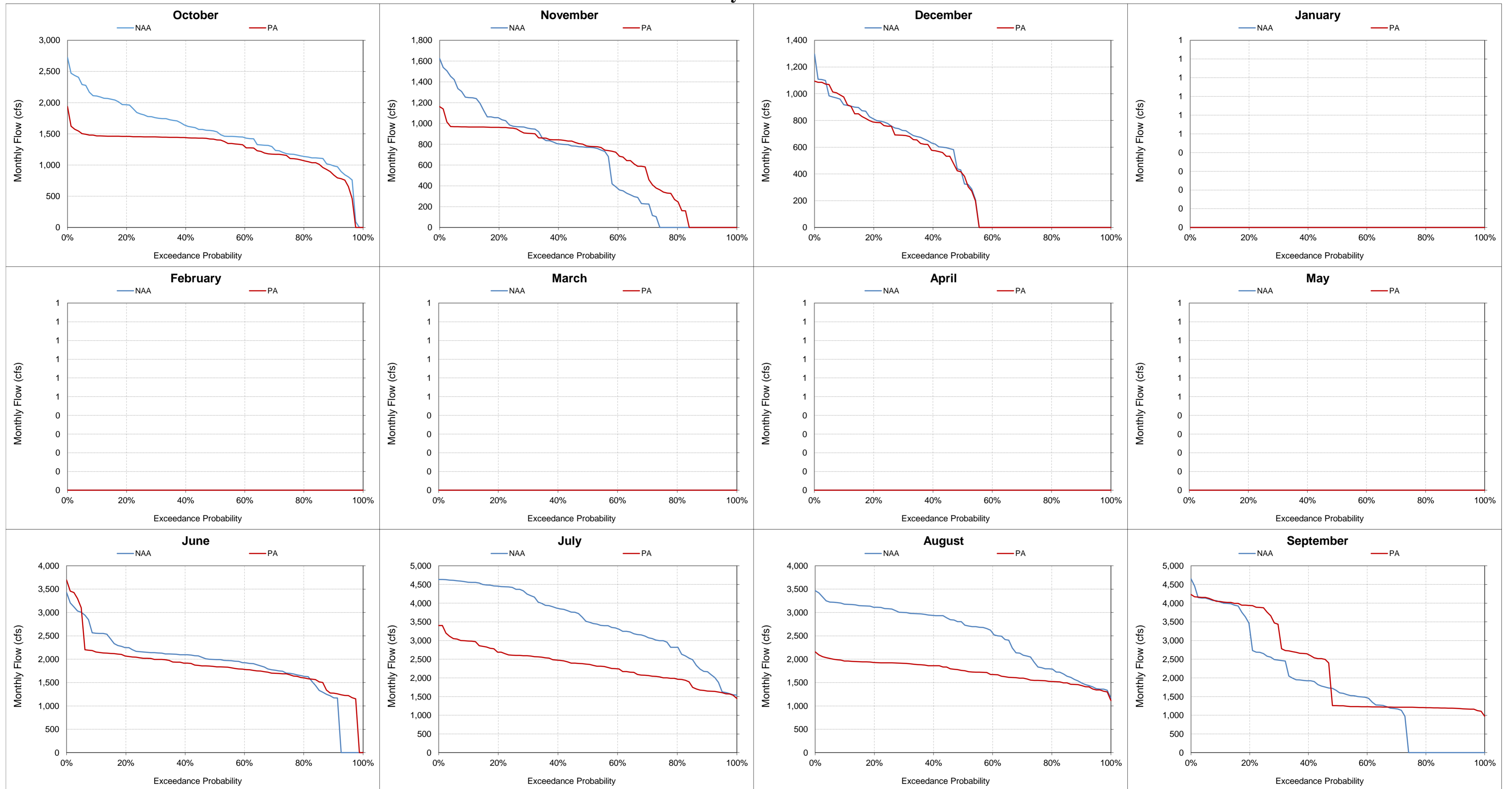
Figure 5.A.6-32-7. Delta Cross Channel, Monthly Flow Probability of Exceedance
