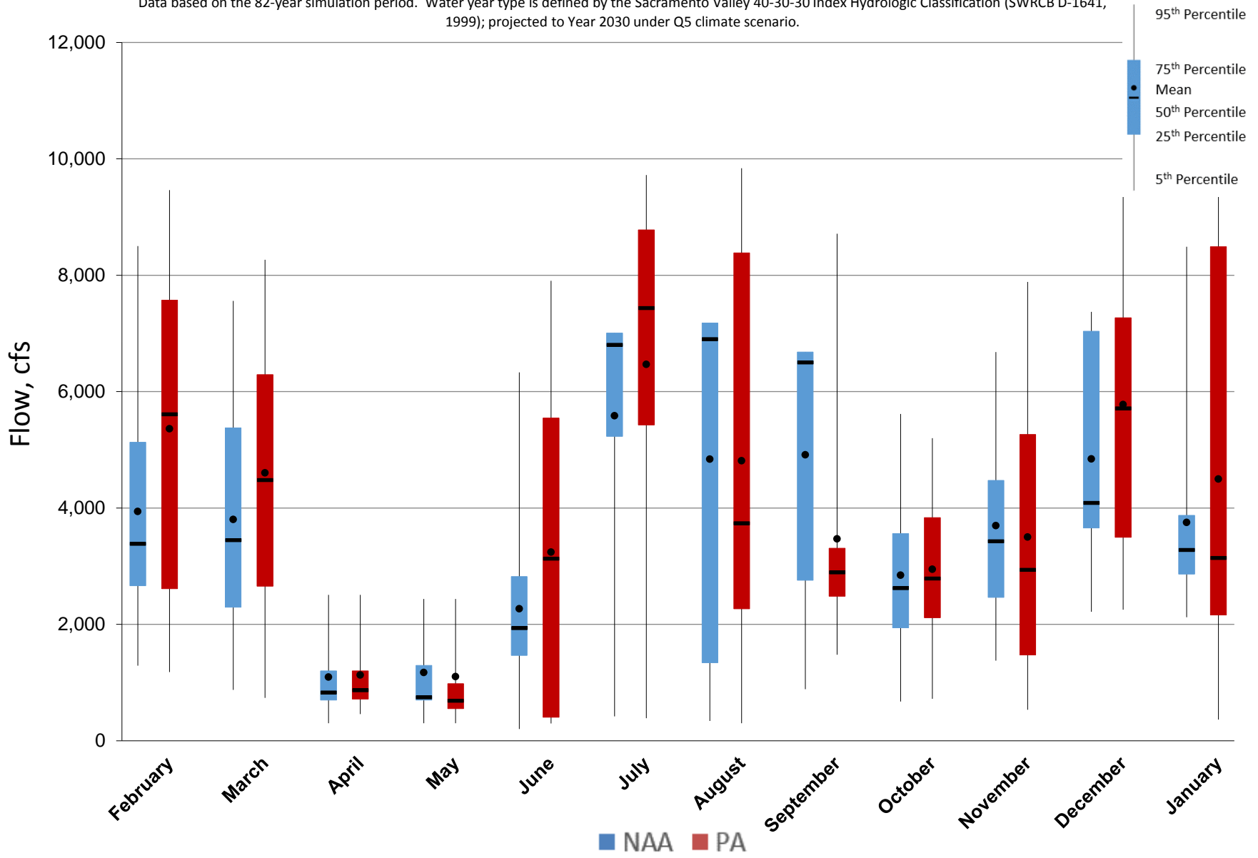
Figure 5.A.6-34-1. Monthly Flow Ranges For Total Banks Pumping Plant Exports, All Years
