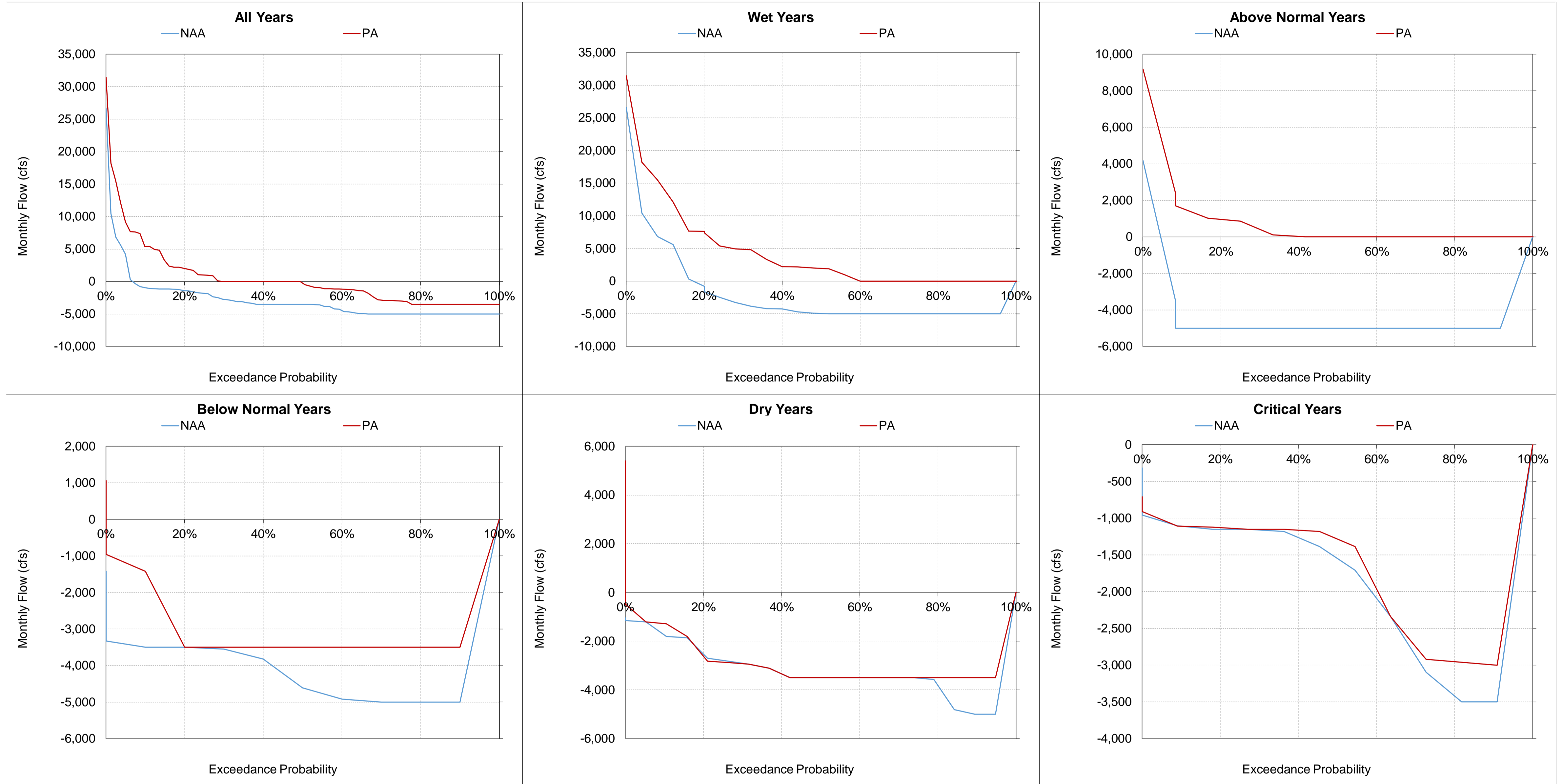
Figure 5.A.6-25-13. Old and Middle River, Monthly Flow March
