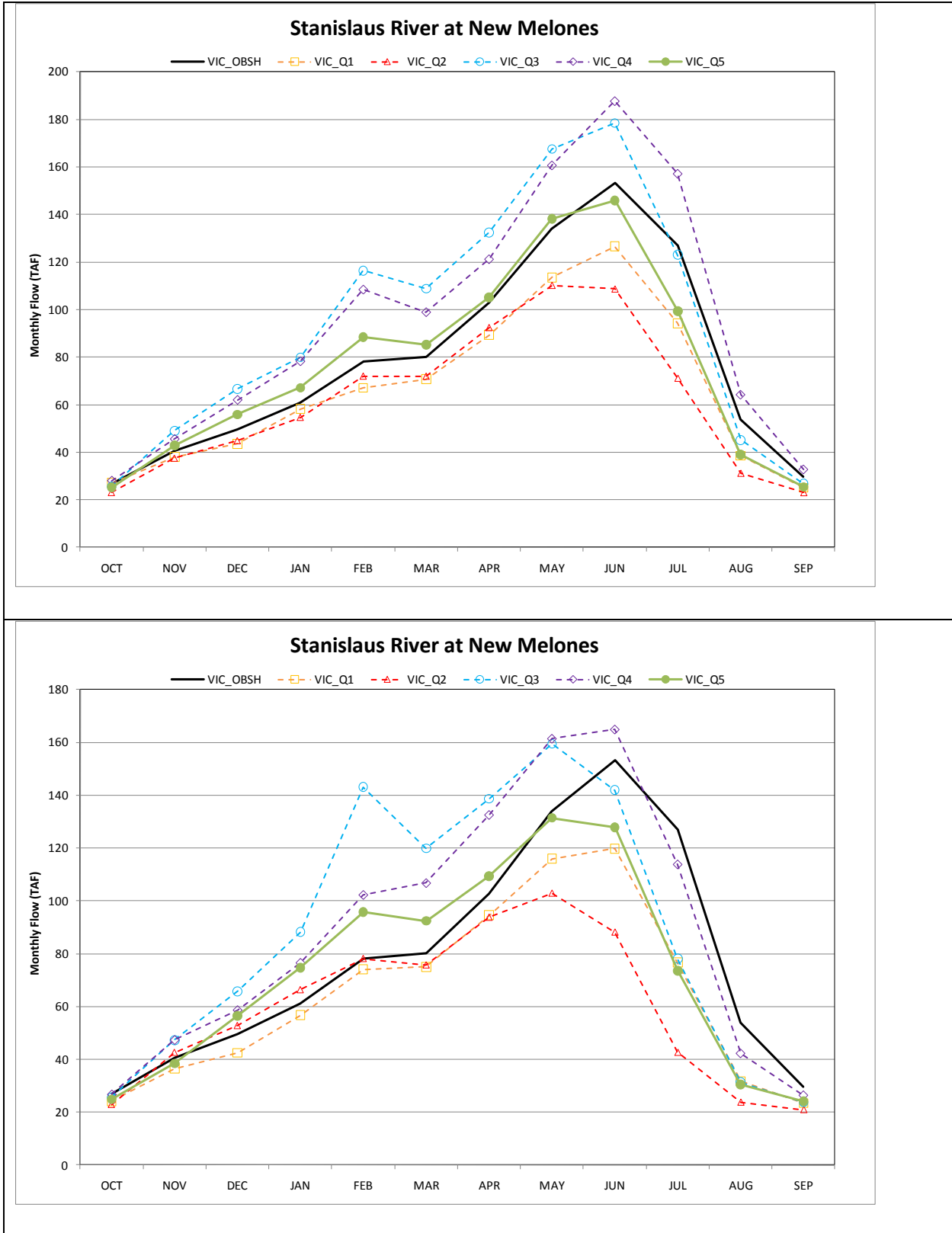
Figure 5.A.A.2-12. Simulated Changes in Monthly Natural Streamflow for Stanislaus River at New Melones (top, 2025 changes; bottom, 2060 changes).
