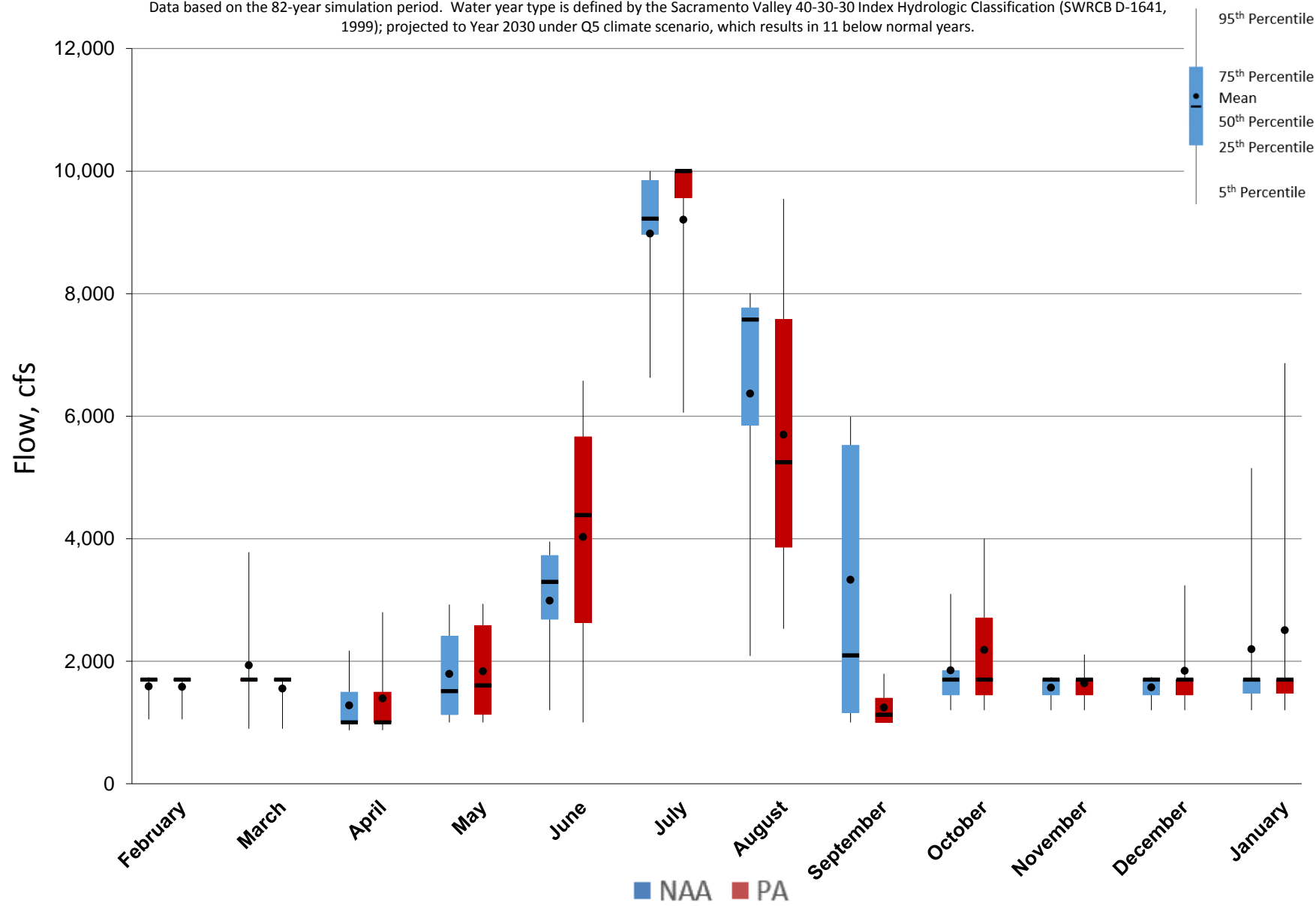
Figure 5.A.6-12-4. Monthly Flow Ranges For Feather River below Thermalito Diversion Dam, Below Normal Years
