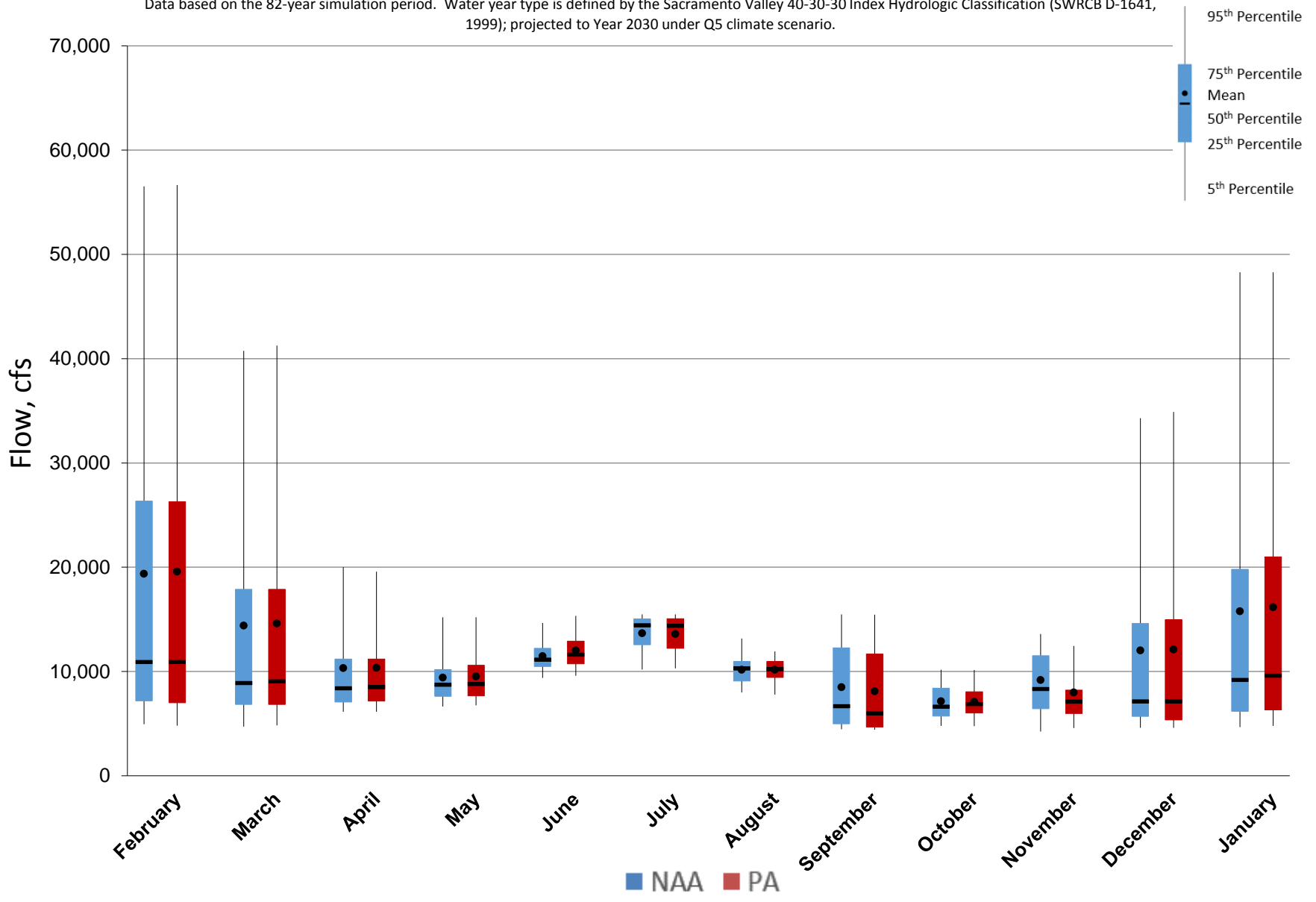
Figure 5.A.6-35-1. Monthly Flow Ranges For Sacramento River above Red Bluff Diversion Dam, All Years
