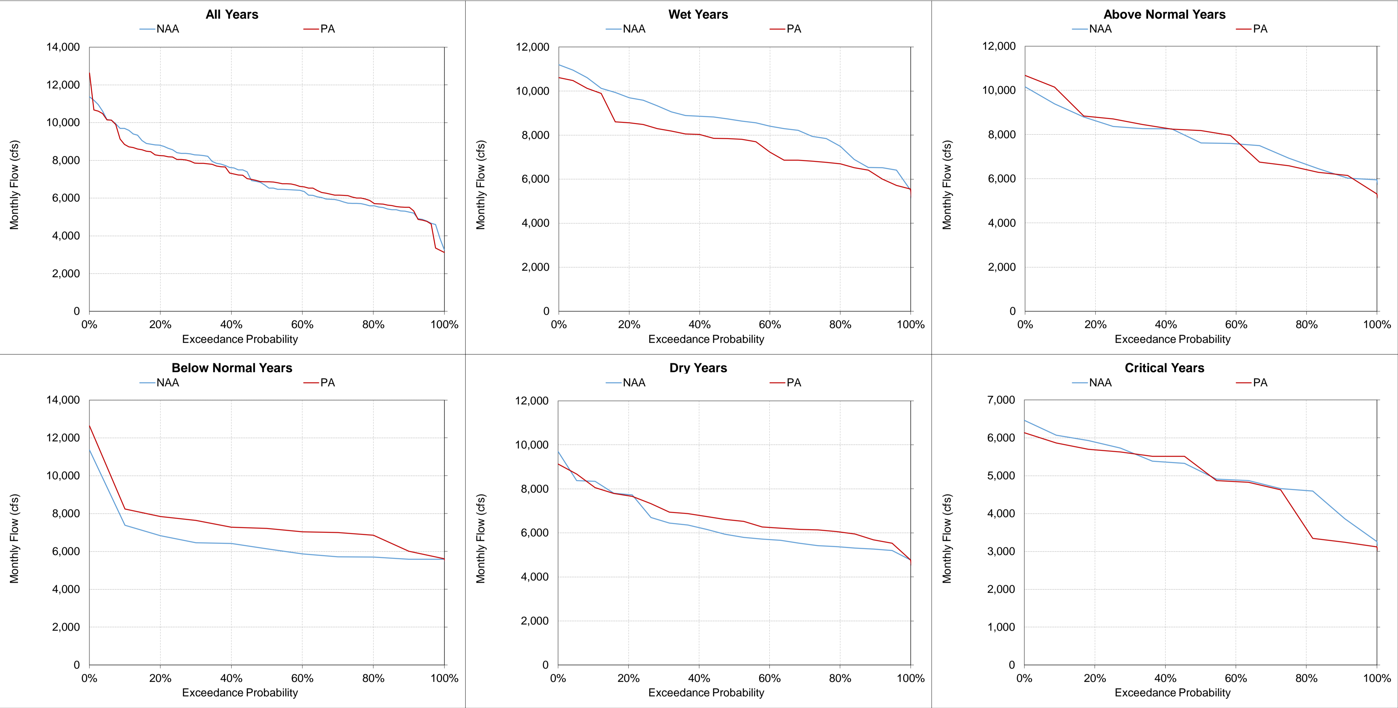
Figure 5.A.6-35-8. Sacramento River above Red Bluff Diversion Dam, Monthly Flow October
