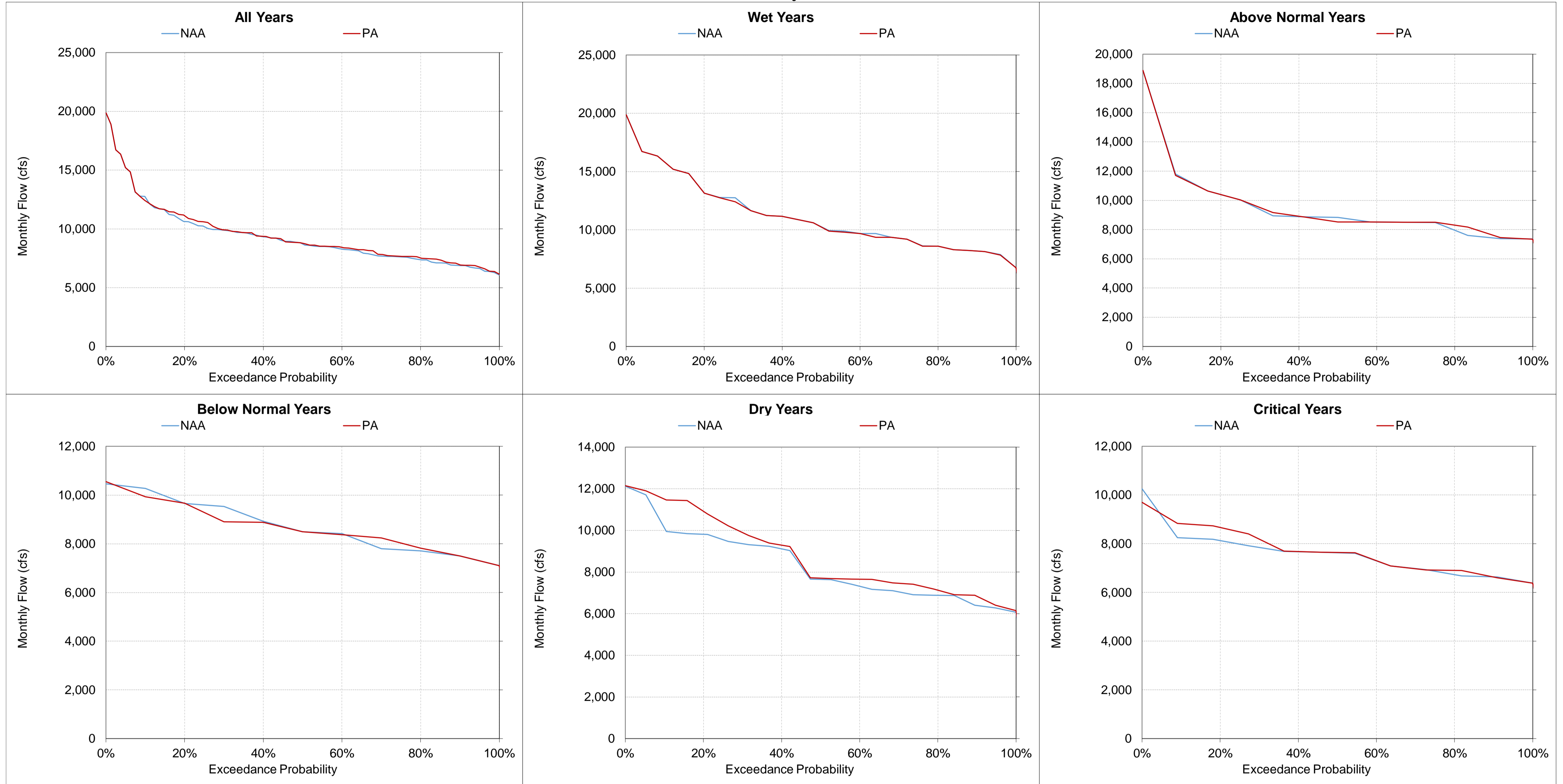
Figure 5.A.6-35-15. Sacramento River above Red Bluff Diversion Dam, Monthly Flow May
