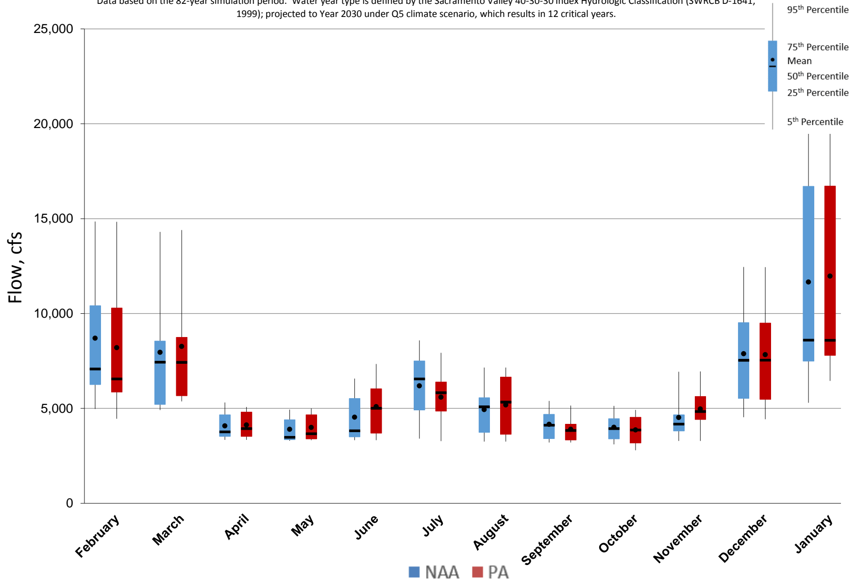
Figure 5.A.6-36-6. Monthly Flow Ranges For Sacramento River at Wilkins Slough, Critical Years
