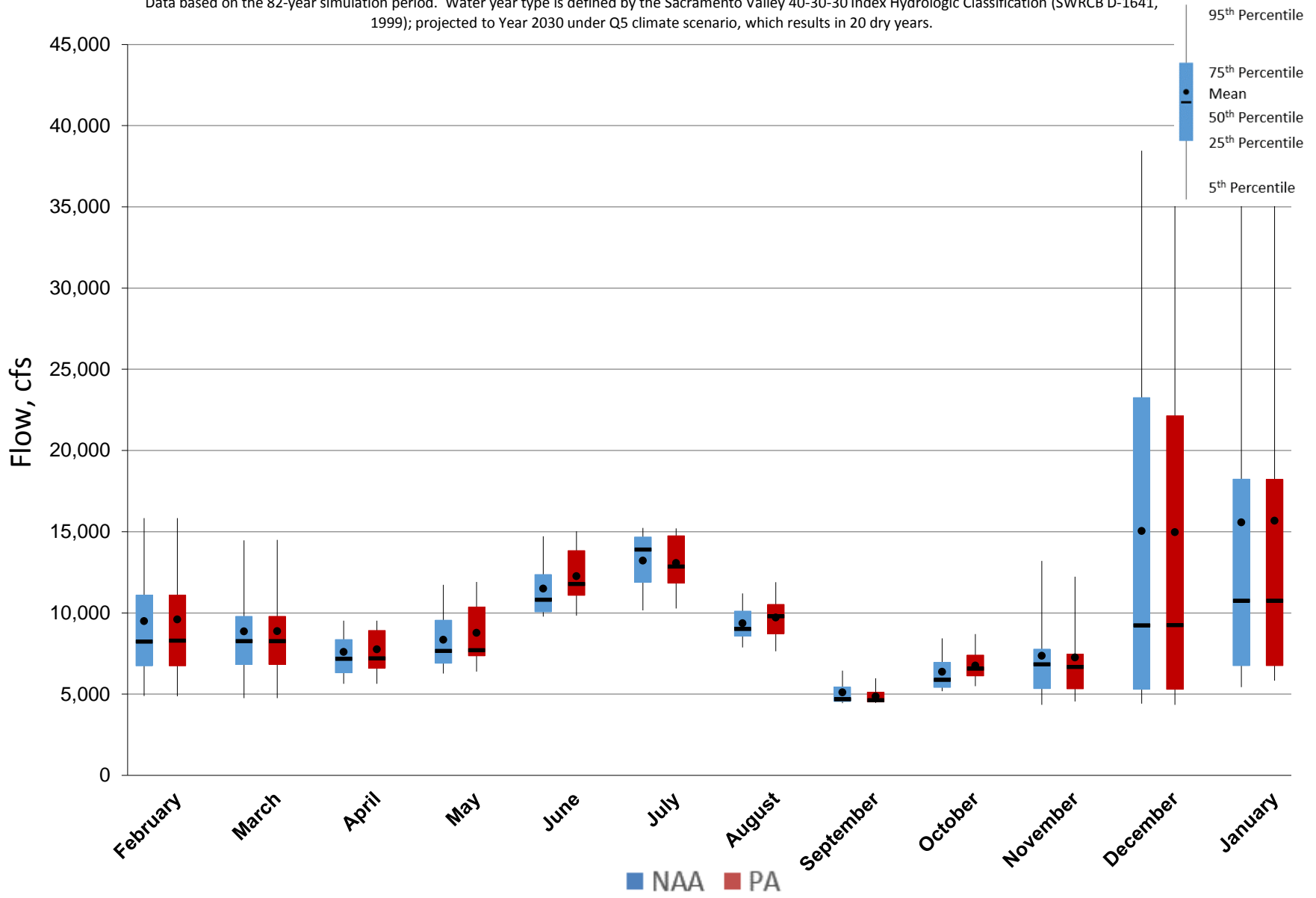
Figure 5.A.6-35-5. Monthly Flow Ranges For Sacramento River above Red Bluff Diversion Dam, Dry Years
