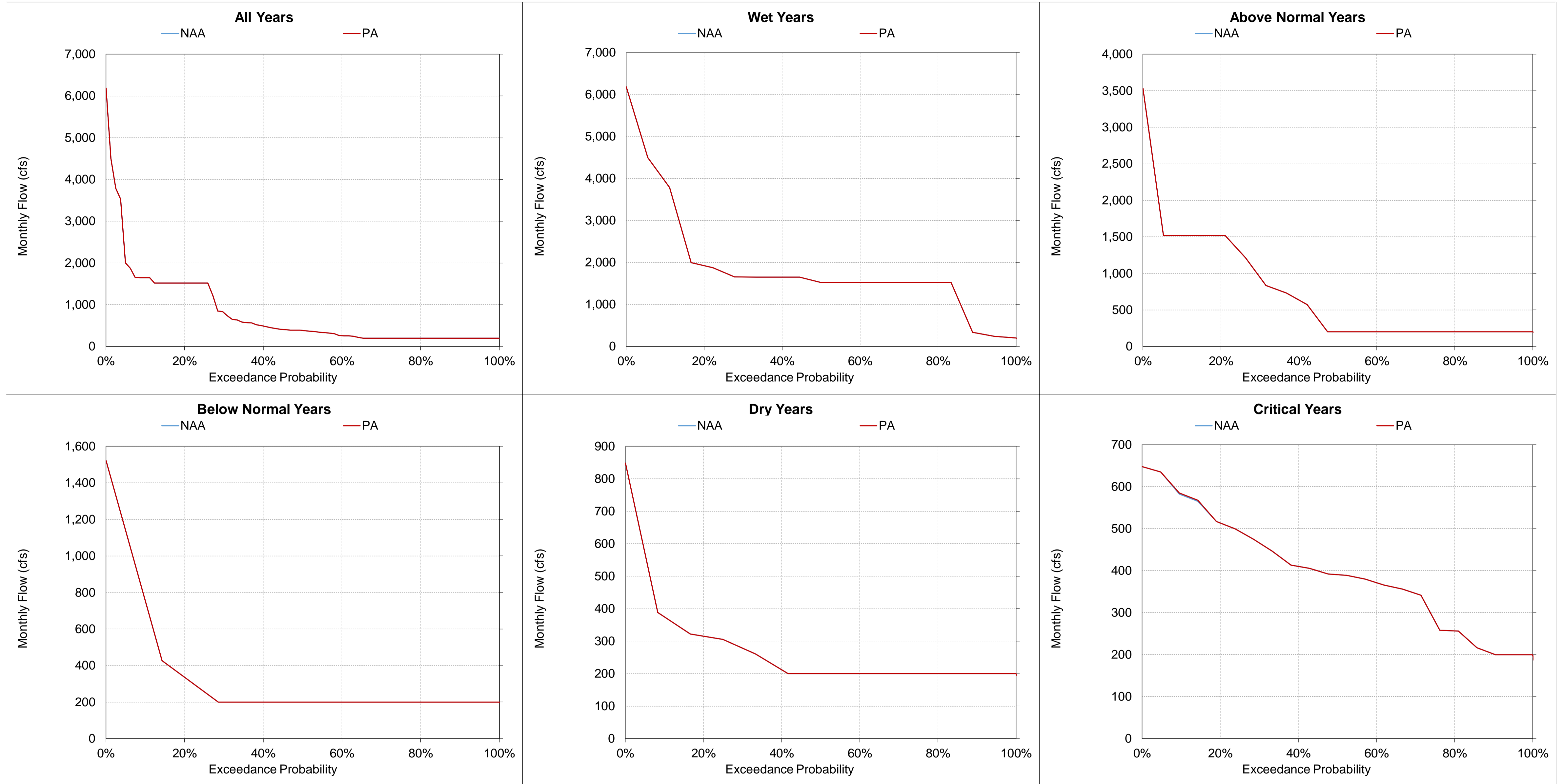
Figure 5.A.6-21-13. Stanislaus River at Goodwin, Monthly Flow March
