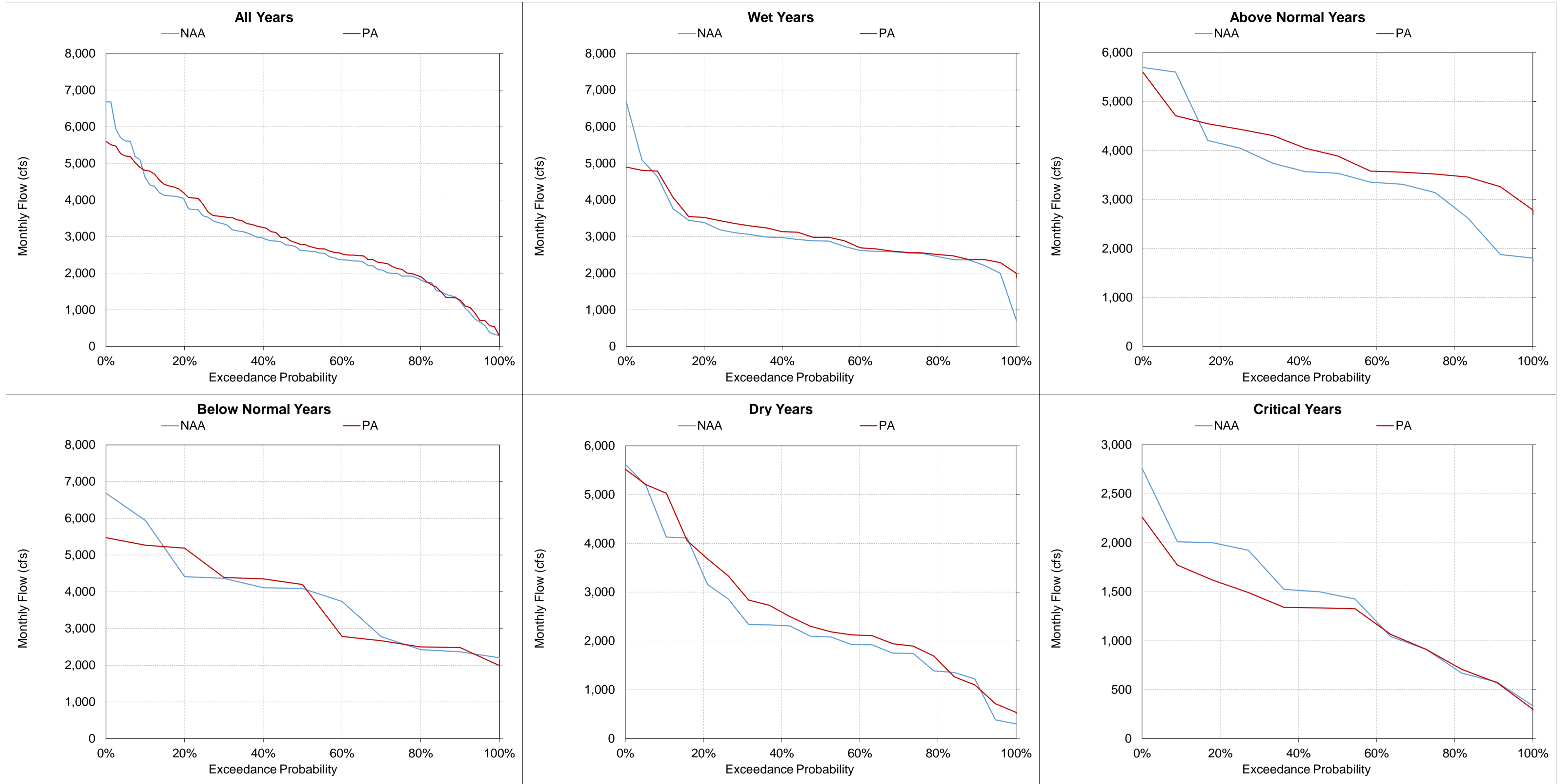
Figure 5.A.6-34-8. Total Banks Pumping Plant Exports, Monthly Flow October
