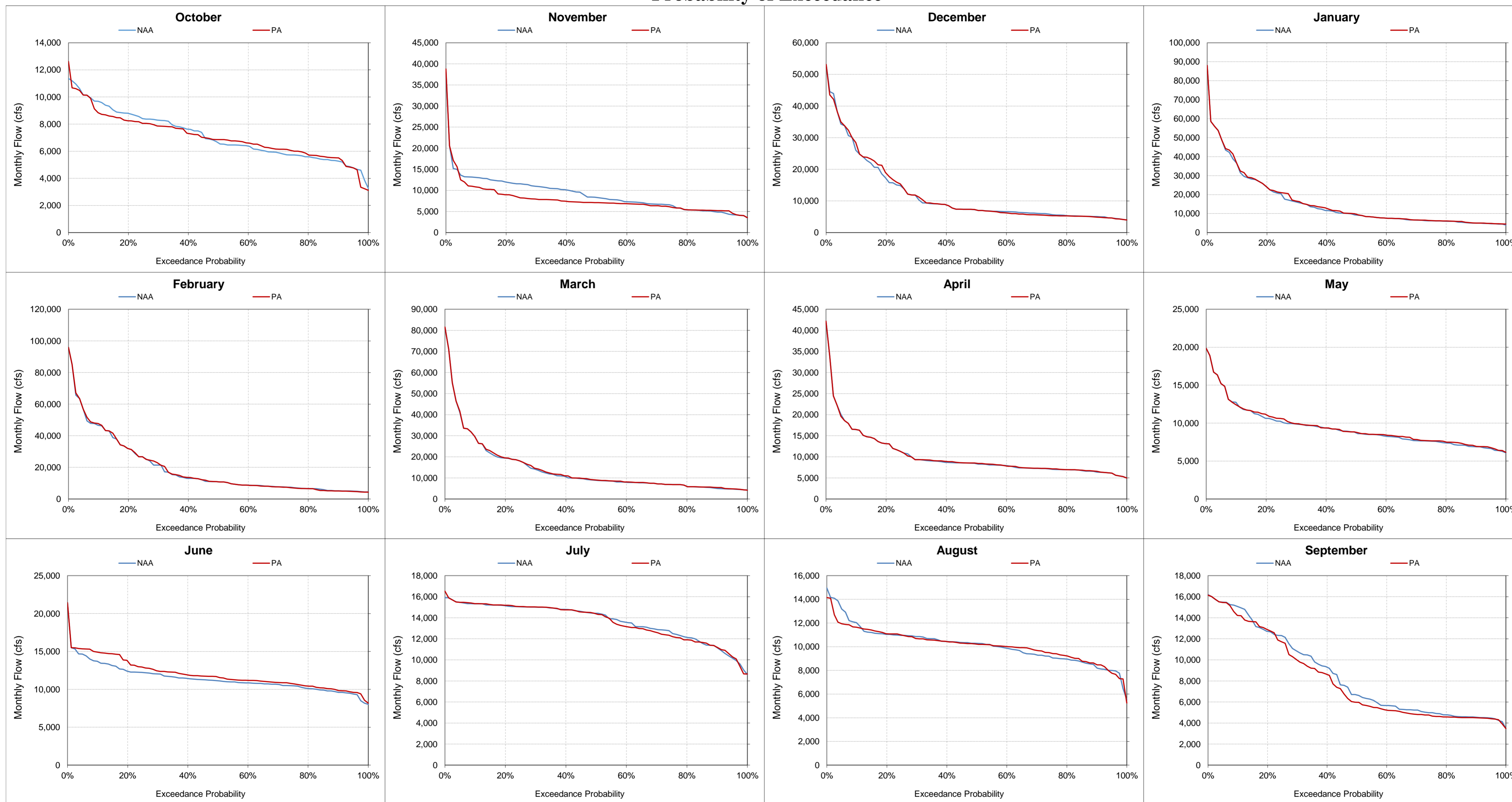
Figure 5.A.6-35-7. Sacramento River above Red Bluff Diversion Dam, Monthly Flow Probability of Exceedance
