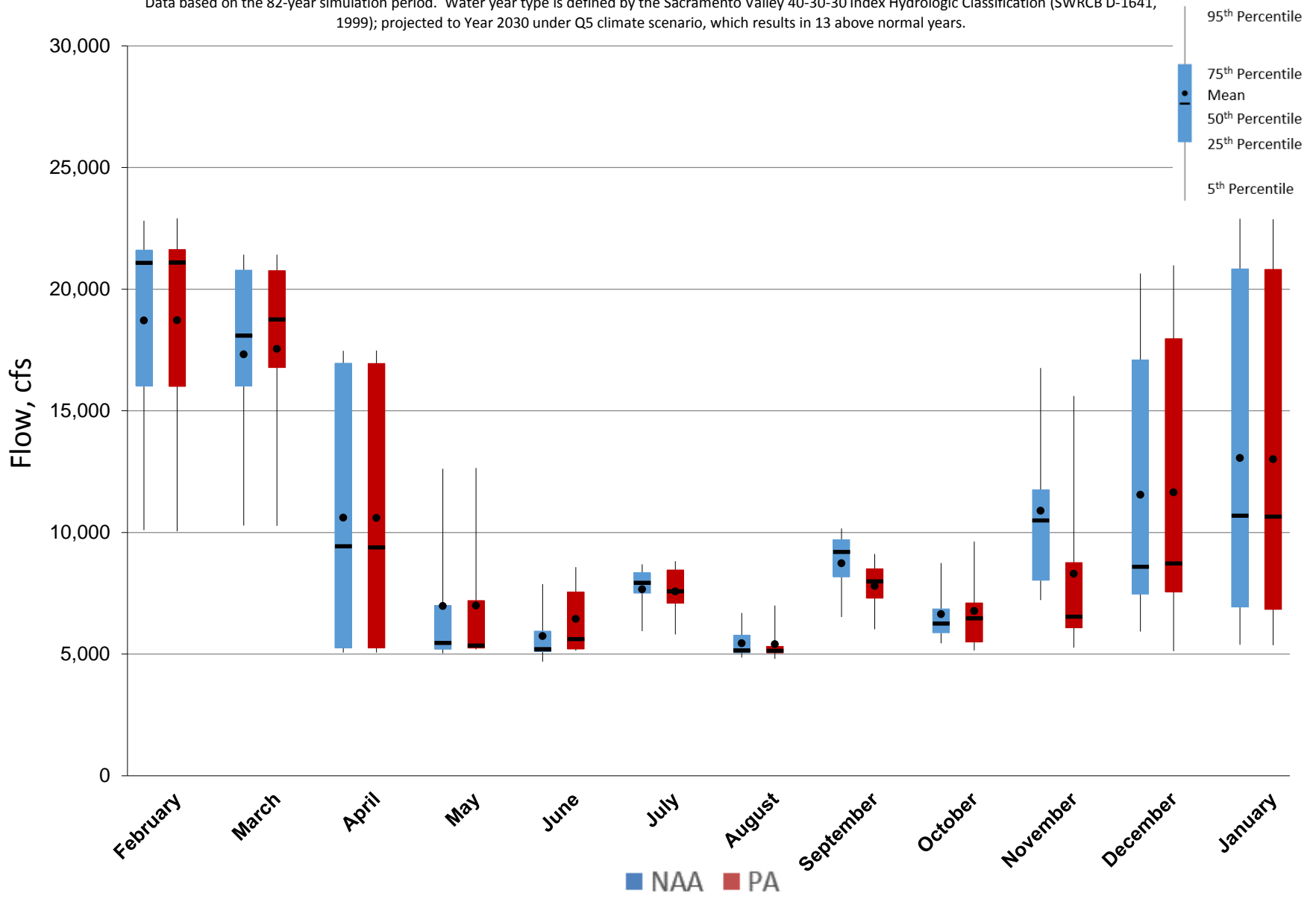
Figure 5.A.6-36-3. Monthly Flow Ranges For Sacramento River at Wilkins Slough, Above Normal Years
