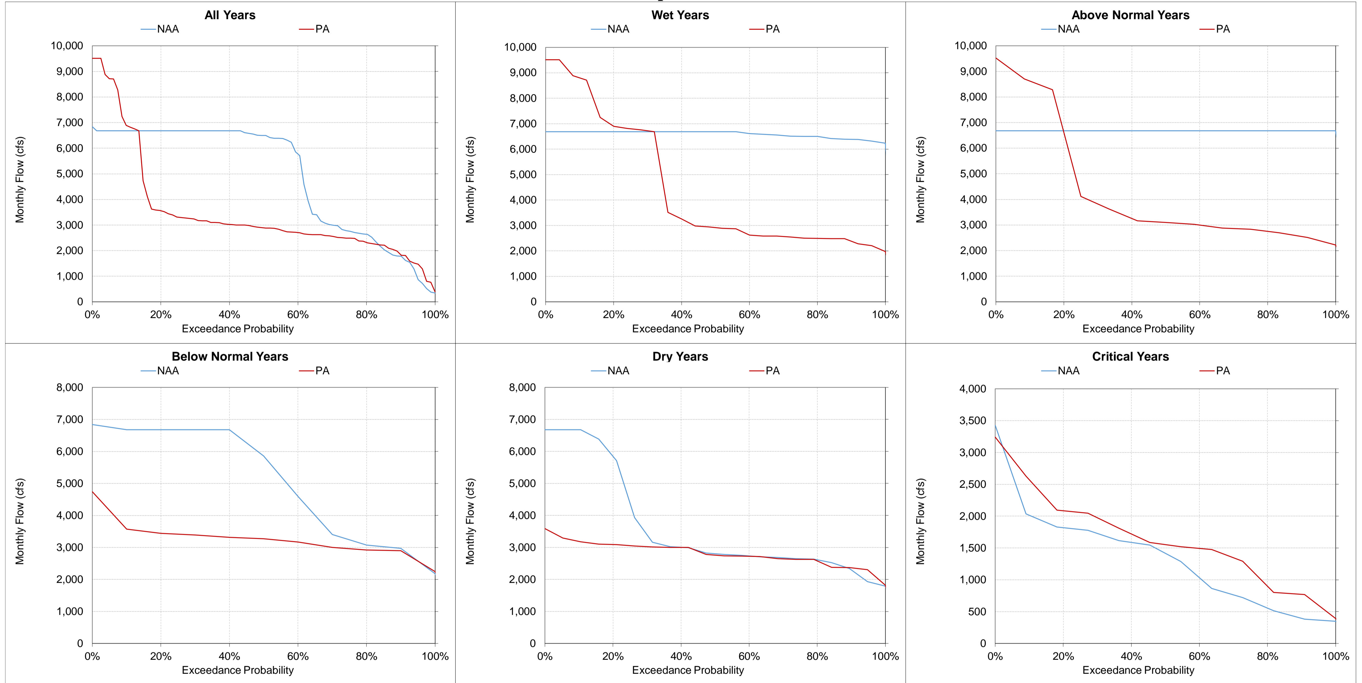
Figure 5.A.6-34-19. Total Banks Pumping Plant Exports, Monthly Flow September
