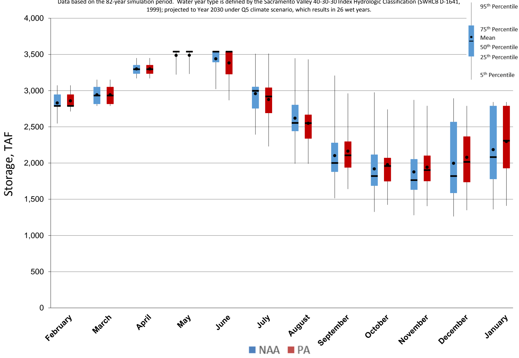
Figure 5.A.6-4-2. End of Month Storage Ranges For Lake Oroville, Wet Years
