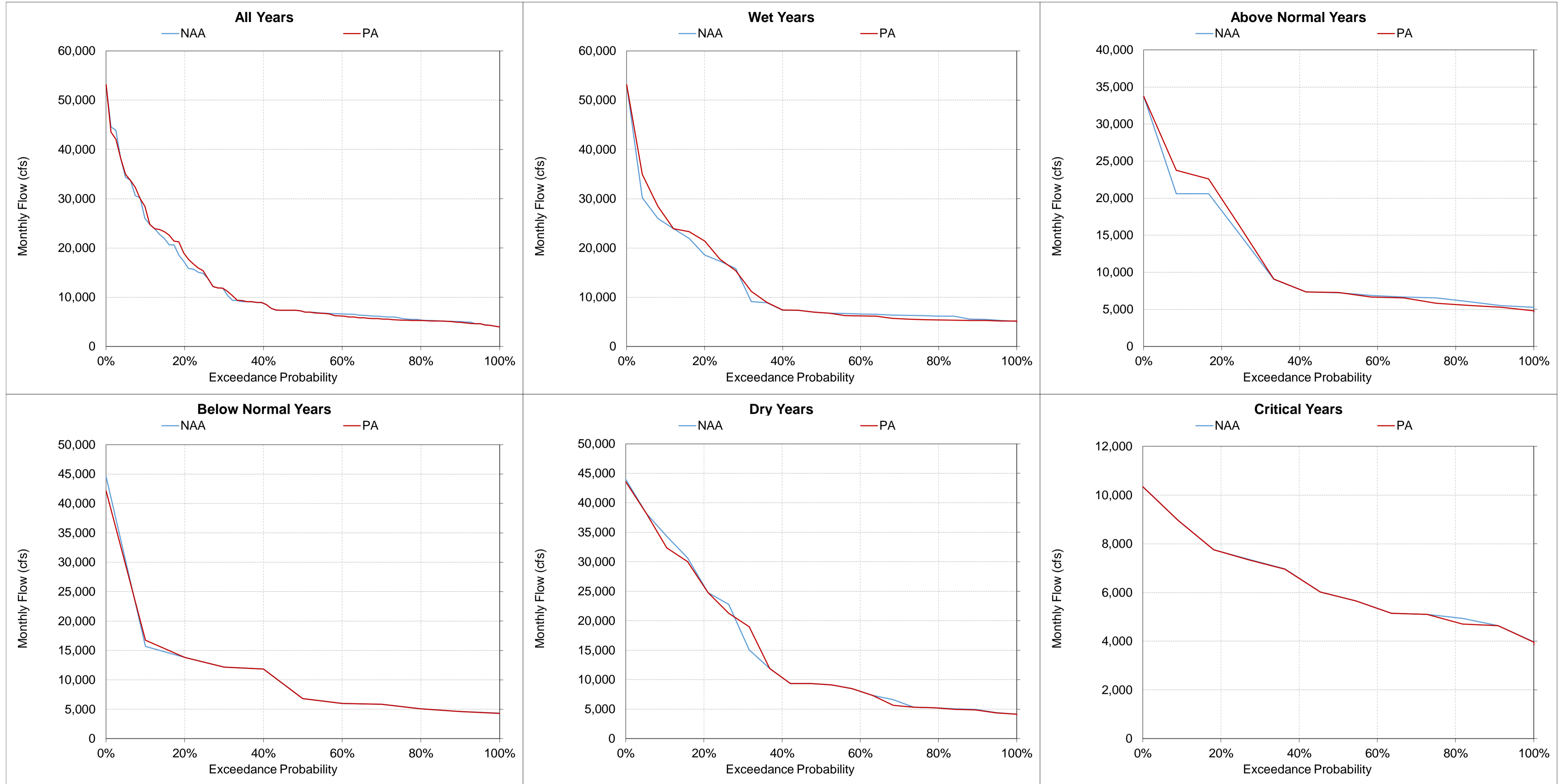
Figure 5.A.6-35-10. Sacramento River above Red Bluff Diversion Dam, Monthly Flow December
