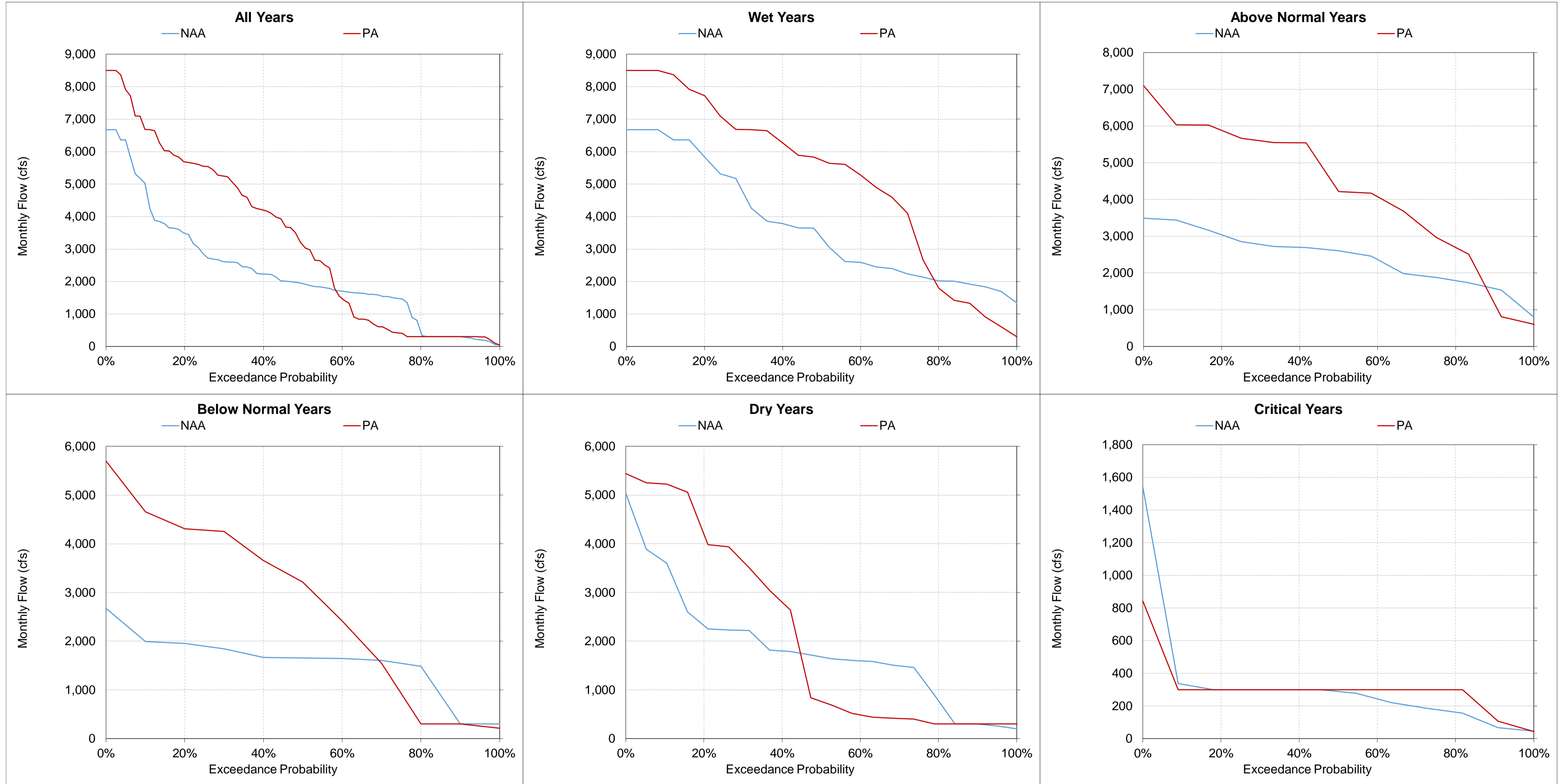
Figure 5.A.6-34-16. Total Banks Pumping Plant Exports, Monthly Flow June
