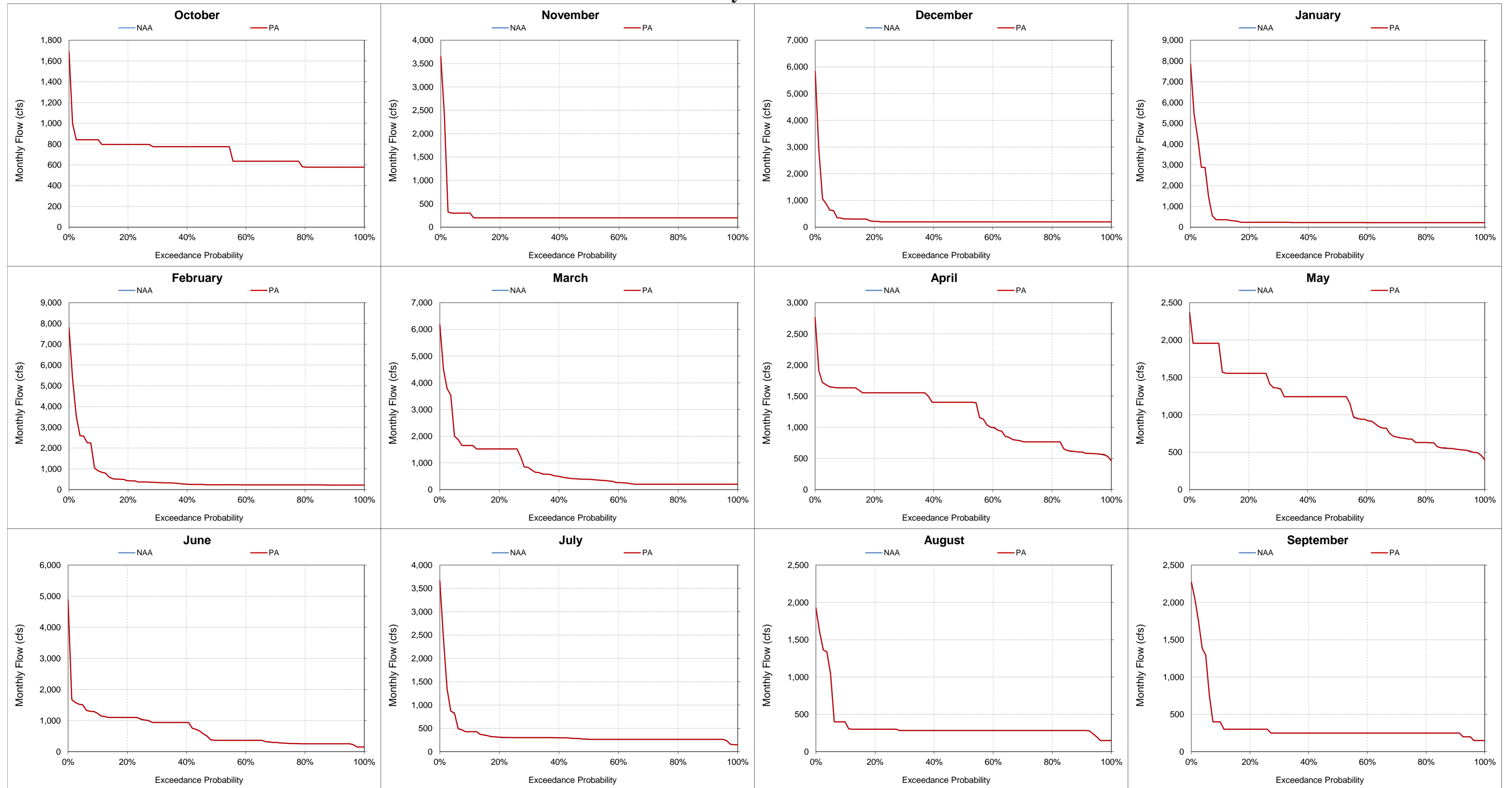
Figure 5.A.6-21-7. Stanislaus River at Goodwin, Monthly Flow Probability of Exceedance
