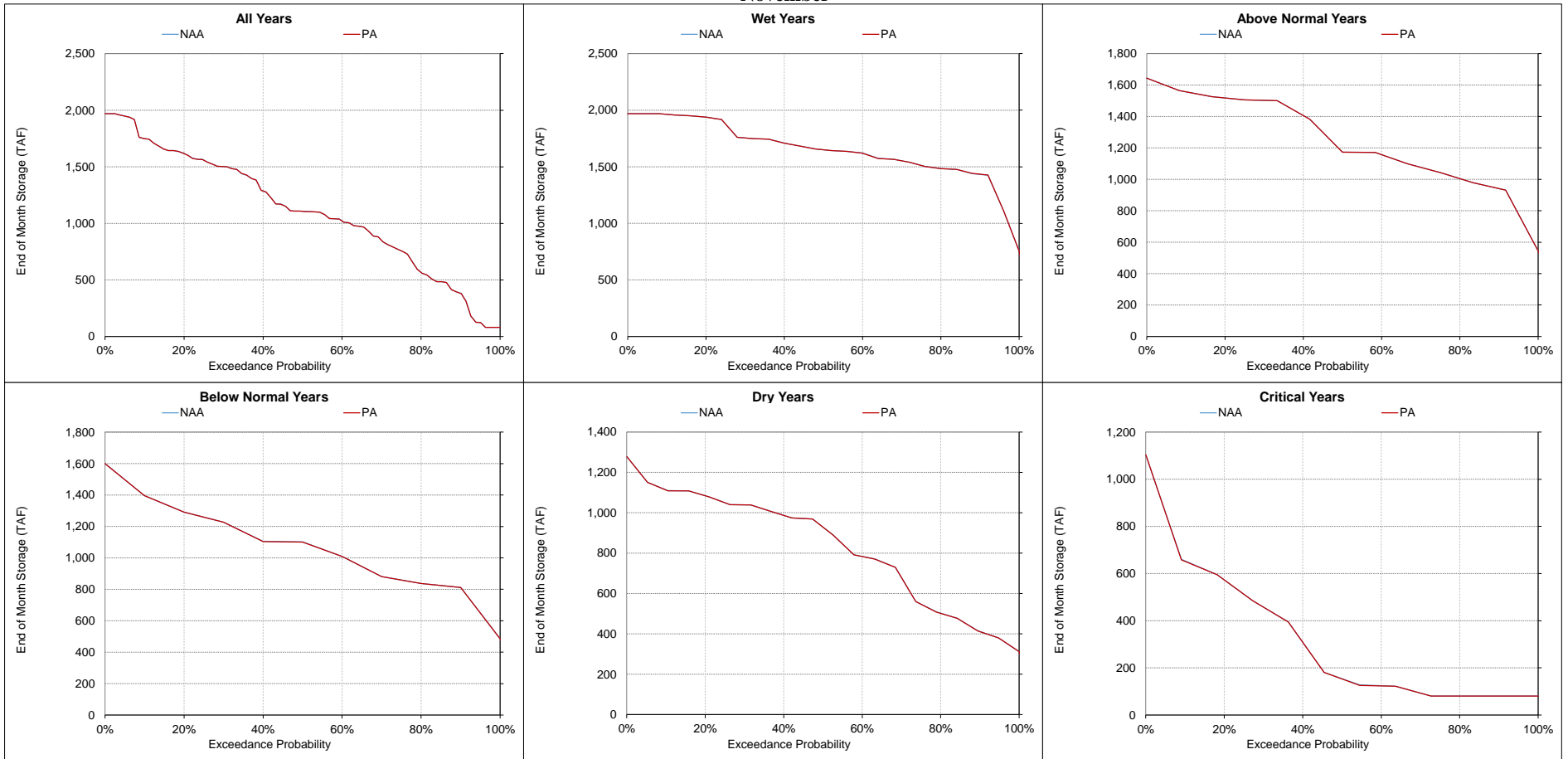
Figure 5.A.6-9. New Melones Lake, End of Month Storage November
