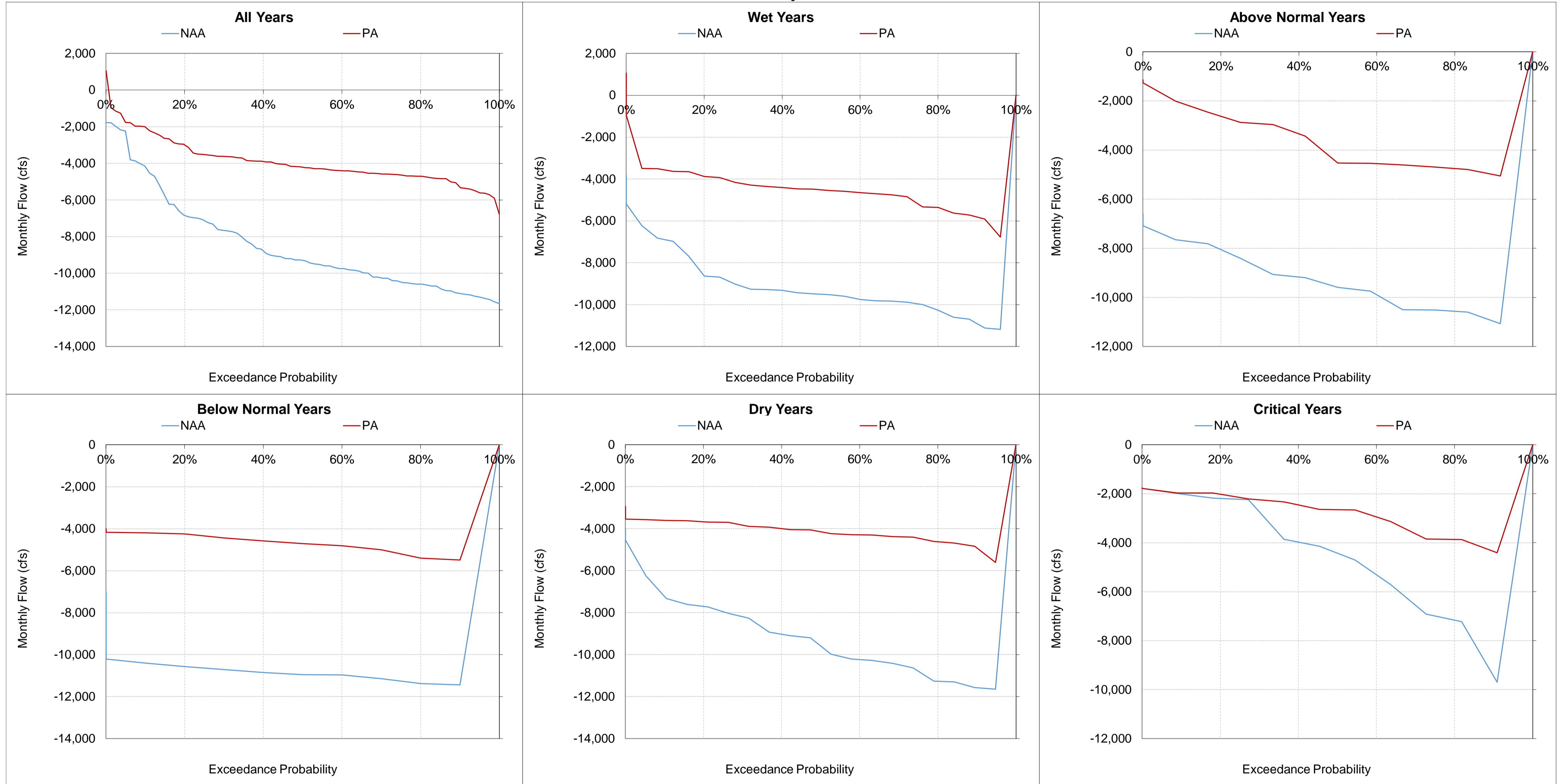
Figure 5.A.6-25-17. Old and Middle River, Monthly Flow July
