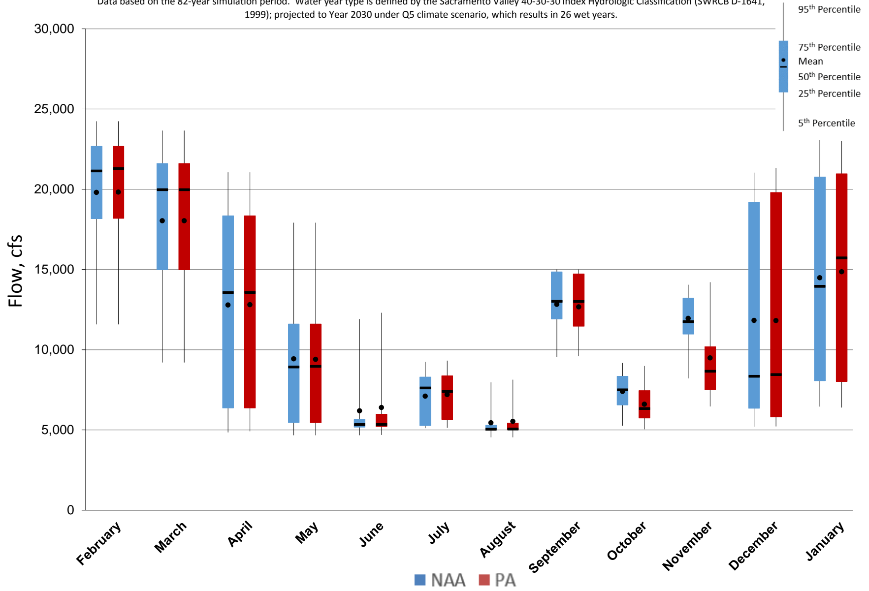
Figure 5.A.6-36-2. Monthly Flow Ranges For Sacramento River at Wilkins Slough, Wet Years
