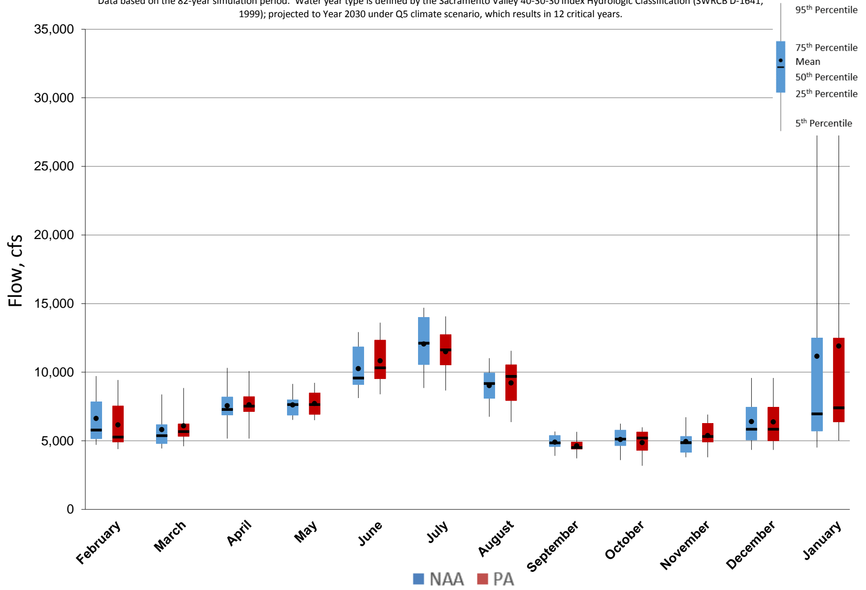
Figure 5.A.6-35-6. Monthly Flow Ranges For Sacramento River above Red Bluff Diversion Dam, Critical Years
