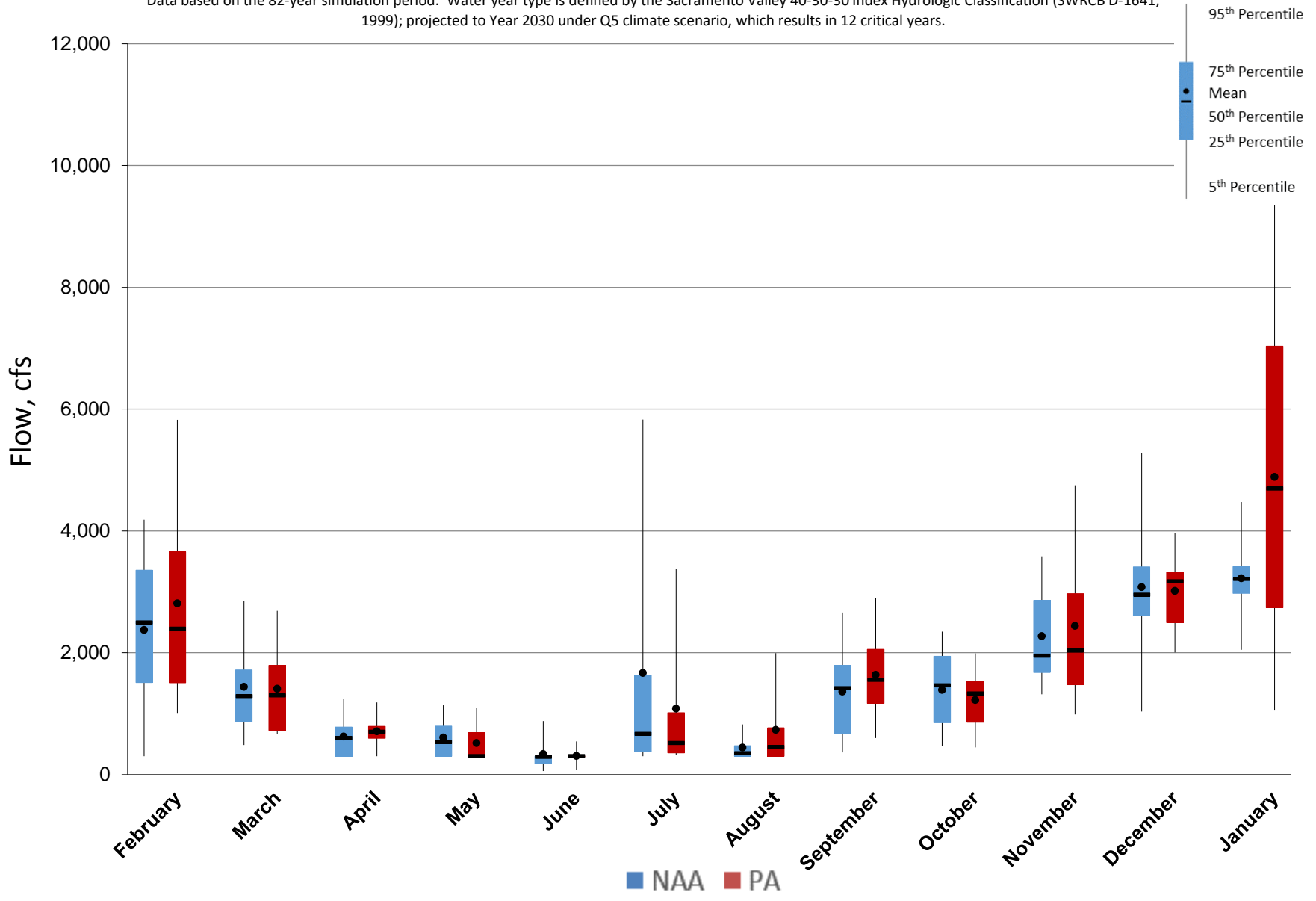
Figure 5.A.6-34-6. Monthly Flow Ranges For Total Banks Pumping Plant Exports, Critical Years
