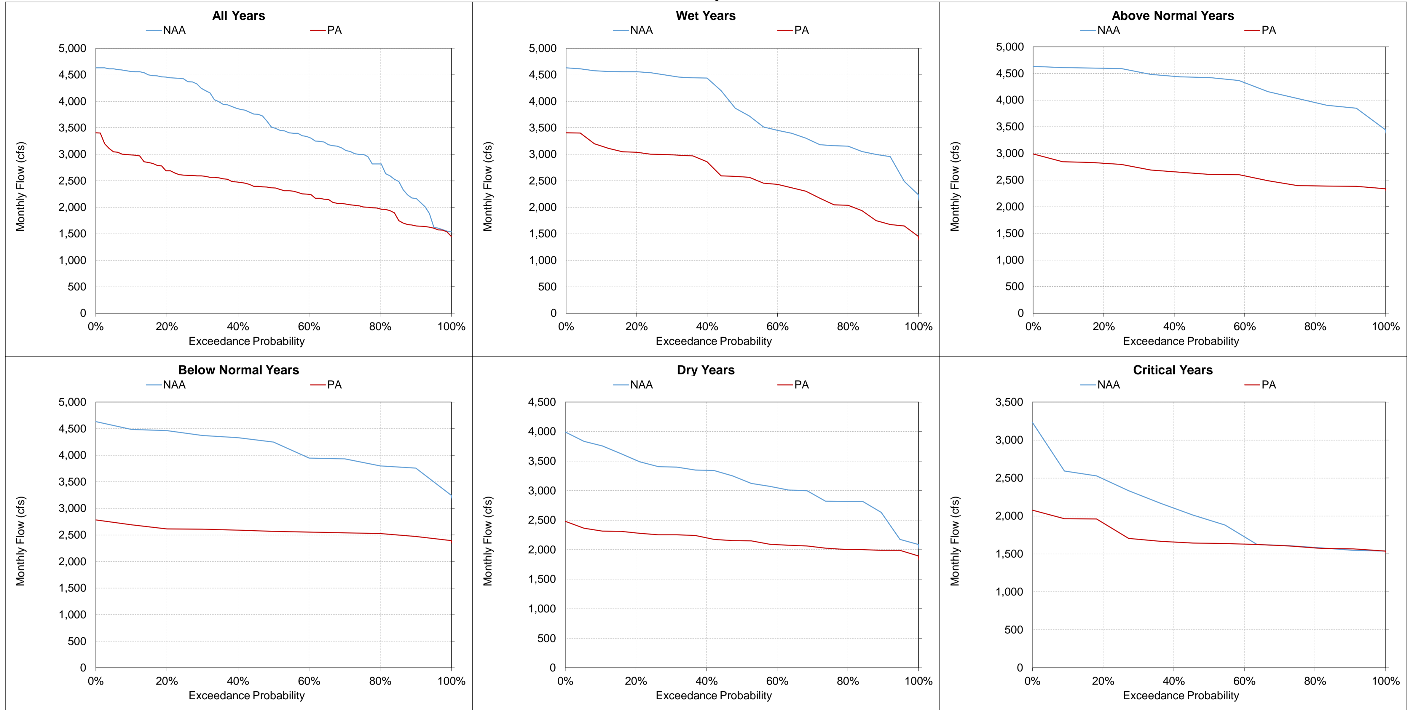
Figure 5.A.6-32-17. Delta Cross Channel, Monthly Flow July
