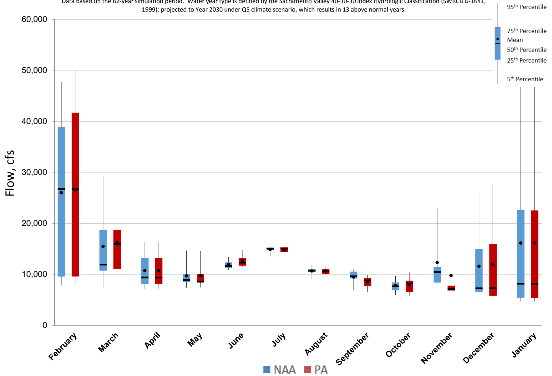
Figure 5.A.6-35-3. Monthly Flow Ranges For Sacramento River above Red Bluff Diversion Dam, Above Normal Years
