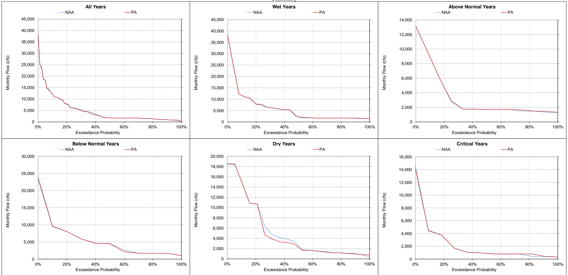
Figure 5.A.6-16-11. American River below Nimbus Dam, Monthly Flow January
