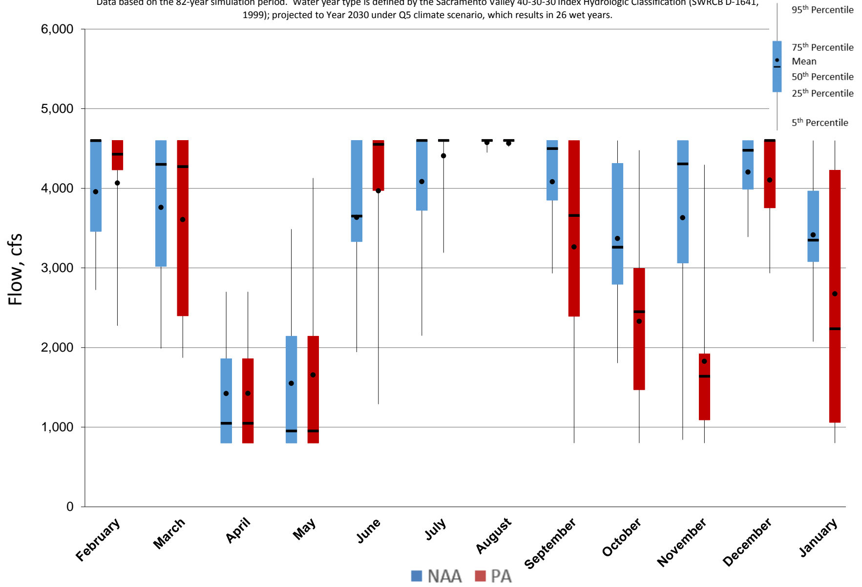
Figure 5.A.6-33-2. Monthly Flow Ranges For Total Jones Pumping Plant Exports, Wet Years
