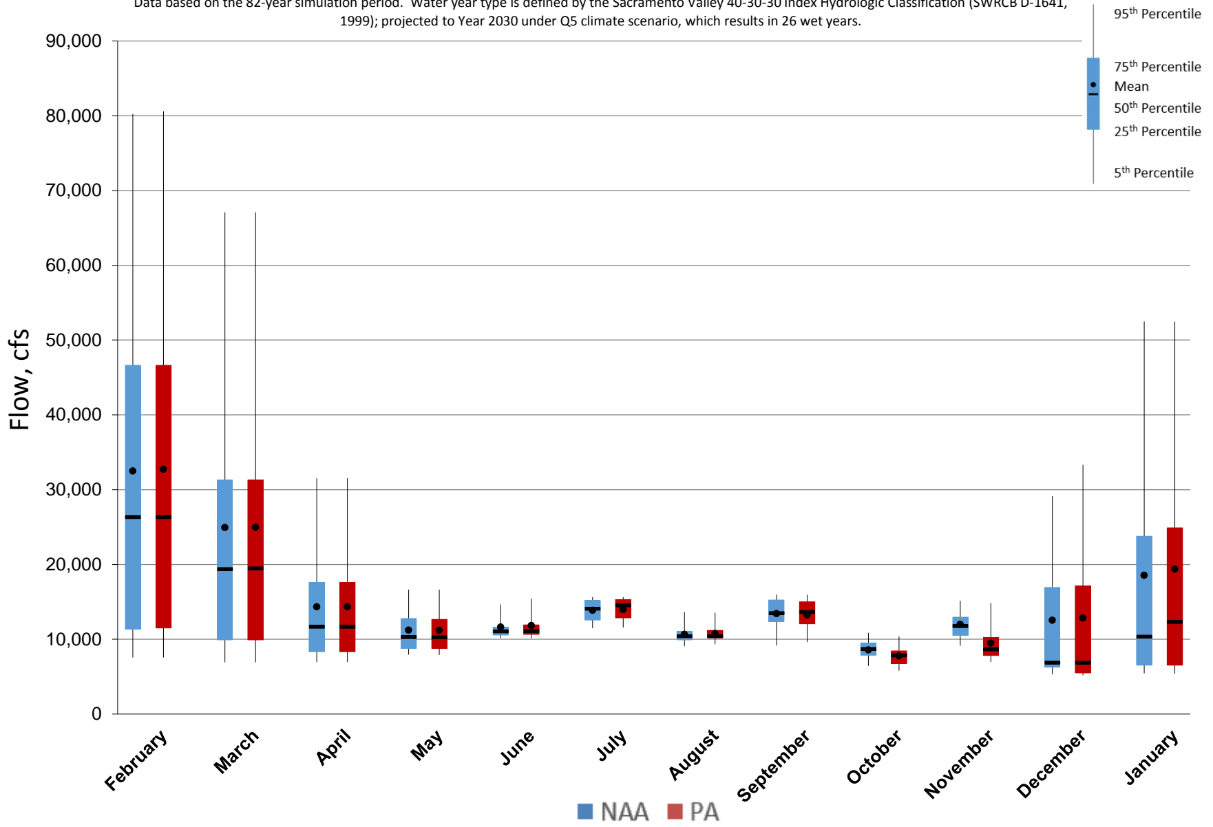
Figure 5.A.6-35-2. Monthly Flow Ranges For Sacramento River above Red Bluff Diversion Dam, Wet Years
