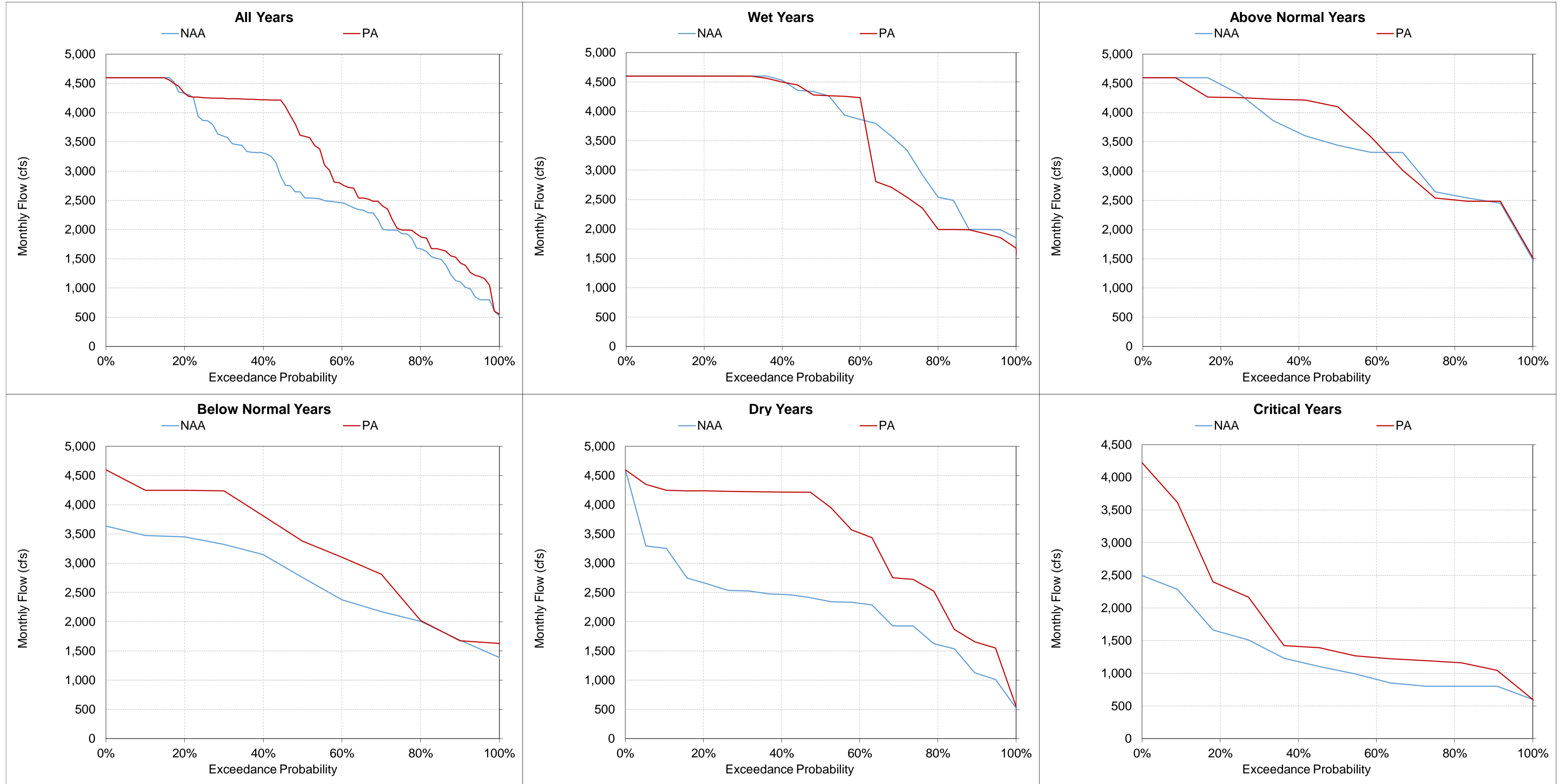
Figure 5.A.6-33-13. Total Jones Pumping Plant Exports, Monthly Flow March
