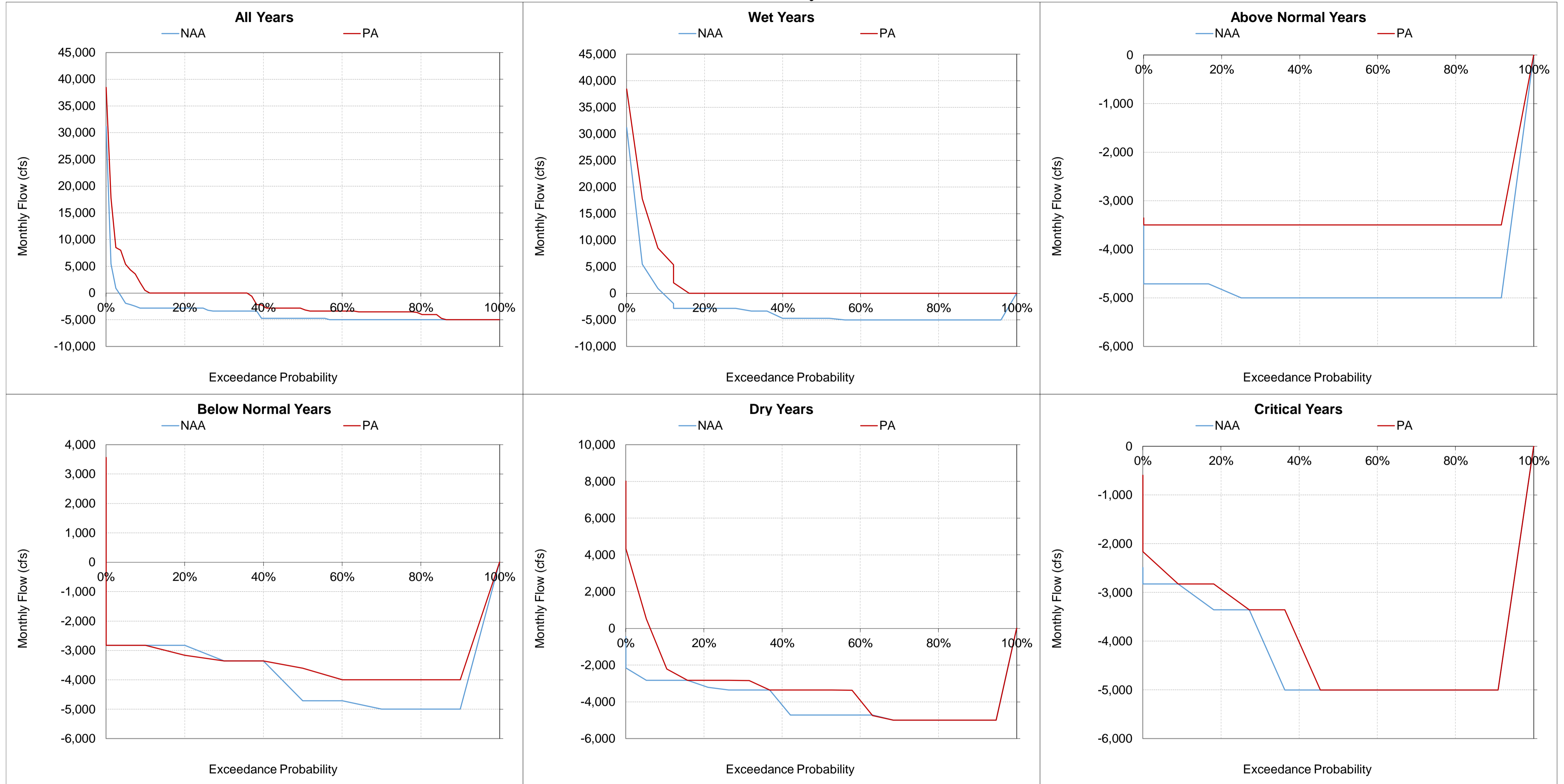
Figure 5.A.6-25-11. Old and Middle River, Monthly Flow January
