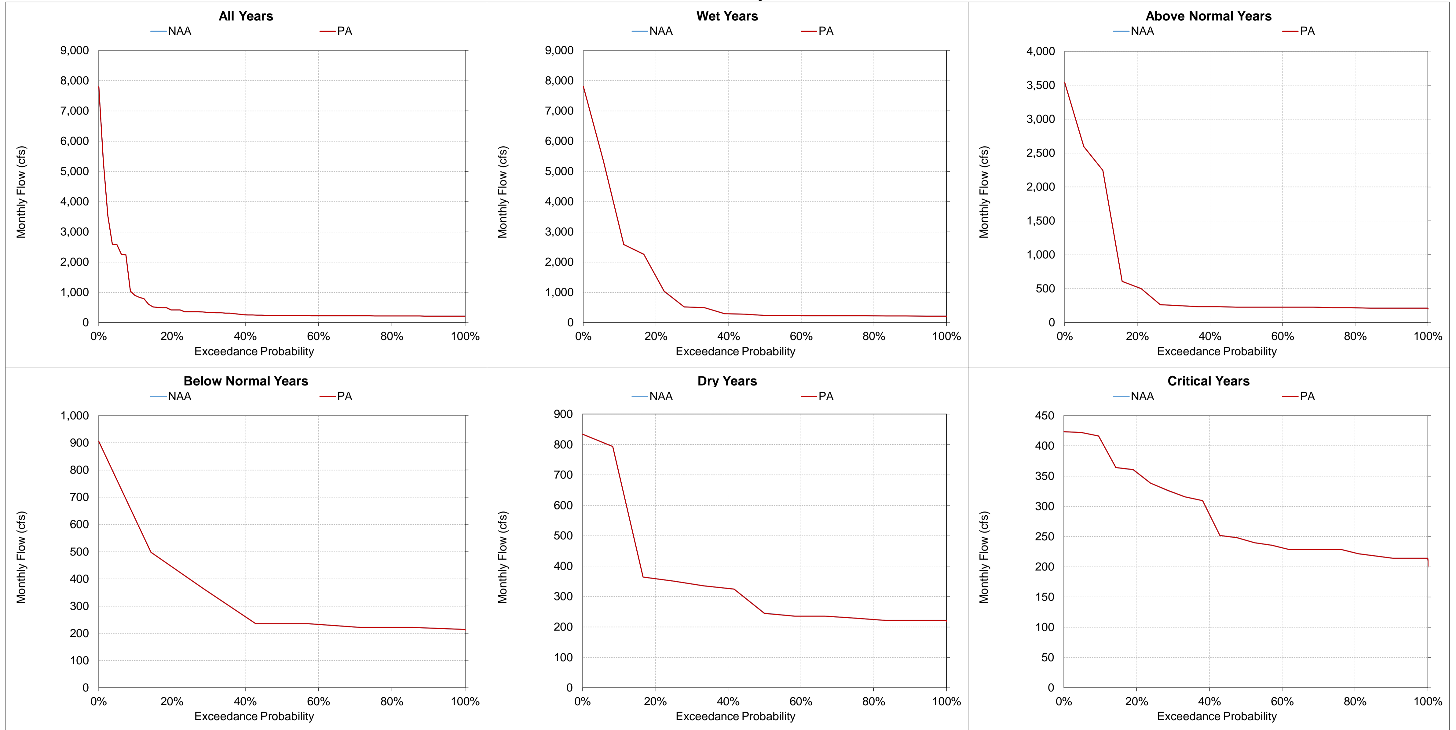
Figure 5.A.6-21-12. Stanislaus River at Goodwin, Monthly Flow February
