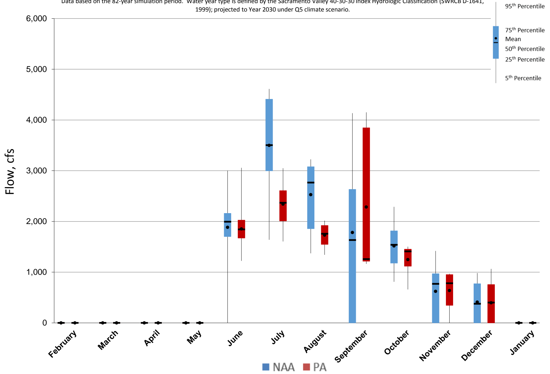
Figure 5.A.6-32-1. Monthly Flow Ranges For Delta Cross Channel, All Years
