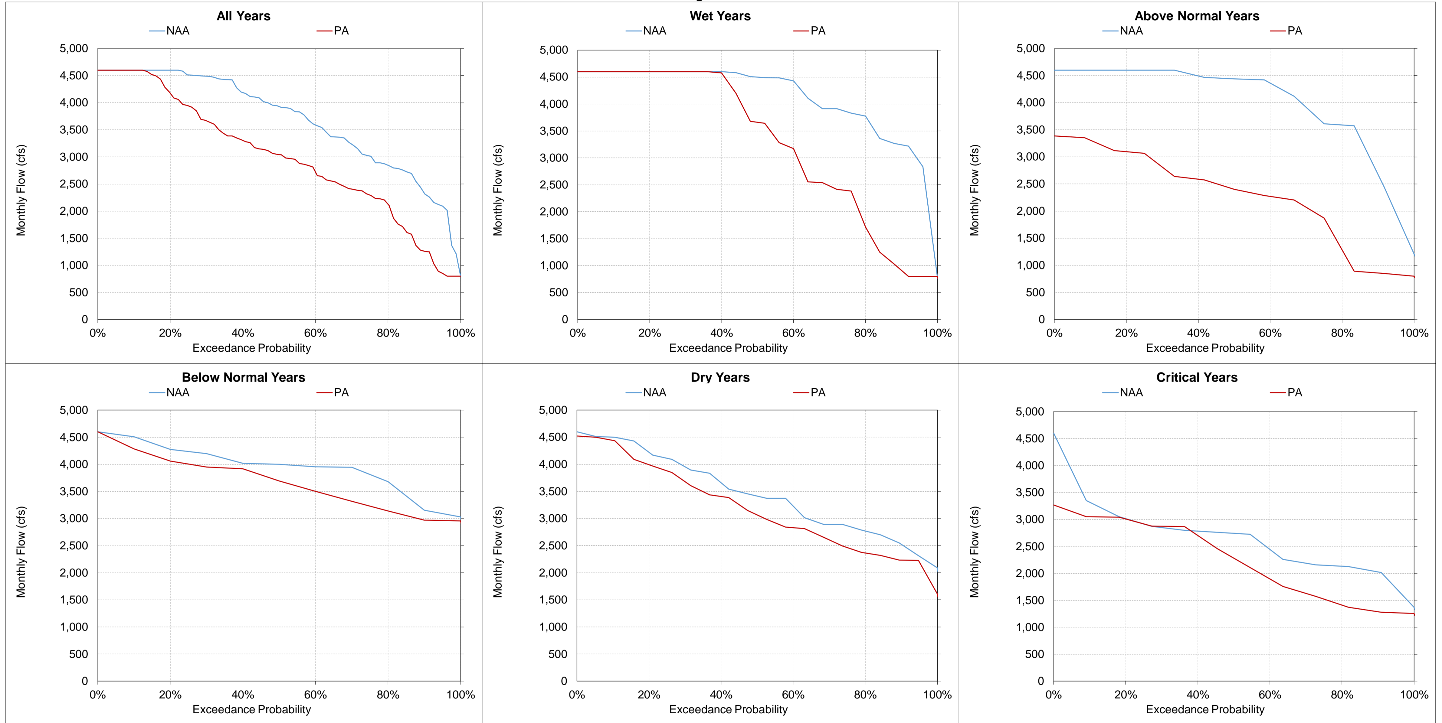
Figure 5.A.6-33-19. Total Jones Pumping Plant Exports, Monthly Flow September
