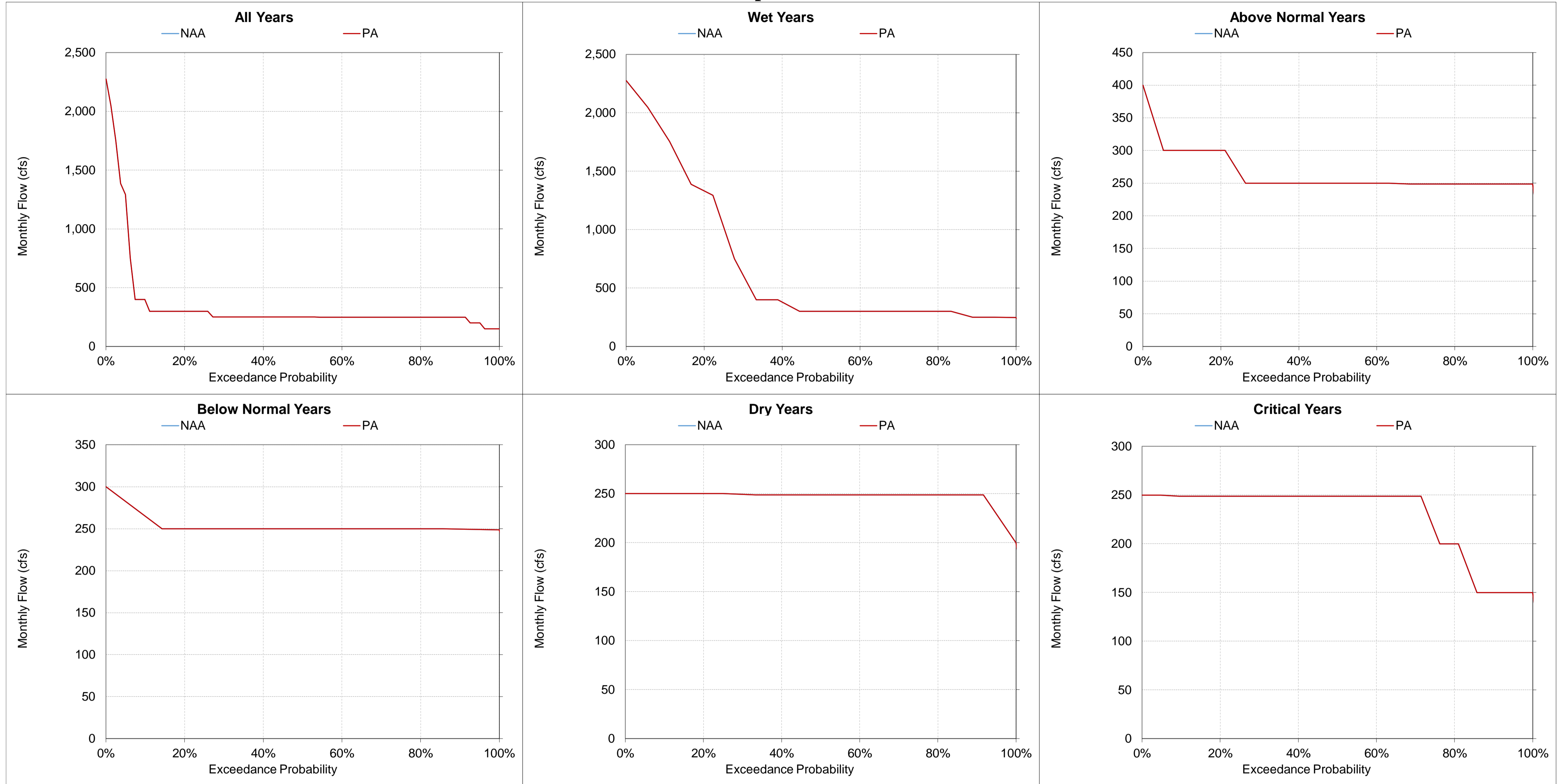
Figure 5.A.6-21-19. Stanislaus River at Goodwin, Monthly Flow September
