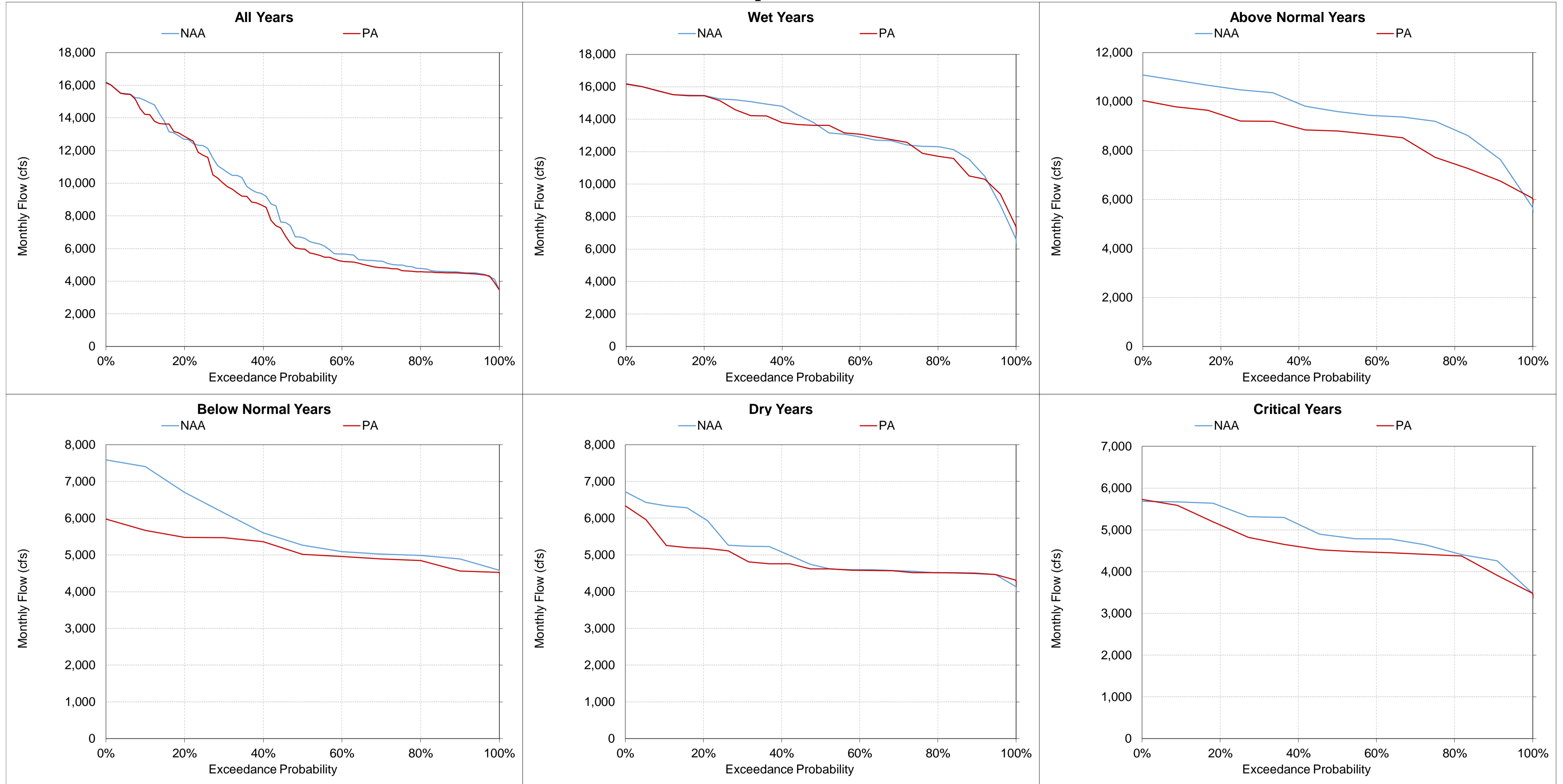
Figure 5.A.6-35-19. Sacramento River above Red Bluff Diversion Dam, Monthly Flow September
