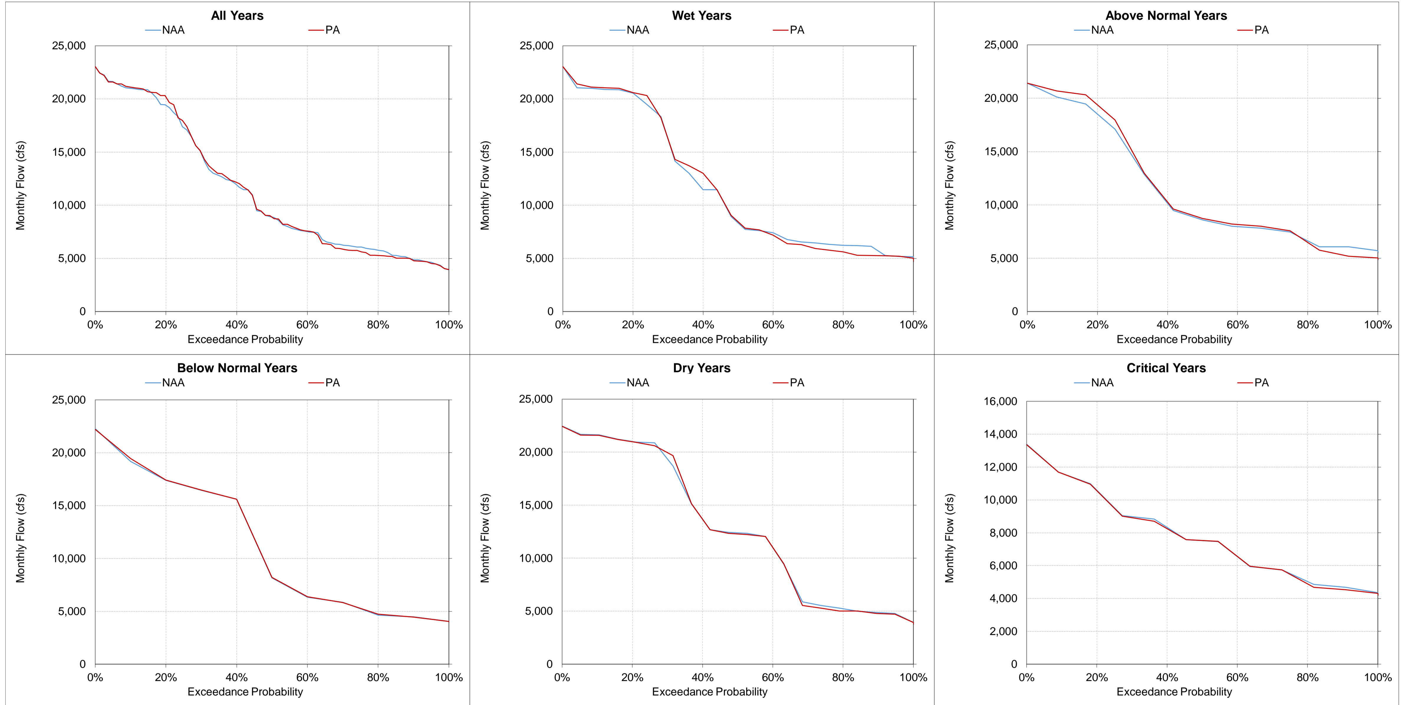
Figure 5.A.6-36-10. Sacramento River at Wilkins Slough, Monthly Flow December
