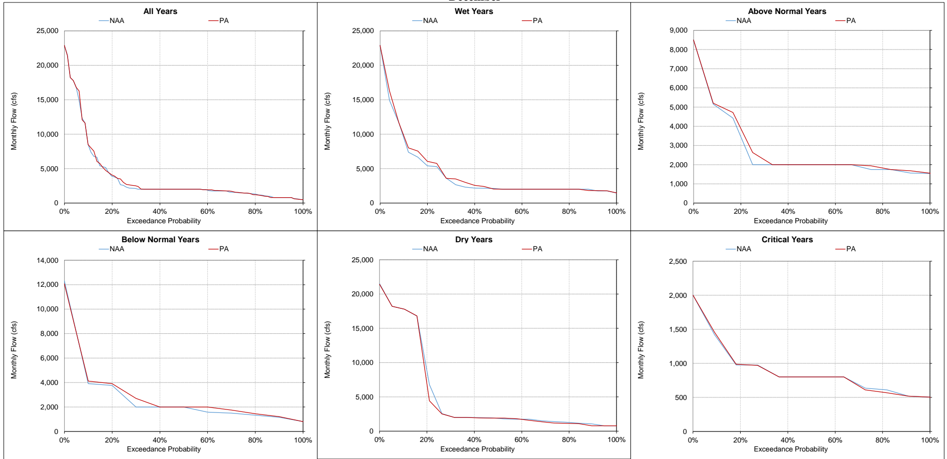
Figure 5.A.6-16-10. American River below Nimbus Dam, Monthly Flow December
