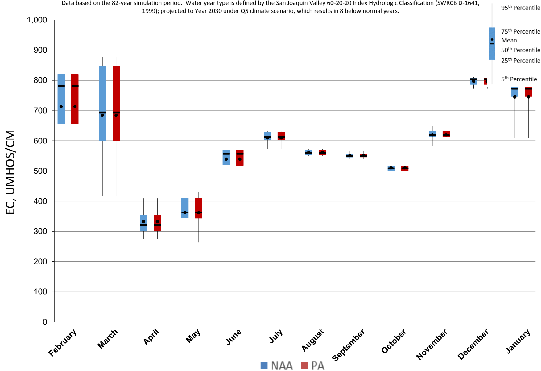
Figure 5.A.6-30-4. Monthly EC Ranges for San Joaquin River at Vernalis, Below Normal Years
