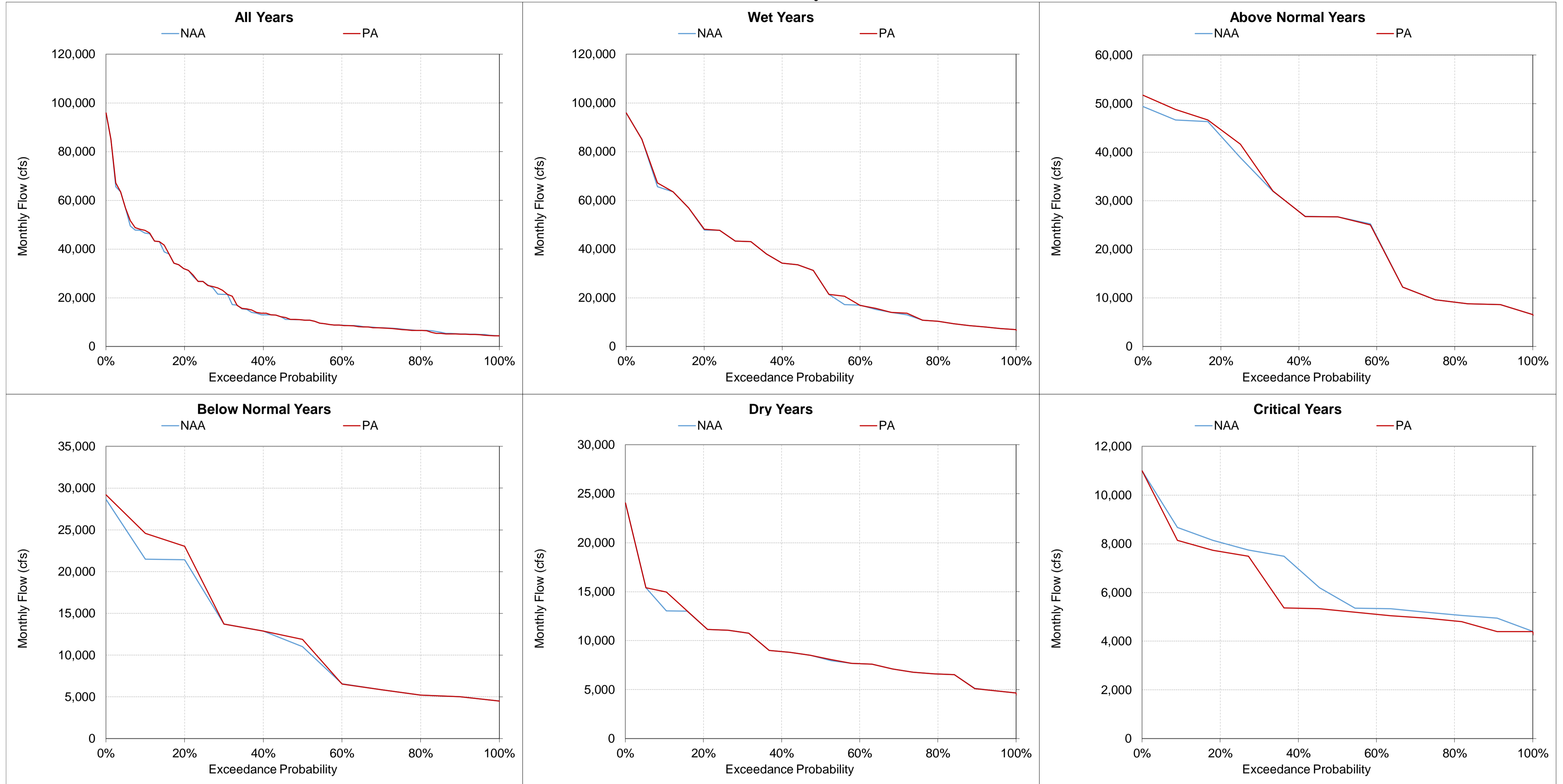
Figure 5.A.6-35-12. Sacramento River above Red Bluff Diversion Dam, Monthly Flow February
