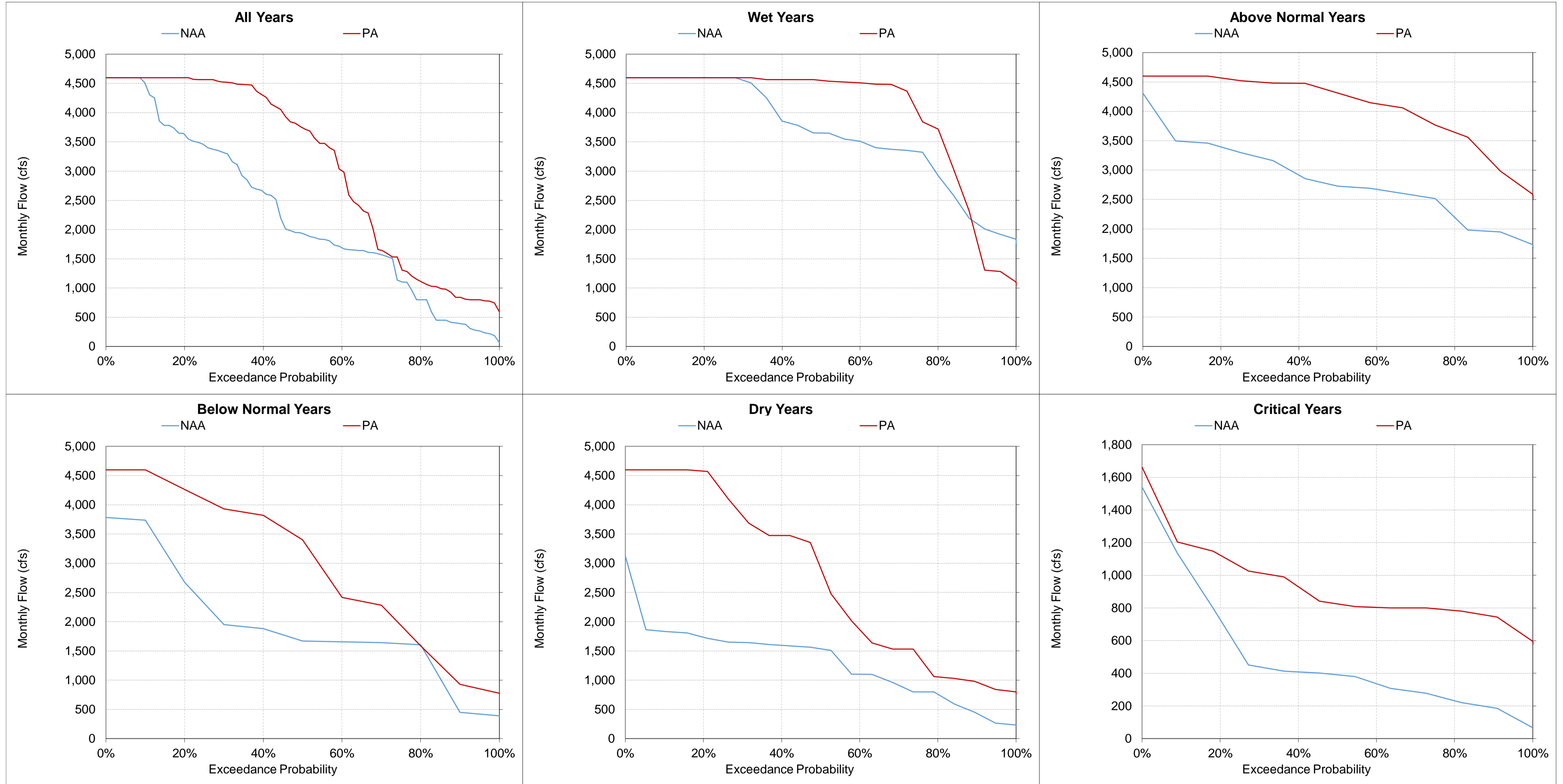
Figure 5.A.6-33-16. Total Jones Pumping Plant Exports, Monthly Flow June
