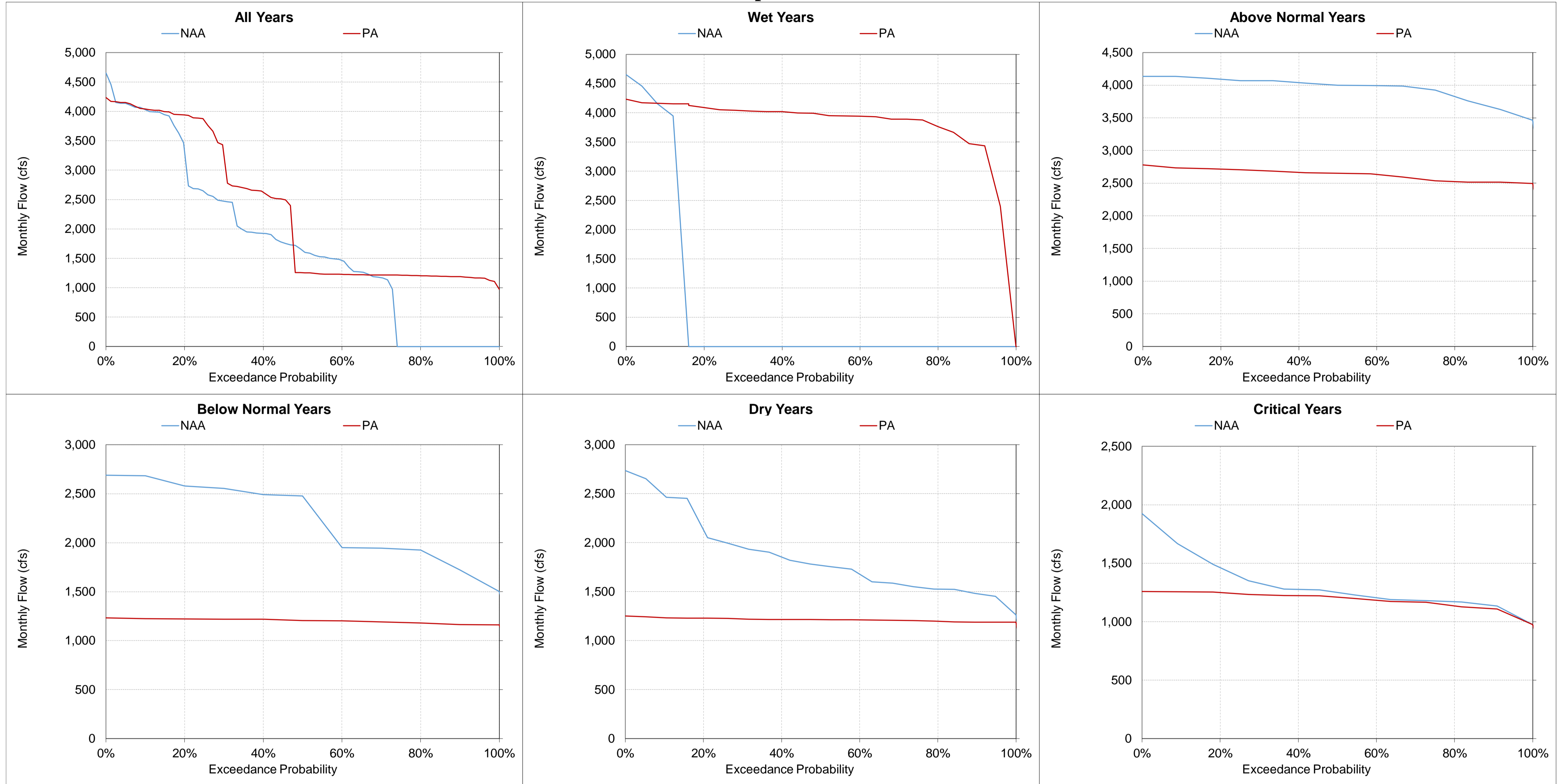
Figure 5.A.6-32-19. Delta Cross Channel, Monthly Flow September
