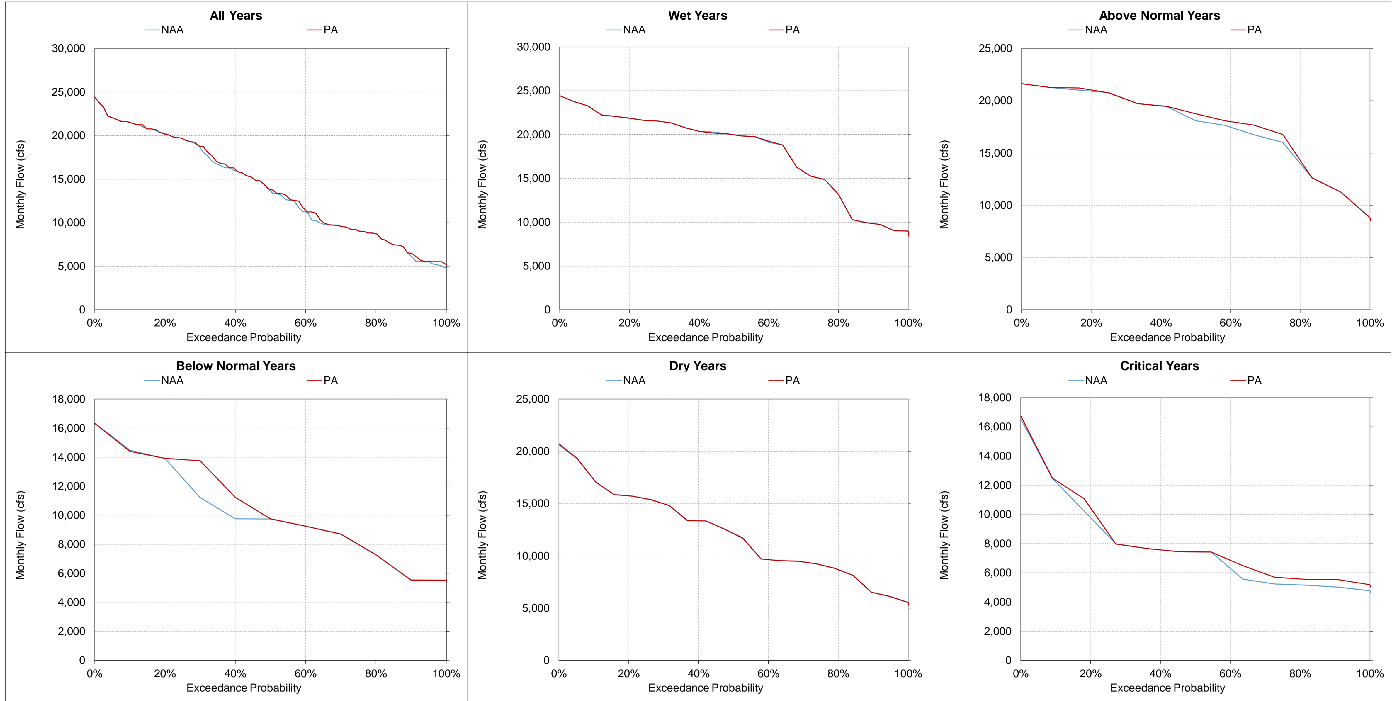
Figure 5.A.6-36-13. Sacramento River at Wilkins Slough, Monthly Flow March
