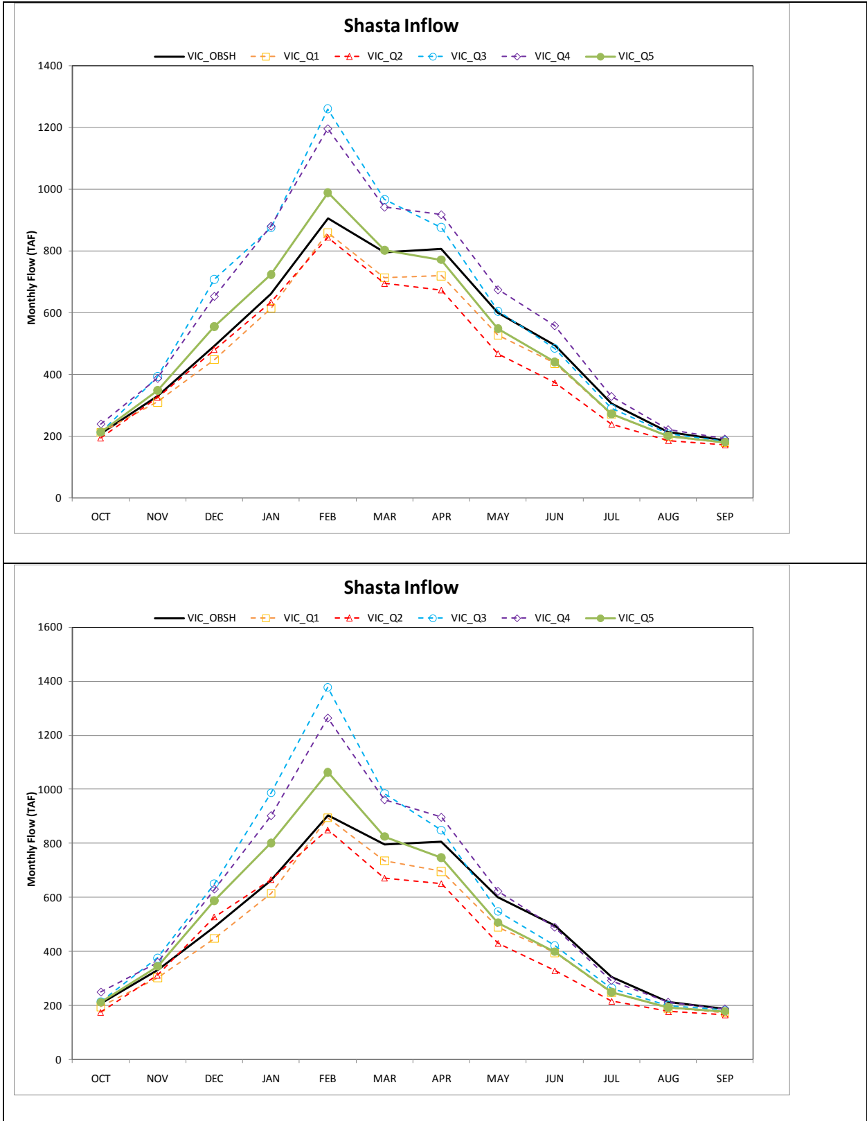
Figure 5.A.A.2-7. Simulated Changes in Monthly Natural Streamflow for Shasta Inflow (top, 2025 changes; bottom, 2060 changes).
