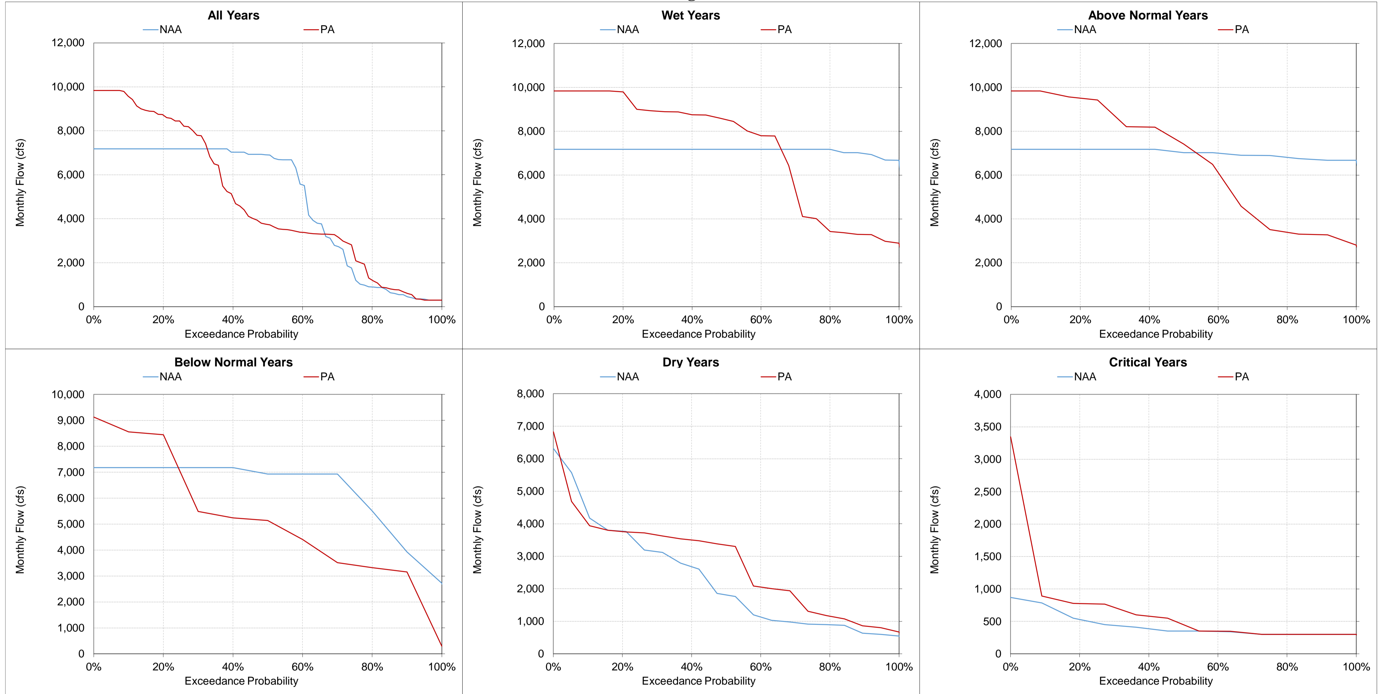
Figure 5.A.6-34-18. Total Banks Pumping Plant Exports, Monthly Flow August
