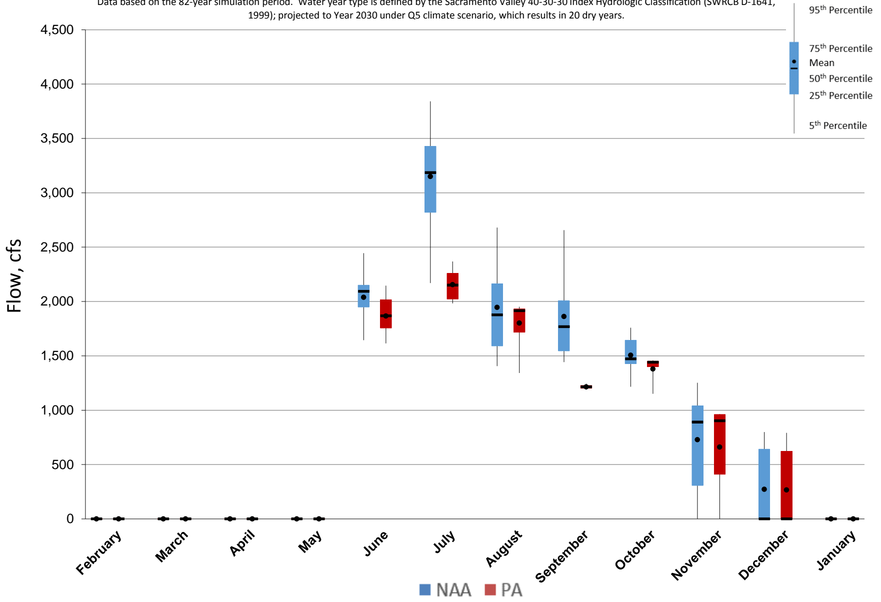
Figure 5.A.6-32-5. Monthly Flow Ranges For Delta Cross Channel, Dry Years
