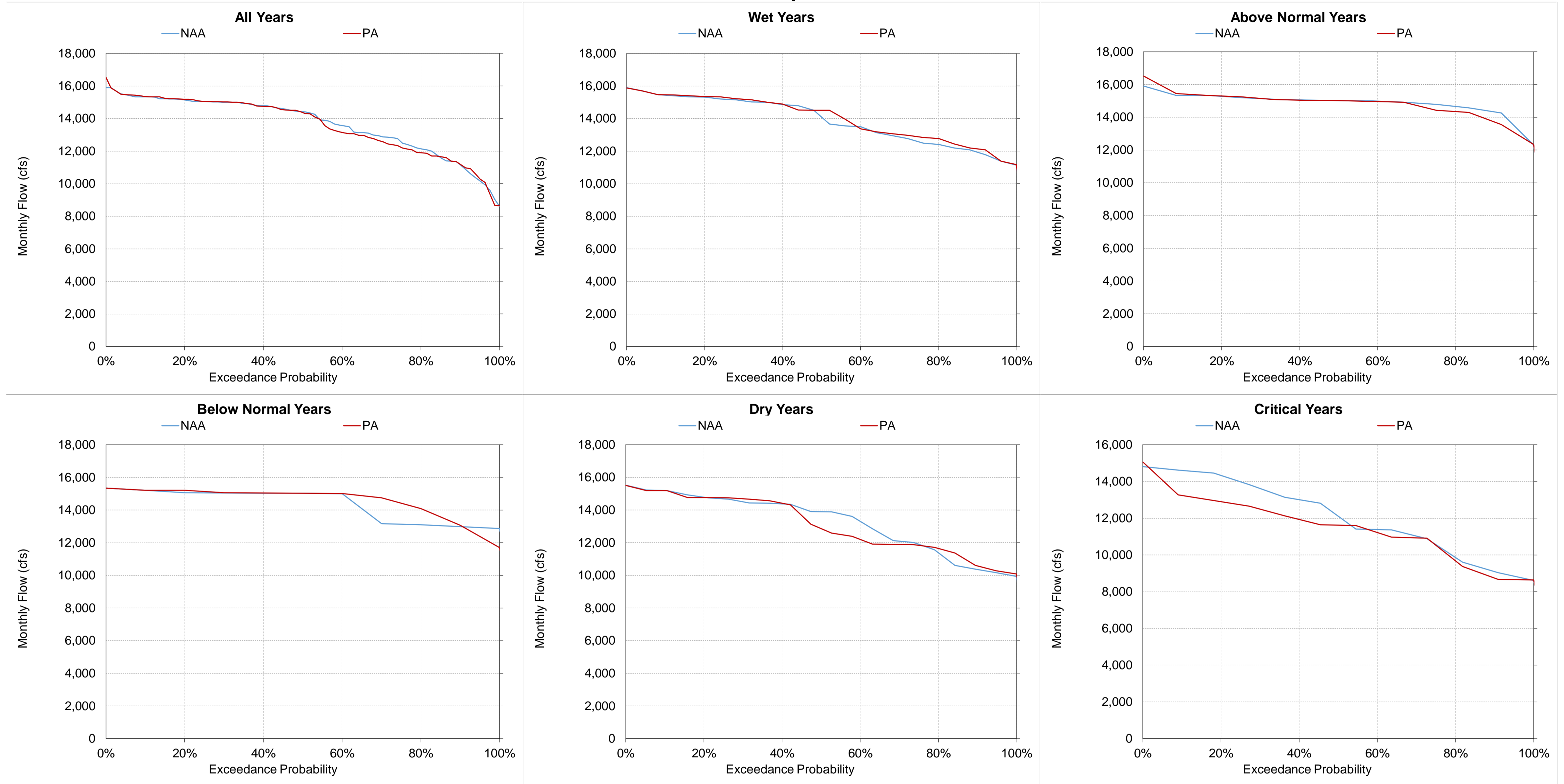
Figure 5.A.6-35-17. Sacramento River above Red Bluff Diversion Dam, Monthly Flow July
