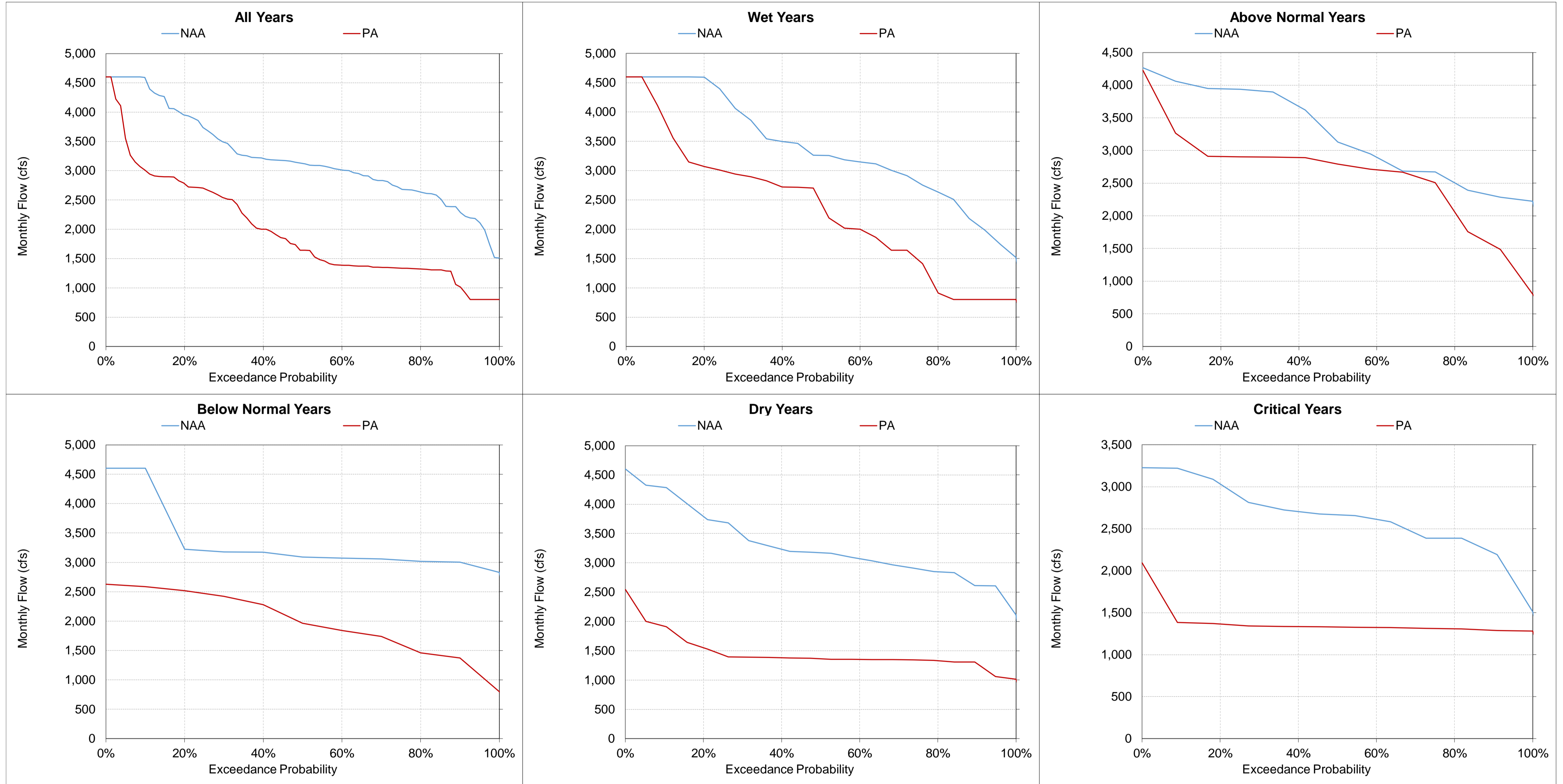
Figure 5.A.6-33-8. Total Jones Pumping Plant Exports, Monthly Flow October
