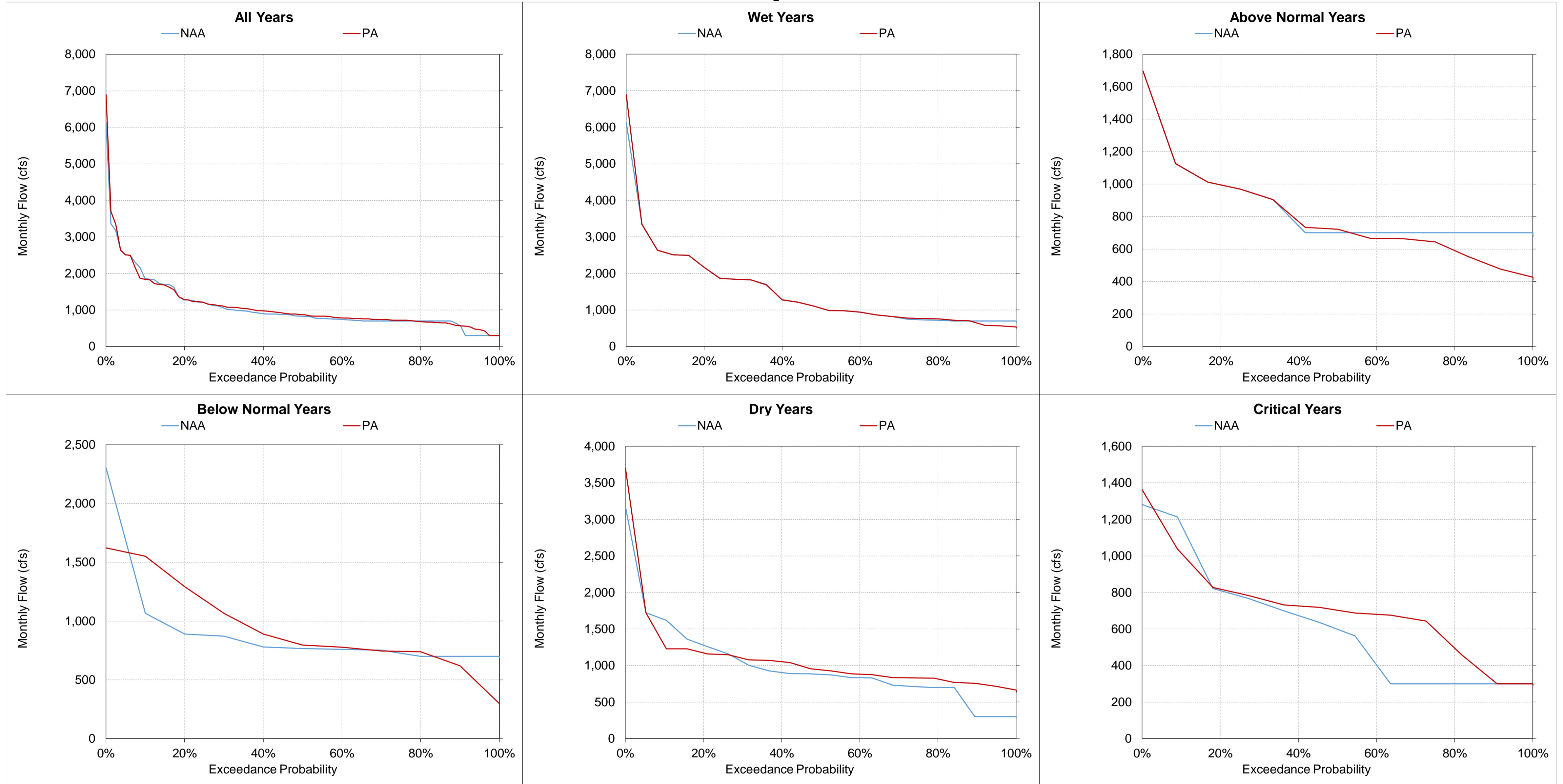
Figure 5.A.6-34-14. Total Banks Pumping Plant Exports, Monthly Flow April
