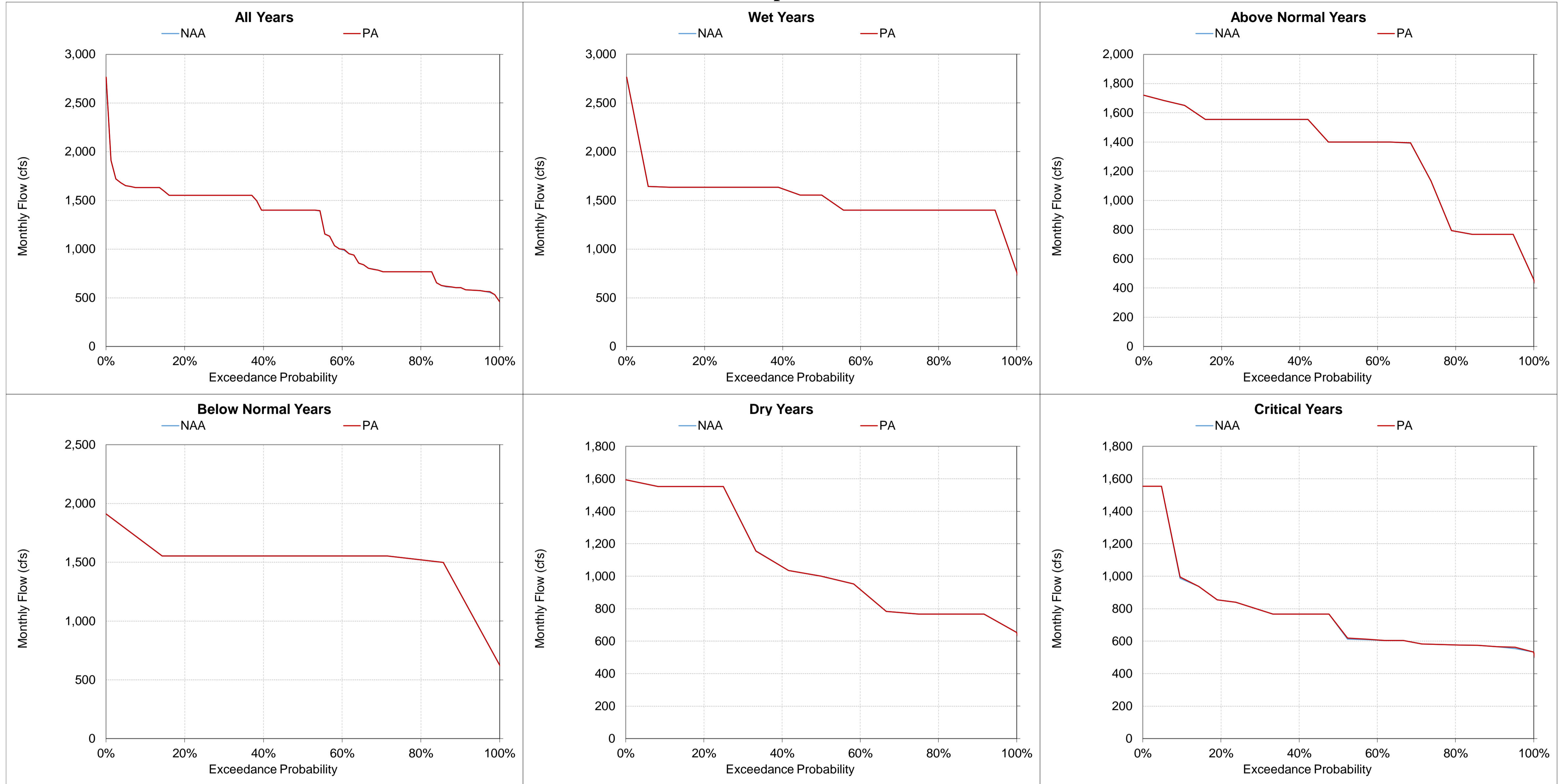
Figure 5.A.6-21-14. Stanislaus River at Goodwin, Monthly Flow April
