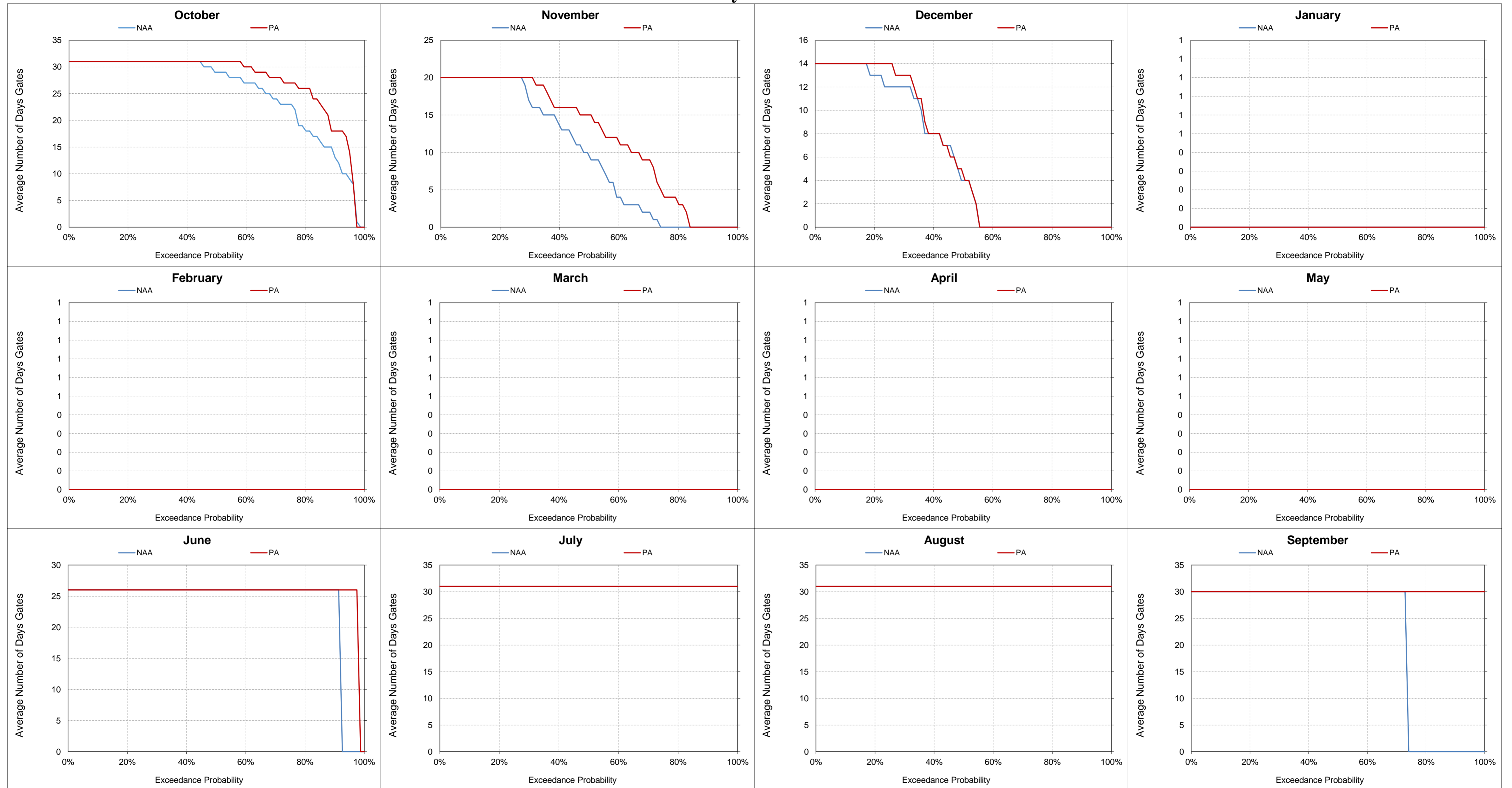
Figure 5.A.6-31-7. Delta Cross Channel, Average Number of Days Gates Open Probability of Exceedance
