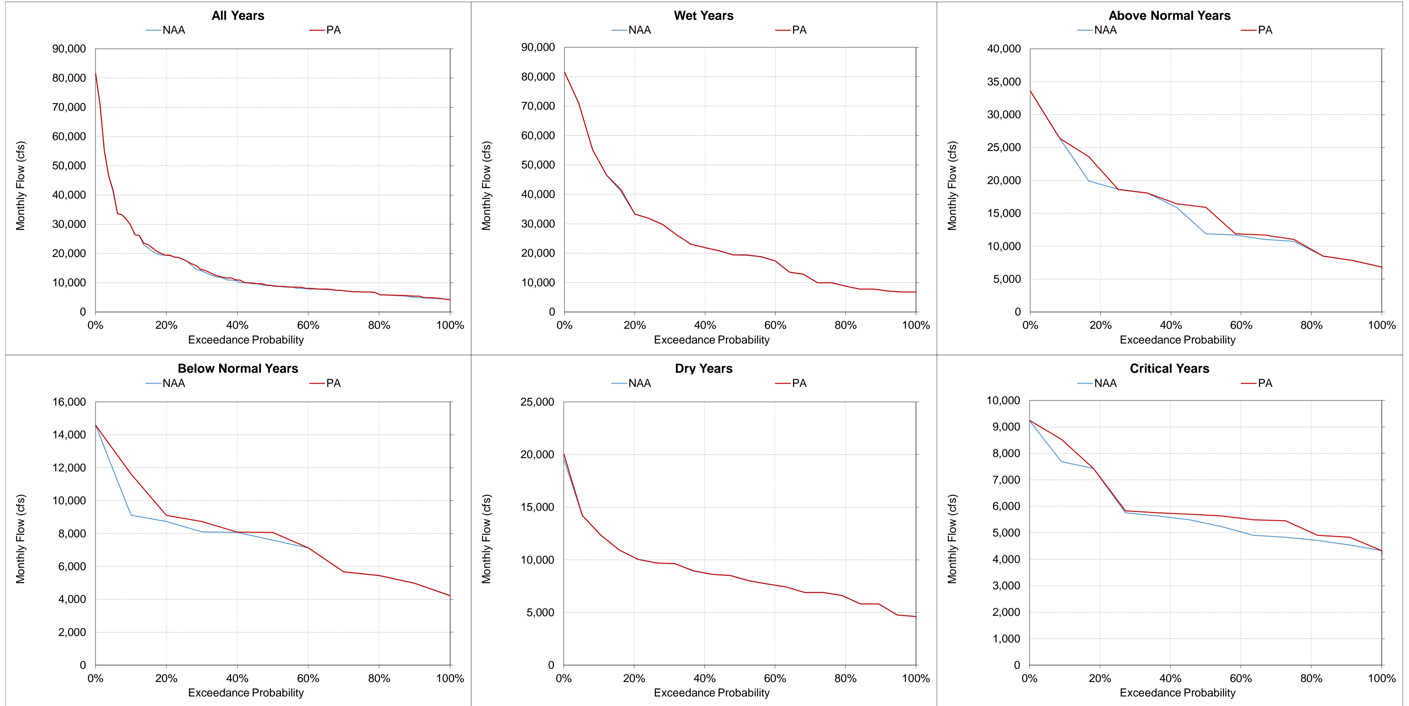
Figure 5.A.6-35-13. Sacramento River above Red Bluff Diversion Dam, Monthly Flow March
