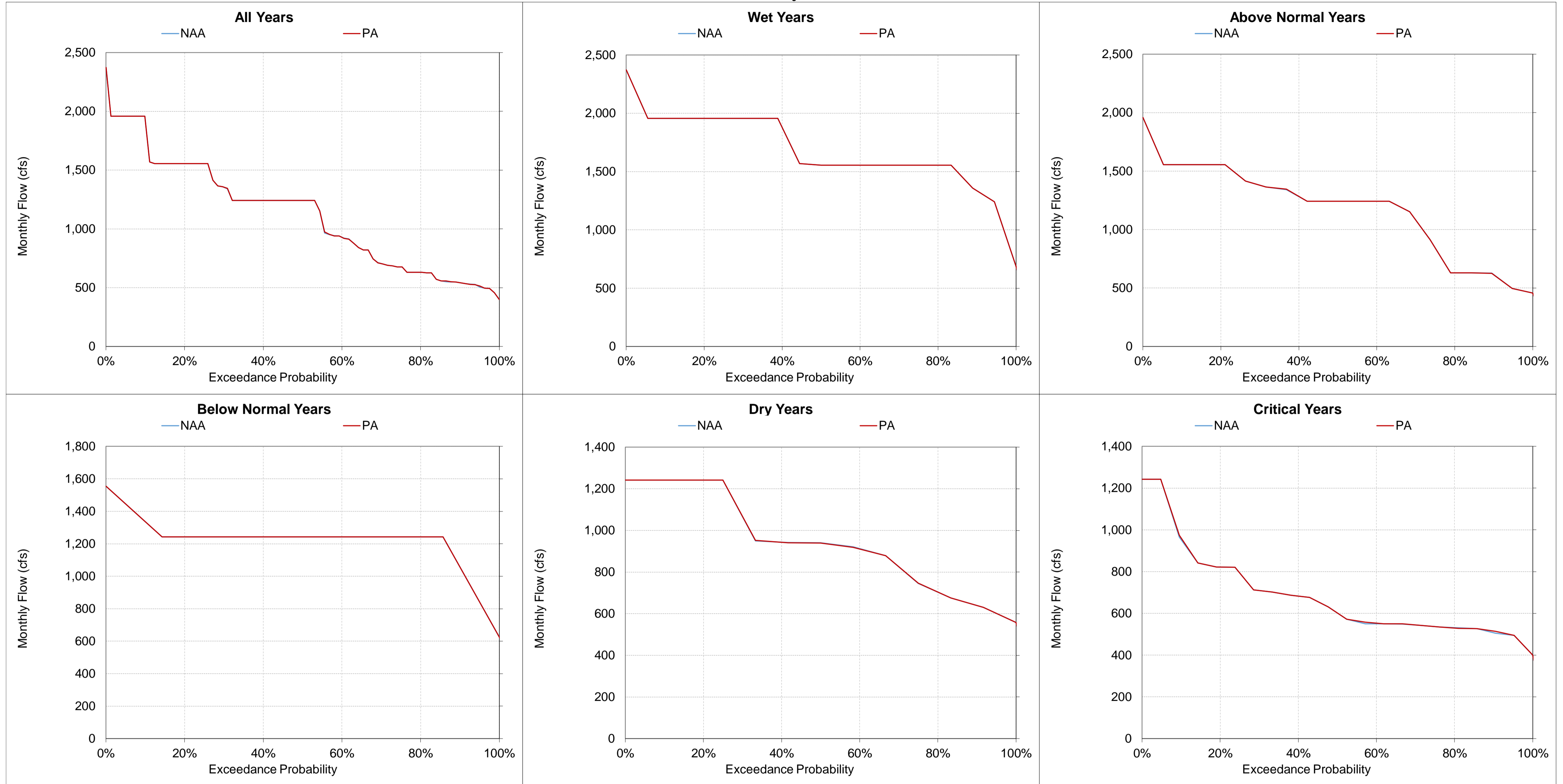
Figure 5.A.6-21-15. Stanislaus River at Goodwin, Monthly Flow May
