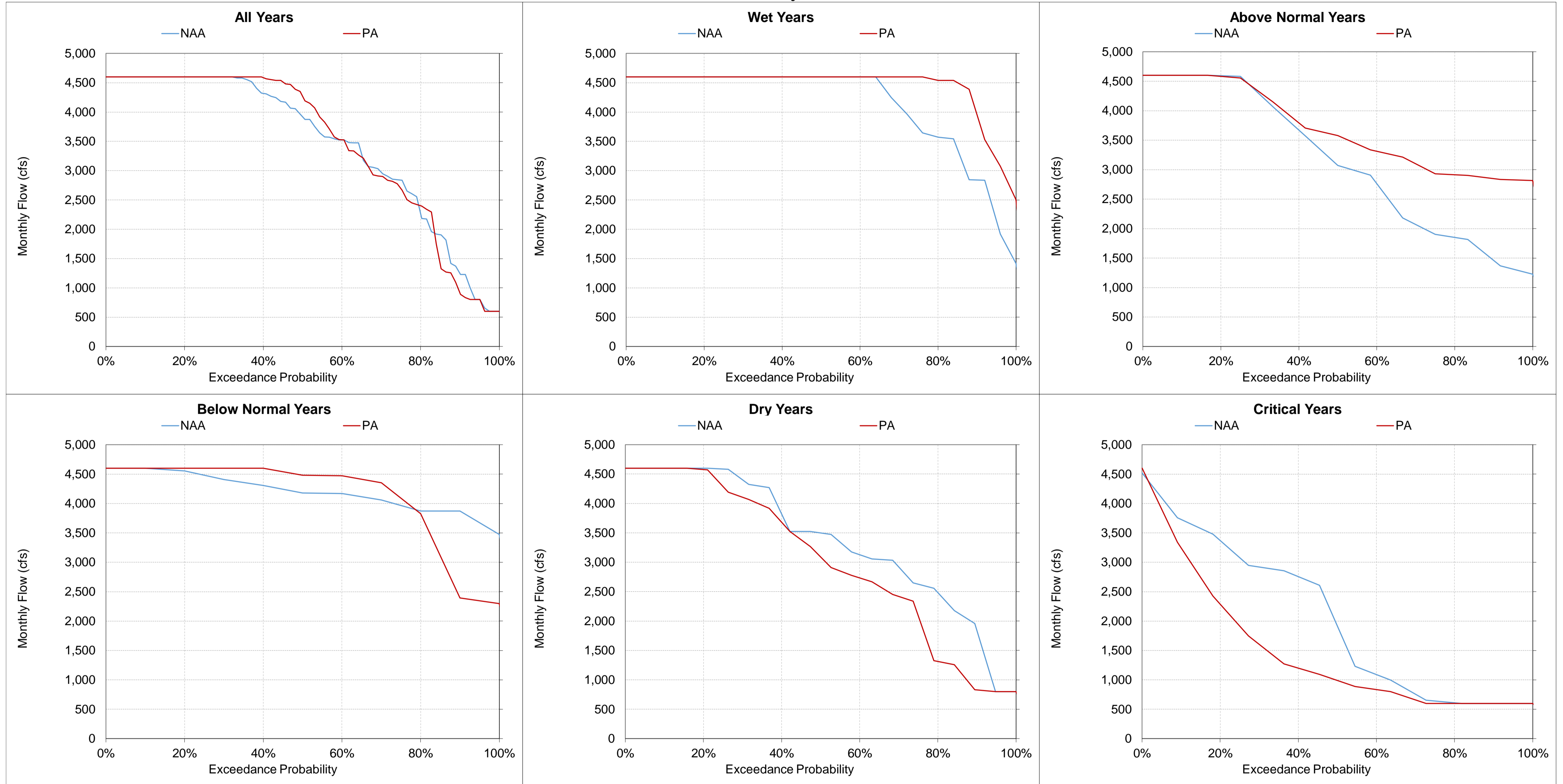
Figure 5.A.6-33-17. Total Jones Pumping Plant Exports, Monthly Flow July
