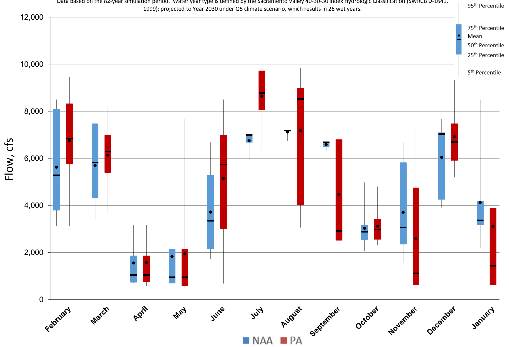
Figure 5.A.6-34-2. Monthly Flow Ranges For Total Banks Pumping Plant Exports, Wet Years
