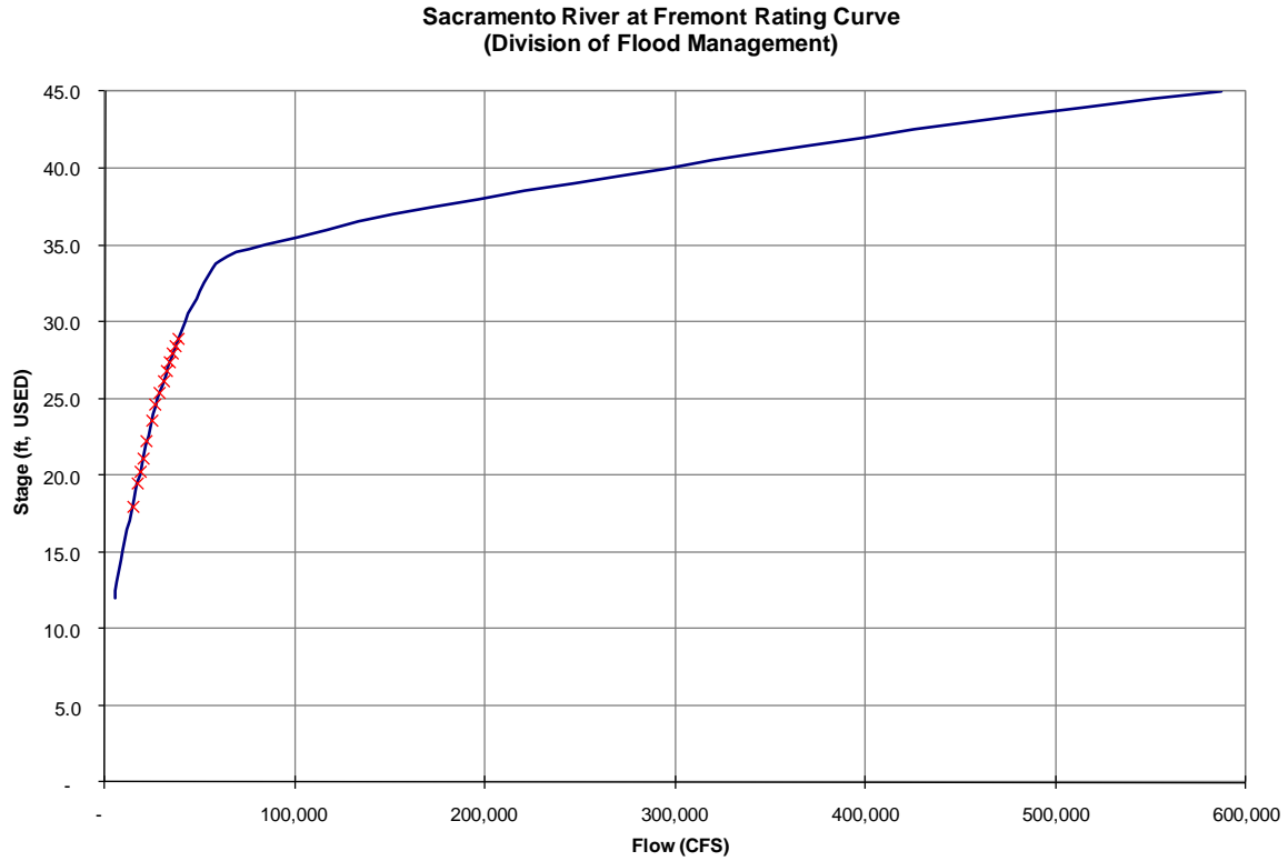
Figure 5.A.A.4-14. Sacramento River at Fremont rating curve (Source: California Division of Flood Management)
