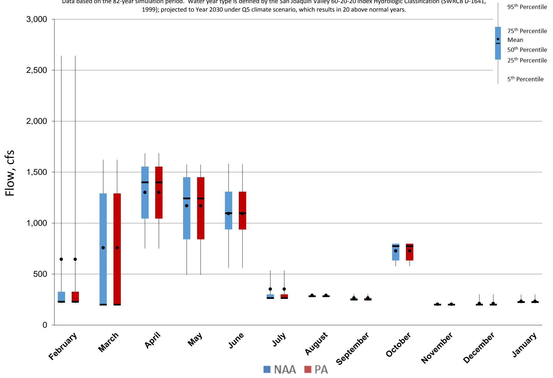
Figure 5.A.6-21-3. Monthly Flow Ranges for Stanislaus River at Goodwin, Above Normal Years
