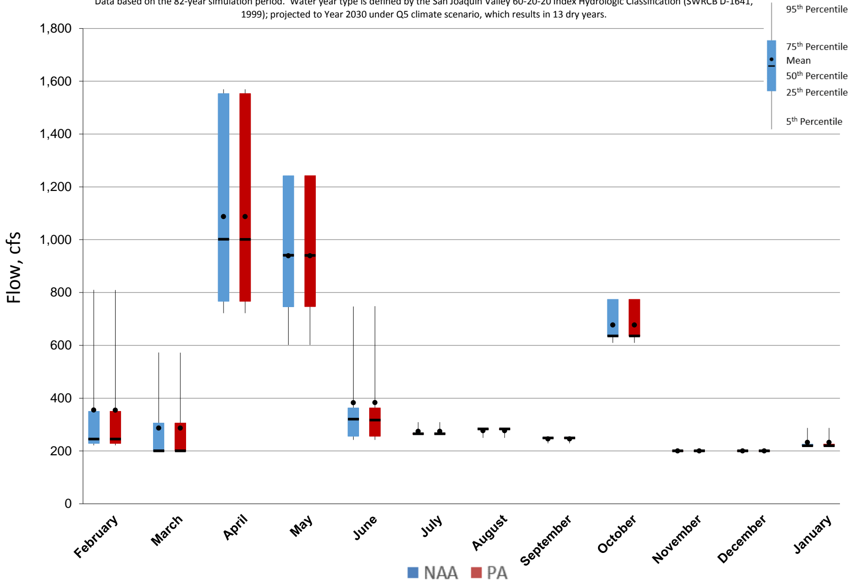
Figure 5.A.6-21-5. Monthly Flow Ranges for Stanislaus River at Goodwin, Dry Years
