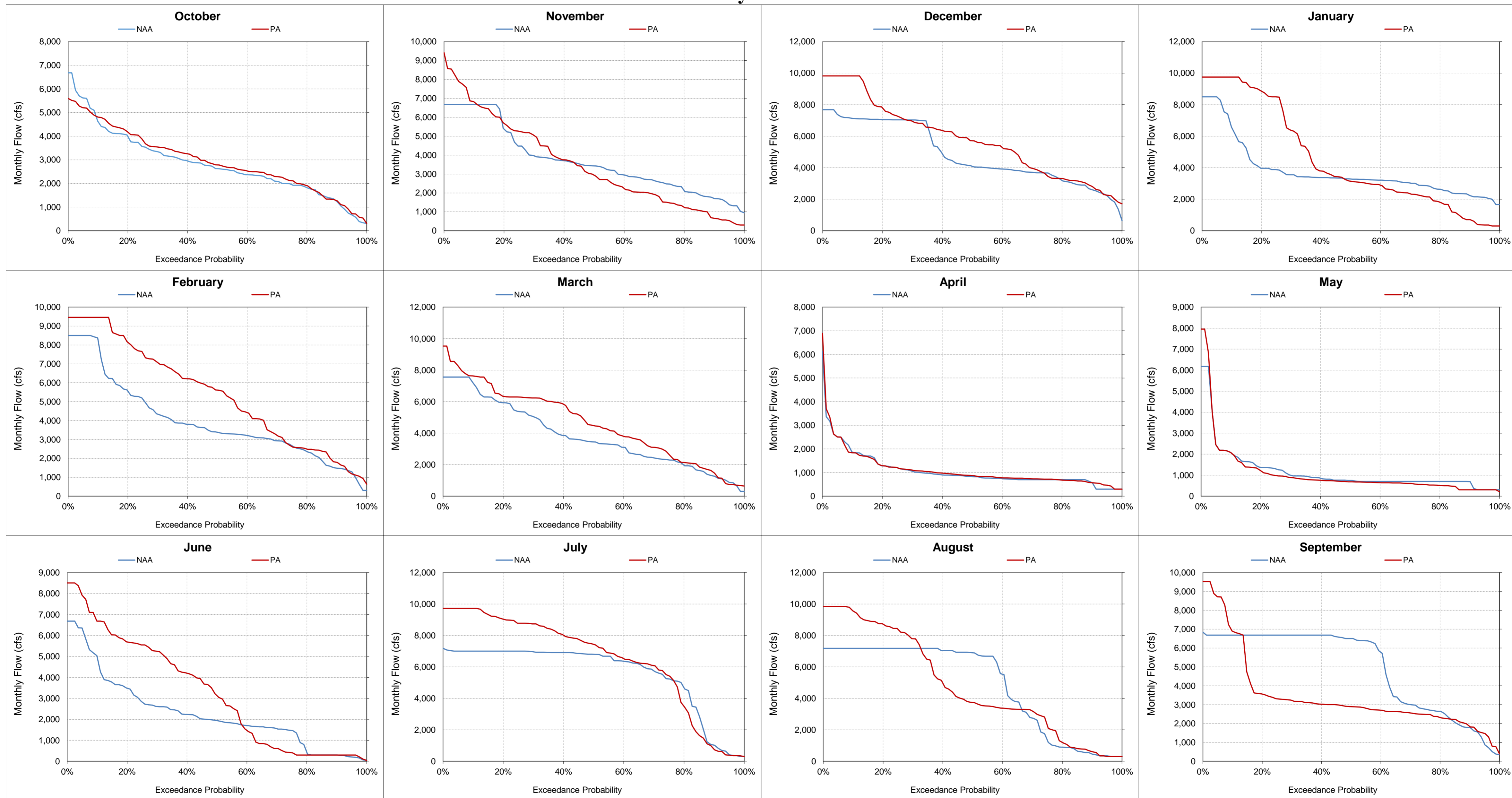
Figure 5.A.6-34-7. Total Banks Pumping Plant Exports, Monthly Flow Probability of Exceedance
