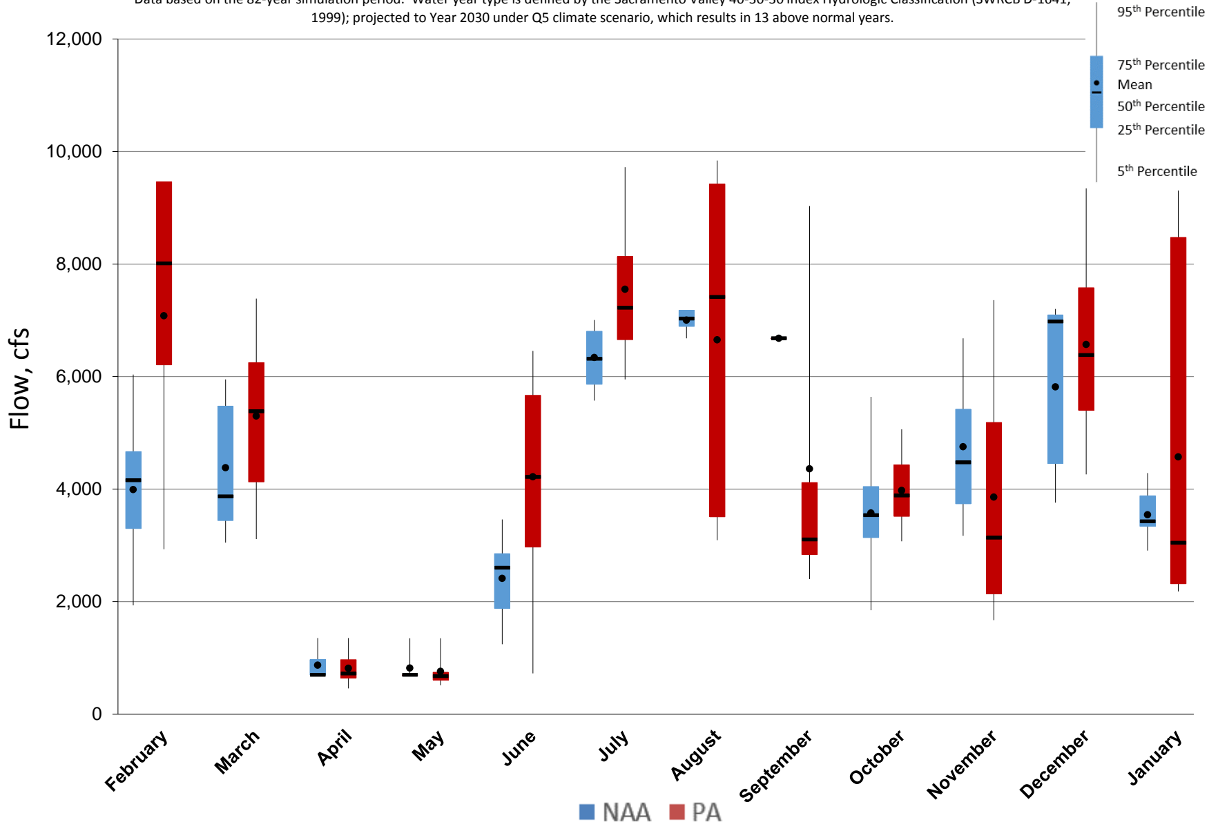
Figure 5.A.6-34-3. Monthly Flow Ranges For Total Banks Pumping Plant Exports, Above Normal Years
