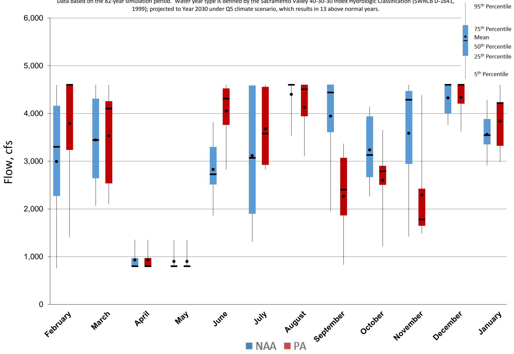
Figure 5.A.6-33-3. Monthly Flow Ranges For Total Jones Pumping Plant Exports, Above Normal Years
