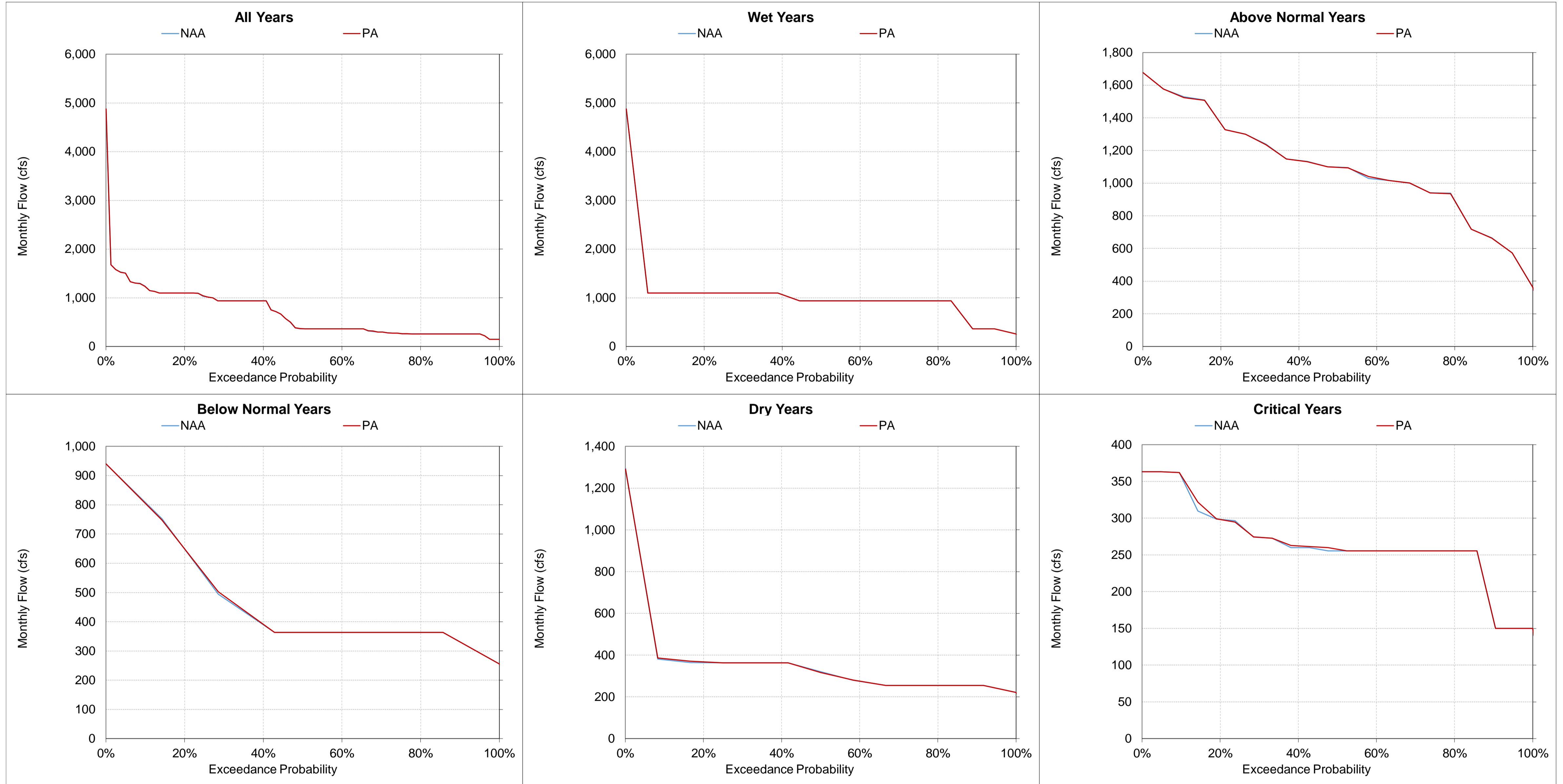
Figure 5.A.6-21-16. Stanislaus River at Goodwin, Monthly Flow June
