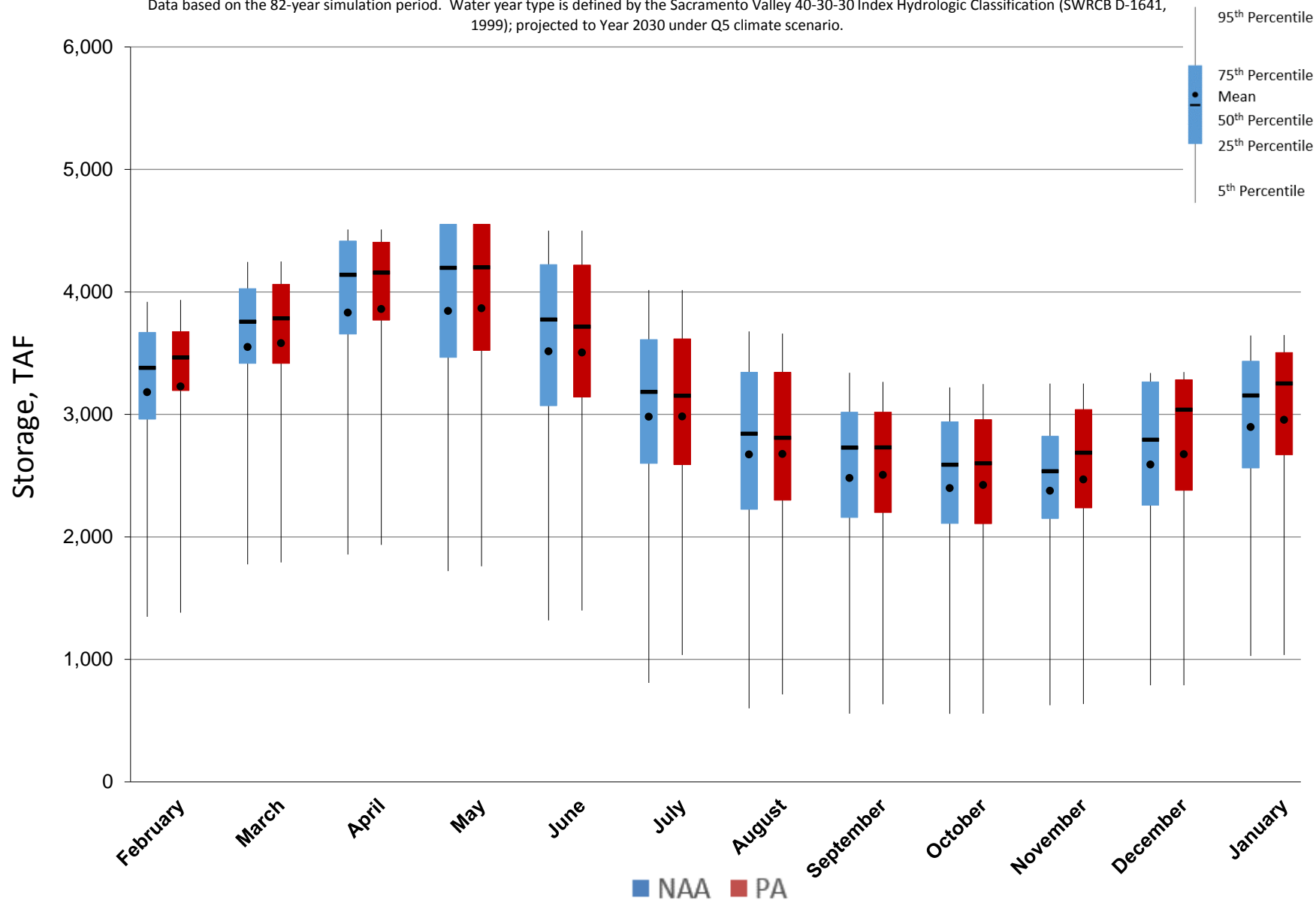
Figure 5.A.6-3-1. End of Month Storage Ranges For Shasta Lake, All Years
