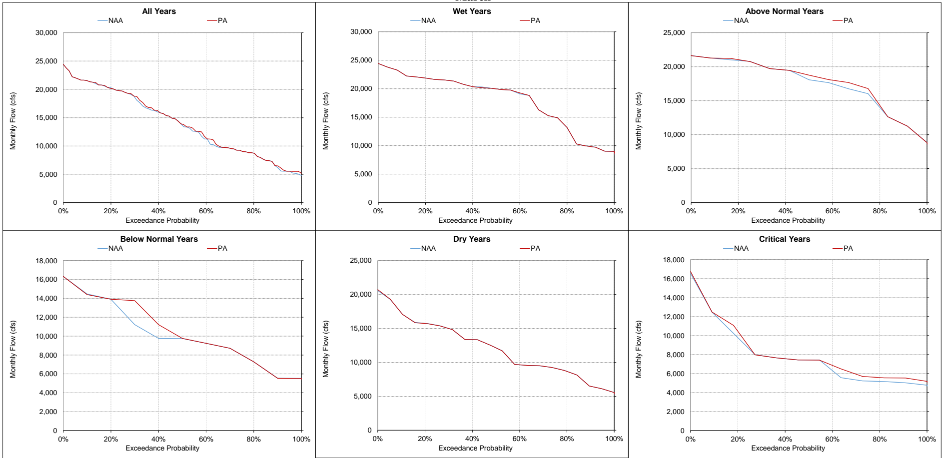
Figure 5.A.6-11-13. Sacramento River at Bend Bridge, Monthly Flow March
