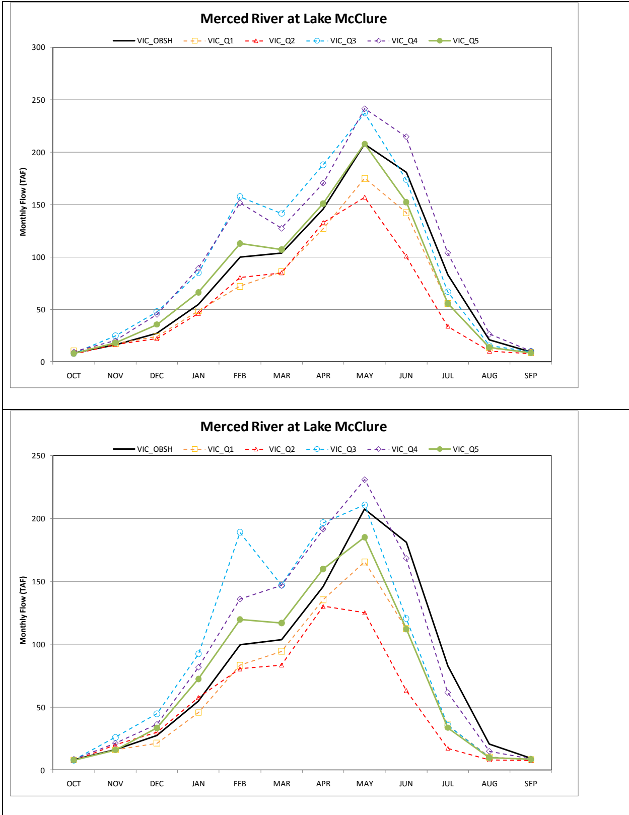
Figure 5.A.A.2-14. Simulated Changes in Monthly Natural Streamflow for Merced River at Lake McClure (top, 2025 changes; bottom, 2060 changes).
