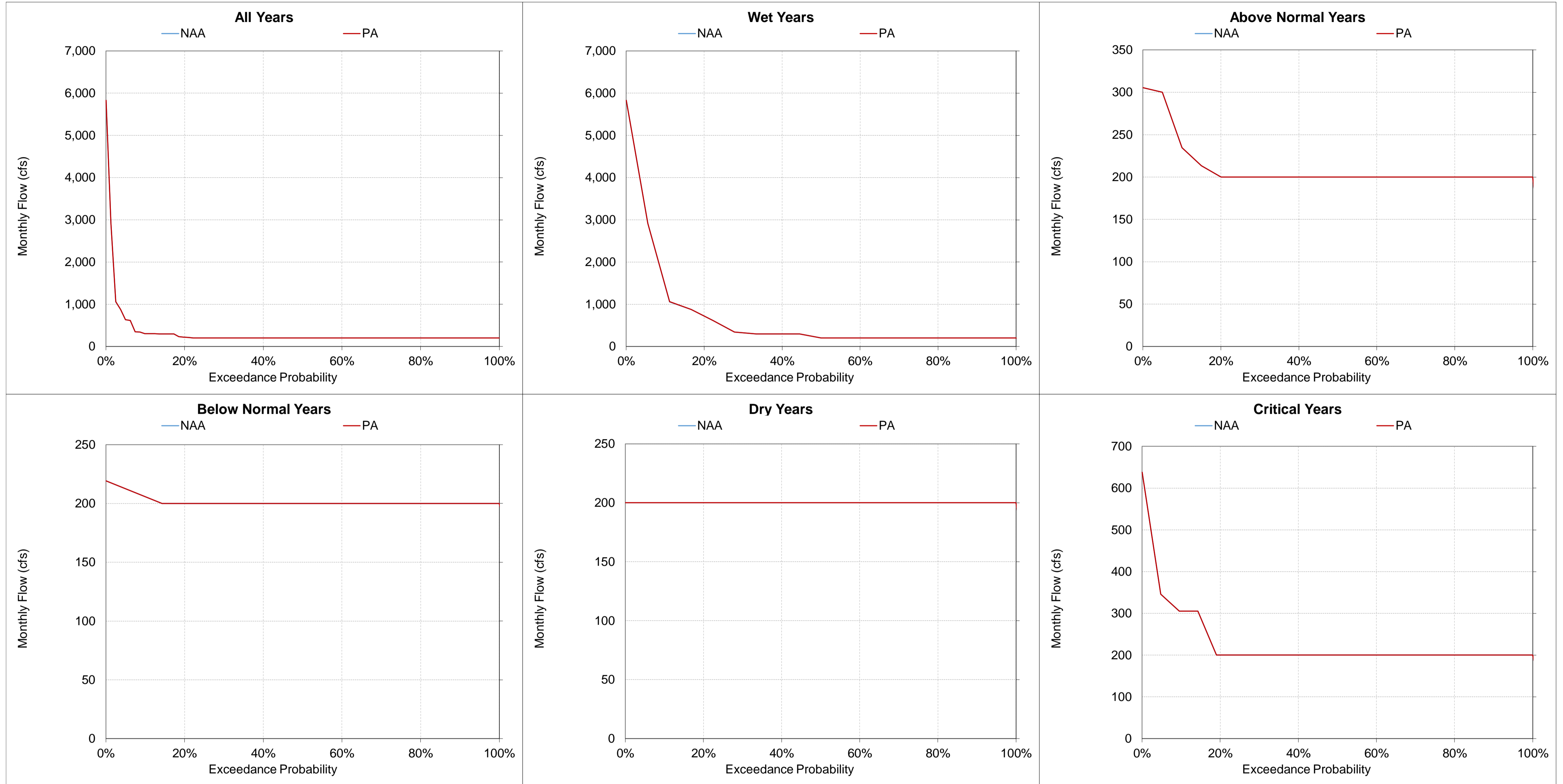
Figure 5.A.6-21-10. Stanislaus River at Goodwin, Monthly Flow December
