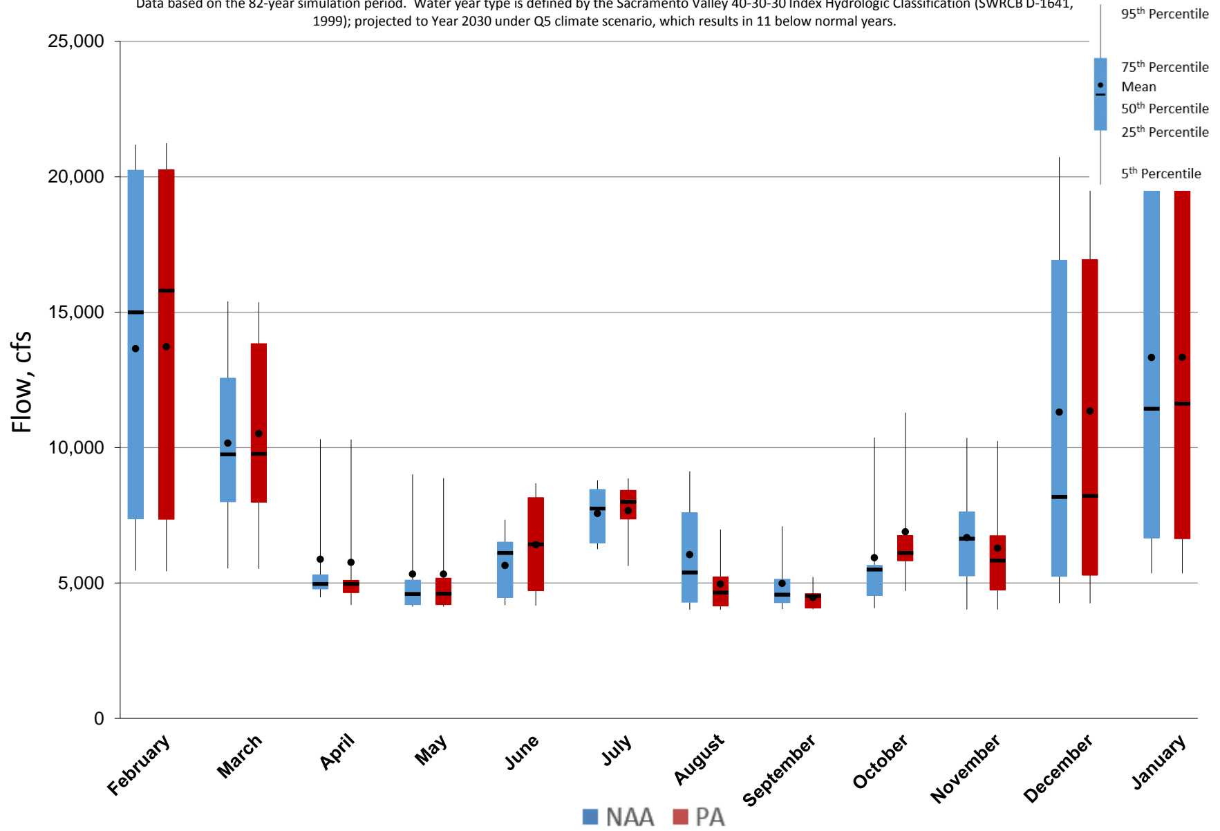
Figure 5.A.6-36-4. Monthly Flow Ranges For Sacramento River at Wilkins Slough, Below Normal Years
