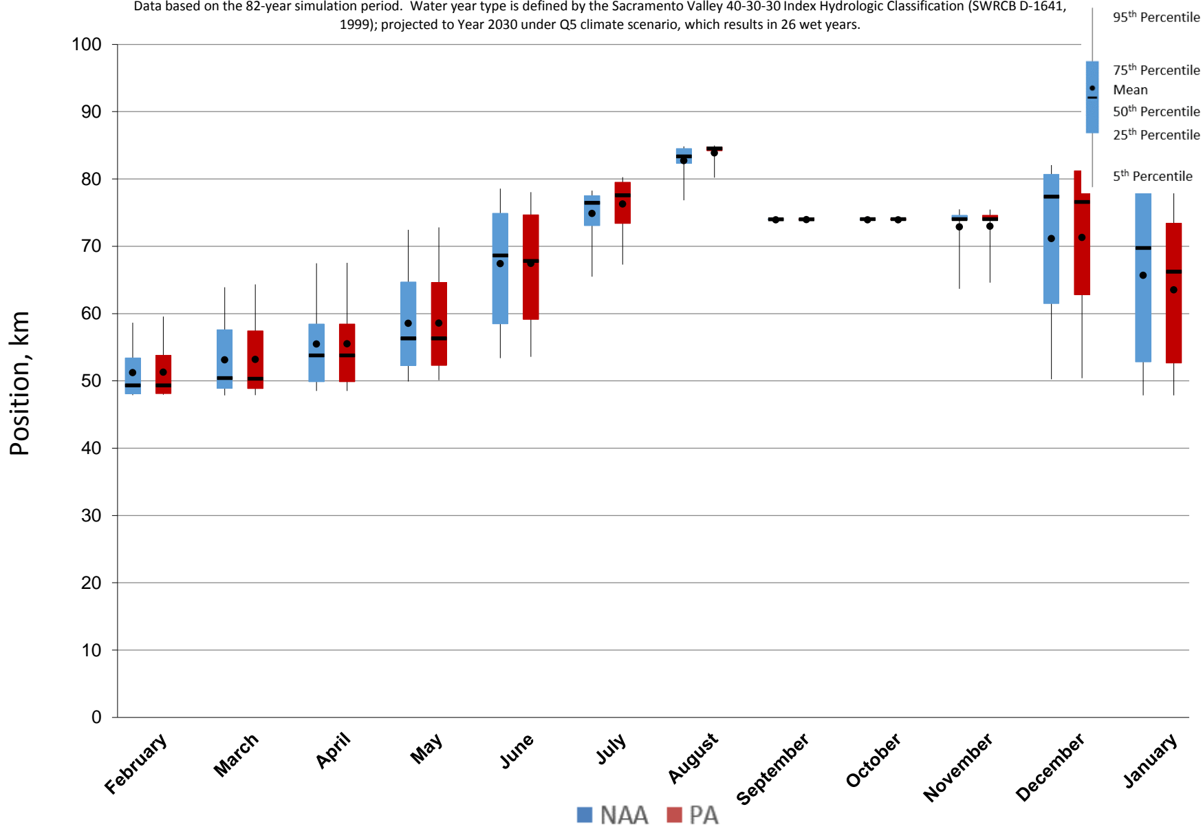
Figure 5.A.6-29-2. End of Month Position Ranges For X2, Wet Years
