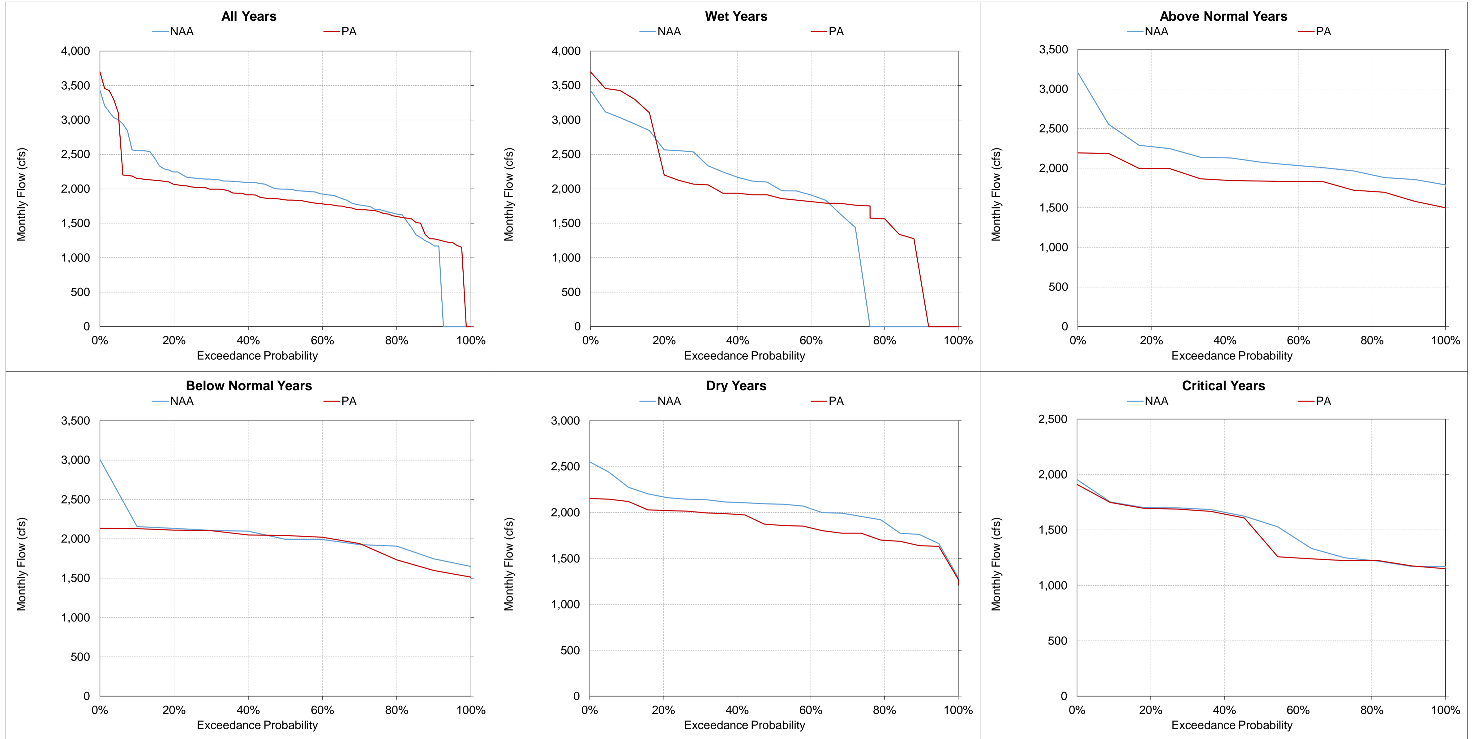
Figure 5.A.6-32-16. Delta Cross Channel, Monthly Flow June
