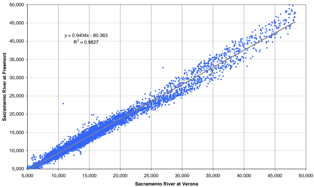
Sacramento River Flows Comparison Between Fremont and Verona Data from CDEC and USGS
