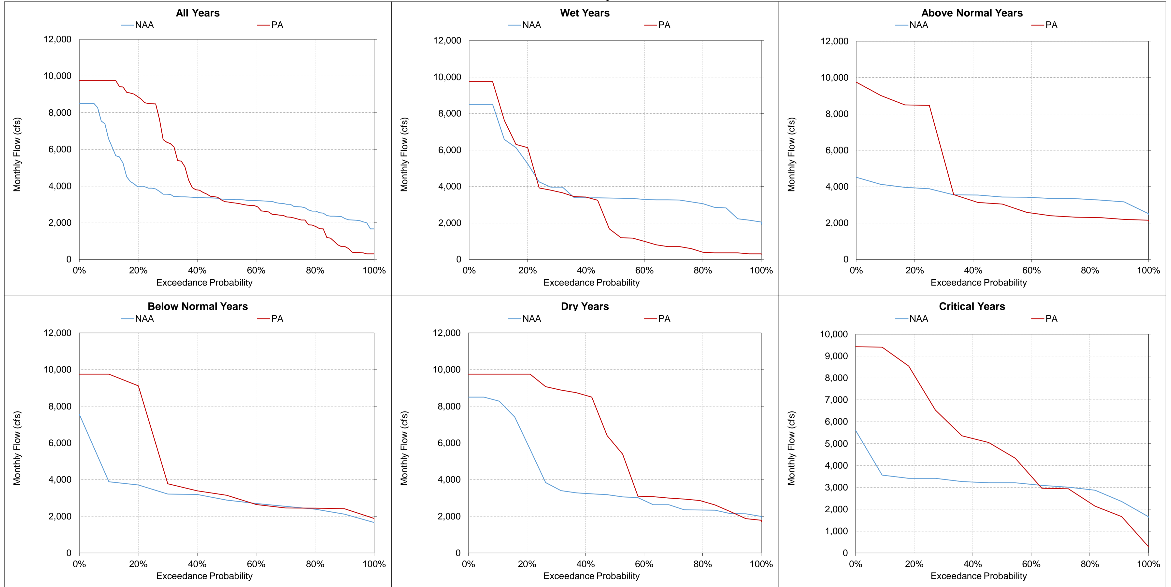
Figure 5.A.6-34-11. Total Banks Pumping Plant Exports, Monthly Flow January
