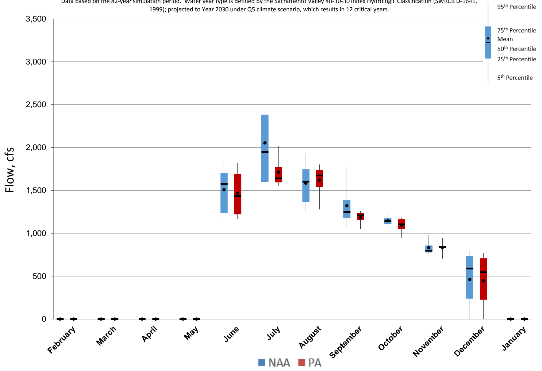
Figure 5.A.6-32-6. Monthly Flow Ranges For Delta Cross Channel, Critical Years
