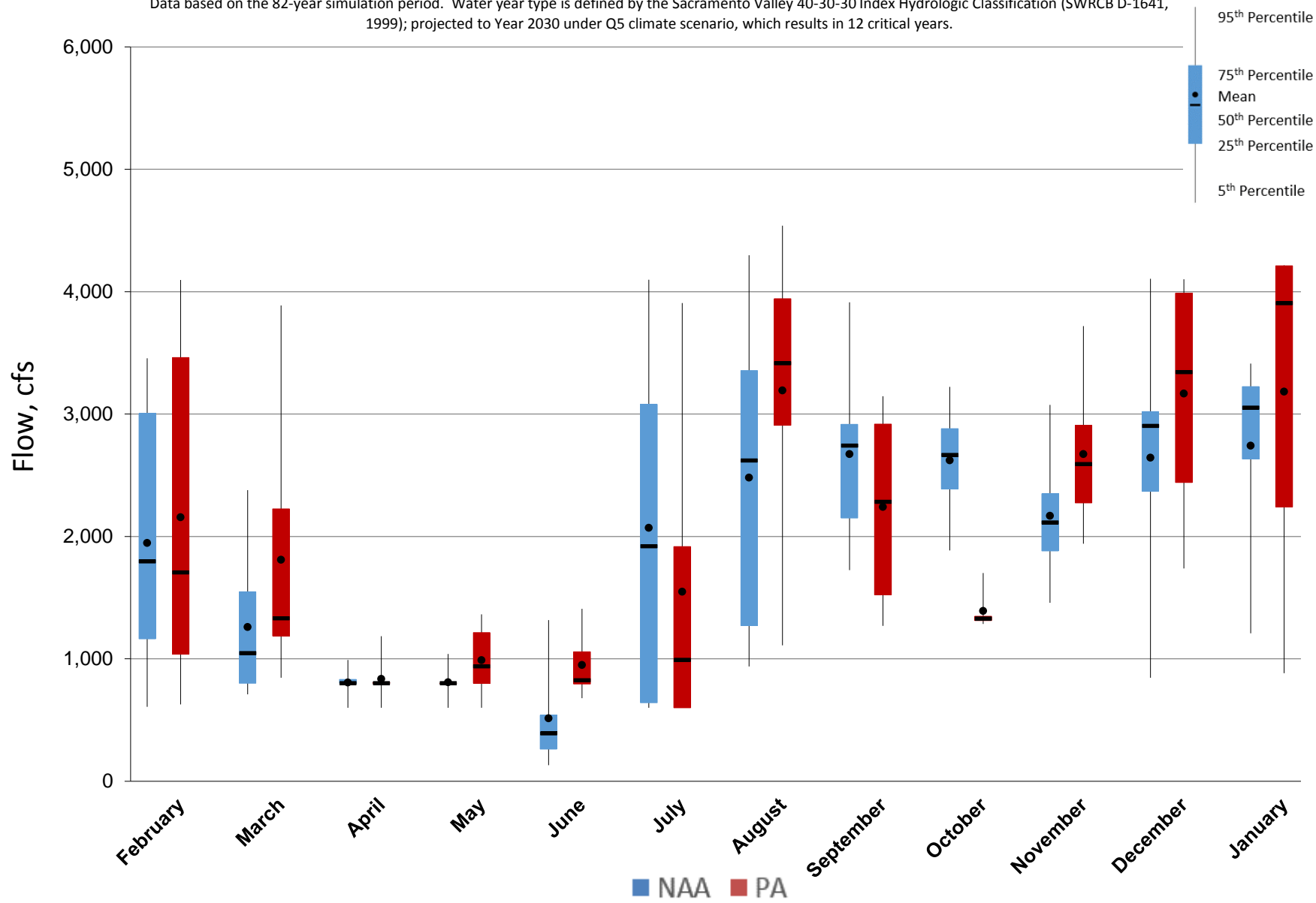
Figure 5.A.6-33-6. Monthly Flow Ranges For Total Jones Pumping Plant Exports, Critical Years
