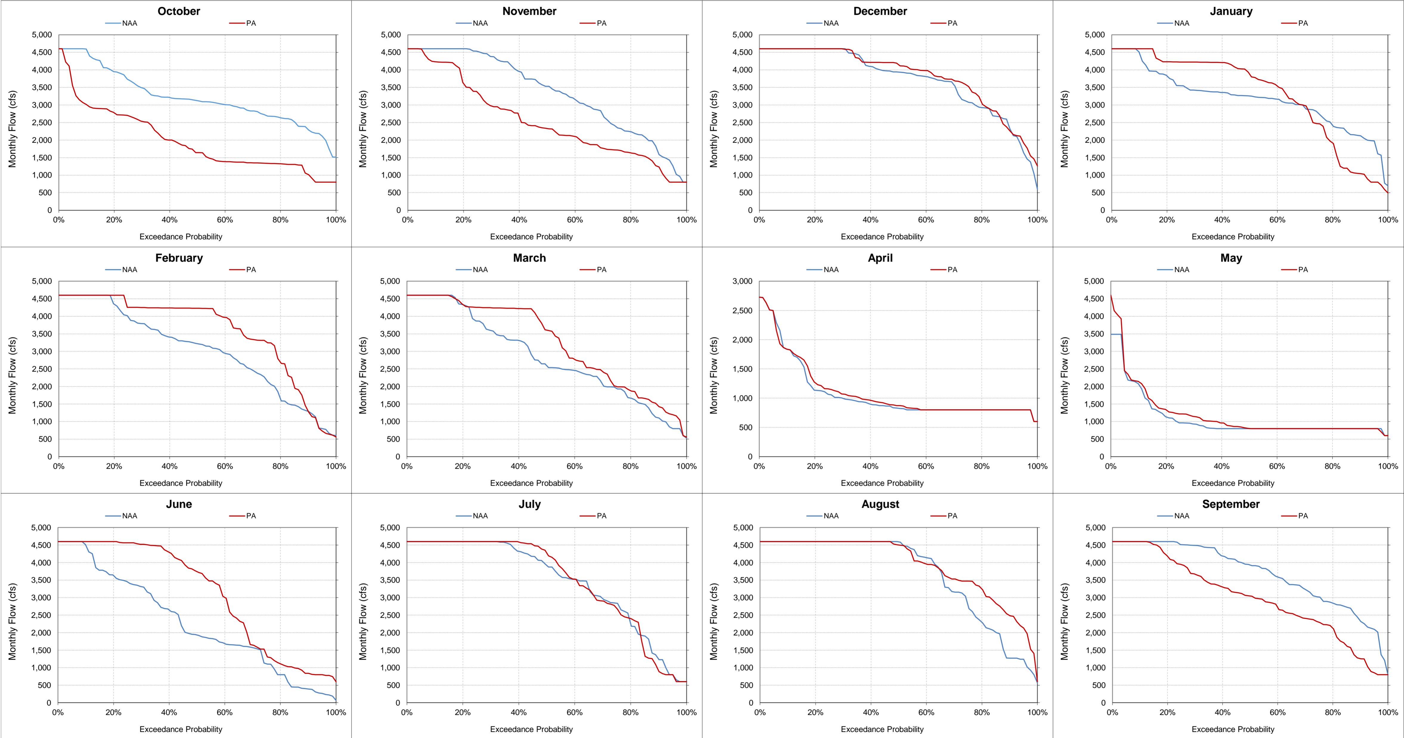
Figure 5.A.6-33-7. Total Jones Pumping Plant Exports, Monthly Flow Probability of Exceedance
