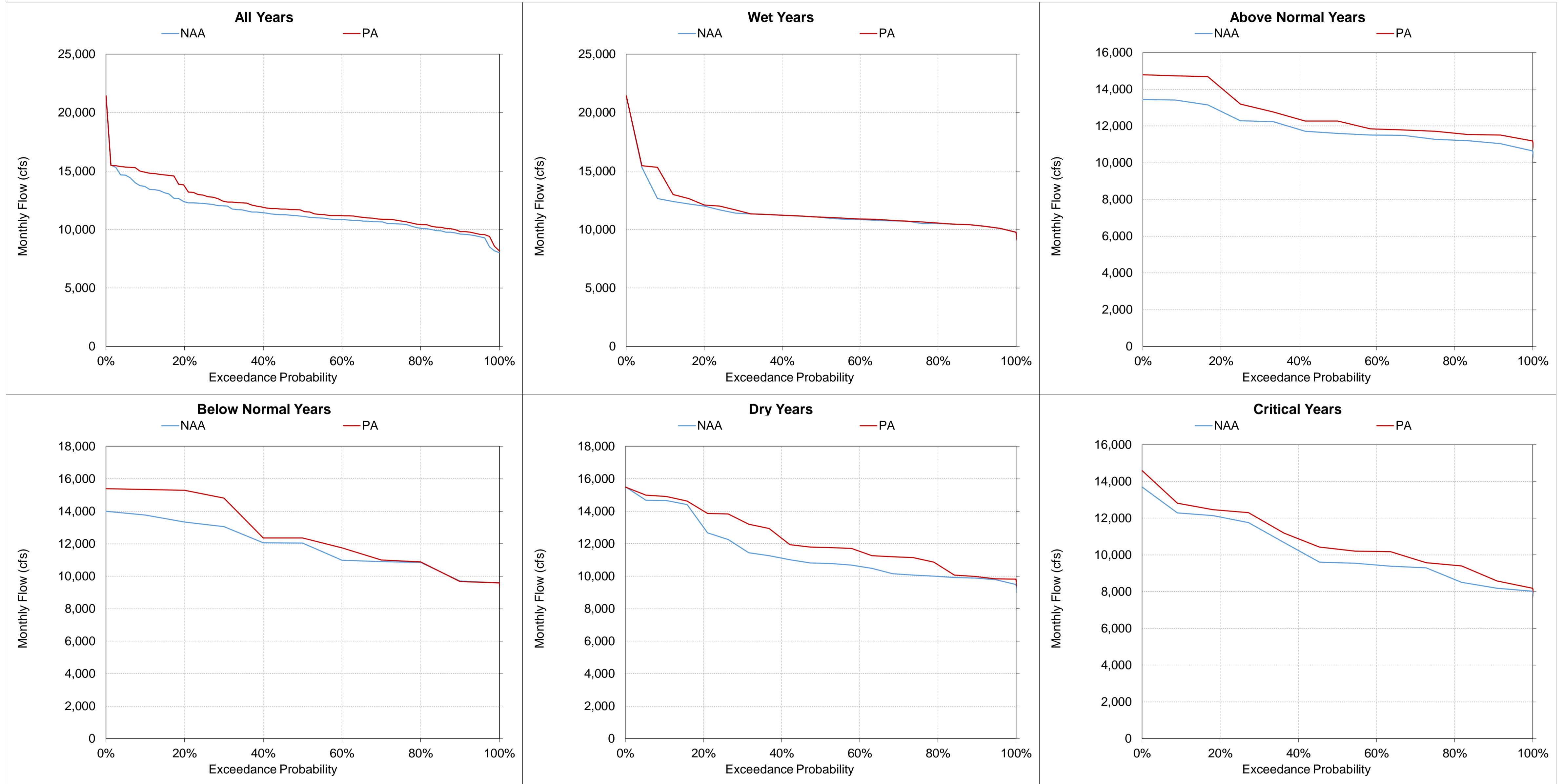
Figure 5.A.6-35-16. Sacramento River above Red Bluff Diversion Dam, Monthly Flow June
