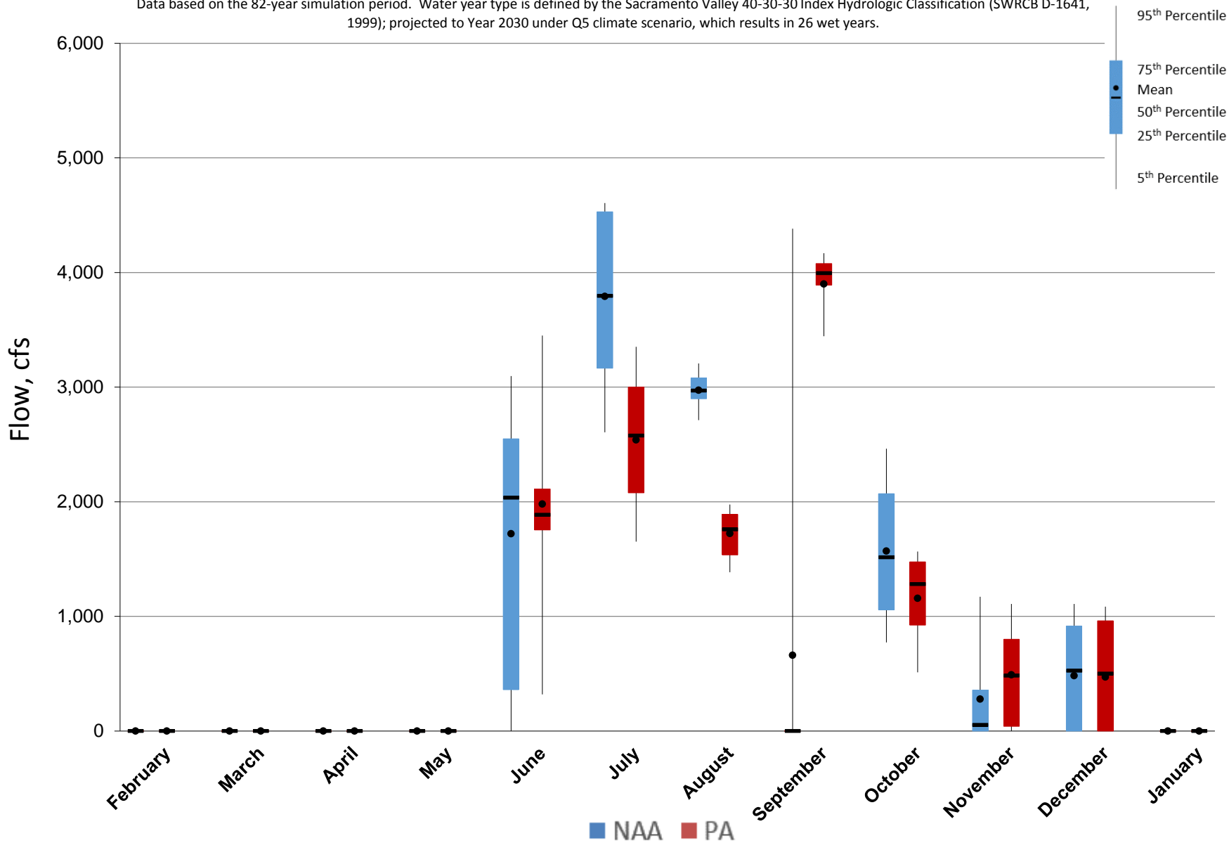
Figure 5.A.6-32-2. Monthly Flow Ranges For Delta Cross Channel, Wet Years
