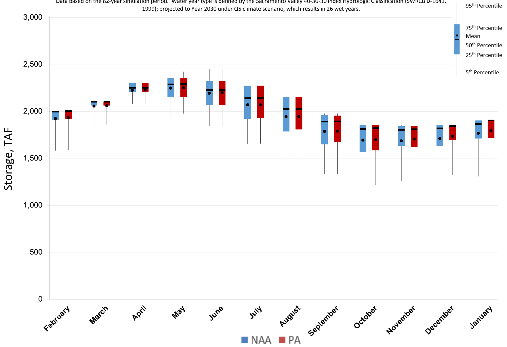
Figure 5.A.6-1-2. End of Month Storage Ranges For Trinity Lake, Wet Years
