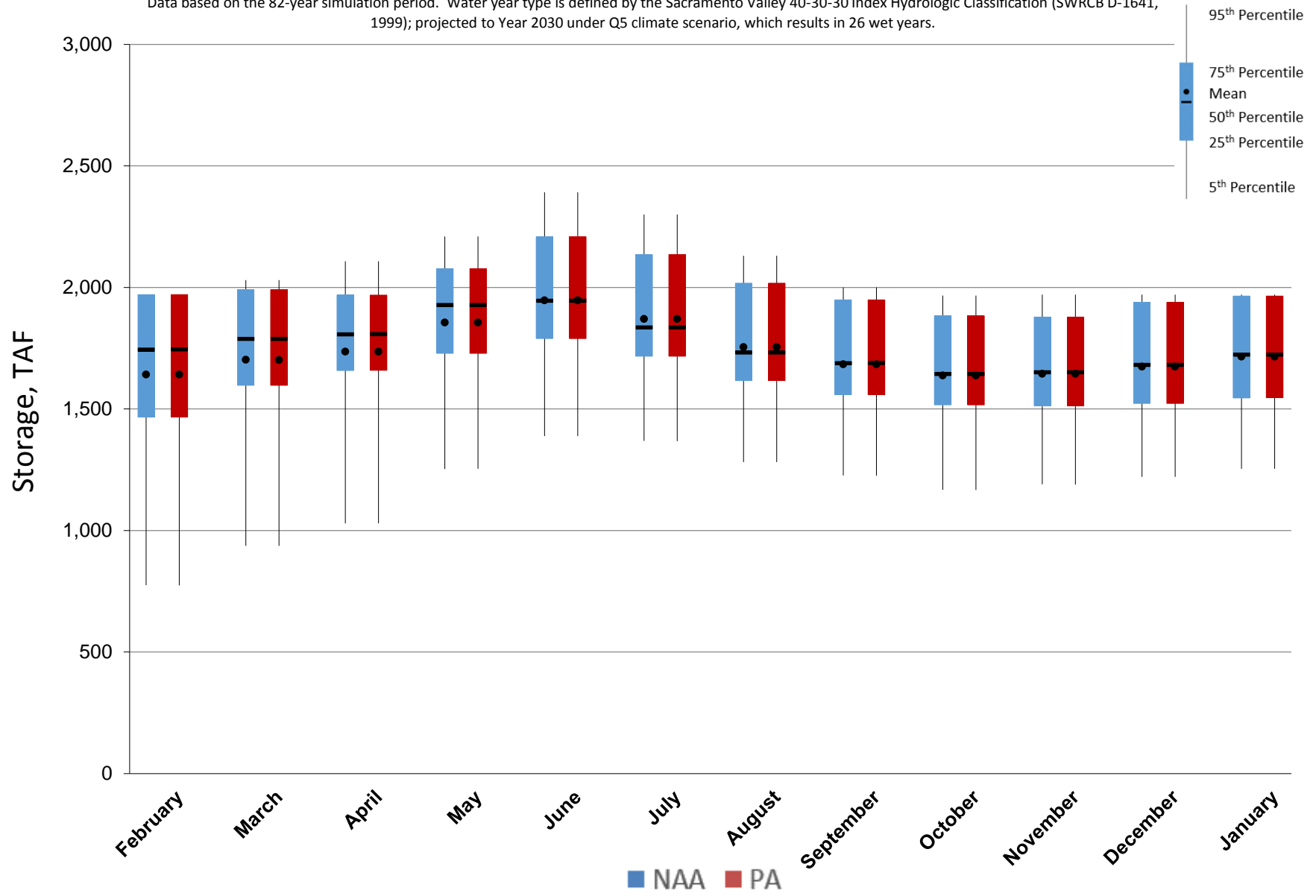
Figure 5.A.6-6-2. End of Month Storage Ranges For New Melones Lake, Wet Years
