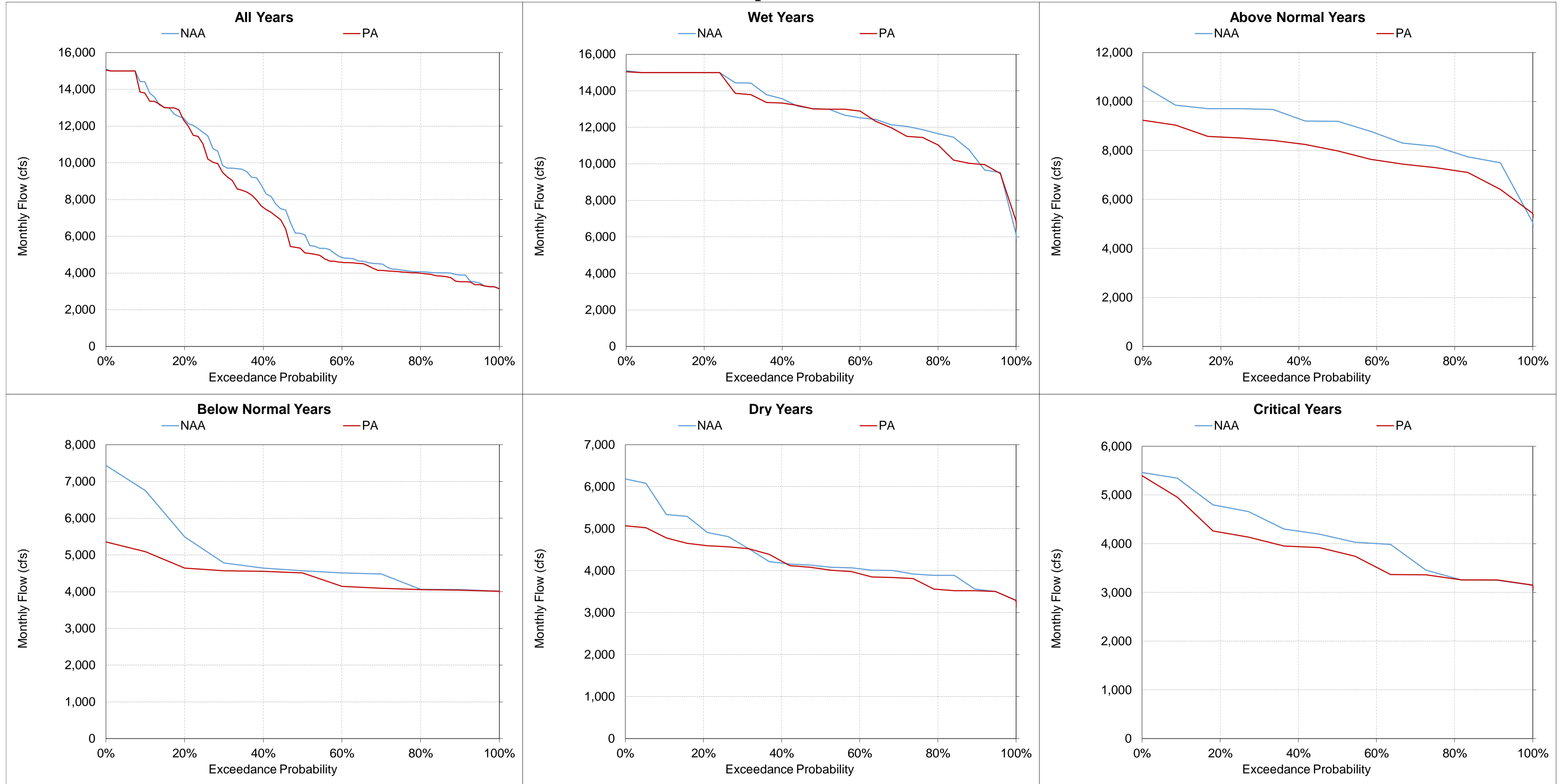
Figure 5.A.6-36-19. Sacramento River at Wilkins Slough, Monthly Flow September
