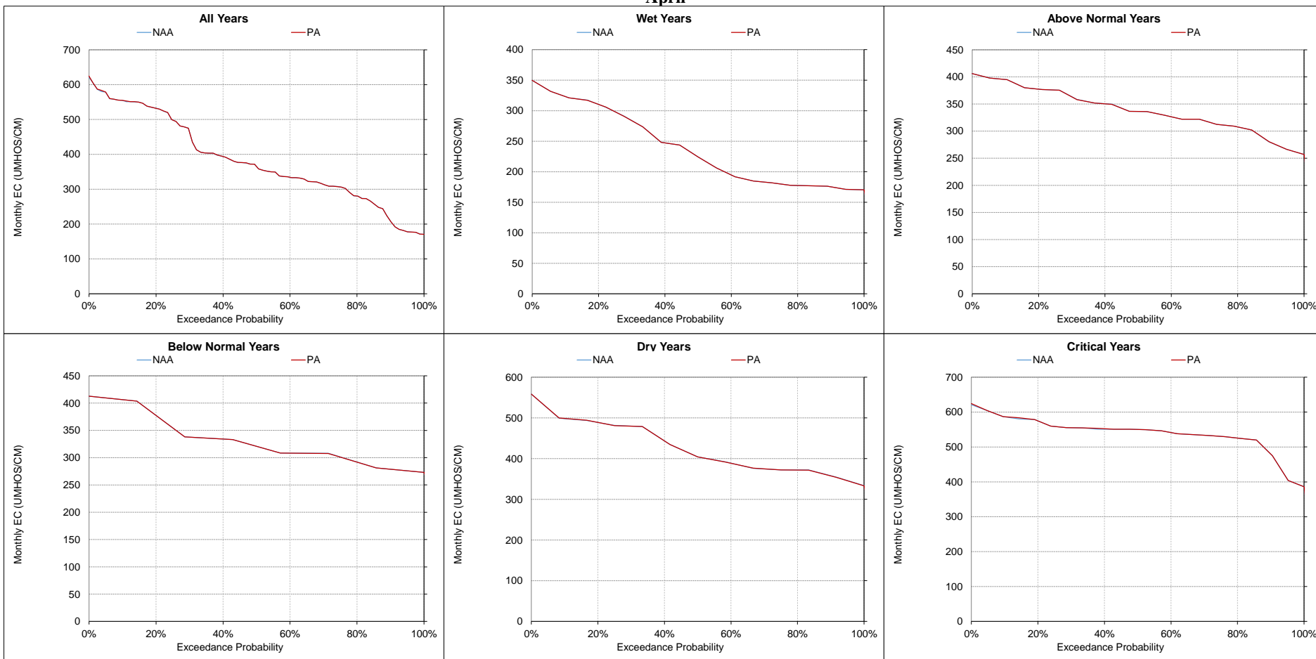
Figure 5.A.6-30-14. San Joaquin River at Vernalis, Monthly EC
