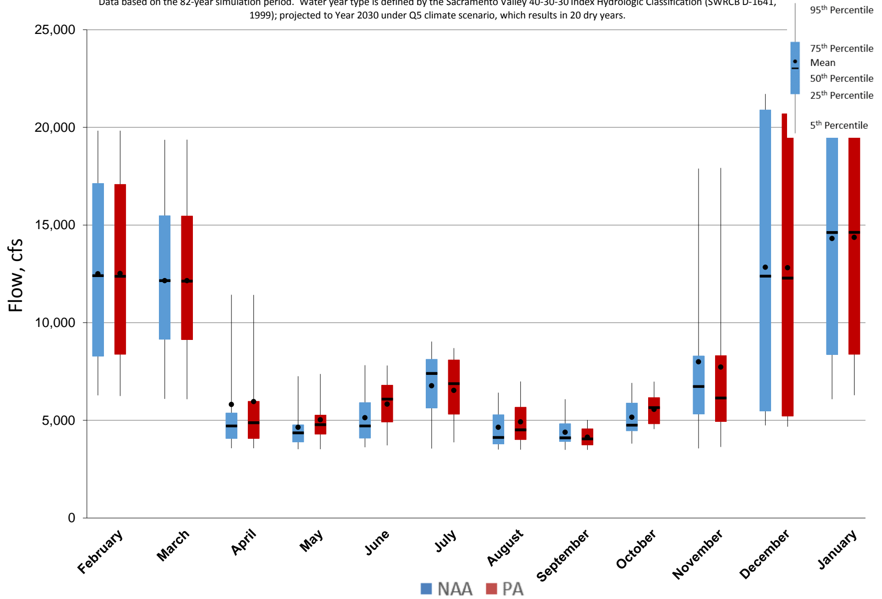
Figure 5.A.6-36-5. Monthly Flow Ranges For Sacramento River at Wilkins Slough, Dry Years
