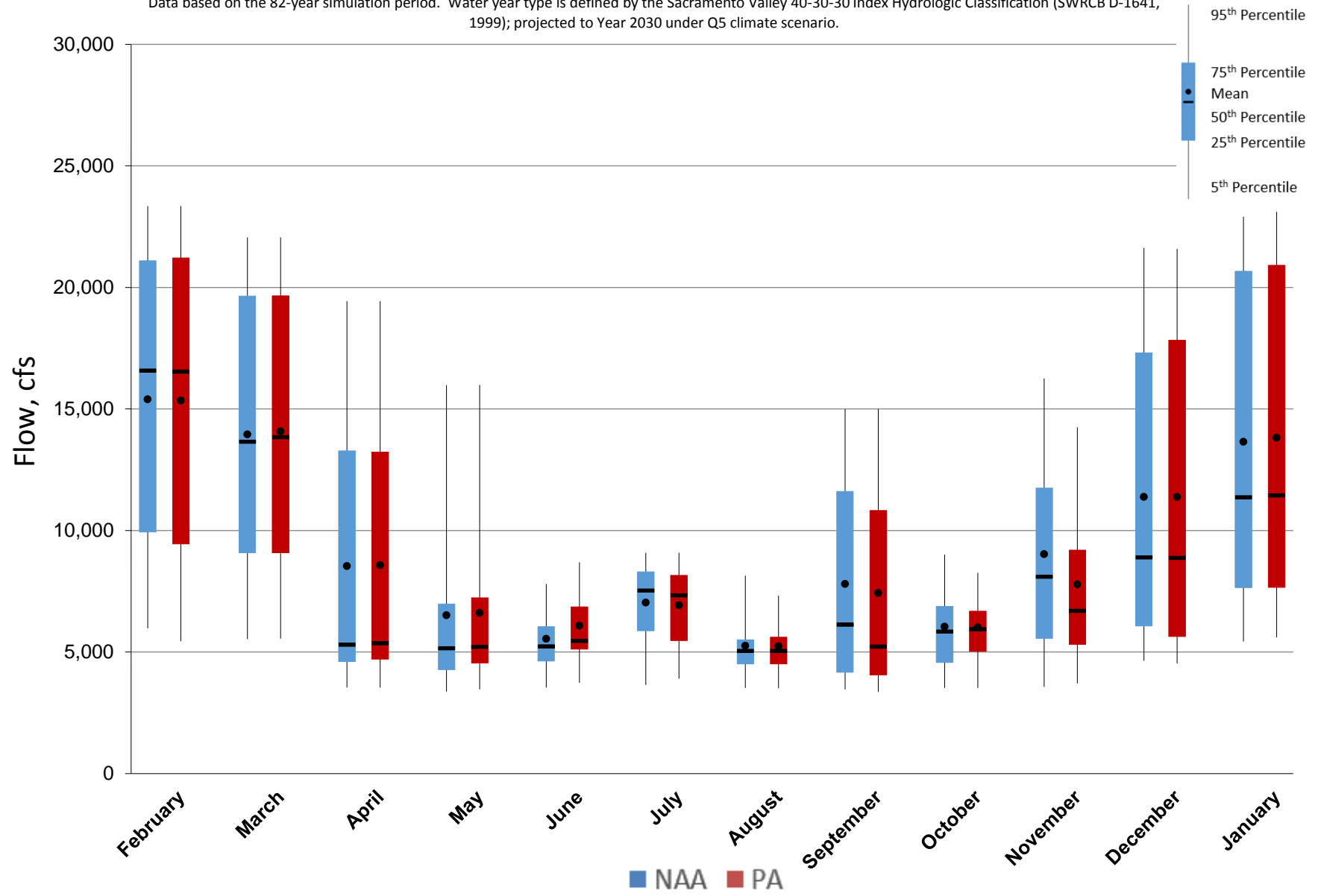
Figure 5.A.6-36-1. Monthly Flow Ranges For Sacramento River at Wilkins Slough, All Years
