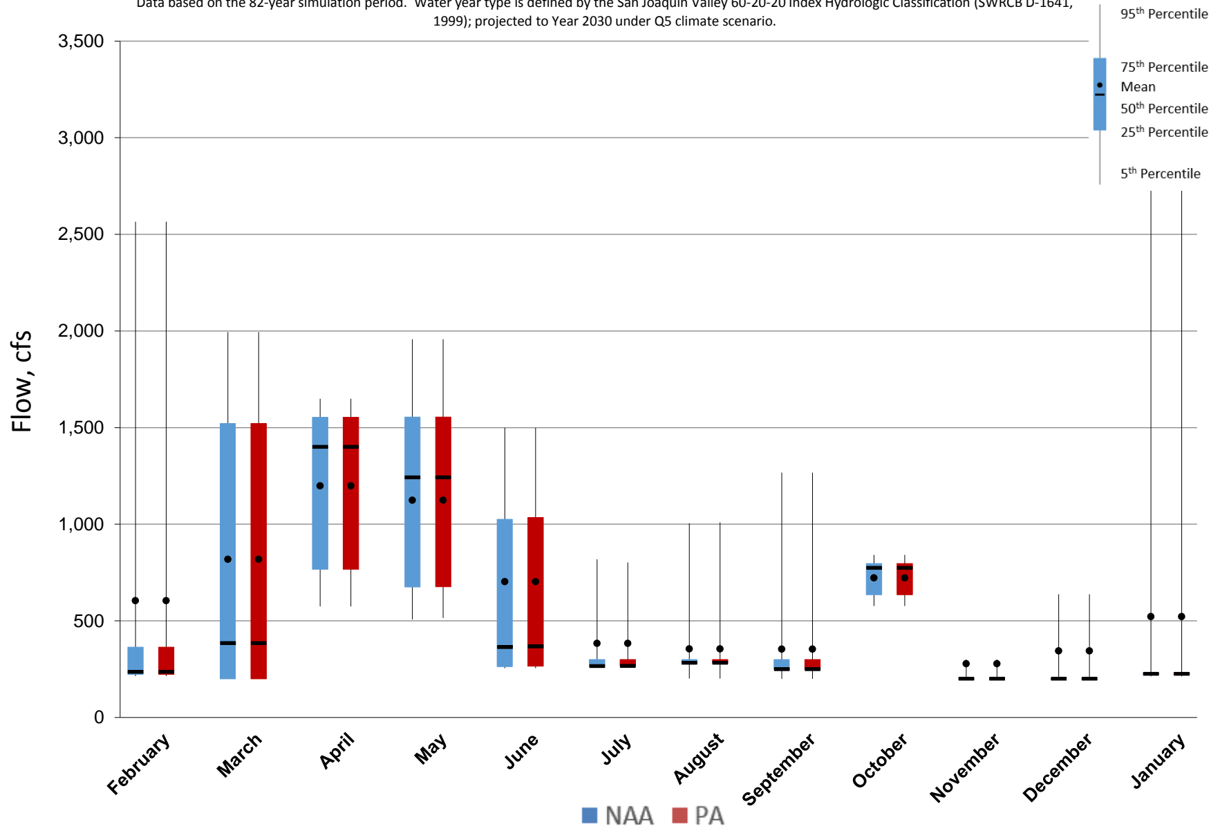
Figure 5.A.6-21-1. Monthly Flow Ranges for Stanislaus River at Goodwin, All Years
