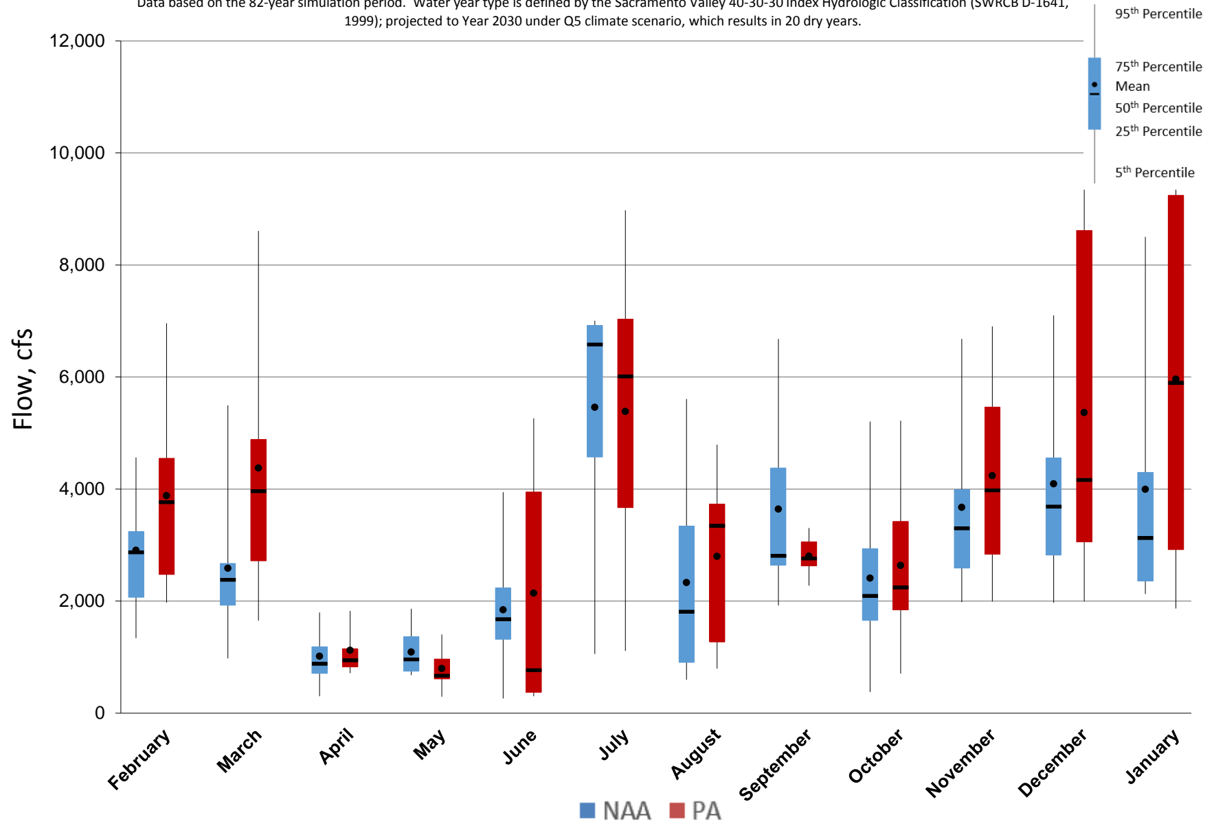
Figure 5.A.6-34-5. Monthly Flow Ranges For Total Banks Pumping Plant Exports, Dry Years
