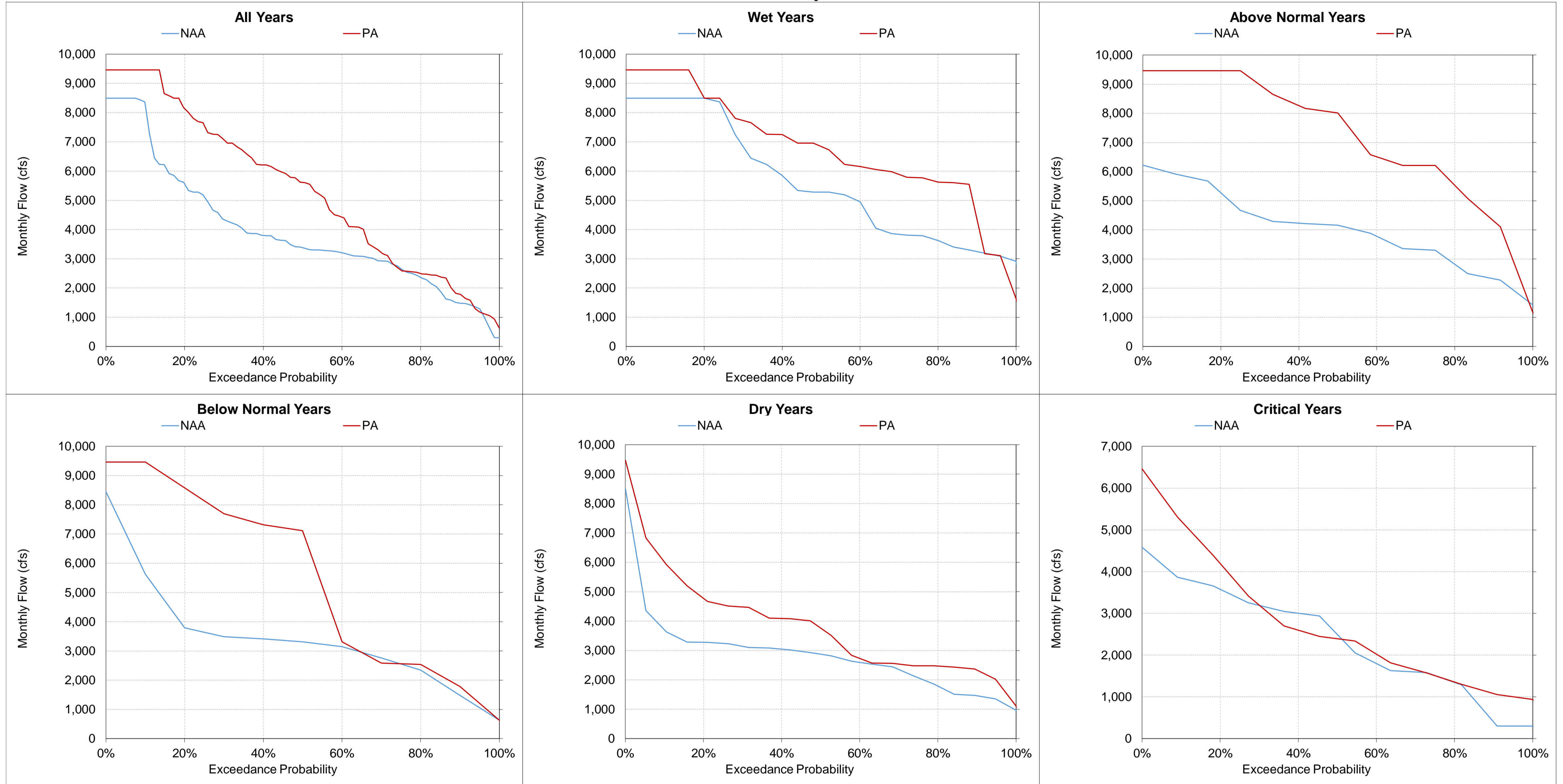
Figure 5.A.6-34-12. Total Banks Pumping Plant Exports, Monthly Flow February
