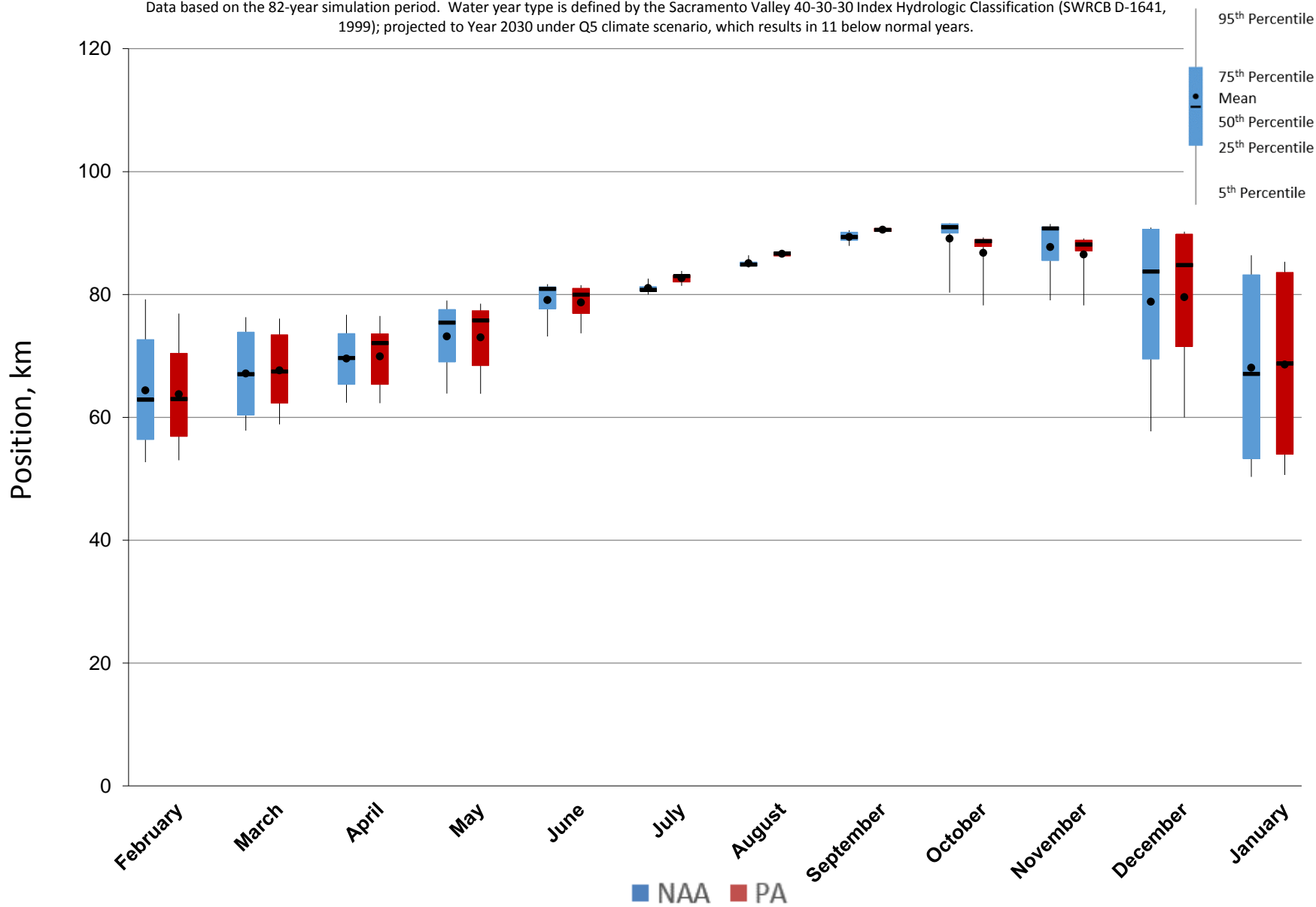
Figure 5.A.6-29-4. End of Month Position Ranges For X2, Below Normal Years
