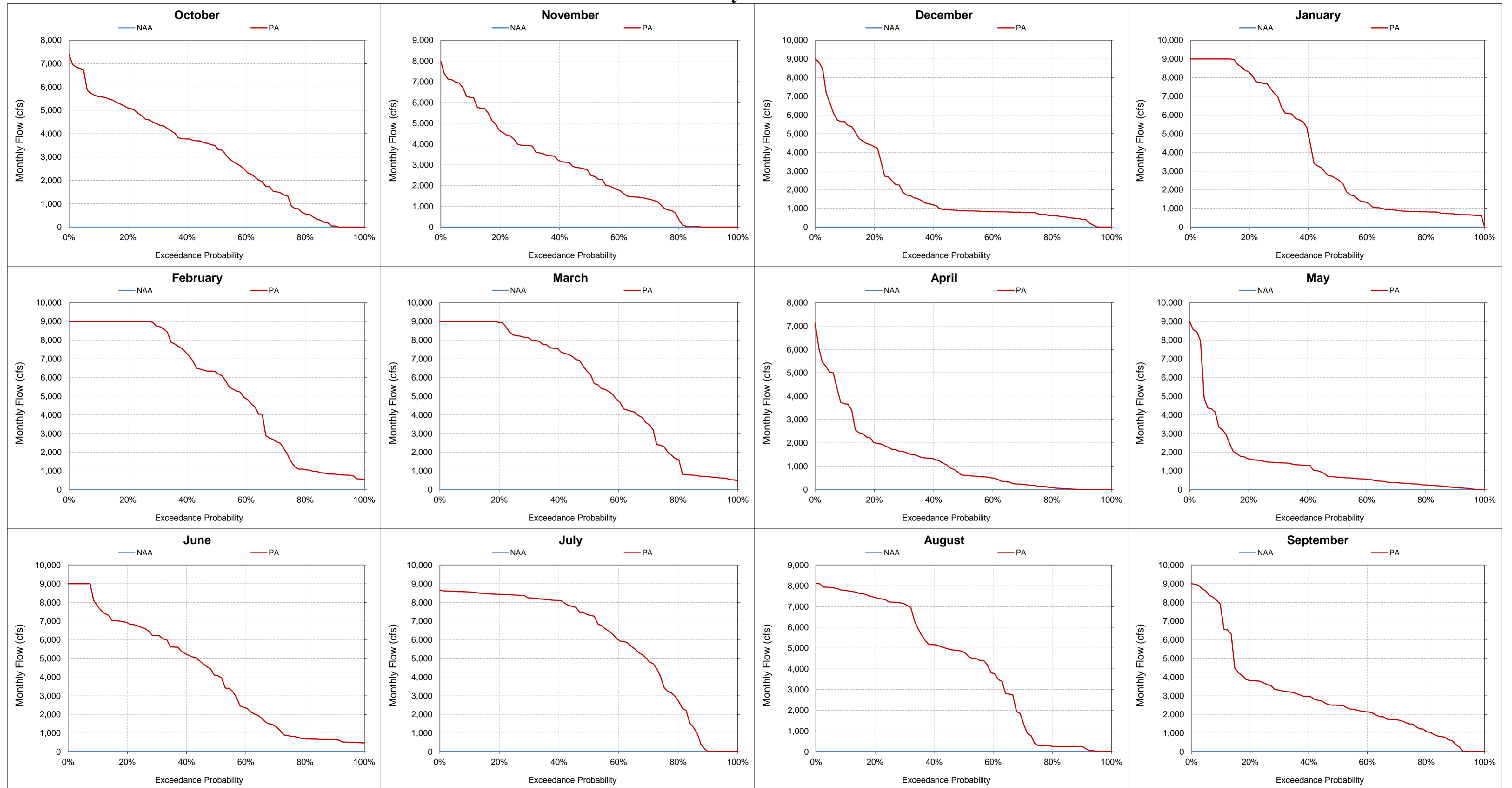
Figure 5.A.6-19-7. North Delta Diversions near Hood, Monthly Flow Probability of Exceedance
