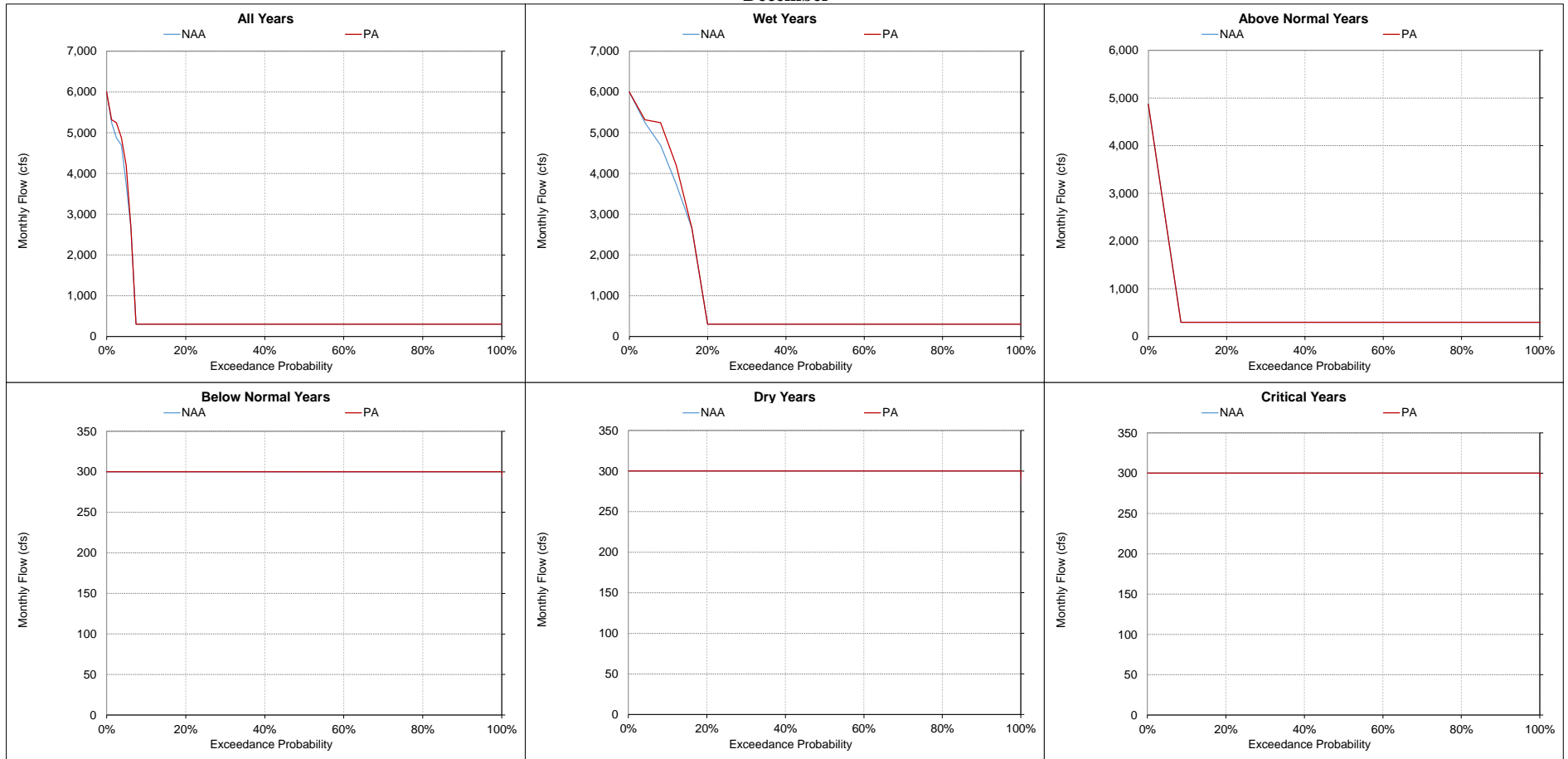
Figure 5.A.6-7-10. Trinity River below Lewiston Dam, Monthly Flow December
