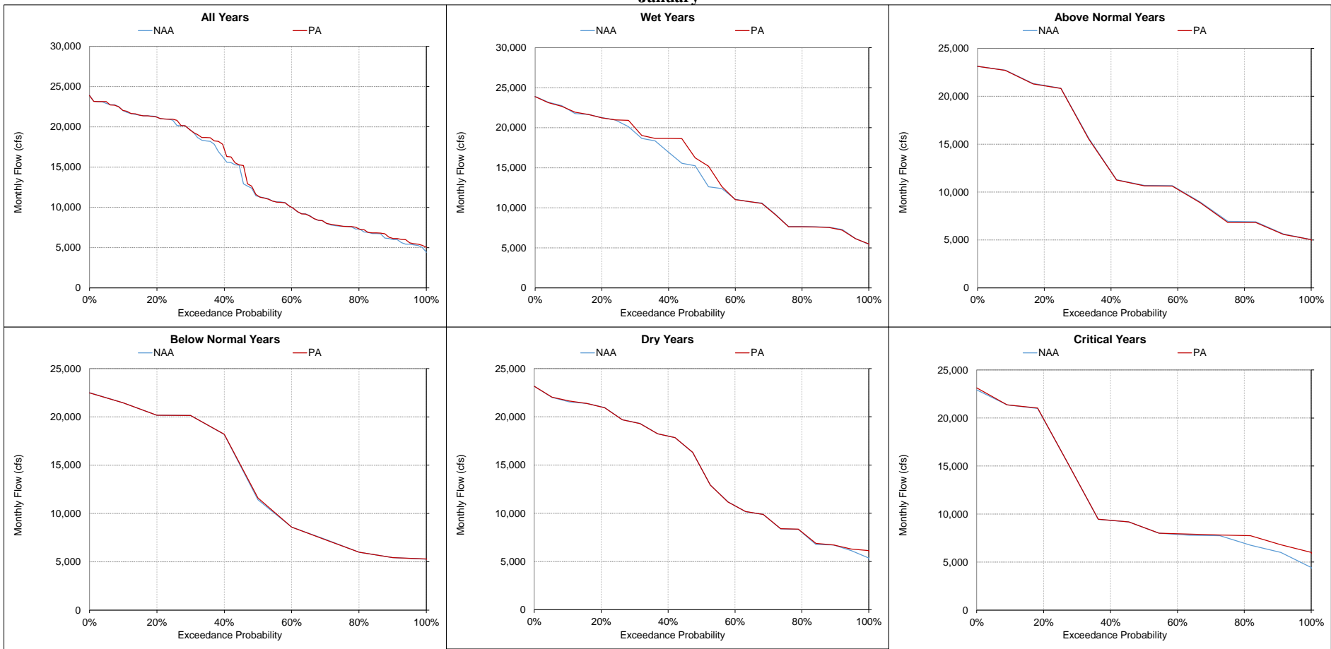
Figure 5.A.6-11-11. Sacramento River at Bend Bridge, Monthly Flow January
