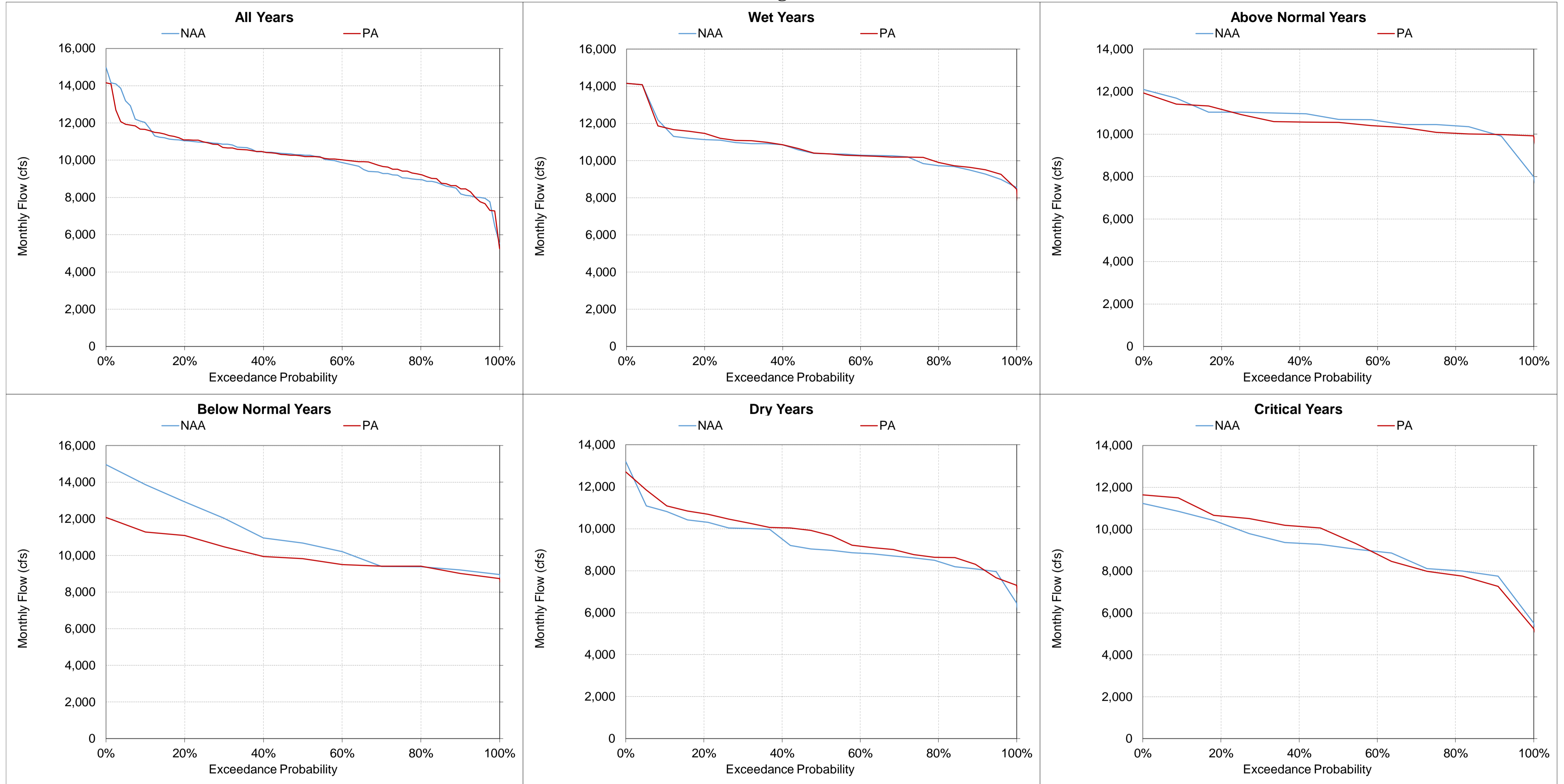
Figure 5.A.6-35-18. Sacramento River above Red Bluff Diversion Dam, Monthly Flow August
