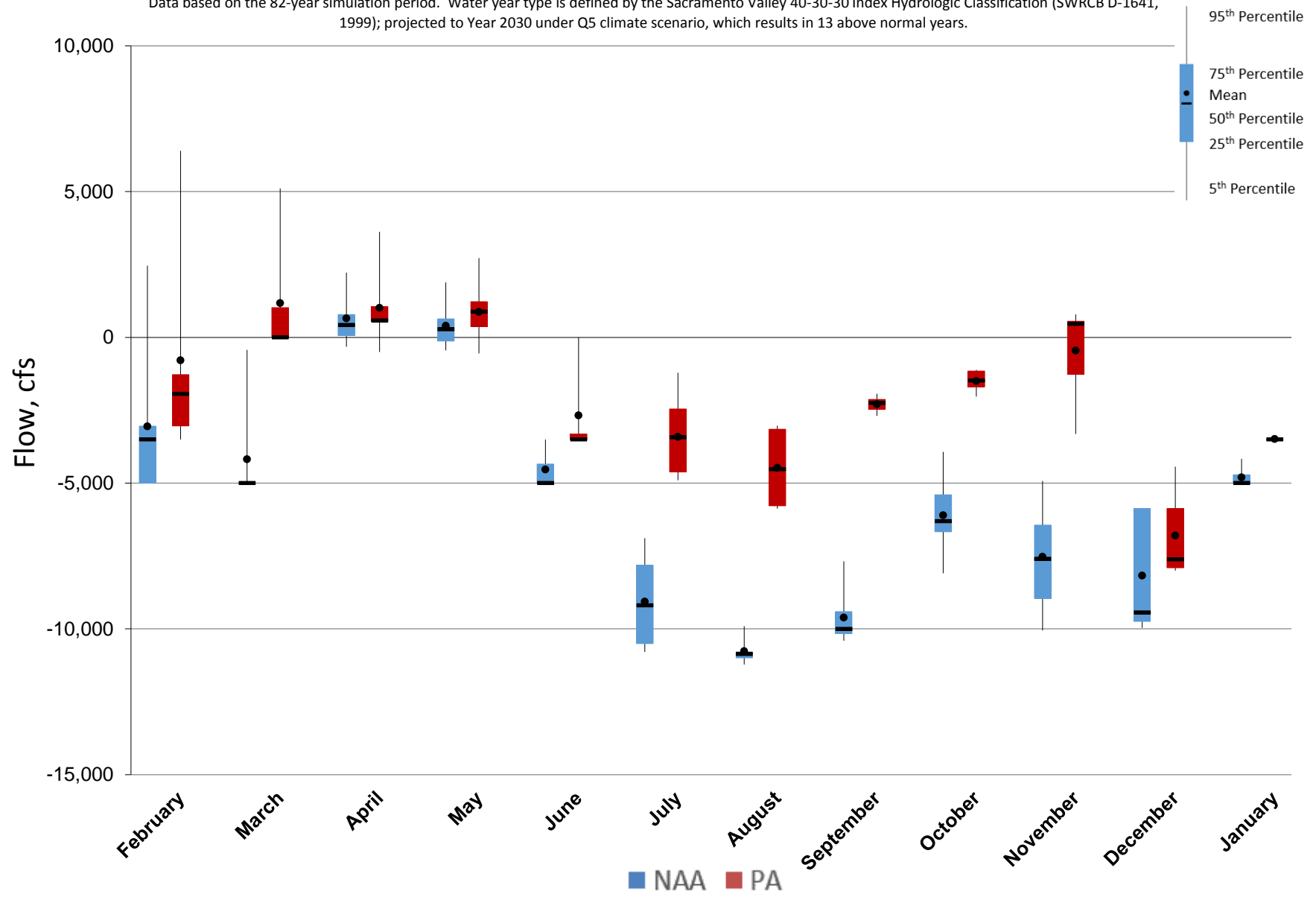
Figure 5.A.6-25-3. Monthly Flow Ranges For Old and Middle River, Above Normal Years
