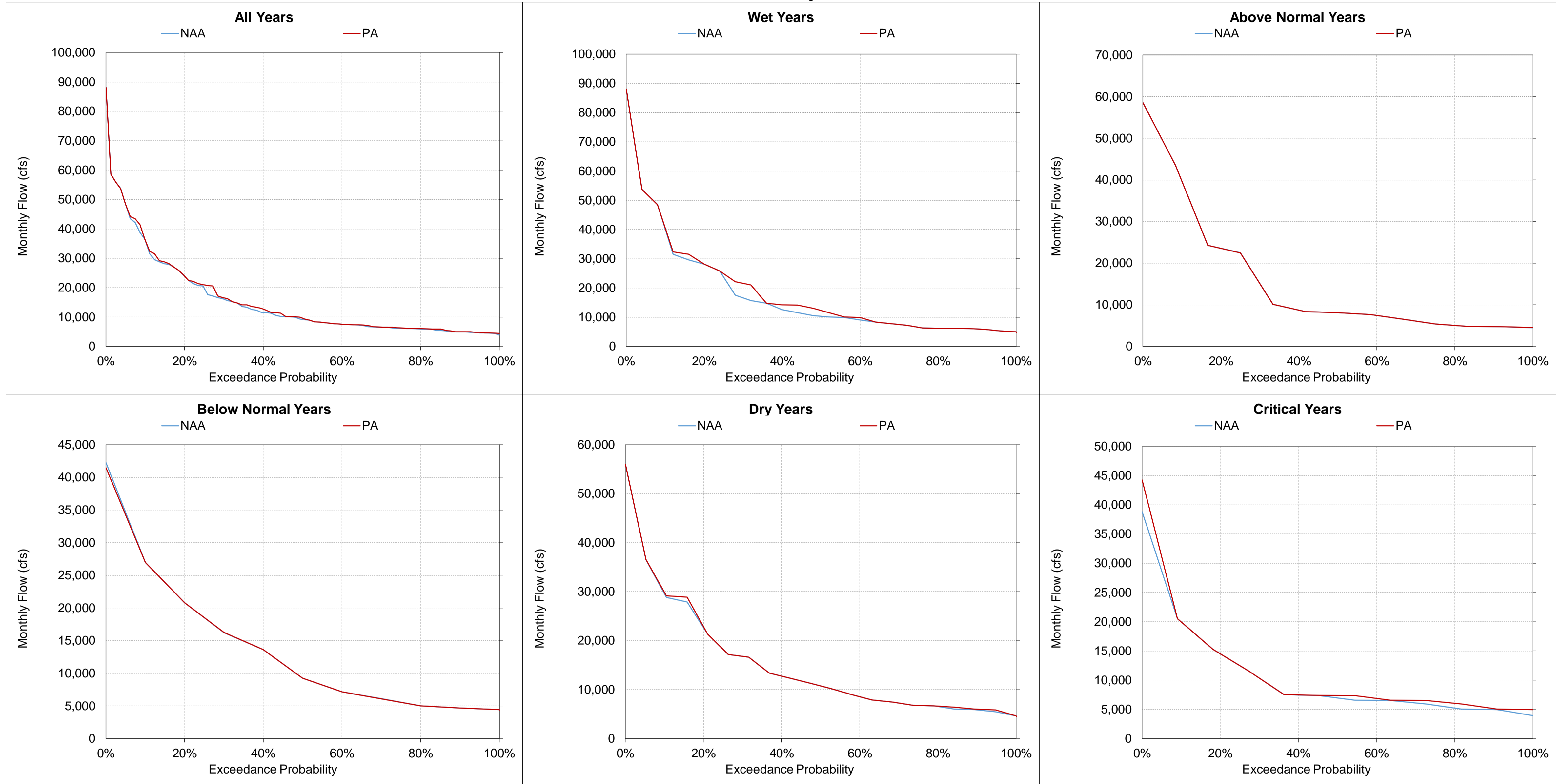
Figure 5.A.6-35-11. Sacramento River above Red Bluff Diversion Dam, Monthly Flow January
