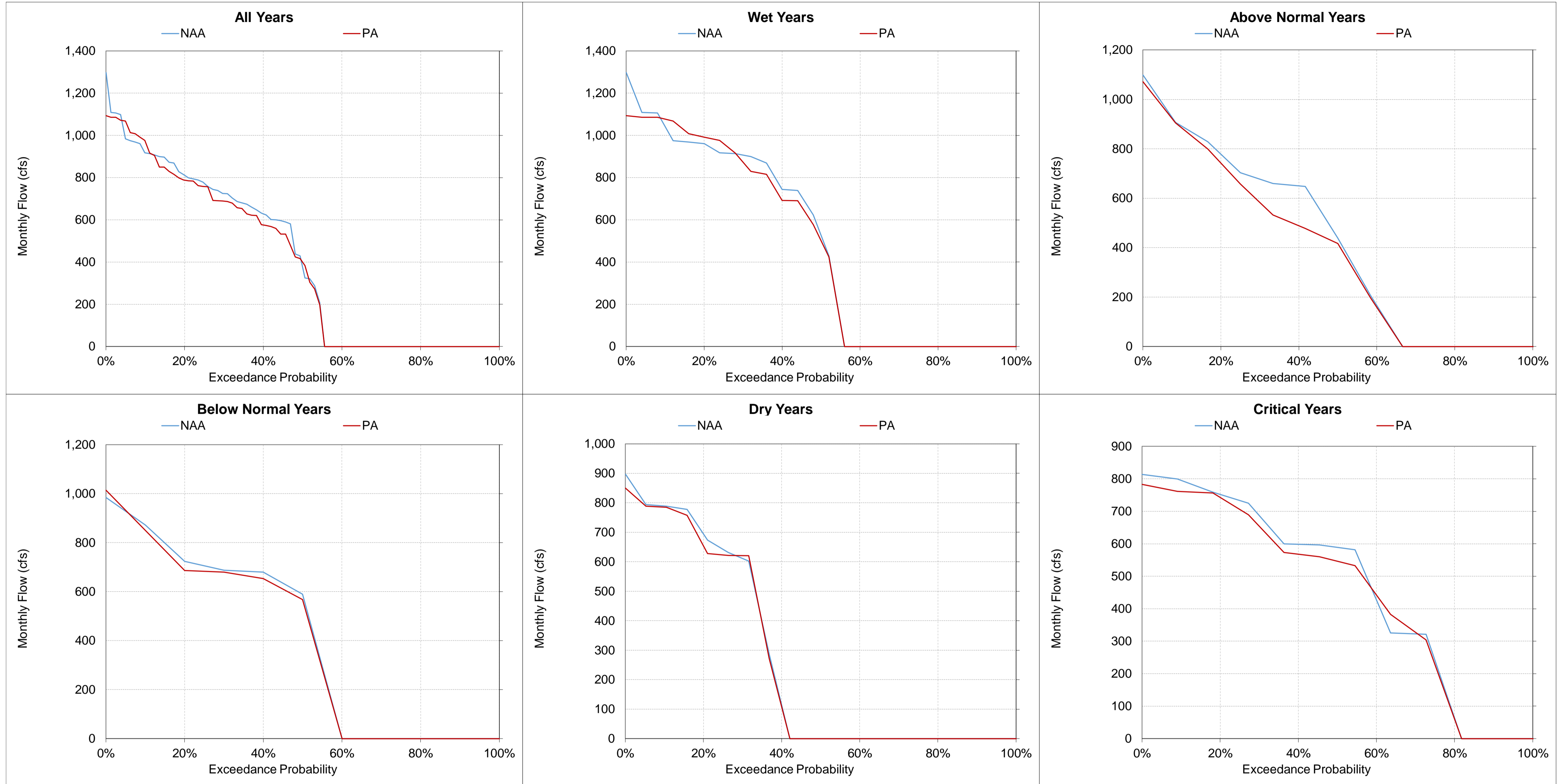
Figure 5.A.6-32-10. Delta Cross Channel, Monthly Flow December
