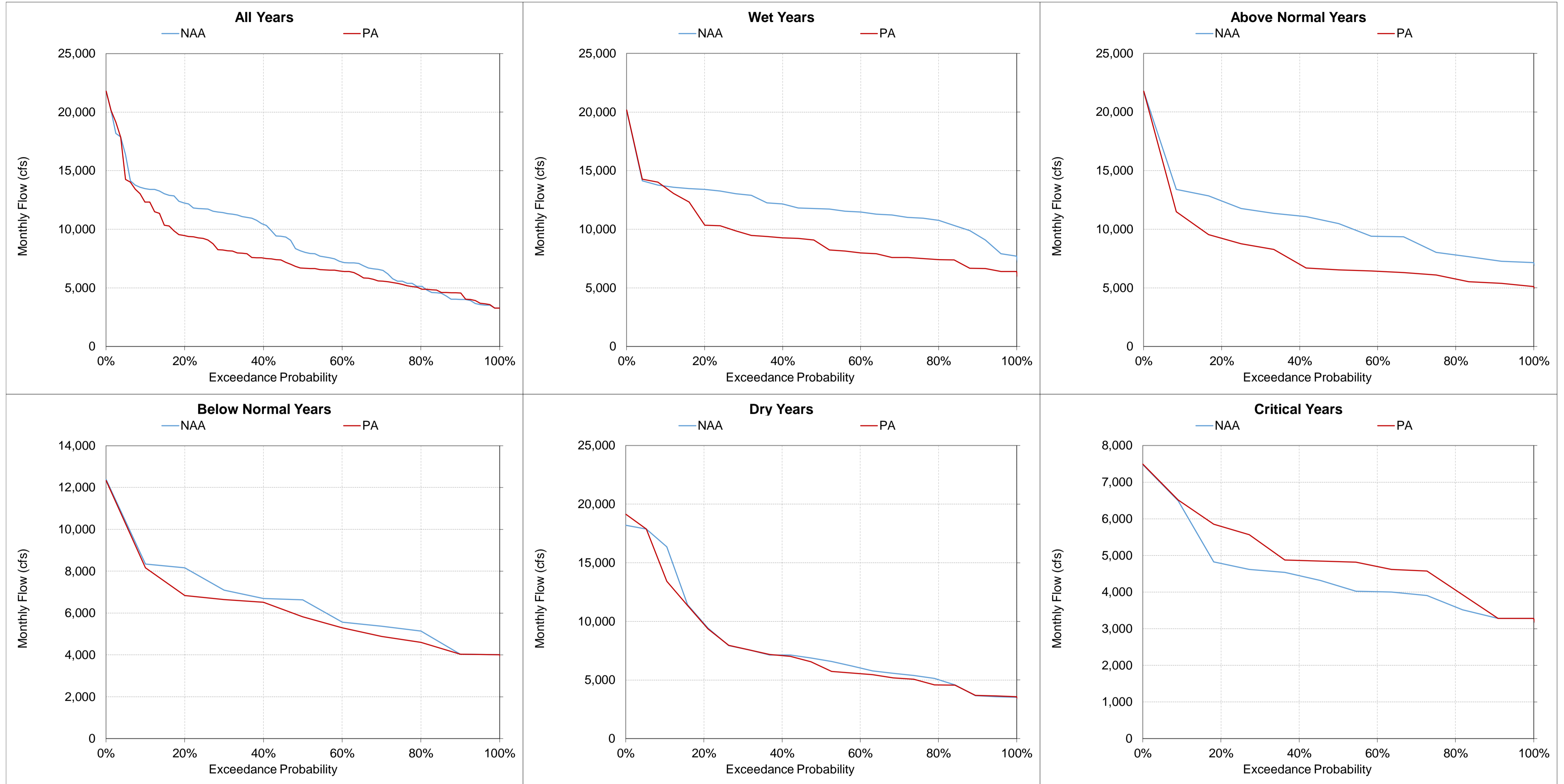
Figure 5.A.6-36-9. Sacramento River at Wilkins Slough, Monthly Flow November
