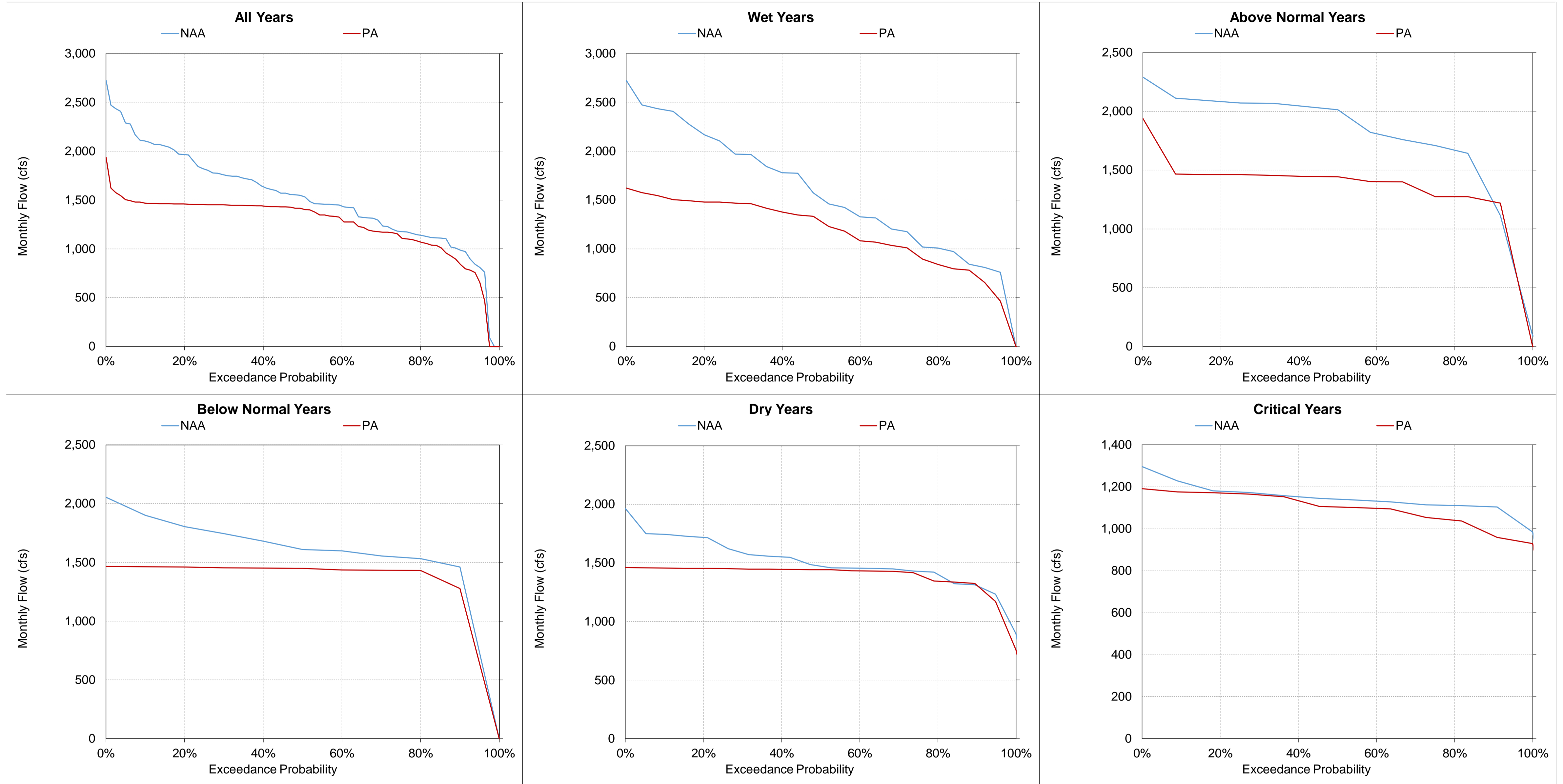
Figure 5.A.6-32-8. Delta Cross Channel, Monthly Flow October
