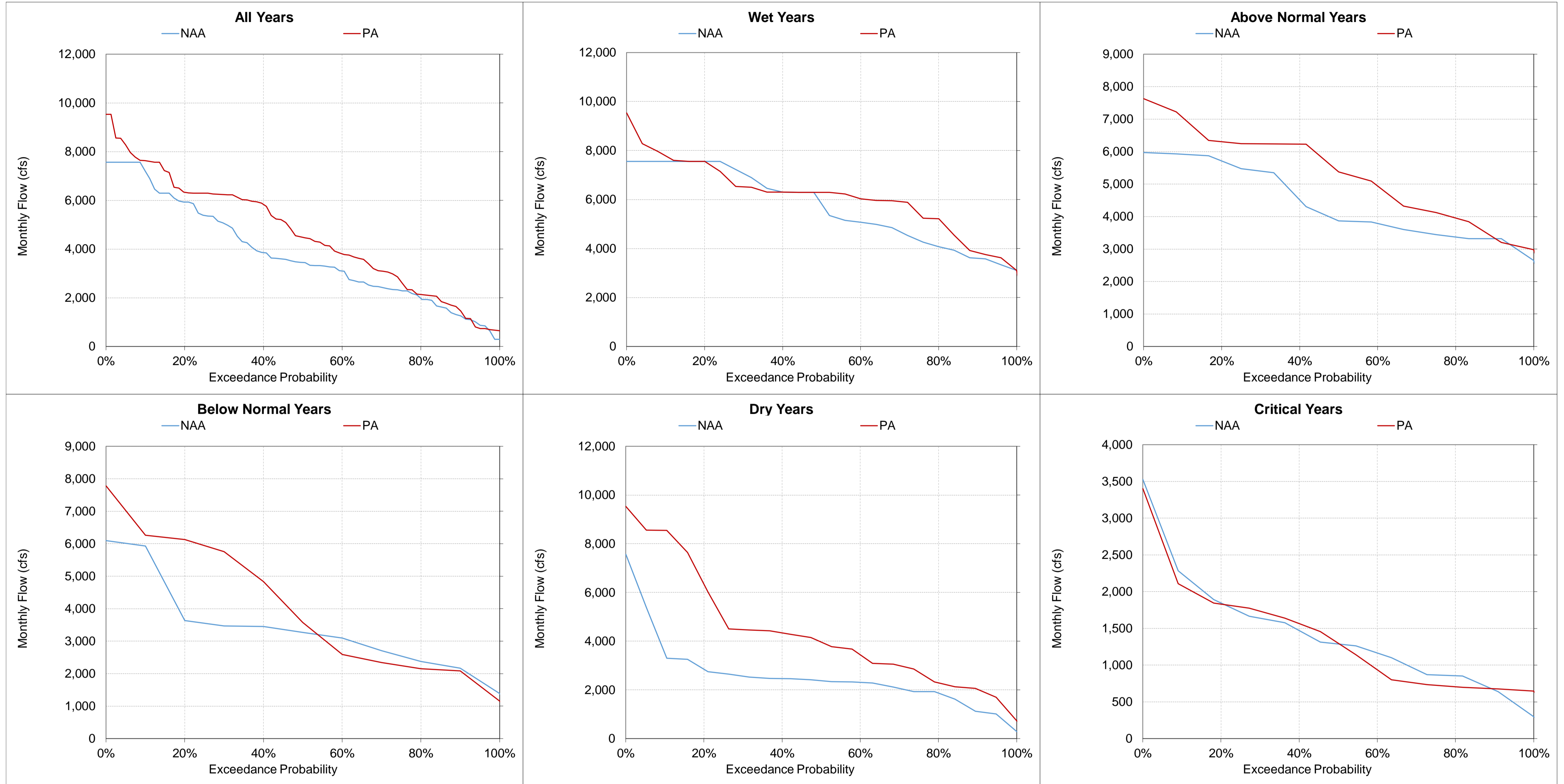
Figure 5.A.6-34-13. Total Banks Pumping Plant Exports, Monthly Flow March
