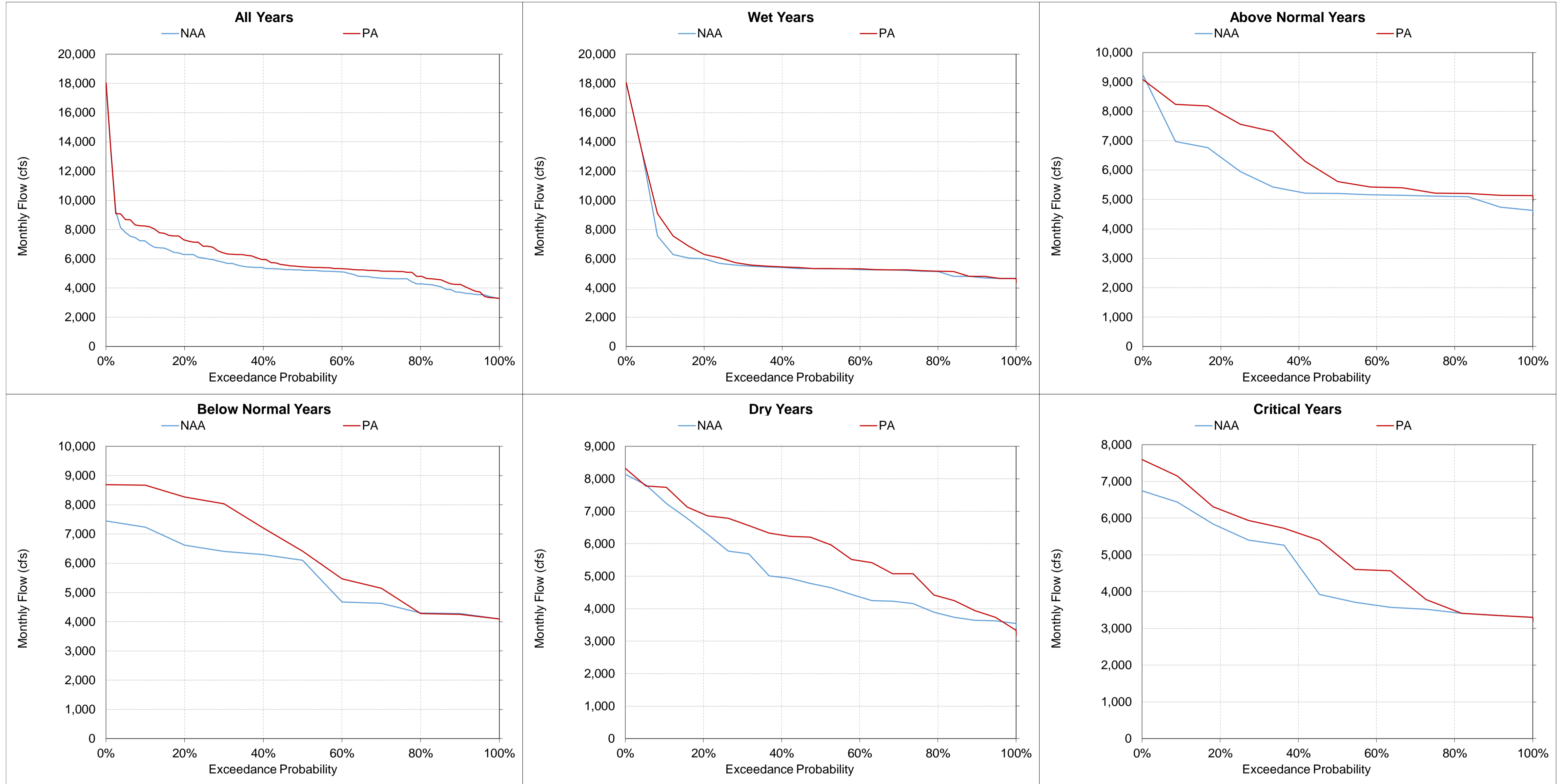
Figure 5.A.6-36-16. Sacramento River at Wilkins Slough, Monthly Flow June
