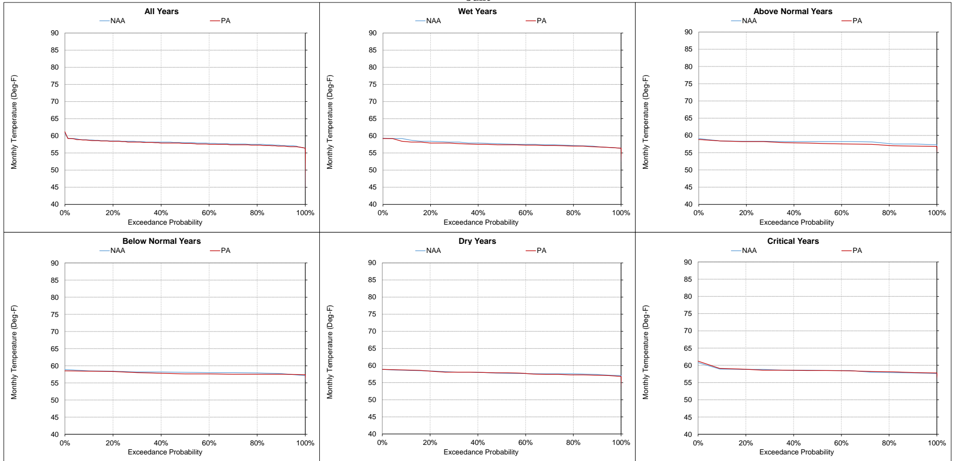
Figure 5.C.7-11-16. Feather River Low Flow Channel near Fish Dam, Monthly Temperature June
