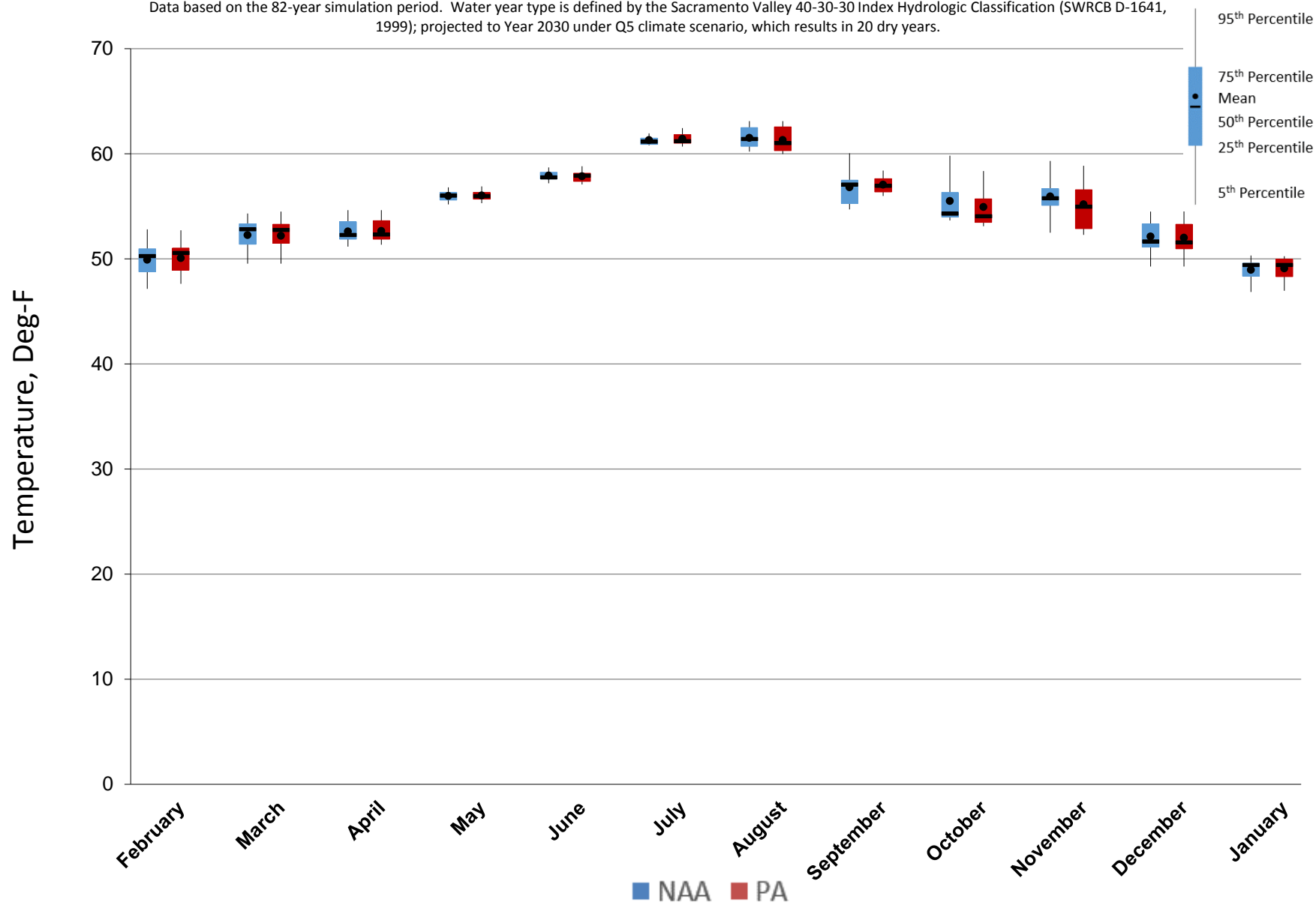
Figure 5.C.7-11-5. Monthly Temperature Ranges for Feather River Low Flow Channel near Fish Dam, Dry Years
