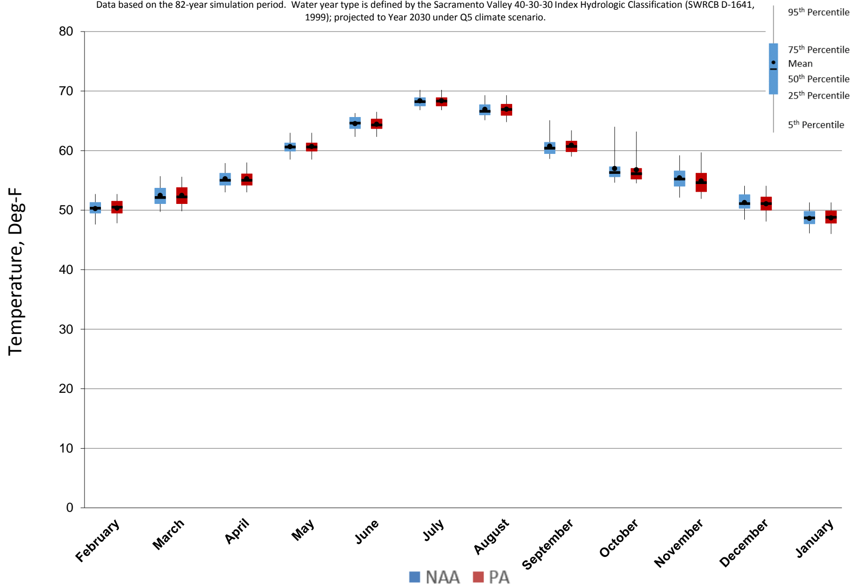
Figure 5.C.7-12-1. Monthly Temperature Ranges for Feather River Low Flow Channel at Robinson Riffle, All Years
