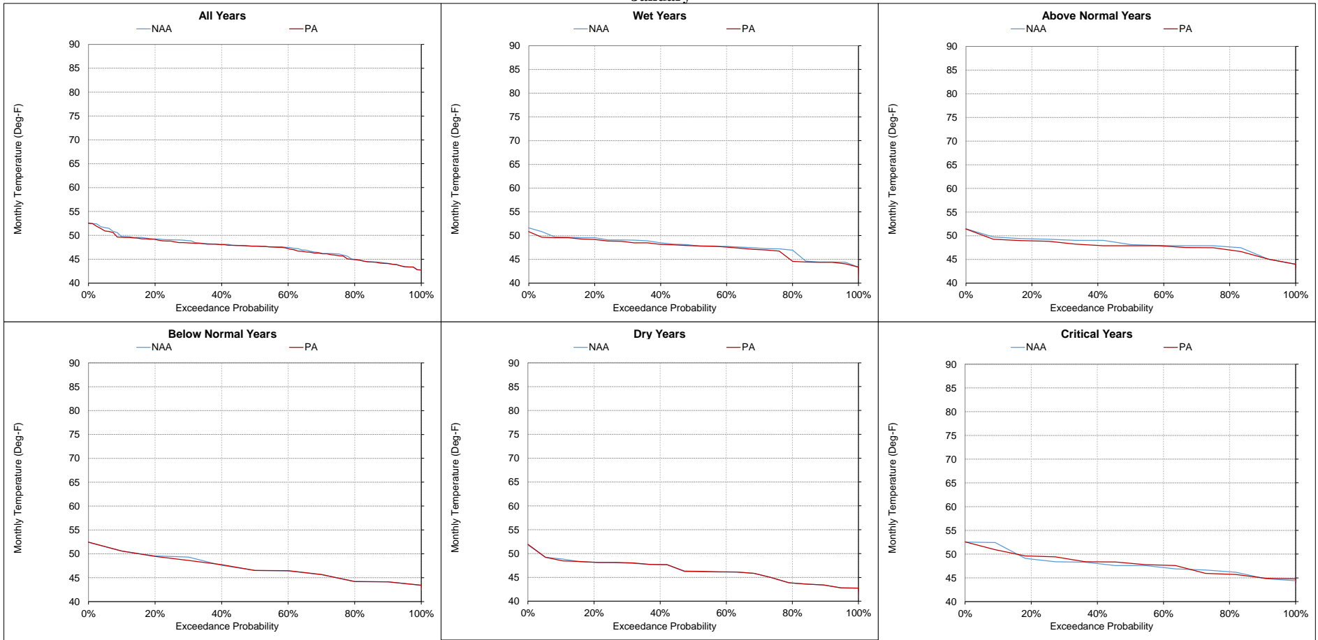
Figure 5.C.7-1-11. Trinity River below Lewiston Dam, Monthly Temperature
