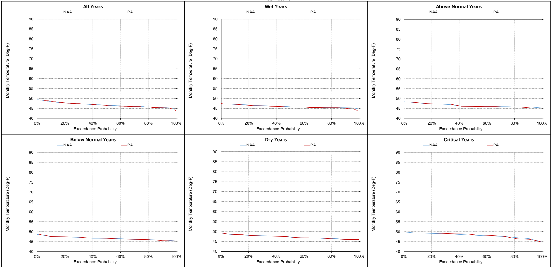
Figure 5.C.7-14-12. American River at Hazel Ave, Monthly Temperature February
