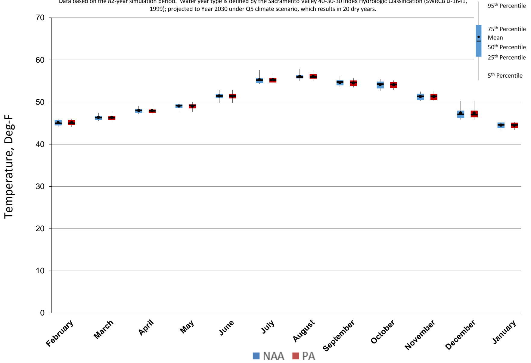
Figure 5.C.7-2-5. Monthly Temperature Ranges for Clear Creek at Igo, Dry Years
