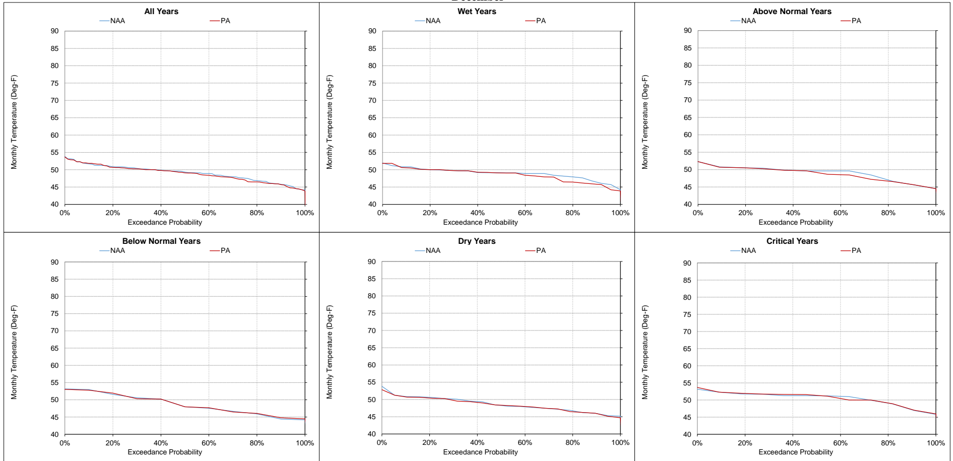
Figure 5.C.7-1-10. Trinity River below Lewiston Dam, Monthly Temperature December
