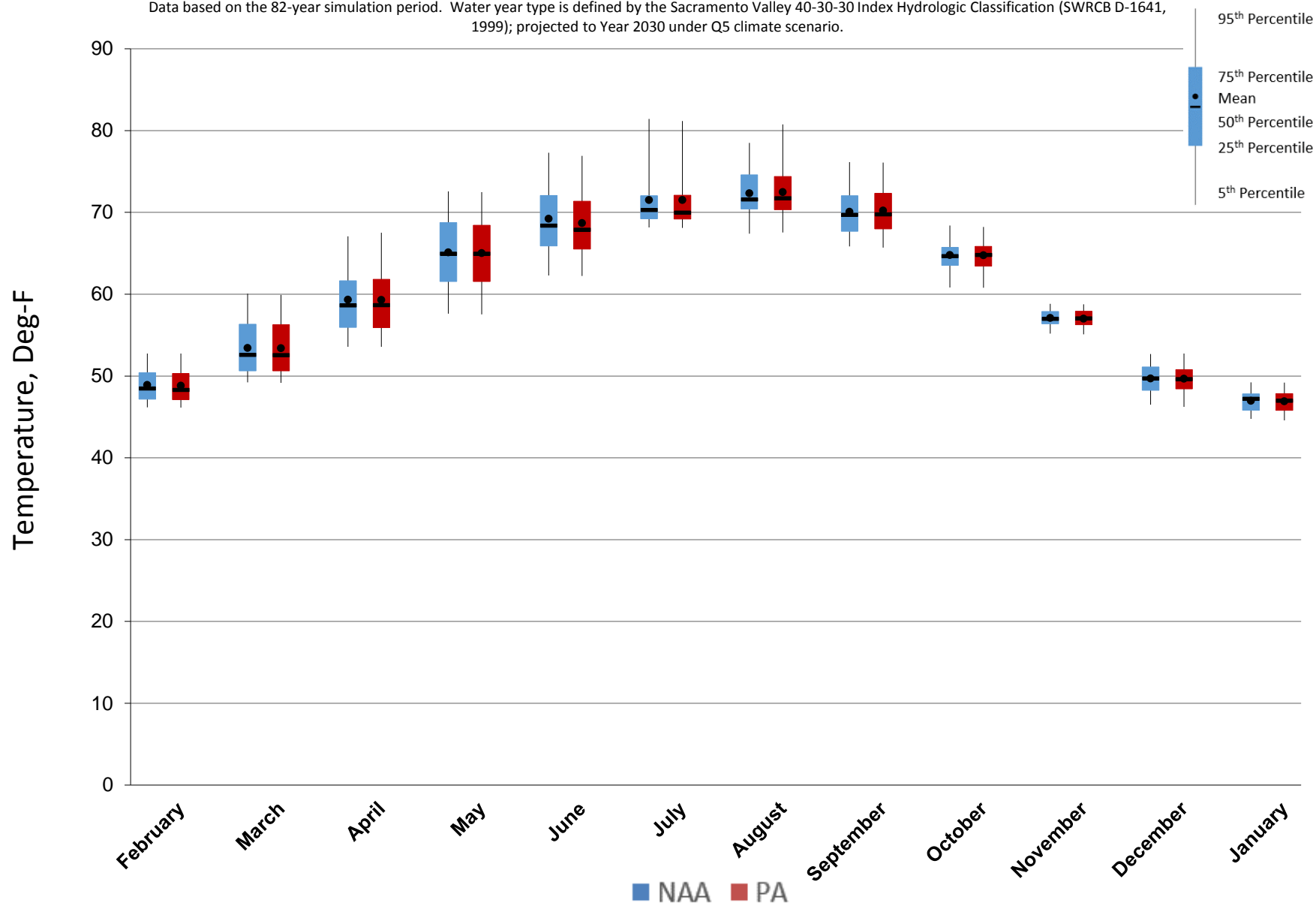
Figure 5.C.7-16-1. Monthly Temperature Ranges for American River at Sacramento River Confluence, All Years
