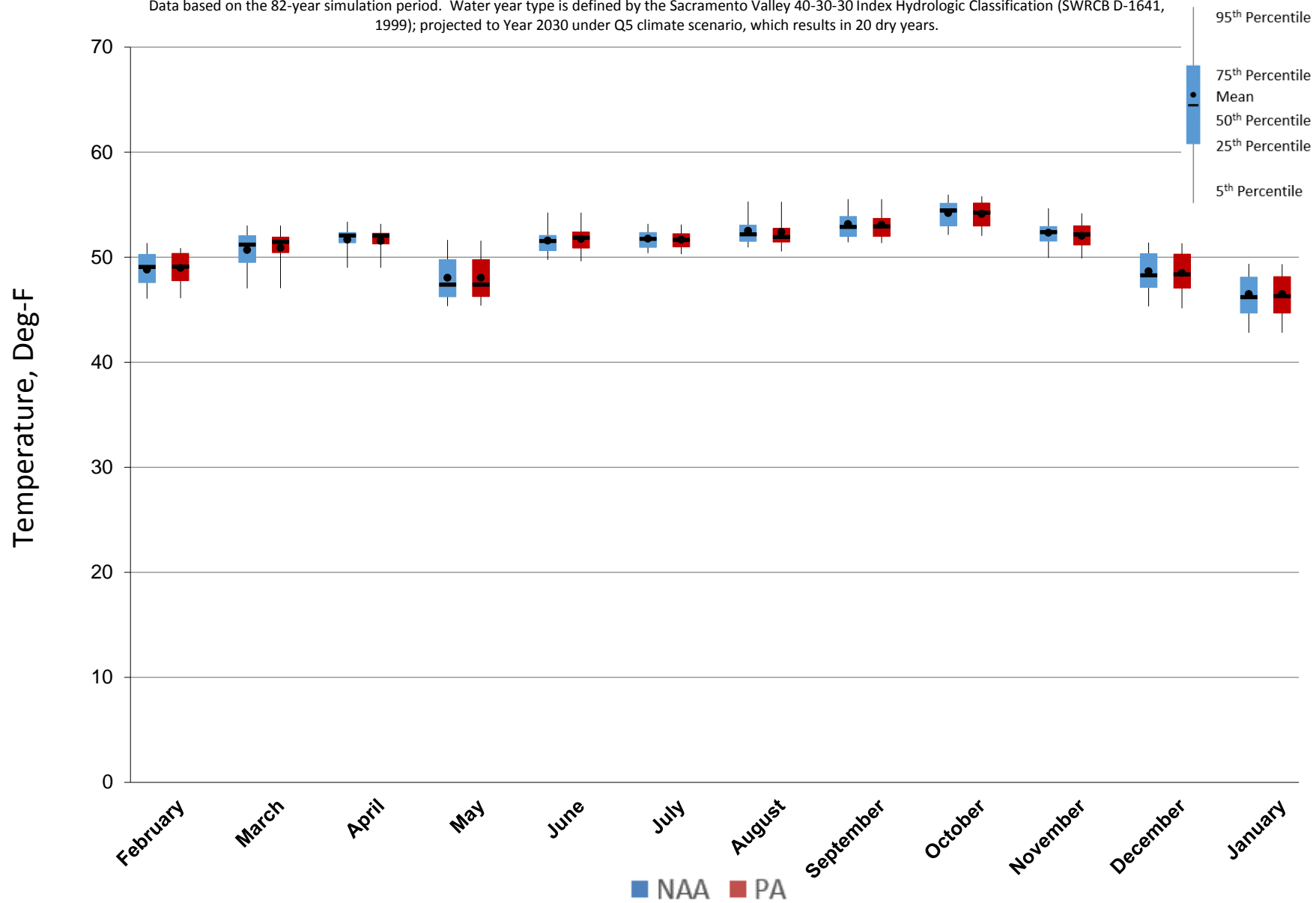
Figure 5.C.7-1-5. Monthly Temperature Ranges for Trinity River below Lewiston Dam, Dry Years
