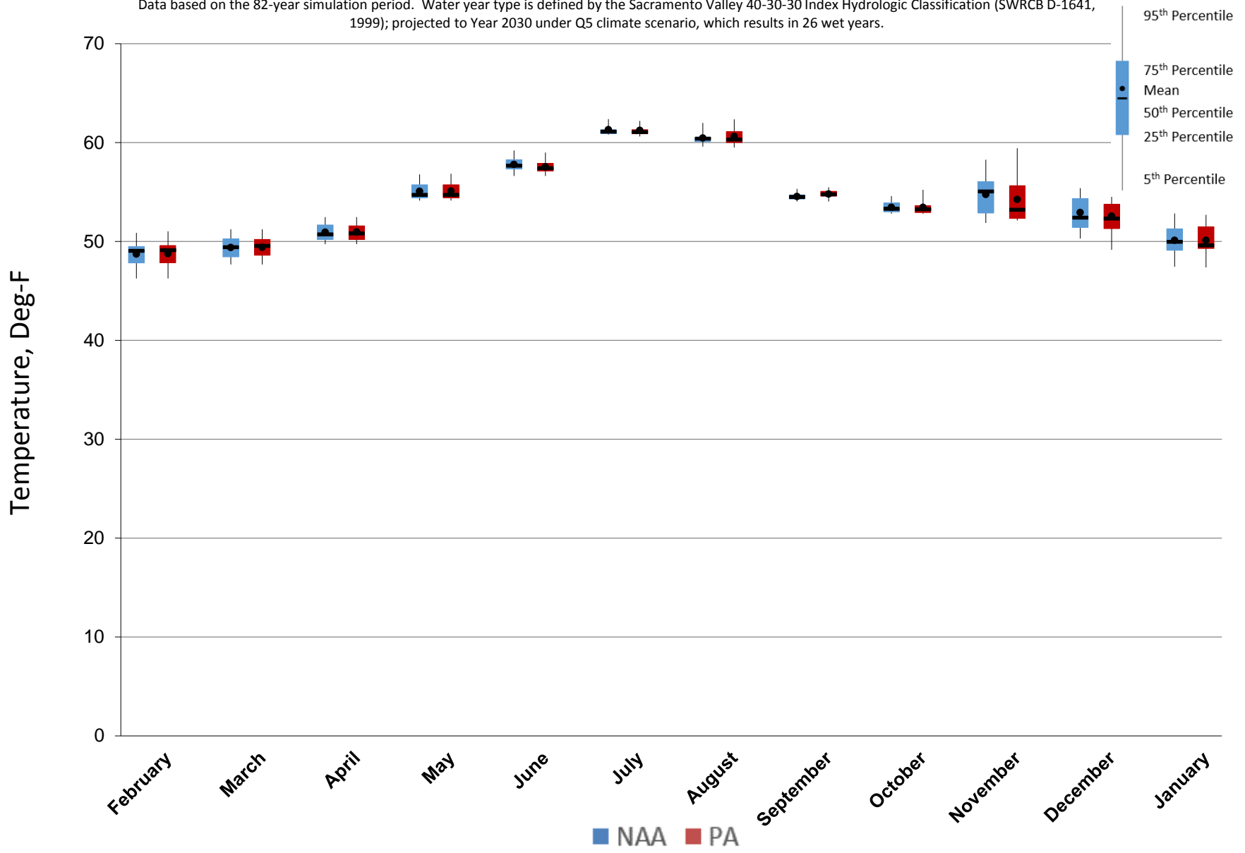
Figure 5.C.7-11-2. Monthly Temperature Ranges for Feather River Low Flow Channel near Fish Dam, Wet Years
