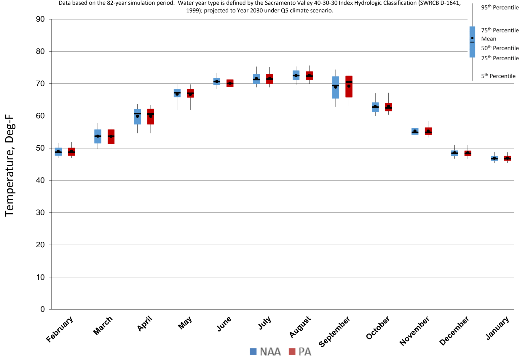
Figure 5.C.7-10-1. Monthly Temperature Ranges for Sacramento River at Knights Landing, All Years
