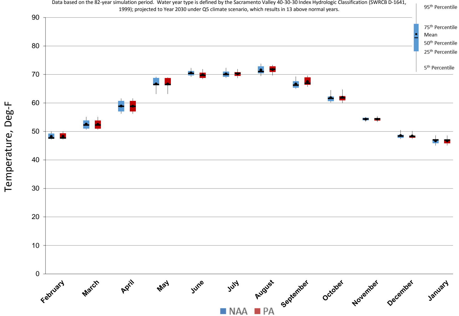
Figure 5.C.7-10-3. Monthly Temperature Ranges for Sacramento River at Knights Landing, Above Normal Years
