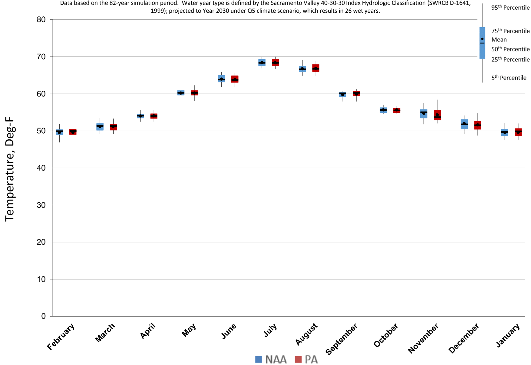
Figure 5.C.7-12-2. Monthly Temperature Ranges for Feather River Low Flow Channel at Robinson Riffle, Wet Years
