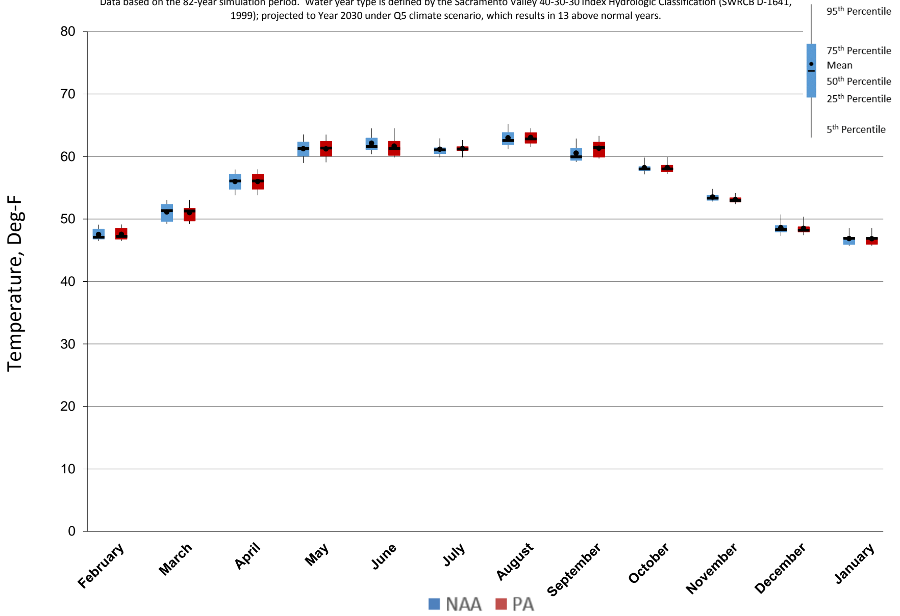
Figure 5.C.7-9-3. Monthly Temperature Ranges for Sacramento River at Hamilton City, Above Normal Years
