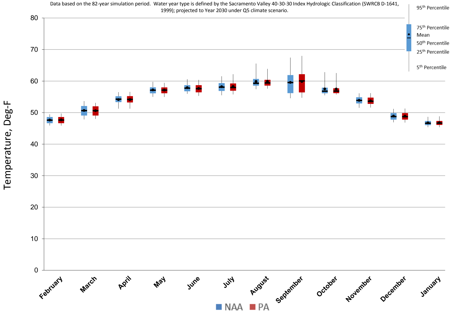
Figure 5.C.7-8-1. Monthly Temperature Ranges for Sacramento River at Red Bluff Diversion Dam, All Years
